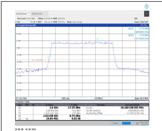
1-N38--30-20-H-9-CP-256QAM-Outer_Full-51@0-An t0-18.26-19.840-≤20-PASS
