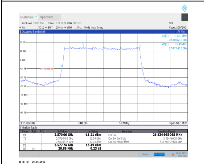
1-N38--30-30-L-2-DFT-PI2BPSK-Outer_Full-75@0-A nt0-26.835-28.860-≤30-PASS
