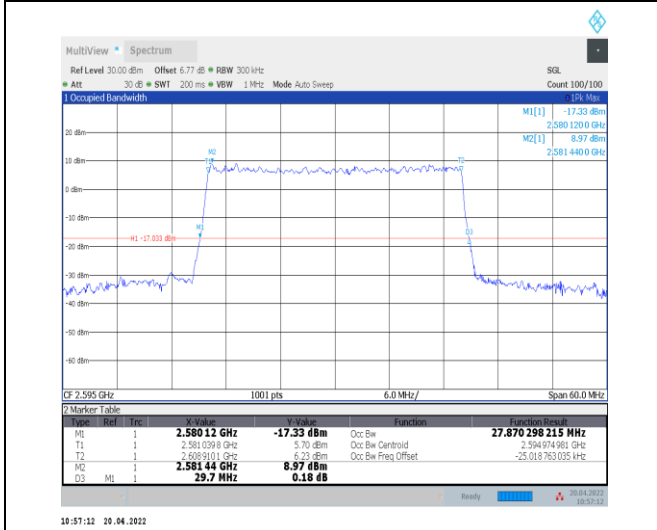
1-N38--30-30-M-9-CP-256QAM-Outer_Full-78@0-Ant t0-27.87-29.700-≤30-PASS
