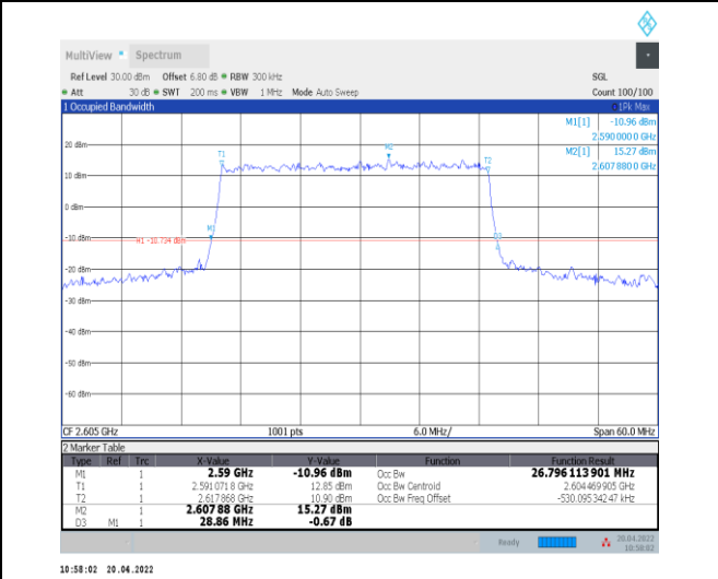
1-N38--30-30-H-1-DFT-QPSK-Outer_Full-75@0-Ant 0-26.796-28.860-≤30-PASS
