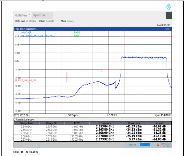
1-N38--30-15-L-3-DFT-PI2BPSK-Outer_Full-36@0-Ant0-PASS-see graph
