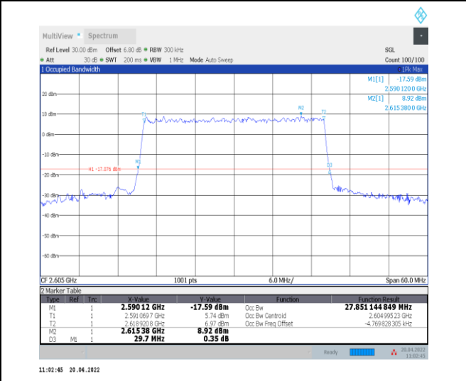
1-N38--30-30-H-9-CP-256QAM-Outer_Full-78@0-Ant0-27.851-29.700-≤30-PASS
