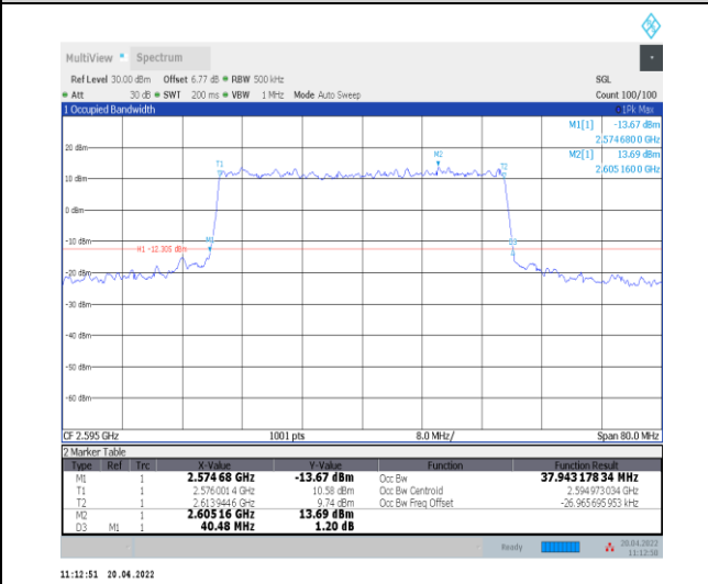
1-N38--30-40-M-7-CP-16QAM-Outer_Full-106@0-A nt0-37.943-40.480-≤40-PASS
