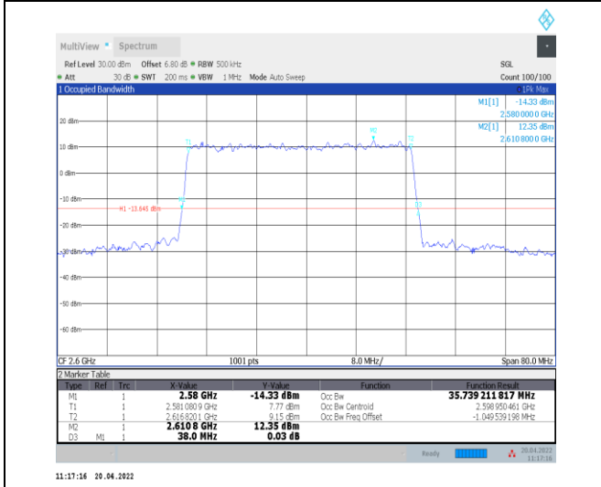
1-N38--30-40-H-5-DFT-256QAM-Outer_Full-100@0-A Ant0-35.739-38.000≤40-PASS
