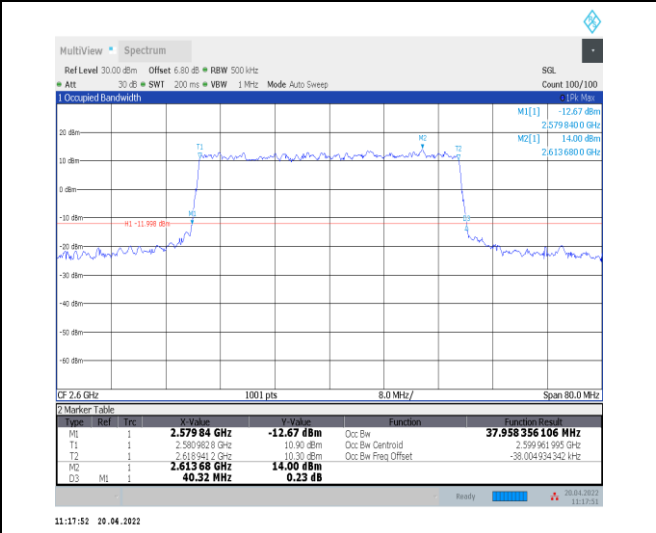
1-N38--30-40-H-6-CP-QPSK-Outer_Full-106@0-Ant 0-37.958-40.320≤40-PASS
