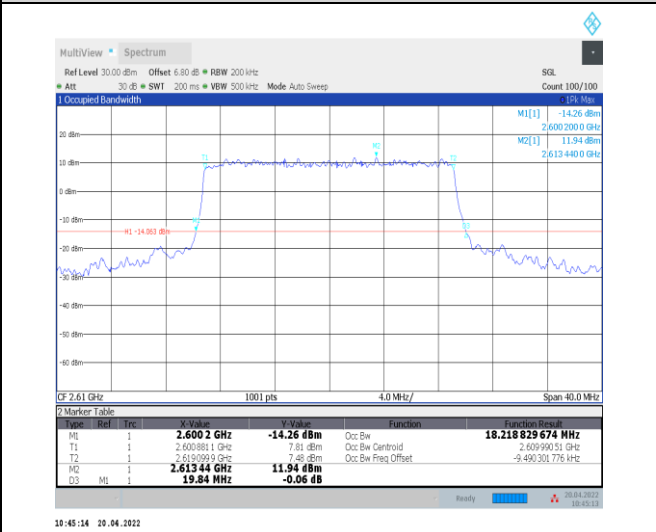
1-N38--30-20-H-8-CP-64QAM-Outer_Full-51@0-Ant 0-18.219-19.840-≤20-PASS
