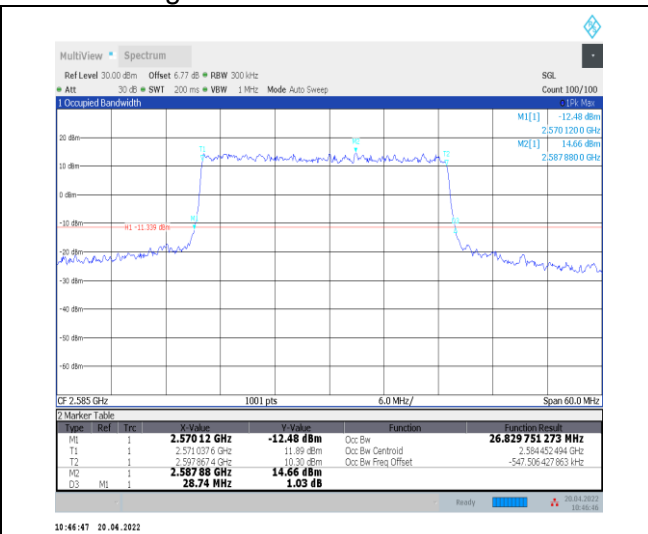
1-N38--30-30-L-1-DFT-QPSK-Outer_Full-75@0-Ant0 -26.83-28.740-≤30-PASS
