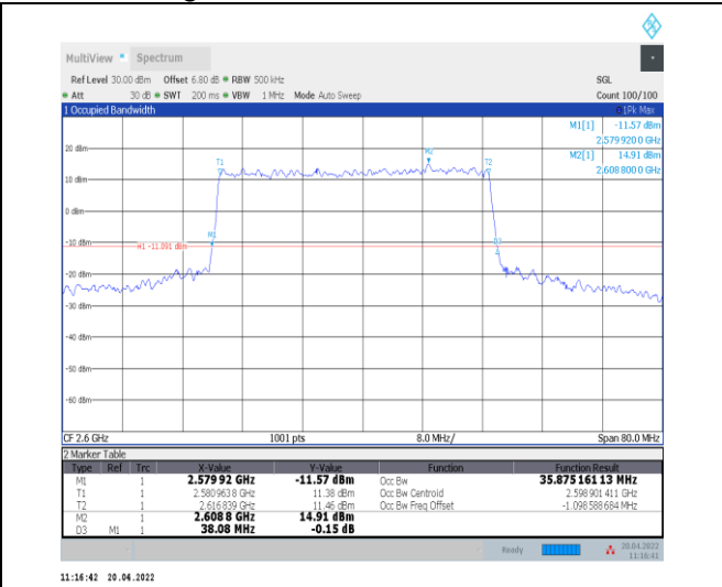
1-N38--30-40-H-4-DFT-64QAM-Outer_Full-100@0-A nt0-35.875-38.080≤40-PASS
