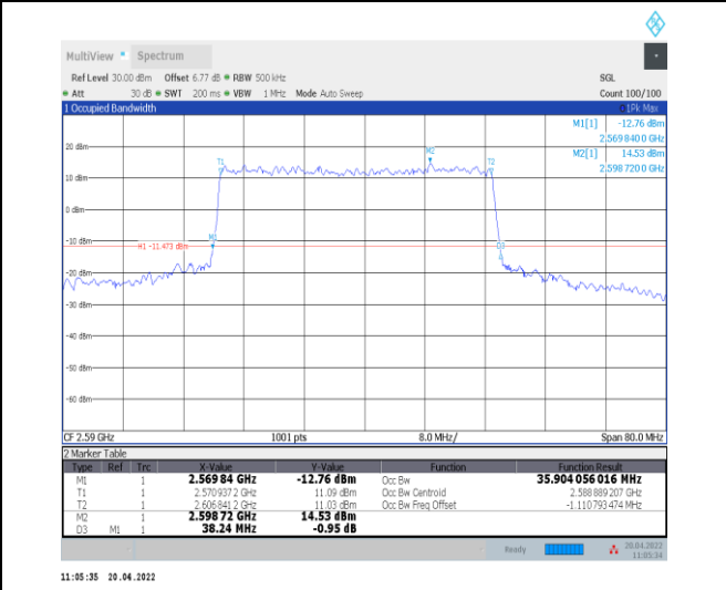
1-N38--30-40-L-4-DFT-64QAM-Outer_Full-100@0-Ant0-35.904-38.240-≤40-PASS
