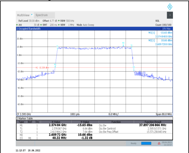
1-N38--30-40-M-9-CP-256QAM-Outer_Full-106@0-Ant0-37.897-40.320-≤40-PASS
