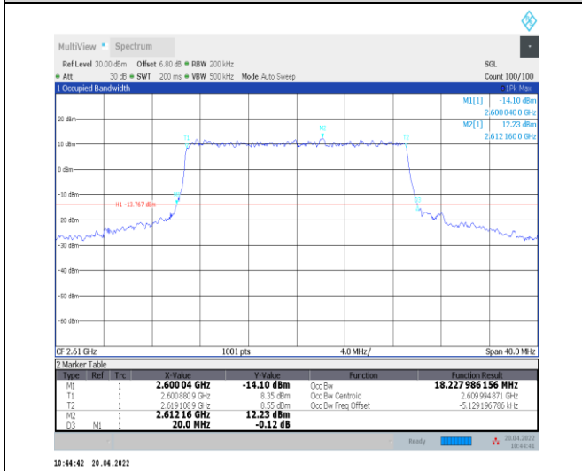
1-N38--30-20-H-7-CP-16QAM-Outer_Full-51@0-Ant 0-18.228-20.000-≤20-PASS
