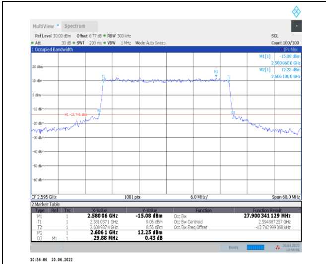
1-N38--30-30-M-7-CP-16QAM-Outer_Full-78@0-Ant 0-27.9-29.880-≤30-PASS
