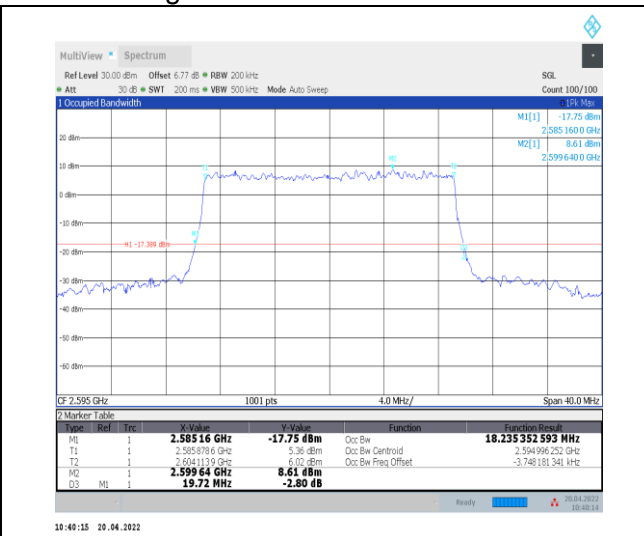
1-N38--30-20-M-7-CP-16QAM-Outer_Full-51@0-Ant-0-18.206-19.960-≤20-PASS
