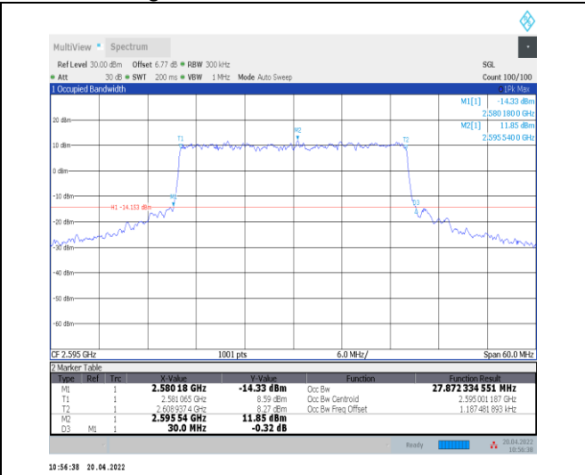
1-N38--30-30-M-8-CP-64QAM-Outer_Full-78@0-Ant 0-27.872-30.000-≤30-PASS
