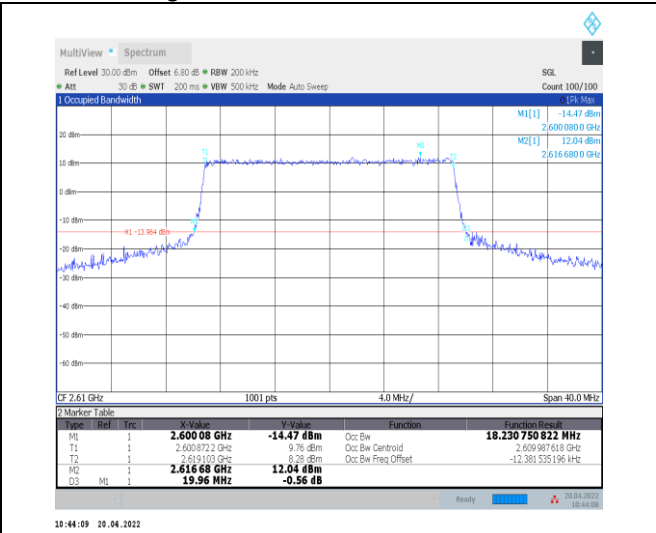
1-N38--30-20-H-6-CP-QPSK-Outer_Full-51@0-Ant0- 18.231-19.960-≤20-PASS
