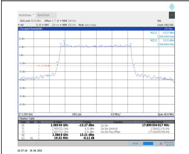
1-N38--30-20-M-4-DFT-64QAM-Outer_Full-50@0-Ant0-17.9-19.520-<=20-PASS
