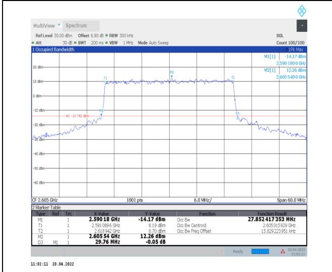
1-N38--30-30-H-8-CP-64QAM-Outer_Full-78@0-Ant0-27.852-29.760-≤30-PASS
