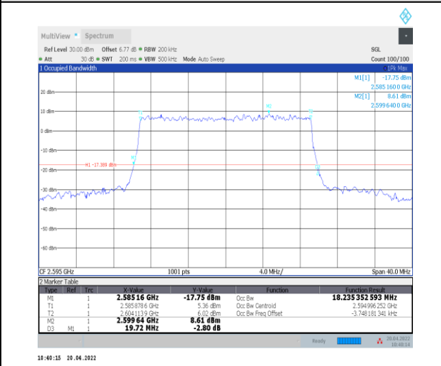
1-N38--30-20-M-9-CP-256QAM-Outer_Full-51@0-A-nt-0-18.235-19.720-≤20-PASS
