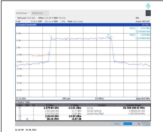
1-N38--30-40-H-3-DFT-16QAM-Outer_Full-100@0-A nt0-35.769-38.160≤40-PASS
