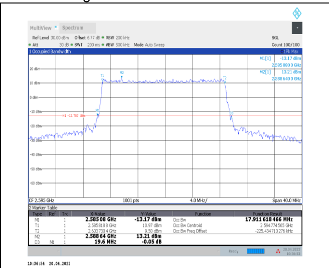
1-N38--30-20-M-3-DFT-16QAM-Outer_Full-50@0-Ant0-17.912-19.600-<=20-PASS
