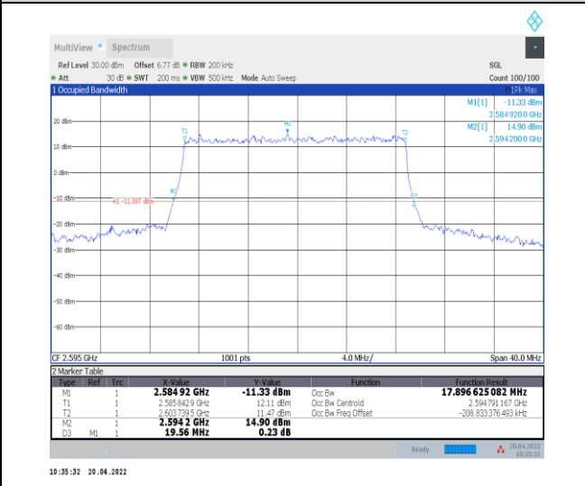
1-N38--30-20-M-1-DFT-QPSK-Outer_Full-50@0-Ant0 0-17.897-19.560-≤20-PASS
