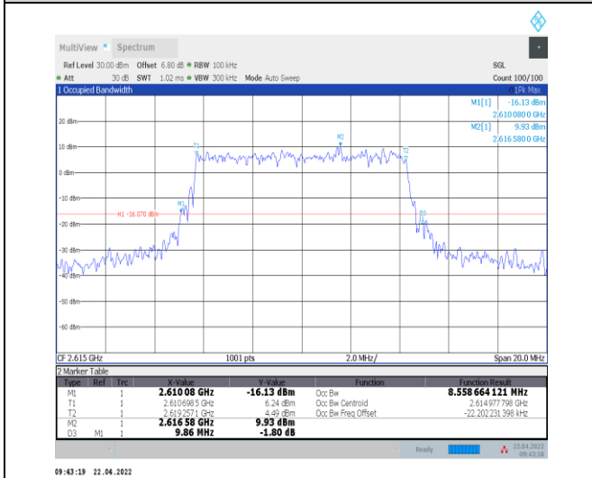
1-N38--30-10-H-5-DFT-256QAM-Outer_Full-24@0-A nt0-8.559-9.860-≤10-PASS
