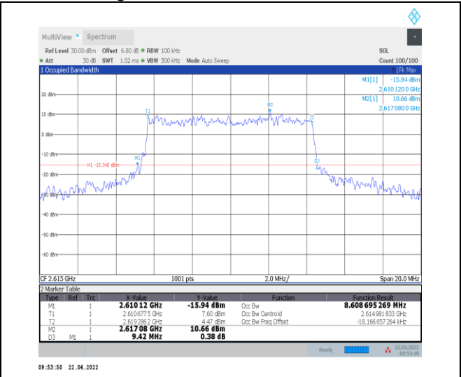
1-N38--30-10-H-8-CP-64QAM-Outer_Full-24@0-Ant 0-8.609-9.420-≤10-PASS
