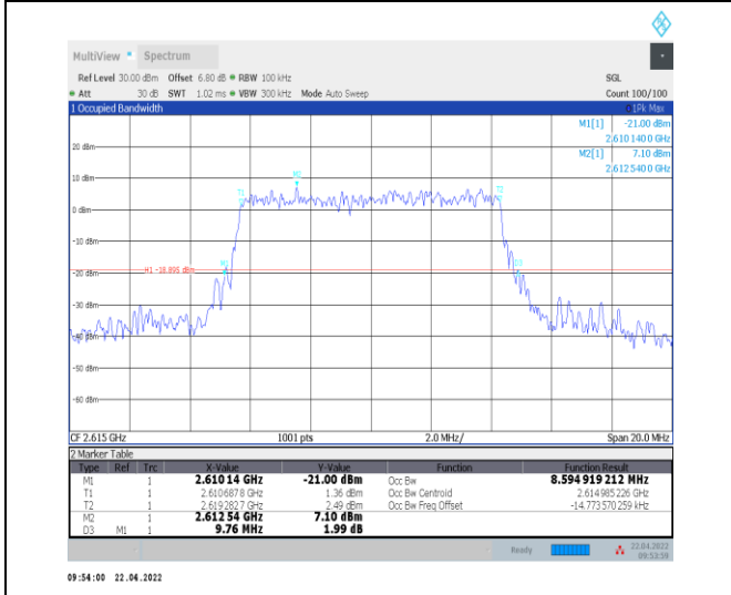
1-N38--30-10-H-9-CP-256QAM-Outer_Full-24@0-Ant t0-8.595-9.760-≤10-PASS
