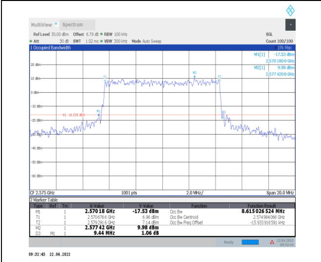
1-N38--30-10-L-7-CP-16QAM-Outer_Full-24@0-Ant0 -8.615-9.440-≤10-PASS
