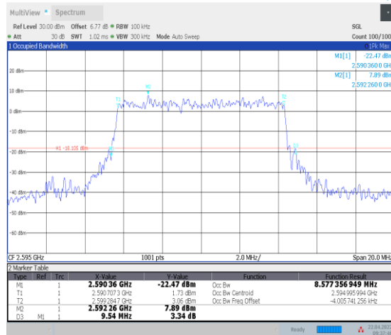
1-N38--30-10-M-9-CP-256QAM-Outer_Full-24@0-Ant 0-8.577-9.540-≤10-PASS
