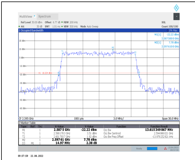
1-N38--30-15-M-9-CP-256QAM-Outer_Full-38@0-An t0-13.615-14.970-≤15-PASS
