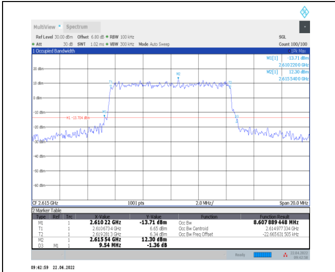
1-N38--30-10-H-3-DFT-16QAM-Outer_Full-24@0-An t0-8.608-9.540-≤10-PASS
