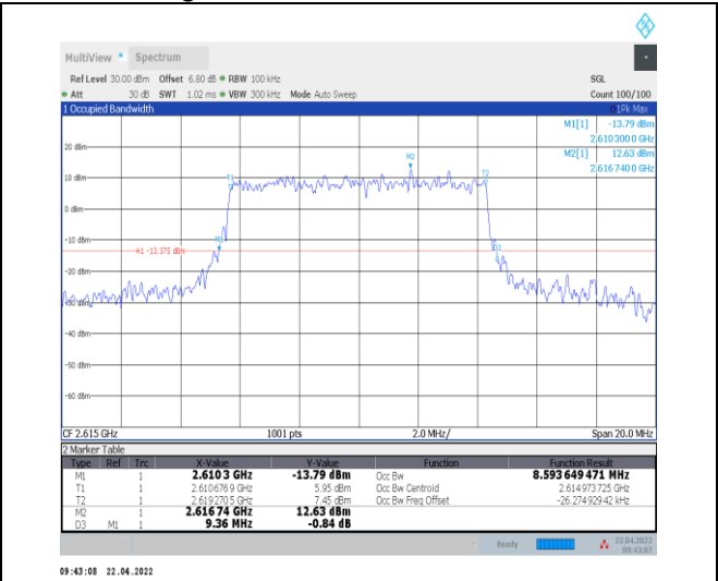
1-N38--30-10-H-4-DFT-64QAM-Outer_Full-24@0-An t0-8.594-9.360-≤10-PASS
