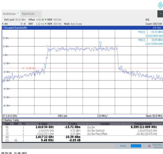
1-N38--30-10-H-1-DFT-QPSK-Outer_Full-24@0-Ant 0-8.599-9.480-≤10-PASS
