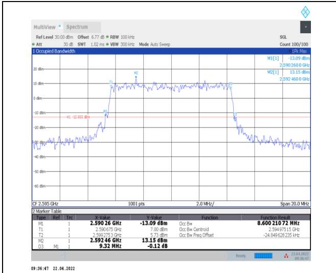
1-N38--30-10-M-4-DFT-64QAM-Outer_Full-24@0-Ant t0-8.6-9.320-<=10-PASS
