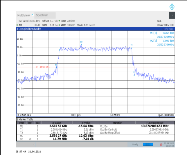
1-N38--30-15-M-8-CP-64QAM-Outer_Full-38@0-Ant 0-13.675-14.790-≤15-PASS
