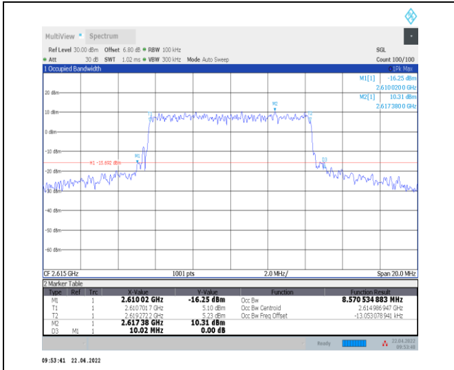
1-N38--30-10-H-7-CP-16QAM-Outer_Full-24@0-Ant 0-8.571-10.020-≤10-PASS
