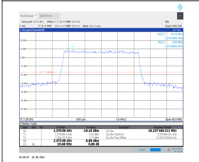
1-N38--30-20-L-9-CP-256QAM-Outer_Full-51@0-Ant0 0-18.237-19.680-≤20-PASS
