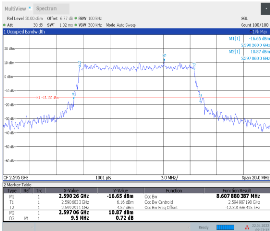
1-N38--30-10-M-8-CP-64QAM-Outer_Full-24@0-Ant 0-8.608-9.500-≤10-PASS
