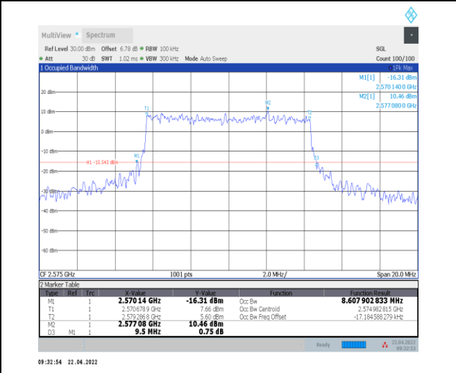
1-N38--30-10-L-8-CP-64QAM-Outer_Full-24@0-Ant 0-8.608-9.500-≤10-PASS
