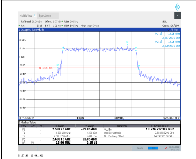
1-N38--30-15-M-7-CP-16QAM-Outer_Full-38@0-Ant 0-13.575-15.060-≤15-PASS
