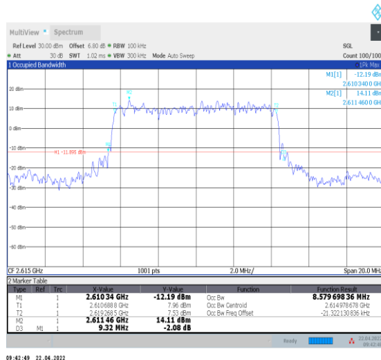
1-N38--30-10-H-2-DFT-PI2BPSK-Outer_Full-24@0-Ant 0-8.58-9.320-≤10-PASS
