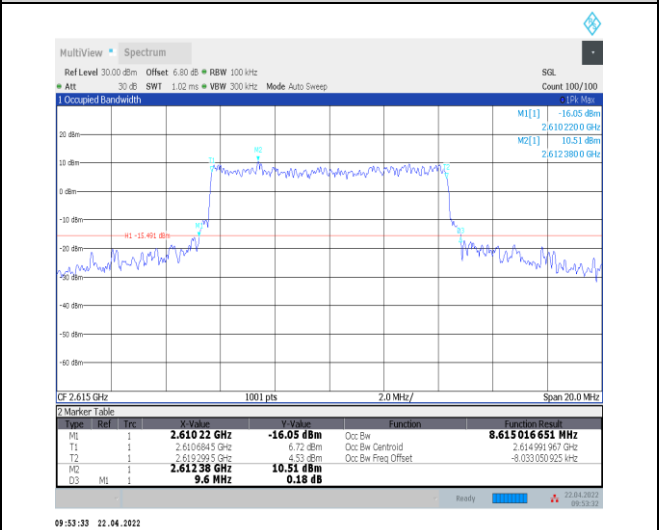
1-N38--30-10-H-6-CP-QPSK-Outer_Full-24@0-Ant0- 8.615-9.600-≤10-PASS
