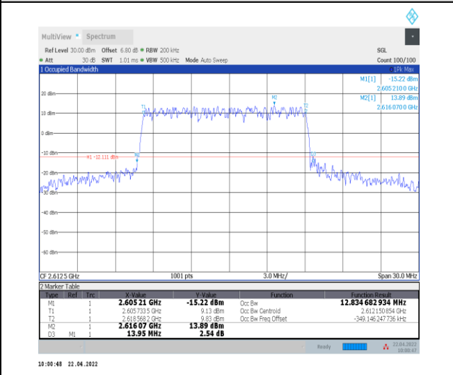
1-N38--30-15-H-3-DFT-16QAM-Outer_Full-36@0-An t0-12.835-13.950-≤15-PASS
