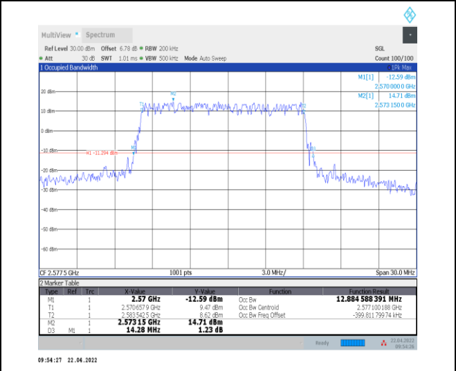
1-N38--30-15-L-1-DFT-QPSK-Outer_Full-36@0-Ant0 -12.885-14.280-≤15-PASS
