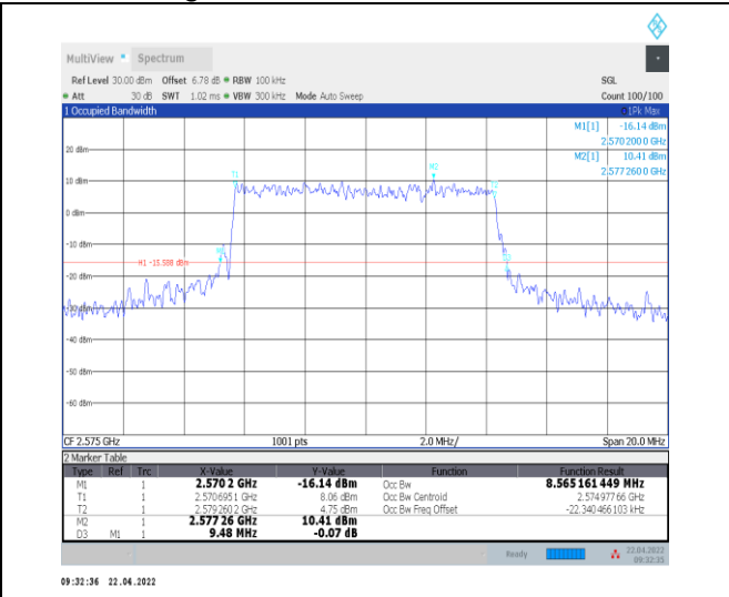
1-N38--30-10-L-6-CP-QPSK-Outer_Full-24@0-Ant0 8.565-9.480-≤10-PASS
