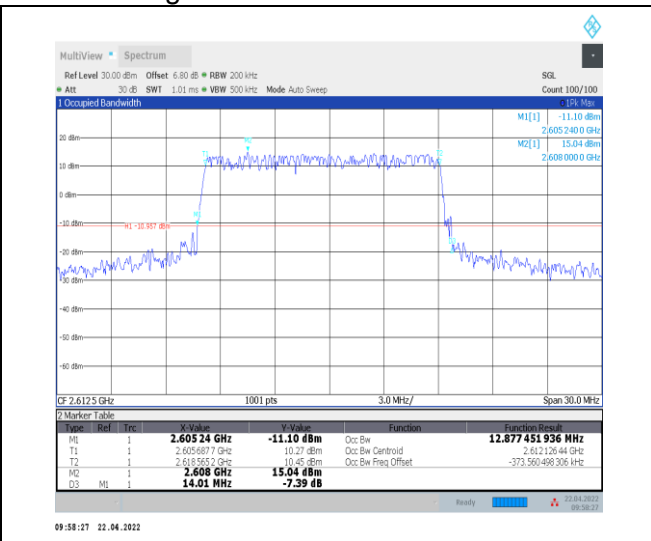
1-N38--30-15-H-1-DFT-QPSK-Outer_Full-36@0-Ant 0-12.877-14.010-≤15-PASS
