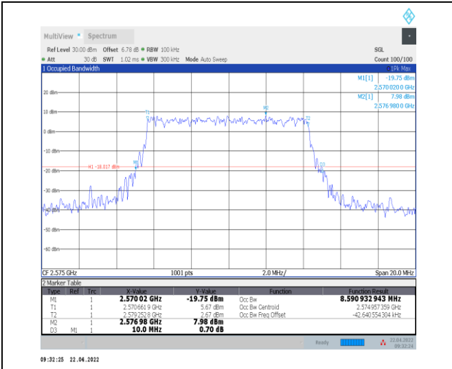
1-N38--30-10-L-5-DFT-256QAM-Outer_Full-24@0-A nt0-8.591-10.000-≤10-PASS
