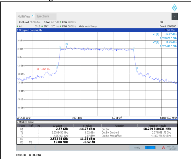
1-N38--30-20-L-8-CP-64QAM-Outer_Full-51@0-Ant0 0-18.23-19.880-≤20-PASS
