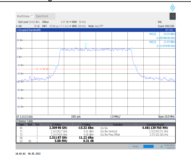
1-N30--15-5-H-4-DFT-64QAM-Outer_Full-25@0-Ant 0-4.481-5.080-≤5-PASS
