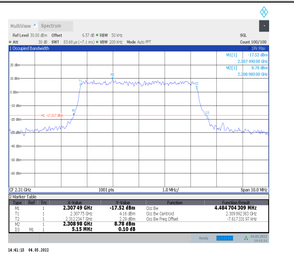
1-N30--15-5-M-7-CP-16QAM-Outer_Full-25@0-Ant0 -4.485-5.150-<math>\leq</math>5-PASS
