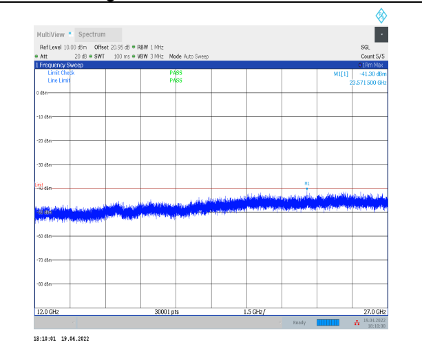
1-N30--15-10-H-1-DFT-PI2BPSK-Inner_1RB_Left-1 @1-12000-27000-Ant0--41.30--40-PASS
