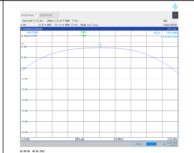
1-N30-PC3-15-10-L-3-DFT-PI2BPSK-Outter_Full-50 @0-2300-2320-Ant0-18.82-23.98-PASS
