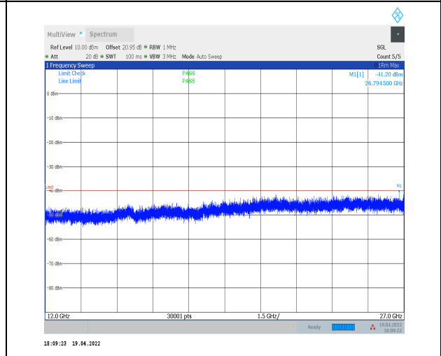
1-N30--15-10-M-1-DFT-PI2BPSK-Inner_1RB_Left-1 @1-12000-27000-Ant0--41.20--40-PASS
