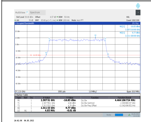
1-N30--15-5-M-6-CP-QPSK-Outer_Full-25@0-Ant0 4.464-4.930-<math>\leq</math>5-PASS
