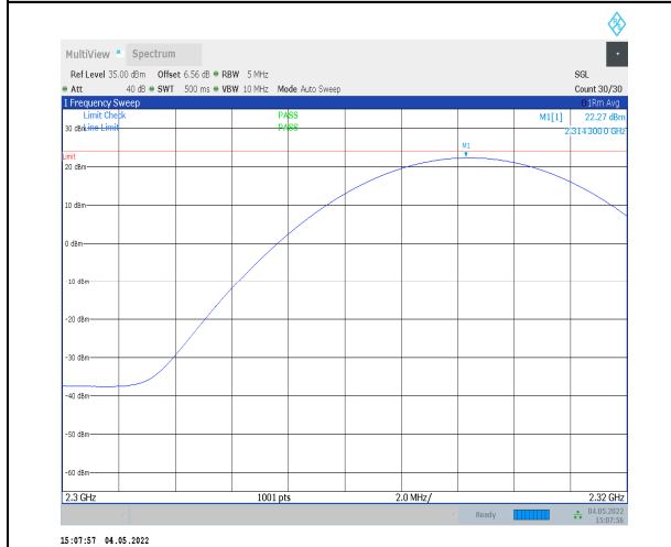
1-N30-PC3-15-10-L-2-DFT-PI2BPSK-Inner_1RB_Ri ght-1@50-2300-2320-Ant0-22.27-23.98-PASS
