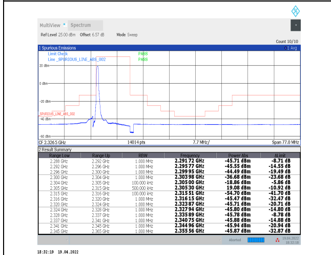
1-N30--30-10-L-4-CP-QPSK-Edge_1RB_Left-1@0-Ant0-PASS-see graph
