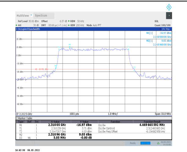
1-N30--15-5-H-6-CP-QPSK-Outer_Full-25@0-Ant0-4 .47-5.050-≤5-PASS
