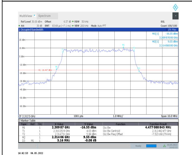
1-N30--15-5-H-5-DFT-256QAM-Outer_Full-25@0-Ant t0-4.477-5.160-≤5-PASS
