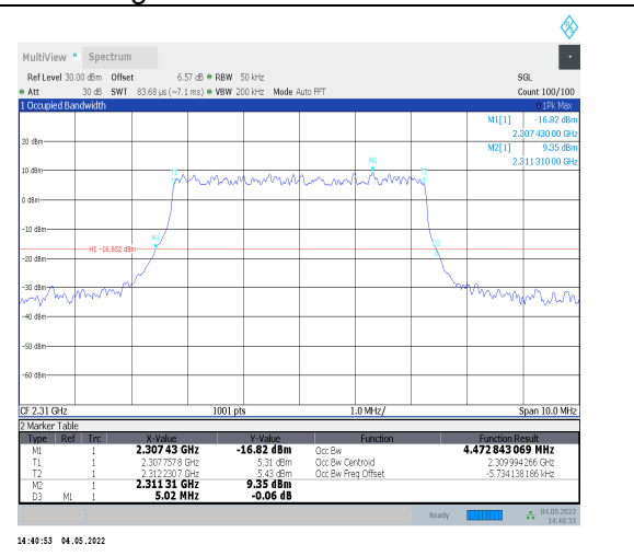
1-N30--15-5-M-5-DFT-256QAM-Outer_Full-25@0-Ant 0-4.473-5.020-<math>\leq</math>5-PASS
