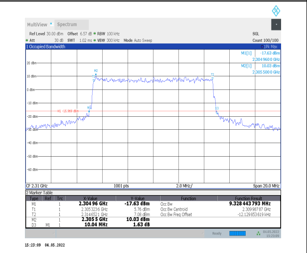
1-N30--15-10-H-7-CP-16QAM-Outer_Full-52@0-Ant 0-9.328-10.040-≤10-PASS
