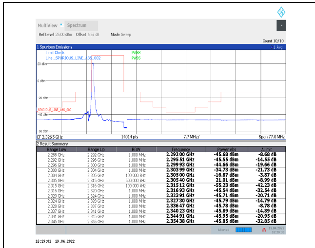
1-N30--30-10-L-1-DFT-PI2BPSK-Edge_1RB_Left-1@0-Ant0-PASS-see graph
