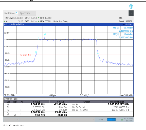
1-N30--15-10-H-1-DFT-QPSK-Outer_Full-50@0-Ant 0-8.965-9.580-<math>\leq 10</math>-PASS
