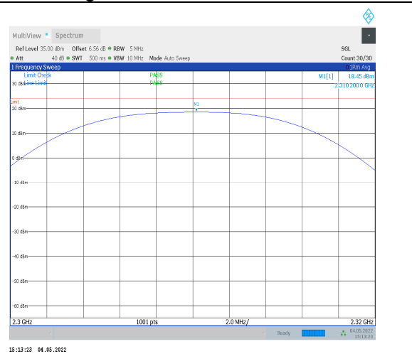
1-N30-PC3-15-10-H-3-DFT-PI2BPSK-Outer_Full-50 @0-2300-2320-Ant0-18.45-23.98-PASS
