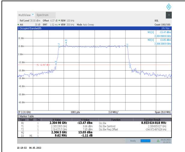
1-N30--15-10-M-1-DFT-QPSK-Outer_Full-50@0-Ant 0-8.933-9.620-<=10-PASS
