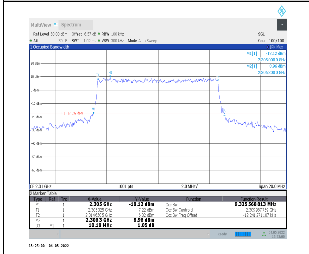
1-N30--15-10-H-6-CP-QPSK-Outer_Full-52@0-Ant0 9.326-10.180-≤10-PASS
