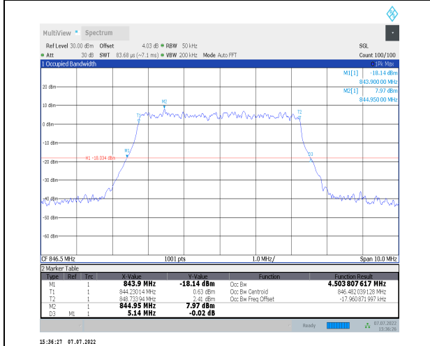
1-N26-824-849--15-5-H-9-CP-256QAM-Outer_Full-2 5@0-Ant0-4.504-5.140-<math>\leq 5</math>-PASS
