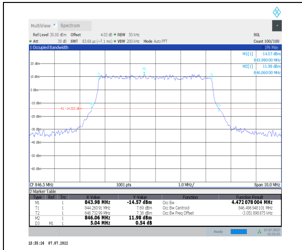
1-N26-824-849--15-5-H-3-DFT-16QAM-Outer_Full-2 5@0-Ant0-4.472-5.040-<math>\leq 5</math>-PASS
