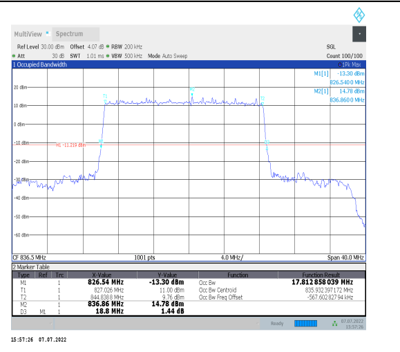
1-N26-824-849--15-20-M-2-DFT-PI2BPSK-Outer_Ful I-100@0-Ant0-17.813-18.800-<math>\leq 20</math>-PASS
