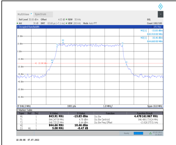
1-N26-824-849--15-5-H-7-CP-16QAM-Outer_Full-25 @0-Ant0-4.478-5.080-<math>\leq 5</math>-PASS
