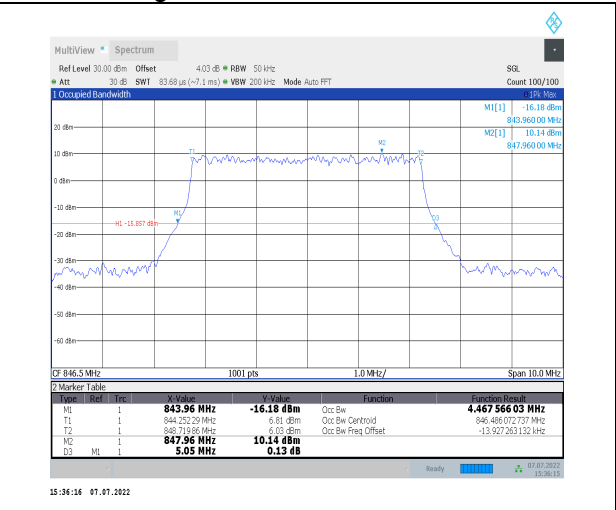
1-N26-824-849--15-5-H-8-CP-64QAM-Outer_Full-25 @0-Ant0-4.468-5.050-<math>\leq 5</math>-PASS
