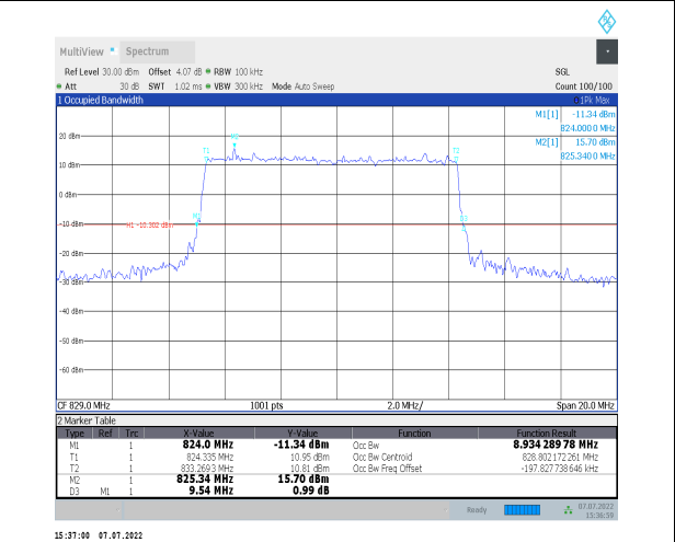
1-N26-824-849--15-10-L-1-DFT-QPSK-Outer_Full-50 @0-Ant0-8.934-9.540-<math>\leq 10</math>-PASS
