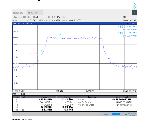
1-N26-824-849--15-5-H-4-DFT-64QAM-Outer_Full-2 5@0-Ant0-4.48-5.110-<math>\leq 5</math>-PASS
