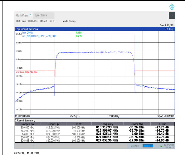
1-N26-814-824--15-10-M-6-CP-QPSK-Outer_Full-52@0-Ant0-PASS-see graph
