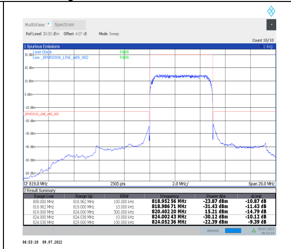
1-N26-814-824--15-5-H-3-DFT-PI2BPSK-Outer_Full-25@0-Ant0-PASS-see graph
