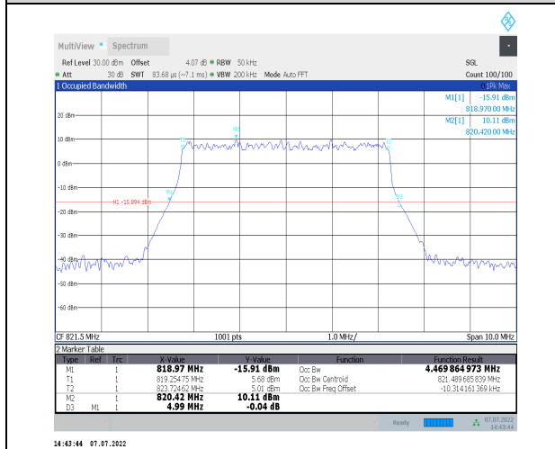
1-N26-814-824--15-5-H-5-DFT-256QAM-Outer_Full-2 25@0-Ant0-4.47-4.990-≤5-PASS
