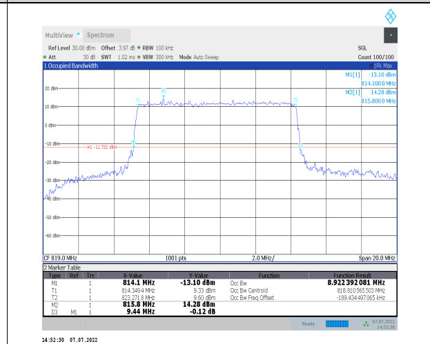
1-N26-814-824--15-10-M-1-DFT-QPSK-Outer_Full-5 0@0-Ant0-8.922-9.440-<math>\leq 10</math>-PASS
