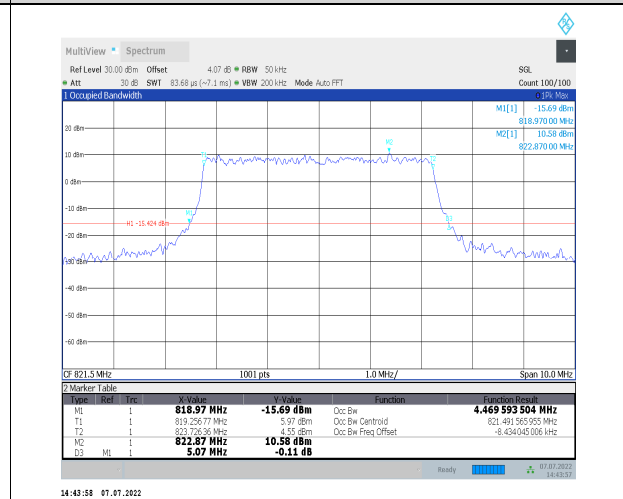
1-N26-814-824--15-5-H-6-CP-QPSK-Outer_Full-25 @0-Ant0-4.47-5.070-≤5-PASS
