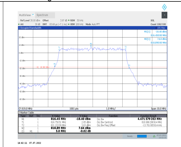
1-N26-814-824--15-5-M-9-CP-256QAM-Outer_Full-2 5@0-Ant0-4.472-5.000-<math>\leq</math>5-PASS
