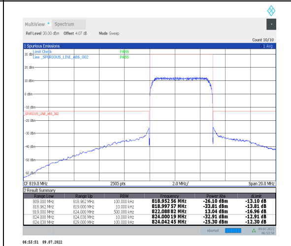
1-N26-814-824--15-5-H-6-CP-QPSK-Outer_Full-25@0-Ant0-PASS-see graph
