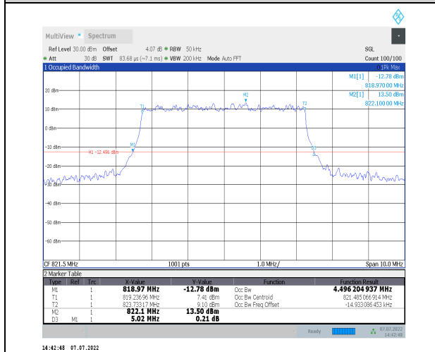
1-N26-814-824--15-5-H-1-DFT-QPSK-Outer_Full-25 @0-Ant0-4.496-5.020-<math>\leq</math>5-PASS
