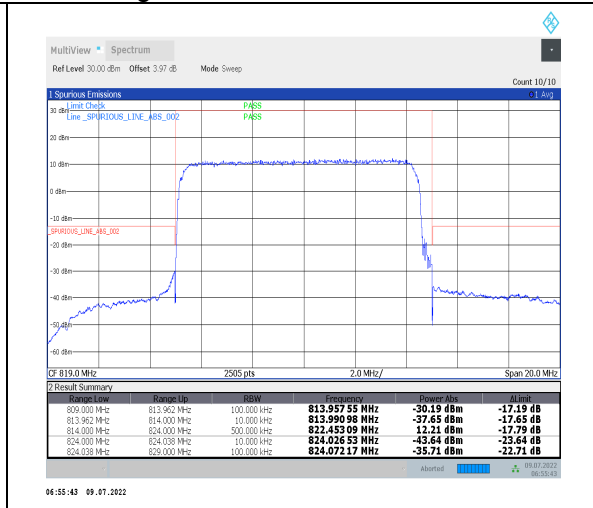
1-N26-814-824--15-10-M-3-DFT-PI2BPSK-Outer_Full-50@0-Ant0-PASS-see graph
