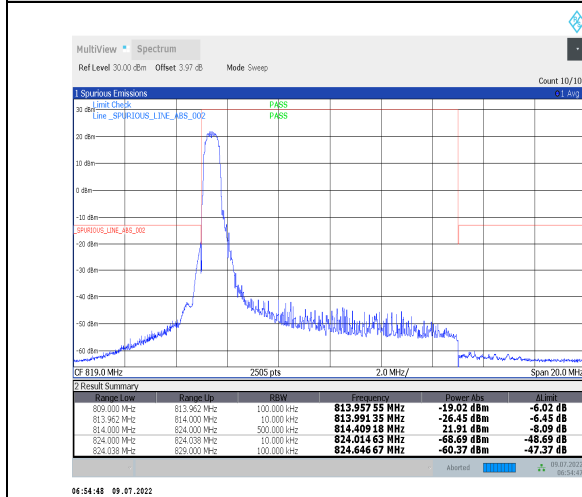
1-N26-814-824--15-10-M-4-CP-QPSK-Edge_1RB_Left-1@0-Ant0-PASS-see graph
