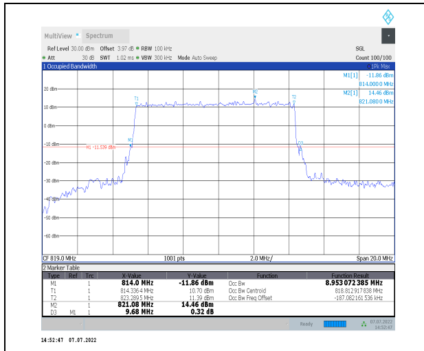
1-N26-814-824--15-10-M-2-DFT-PI2BPSK-Outer_Full-I-50@0-Ant0-8.953-9.680-<=10-PASS
