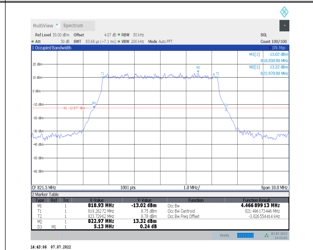
1-N26-814-824--15-5-H-2-DFT-PI2BPSK-Outer_Full-25 @0-Ant0-4.467-5.130-<math>\leq</math>5-PASS
