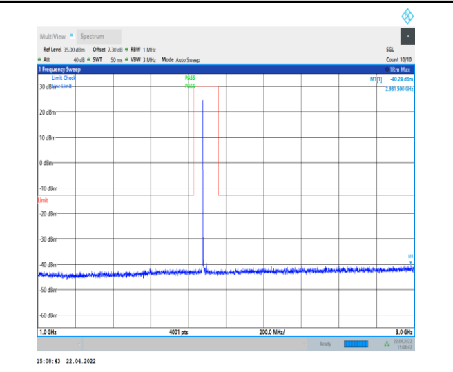
1-N25--15-40-H-1-DFT-PI2BPSK-Inner_1RB_Left-1 @ 1-1000-3000-Ant0--40.24--13-PASS
