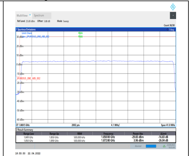
1-N25--15-40-L-3-DFT-PI2BPSK-Outer_Full-216@0-Ant0-seegraph-PASS-see graph
