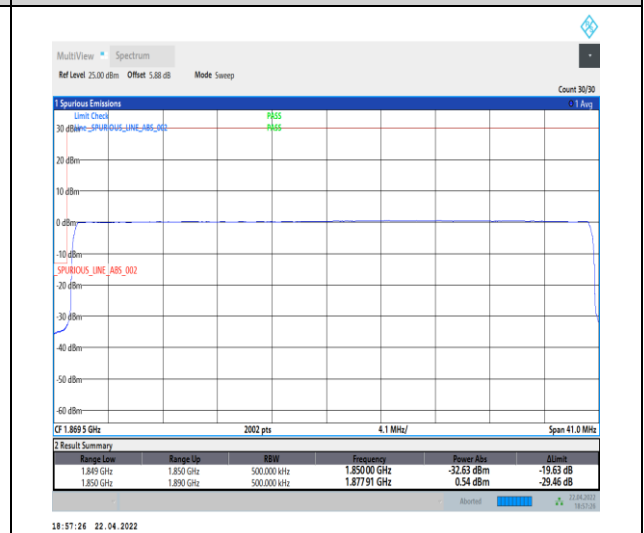
1-N25--15-40-L-6-CP-QPSK-Outer_Full-216@0-Ant0-seegraph-PASS-see graph
