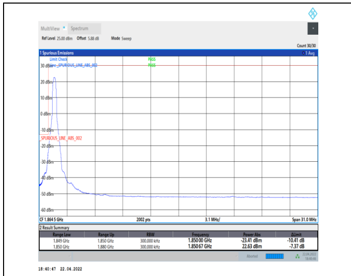
1-N25--15-30-L-1-DFT-PI2BPSK-Edge_1RB_Left-1@0-Ant0-seegraph-PASS-see graph
