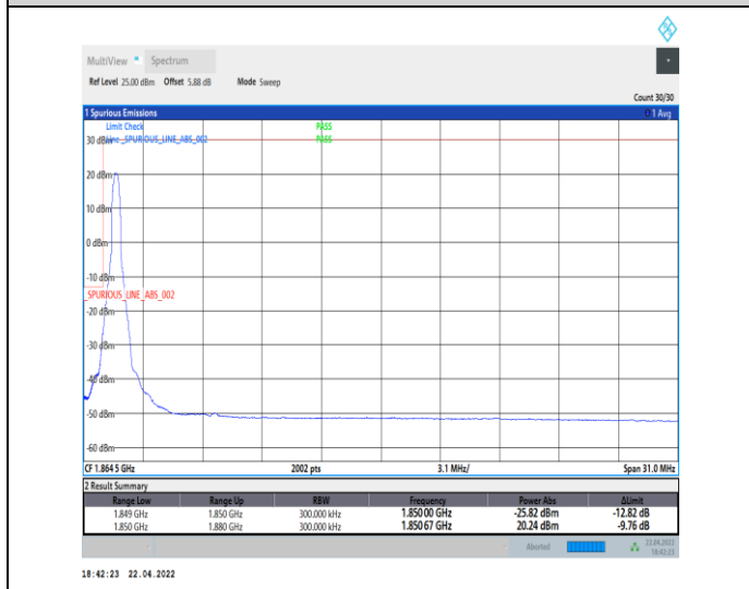
1-N25--15-30-L-4-CP-QPSK-Edge_1RB_Left-1@0-Ant0-seegraph-PASS-see graph
