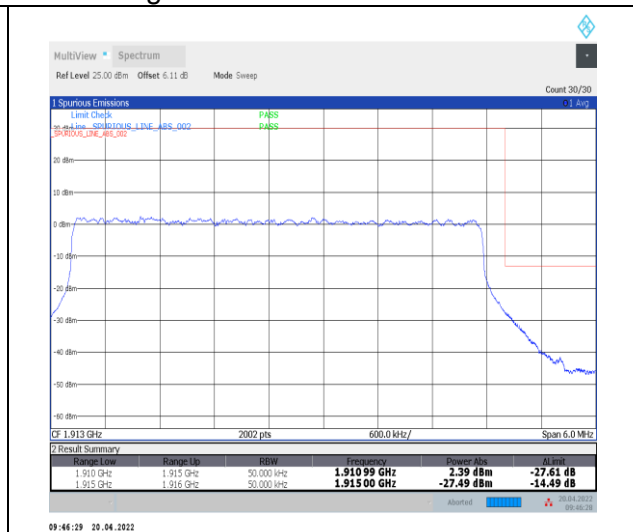
1-N25--15-5-H-3-DFT-PI2BPSK-Outer_Full-25@0-Ant0-seegraph-PASS-see graph
