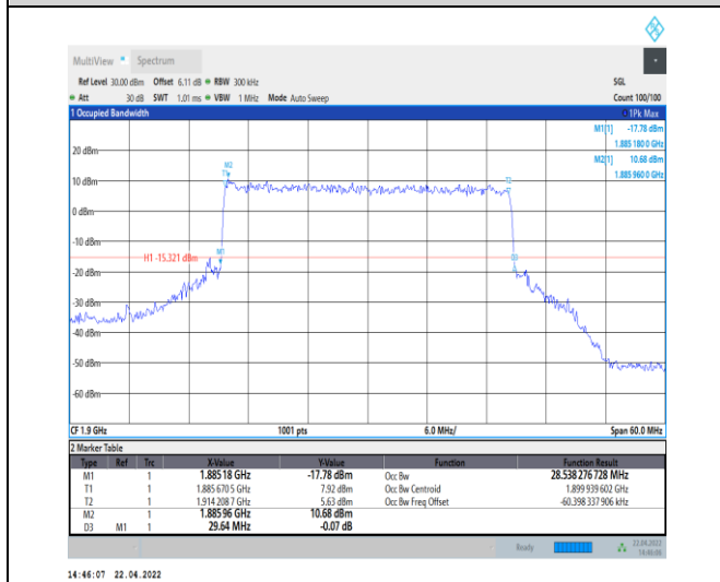
1-N25--15-30-H-6-CP-QPSK-Outer_Full-160@0-Ant 0-28.538-29.640-≤30-PASS
