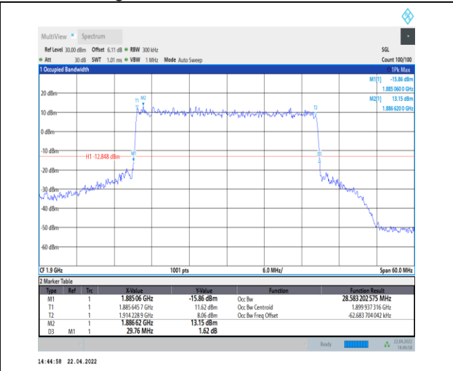
1-N25--15-30-H-1-DFT-QPSK-Outer_Full-160@0-An t0-28.583-29.760-<30-PASS
