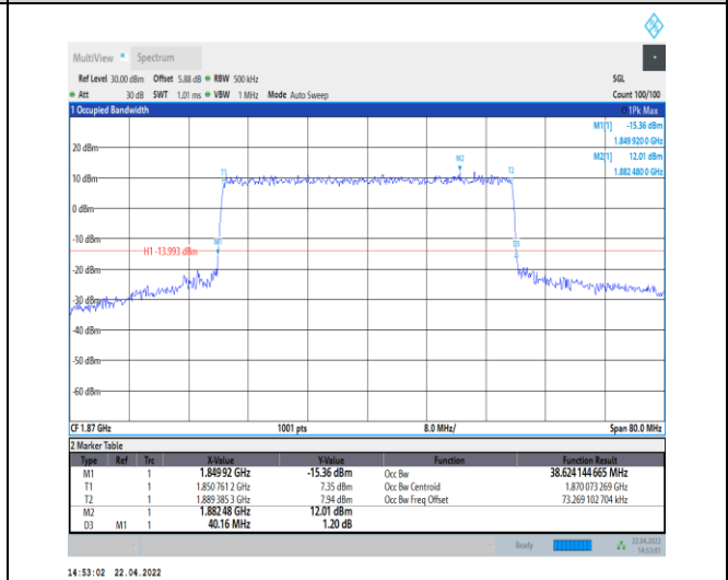
1-N25--15-40-L-6-CP-QPSK-Outer_Full-216@0-Ant0 -38.624-40.160-≤40-PASS
