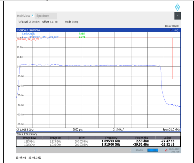
1-N25--15-20-H-3-DFT-PI2BPSK-Outer_Full-100 @ 0-Ant0-seegraph-PASS-see graph
