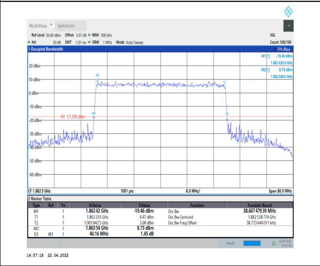
1-N25--15-40-M-9-CP-256QAM-Outer_Full-216@0-A Ant0-38.607-40.160-≤40-PASS
