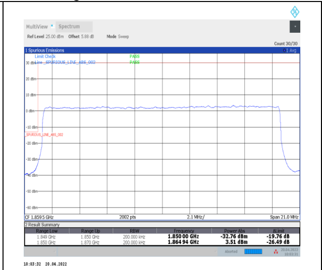
1-N25--15-20-L-3-DFT-PI2BPSK-Outer_Full-100@0-Ant0-seegraph-PASS-see graph
