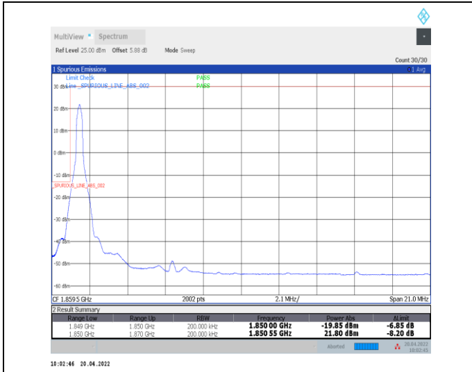
1-N25--15-20-L-1-DFT-PI2BPSK-Edge_1RB_Left-1@0-Ant0-seegraph-PASS-see graph
