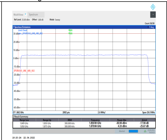
1-N25--15-25-L-3-DFT-PI2BPSK-Outer_Full-128@0-Ant0-seegraph-PASS-see graph
