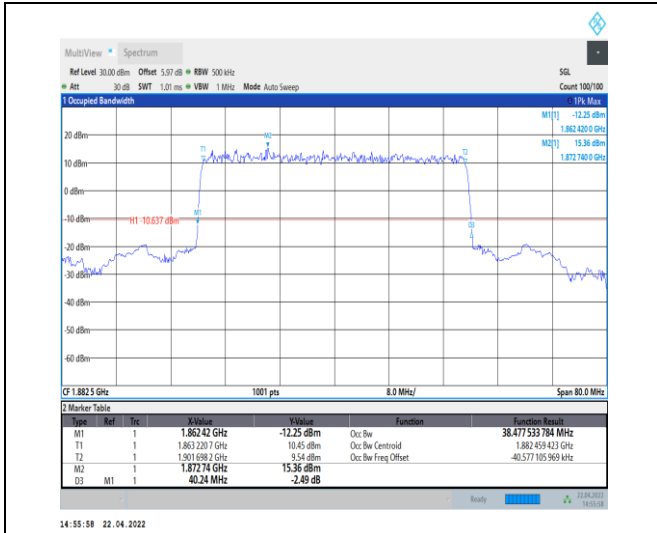
1-N25--15-40-M-2-DFT-PI2BPSK-Outer_Full-216@0-Ant0-38.478-40.240-≤40-PASS
