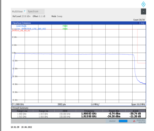
1-N25--15-15-H-6-CP-QPSK-Outer_Full-79@0-Ant0-seegraph-PASS-see graph
