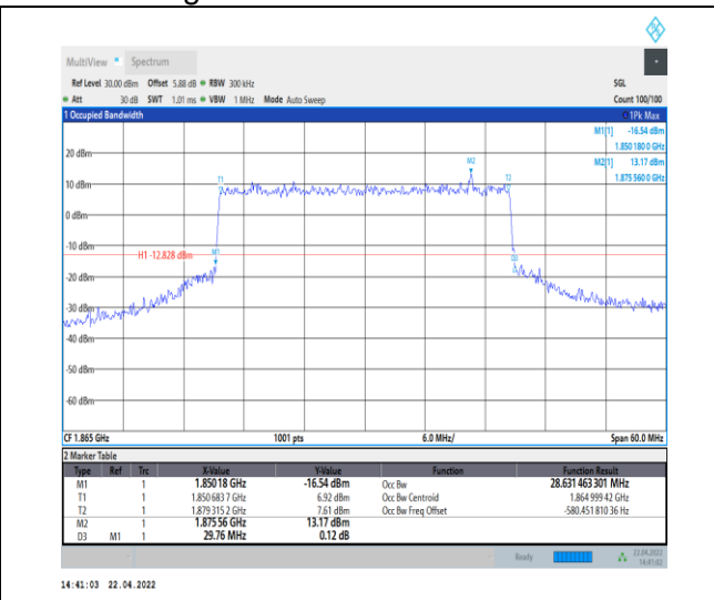
1-N25--15-30-L-7-CP-16QAM-Outer_Full-160@0-Ant0 -28.631-29.760-≤30-PASS
