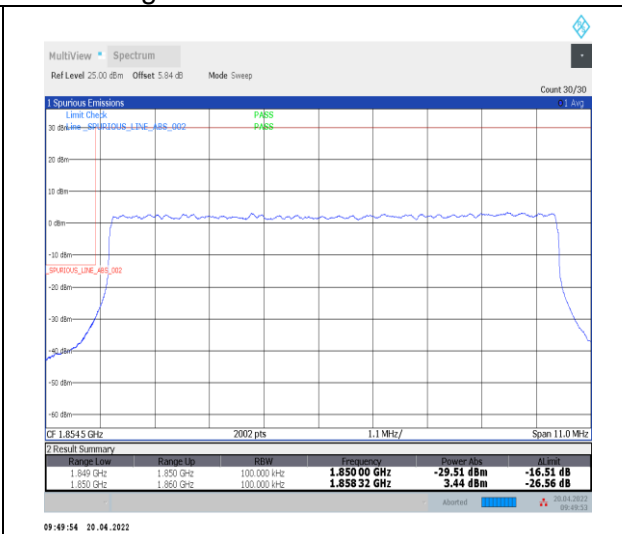
1-N25--15-10-L-3-DFT-PI2BPSK-Outer_Full-50@0 -Ant0-seegraph-PASS-see graph
