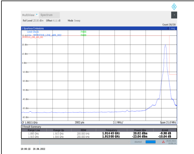
1-N25--15-20-H-2-DFT-PI2BPSK-Edge_1RB_Right-1 @ 105-Ant0-seegraph-PASS-see graph
