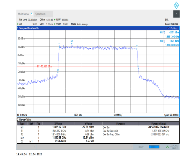
1-N25--15-30-H-3-DFT-16QAM-Outer_Full-160@0-A nt0-28.568-29.760-<30-PASS
