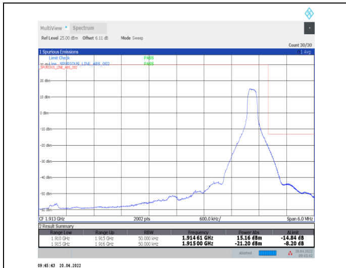
1-N25--15-5-H-2-DFT-PI2BPSK-Edge_1RB_Right-1@24-Ant0-seegraph-PASS-see graph
