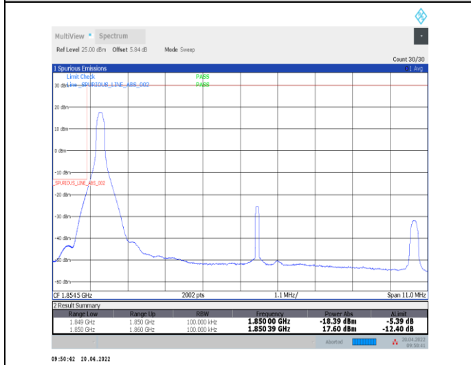
1-N25--15-10-L-4-CP-QPSK-Edge_1RB_Left-1@0-Ant 0-seegraph-PASS-see graph
