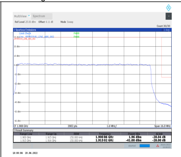
1-N25--15-15-H-3-DFT-PI2BPSK-Outer_Full-75@0-Ant0-seegraph-PASS-see graph
