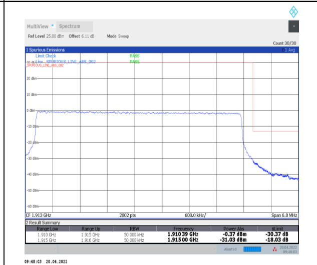
1-N25--15-5-H-6-CP-QPSK-Outer_Full-25@0-Ant0-seegraph-PASS-see graph
