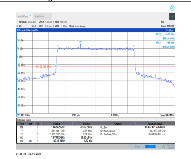
1-N25--15-40-M-7-CP-16QAM-Outer_Full-216@0-A nt0-38.432-40.160-≤40-PASS
