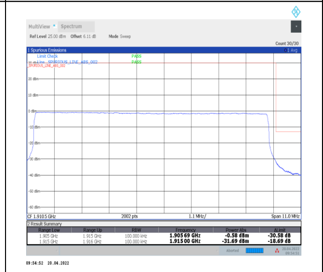
1-N25--15-10-H-6-CP-QPSK-Outer_Full-52@0-Ant0-seegraph-PASS-see graph
