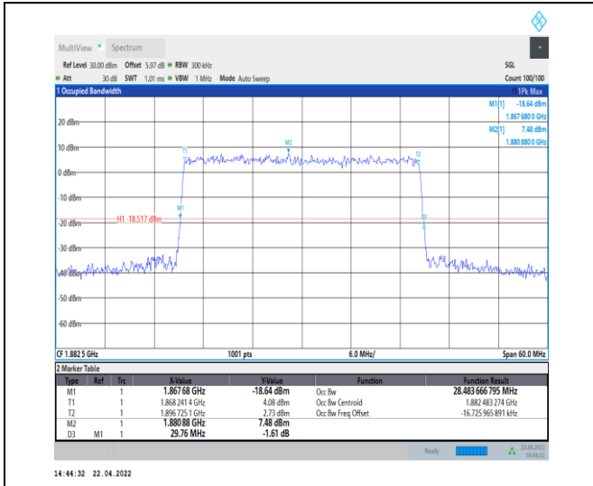
1-N25--15-30-M-9-CP-256QAM-Outer_Full-160@0-Ant0-28.484-29.760-<30-PASS
