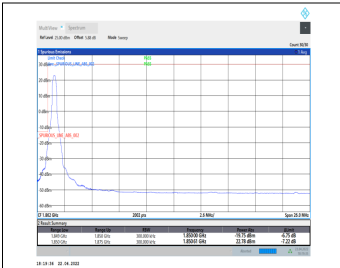
1-N25--15-25-L-1-DFT-PI2BPSK-Edge_1RB_Left-1@0-Ant0-seegraph-PASS-see graph
