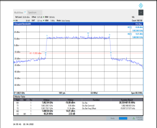
1-N25--15-40-M-1-DFT-QPSK-Outer_Full-216@0-An t0-38.559-40.240-<math>\leq 40</math>-PASS
