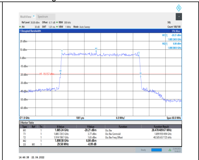
1-N25--15-30-H-9-CP-256QAM-Outer_Full-160@0-Ant nt0-28.478-29.580-≤30-PASS
