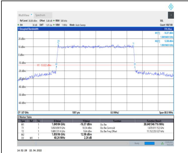
1-N25--15-40-L-3-DFT-16QAM-Outer_Full-216@0-A nt0-38.641-40.240-≤40-PASS
