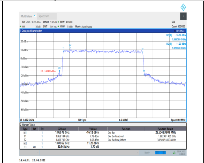
1-N25--15-30-M-6-CP-QPSK-Outer_Full-160@0-Ant0-28.555-30.540-<=30-PASS
