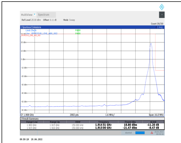
1-N25--15-15-H-2-DFT-PI2BPSK-Edge_1RB_Right-1 @78-Ant0-seegraph-PASS-see graph
