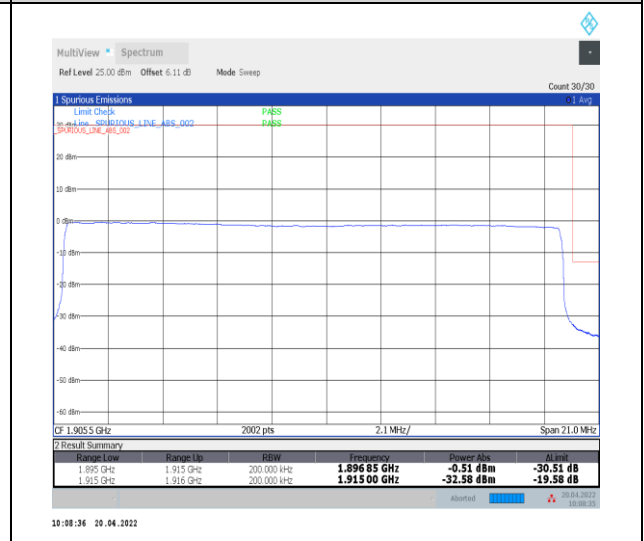
1-N25--15-20-H-6-CP-QPSK-Outer_Full-106 @ 0-A -nt0-seegraph-PASS-see graph
