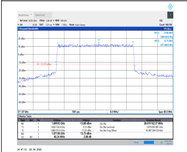
1-N25--15-40-L-1-DFT-QPSK-Outer_Full-216@0-Ant 0-38.619-40.240-≤40-PASS
