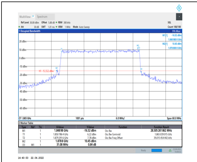
1-N25--15-30-L-6-CP-QPSK-Outer_Full-160@0-Ant0 -28.505-31.080-≤30-PASS
