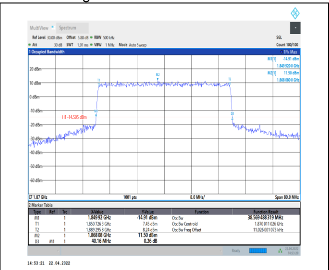
1-N25--15-40-L-8-CP-64QAM-Outer_Full-216@0-An t0-38.569-40.160-<math>\leq 40</math>-PASS
