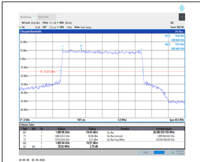
1-N25--15-30-H-4-DFT-64QAM-Outer_Full-160@0-A nt0-28.58-29.820-≤30-PASS
