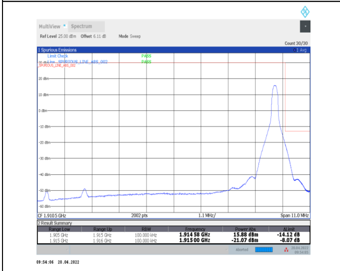
1-N25--15-10-H-5-CP-QPSK-Edge_1RB_Right-1 @51-Ant0-seegraph-PASS-see graph
