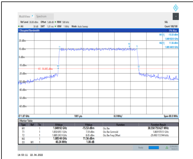
1-N25--15-40-L-7-CP-16QAM-Outer_Full-216@0-An t0-38.551-40.240-<math>\leq 40</math>-PASS
