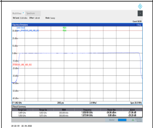
1-N25--15-25-L-6-CP-QPSK-Outer_Full-133@0-Ant0-seegraph-PASS-see graph
