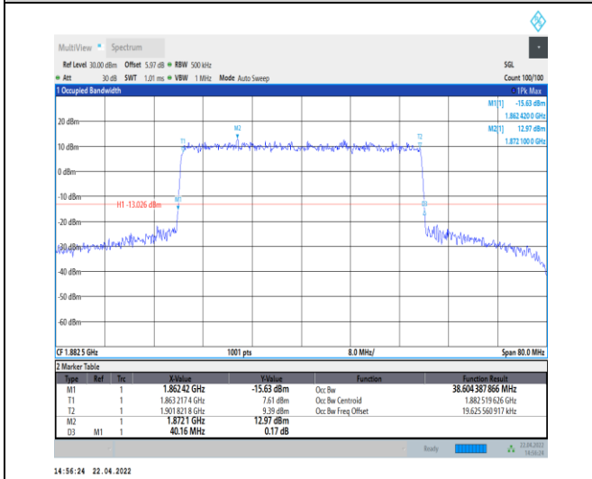
1-N25--15-40-M-4-DFT-64QAM-Outer_Full-216@0-Ant0-38.604-40.160-≤40-PASS
