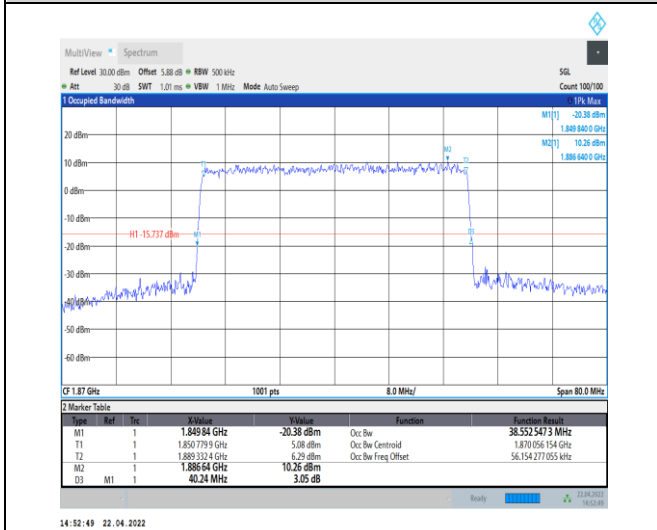
1-N25--15-40-L-5-DFT-256QAM-Outer_Full-216@0-A Ant0-38.553-40.240-≤40-PASS
