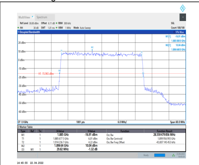
1-N25--15-30-H-5-DFT-256QAM-Outer_Full-160@0-Ant0-28.559-29.820-≤30-PASS
