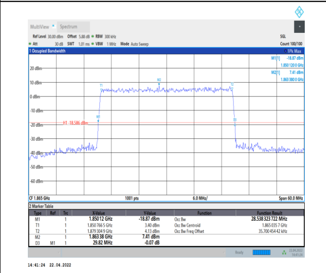
1-N25--15-30-L-9-CP-256QAM-Outer_Full-160@0-Ant0 -28.538-29.820-≤30-PASS
