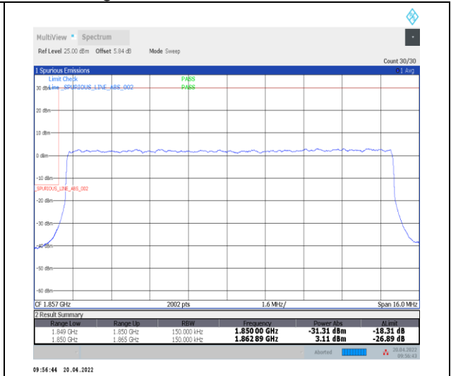
1-N25--15-15-L-3-DFT-PI2BPSK-Outer_Full-75@0 -Ant0-seegraph-PASS-see graph
