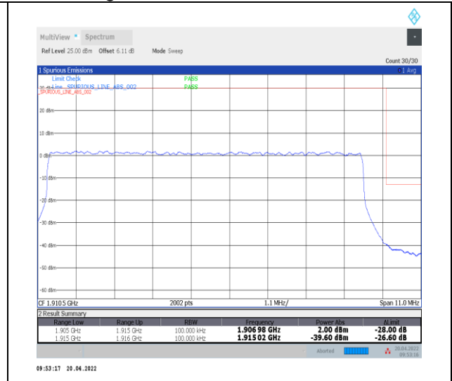
1-N25--15-10-H-3-DFT-PI2BPSK-Outer_Full-50@0-Ant0-seegraph-PASS-see graph
