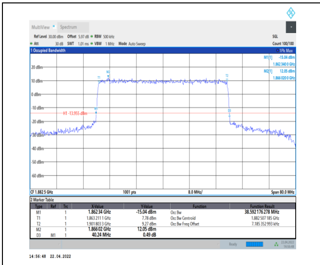
1-N25--15-40-M-6-CP-QPSK-Outer_Full-216@0-Ant 0-38.592-40.240-≤40-PASS
