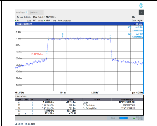
1-N25--15-40-L-4-DFT-64QAM-Outer_Full-216@0-A nt0-38.586-40.320-≤40-PASS
