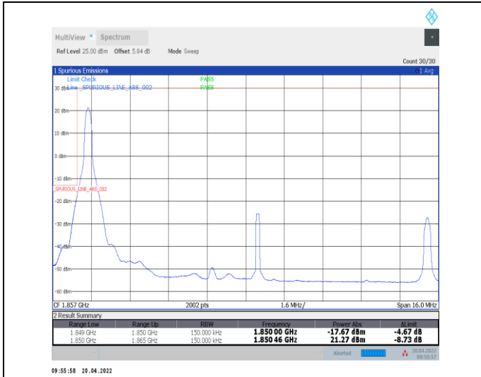
1-N25--15-15-L-1-DFT-PI2BPSK-Edge_1RB_Left-1@0 -Ant0-seegraph-PASS-see graph
