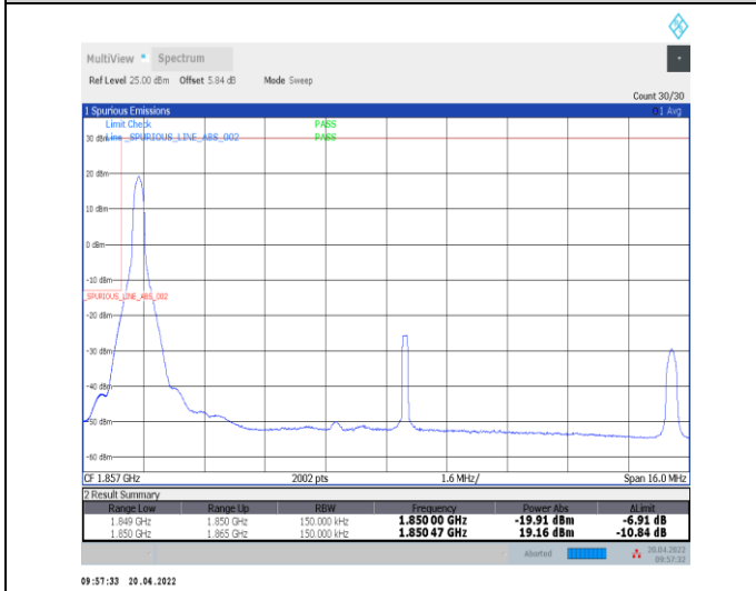
1-N25--15-15-L-4-CP-QPSK-Edge_1RB_Left-1@0-Ant 0-seegraph-PASS-see graph
