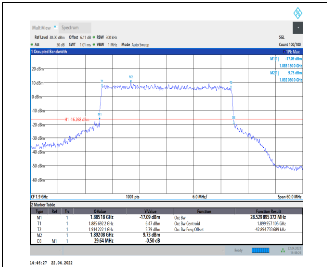
1-N25--15-30-H-8-CP-64QAM-Outer_Full-160@0-Ant t0-28.53-29.640-≤30-PASS
