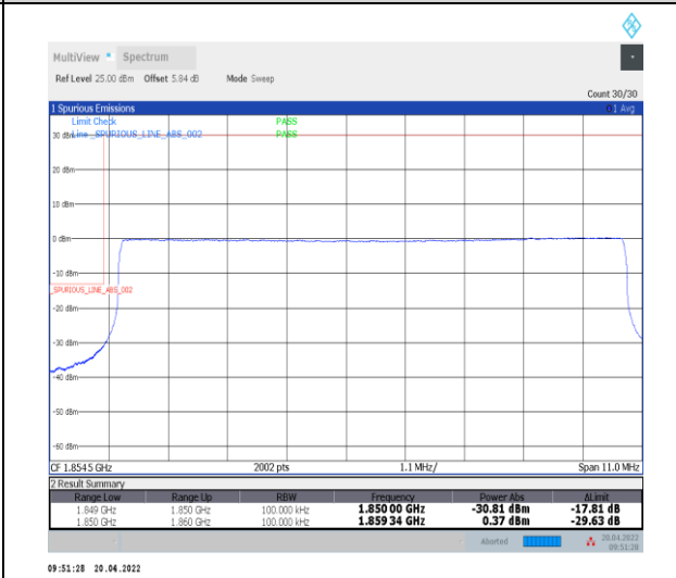
1-N25--15-10-L-6-CP-QPSK-Outer_Full-52@0-Ant 0-seegraph-PASS-see graph
