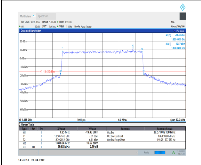
1-N25--15-30-L-8-CP-64QAM-Outer_Full-160@0-Ant0 -28.571-29.880-≤30-PASS
