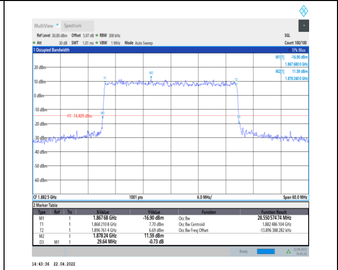
1-N25--15-30-M-4-DFT-64QAM-Outer_Full-160@0-Ant0-28.551-29.640-<30-PASS
