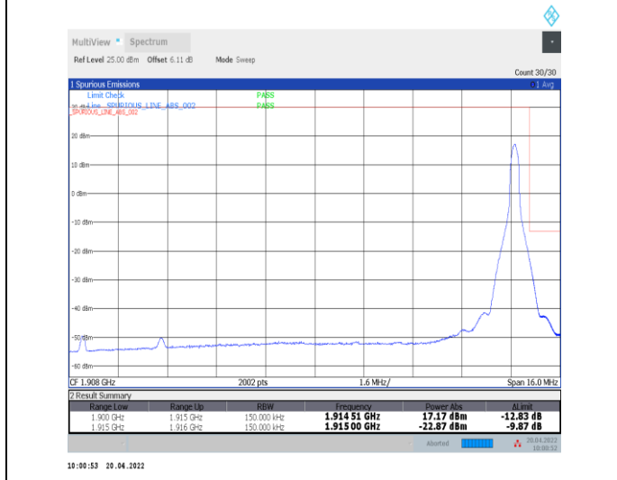
1-N25--15-15-H-5-CP-QPSK-Edge_1RB_Right-1 @78-Ant0-seegraph-PASS-see graph
