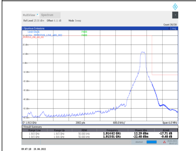
1-N25--15-5-H-5-CP-QPSK-Edge_1RB_Right-1@24-Ant0-seegraph-PASS-see graph
