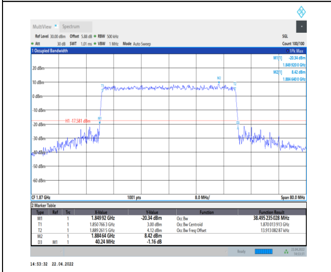
1-N25--15-40-L-9-CP-256QAM-Outer_Full-216@0-A nt0-38.495-40.240-<math>\leq 40</math>-PASS
