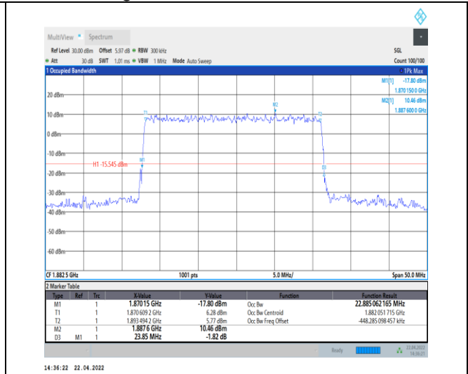
1-N25--15-25-M-5-DFT-256QAM-Outer_Full-128@0-A Ant0-22.885-23.850-≤25-PASS
