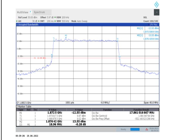
1-N25--15-20-M-1-DFT-QPSK-Outer_Full-100@0-An t0-17.861-18.960-<20-PASS
