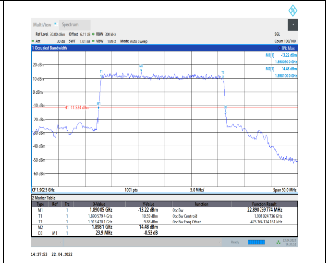
1-N25--15-25-H-2-DFT-PI2BPSK-Outer_Full-128@0- Ant0-22.891-23.900-≤25-PASS
