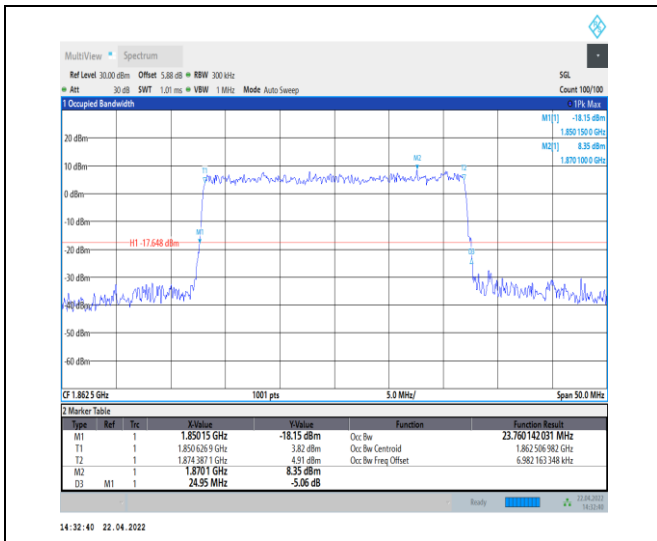
1-N25--15-25-L-9-CP-256QAM-Outer_Full-133@0-A nt0-23.76-24.950-≤25-PASS
