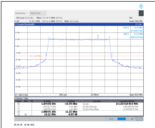
1-N25--15-15-M-6-CP-QPSK-Outer_Full-79@0-Ant0 -14.133-15.210-≤15-PASS
