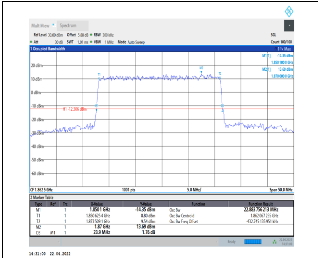
1-N25--15-25-L-1-DFT-QPSK-Outer_Full-128@0-Ant 0-22.884-23.900-≤25-PASS
