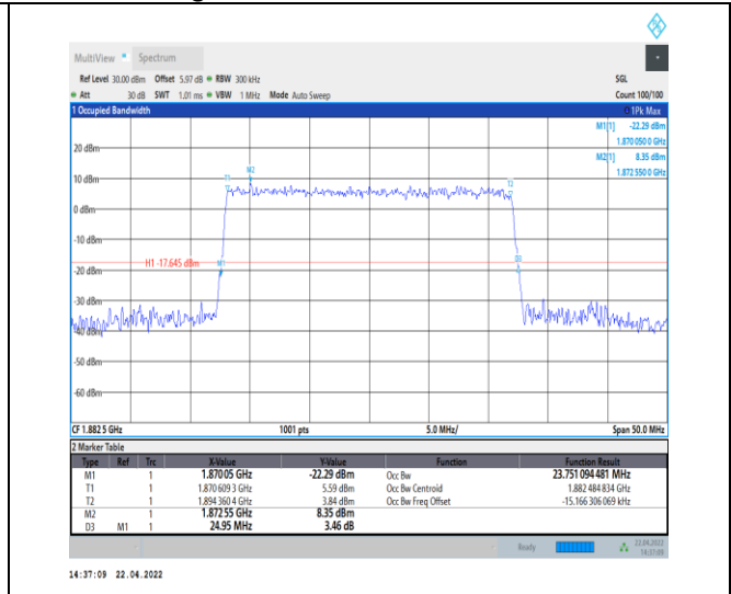
1-N25--15-25-M-9-CP-256QAM-Outer_Full-133@0- Ant0-23.751-24.950-≤25-PASS
