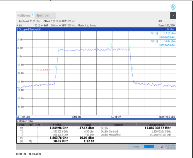
1-N25--15-20-L-5-DFT-256QAM-Outer_Full-100@0-A Ant0-17.887-18.920-≤20-PASS
