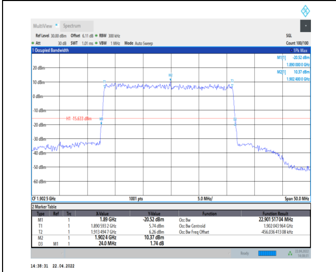
1-N25--15-25-H-5-DFT-256QAM-Outer_Full-128@0-A Ant0-22.902-24.000-<=25-PASS
