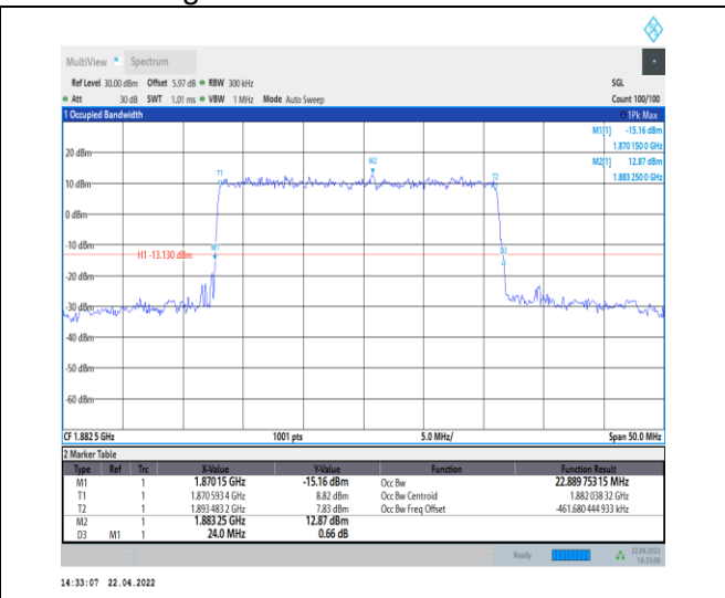
1-N25--15-25-M-1-DFT-QPSK-Outer_Full-128@0-An t0-22.89-24.000-≤25-PASS
