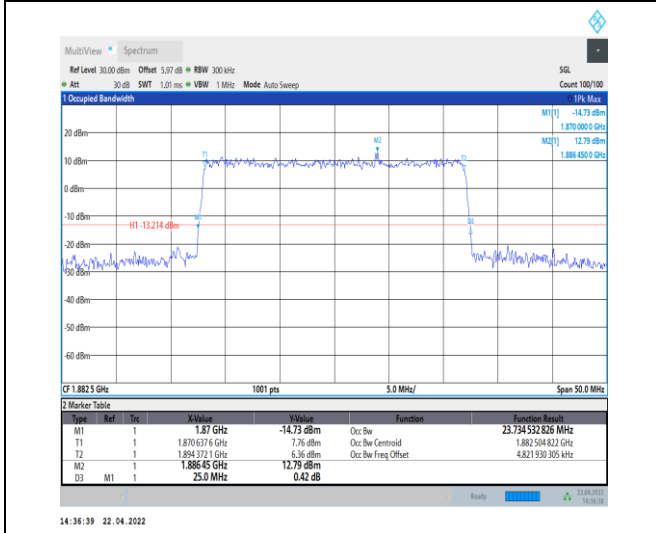
1-N25--15-25-M-6-CP-QPSK-Outer_Full-133@0-Ant 0-23.735-25.000-≤25-PASS
