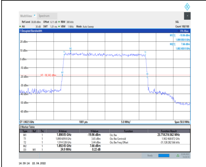
1-N25--15-25-H-9-CP-256QAM-Outer_Full-133@0-A nt0-23.718-24.900-<=25-PASS
