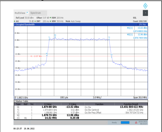
1-N25--15-15-M-3-DFT-16QAM-Outer_Full-75@0-An t0-13.452-14.520-≤15-PASS
