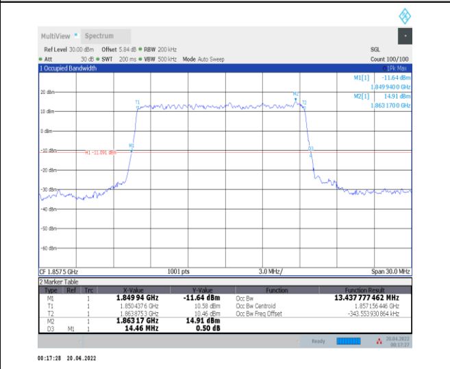
1-N25--15-15-L-2-DFT-PI2BPSK-Outer_Full-75@0-A nt0-13.438-14.460-≤15-PASS
