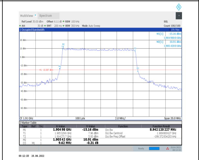
1-N25--15-10-H-3-DFT-16QAM-Outer_Full-50@0-Ant t0-8.942-9.620-≤10-PASS
