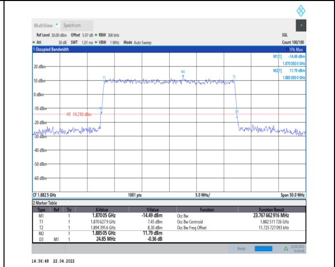
1-N25--15-25-M-7-CP-16QAM-Outer_Full-133@0-A nt0-23.768-24.850-≤25-PASS
