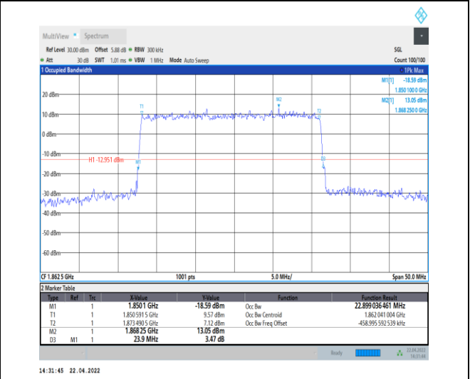
1-N25--15-25-L-4-DFT-64QAM-Outer_Full-128@0-Ant 0-22.899-23.900-≤25-PASS
