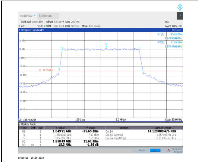
1-N25--15-15-L-7-CP-16QAM-Outer_Full-79@0-Ant 0-14.129-15.300-≤15-PASS
