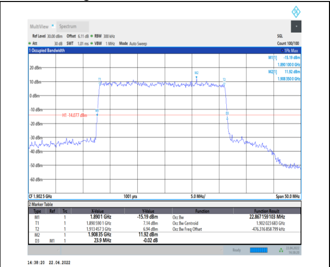
1-N25--15-25-H-4-DFT-64QAM-Outer_Full-128@0-A nt0-22.867-23.900-<=25-PASS
