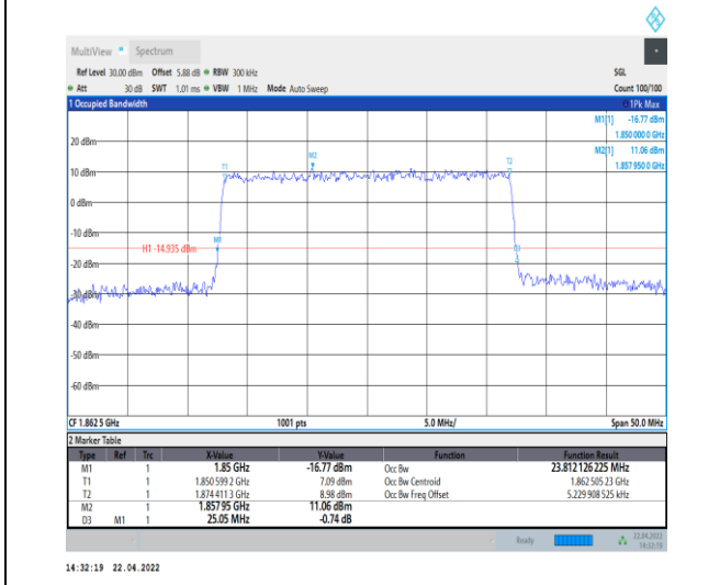
1-N25--15-25-L-7-CP-16QAM-Outer_Full-133@0-An t0-23.812-25.050-<=25-PASS
