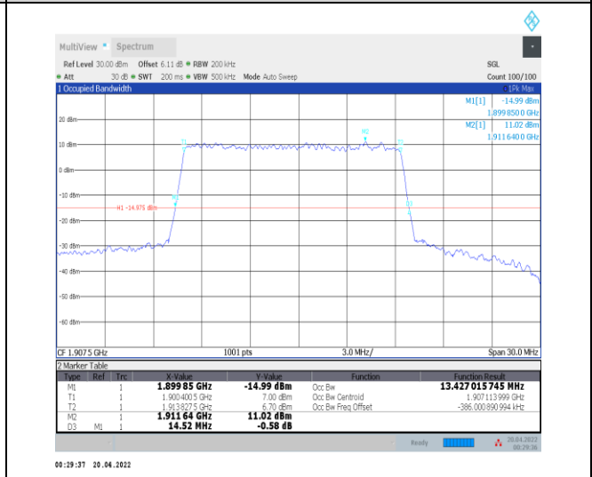
1-N25--15-15-H-4-DFT-64QAM-Outer_Full-75@0-Ant t0-13.427-14.520-≤15-PASS
