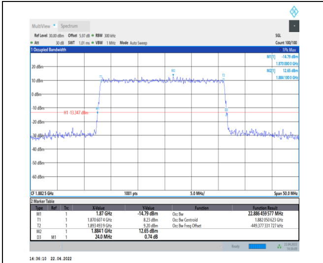
1-N25--15-25-M-4-DFT-64QAM-Outer_Full-128@0-A nt0-22.886-24.000-≤25-PASS
