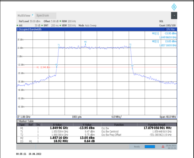
1-N25--15-20-L-3-DFT-16QAM-Outer_Full-100@0-Ant 0-17.879-18.920-≤20-PASS
