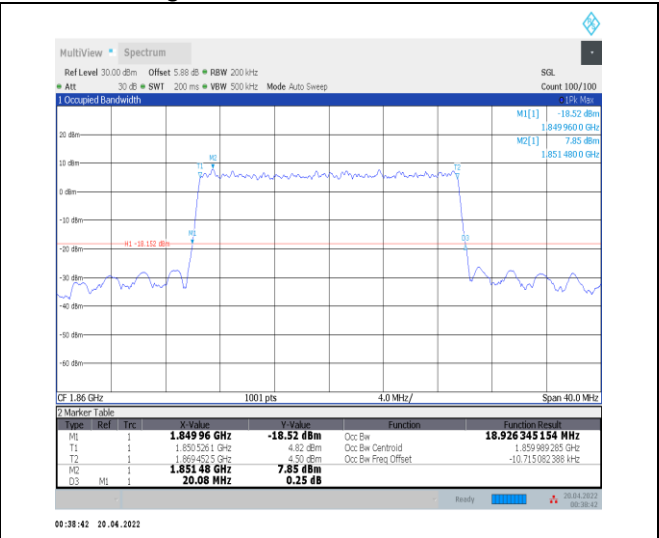
1-N25--15-20-L-9-CP-256QAM-Outer_Full-106@0-A nt0-18.926-20.080-<20-PASS
