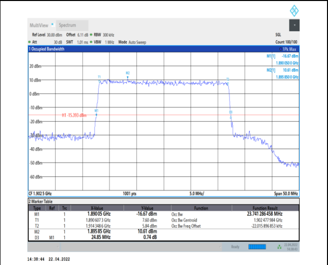
1-N25--15-25-H-6-CP-QPSK-Outer_Full-133@0-Ant 0-23.741-24.850-<=25-PASS
