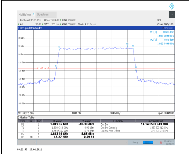
1-N25--15-15-L-9-CP-256QAM-Outer_Full-79@0-Ant t0-14.144-15.270-≤15-PASS
