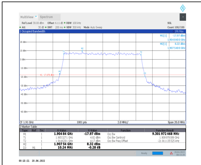
1-N25--15-10-H-8-CP-64QAM-Outer_Full-52@0-Ant 0-9.302-10.240-≤10-PASS
