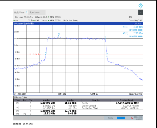
1-N25--15-20-H-1-DFT-QPSK-Outer_Full-100@0-An t0-17.848-18.920-<=20-PASS
