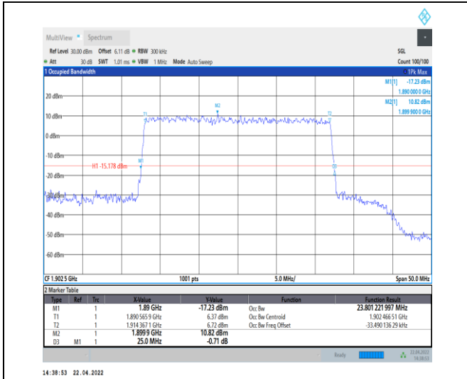
1-N25--15-25-H-7-CP-16QAM-Outer_Full-133@0-An t0-23.801-25.000-<=25-PASS
