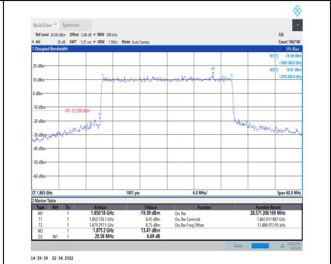
1-N25--15-30-L-1-DFT-QPSK-Outer_Full-160@0-Ant 0-28.571-29.580-<=30-PASS
