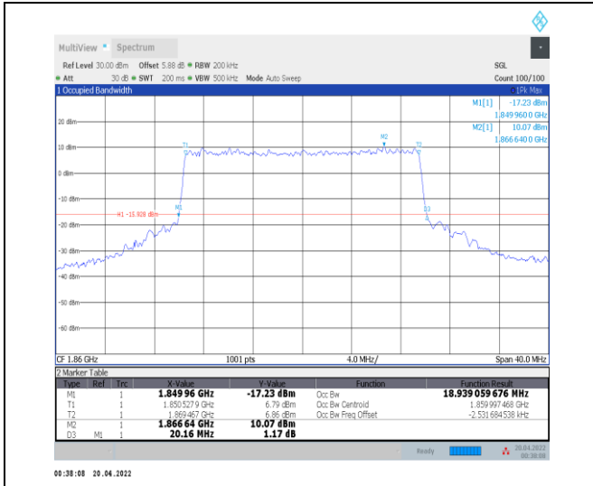
1-N25--15-20-L-8-CP-64QAM-Outer_Full-106@0-An t0-18.939-20.160-<20-PASS
