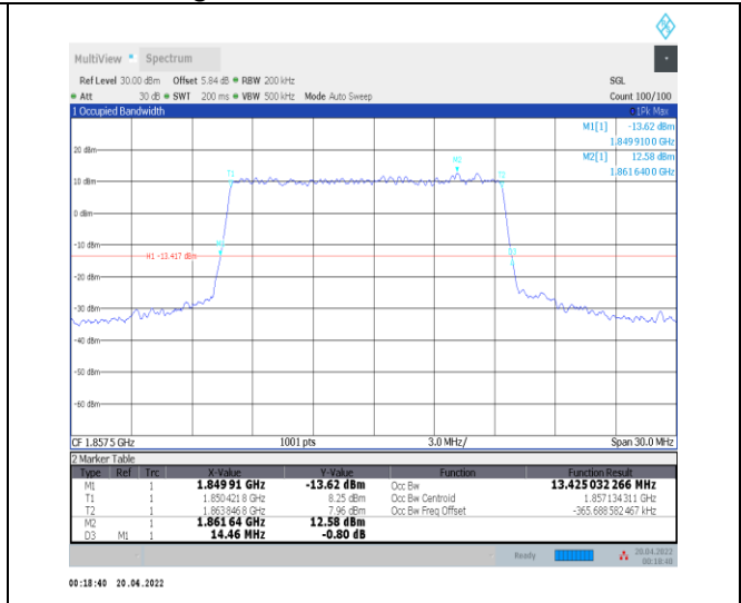
1-N25--15-15-L-4-DFT-64QAM-Outer_Full-75@0-Ant 0-13.425-14.460-≤15-PASS
