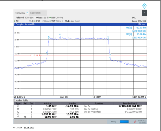
1-N25--15-20-L-1-DFT-QPSK-Outer_Full-100@0-Ant 0-17.855-18.920-≤20-PASS
