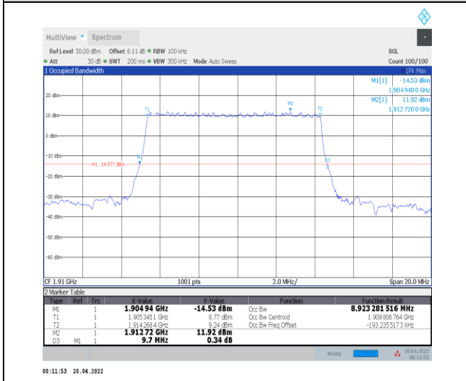
1-N25--15-10-H-2-DFT-PI2BPSK-Outer_Full-50@0-Ant Ant0-8.923-9.700-≤10-PASS
