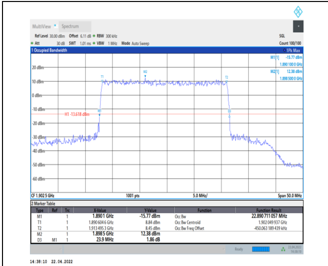
1-N25--15-25-H-3-DFT-16QAM-Outer_Full-128@0-A nt0-22.891-23.900-<=25-PASS
