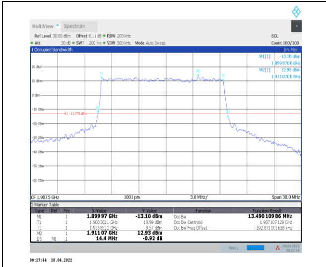
1-N25--15-15-H-1-DFT-QPSK-Outer_Full-75@0-Ant 0-13.49-14.400-≤15-PASS
