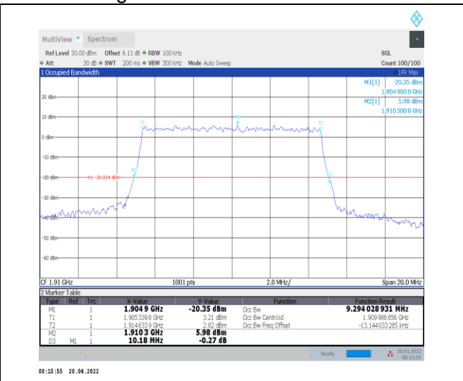
1-N25--15-10-H-9-CP-256QAM-Outer_Full-52@0-An t0-9.294-10.180-≤10-PASS
