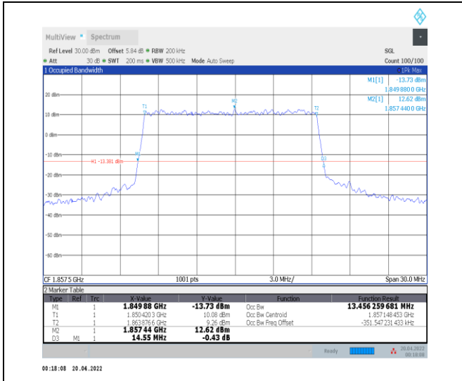
1-N25--15-15-L-3-DFT-16QAM-Outer_Full-75@0-Ant 0-13.456-14.550-≤15-PASS
