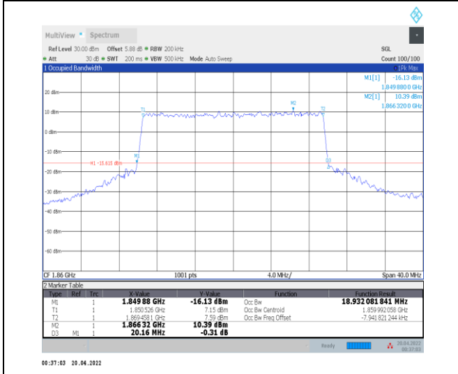
1-N25--15-20-L-6-CP-QPSK-Outer_Full-106@0-Ant0 -18.932-20.160-≤20-PASS
