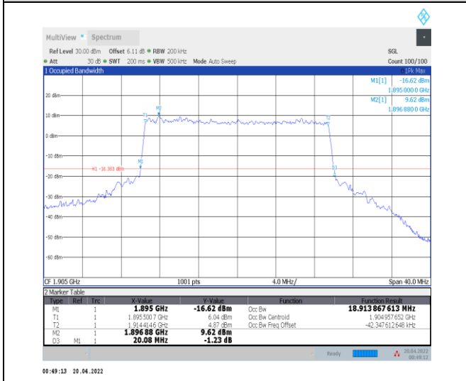
1-N25--15-20-H-8-CP-64QAM-Outer_Full-106@0-Ant 0-18.914-20.080-≤20-PASS
