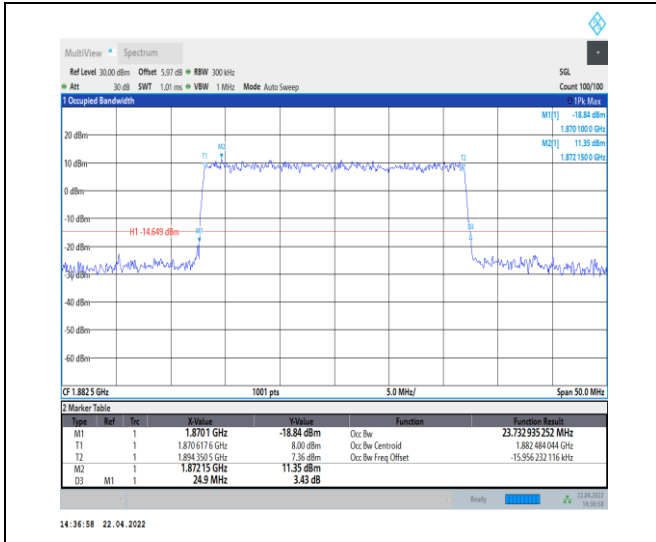
1-N25--15-25-M-8-CP-64QAM-Outer_Full-133@0-A nt0-23.733-24.900-≤25-PASS
