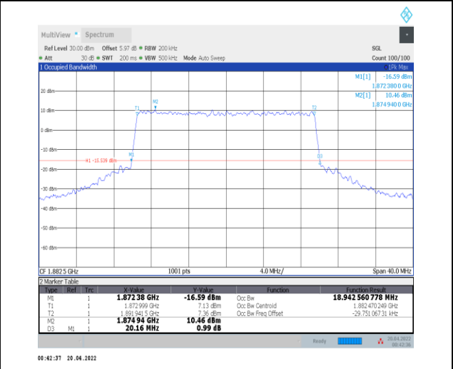
1-N25--15-20-M-6-CP-QPSK-Outer_Full-106@0-Ant 0-18.943-20.160-≤20-PASS
