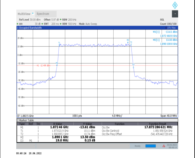
1-N25--15-20-M-2-DFT-PI2BPSK-Outer_Full-100@0 -Ant0-17.873-19.000-<20-PASS
