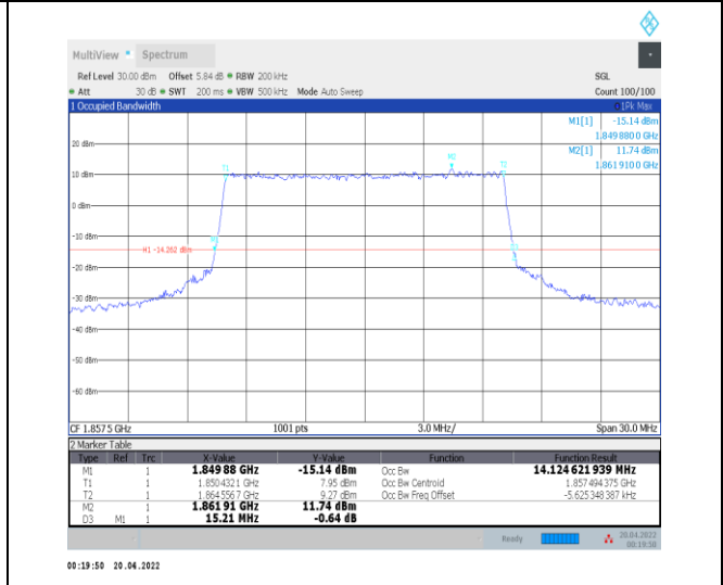
1-N25--15-15-L-6-CP-QPSK-Outer_Full-79@0-Ant0 14.125-15.210-≤15-PASS
