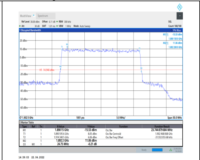
1-N25--15-25-H-8-CP-64QAM-Outer_Full-133@0-An t0-23.745-24.750-<=25-PASS
