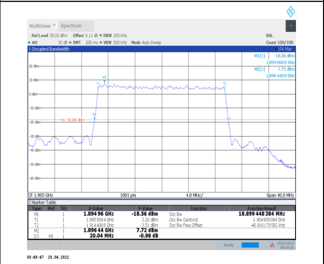
1-N25--15-20-H-9-CP-256QAM-Outer_Full-106@0-Ant 0-18.899-20.040-≤20-PASS
