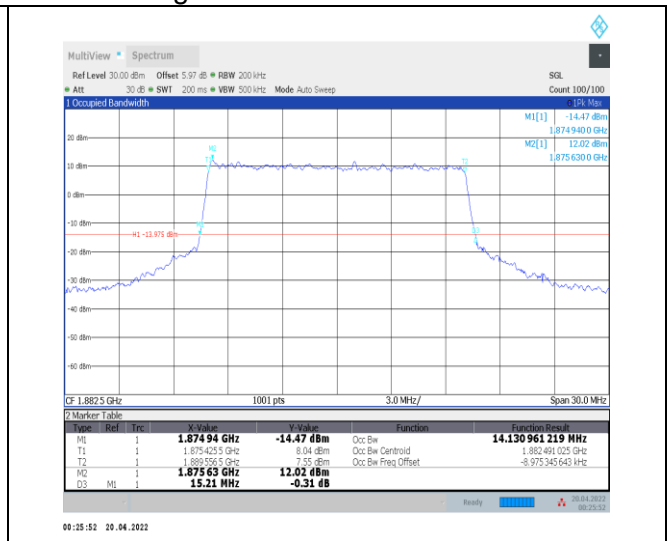
1-N25--15-15-M-7-CP-16QAM-Outer_Full-79@0-Ant0 0-14.131-15.210-≤15-PASS
