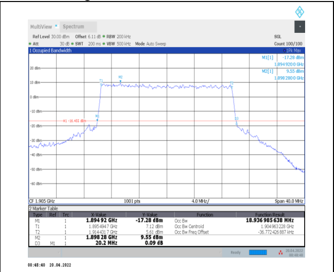
1-N25--15-20-H-7-CP-16QAM-Outer_Full-106@0-Ant 0-18.937-20.200-≤20-PASS
