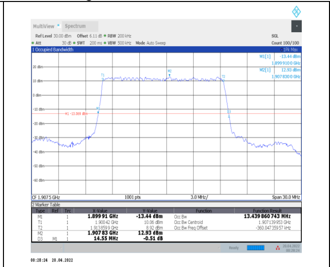
1-N25--15-15-H-2-DFT-PI2BPSK-Outer_Full-75@0-Ant 0-13.44-14.550-≤15-PASS
