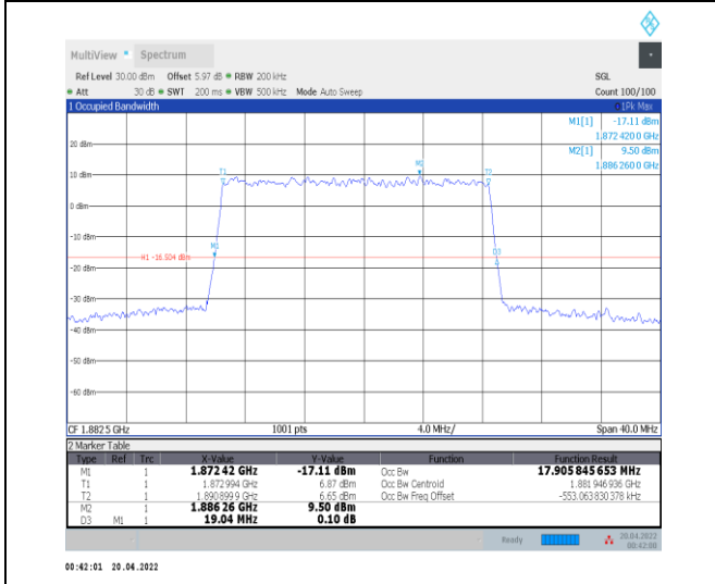
1-N25--15-20-M-5-DFT-256QAM-Outer_Full-100@0-A Ant0-17.906-19.040-≤20-PASS
