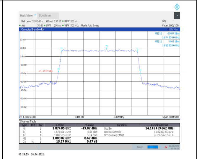
1-N25--15-15-M-9-CP-256QAM-Outer_Full-79@0-Ant0 nt0-14.145-15.270-≤15-PASS
