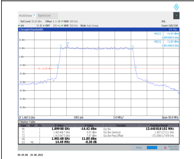
1-N25--15-15-H-3-DFT-16QAM-Outer_Full-75@0-Ant t0-13.441-14.490-≤15-PASS
