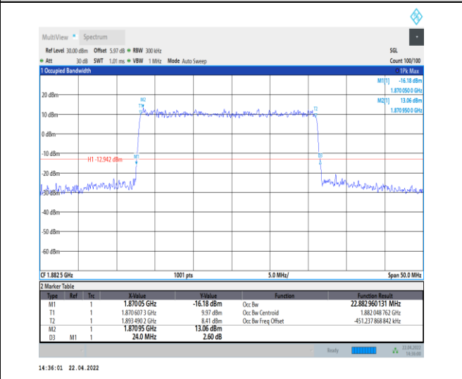
1-N25--15-25-M-3-DFT-16QAM-Outer_Full-128@0-A nt0-22.883-24.000-≤25-PASS
