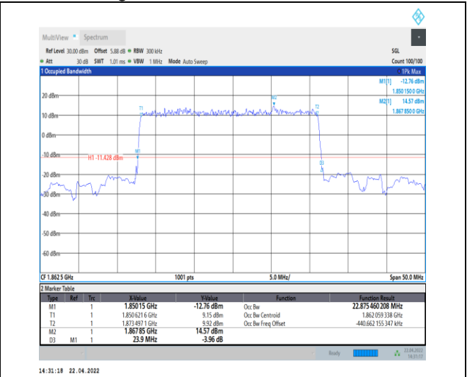
1-N25--15-25-L-2-DFT-PI2BPSK-Outer_Full-128@0-Ant 0-22.875-23.900-≤25-PASS
