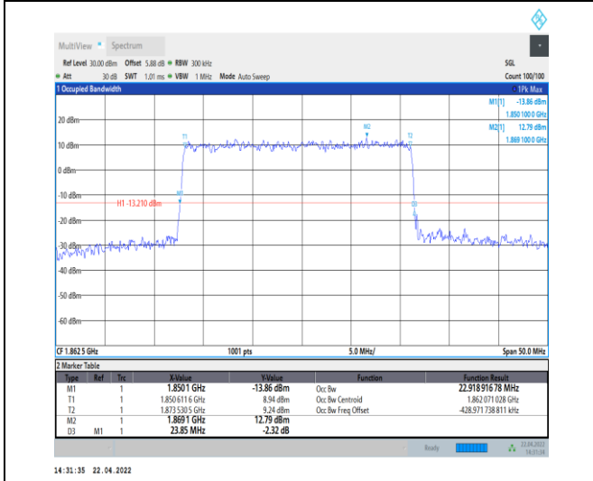
1-N25--15-25-L-3-DFT-16QAM-Outer_Full-128@0-Ant 0-22.919-23.850-≤25-PASS
