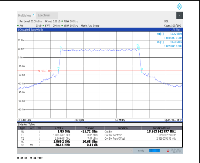
1-N25--15-20-L-7-CP-16QAM-Outer_Full-106@0-Ant0 t0-18.963-20.160-≤20-PASS
