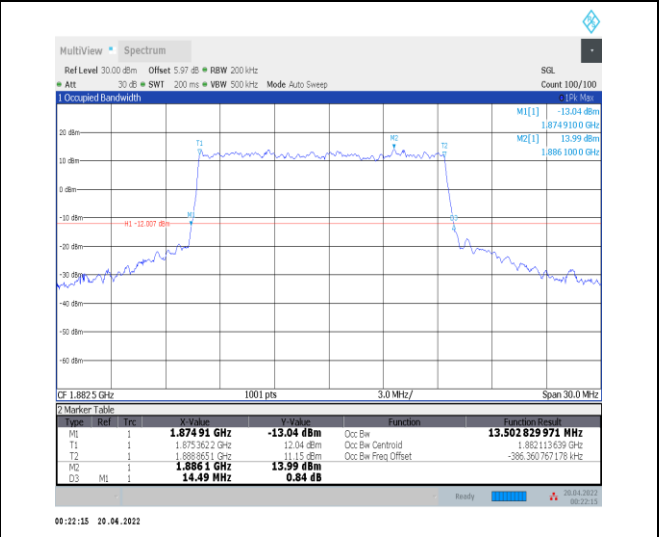
1-N25--15-15-M-1-DFT-QPSK-Outer_Full-75@0-Ant 0-13.503-14.490-≤15-PASS
