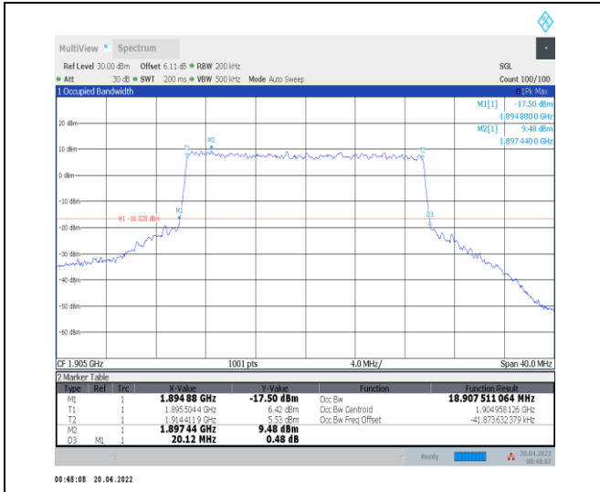
1-N25--15-20-H-6-CP-QPSK-Outer_Full-106@0-Ant 0-18.908-20.120-≤20-PASS
