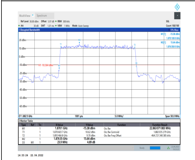
1-N25--15-25-M-2-DFT-PI2BPSK-Outer_Full-128@0 -Ant0-22.863-23.900-≤25-PASS
