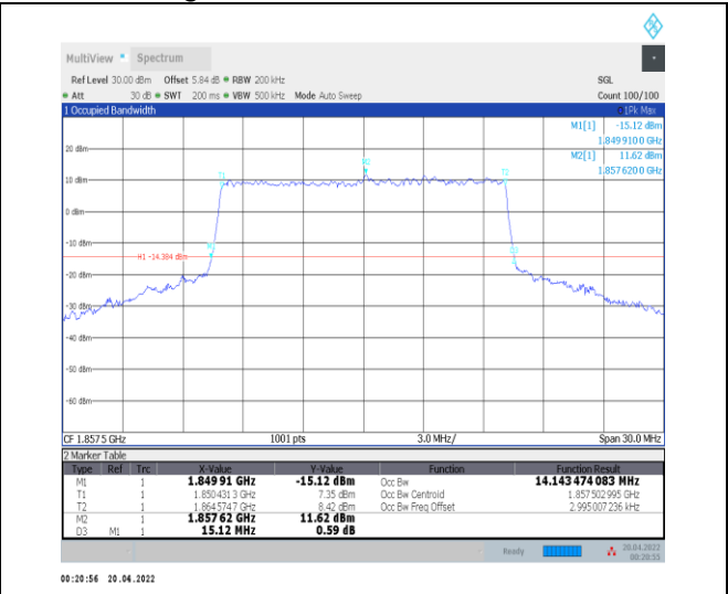
1-N25--15-15-L-8-CP-64QAM-Outer_Full-79@0-Ant 0-14.143-15.120-≤15-PASS
