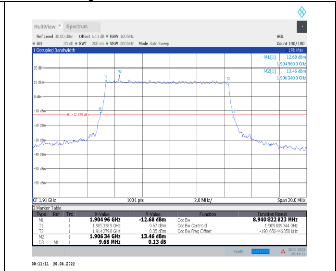
1-N25--15-10-H-1-DFT-QPSK-Outer_Full-50@0-Ant 0-8.941-9.680-≤10-PASS
