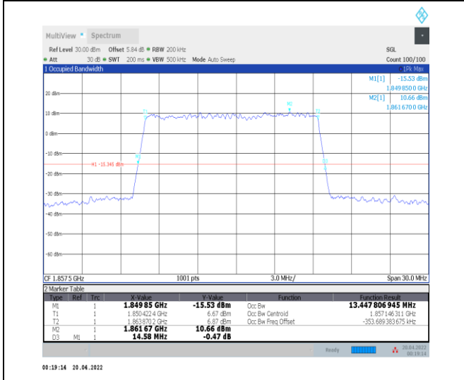
1-N25--15-15-L-5-DFT-256QAM-Outer_Full-75@0-A nt0-13.448-14.580-≤15-PASS
