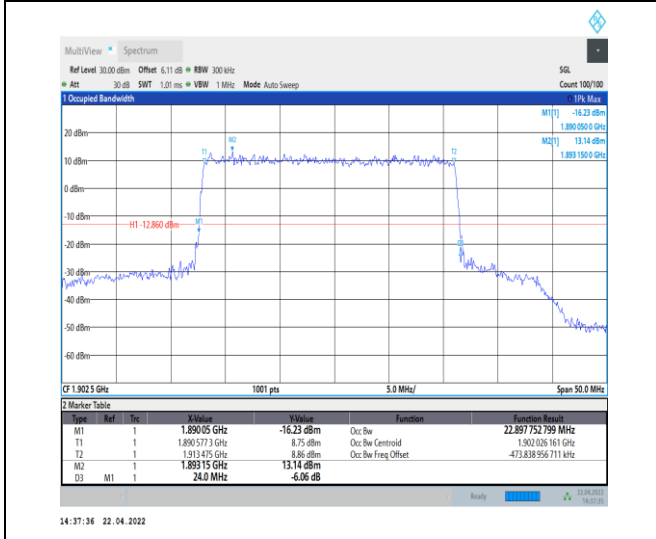
1-N25--15-25-H-1-DFT-QPSK-Outer_Full-128@0-An t0-22.898-24.000-≤25-PASS
