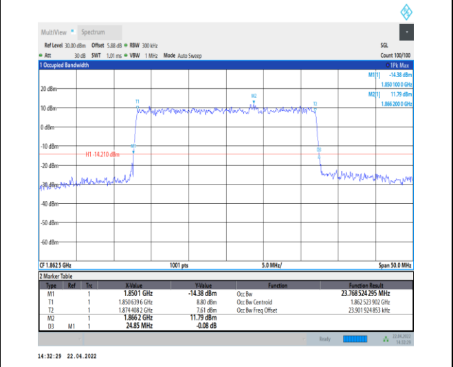
1-N25--15-25-L-8-CP-64QAM-Outer_Full-133@0-An t0-23.769-24.850-<=25-PASS
