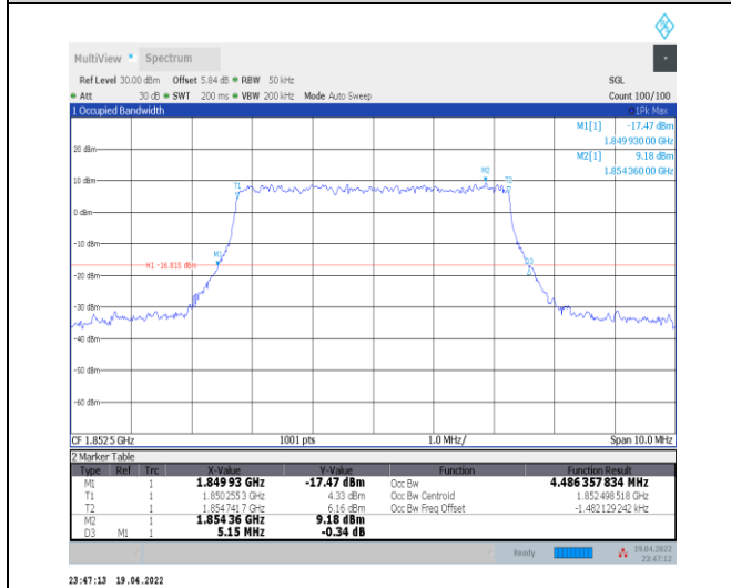
1-N25--15-5-L-7-CP-16QAM-Outer_Full-25@0-Ant0- 4.486-5.150-≤5-PASS
