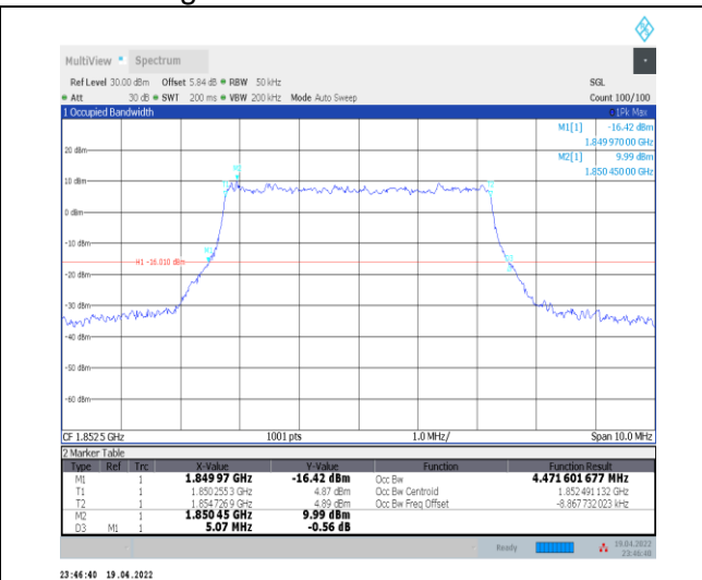
1-N25--15-5-L-6-CP-QPSK-Outer_Full-25@0-Ant0-4 .472-5.070-≤5-PASS
