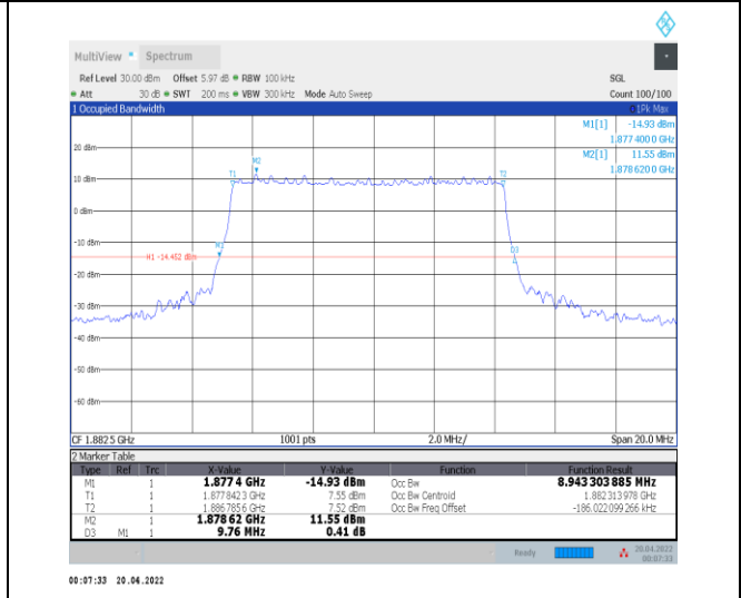
1-N25--15-10-M-4-DFT-64QAM-Outer_Full-50@0-Ant t0-8.943-9.760-≤10-PASS
