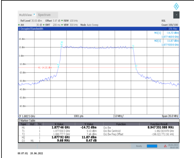
1-N25--15-10-M-3-DFT-16QAM-Outer_Full-50@0-Ant t0-8.947-9.680-≤10-PASS
