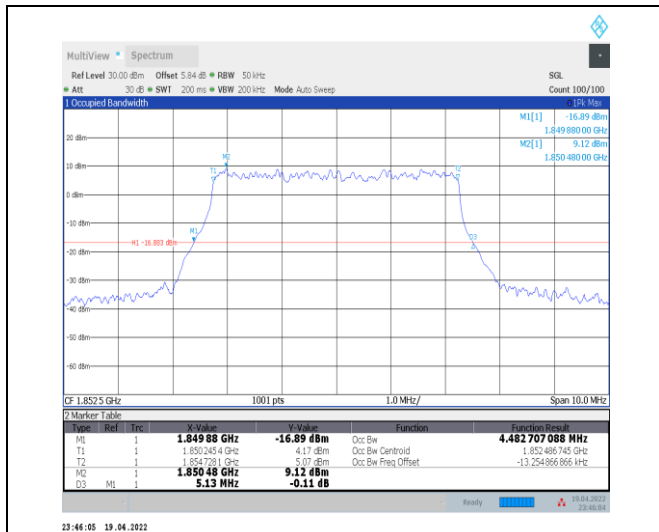
1-N25--15-5-L-5-DFT-256QAM-Outer_Full-25@0-Ant 0-4.483-5.130-≤5-PASS
