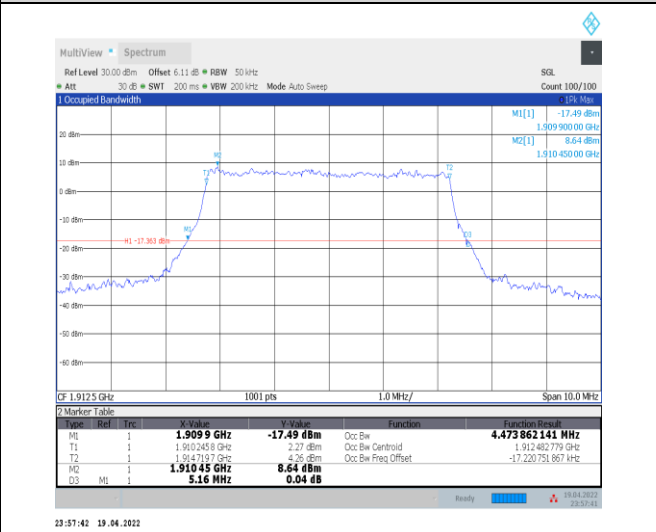
1-N25--15-5-H-6-CP-QPSK-Outer_Full-25@0-Ant0-4 .474-5.160-≤5-PASS
