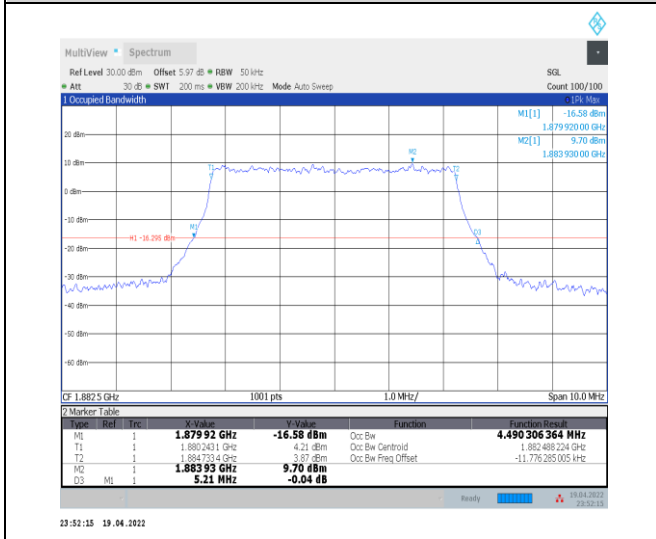
1-N25--15-5-M-6-CP-QPSK-Outer_Full-25@0-Ant0-4.49-5.210-<math>\leq</math>5-PASS
