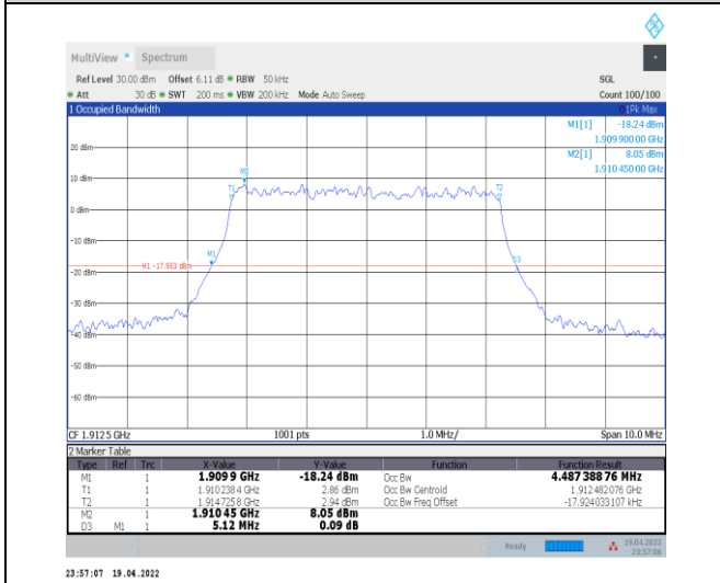
1-N25--15-5-H-5-DFT-256QAM-Outer_Full-25@0-Ant t0-4.487-5.120-≤5-PASS
