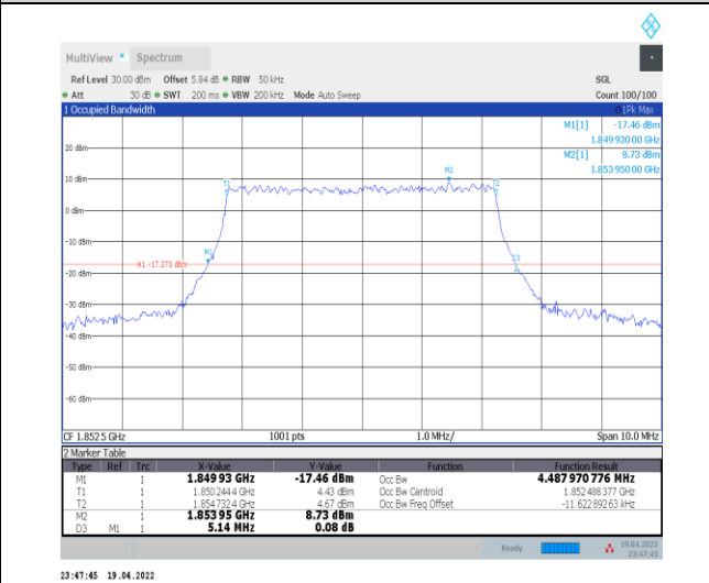
1-N25--15-5-L-8-CP-64QAM-Outer_Full-25@0-Ant0- 4.488-5.140-≤5-PASS
