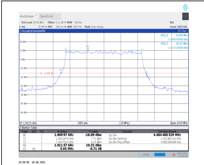
1-N25--15-5-H-3-DFT-16QAM-Outer_Full-25@0-Ant 0-4.484-5.050-≤5-PASS
