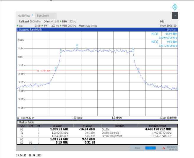
1-N25--15-5-H-4-DFT-64QAM-Outer_Full-25@0-Ant 0-4.486-5.150-≤5-PASS
