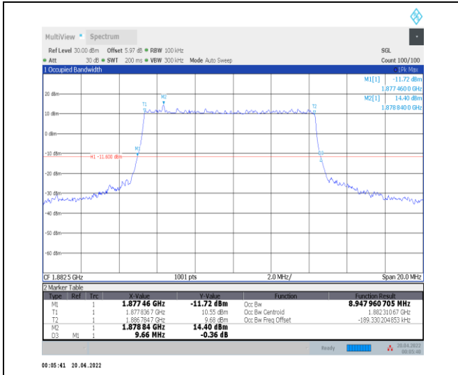
1-N25--15-10-M-1-DFT-QPSK-Outer_Full-50@0-Ant 0-8.948-9.660-≤10-PASS
