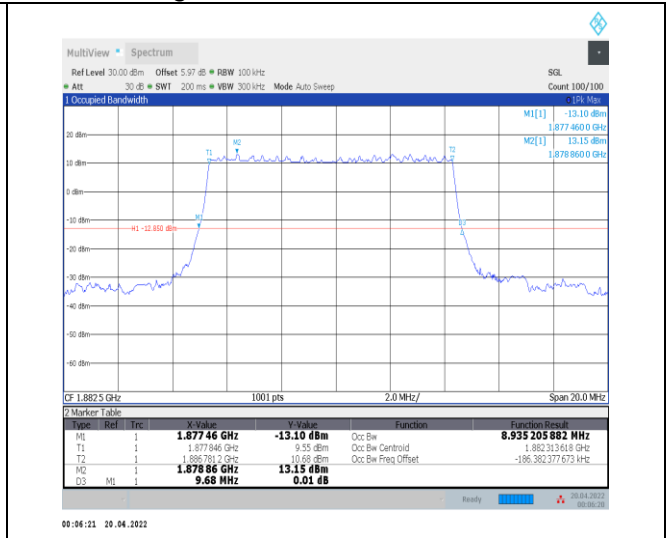
1-N25--15-10-M-2-DFT-PI2BPSK-Outer_Full-50@0-Ant 0-8.935-9.680-≤10-PASS
