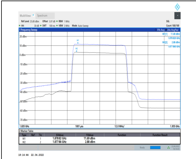
1-N25--15-40-H-1-DFT-256QAM-Outer_Full-216@0-Ant0-8.81-100%-0.00-8.81-PASS-≤13
