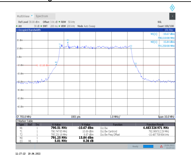
1-N14--15-5-M-1-DFT-QPSK-Outer_Full-25@0-Ant0- 4.483-5.010-≤5-PASS
