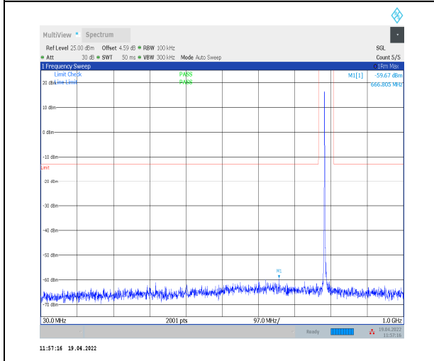
1-N14--15-10-H-1-DFT-PI2BPSK-Inner_1RB_Left-1 @1-30-1000-Ant0--59.67--13-PASS
