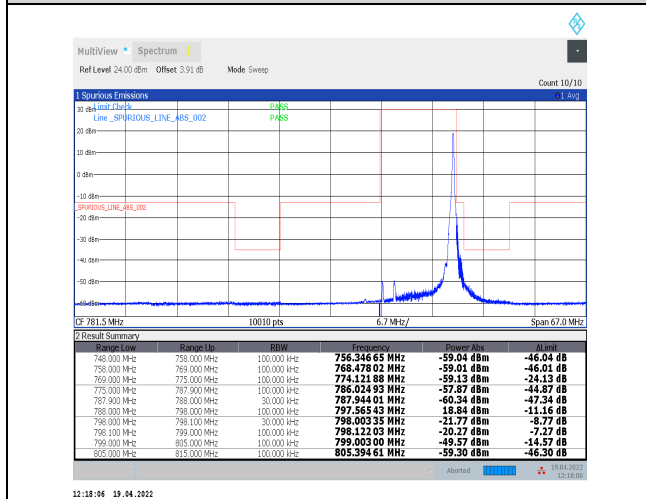
1-N14--15-10-H-5-CP-QPSK-Edge_1RB_Right-1@51-Ant0-PASS-see graph
