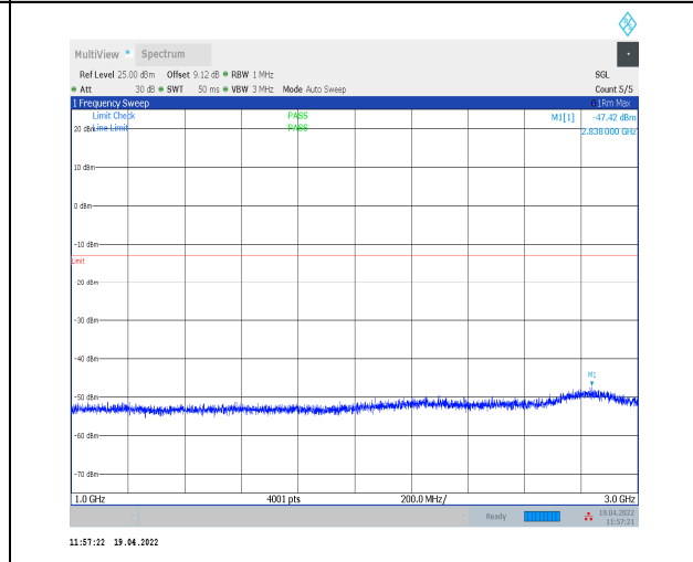
1-N14--15-10-H-1-DFT-PI2BPSK-Inner_1RB_Left-1 @1-1000-3000-Ant0--47.42--13-PASS
