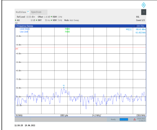
1-N14--15-10-M-1-DFT-PI2BPSK-Inner_1RB_Left-1 @1-0.009-0.15-Ant0--80.41--33-PASS
