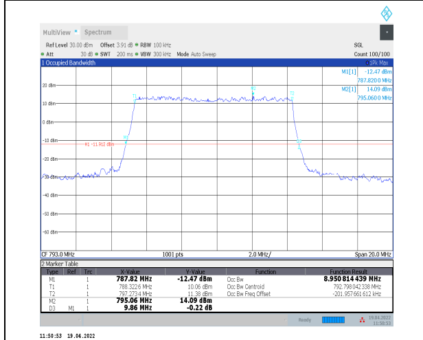
1-N14--15-10-H-2-DFT-PI2BPSK-Outer_Full-50@0-0- Ant0-8.951-9.860-<=10-PASS
