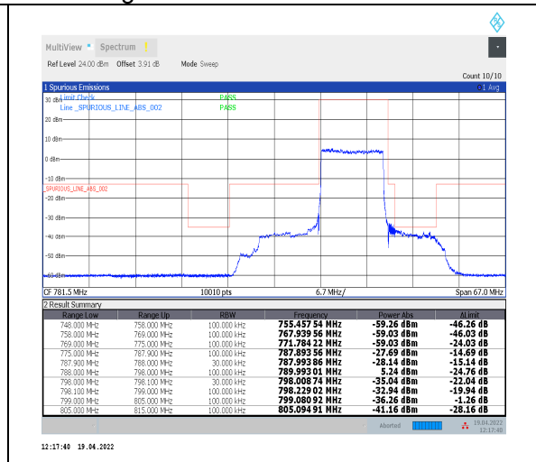
1-N14--15-10-H-3-DFT-PI2BPSK-Outer_Full-50@0-Ant0-PASS-see graph
