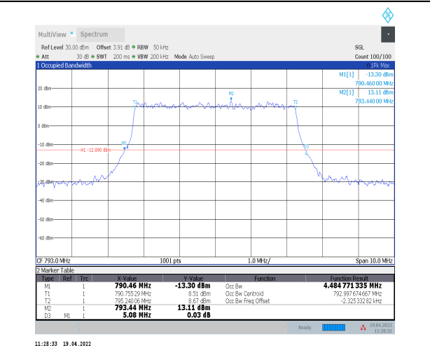
1-N14--15-5-M-3-DFT-16QAM-Outer_Full-25@0-Ant 0-4.485-5.080-≤5-PASS
