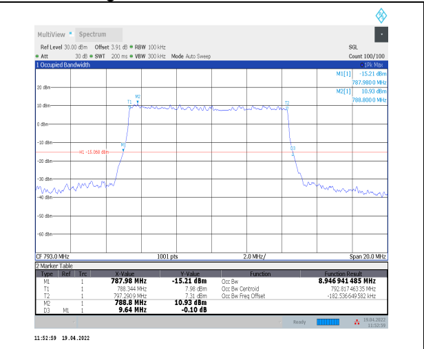
1-N14--15-10-H-5-DFT-256QAM-Outer_Full-50@0-Ant nt0-8.947-9.640-≤10-PASS
