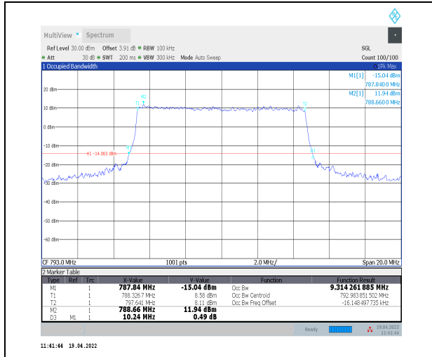
1-N14--15-10-L-6-CP-QPSK-Outer_Full-52@0-Ant0 9.314-10.240≤10-PASS
