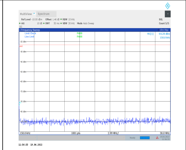
1-N14--15-10-M-1-DFT-PI2BPSK-Inner_1RB_Left-1 @1-0.15-30-Ant0--84.28--23-PASS
