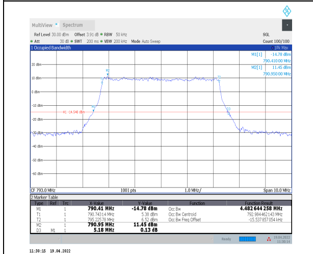
1-N14--15-5-M-6-CP-QPSK-Outer_Full-25@0-Ant0- 4.483-5.180-<math>\leq</math>5-PASS
