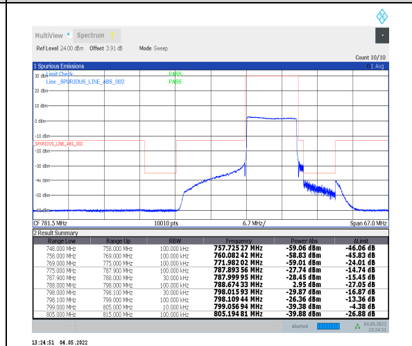
1-N14--15-10-H-6-CP-QPSK-Outer_Full-52@0-Ant0-PASS-see graph
