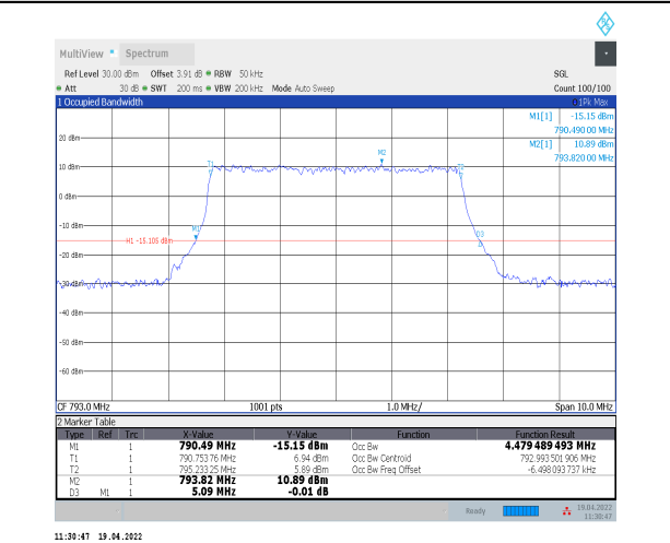
1-N14--15-5-M-7-CP-16QAM-Outer_Full-25@0-Ant0- -4.479-5.090-<math>\leq</math>5-PASS
