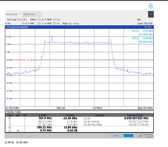
1-N14--15-10-L-1-DFT-QPSK-Outer_Full-50@0-Ant0 -8.96-9.740-≤10-PASS
