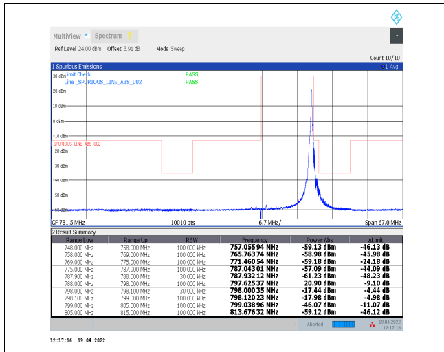
1-N14--15-10-H-2-DFT-PI2BPSK-Edge_1RB_Right-1@51-Ant0-PASS-see graph
