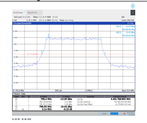
1-N14--15-5-M-5-DFT-256QAM-Outer_Full-25@0-An t0-4.492-5.140-<math>\leq</math>5-PASS
