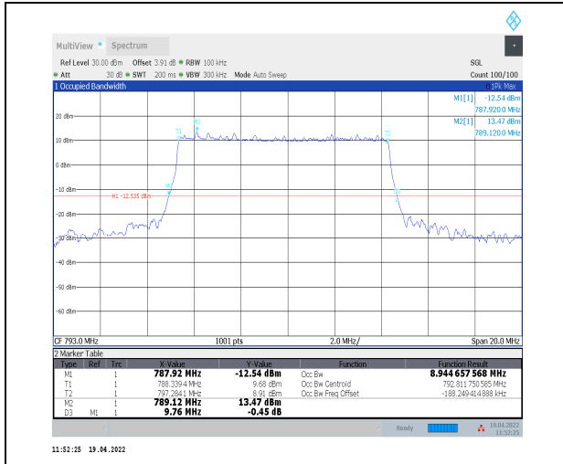
1-N14--15-10-H-4-DFT-64QAM-Outer_Full-50@0-Ant t0-8.945-9.760-≤10-PASS
