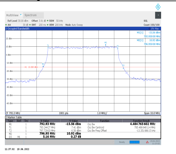
1-N14--15-5-H-8-CP-64QAM-Outer_Full-25@0-Ant0- 4.485-5.160-≤5-PASS
