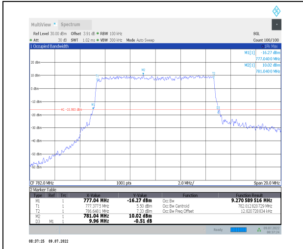
1-N13--15-10-M-6-CP-QPSK-Outer_Full-52@0-Ant0-9.271-9.960-≤10-PASS
