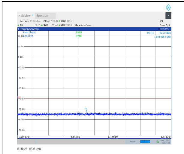
1-N13--15-10-M-1-DFT-PI2BPSK-Inner_1RB_Left-1 @1-1559-1610-Ant0--52.72--40-PASS
