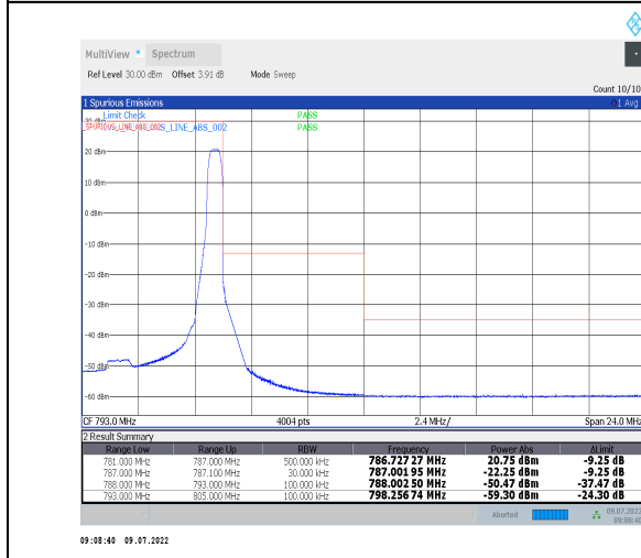
1-N13-PC3-15-5-H-5-CP-QPSK-Edge_1RB_Right-1@24-Ant0-PASS-see graph
