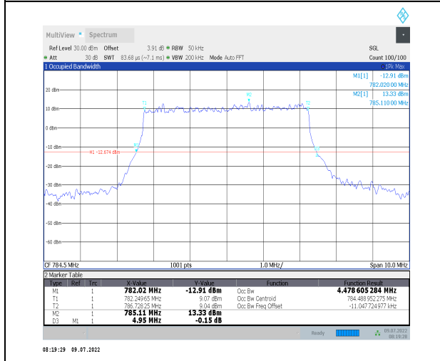
1-N13--15-5-H-1-DFT-QPSK-Outer_Full-25@0-Ant0 4.479-4.950-≤5-PASS
