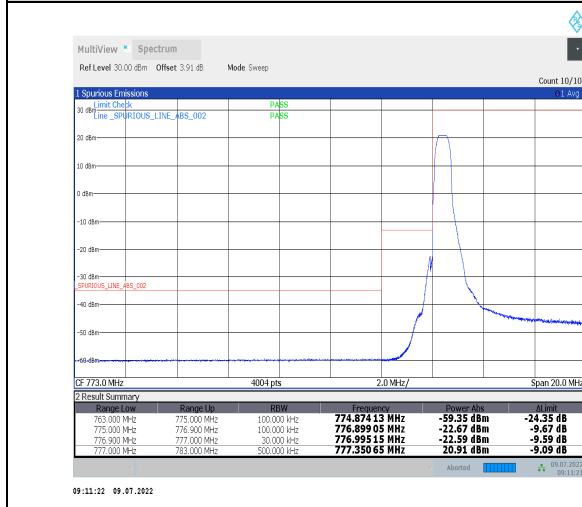
1-N13-PC3-15-10-L-4-CP-QPSK-Edge_1RB_Left-1@0-Ant0-PASS-see graph
