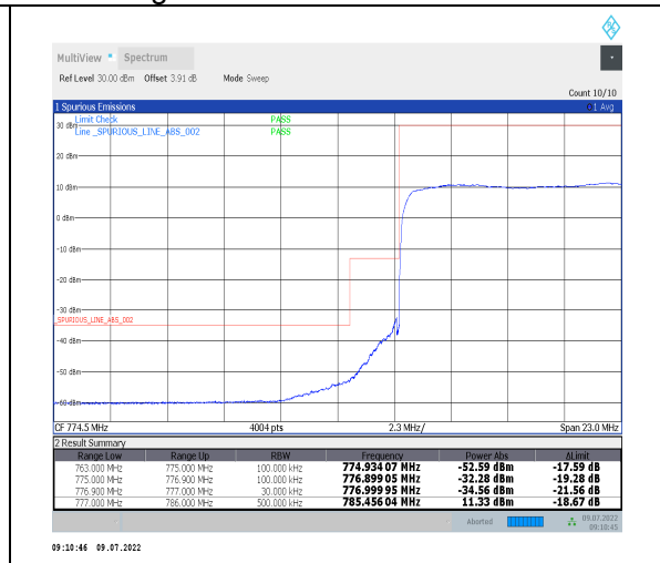
1-N13-PC3-15-10-L-3-DFT-PI2BPSK-Outer_Full-50@0-Ant0-PASS-see graph
