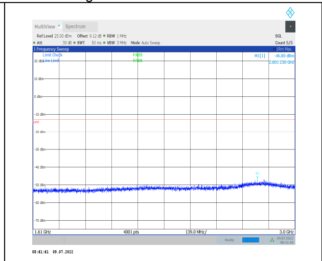
1-N13--15-10-M-1-DFT-PI2BPSK-Inner_1RB_Left-1 @1-1610-3000-Ant0--46.80--13-PASS
