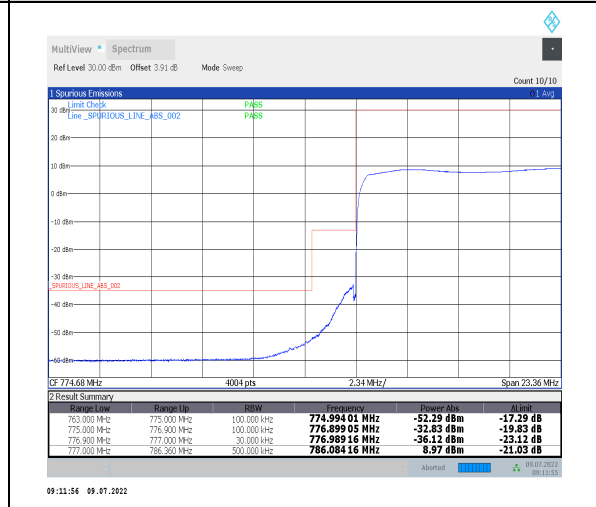
1-N13-PC3-15-10-L-6-CP-QPSK-Outer_Full-52@0-Ant0-PASS-see graph
