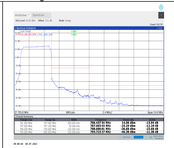
1-N13-PC3-15-5-H-3-DFT-PI2BPSK-Outer_Full-25@0-Ant0-PASS-see graph
