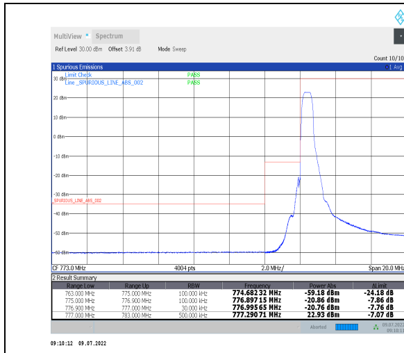
1-N13-PC3-15-10-L-1-DFT-PI2BPSK-Edge_1RB_Left-1@0-Ant0-PASS-see graph
