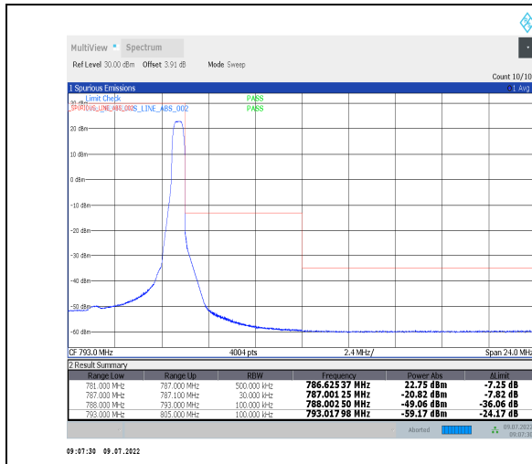
1-N13-PC3-15-5-H-2-DFT-PI2BPSK-Edge_1RB_Right-1@24-Ant0-PASS-see graph
