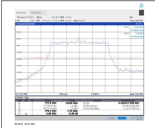
1-N13--15-5-L-9-CP-256QAM-Outer_Full-25@0-Ant0 -4.45-4.960-≤5-PASS
