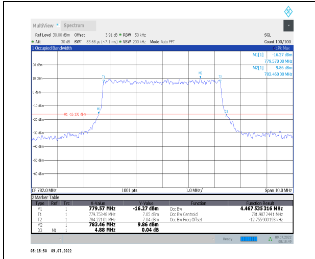
1-N13--15-5-M-8-CP-64QAM-Outer_Full-25@0-Ant0 -4.468-4.880-≤5-PASS
