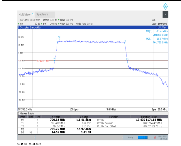
1-N12--15-15-H-3-DFT-16QAM-Outer_Full-75@0-An t0-13.439-14.550≤15-PASS
