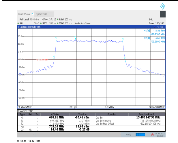
1-N12--15-15-L-1-DFT-QPSK-Outer_Full-75@0-Ant0 -13.488-14.460-≤15-PASS
