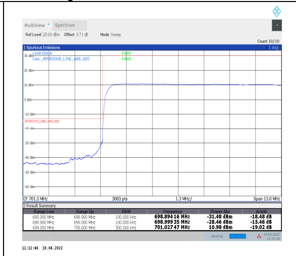
1-N12--15-10-L-3-DFT-PI2BPSK-Outer_Full-50@0-Ant0-PASS-see graph
