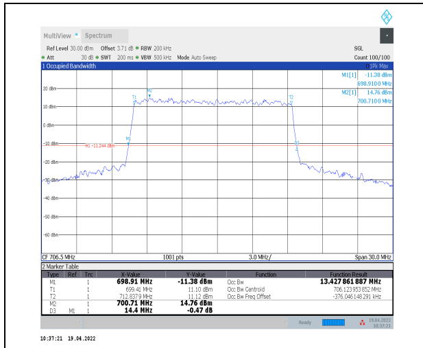
1-N12--15-15-L-3-DFT-16QAM-Outer_Full-75@0-Ant 0-13.428-14.400≤15-PASS
