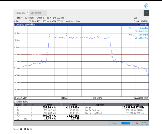
1-N12--15-15-M-1-DFT-QPSK-Outer_Full-75@0-Ant 0-13.492-14.430≤15-PASS
