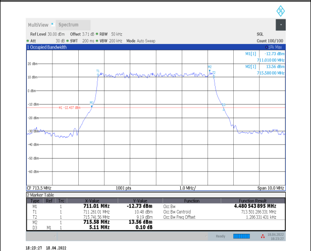
1-N12--15-5-H-2-DFT-PI2BPSK-Outer_Full-25@0-Ant0 4.481-5.110-≤5-PASS
