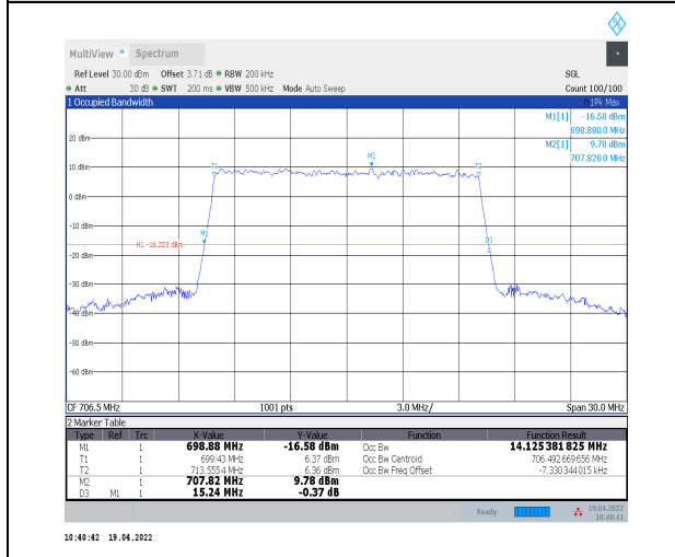
1-N12--15-15-L-9-CP-256QAM-Outer_Full-79@0-Ant 0-14.125-15.240≤15-PASS
