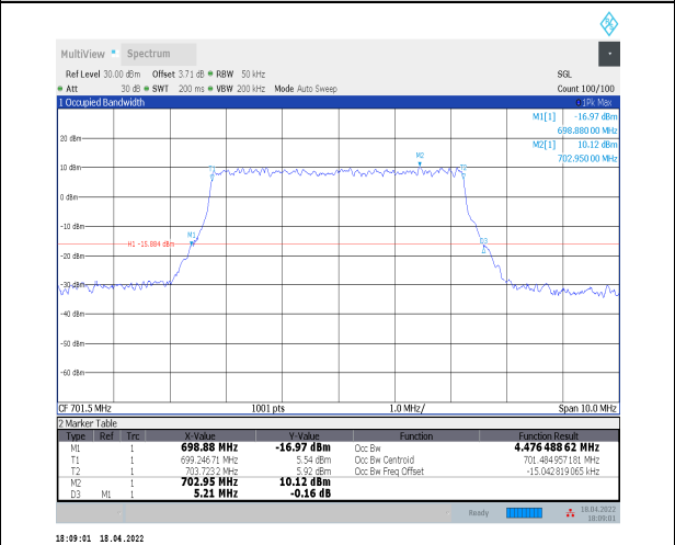
1-N12--15-5-L-8-CP-64QAM-Outer_Full-25@0-Ant0- 4.476-5.210-<math>\leq</math>5-PASS
