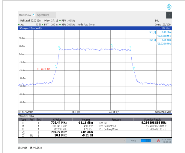
1-N12--15-10-M-9-CP-256QAM-Outer_Full-52@0-An t0-9.285-10.100-<=10-PASS
