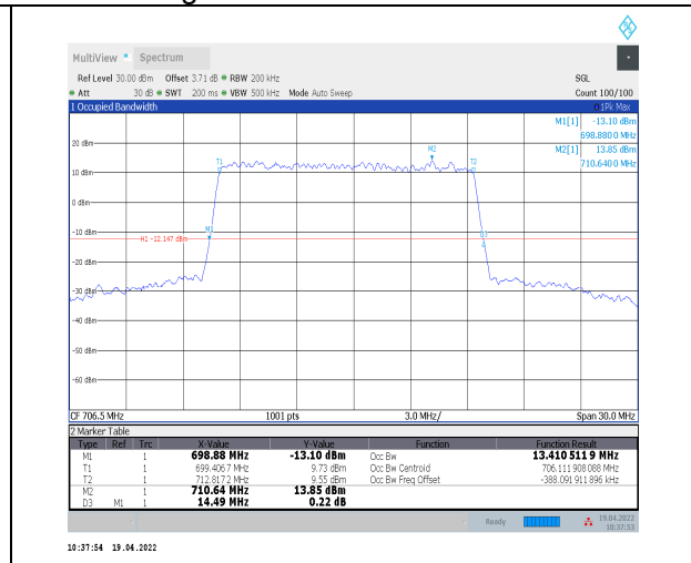
1-N12--15-15-L-4-DFT-64QAM-Outer_Full-75@0-Ant t0-13.411-14.490≤15-PASS
