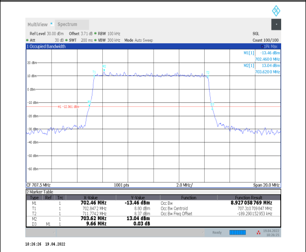
1-N12--15-10-M-4-DFT-64QAM-Outer_Full-50@0-A nt0-8.927-9.660-<=10-PASS
