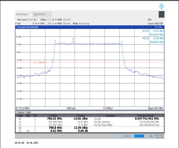
1-N12--15-10-H-3-DFT-16QAM-Outer_Full-50@0-An t0-8.948-9.620-<=10-PASS
