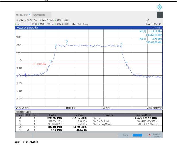
1-N12--15-5-L-6-CP-QPSK-Outer_Full-25@0-Ant0-4 .47-5.140-<math>\leq</math>5-PASS
