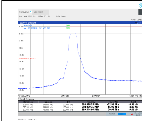
1-N12--15-10-L-4-CP-QPSK-Edge_1RB_Left-1@0-Ant0-PASS-see graph
