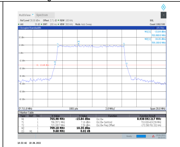
1-N12--15-10-H-5-DFT-256QAM-Outer_Full-50@0-A nt0-8.939-9.680-≤10-PASS
