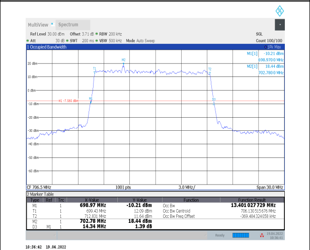
1-N12--15-15-L-2-DFT-PI2BPSK-Outer_Full-75@0-A n0-13.401-14.340-≤15-PASS
