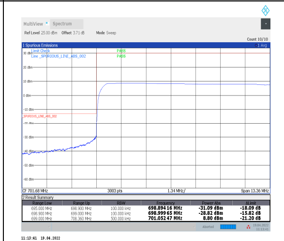
1-N12--15-10-L-6-CP-QPSK-Outer_Full-52@0-Ant0-PASS-see graph
