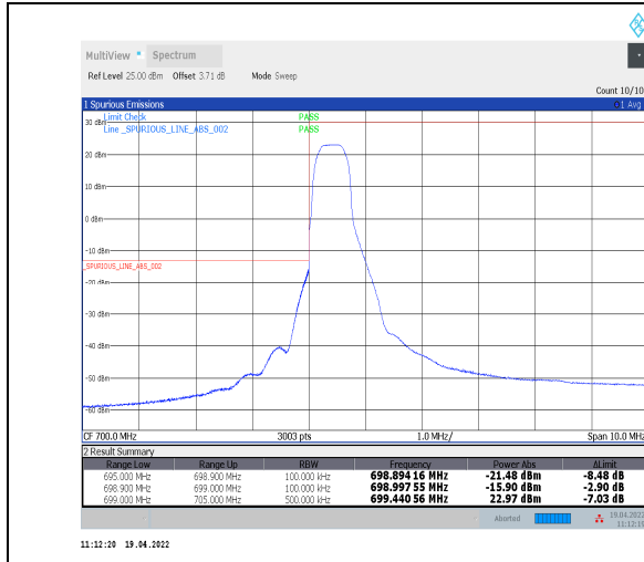
1-N12--15-10-L-1-DFT-PI2BPSK-Edge_1RB_Left-1@0-Ant0-PASS-see graph
