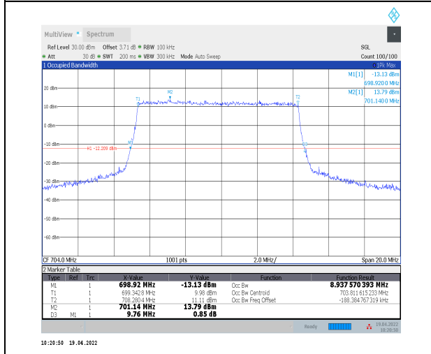
1-N12--15-10-L-4-DFT-64QAM-Outter_Full-50@0-Ant 0-8.938-9.760-≤10-PASS
