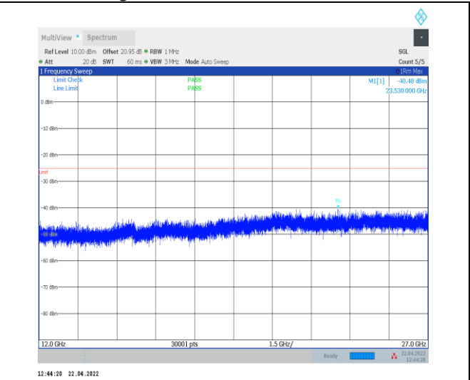
1-N7--15-40-L-1-DFT-PI2BPSK-Inner_1RB_Left-1 @ 1 -12000-27000-Ant0--40.48--25-PASS
