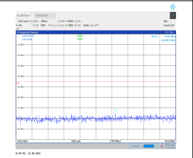
1-N7--15-40-M-1-DFT-PI2BPSK-Inner_1RB_Left-1 @ 1-0.15-30-Ant0--74.86--45-PASS
