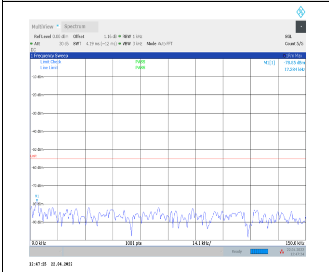
1-N7--15-40-M-1-DFT-PI2BPSK-Inner_1RB_Left-1 @ 1-0.009-0.15-Ant0--78.85--55-PASS
