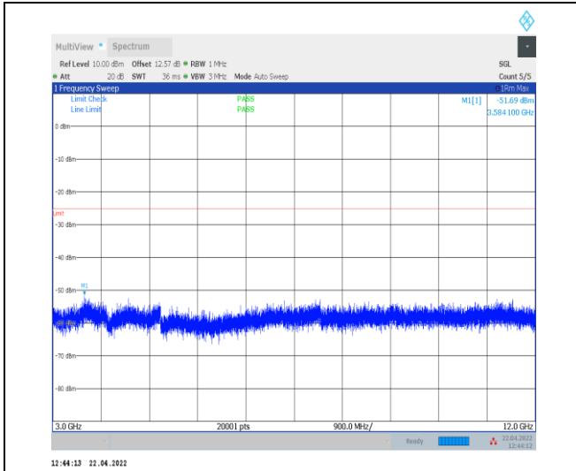
1-N7--15-40-L-1-DFT-PI2BPSK-Inner_1RB_Left-1 @ 1-3000-12000-Ant0--51.69--25-PASS
