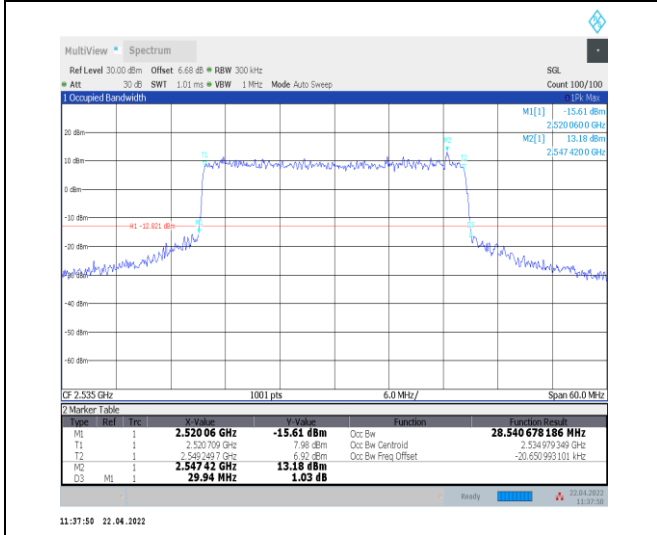
1-N7--15-30-M-7-CP-16QAM-Outer_Full-160@0-Ant 0-28.541-29.940-≤30-PASS
