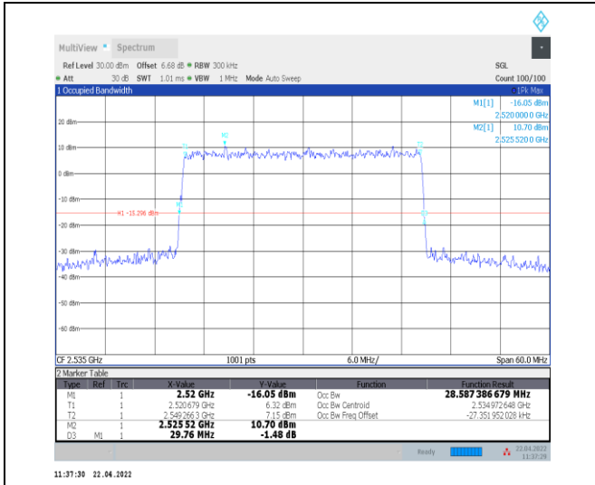
1-N7--15-30-M-5-DFT-256QAM-Outer_Full-160@0-A nt0-28.587-29.760-≤30-PASS
