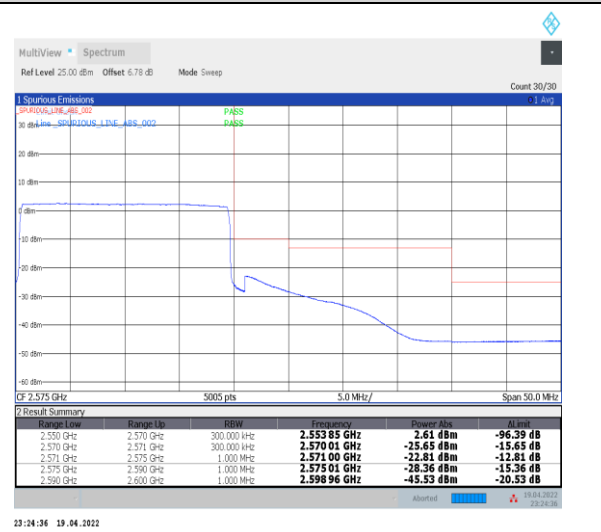
1-N7--15-20-H-6-CP-QPSK-Outer_Full-106@0-Ant0-PASS-see graph
