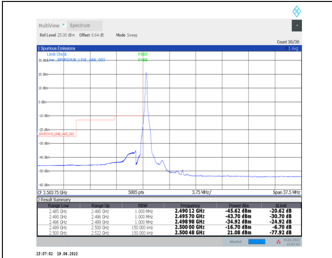
1-N7--15-15-L-1-DFT-PI2BPSK-Edge_1RB_Left-1@0-Ant0-PASS-see graph
