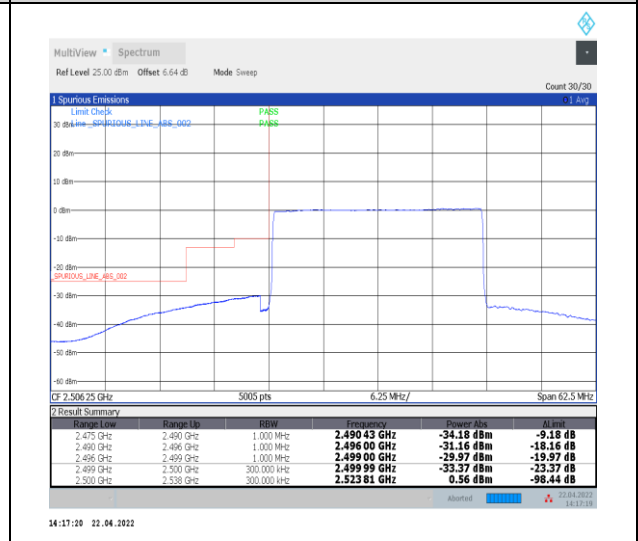
1-N7--15-25-L-6-CP-QPSK-Outer_Full-133@0-Ant0-PASS-see graph
