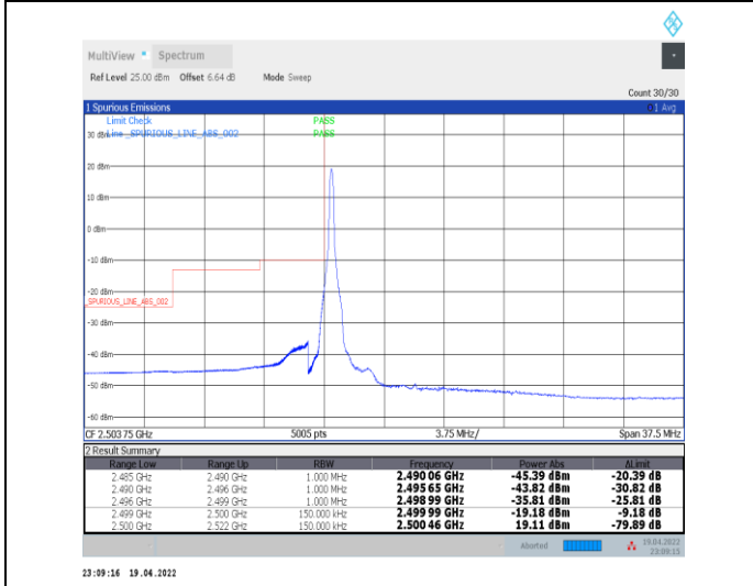
1-N7--15-15-L-4-CP-QPSK-Edge_1RB_Left-1@0-Ant0-PASS-see graph
