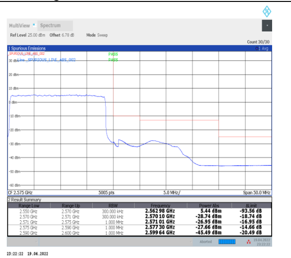
1-N7--15-20-H-3-DFT-PI2BPSK-Outer_Full-100@0-Ant0-PASS-see graph
