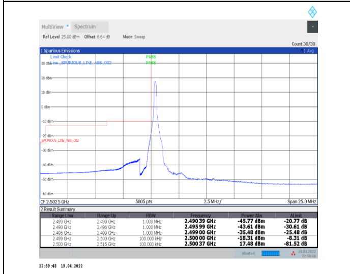
1-N7--15-10-L-4-CP-QPSK-Edge_1RB_Left-1@0-Ant0-PASS-see graph
