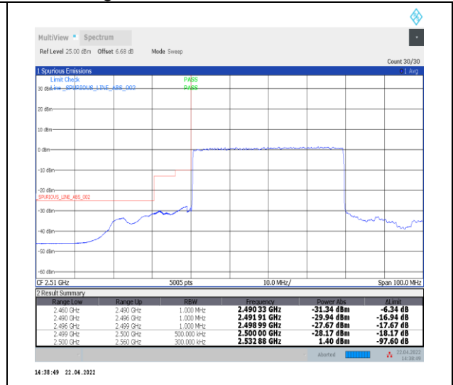
1-N7--15-40-L-3-DFT-PI2BPSK-Outer_Full-216@0-Ant0-PASS-see graph
