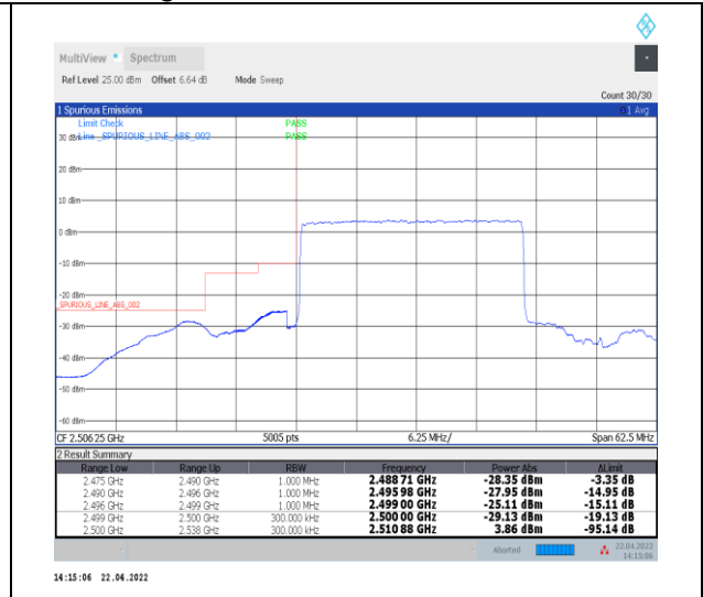
1-N7--15-25-L-3-DFT-PI2BPSK-Outer_Full-128@0-Ant0-PASS-see graph
