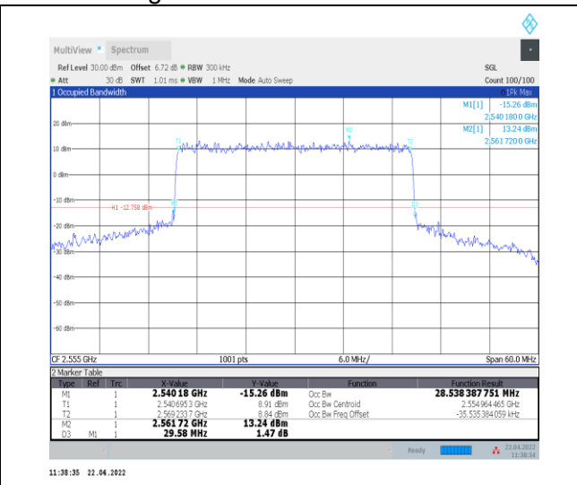
1-N7--15-30-H-1-DFT-QPSK-Outer_Full-160@0-Ant 0-28.539-29.580-<=30-PASS
