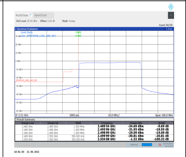
1-N7--15-40-L-6-CP-QPSK-Outer_Full-216@0-Ant0-PASS-see graph
