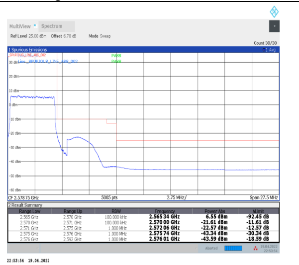
1-N7--15-5-H-3-DFT-PI2BPSK-Outer_Full-25@0-Ant0-PASS-see graph
