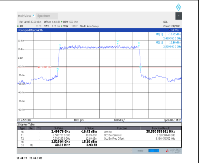
1-N7--15-40-L-2-DFT-PI2BPSK-Outer_Full-216@0-A nt0-38.552-40.320-≤40-PASS
