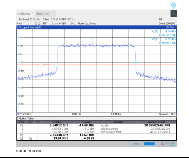
1-N7--15-30-H-3-DFT-16QAM-Outer_Full-160@0-Ant t0-28.565-29.640-<=30-PASS
