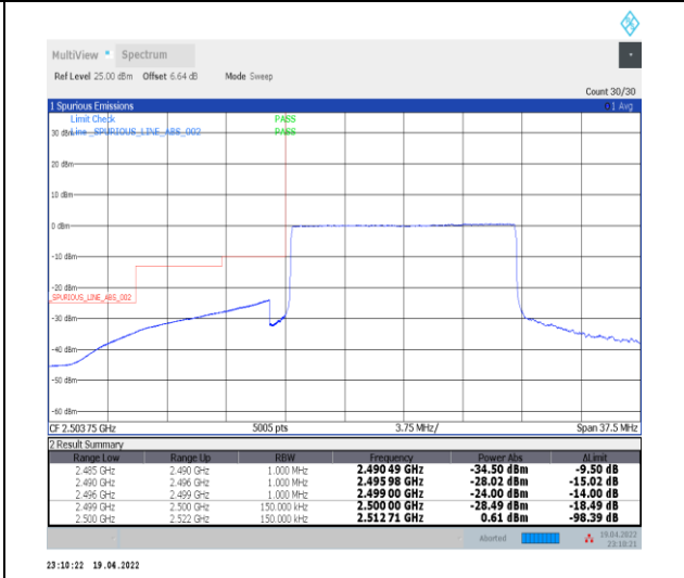
1-N7--15-15-L-6-CP-QPSK-Outer_Full-79@0-Ant0-PASS-see graph
