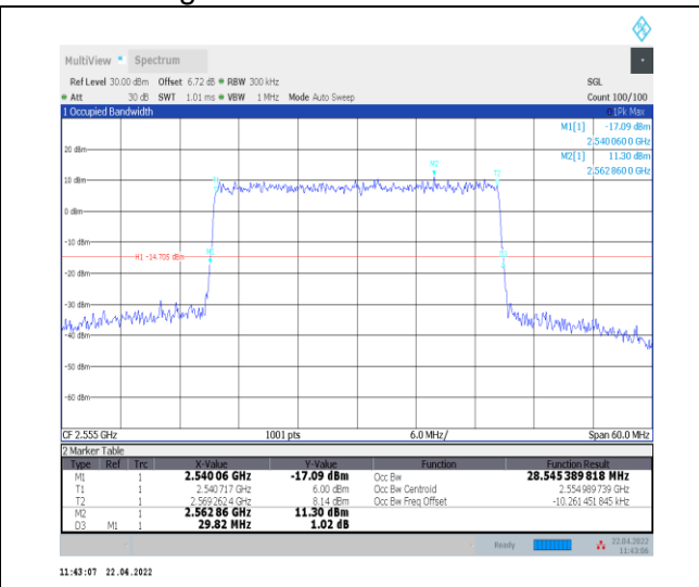
1-N7--15-30-H-5-DFT-256QAM-Outer_Full-160@0-Ant0-28.549-29.820-≤30-PASS
