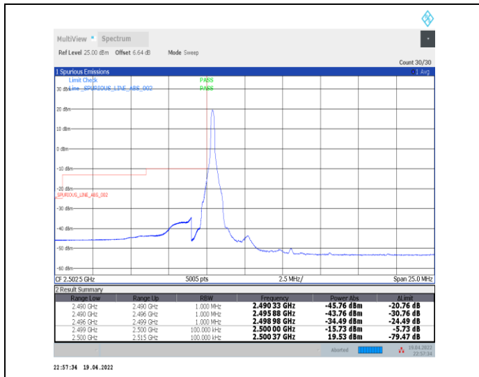
1-N7--15-10-L-1-DFT-PI2BPSK-Edge_1RB_Left-1@0-Ant0-PASS-see graph
