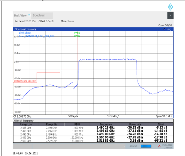
1-N7--15-15-L-3-DFT-PI2BPSK-Outer_Full-75@0-Ant0-PASS-see graph
