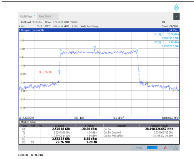
1-N7--15-30-M-9-CP-256QAM-Outer_Full-160@0-A nt0-28.5-29.760-<=30-PASS
