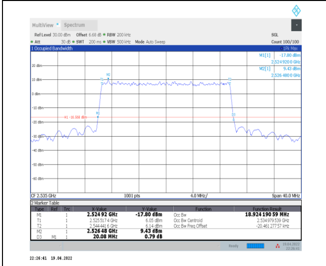
1-N7--15-20-M-9-CP-256QAM-Outer_Full-106@0-A nt0-18.924-20.080-≤20-PASS
