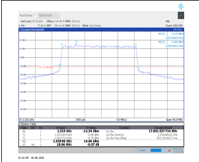
1-N7--15-20-M-1-DFT-QPSK-Outer_Full-100@0-Ant 0-17.852-18.960-≤20-PASS
