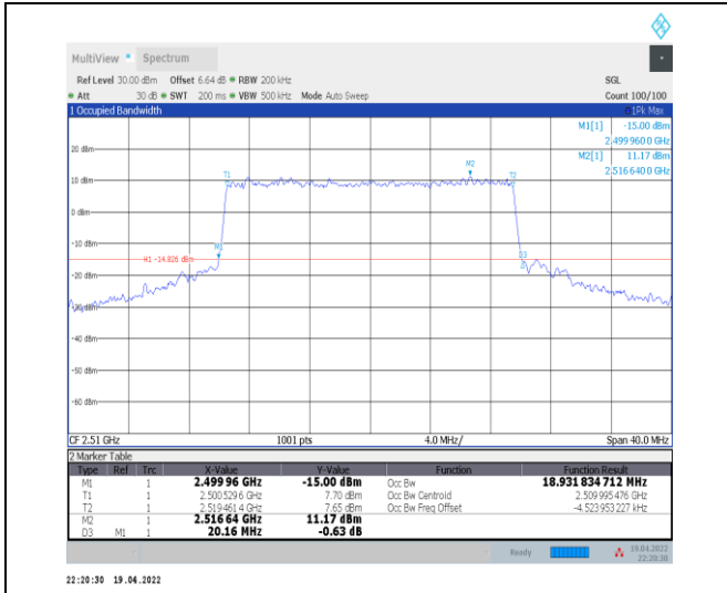
1-N7--15-20-L-8-CP-64QAM-Outer_Full-106@0-Ant 0-18.932-20.160-≤20-PASS
