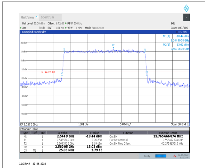
1-N7--15-25-H-7-CP-16QAM-Outer_Full-133@0-Ant 0-23.766-25.050-≤25-PASS
