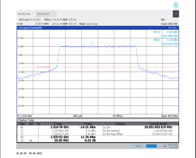
1-N7--15-20-M-6-CP-QPSK-Outer_Full-106@0-Ant0 -18.951-20.360-≤20-PASS
