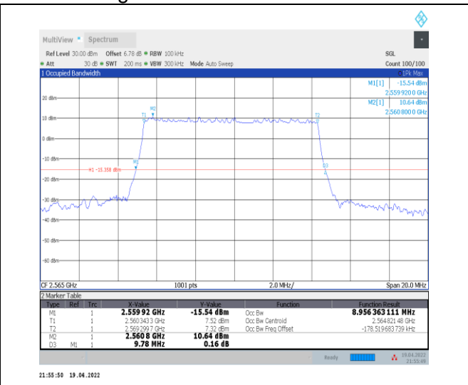
1-N7--15-10-H-5-DFT-256QAM-Outer_Full-50@0-Ant t0-8.956-9.780≤10-PASS
