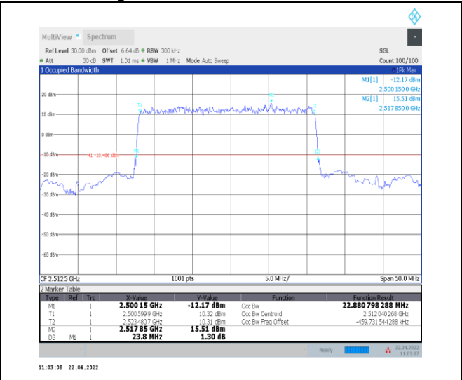
1-N7--15-25-L-2-DFT-PI2BPSK-Outer_Full-128@0-Ant0 -22.881-23.800-≤25-PASS
