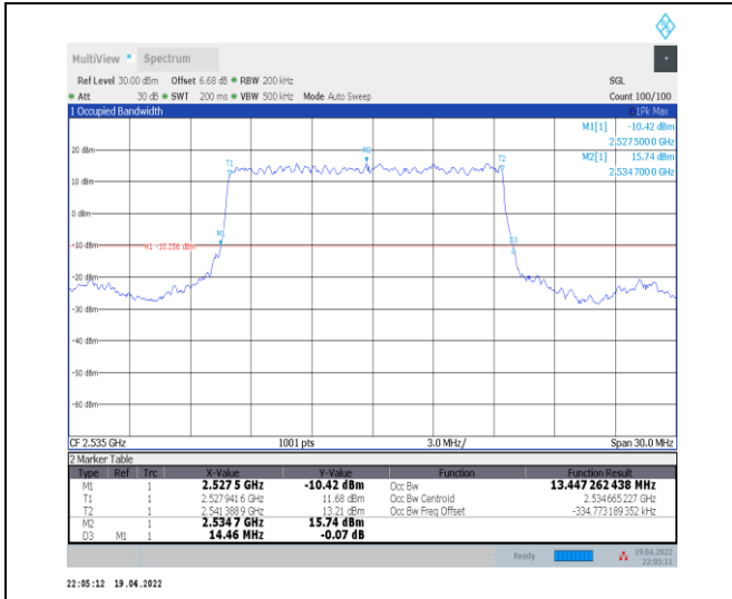
1-N7--15-15-M-2-DFT-PI2BPSK-Outer_Full-75@0-A nt0-13.447-14.460-≤15-PASS
