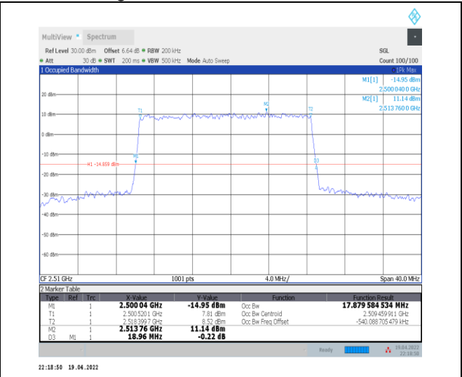
1-N7--15-20-L-5-DFT-256QAM-Outer_Full-100@0-A nt0-17.88-18.960-≤20-PASS
