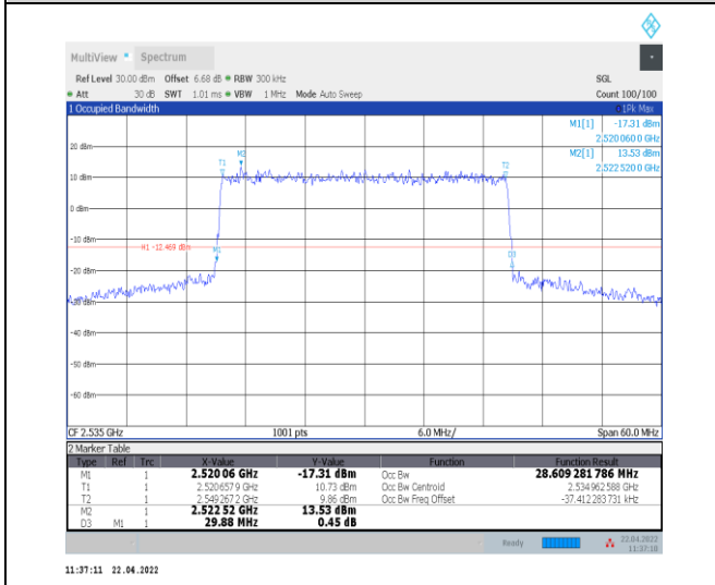
1-N7--15-30-M-3-DFT-16QAM-Outer_Full-160@0-Ant t0-28.61-29.880-≤30-PASS
