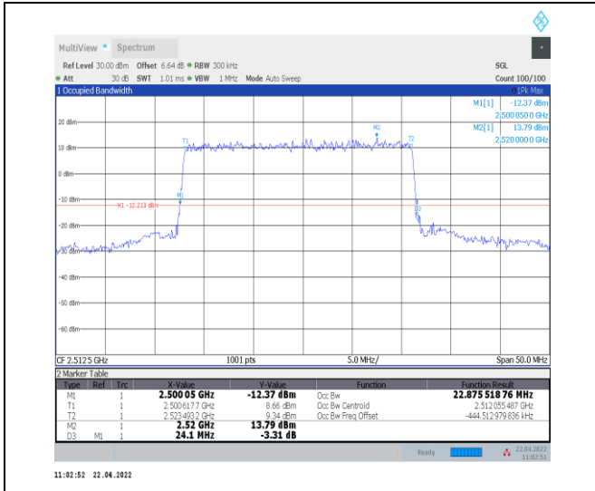
1-N7--15-25-L-1-DFT-QPSK-Outer_Full-128@0-Ant0 -22.876-24.100-≤25-PASS
