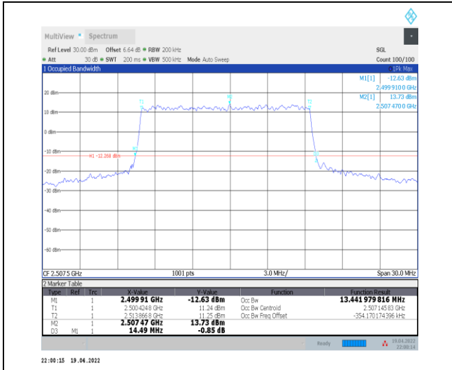
1-N7--15-15-L-3-DFT-16QAM-Outer_Full-75@0-Ant0 -13.442-14.490-≤15-PASS
