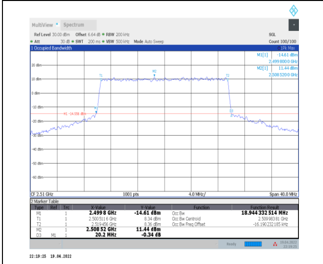
1-N7--15-20-L-6-CP-QPSK-Outer_Full-106@0-Ant0- 18.944-20.200-≤20-PASS
