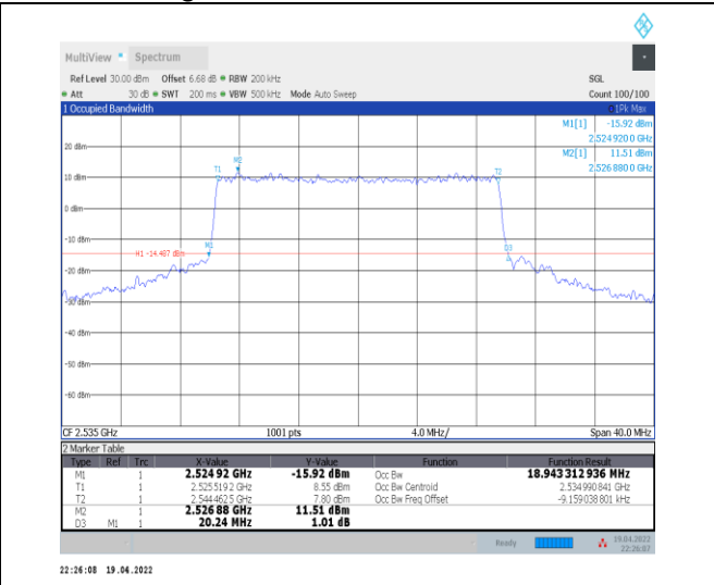
1-N7--15-20-M-8-CP-64QAM-Outer_Full-106@0-Ant 0-18.943-20.240-≤20-PASS
