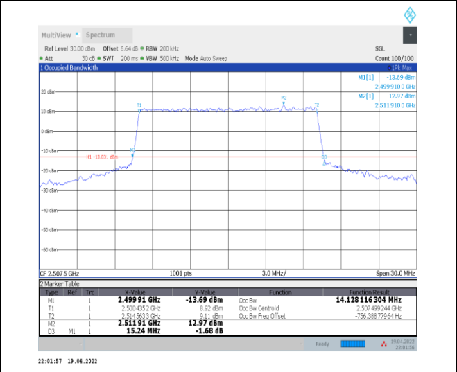
1-N7--15-15-L-6-CP-QPSK-Outer_Full-79@0-Ant0-1 4.128-15.240-≤15-PASS
