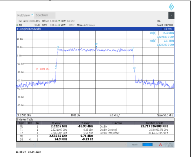
1-N7--15-25-M-9-CP-256QAM-Outer_Full-133@0-Ant 0-23.718-24.900-≤25-PASS
