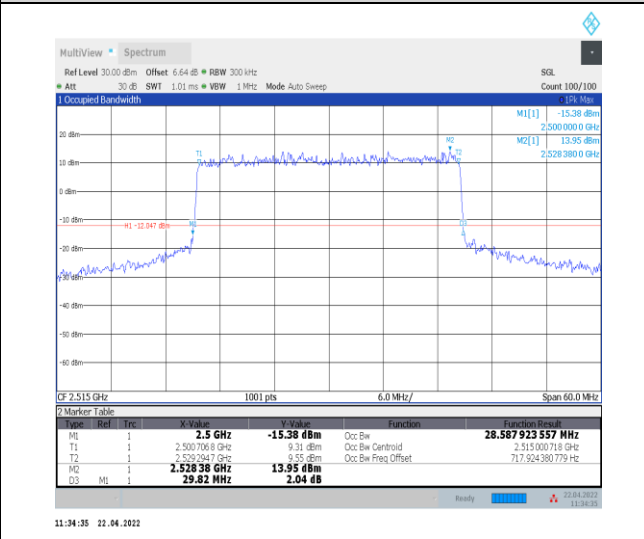
1-N7--15-30-L-1-DFT-QPSK-Outer_Full-160@0-Ant0 -28.589-29.820-≤30-PASS
