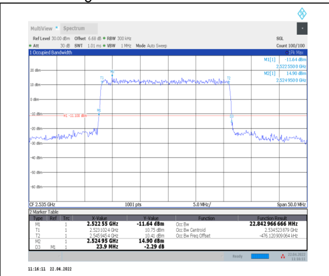
1-N7--15-25-M-1-DFT-QPSK-Outer_Full-128@0-Ant 0-22.843-23.900-<=25-PASS
