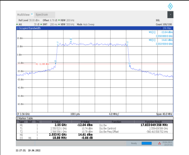
1-N7--15-20-H-1-DFT-QPSK-Outer_Full-100@0-Ant 0-17.833-18.880-≤20-PASS
