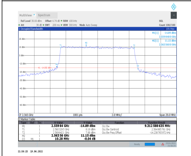
1-N7--15-10-H-6-CP-QPSK-Outer_Full-52@0-Ant0-9 .313-10.280≤10-PASS
