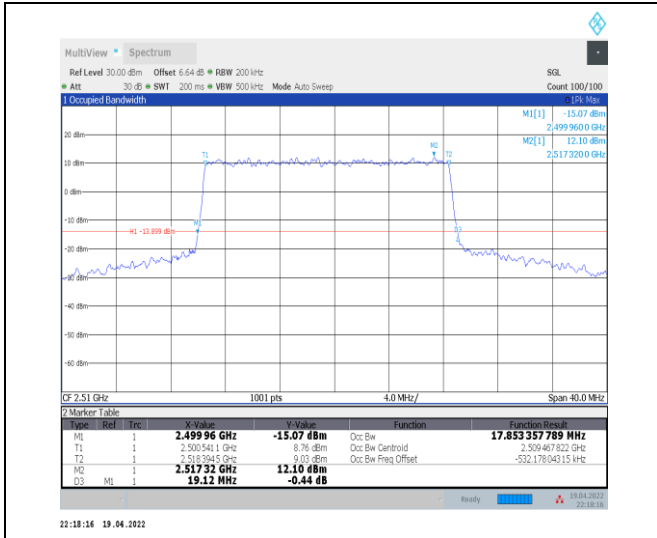
1-N7--15-20-L-4-DFT-64QAM-Outer_Full-100@0-Ant 0-17.853-19.120-≤20-PASS
