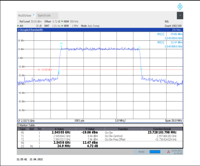
1-N7--15-25-H-6-CP-QPSK-Outer_Full-133@0-Ant0- 23.728-24.900-<=25-PASS
