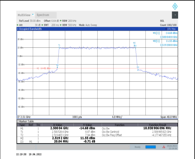
1-N7--15-20-L-7-CP-16QAM-Outer_Full-106@0-Ant 0-18.939-20.040-≤20-PASS
