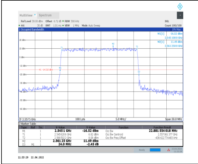
1-N7--15-25-H-5-DFT-256QAM-Outer_Full-128@0-A nt0-22.882-24.000-<=25-PASS
