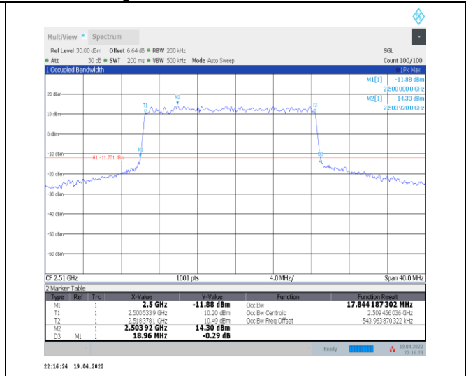
1-N7--15-20-L-1-DFT-QPSK-Outer_Full-100@0-Ant0 -17.844-18.960≤20-PASS
