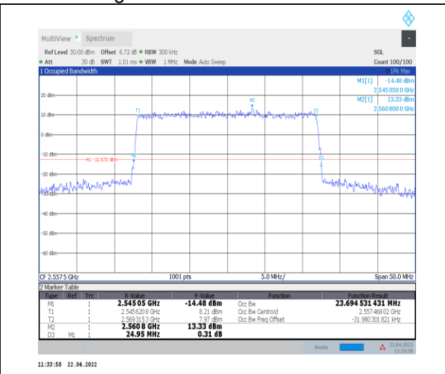
1-N7--15-25-H-8-CP-64QAM-Outer_Full-133@0-Ant 0-23.695-24.950-≤25-PASS
