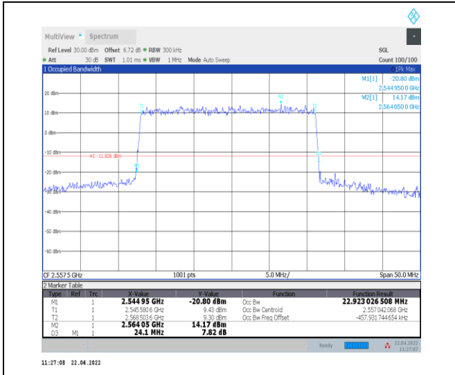
1-N7--15-25-H-3-DFT-16QAM-Outer_Full-128@0-An t0-22.923-24.100-<=25-PASS
