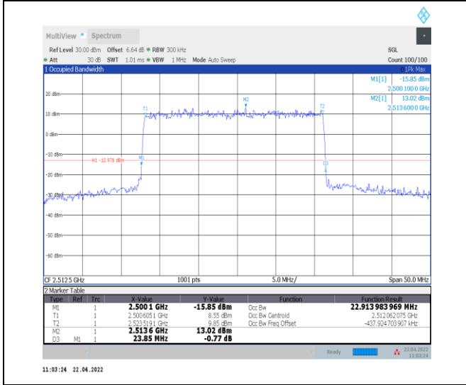
1-N7--15-25-L-3-DFT-16QAM-Outer_Full-128@0-Ant0 0-22.914-23.850-≤25-PASS
