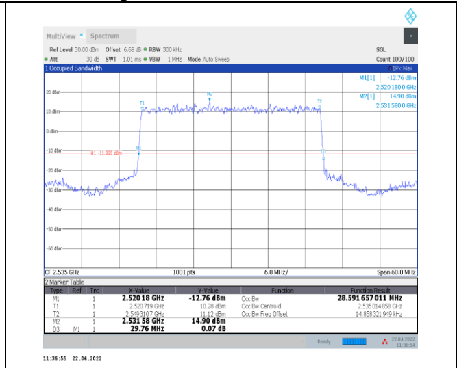
1-N7--15-30-M-2-DFT-PI2BPSK-Outer_Full-160@0-Ant 0-28.592-29.760-≤30-PASS
