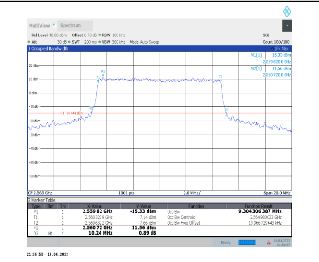
1-N7--15-10-H-7-CP-16QAM-Outer_Full-52@0-Ant0- 9.304-10.240≤10-PASS
