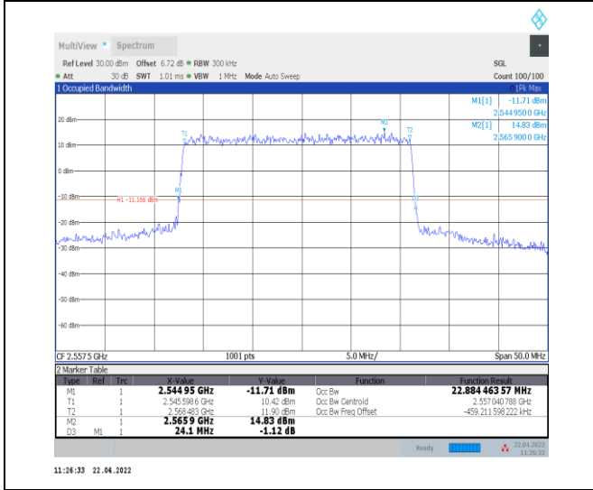
1-N7--15-25-H-1-DFT-QPSK-Outer_Full-128@0-Ant 0-22.884-24.100-≤25-PASS
