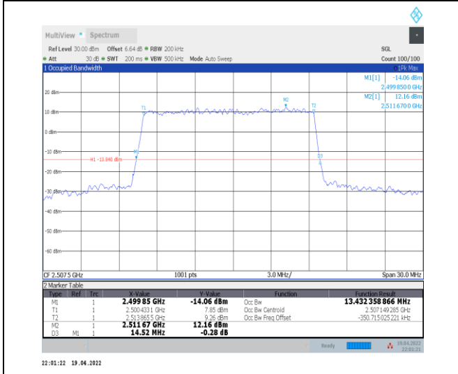
1-N7--15-15-L-5-DFT-256QAM-Outer_Full-75@0-Ant0 0-13.432-14.520-≤15-PASS
