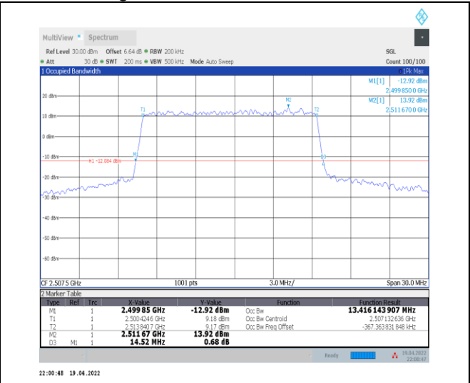
1-N7--15-15-L-4-DFT-64QAM-Outer_Full-75@0-Ant0 -13.416-14.520-≤15-PASS
