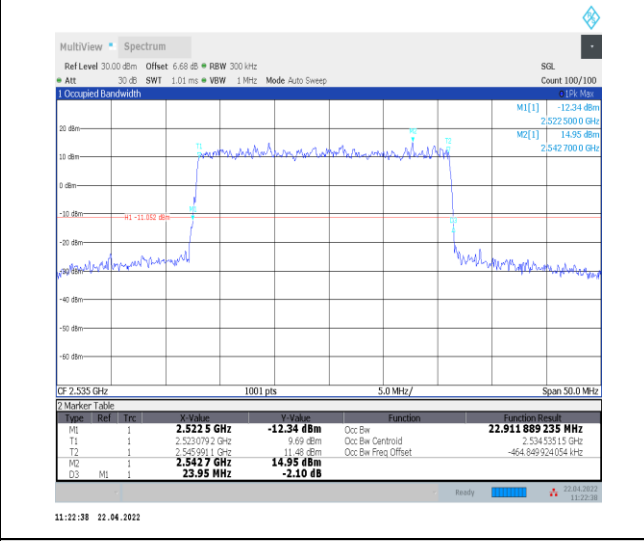
1-N7--15-25-M-3-DFT-16QAM-Outer_Full-128@0-Ant t0-22.912-23.950-<=25-PASS
