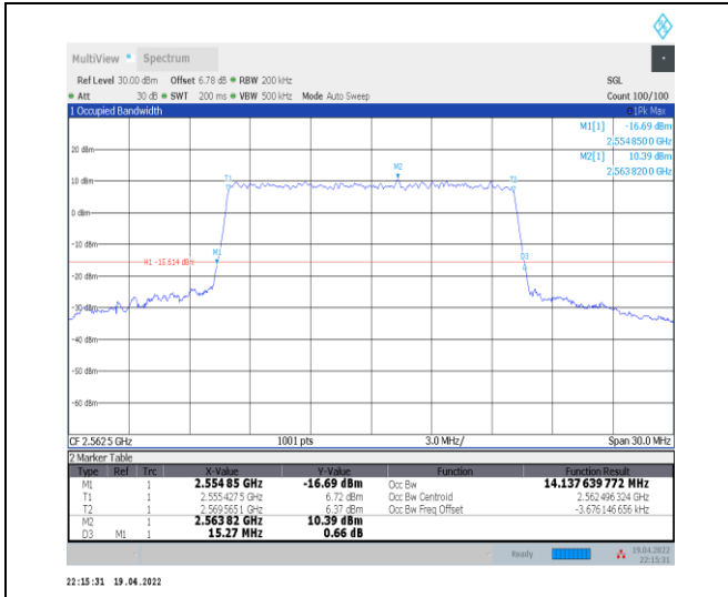
1-N7--15-15-H-CP-256QAM-Outer_Full-79@0-Ant 0-14.138-15.270≤15-PASS
