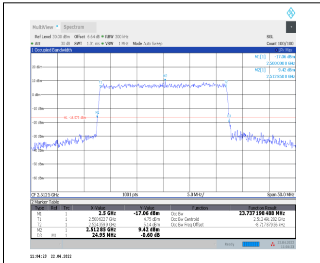
1-N7--15-25-L-9-CP-256QAM-Outer_Full-133@0-An t0-23.737-24.950-<=25-PASS
