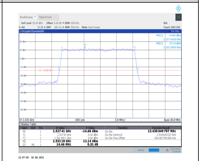
1-N7--15-15-M-5-DFT-256QAM-Outer_Full-75@0-Ant 0-13.43-14.460-≤15-PASS
