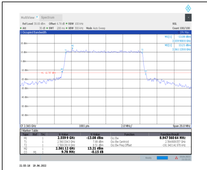
1-N7--15-10-H-4-DFT-64QAM-Outer_Full-50@0-Ant 0-8.948-9.780≤10-PASS
