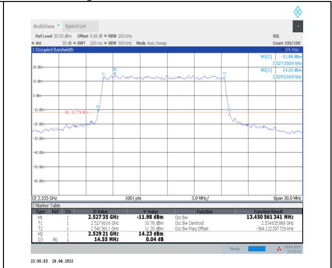
1-N7--15-15-M-3-DFT-16QAM-Outer_Full-75@0-Ant 0-13.451-14.550-≤15-PASS
