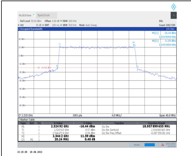
1-N7--15-20-M-7-CP-16QAM-Outer_Full-106@0-Ant 0-18.958-20.240-≤20-PASS
