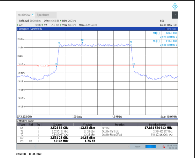
1-N7--15-20-M-2-DFT-PI2BPSK-Outer_Full-100@0-Ant 0-17.882-19.120-≤20-PASS
