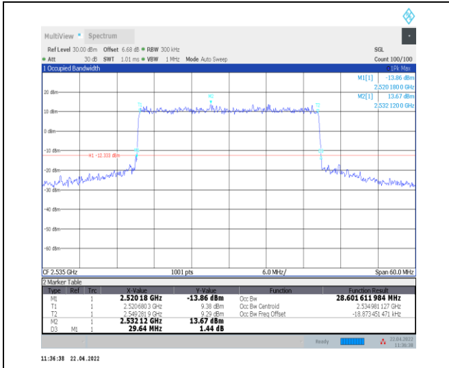
1-N7--15-30-M-1-DFT-QPSK-Outer_Full-160@0-Ant 0-28.602-29.640-≤30-PASS
