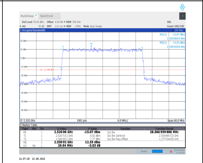
1-N7--15-30-M-4-DFT-64QAM-Outer_Full-160@0-Ant t0-28.567-29.940-≤30-PASS
