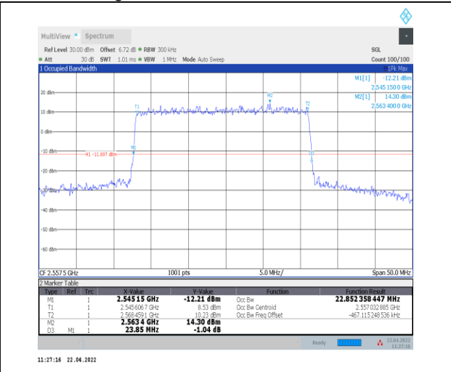
1-N7--15-25-H-4-DFT-64QAM-Outer_Full-128@0-An t0-22.852-23.850-<=25-PASS
