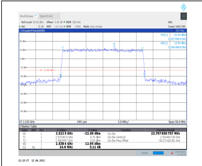
1-N7--15-25-M-8-CP-64QAM-Outer_Full-133@0-Ant 0-23.798-24.900-≤25-PASS
