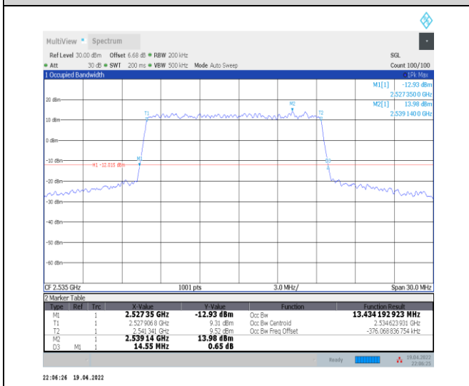
1-N7--15-15-M-4-DFT-64QAM-Outer_Full-75@0-Ant 0-13.434-14.550-≤15-PASS
