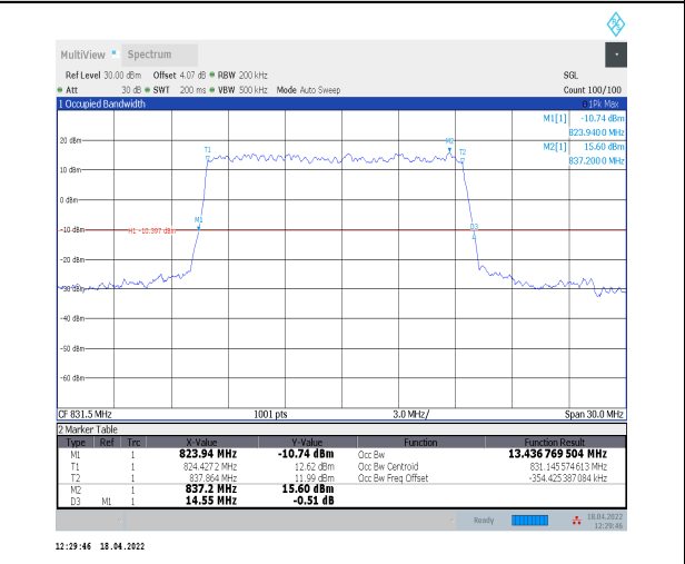
1-N5--15-15-L-2-DFT-PI2BPSK-Outer_Full-75@0-An t0-13.437-14.550≤15-PASS
