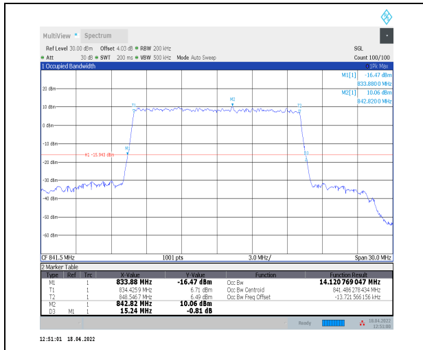
1-N5--15-15-H-9-CP-256QAM-Outer_Full-79@0-Ant 0-14.121-15.240-≤15-PASS
