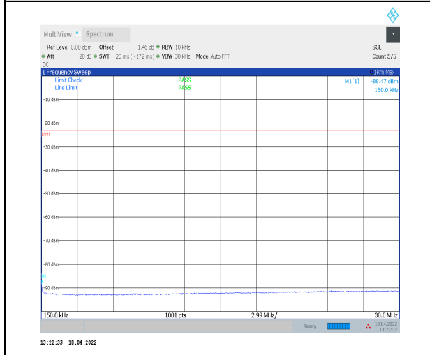
1-N5--15-20-M-1-DFT-PI2BPSK-Inner_1RB_Left-1@ 1-0.15-30-Ant0--88.47--23-PASS
