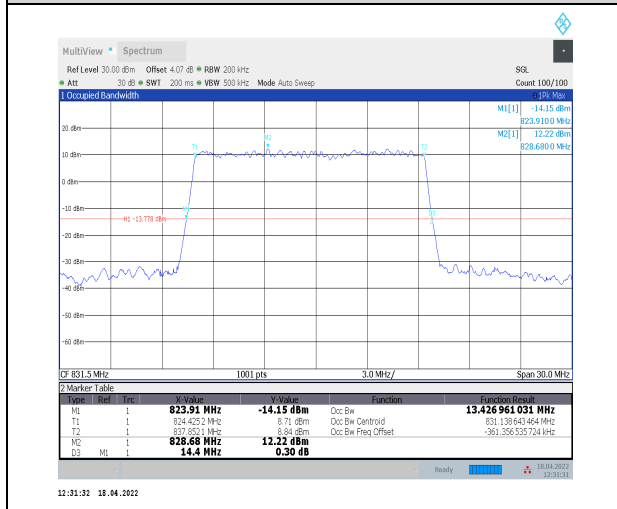
1-N5--15-15-L-5-DFT-256QAM-Outer_Full-75@0-Ant t0-13.427-14.400≤15-PASS
