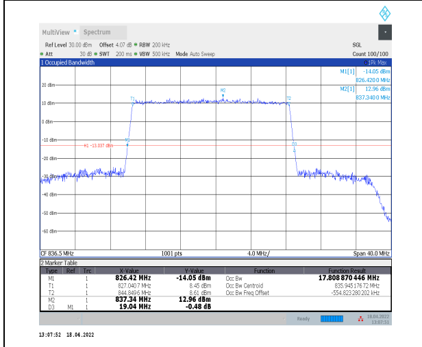
1-N5--15-20-M-5-DFT-256QAM-Outer_Full-100@0-A Ant0-17.809-19.040-≤20-PASS
