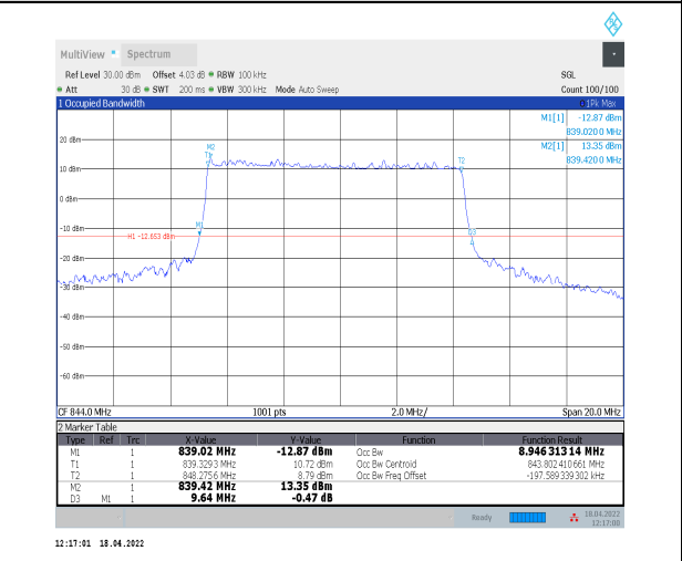
1-N5--15-10-H-3-DFT-16QAM-Outer_Full-50@0-Ant 0-8.946-9.640-≤10-PASS
