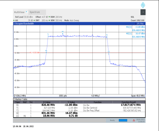
1-N5--15-20-M-2-DFT-PI2BPSK-Outer_Full-100@0-Ant 0-17.817-18.960≤20-PASS
