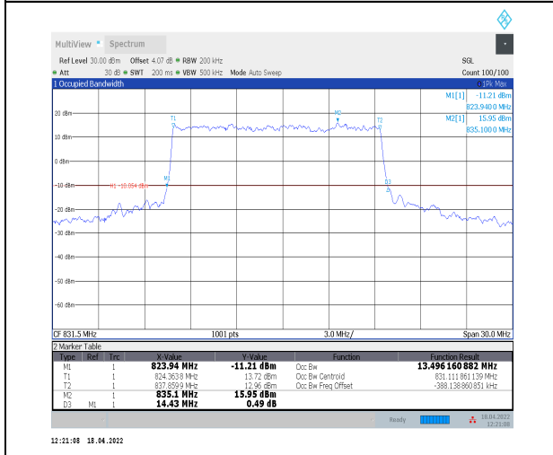
1-N5--15-15-L-1-DFT-QPSK-Outer_Full-75@0-Ant0 13.496-14.430≤15-PASS
