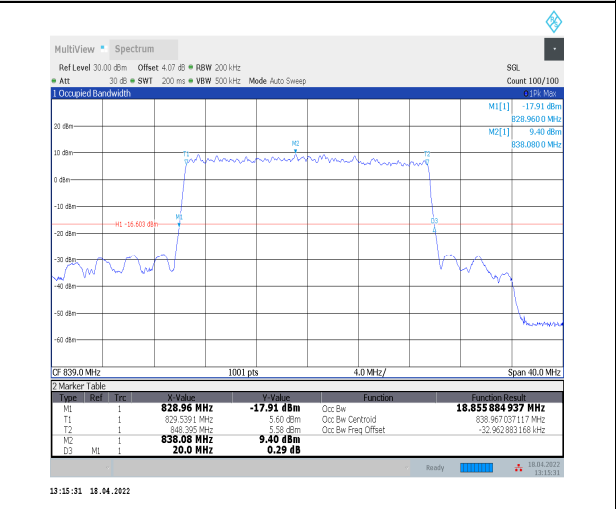
1-N5--15-20-H-9-CP-256QAM-Outer_Full-106@0-Ant-0-18.856-20.000-≤20-PASS
