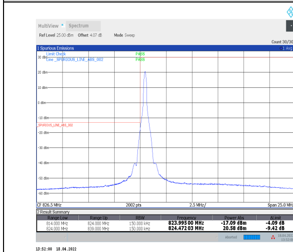
1-N5--15-15-L-4-CP-QPSK-Edge_1RB_Left-1@0-Ant0-seegraph-PASS-see graph
