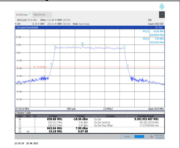
1-N5--15-10-H-9-CP-256QAM-Outer_Full-52@0-Ant 0-9.302-10.180≤10-PASS
