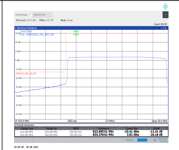
1-N5--15-20-L-6-CP-QPSK-Outer_Full-106@0-Ant0-seegraph-PASS-see graph
