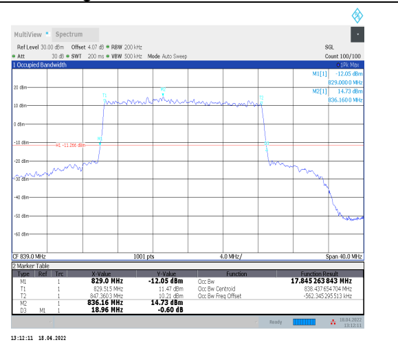
1-N5--15-20-H-3-DFT-16QAM-Outer_Full-100@0-An t0-17.845-18.960-≤20-PASS
