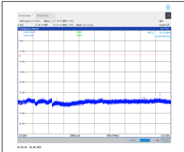
1-N5--15-20-L-1-DFT-PI2BPSK-Inner_1RB_Left-1@ 1-3000-12000-Ant0--53.70--13-PASS
