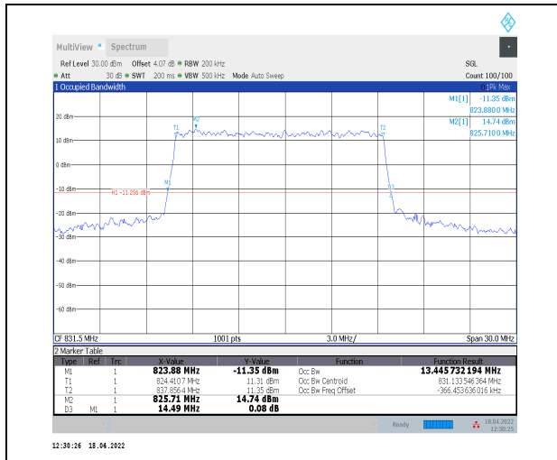
1-N5--15-15-L-3-DFT-16QAM-Outer_Full-75@0-Ant 0-13.446-14.490≤15-PASS
