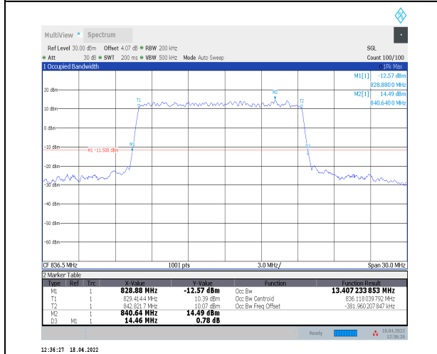
1-N5--15-15-M-4-DFT-64QAM-Outer_Full-75@0-Ant 0-13.407-14.460-≤15-PASS
