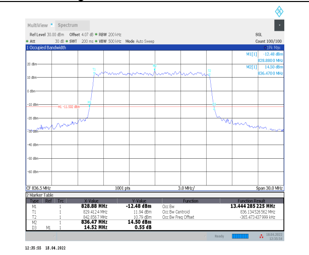
1-N5--15-15-M-3-DFT-16QAM-Outer_Full-75@0-Ant 0-13.444-14.520-≤15-PASS
