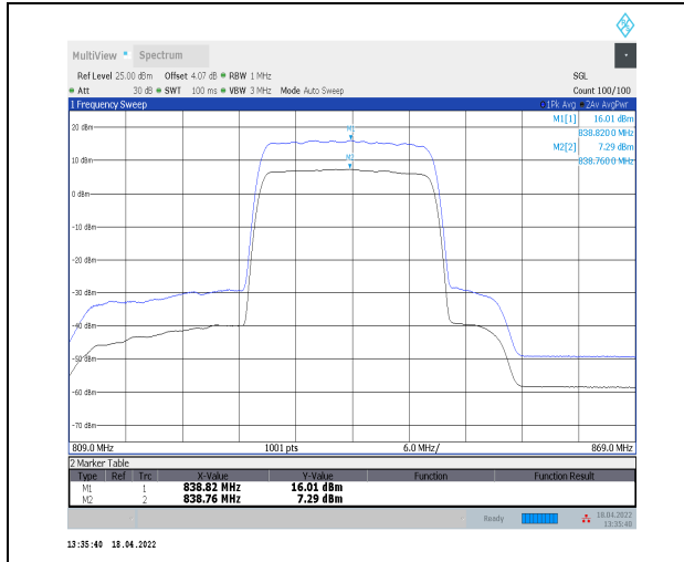
1-N5--15-20-H-1-DFT-256QAM-Outer_Full-100@0-A nt0-8.72-100%-0.00-8.72-PASS≤13
