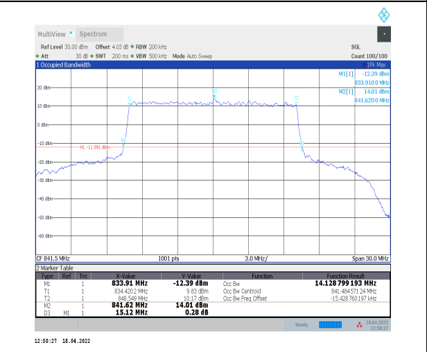
1-N5--15-15-H-8-CP-64QAM-Outer_Full-79@0-Ant0-0 14.129-15.120-≤15-PASS
