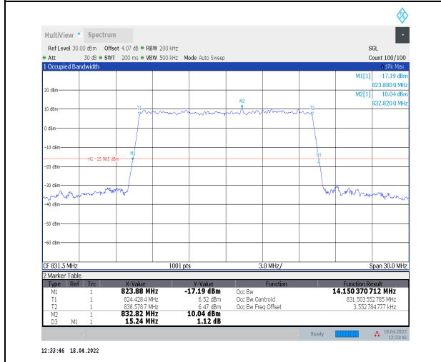
1-N5--15-15-L-9-CP-256QAM-Outer_Full-79@0-Ant0-0-14.15-15.240-<=15-PASS
