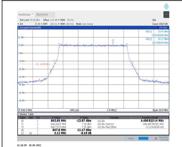
1-N5--15-5-H-5-DFT-256QAM-Outer_Full-25@0-Ant0-0-4.491-5.120-≤5-PASS
