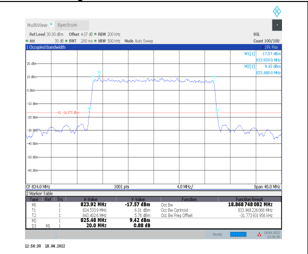
1-N5--15-20-L-9-CP-256QAM-Outer_Full-106@0-Ant 0-18.869-20.000≤20-PASS
