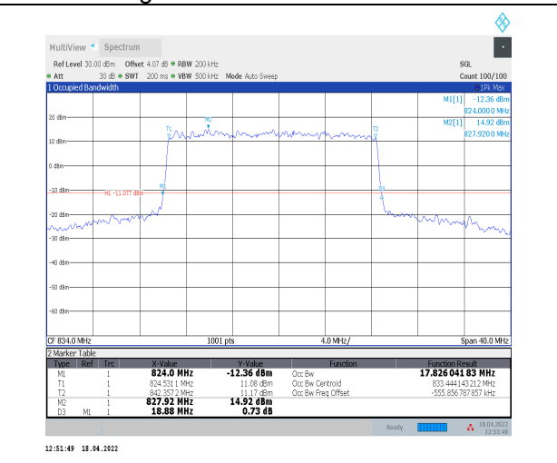
1-N5--15-20-L-1-DFT-QPSK-Outer_Full-100@0-Ant0 -17.826-18.880-≤20-PASS
