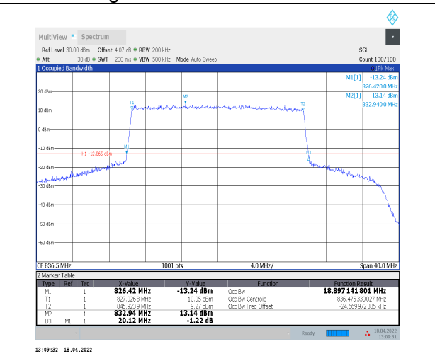
1-N5--15-20-M-8-CP-64QAM-Outer_Full-106@0-Ant 0-18.897-20.120-≤20-PASS
