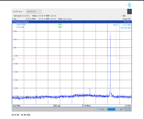
1-N5--15-20-M-1-DFT-PI2BPSK-Inner_1RB_Left-1@ 1-30-1000-Ant0--54.47--13-PASS
