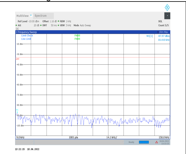
1-N5--15-20-M-1-DFT-PI2BPSK-Inner_1RB_Left-1@ 1-0.009-0.15-Ant0--87.97--33-PASS
