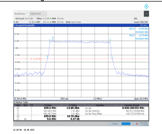
1-N5--15-10-H-5-DFT-256QAM-Outer_Full-50@0-An t0-8.936-9.600-<=10-PASS
