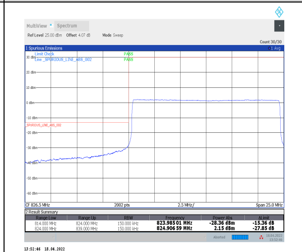
1-N5--15-15-L-6-CP-QPSK-Outer_Full-79@0-Ant0-seegraph-PASS-see graph
