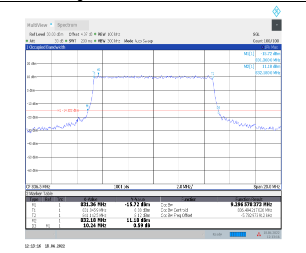
1-N5--15-10-M-6-CP-QPSK-Outer_Full-52@0-Ant0-9 .297-10.240≤10-PASS
