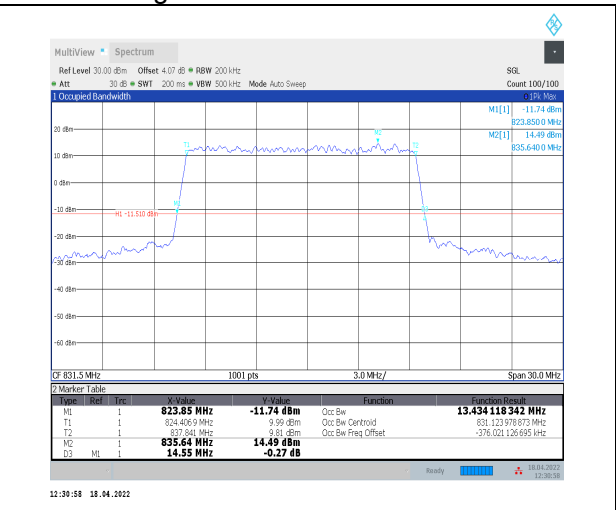
1-N5--15-15-L-4-DFT-64QAM-Outer_Full-75@0-Ant0 -13.434-14.550≤15-PASS
