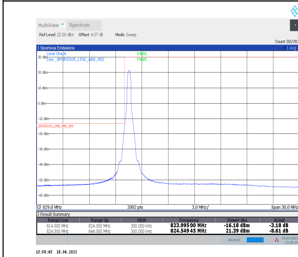
1-N5--15-20-L-4-CP-QPSK-Edge_1RB_Left-1@0-Ant0-seegraph-PASS-see graph
