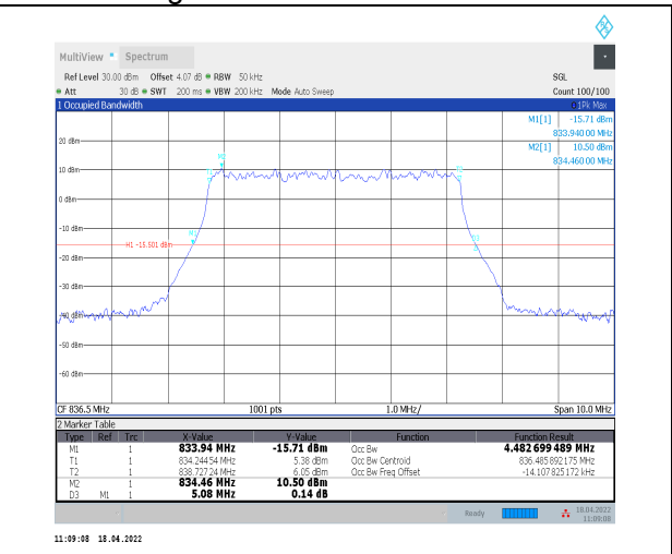
1-N5--15-5-M-5-DFT-256QAM-Outer_Full-25@0-Ant 0-4.483-5.080≤5-PASS
