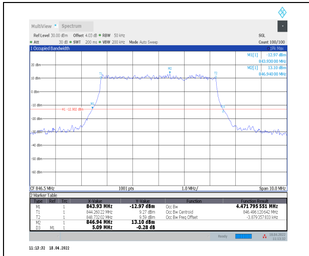
1-N5--15-5-H-3-DFT-16QAM-Outer_Full-25@0-Ant0-4.472-5.090-≤5-PASS
