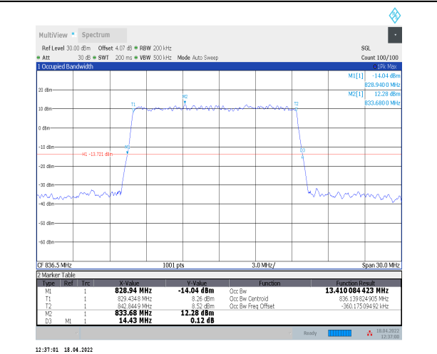
1-N5--15-15-M-5-DFT-256QAM-Outer_Full-75@0-Ant t0-13.41-14.430-≤15-PASS
