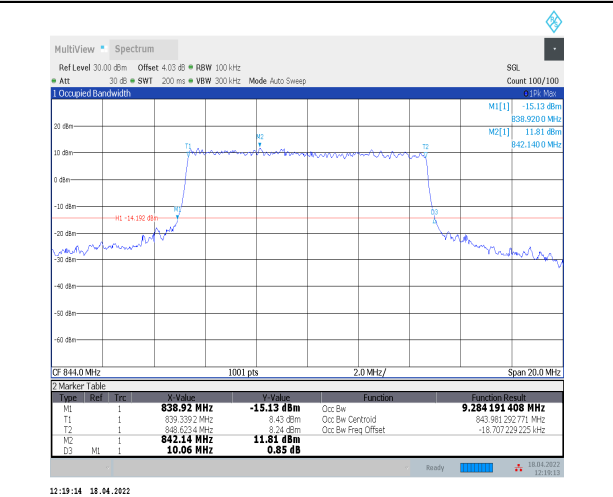
1-N5--15-10-H-7-CP-16QAM-Outer_Full-52@0-Ant0- 9.284-10.060-<=10-PASS
