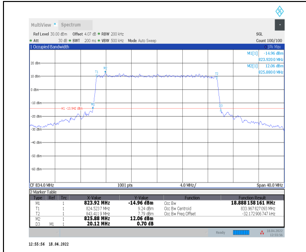
1-N5--15-20-L-8-CP-64QAM-Outer_Full-106@0-Ant 0-18.888-20.120≤20-PASS
