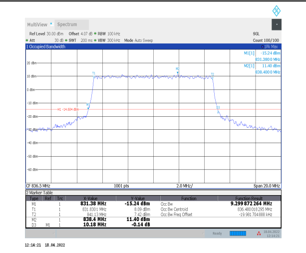
1-N5--15-10-M-8-CP-64QAM-Outer_Full-52@0-Ant0 -9.3-10.180≤10-PASS
