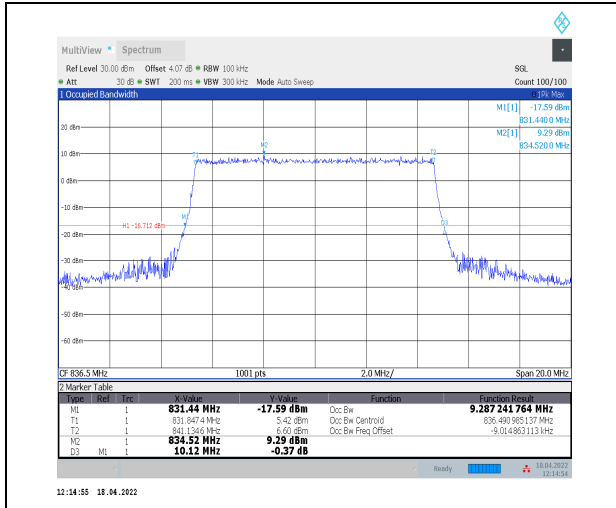
1-N5--15-10-M-9-CP-256QAM-Outer_Full-52@0-Ant 0-9.287-10.120-≤10-PASS
