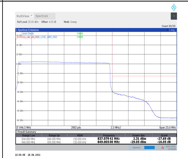
1-N5--15-15-H-6-CP-QPSK-Outer_Full-79@0-Ant0-seegraph-PASS-see graph
