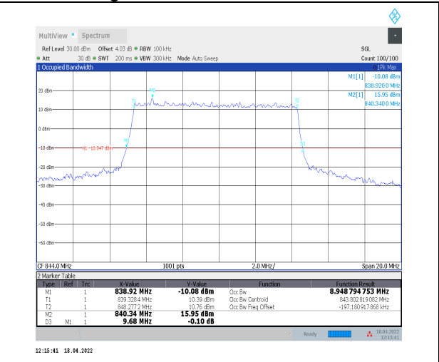
1-N5--15-10-H-1-DFT-QPSK-Outer_Full-50@0-Ant0- 8.949-9.680-≤10-PASS
