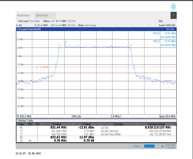
1-N5--15-10-M-4-DFT-64QAM-Outer_Full-50@0-Ant0 0-8.928-9.760-≤10-PASS
