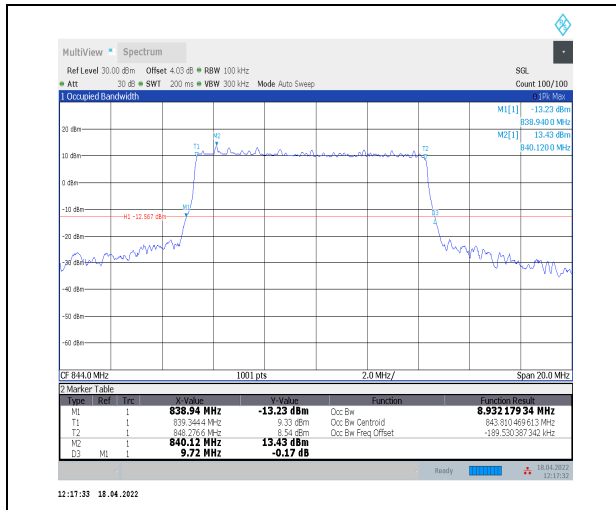
1-N5--15-10-H-4-DFT-64QAM-Outer_Full-50@0-Ant 0-8.932-9.720-<=10-PASS
