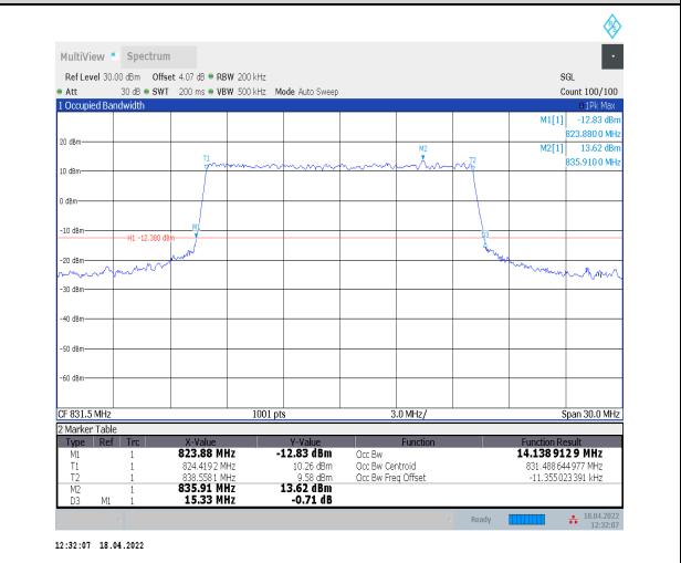
1-N5--15-15-L-6-CP-QPSK-Outer_Full-79@0-Ant0-1 4.139-15.330≤15-PASS
