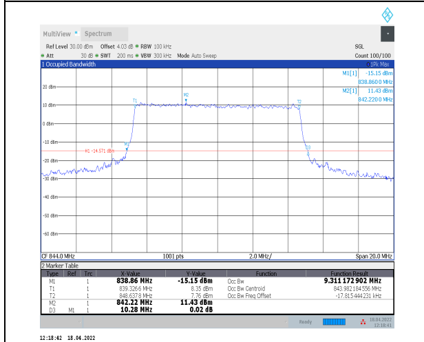
1-N5--15-10-H-6-CP-QPSK-Outer_Full-52@0-Ant0-9 .311-10.280-<=10-PASS
