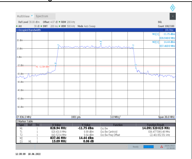
1-N5--15-15-M-7-CP-16QAM-Outer_Full-79@0-Ant0-14.092-15.090-<=15-PASS
