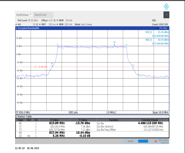
1-N5--15-5-L-8-CP-64QAM-Outer_Full-25@0-Ant0-4.486-5.260-<math>\leq</math>5-PASS
