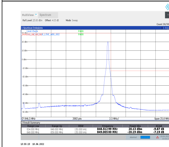
1-N5--15-15-H-5-CP-QPSK-Edge_1RB_Right-1@78-Ant0-seegraph-PASS-see graph
