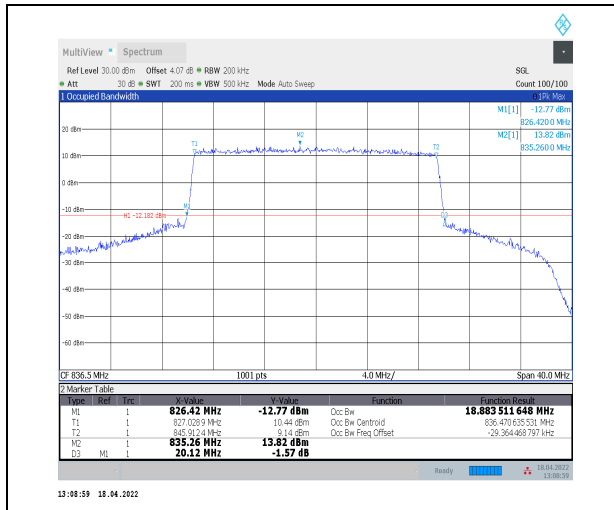
1-N5--15-20-M-7-CP-16QAM-Outer_Full-106@0-Ant 0-18.884-20.120-≤20-PASS
