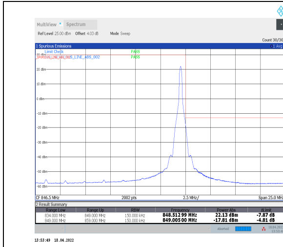
1-N5--15-15-H-2-DFT-PI2BPSK-Edge_1RB_Right-1@78-Ant0-seegraph-PASS-see graph
