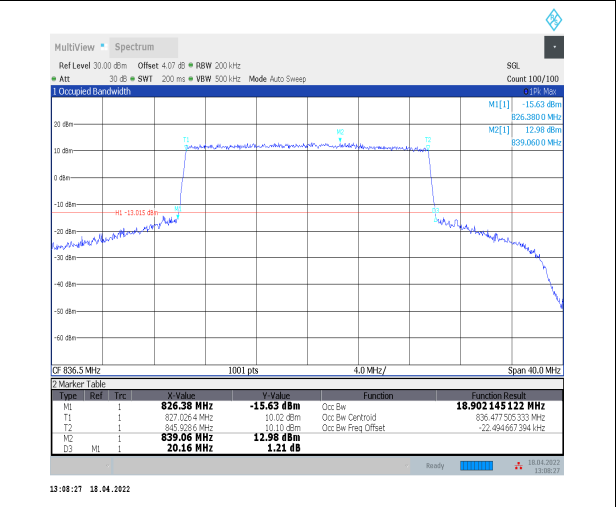
1-N5--15-20-M-6-CP-QPSK-Outer_Full-106@0-Ant0- 18.902-20.160-≤20-PASS
