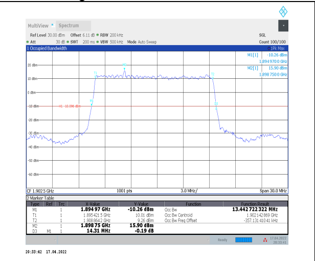
1-N2--15-15-H-2-DFT-PI2BPSK-Outer_Full-75@0-Ant-0 nt0-13.443-14.310≤15-PASS
