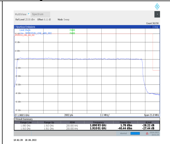
1-N2--15-20-H-3-DFT-PI2BPSK-Outer_Full-100@0-Ant0-seegraph-PASS-see graph
