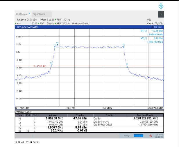
1-N2--15-10-H-7-CP-16QAM-Outer_Full-52@0-Ant0- 9.298-10.200-<=10-PASS
