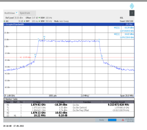
1-N2--15-10-M-8-CP-64QAM-Outer_Full-52@0-Ant0 -9.324-10.220-≤10-PASS
