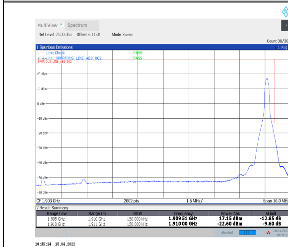
1-N2--15-15-H-5-CP-QPSK-Edge_1RB_Right-1@78-Ant0-seegraph-PASS-see graph
