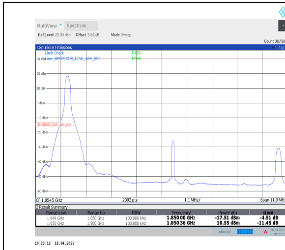
1-N2--15-10-L-1-DFT-PI2BPSK-Edge_1RB_Left-1@0-Ant0-seegraph-PASS-see graph
