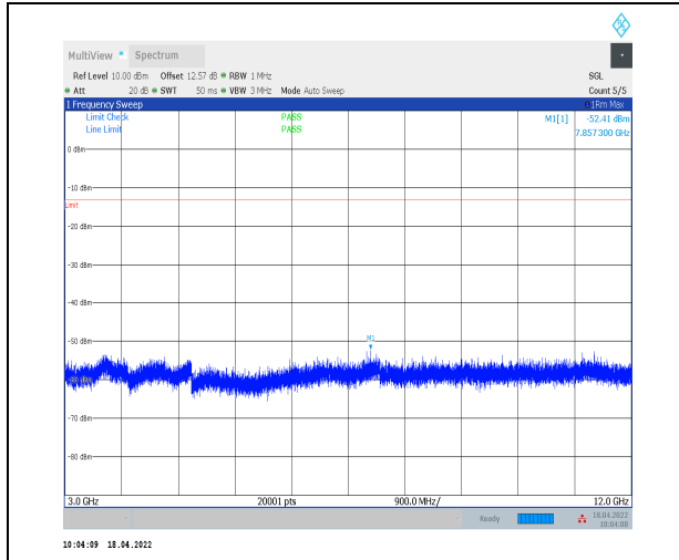
1-N2--15-20-H-1-DFT-PI2BPSK-Inner_1RB_Left-1@ 1-3000-12000-Ant0--52.41--13-PASS
