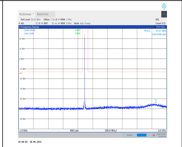
1-N2--15-20-H-1-DFT-PI2BPSK-Inner_1RB_Left-1@ 1-1000-3000-Ant0--44.57--13-PASS
