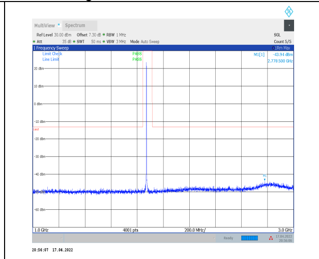
1-N2--15-20-M-1-DFT-PI2BPSK-Inner_1RB_Left-1@ 1-1000-3000-Ant0--43.94--13-PASS
