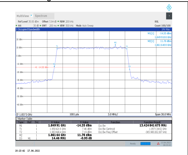
1-N2--15-15-L-4-DFT-64QAM-Outer_Full-75@0-Ant0 -13.425-14.460≤15-PASS
