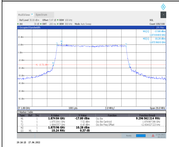
1-N2--15-10-M-7-CP-16QAM-Outer_Full-52@0-Ant0 -9.297-10.240-≤10-PASS
