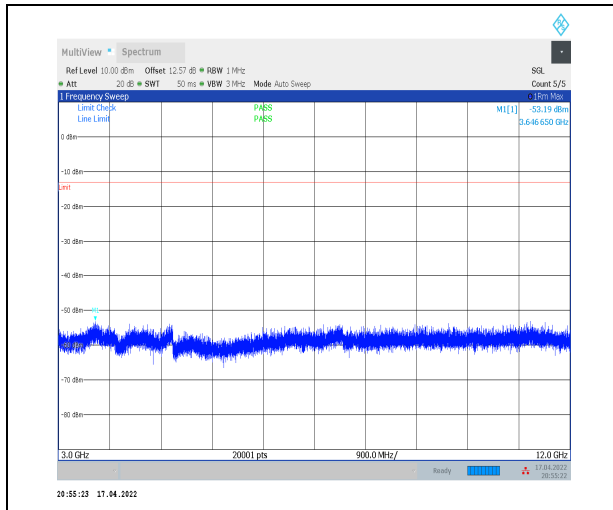
1-N2--15-20-L-1-DFT-PI2BPSK-Inner_1RB_Left-1@ 1-3000-12000-Ant0--53.19--13-PASS
