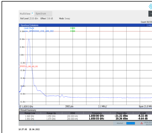
1-N2--15-20-L-1-DFT-PI2BPSK-Edge_1RB_Left-1@0-Ant0-seegraph-PASS-see graph
