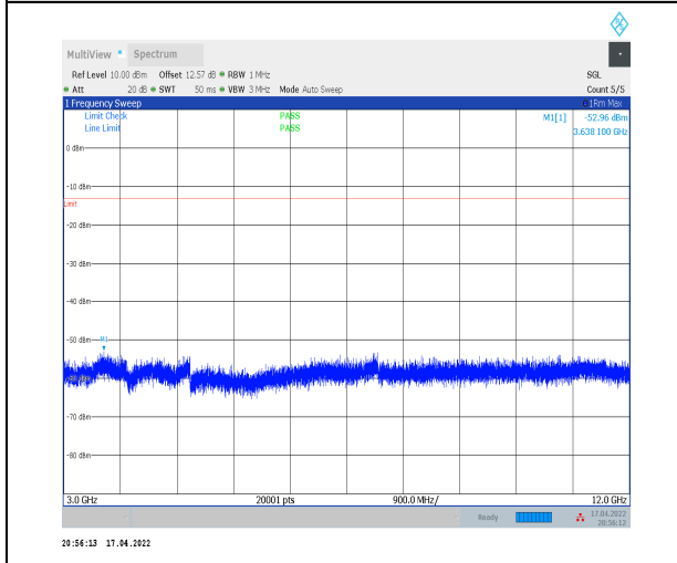
1-N2--15-20-M-1-DFT-PI2BPSK-Inner_1RB_Left-1 @1-3000-12000-Ant0--52.96--13-PASS
