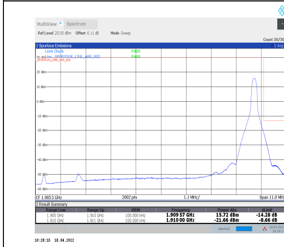
1-N2--15-10-H-5-CP-QPSK-Edge_1RB_Right-1@51-Ant0-seegraph-PASS-see graph
