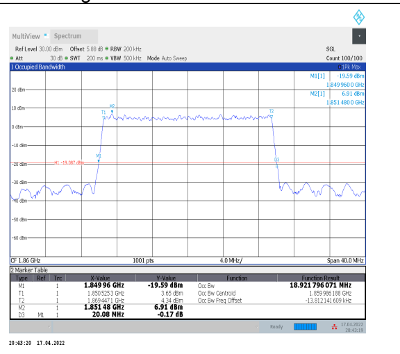
1-N2--15-20-L-9-CP-256QAM-Outer_Full-106@0-Ant 0-18.922-20.080-≤20-PASS
