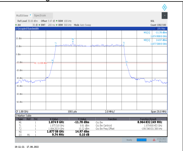
1-N2--15-10-M-2-DFT-PI2BPSK-Outer_Full-50@0-Ant0 -8.965-9.740-≤10-PASS
