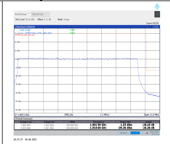
1-N2--15-10-H-3-DFT-PI2BPSK-Outer_Full-50@0-Ant0-seegraph-PASS-see graph
