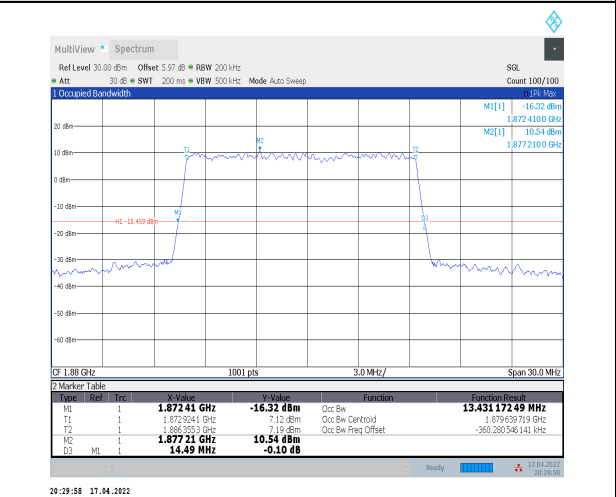
1-N2--15-15-M-5-DFT-256QAM-Outer_Full-75@0-Ant t0-13.431-14.490-≤15-PASS
