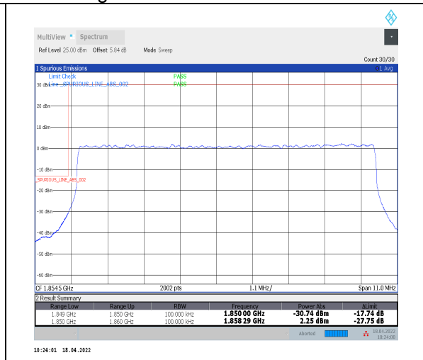
1-N2--15-10-L-3-DFT-PI2BPSK-Outer_Full-50@0-Ant0-seegraph-PASS-see graph
