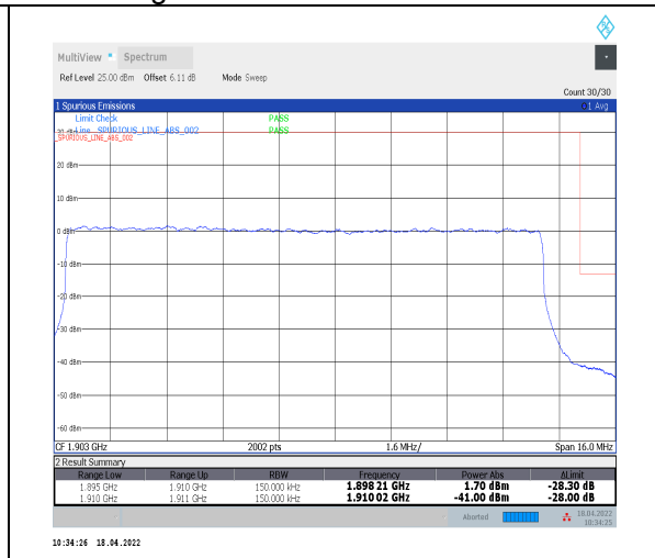
1-N2--15-15-H-3-DFT-PI2BPSK-Outer_Full-75@0-Ant0-seegraph-PASS-see graph
