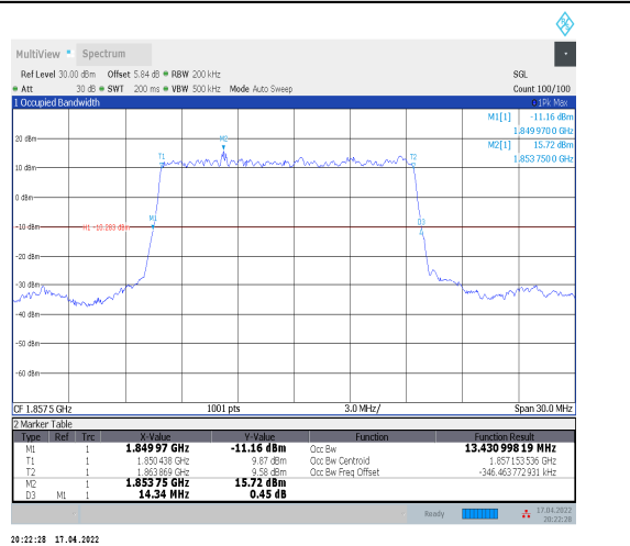
1-N2--15-15-L-2-DFT-PI2BPSK-Outer_Full-75@0-An t0-13.431-14.340≤15-PASS
