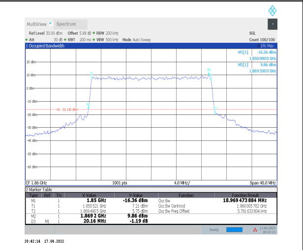
1-N2--15-20-L-7-CP-16QAM-Outer_Full-106@0-Ant0- -18.969-20.160-<20-PASS
