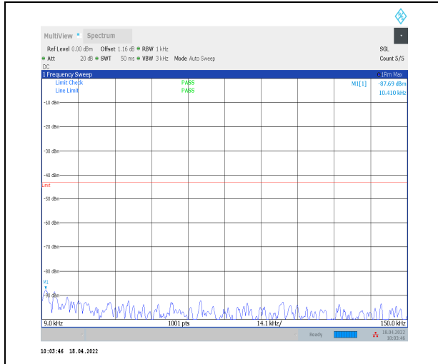
1-N2--15-20-H-1-DFT-PI2BPSK-Inner_1RB_Left-1@ 1-0.009-0.15-Ant0--87.69--43-PASS
