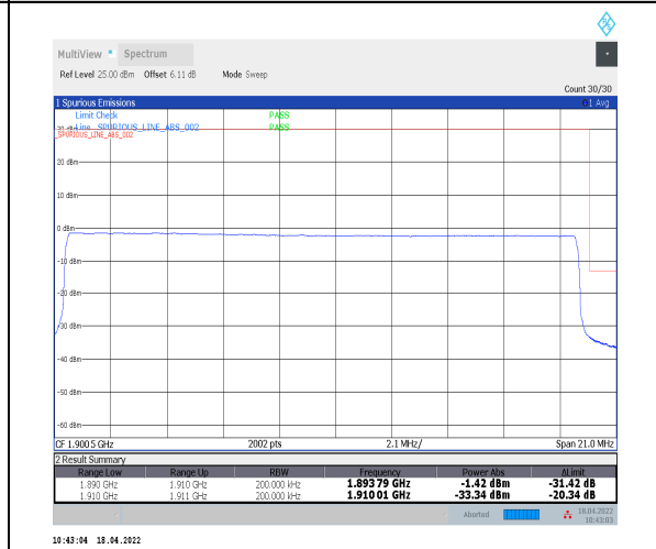
1-N2--15-20-H-6-CP-QPSK-Outer_Full-106@0-Ant0-seegraph-PASS-see graph
