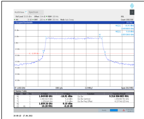
1-N2--15-10-L-6-CP-QPSK-Outer_Full-52@0-Ant0-9 9.317-10.280-≤10-PASS
