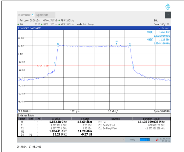
1-N2--15-15-M-6-CP-QPSK-Outer_Full-79@0-Ant0 -14.134-15.270≤15-PASS
