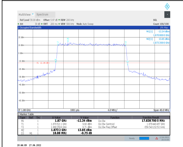
1-N2--15-20-M-1-DFT-QPSK-Outer_Full-100@0-Ant 0-17.839-18.880-≤20-PASS
