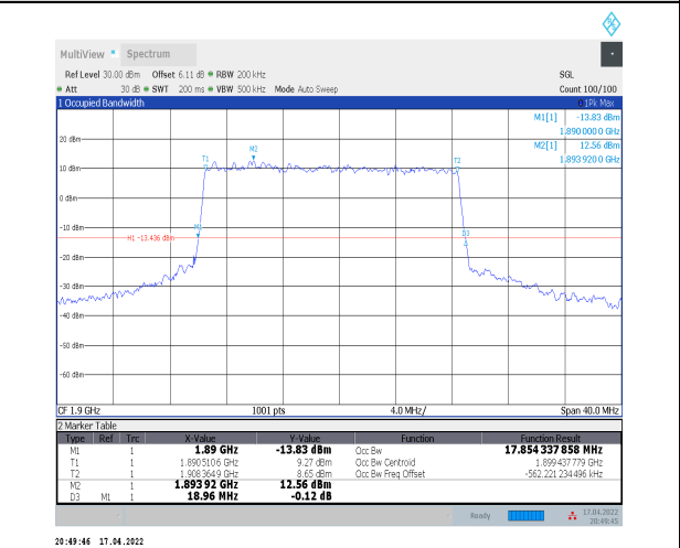
1-N2--15-20-H-1-DFT-QPSK-Outer_Full-100@0-Ant 0-17.854-18.960-≤20-PASS
