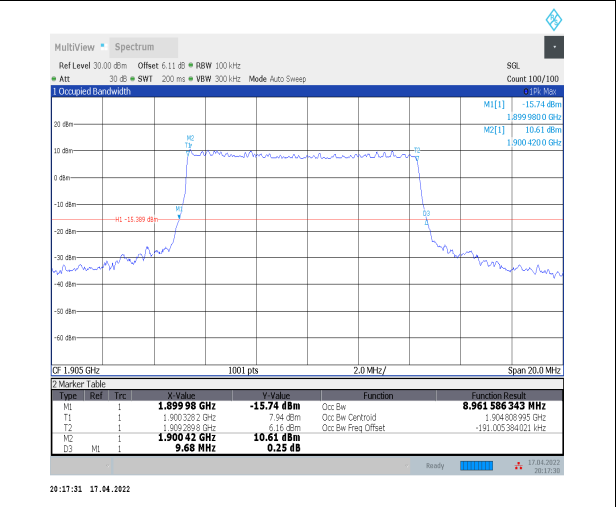
1-N2--15-10-H-3-DFT-16QAM-Outer_Full-50@0-Ant 0-8.962-9.680-≤10-PASS
