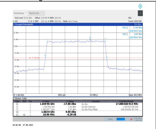
1-N2--15-20-L-5-DFT-256QAM-Outer_Full-100@0-A nt0-17.889-18.960-<20-PASS
