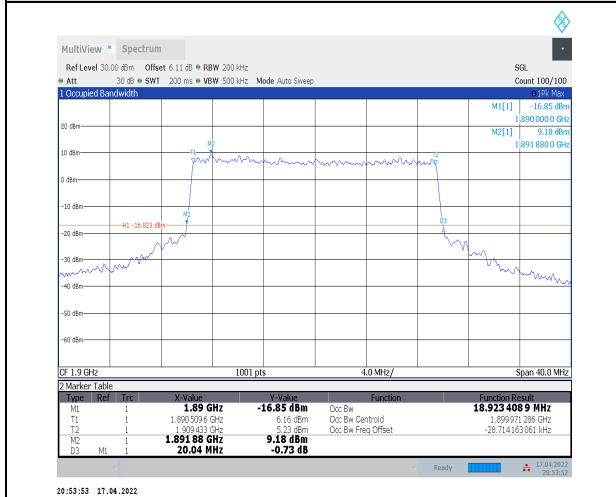
1-N2--15-20-H-8-CP-64QAM-Outer_Full-106@0-Ant-0 0-18.923-20.040-≤20-PASS
