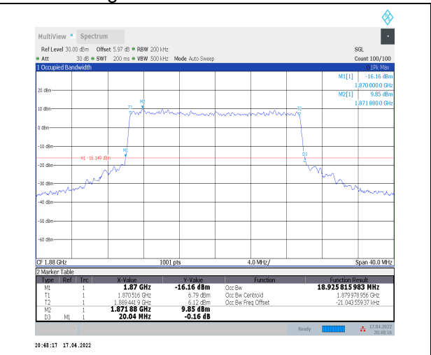
1-N2--15-20-M-8-CP-64QAM-Outer_Full-106@0-Ant 0-18.926-20.040-≤20-PASS
