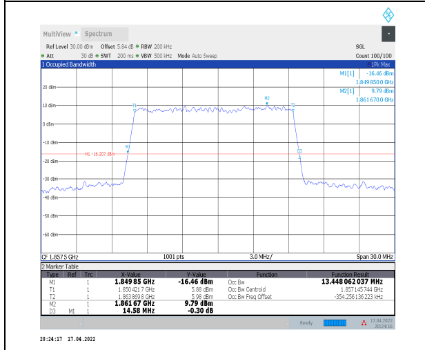
1-N2--15-15-L-5-DFT-256QAM-Outer_Full-75@0-Ant t0-13.448-14.580≤15-PASS
