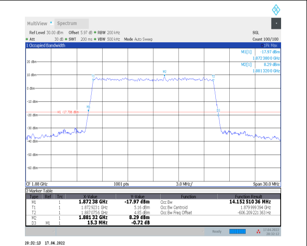
1-N2--15-15-M-9-CP-256QAM-Outer_Full-79@0-Ant 0-14.153-15.300≤15-PASS
