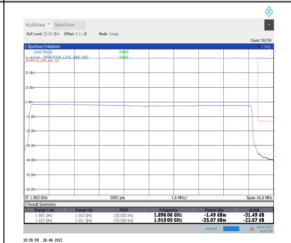
1-N2--15-15-H-6-CP-QPSK-Outer_Full-79@0-Ant0-seegraph-PASS-see graph
