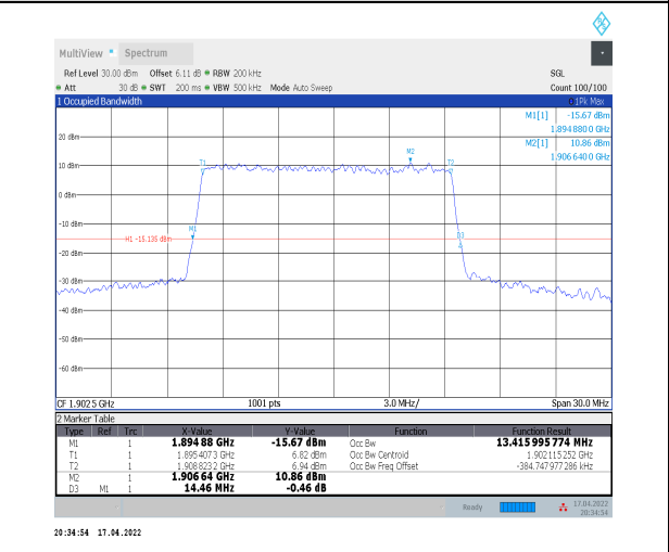
1-N2--15-15-H-4-DFT-64QAM-Outer_Full-75@0-Ant-0 0-13.416-14.460≤15-PASS
