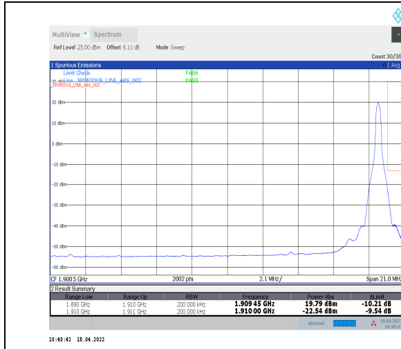
1-N2--15-20-H-2-DFT-PI2BPSK-Edge_1RB_Right-1@105-Ant0-seegraph-PASS-see graph
