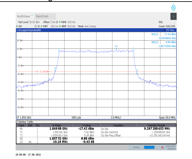
1-N2--15-10-L-7-CP-16QAM-Outer_Full-52@0-Ant0-9 9.297-10.180-≤10-PASS
