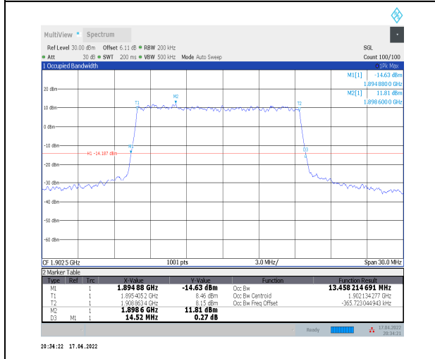
1-N2--15-15-H-3-DFT-16QAM-Outer_Full-75@0-Ant-0 0-13.458-14.520≤15-PASS
