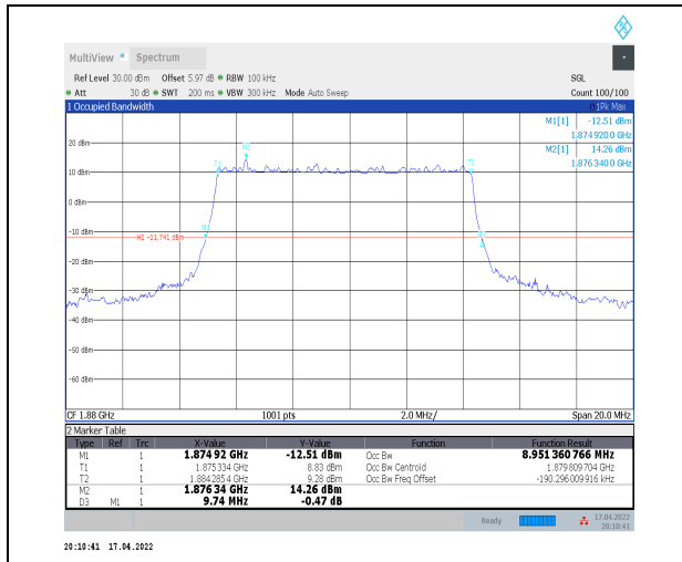
1-N2--15-10-M-1-DFT-QPSK-Outer_Full-50@0-Ant0 -8.951-9.740-≤10-PASS
