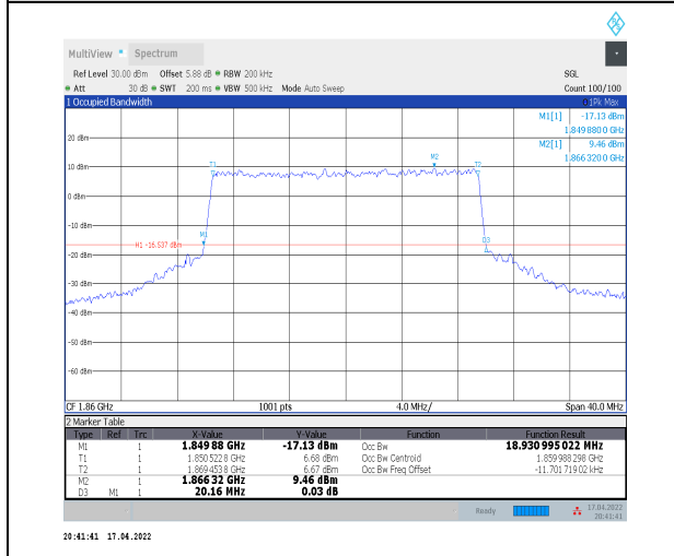
1-N2--15-20-L-6-CP-QPSK-Outer_Full-106@0-Ant0- 18.931-20.160-<20-PASS
