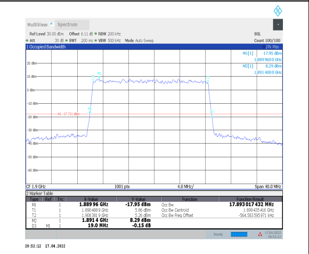
1-N2--15-20-H-5-DFT-256QAM-Outer_Full-100@0-An nt0-17.893-19.000-≤20-PASS
