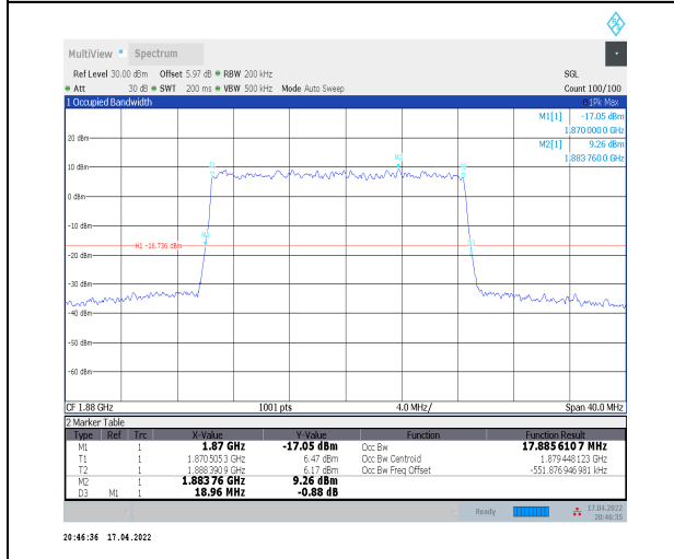
1-N2--15-20-M-5-DFT-256QAM-Outer_Full-100@0-A Ant0-17.886-18.960-≤20-PASS
