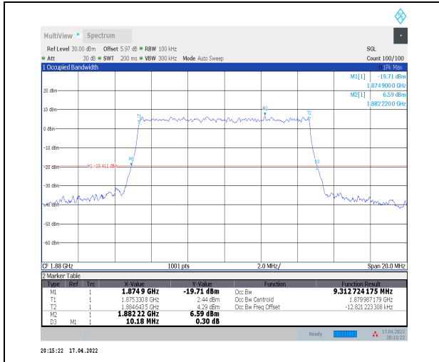
1-N2--15-10-M-9-CP-256QAM-Outer_Full-52@0-Ant 0-9.313-10.180-≤10-PASS
