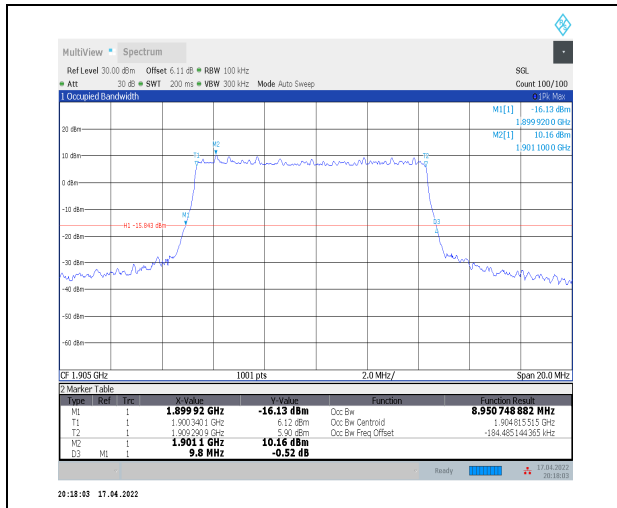
1-N2--15-10-H-4-DFT-64QAM-Outer_Full-50@0-Ant 0-8.951-9.800-<=10-PASS
