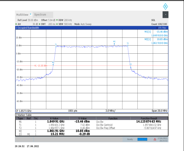
1-N2--15-15-L-6-CP-QPSK-Outer_Full-79@0-Ant0-1 4.126-15.210≤15-PASS
