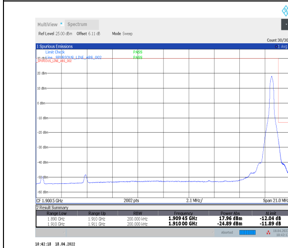
1-N2--15-20-H-5-CP-QPSK-Edge_1RB_Right-1@105-Ant0-seegraph-PASS-see graph
