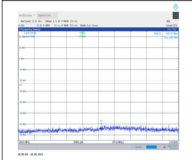
1-N2--15-20-H-1-DFT-PI2BPSK-Inner_1RB_Left-1@ 1-30-1000-Ant0--60.41--23-PASS
