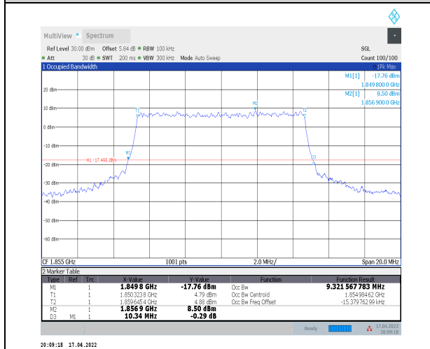
1-N2--15-10-L-8-CP-64QAM-Outer_Full-52@0-Ant0-9 9.322-10.340-≤10-PASS
