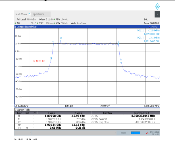
1-N2--15-10-H-1-DFT-QPSK-Outer_Full-50@0-Ant0- 8.95-9.660-≤10-PASS
