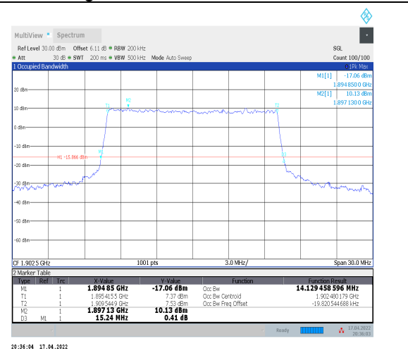
1-N2--15-15-H-6-CP-QPSK-Outer_Full-79@0-Ant0-1 4.129-15.240-<=15-PASS
