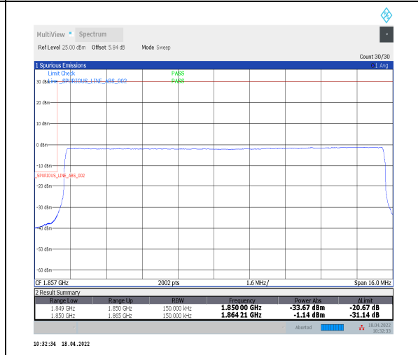
1-N2--15-15-L-6-CP-QPSK-Outer_Full-79@0-Ant0-seegraph-PASS-see graph
