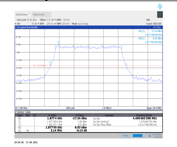
1-N2--15-5-M-5-DFT-256QAM-Outer_Full-25@0-Ant 0-4.491-5.140≤5-PASS
