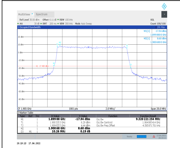
1-N2--15-10-H-6-CP-QPSK-Outer_Full-52@0-Ant0-9 .32-10.260-<=10-PASS
