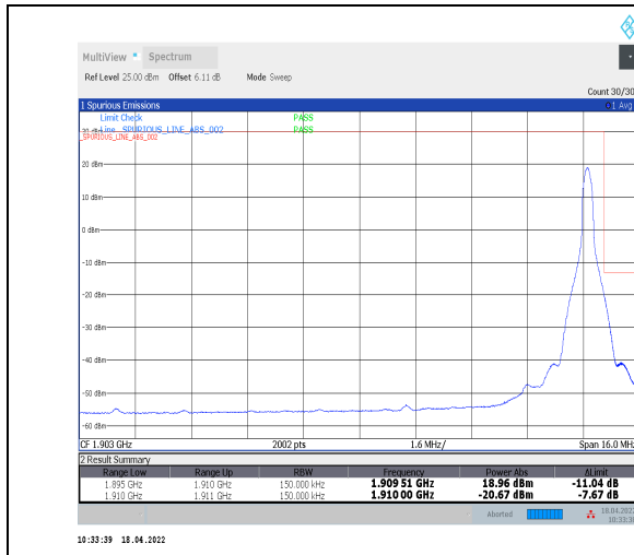
1-N2--15-15-H-2-DFT-PI2BPSK-Edge_1RB_Right-1@78-Ant0-seegraph-PASS-see graph
