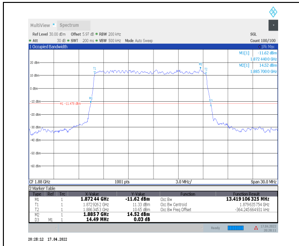
1-N2--15-15-M-2-DFT-PI2BPSK-Outer_Full-75@0-A nt0-13.419-14.490-≤15-PASS
