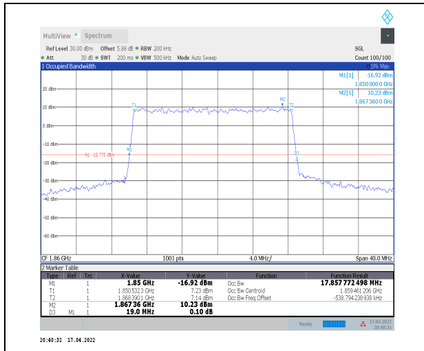
1-N2--15-20-L-4-DFT-64QAM-Outer_Full-100@0-An t0-17.858-19.000-<20-PASS
