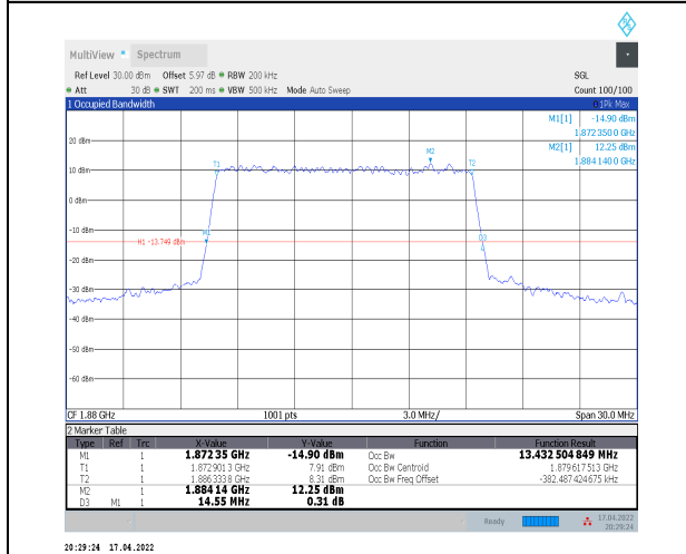
1-N2--15-15-M-4-DFT-64QAM-Outer_Full-75@0-Ant 0-13.433-14.550-≤15-PASS
