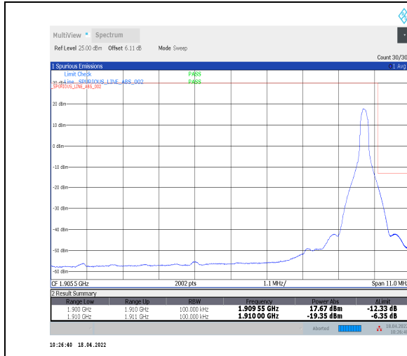
1-N2--15-10-H-2-DFT-PI2BPSK-Edge_1RB_Right-1@51-Ant0-seegraph-PASS-see graph
