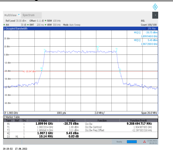
1-N2--15-10-H-9-CP-256QAM-Outer_Full-52@0-Ant 0-9.308-10.140≤10-PASS
