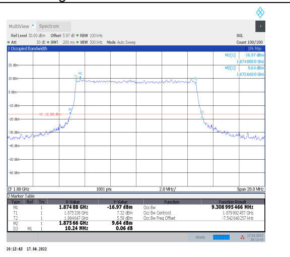
1-N2--15-10-M-6-CP-QPSK-Outer_Full-52@0-Ant0-9 .309-10.240-≤10-PASS
