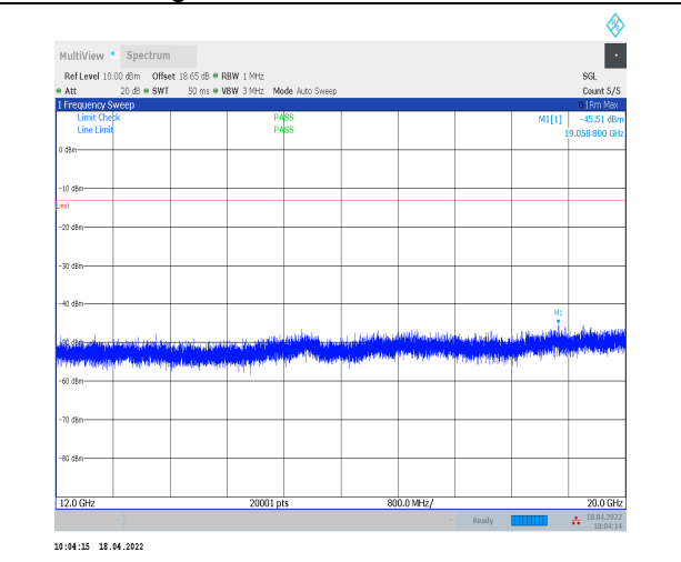
1-N2--15-20-H-1-DFT-PI2BPSK-Inner_1RB_Left-1@ 1-12000-20000-Ant0--45.51--13-PASS
