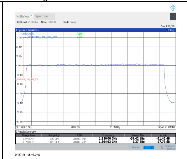
1-N2--15-20-L-3-DFT-PI2BPSK-Outer_Full-100@0-Ant0-seegraph-PASS-see graph
