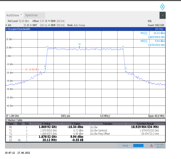
1-N2--15-20-M-6-CP-QPSK-Outer_Full-106@0-Ant0- 18.93-20.120-≤20-PASS
