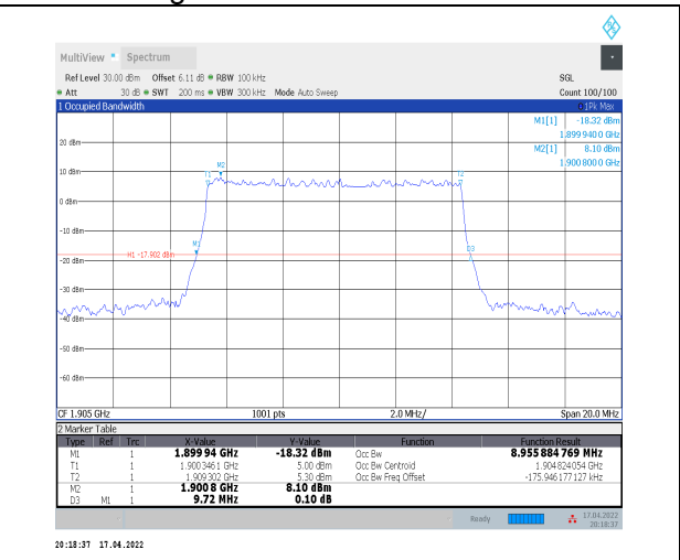
1-N2--15-10-H-5-DFT-256QAM-Outer_Full-50@0-An t0-8.956-9.720-<=10-PASS
