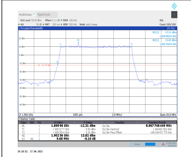
1-N2--15-10-H-2-DFT-PI2BPSK-Outer_Full-50@0-A nt0-8.968-9.680-≤10-PASS
