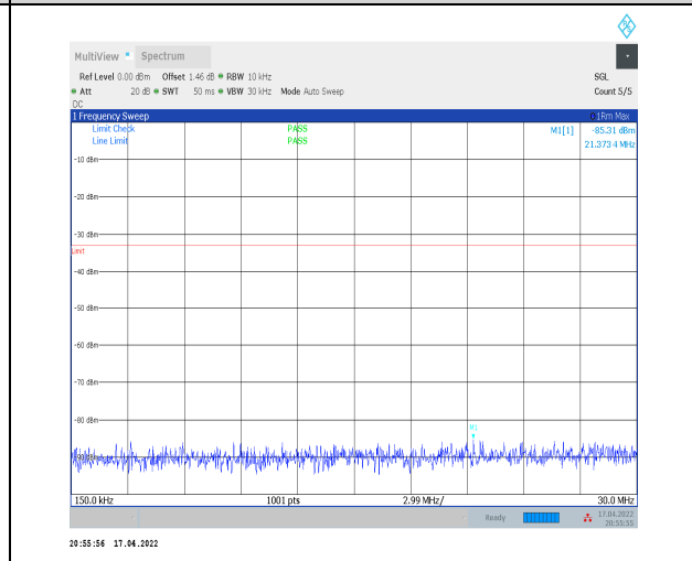
1-N2--15-20-M-1-DFT-PI2BPSK-Inner_1RB_Left-1@ 1-0.15-30-Ant0--85.31--33-PASS
