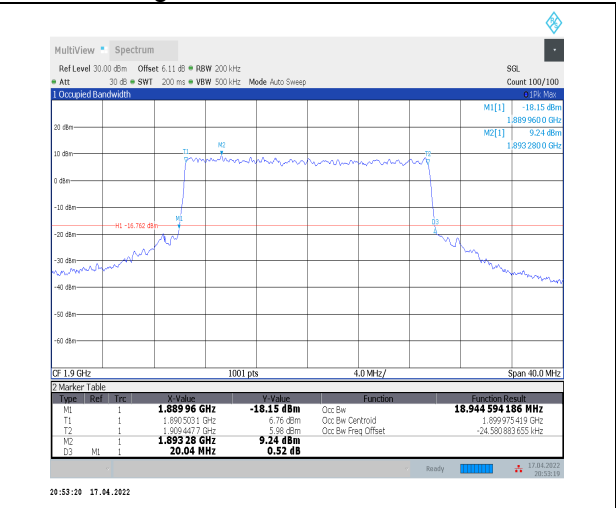
1-N2--15-20-H-7-CP-16QAM-Outer_Full-106@0-Ant-0 0-18.945-20.040-≤20-PASS
