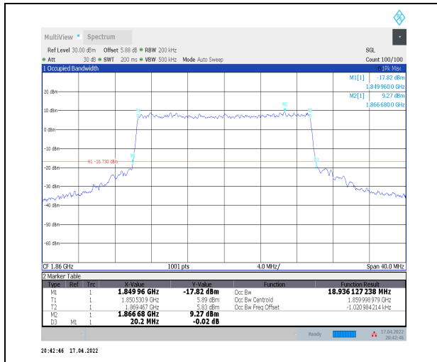
1-N2--15-20-L-8-CP-64QAM-Outer_Full-106@0-Ant 0-18.936-20.200-≤20-PASS
