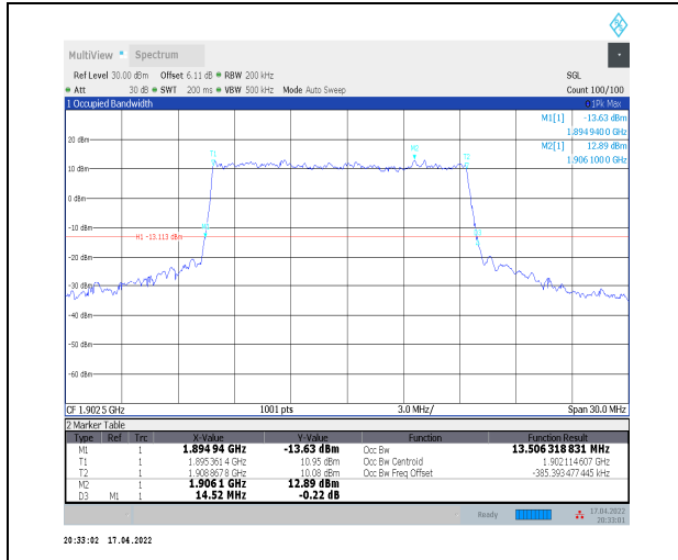
1-N2--15-15-H-1-DFT-QPSK-Outer_Full-75@0-Ant-0 13.506-14.520≤15-PASS
