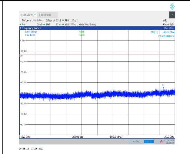
1-N2--15-20-M-1-DFT-PI2BPSK-Inner_1RB_Left-1@ 1-12000-20000-Ant0--45.64--13-PASS
