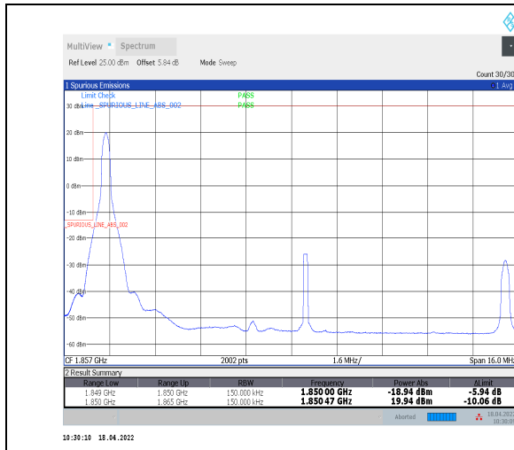
1-N2--15-15-L-1-DFT-PI2BPSK-Edge_1RB_Left-1@0-Ant0-seegraph-PASS-see graph
