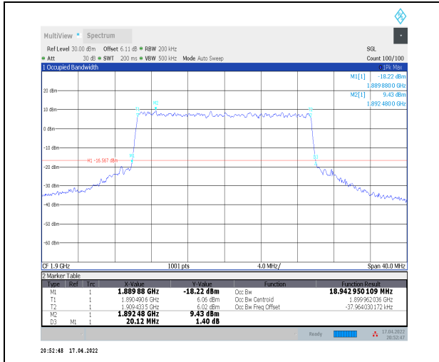
1-N2--15-20-H-6-CP-QPSK-Outer_Full-106@0-Ant-0 18.943-20.120-≤20-PASS
