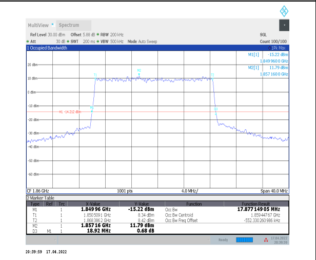
1-N2--15-20-L-3-DFT-16QAM-Outer_Full-100@0-Ant 0-17.877-18.920≤20-PASS
