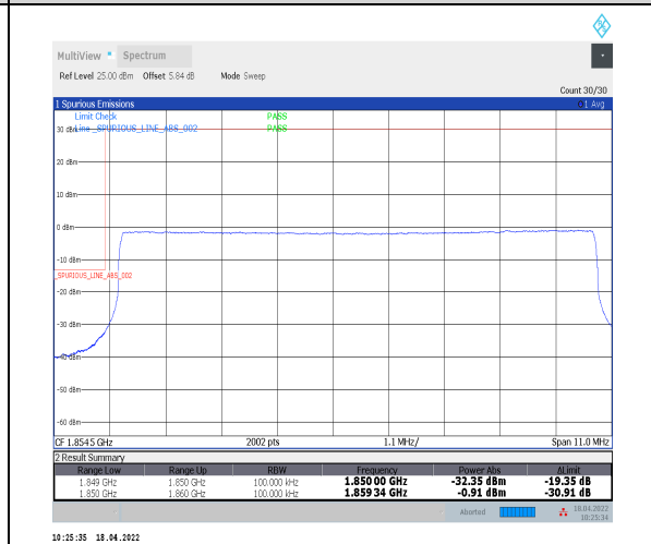
1-N2--15-10-L-6-CP-QPSK-Outer_Full-52@0-Ant0-seegraph-PASS-see graph
