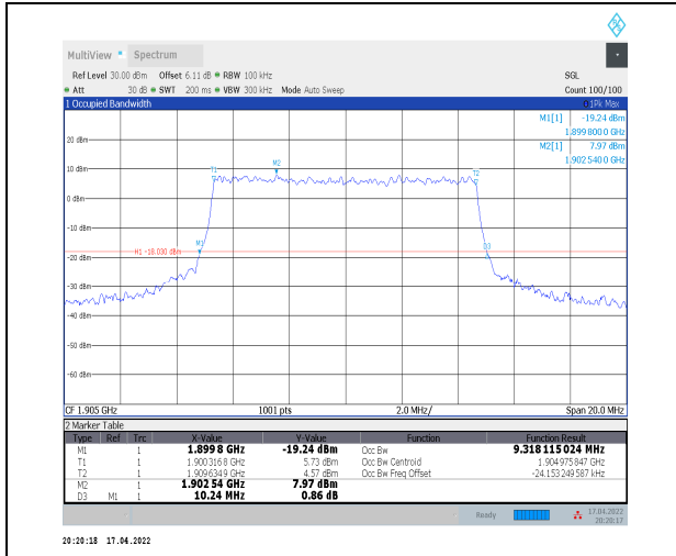
1-N2--15-10-H-8-CP-64QAM-Outer_Full-52@0-Ant0 -9.318-10.240≤10-PASS
