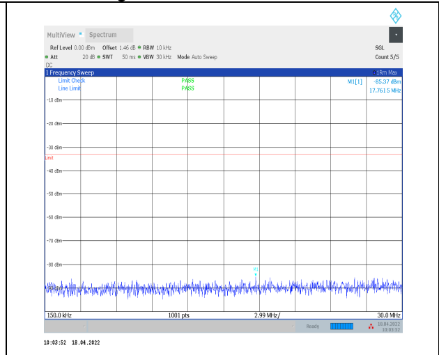
1-N2--15-20-H-1-DFT-PI2BPSK-Inner_1RB_Left-1@ 1-0.15-30-Ant0--85.37--33-PASS
