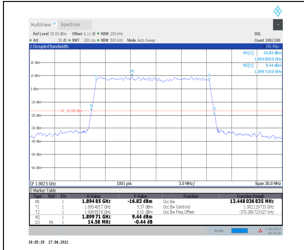
1-N2--15-15-H-5-DFT-256QAM-Outer_Full-75@0-Ant t0-13.448-14.580-<=15-PASS
