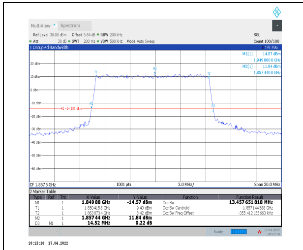
1-N2--15-15-L-3-DFT-16QAM-Outer_Full-75@0-Ant 0-13.458-14.520≤15-PASS
