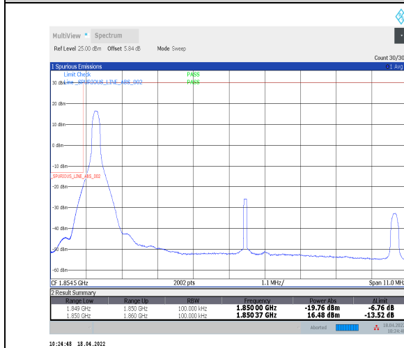
1-N2--15-10-L-4-CP-QPSK-Edge_1RB_Left-1@0-Ant0-seegraph-PASS-see graph
