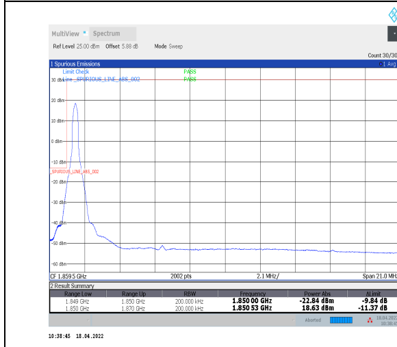
1-N2--15-20-L-4-CP-QPSK-Edge_1RB_Left-1@0-Ant0-seegraph-PASS-see graph
