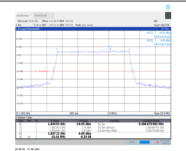
1-N2--15-10-L-9-CP-256QAM-Outer_Full-52@0-Ant0-9 9.307-10.160-≤10-PASS
