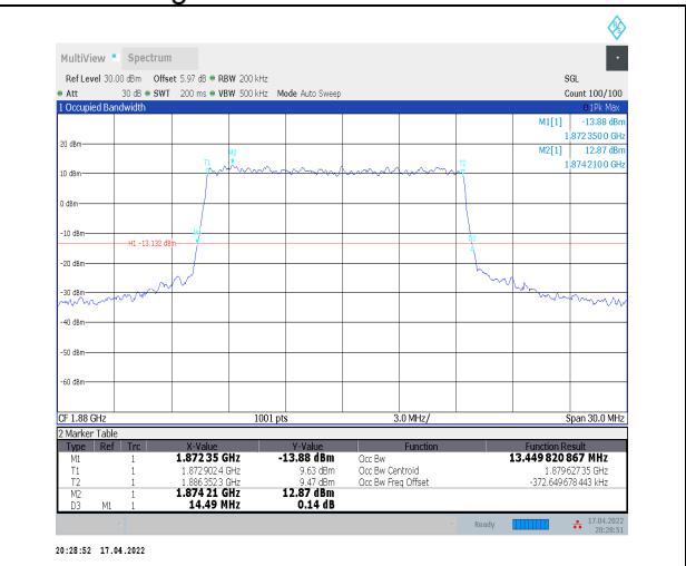
1-N2--15-15-M-3-DFT-16QAM-Outer_Full-75@0-Ant 0-13.45-14.490-≤15-PASS
