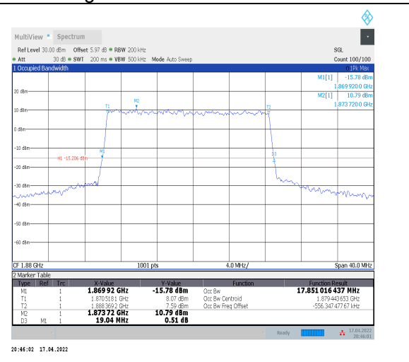
1-N2--15-20-M-4-DFT-64QAM-Outer_Full-100@0-An t0-17.851-19.040-≤20-PASS
