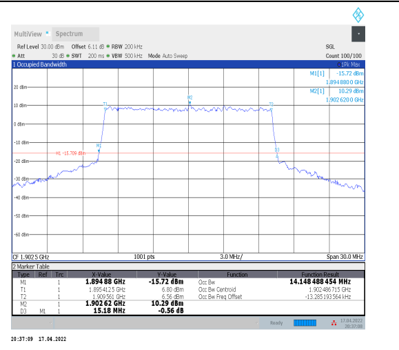
1-N2--15-15-H-8-CP-64QAM-Outer_Full-79@0-Ant0-1 14.148-15.180-<=15-PASS
