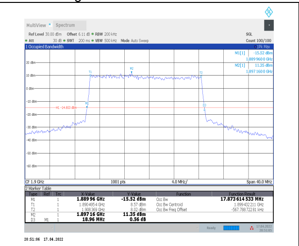
1-N2--15-20-H-3-DFT-16QAM-Outer_Full-100@0-An t0-17.874-18.960-≤20-PASS
