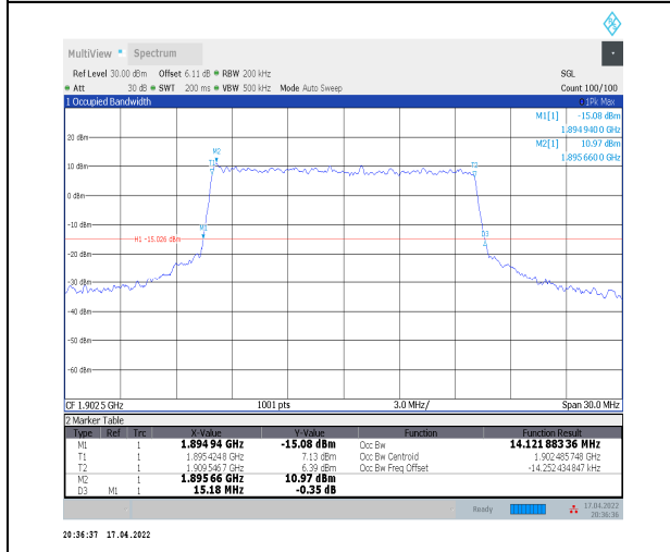
1-N2--15-15-H-7-CP-16QAM-Outer_Full-79@0-Ant0 -14.122-15.180-<=15-PASS
