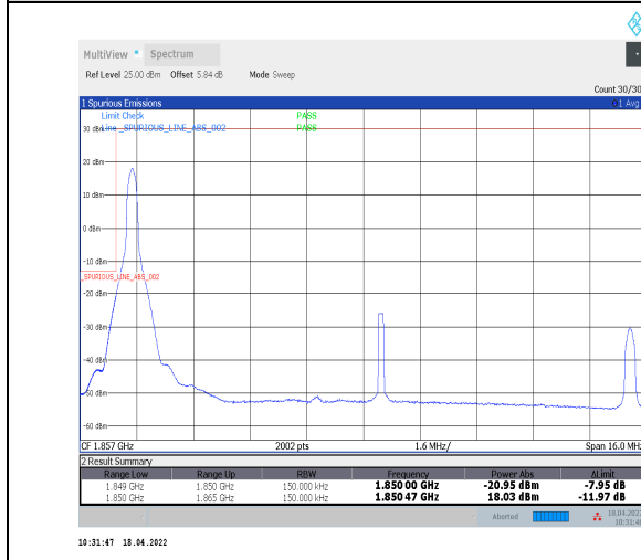
1-N2--15-15-L-4-CP-QPSK-Edge_1RB_Left-1@0-Ant0-seegraph-PASS-see graph
