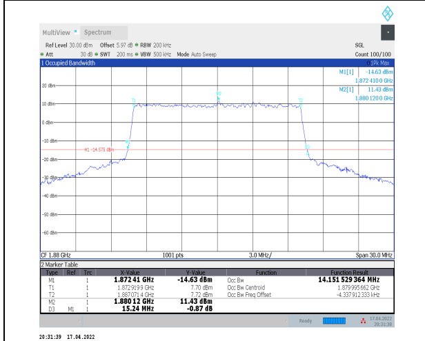
1-N2--15-15-M-8-CP-64QAM-Outer_Full-79@0-Ant0 -14.152-15.240≤15-PASS
