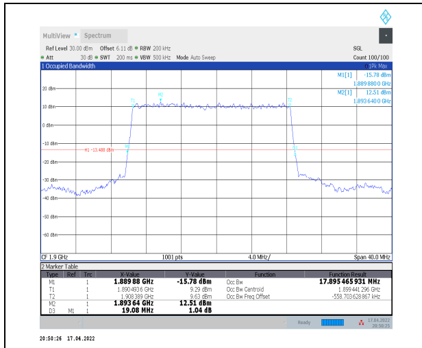
1-N2--15-20-H-2-DFT-PI2BPSK-Outer_Full-100@0-An Ant0-17.895-19.080-≤20-PASS
