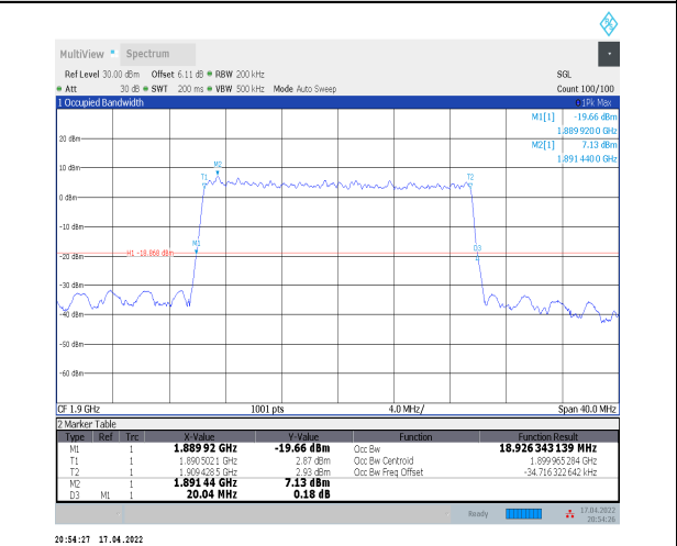
1-N2--15-20-H-9-CP-256QAM-Outer_Full-106@0-Ant-0 t0-18.926-20.040-≤20-PASS
