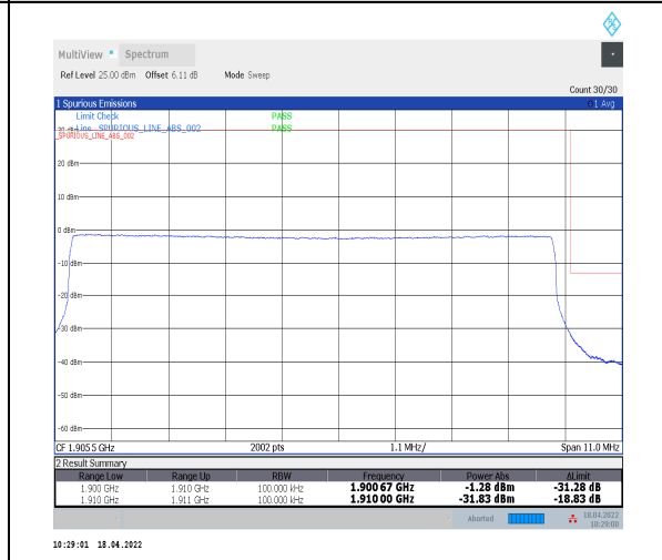
1-N2--15-10-H-6-CP-QPSK-Outer_Full-52@0-Ant0-seegraph-PASS-see graph
