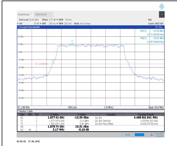
1-N2--15-5-M-4-DFT-64QAM-Outer_Full-25@0-Ant0 -4.489-5.170≤5-PASS
