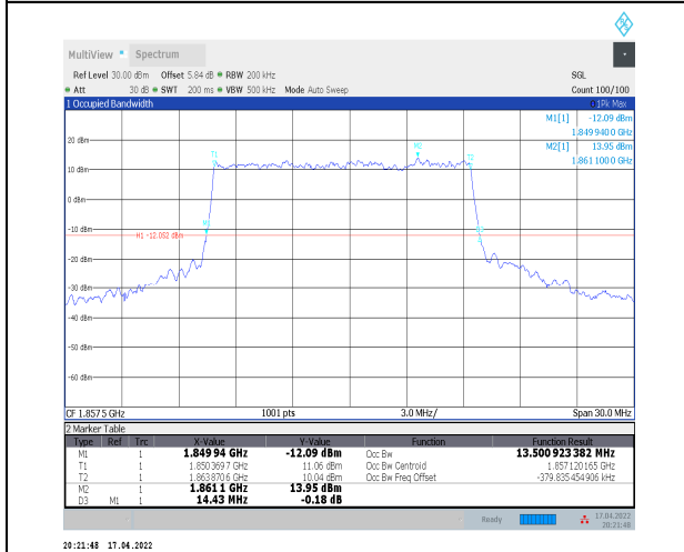
1-N2--15-15-L-1-DFT-QPSK-Outer_Full-75@0-Ant0 13.501-14.430≤15-PASS
