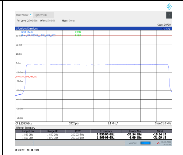
1-N2--15-20-L-6-CP-QPSK-Outer_Full-106@0-Ant0-seegraph-PASS-see graph
