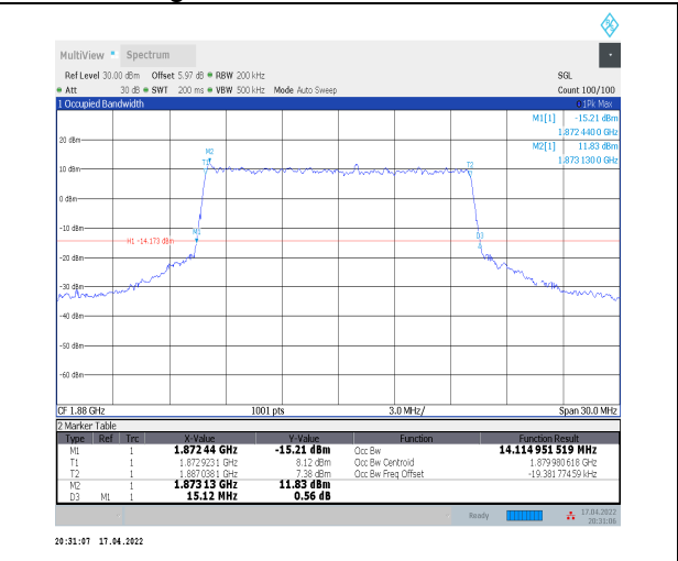
1-N2--15-15-M-7-CP-16QAM-Outer_Full-79@0-Ant0 -14.115-15.120≤15-PASS
