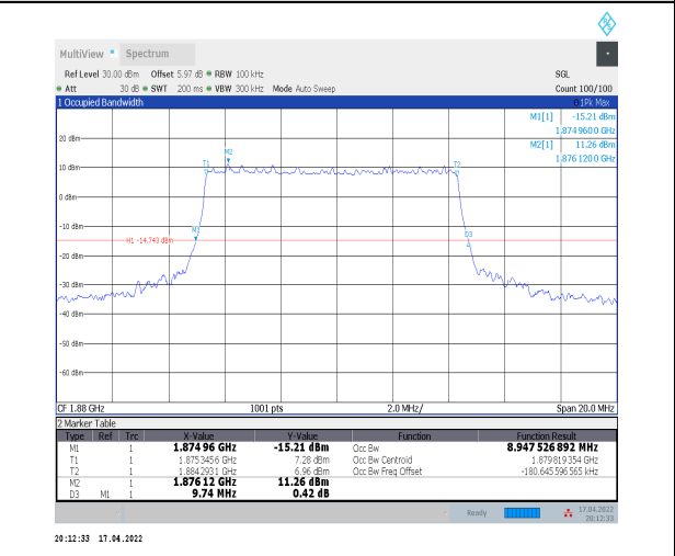
1-N2--15-10-M-4-DFT-64QAM-Outer_Full-50@0-Ant0 0-8.948-9.740-≤10-PASS
