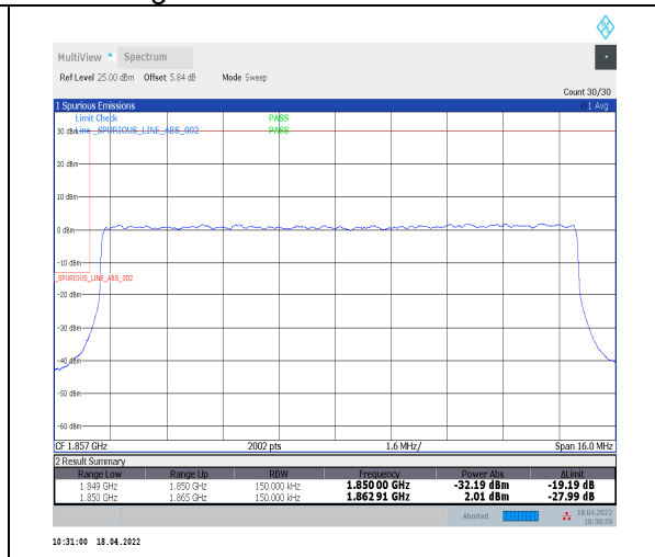
1-N2--15-15-L-3-DFT-PI2BPSK-Outer_Full-75@0-Ant0-seegraph-PASS-see graph
