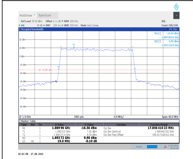
1-N2--15-20-H-4-DFT-64QAM-Outer_Full-100@0-An t0-17.856-19.000-≤20-PASS
