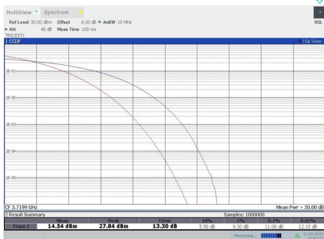
43-43-20MHz-20MHz-QPSK-QPSK-44690-44888-100RB#0-100RB#0
