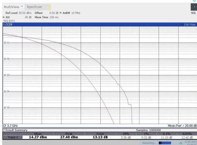
43-43-20MHz-20MHz-QPSK-QPSK-44690-44888-100RB#0-100RB#0
