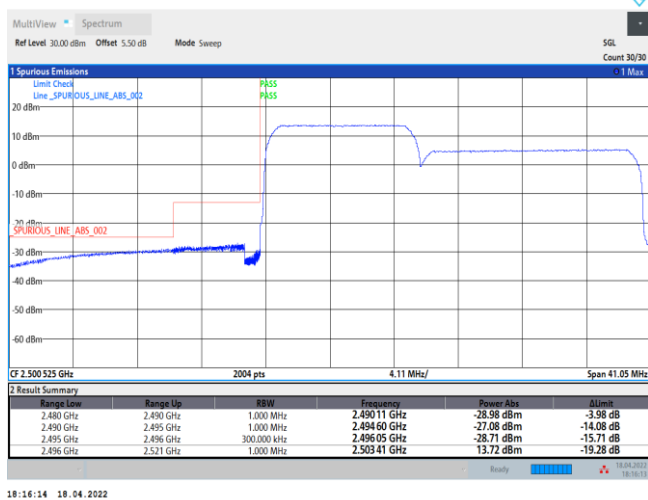
41-41-10MHz-15MHz-QPSK-QPSK-39703-39823-50RB#0-75RB#0
