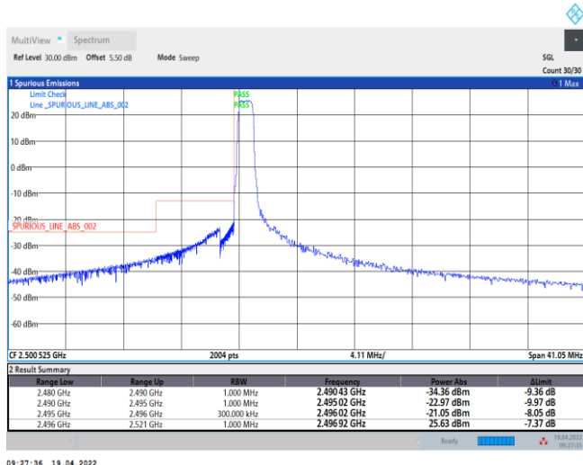
41-41-10MHz-15MHz-QPSK-QPSK-39703-39823-50RB#0-75RB#0
