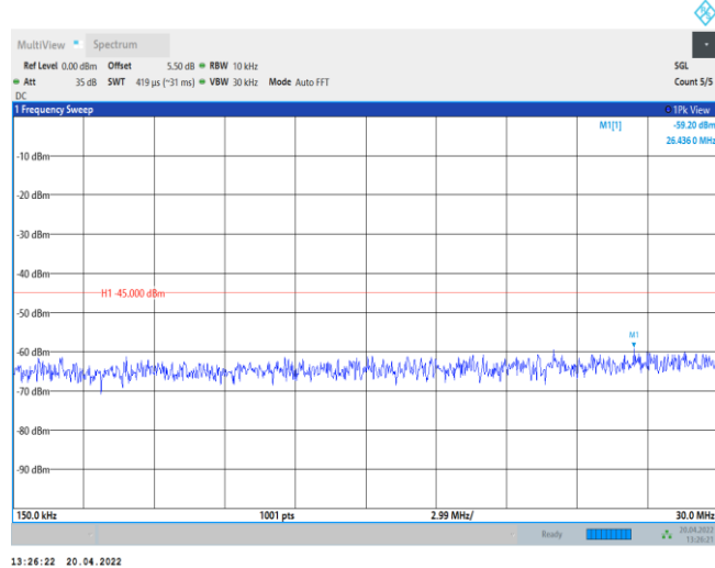
41-41-20MHz-20MHz-QPSK-QPSK-39750-39948-1RB#0-0RB#0-0.15~30MHz
