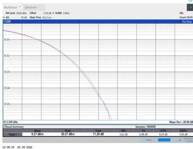
7-7-20MHz-20MHz-QPSK-QPSK-21001-21199-100RB#0-100RB#0
