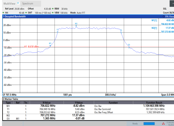
Band12-1.4MHz-QPSK-23095-6RB#0
