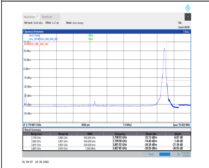
1-N78-3700-3800-PC1-30-60-H-5-CP-QPSK-Edge_1R B_Right-1@161-Ant0-1--PASS-see graph
