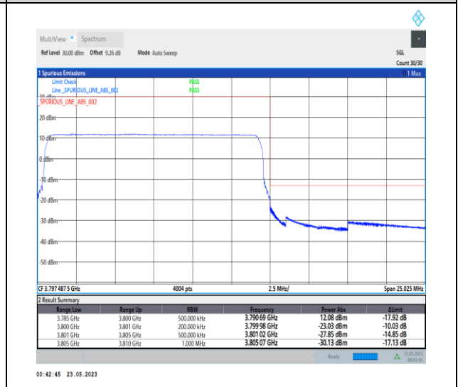
1-N78-3700-3800-PC1-30-15-H-6-CP-QPSK-Outer _Full-38@0-Ant0-1--PASS-see graph
