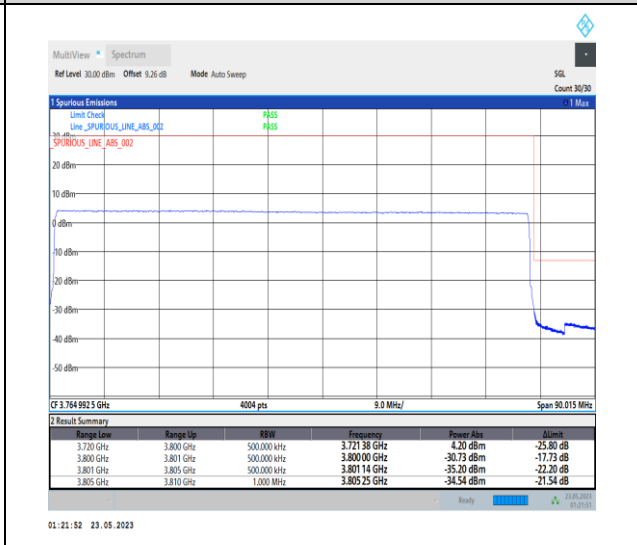
1-N78-3700-3800-PC1-30-80-H-6-CP-QPSK-Outer_Full-217@0-Ant0-1--PASS-see graph
