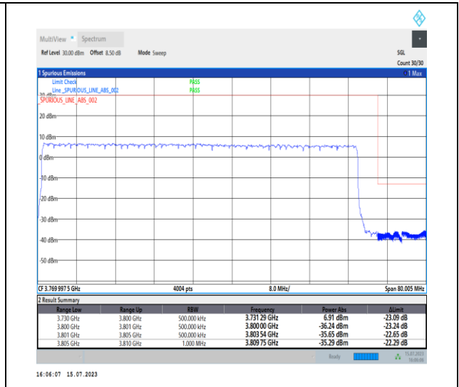
1-N78-3700-3800-PC1-30-70-H-3-DFT-PI2BPSK- Outer_Full-180@0-Ant0-1--PASS-see graph
