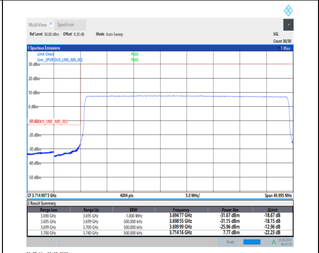
1-N78-3700-3800-PC1-30-40-L-3-DFT-PI2BPSK-Outer_Full-100@0-Ant0-1--PASS-see graph
