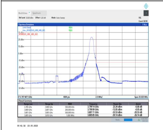
1-N78-3700-3800-PC1-30-15-H-5-CP-QPSK-Edge_1R B_Right-1@37-Ant0-1--PASS-see graph
