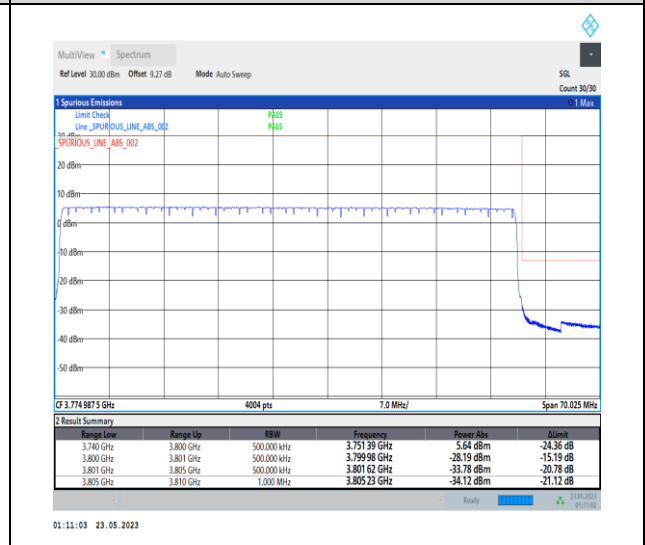
1-N78-3700-3800-PC1-30-60-H-6-CP-QPSK-Outer _Full-162@0-Ant0-1--PASS-see graph
