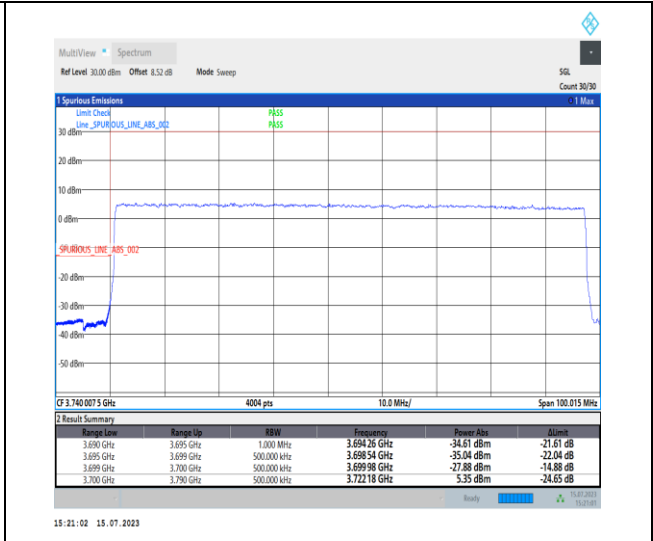
1-N78-3700-3800-PC1-30-90-L-3-DFT-PI2BPSK-Outer_Full-240@0-Ant0-1--PASS-see graph
