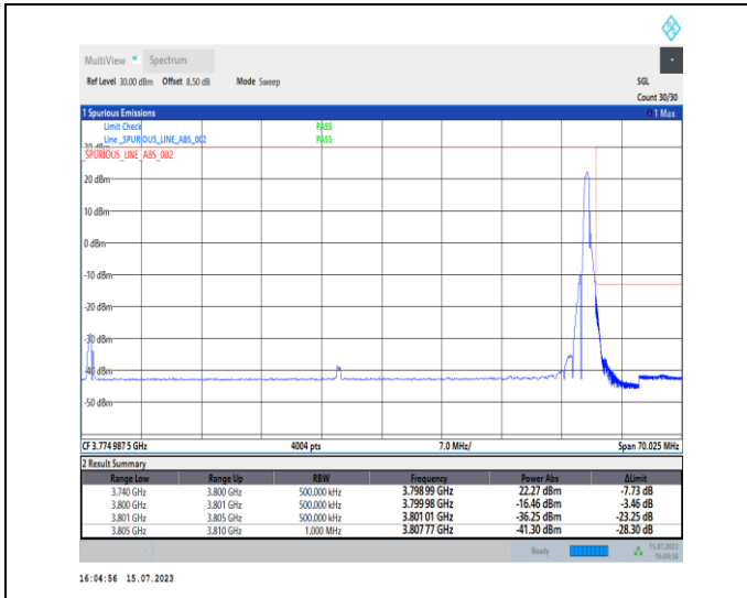
1-N78-3700-3800-PC1-30-60-H-2-DFT-PI2BPSK-Edge _1RB_Right-1@161-Ant0-1--PASS-see graph
