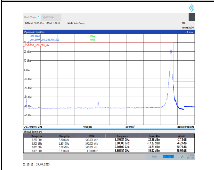
1-N78-3700-3800-PC1-30-70-H-5-CP-QPSK-Edge_1R B_Right-1@188-Ant0-1--PASS-see graph
