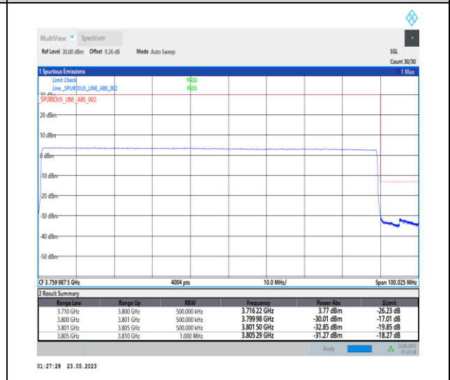
1-N78-3700-3800-PC1-30-90-H-6-CP-QPSK-Outer_Full-245@0-Ant0-1--PASS-see graph
