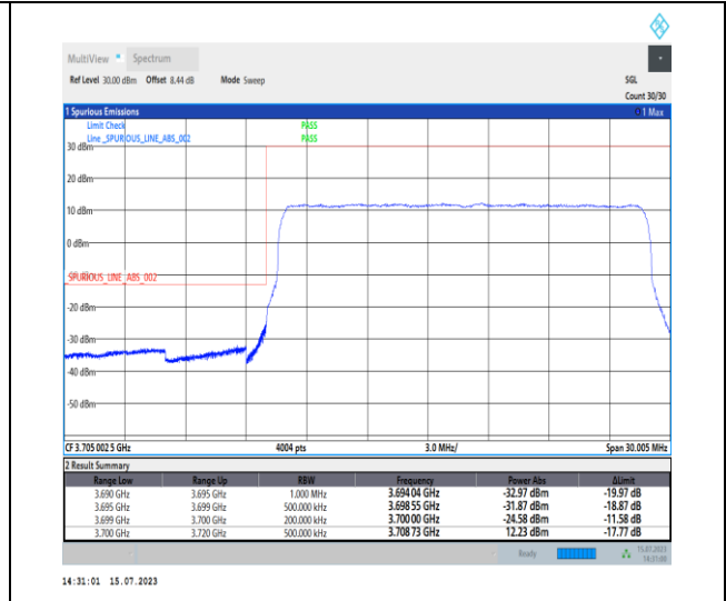
1-N78-3700-3800-PC1-30-20-L-3-DFT-PI2BPSK-Outer_Full-50@0-Ant0-1--PASS-see graph
