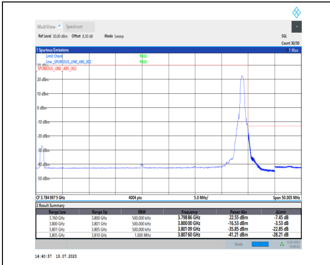
1-N78-3700-3800-PC1-30-40-H-2-DFT-PI2BPSK-Edge_1RB_Right-1@105-Ant0-1--PASS-see graph
