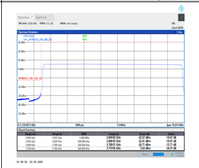
1-N78-3700-3800-PC1-30-60-L-6-CP-QPSK-Outer_Full-162@0-Ant0-1--PASS-see graph
