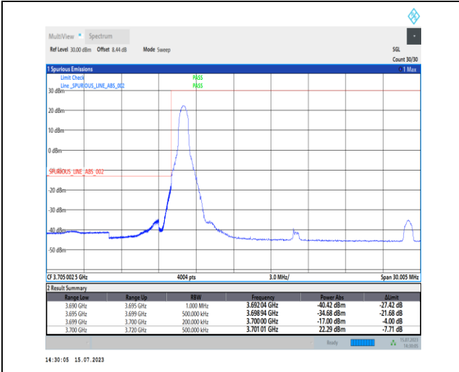
1-N78-3700-3800-PC1-30-20-L-1-DFT-PI2BPSK-Edge_1_RB_Left-1@0-Ant0-1--PASS-see graph
