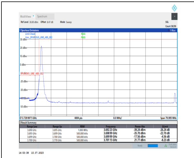
1-N78-3700-3800-PC1-30-70-L-1-DFT-PI2BPSK-Edge_1_RB_Left-1@0-Ant0-1--PASS-see graph
