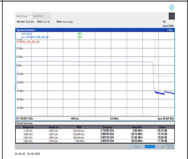
1-N78-3700-3800-PC1-30-70-H-6-CP-QPSK-Outer _Full-189@0-Ant0-1--PASS-see graph
