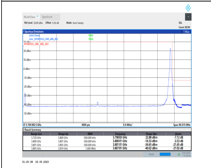
1-N78-3700-3800-PC1-30-80-H-5-CP-QPSK-Edge_1RB_Right-1@216-Ant0-1--PASS-see graph
