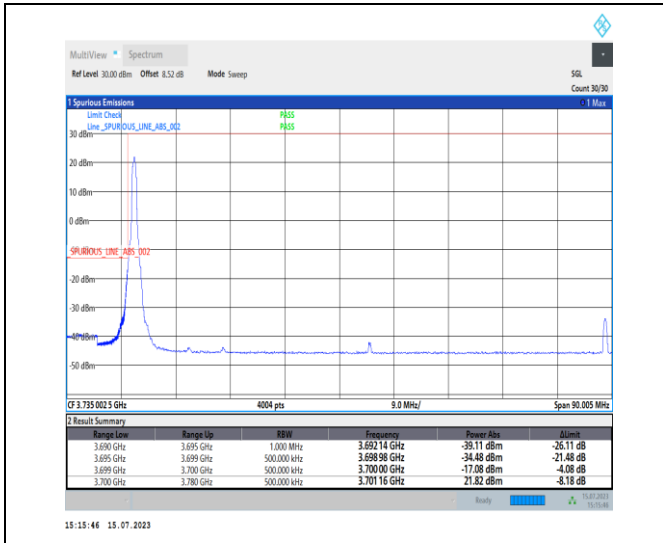
1-N78-3700-3800-PC1-30-80-L-1-DFT-PI2BPSK-Edge_1_RB_Left-1@0-Ant0-1--PASS-see graph
