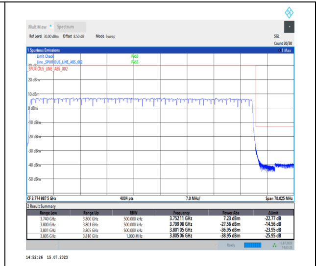
1-N78-3700-3800-PC1-30-60-H-3-DFT-PI2BPSK- Outer_Full-162@0-Ant0-1--PASS-see graph
