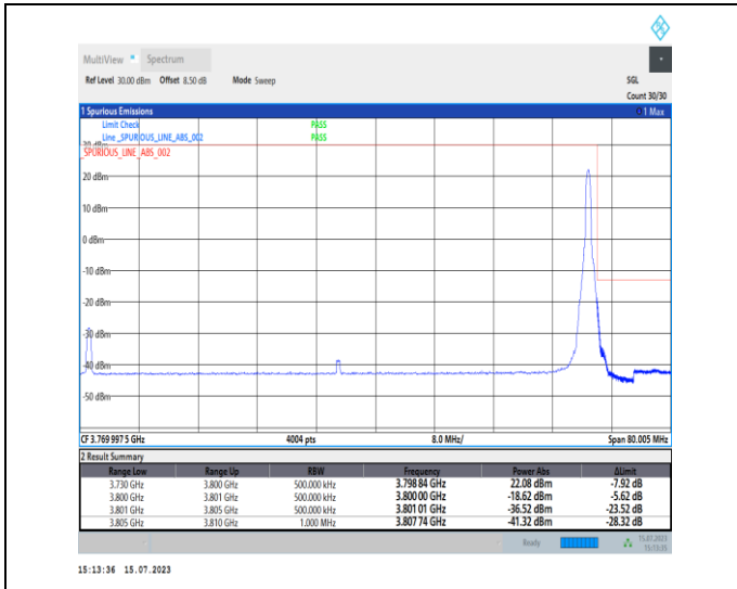
1-N78-3700-3800-PC1-30-70-H-2-DFT-PI2BPSK-Edge _1RB_Right-1@188-Ant0-1--PASS-see graph
