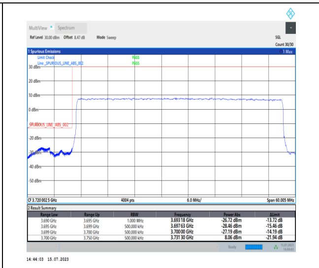
1-N78-3700-3800-PC1-30-50-L-3-DFT-PI2BPSK-Outer_Full-128@0-Ant0-1--PASS-see graph
