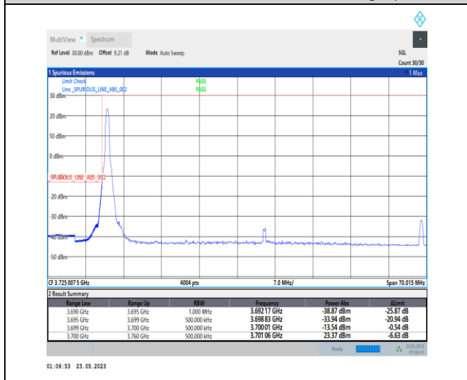
1-N78-3700-3800-PC1-30-60-L-4-CP-QPSK-Edge_1_RB_Left-1@0-Ant0-1--PASS-see graph
