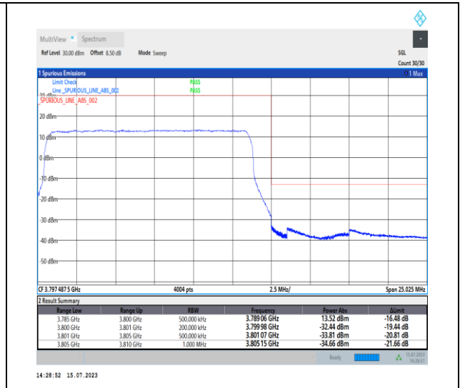
1-N78-3700-3800-PC1-30-15-H-3-DFT-PI2BPSK- Outer_Full-36@0-Ant0-1--PASS-see graph
