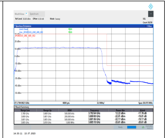
1-N78-3700-3800-PC1-30-20-H-3-DFT-PI2BPSK- Outer_Full-50@0-Ant0-1--PASS-see graph
