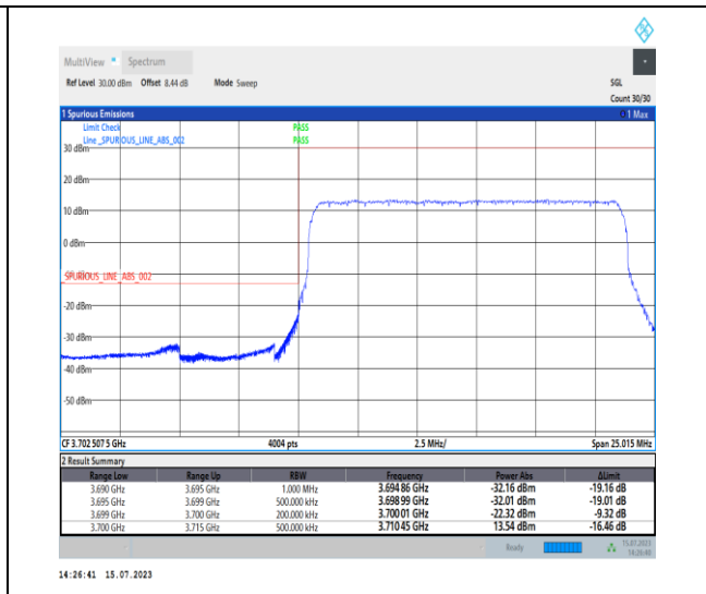
1-N78-3700-3800-PC1-30-15-L-3-DFT-PI2BPSK-Outer_Full-36@0-Ant0-1--PASS-see graph
