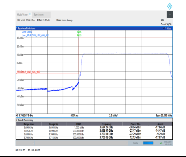
1-N78-3700-3800-PC1-30-15-L-6-CP-QPSK-Outer_Full-38@0-Ant0-1--PASS-see graph
