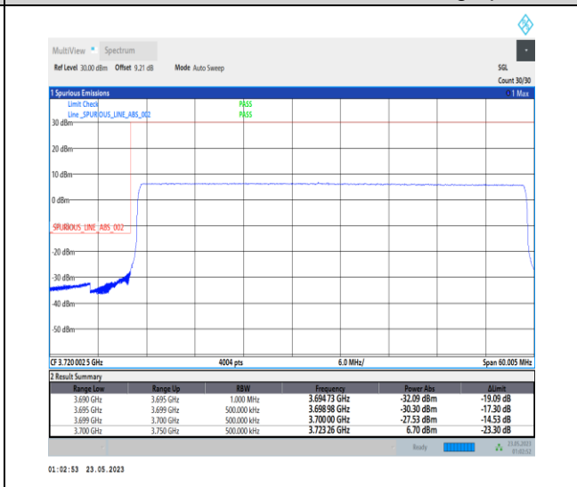
1-N78-3700-3800-PC1-30-50-L-6-CP-QPSK-Outer_Full-133@0-Ant0-1--PASS-see graph
