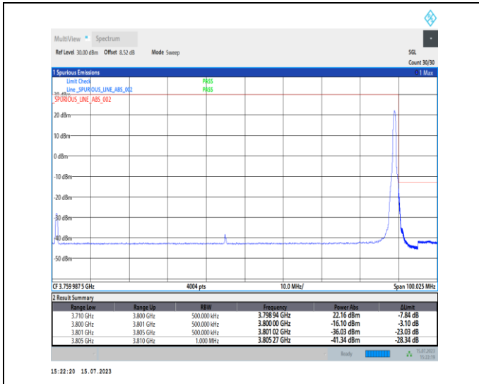
1-N78-3700-3800-PC1-30-90-H-2-DFT-PI2BPSK-Edge _1RB_Right-1@244-Ant0-1--PASS-see graph
