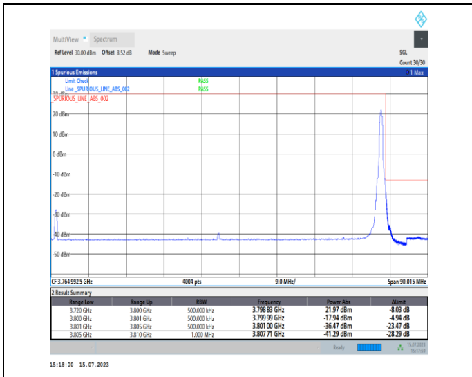
1-N78-3700-3800-PC1-30-80-H-2-DFT-PI2BPSK-Edge_1RB_Right-1@216-Ant0-1--PASS-see graph
