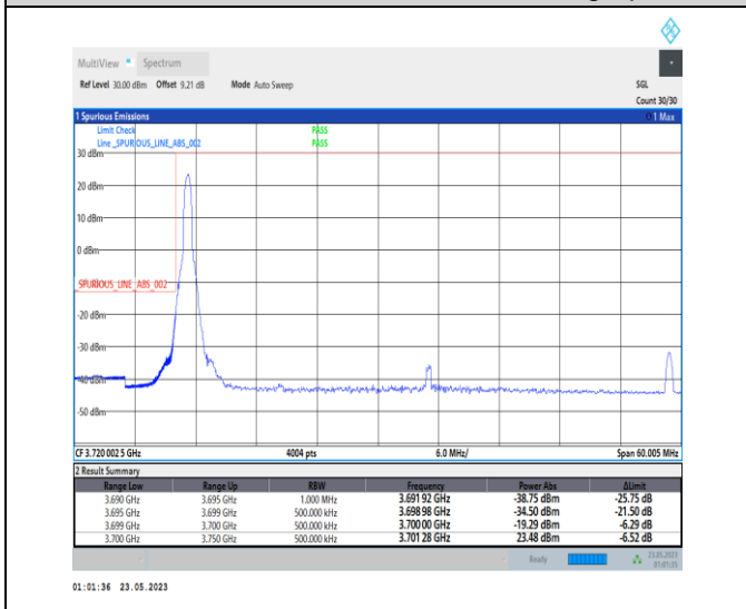
1-N78-3700-3800-PC1-30-50-L-4-CP-QPSK-Edge_1_RB_Left-1@0-Ant0-1--PASS-see graph
