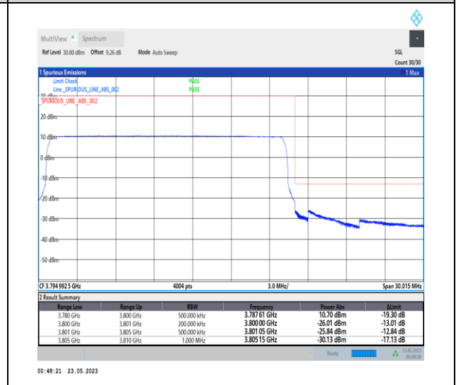
1-N78-3700-3800-PC1-30-20-H-6-CP-QPSK-Outer _Full-51@0-Ant0-1--PASS-see graph
