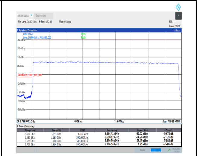
1-N78-3700-3800-PC1-30-100-L-3-DFT-PI2BPSK-Outer_Full-270@0-Ant0-1--PASS-see graph
