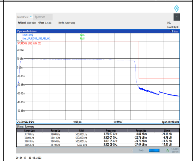
1-N78-3700-3800-PC1-30-30-H-6-CP-QPSK-Outer _Full-78@0-Ant0-1--PASS-see graph
