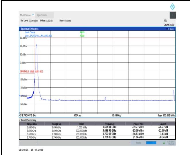
1-N78-3700-3800-PC1-30-90-L-1-DFT-PI2BPSK-Edge_1_RB_Left-1@0-Ant0-1--PASS-see graph
