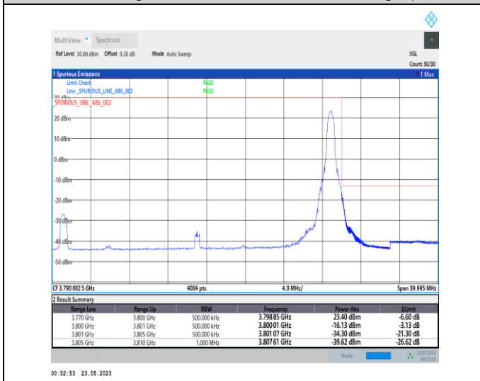
1-N78-3700-3800-PC1-30-30-H-5-CP-QPSK-Edge_1R B_Right-1@77-Ant0-1--PASS-see graph
