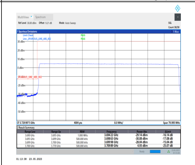
1-N78-3700-3800-PC1-30-70-L-6-CP-QPSK-Outer_Full-189@0-Ant0-1--PASS-see graph
