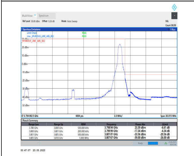
1-N78-3700-3800-PC1-30-20-H-5-CP-QPSK-Edge_1R B_Right-1@50-Ant0-1--PASS-see graph
