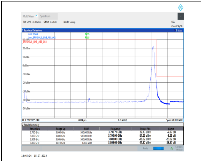
1-N78-3700-3800-PC1-30-50-H-2-DFT-PI2BPSK-Edge _1RB_Right-1@132-Ant0-1--PASS-see graph
