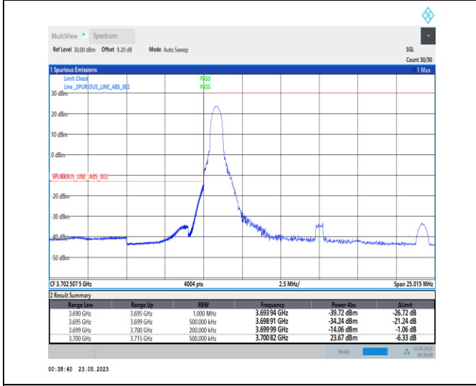
1-N78-3700-3800-PC1-30-15-L-4-CP-QPSK-Edge_1RB_Left-1@0-Ant0-1--PASS-see graph
