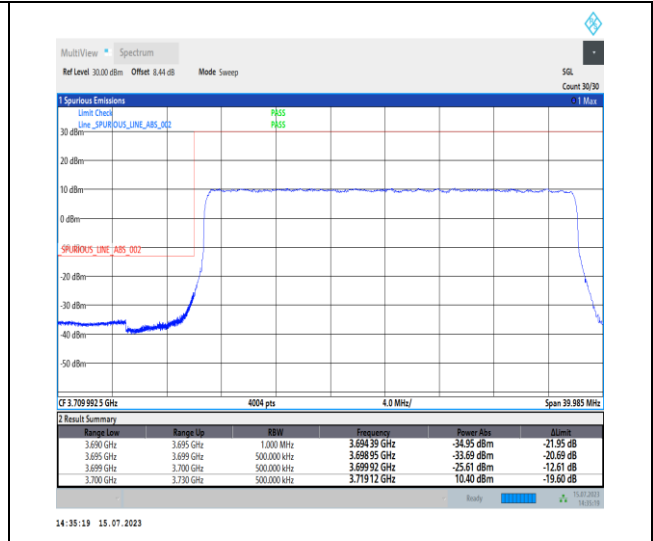
1-N78-3700-3800-PC1-30-30-L-3-DFT-PI2BPSK-Outer_Full-75@0-Ant0-1--PASS-see graph
