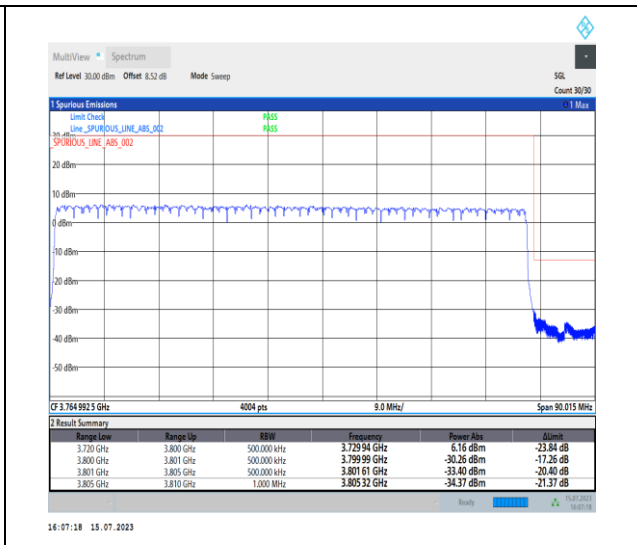
1-N78-3700-3800-PC1-30-80-H-3-DFT-PI2BPSK-Outer_Full-216@0-Ant0-1--PASS-see graph
