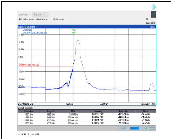
1-N78-3700-3800-PC1-30-15-L-1-DFT-PI2BPSK-Edge_e_1RB_Left-1@0-Ant0-1--PASS-see graph
