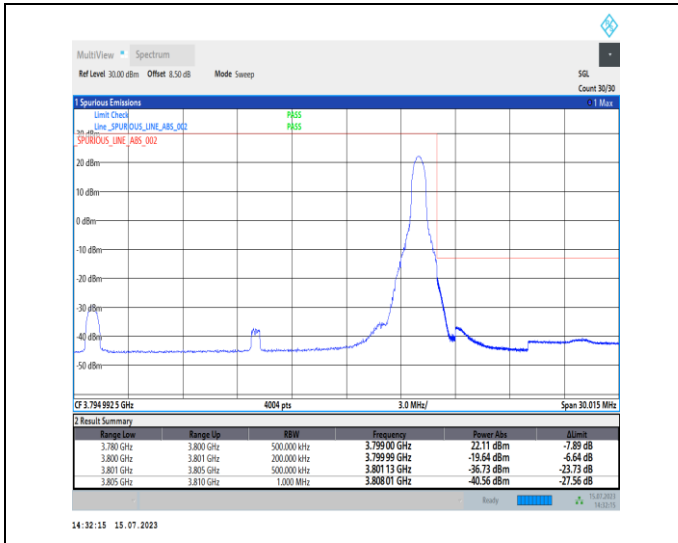
1-N78-3700-3800-PC1-30-20-H-2-DFT-PI2BPSK-Edge _1RB_Right-1@50-Ant0-1--PASS-see graph
