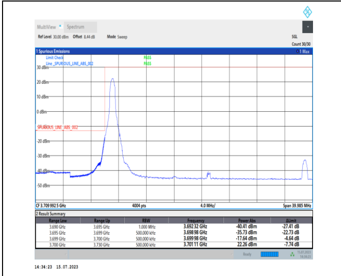
1-N78-3700-3800-PC1-30-30-L-1-DFT-PI2BPSK-Edge_1RB_Left-1@0-Ant0-1--PASS-see graph
