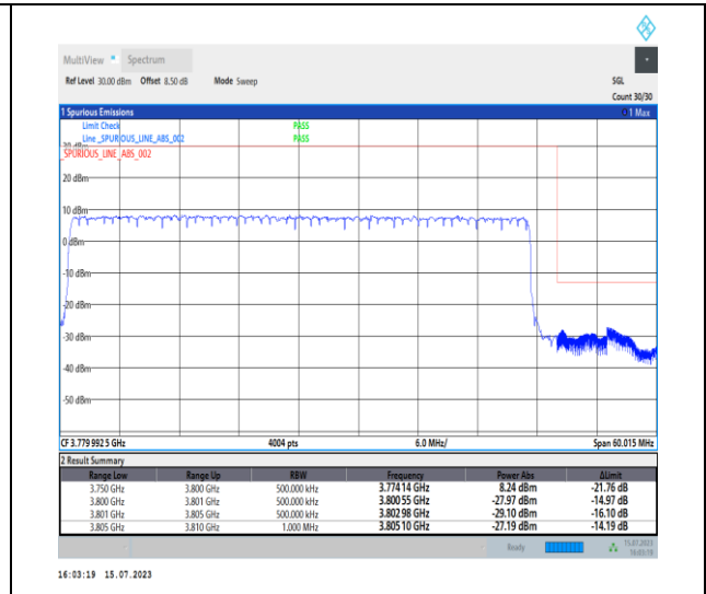
1-N78-3700-3800-PC1-30-50-H-3-DFT-PI2BPSK- Outer_Full-128@0-Ant0-1--PASS-see graph
