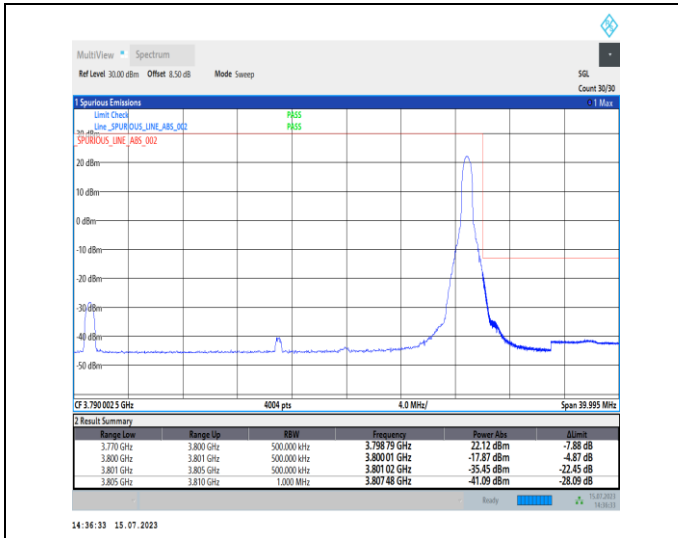
1-N78-3700-3800-PC1-30-30-H-2-DFT-PI2BPSK-Edge _1RB_Right-1@77-Ant0-1--PASS-see graph
