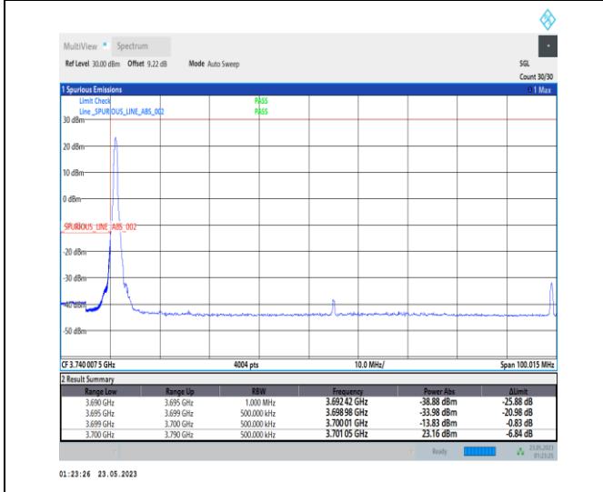
1-N78-3700-3800-PC1-30-90-L-4-CP-QPSK-Edge_1_RB_Left-1@0-Ant0-1--PASS-see graph
