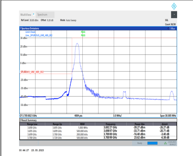
1-N78-3700-3800-PC1-30-20-L-4-CP-QPSK-Edge_1_RB_Left-1@0-Ant0-1--PASS-see graph
