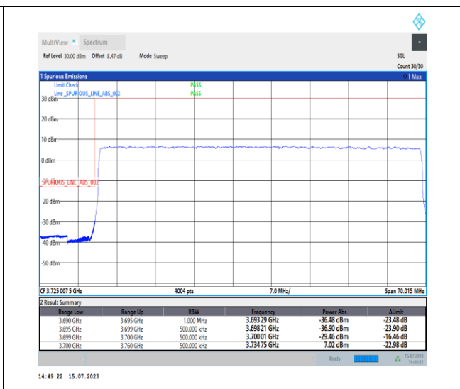
1-N78-3700-3800-PC1-30-60-L-3-DFT-PI2BPSK-Outer_Full-162@0-Ant0-1--PASS-see graph
