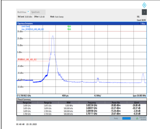
1-N78-3700-3800-PC1-30-30-L-4-CP-QPSK-Edge_1RB_Left-1@0-Ant0-1--PASS-see graph
