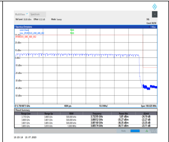
1-N78-3700-3800-PC1-30-90-H-3-DFT-PI2BPSK-Outer_Full-240@0-Ant0-1--PASS-see graph
