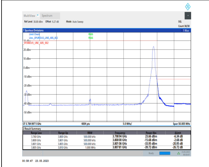
1-N78-3700-3800-PC1-30-40-H-5-CP-QPSK-Edge_1RB_Right-1@105-Ant0-1--PASS-see graph
