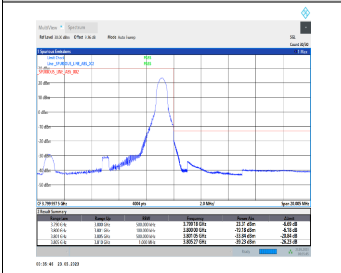
1-N78-3700-3800-PC1-30-10-H-5-CP-QPSK-Edge_1R B_Right-1@23-Ant0-1--PASS-see graph
