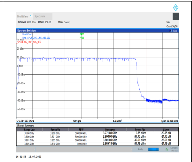
1-N78-3700-3800-PC1-30-40-H-3-DFT-PI2BPSK-Outer_Full-100@0-Ant0-1--PASS-see graph
