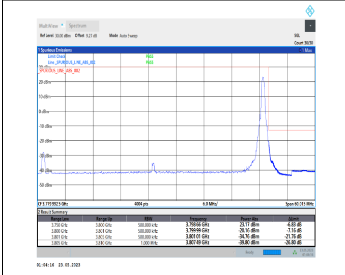
1-N78-3700-3800-PC1-30-50-H-5-CP-QPSK-Edge_1R B_Right-1@132-Ant0-1--PASS-see graph
