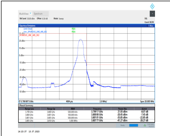
1-N78-3700-3800-PC1-30-10-H-2-DFT-PI2BPSK-Edge _1RB_Right-1@23-Ant0-1--PASS-see graph
