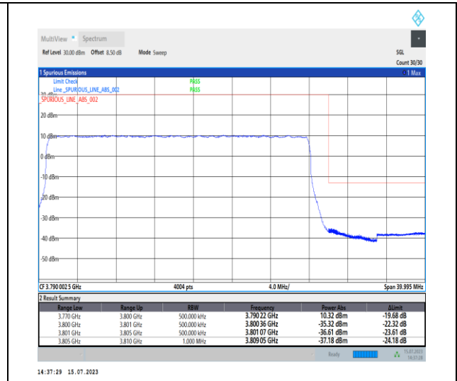
1-N78-3700-3800-PC1-30-30-H-3-DFT-PI2BPSK- Outer_Full-75@0-Ant0-1--PASS-see graph
