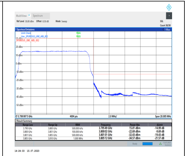
1-N78-3700-3800-PC1-30-10-H-3-DFT-PI2BPSK- Outer_Full-24@0-Ant0-1--PASS-see graph
