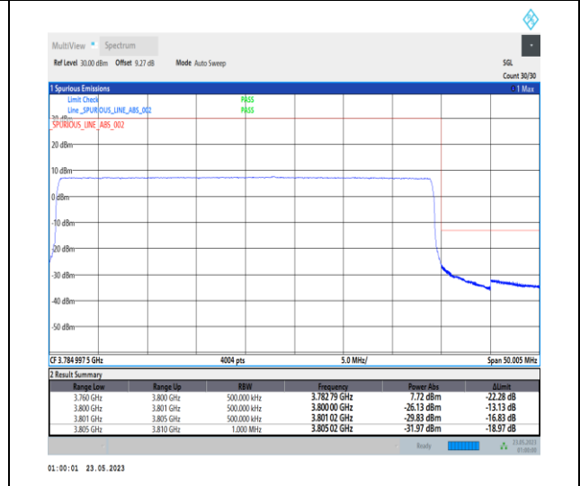
1-N78-3700-3800-PC1-30-40-H-6-CP-QPSK-Outer_Full-106@0-Ant0-1--PASS-see graph
