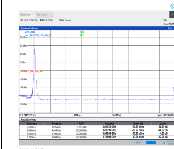
1-N78-3700-3800-PC1-30-100-L-1-DFT-PI2BPSK-Edge_1RB_Left-1@0-Ant0-1--PASS-see graph
