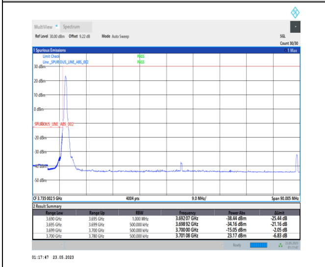
1-N78-3700-3800-PC1-30-80-L-4-CP-QPSK-Edge_1_RB_Left-1@0-Ant0-1--PASS-see graph
