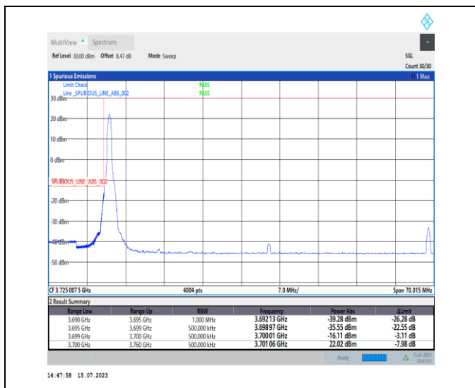
1-N78-3700-3800-PC1-30-60-L-1-DFT-PI2BPSK-Edge_1_RB_Left-1@0-Ant0-1--PASS-see graph
