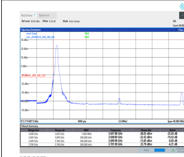
1-N78-3700-3800-PC1-30-40-L-1-DFT-PI2BPSK-Edge_1_RB_Left-1@0-Ant0-1--PASS-see graph
