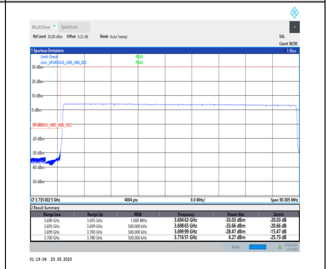
1-N78-3700-3800-PC1-30-80-L-6-CP-QPSK-Outer_Full-217@0-Ant0-1--PASS-see graph
