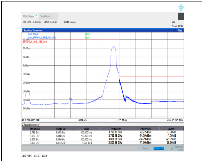
1-N78-3700-3800-PC1-30-15-H-2-DFT-PI2BPSK-Edge _1RB_Right-1@37-Ant0-1--PASS-see graph
