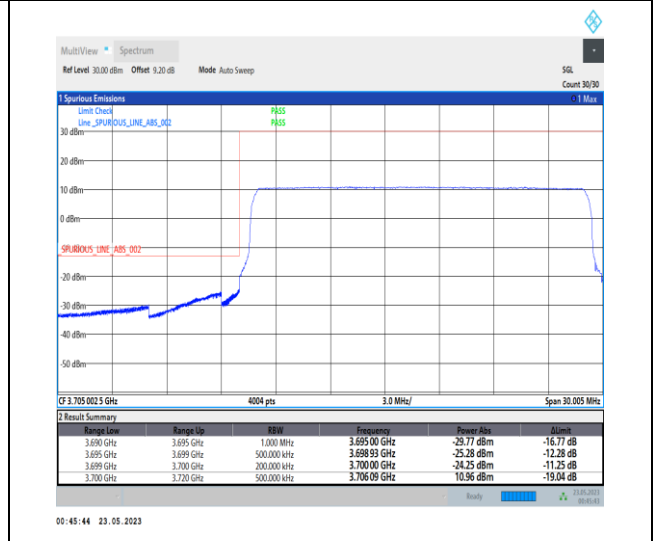
1-N78-3700-3800-PC1-30-20-L-6-CP-QPSK-Outer_Full-51@0-Ant0-1--PASS-see graph
