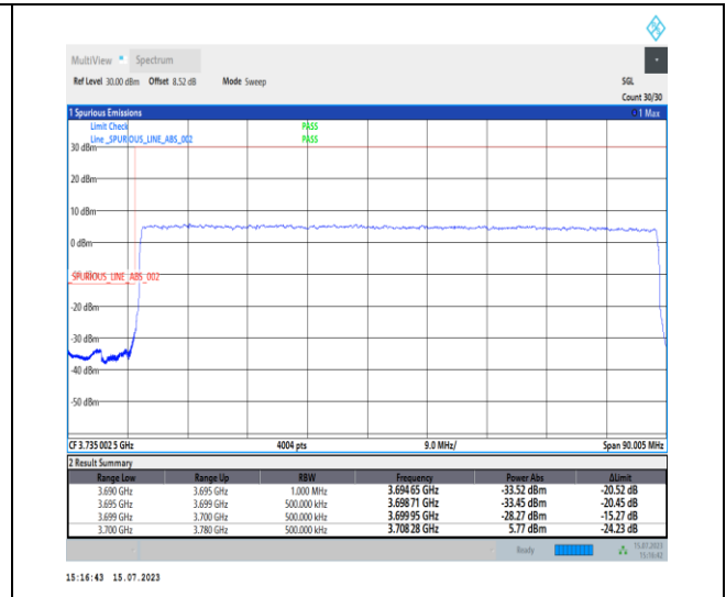
1-N78-3700-3800-PC1-30-80-L-3-DFT-PI2BPSK-Outer_Full-216@0-Ant0-1--PASS-see graph
