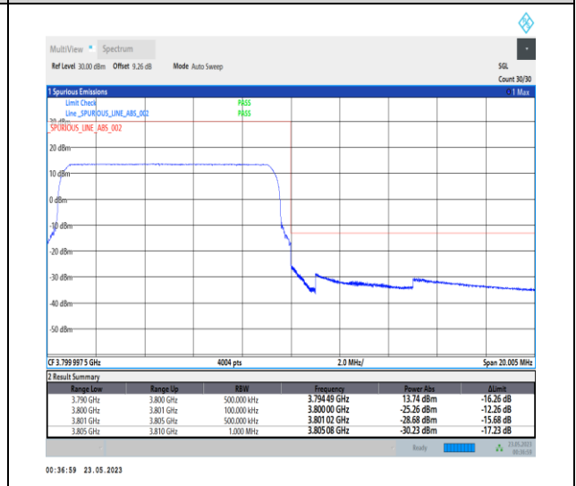
1-N78-3700-3800-PC1-30-10-H-6-CP-QPSK-Outer _Full-24@0-Ant0-1--PASS-see graph
