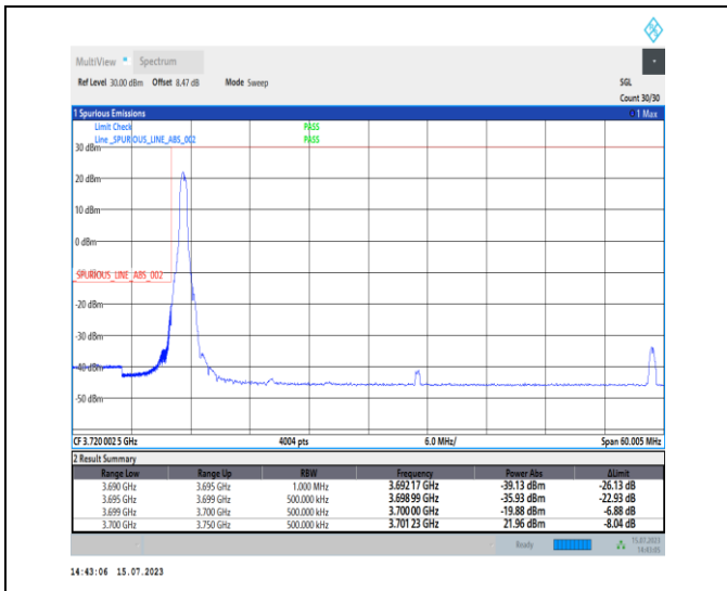
1-N78-3700-3800-PC1-30-50-L-1-DFT-PI2BPSK-Edge_1_RB_Left-1@0-Ant0-1--PASS-see graph
