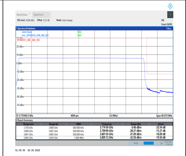
1-N78-3700-3800-PC1-30-50-H-6-CP-QPSK-Outer _Full-133@0-Ant0-1--PASS-see graph
