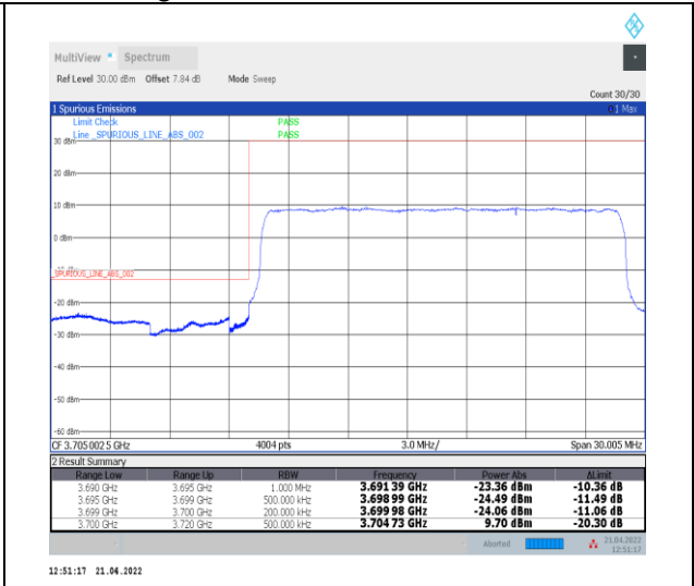
1-N78-3700-3800--30-20-L-3-DFT-PI2BPSK-Outer_Full-50@0-Ant0-PASS-see graph
