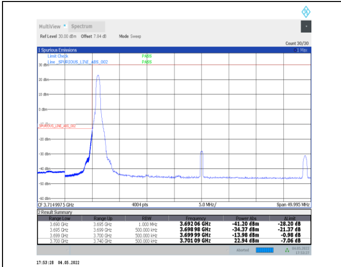
1-N78-3700-3800--30-40-L-1-DFT-PI2BPSK-Edge_1R_B_Left-1@0-Ant0-PASS-see graph
