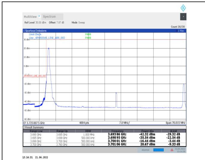
1-N78-3700-3800--30-60-L-1-DFT-PI2BPSK-Edge_1R_B_Left-1@0-Ant0-PASS-see graph
