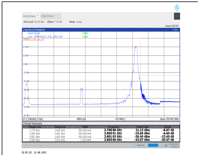
1-N78-3700-3800--30-30-H-2-DFT-PI2BPSK-Edge_1R_B_Right-1@77-Ant0-PASS-see graph
