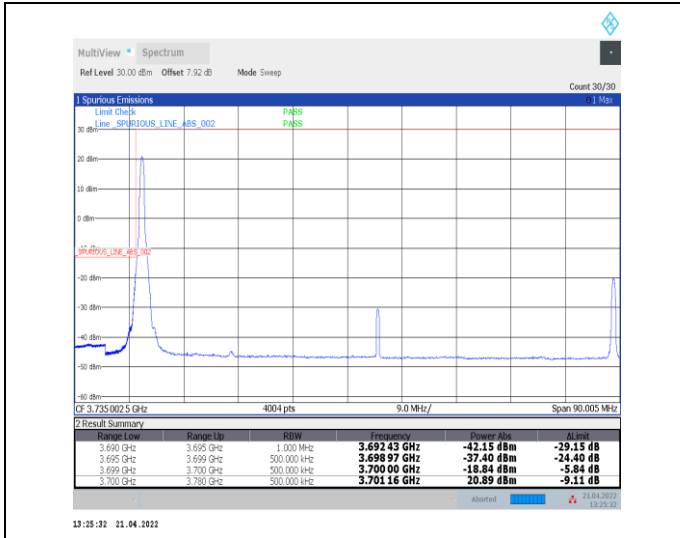
1-N78-3700-3800--30-80-L-1-DFT-PI2BPSK-Edge_1R_B_Left-1@0-Ant0-PASS-see graph
