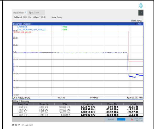
1-N78-3700-3800--30-80-H-6-CP-QPSK-Outer_Full-217@0-Ant0-PASS-see graph
