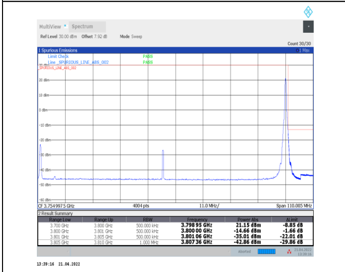
1-N78-3700-3800--30-100-H-5-CP-QPSK-Edge_1RB_Right-1@272-Ant0-PASS-see graph
