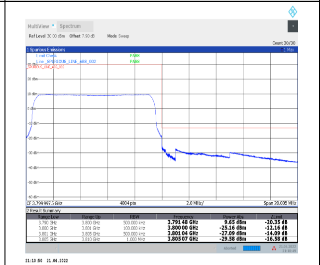
1-N78-3700-3800--30-10-H-6-CP-QPSK-Outer_Full-24@0-Ant0-PASS-see graph
