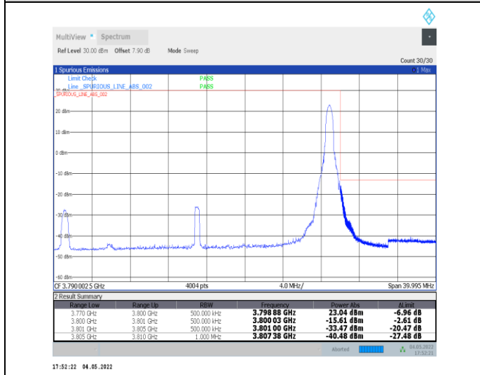
1-N78-3700-3800--30-30-H-5-CP-QPSK-Edge_1RB_Right-1@77-Ant0-PASS-see graph
