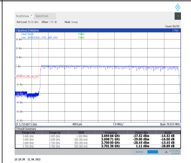
1-N78-3700-3800--30-60-L-6-CP-QPSK-Outer_Ful I-162@0-Ant0-PASS-see graph
