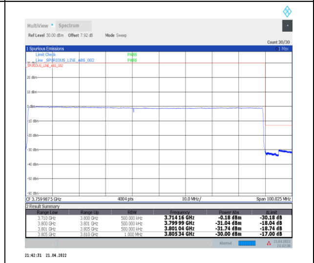
1-N78-3700-3800--30-90-H-6-CP-QPSK-Outer_Full-245@0-Ant0-PASS-see graph
