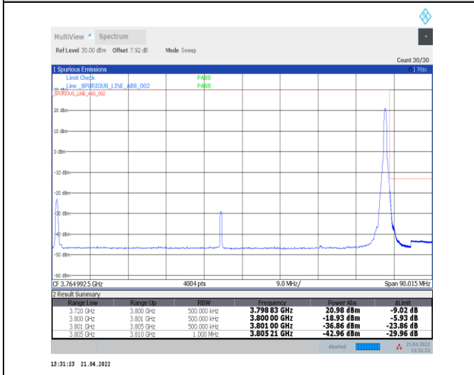
1-N78-3700-3800--30-80-H-5-CP-QPSK-Edge_1RB_Right-1@216-Ant0-PASS-see graph
