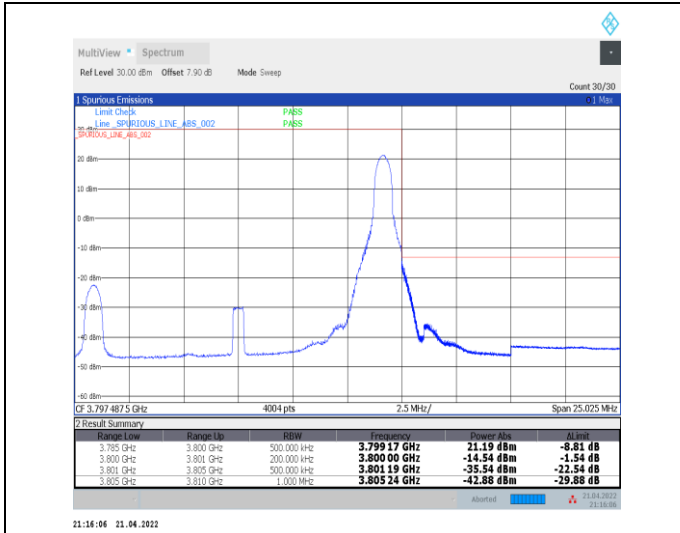
1-N78-3700-3800--30-15-H-2-DFT-PI2BPSK-Edge_1R_B_Right-1@37-Ant0-PASS-see graph
