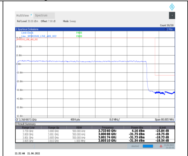
1-N78-3700-3800--30-70-H-3-DFT-PI2BPSK-Outer_Full-180@0-Ant0-PASS-see graph
