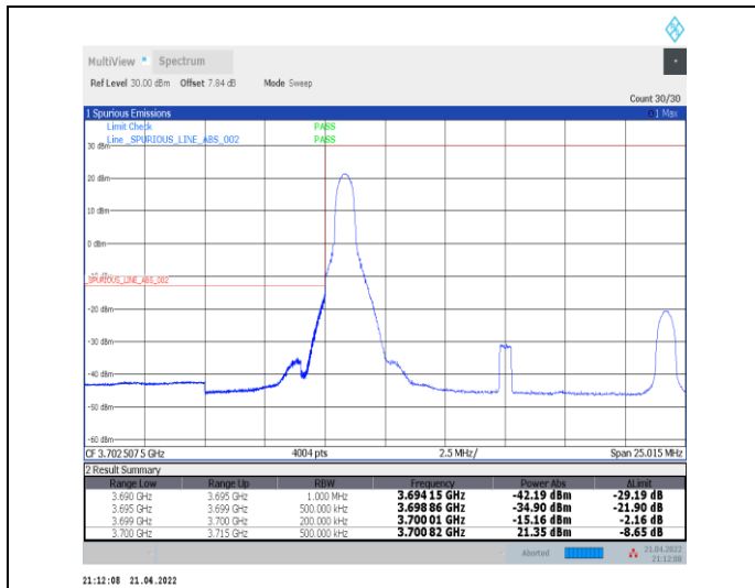
1-N78-3700-3800--30-15-L-1-DFT-PI2BPSK-Edge_1R_B_Left-1@0-Ant0-PASS-see graph
