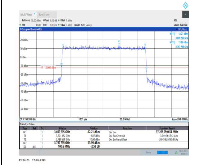
1-N78-3700-3800-PC1-30-100-M-8-CP-64QAM-Outer_Full-273@0-Ant0-97.226-100.600-≤100-PASS
