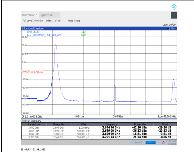
1-N78-3700-3800--30-40-L-4-CP-QPSK-Edge_1RB_L_eft-1@0-Ant0-PASS-see graph
