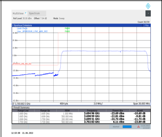
1-N78-3700-3800--30-20-L-6-CP-QPSK-Outer_Ful-l-51@0-Ant0-PASS-see graph
