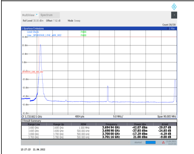
1-N78-3700-3800--30-80-L-4-CP-QPSK-Edge_1RB_L_eff-1@0-Ant0-PASS-see graph
