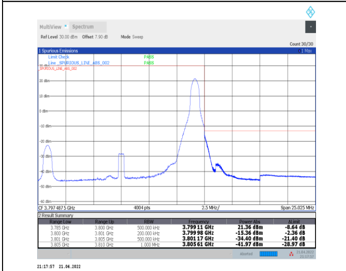
1-N78-3700-3800--30-15-H-5-CP-QPSK-Edge_1RB_R ight-1@37-Ant0-PASS-see graph
