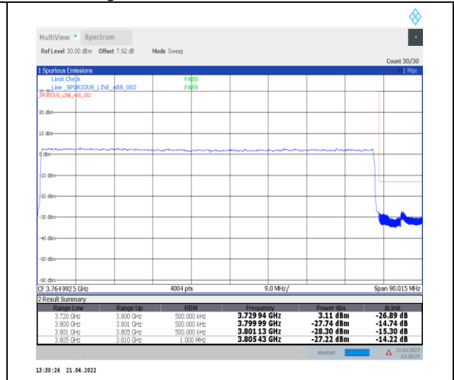
1-N78-3700-3800--30-80-H-3-DFT-PI2BPSK-Outer_Full-216@0-Ant0-PASS-see graph
