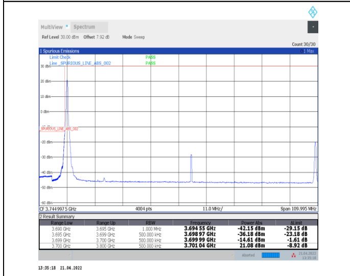
1-N78-3700-3800--30-100-L-4-CP-QPSK-Edge_1RB_Left-1@0-Ant0-PASS-see graph
