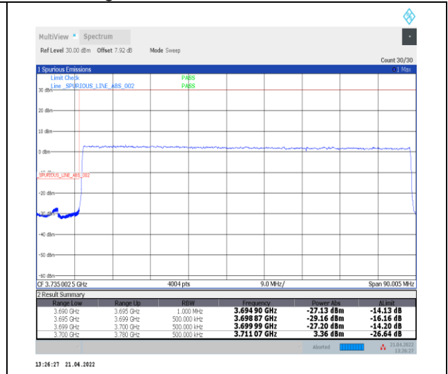
1-N78-3700-3800--30-80-L-3-DFT-PI2BPSK-Outer_Full-216@0-Ant0-PASS-see graph
