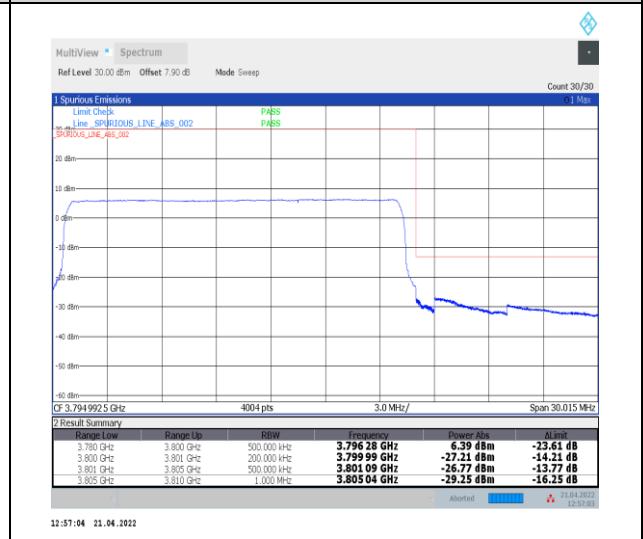
1-N78-3700-3800--30-20-H-6-CP-QPSK-Outer_Fu ll-51@0-Ant0-PASS-see graph
