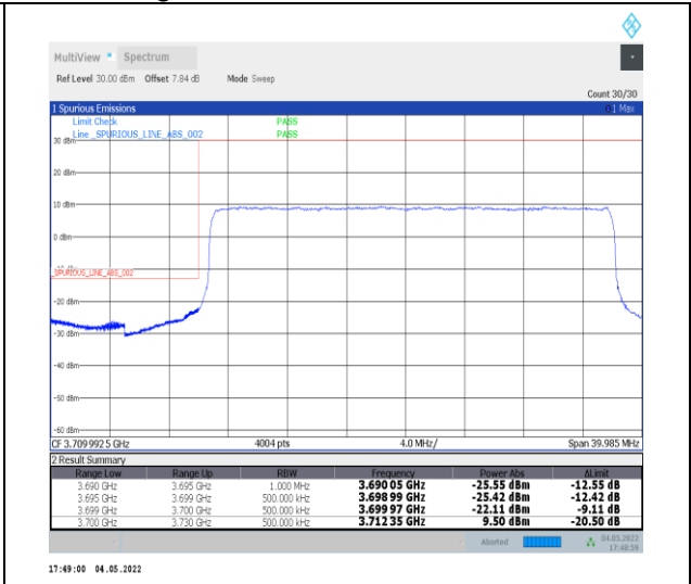
1-N78-3700-3800--30-30-L-3-DFT-PI2BPSK-Outer_Full-75@0-Ant0-PASS-see graph
