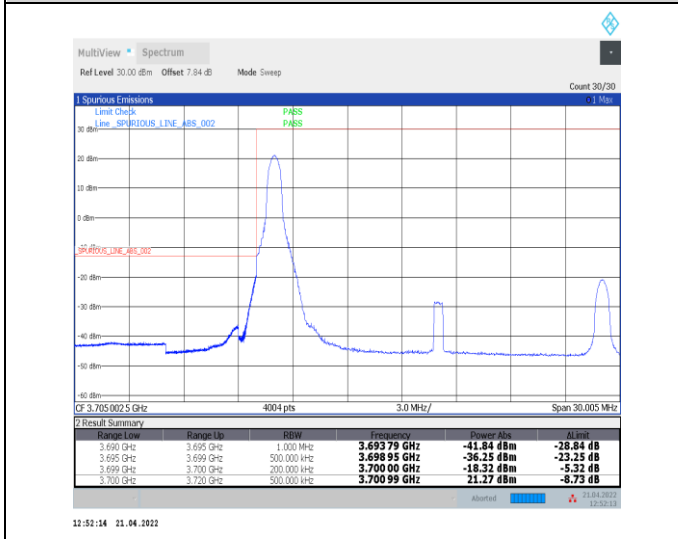
1-N78-3700-3800--30-20-L-4-CP-QPSK-Edge_1RB_L_eff-1@0-Ant0-PASS-see graph
