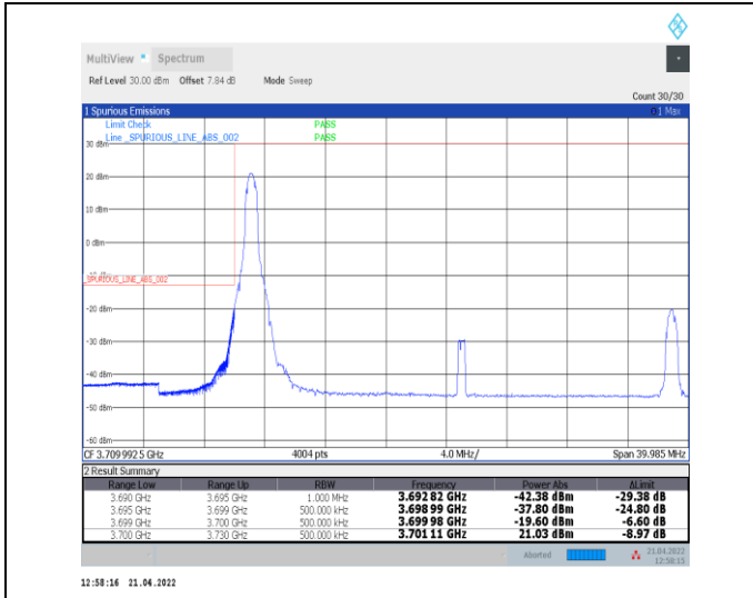
1-N78-3700-3800--30-30-L-1-DFT-PI2BPSK-Edge_1R_B_Left-1@0-Ant0-PASS-see graph
