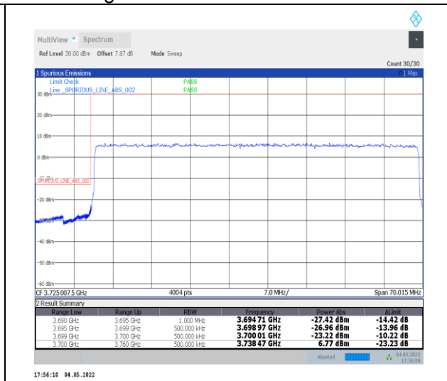
1-N78-3700-3800--30-60-L-3-DFT-PI2BPSK-Outer_Full-162@0-Ant0-PASS-see graph
