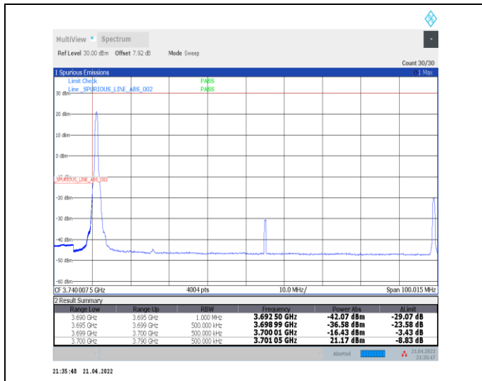
1-N78-3700-3800--30-90-L-1-DFT-PI2BPSK-Edge_1R_B_Left-1@0-Ant0-PASS-see graph
