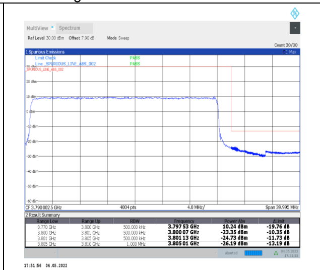
1-N78-3700-3800--30-30-H-3-DFT-PI2BPSK-Outer_Full-75@0-Ant0-PASS-see graph
