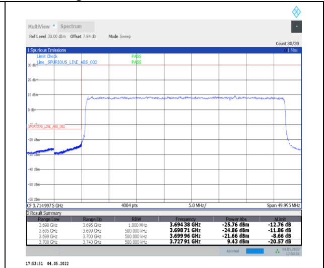
1-N78-3700-3800--30-40-L-3-DFT-PI2BPSK-Outer_Full-100@0-Ant0-PASS-see graph
