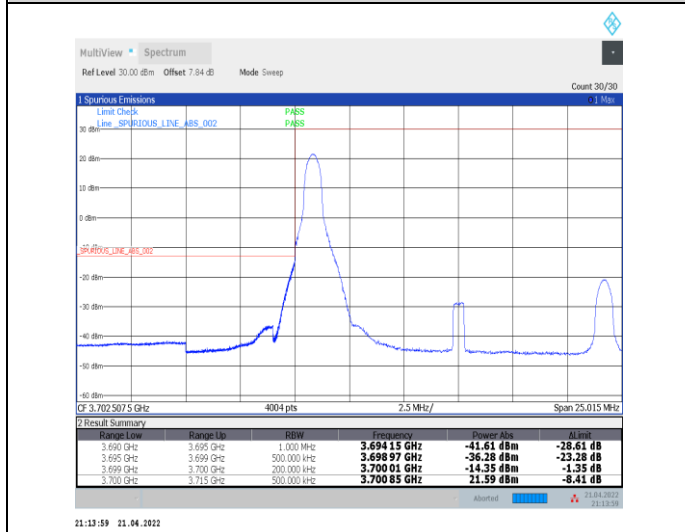
1-N78-3700-3800--30-15-L-4-CP-QPSK-Edge_1RB_L_eff-1@0-Ant0-PASS-see graph
