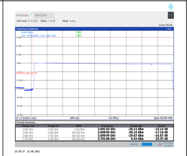
1-N78-3700-3800--30-80-L-6-CP-QPSK-Outer_Ful I-217@0-Ant0-PASS-see graph
