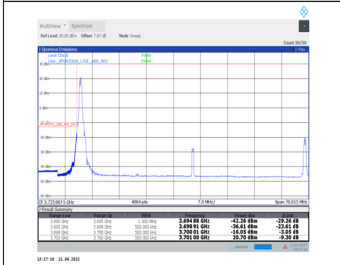
1-N78-3700-3800--30-60-L-4-CP-QPSK-Edge_1RB_L_eff-1@0-Ant0-PASS-see graph
