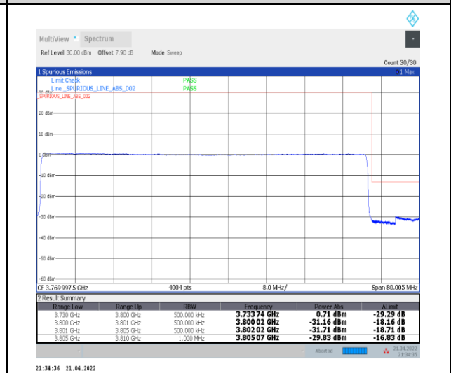
1-N78-3700-3800--30-70-H-6-CP-QPSK-Outer_Full-189@0-Ant0-PASS-see graph
