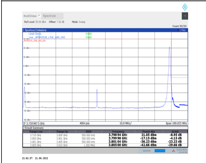
1-N78-3700-3800--30-90-H-5-CP-QPSK-Edge_1RB_Right-1@244-Ant0-PASS-see graph
