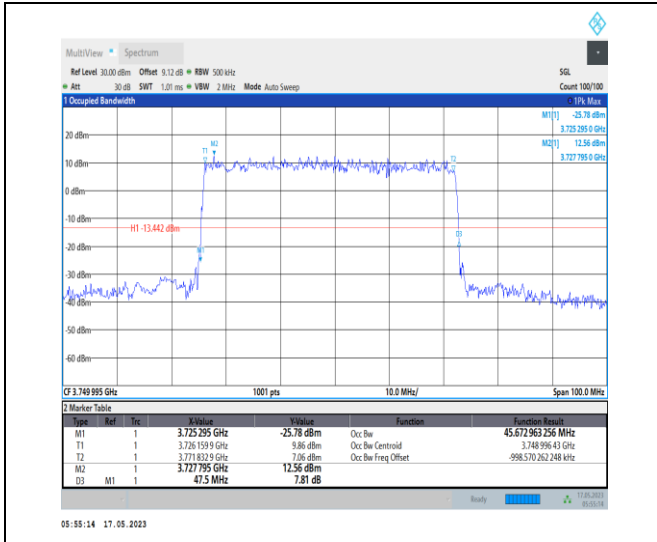
1-N78-3700-3800-PC1-30-50-M-5-DFT-256QAM-Out er_Full-128@0-Ant0-45.673-47.500-≤50-PASS
