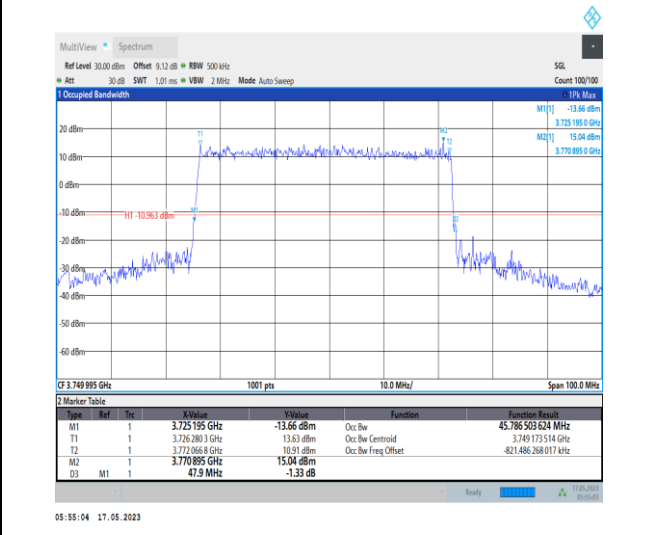
1-N78-3700-3800-PC1-30-50-M-4-DFT-64QAM-Outer_Full-128@0-Ant0-45.787-47.900-≤50-PASS
