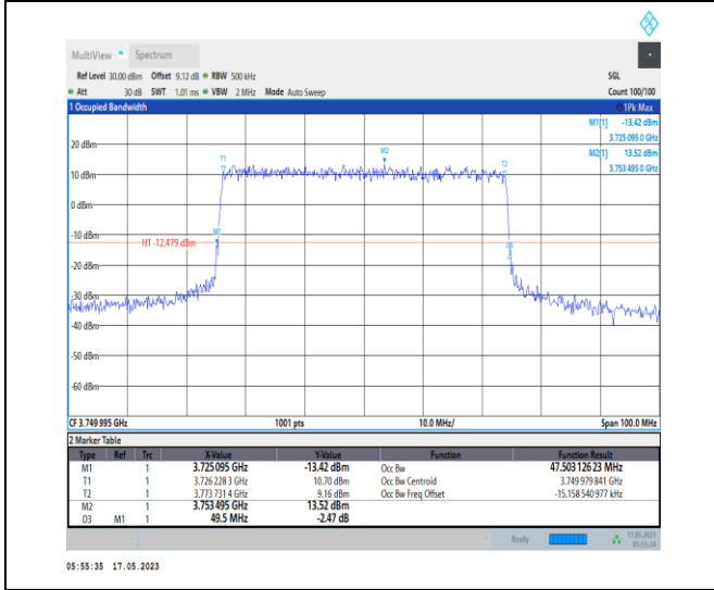
1-N78-3700-3800-PC1-30-50-M-7-CP-16QAM-Outer _Full-133@0-Ant0-47.503-49.500-≤50-PASS
