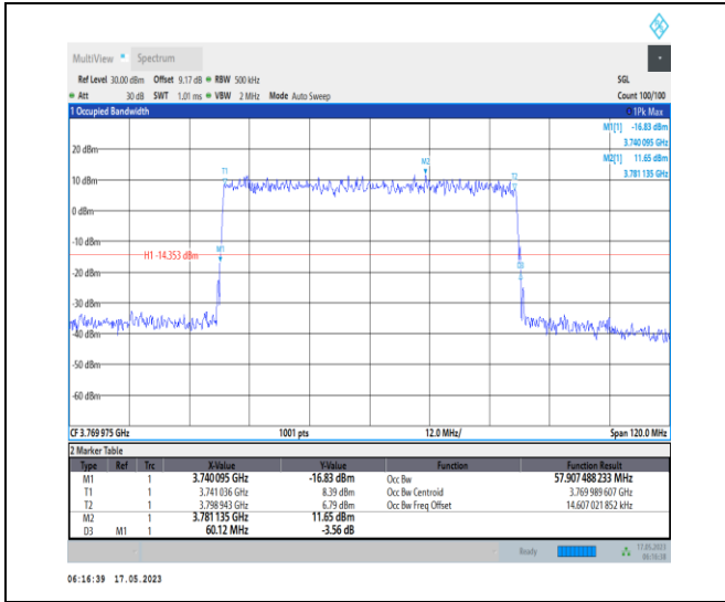
1-N78-3700-3800-PC1-30-60-H-5-DFT-256QAM-Out er_Full-162@0-Ant0-57.907-60.120-≤60-PASS
