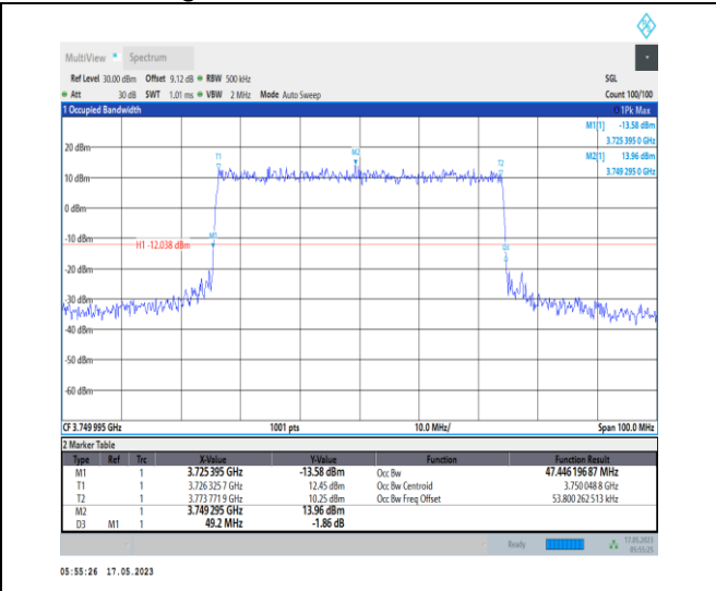
1-N78-3700-3800-PC1-30-50-M-6-CP-QPSK-Outer Full-133@0-Ant0-47.446-49.200-≤50-PASS
