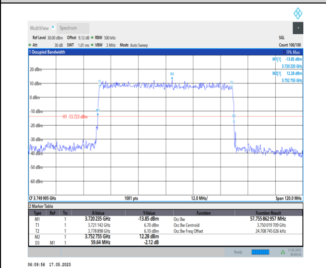
1-N78-3700-3800-PC1-30-60-M-5-DFT-256QAM-Outer_Full-162@0-Ant0-57.756-59.640-≤60-PASS
