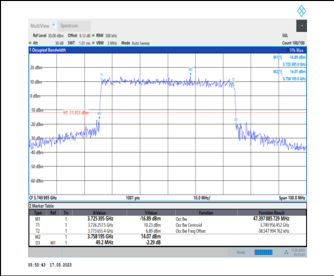
1-N78-3700-3800-PC1-30-50-M-8-CP-64QAM-Outer _Full-133@0-Ant0-47.398-49.200-≤50-PASS
