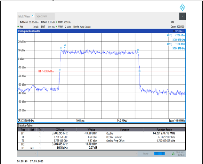
1-N78-3700-3800-PC1-30-70-L-5-DFT-256QAM-Outer_Full-180@0-Ant0-64.281-66.500-≤70-PASS
