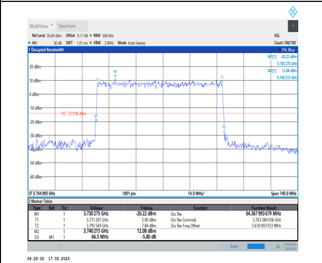
1-N78-3700-3800-PC1-30-70-H-5-DFT-256QAM-Outer_Full-180@0-Ant0-64.368-66.500-≤70-PASS
