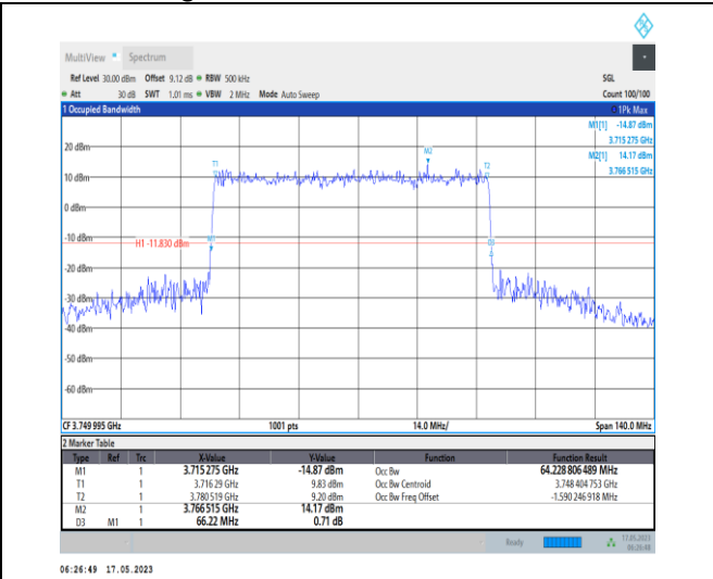
1-N78-3700-3800-PC1-30-70-M-4-DFT-64QAM-Outer_Full-180@0-Ant0-64.229-66.220-≤70-PASS
