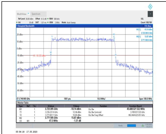
1-N78-3700-3800-PC1-30-50-M-1-DFT-QPSK-Outer_Full-128@0-Ant0-45.6-47.500-≤50-PASS
