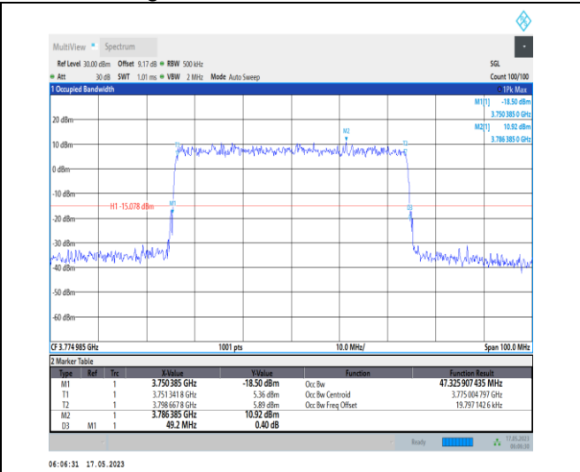
1-N78-3700-3800-PC1-30-50-H-9-CP-256QAM-Outer_Full-133@0-Ant0-47.326-49.200-≤50-PASS
