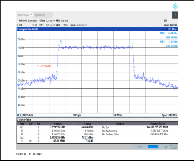
1-N78-3700-3800-PC1-30-70-L-3-DFT-16QAM-Outer_Full-180@0-Ant0-64.188-66.640-≤70-PASS
