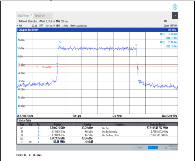
1-N78-3700-3800-PC1-30-60-H-6-CP-QPSK-Outer_Full-162@0-Ant0-57.92-59.880-≤60-PASS
