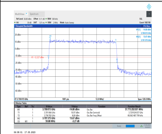
1-N78-3700-3800-PC1-30-60-L-6-CP-QPSK-Outer_Full-162@0-Ant0-57.715-59.880-≤60-PASS
