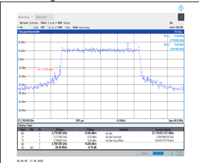
1-N78-3700-3800-PC1-30-30-H-7-CP-16QAM-Outer_Full-78@0-Ant0-27.71-29.340-≤30-PASS
