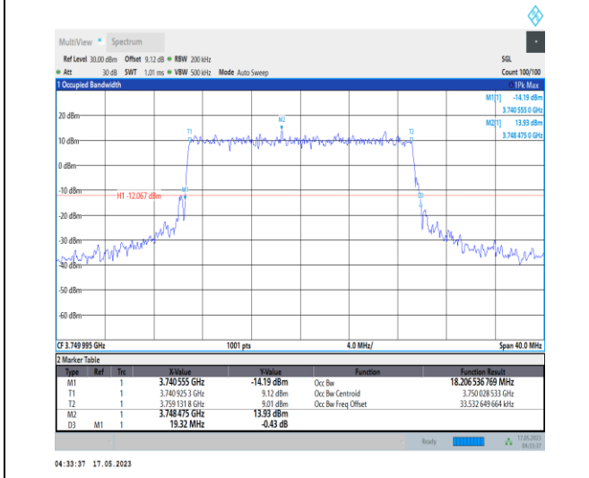
1-N78-3700-3800-PC1-30-20-M-8-CP-64QAM-Outer_Full-51 @ 0-Ant0-18.207-19.320-≤20-PASS
