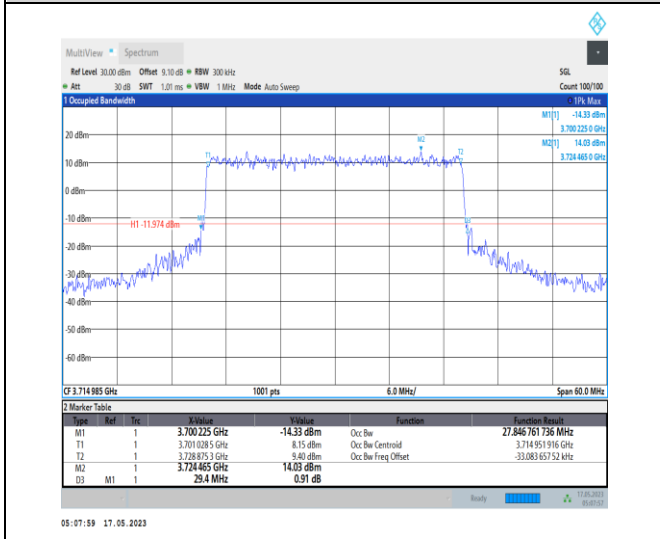
1-N78-3700-3800-PC1-30-30-L-6-CP-QPSK-Outer_Full-78@0-Ant0-27.847-29.400-≤30-PASS
