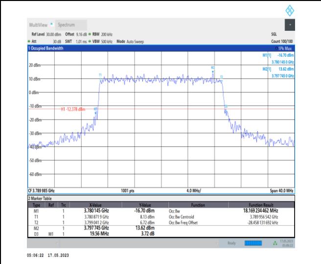
1-N78-3700-3800-PC1-30-20-H-8-CP-64QAM-Outer _Full-51@0-Ant0-18.169-19.560-≤20-PASS
