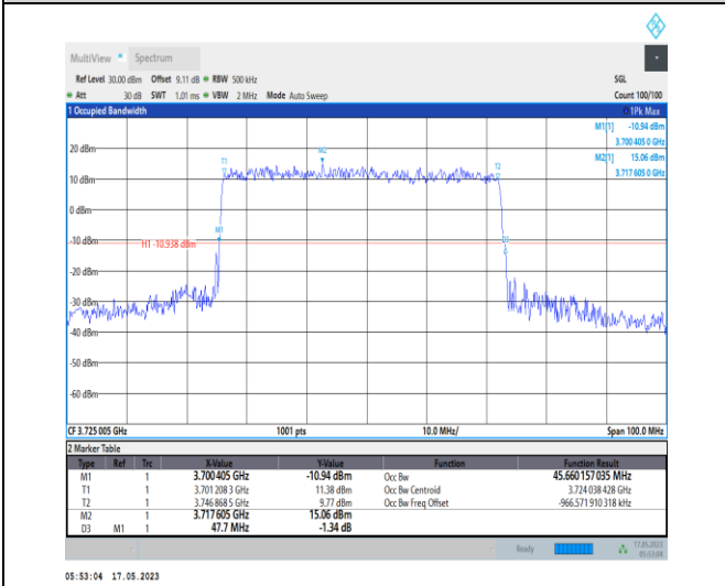
1-N78-3700-3800-PC1-30-50-L-4-DFT-64QAM-Out er_Full-128@0-Ant0-45.66-47.700-≤50-PASS
