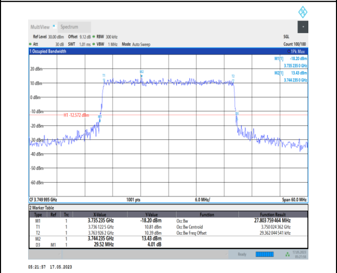
1-N78-3700-3800-PC1-30-30-M-6-CP-QPSK-Outer_Full-78@0-Ant0-27.804-29.520-≤30-PASS
