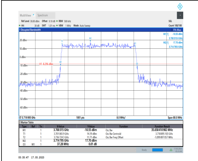
1-N78-3700-3800-PC1-30-40-L-3-DFT-16QAM-Outer_Full-100@0-Ant0-35.658-37.280-≤40-PASS
