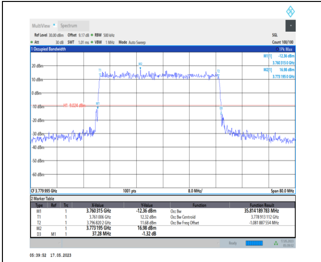
1-N78-3700-3800-PC1-30-40-H-3-DFT-16QAM-Outer_Full-100@0-Ant0-35.814-37.280-≤40-PASS
