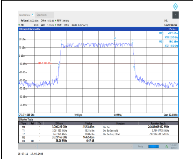
1-N78-3700-3800-PC1-30-30-L-2-DFT-PI2BPSK-Outer_Full-75@0-Ant0-26.688-28.260-≤30-PASS
