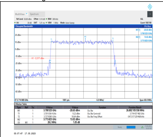
1-N78-3700-3800-PC1-30-30-L-5-DFT-256QAM-Outer_Full-75@0-Ant0-26.802-28.200-≤30-PASS
