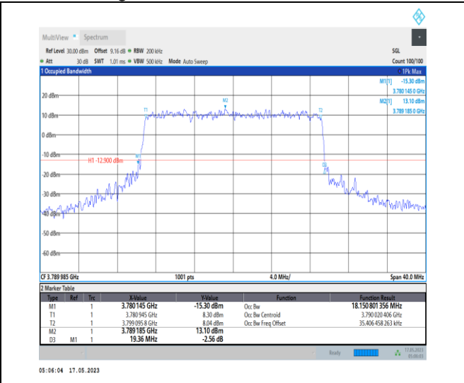
1-N78-3700-3800-PC1-30-20-H-6-CP-QPSK-Outer _Full-51@0-Ant0-18.151-19.360-≤20-PASS
