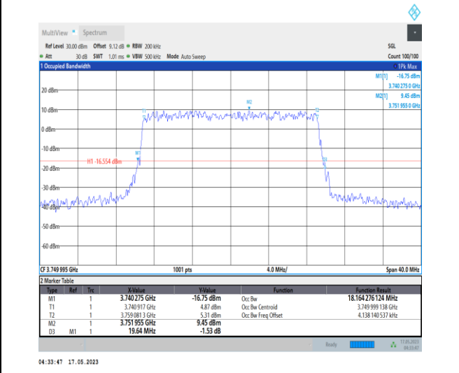
1-N78-3700-3800-PC1-30-20-M-9-CP-256QAM-Outer_Full-51 @ 0-Ant0-18.164-19.640-≤20-PASS
