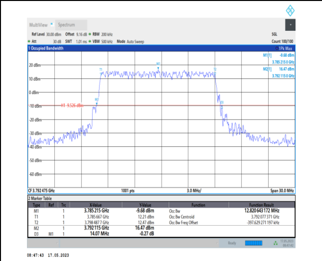
1-N78-3700-3800-PC1-30-15-H-3-DFT-16QAM-Outer_Full-36@0-Ant0-12.821-14.070-≤15-PASS
