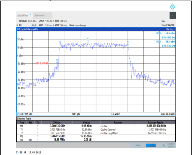
1-N78-3700-3800-PC1-30-15-L-3-DFT-16QAM-Out er_Full-36@0-Ant0-12.838-13.890-≤15-PASS
