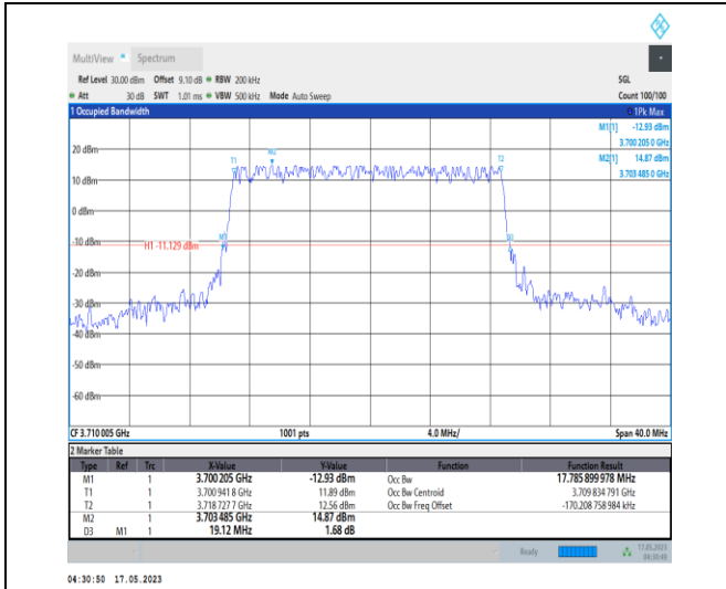
1-N78-3700-3800-PC1-30-20-L-3-DFT-16QAM-Outer_Full-50@0-Ant0-17.786-19.120-≤20-PASS
