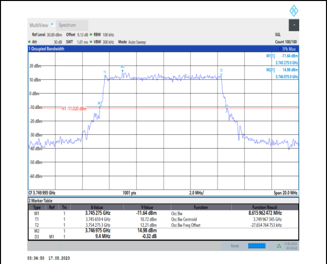
1-N78-3700-3800-PC1-30-10-M-3-DFT-16QAM-Outer_Full-24@0-Ant0-8.616-9.400-≤10-PASS
