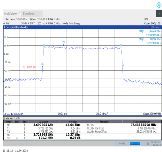
1-N78-3700-3800--30-100-M-9-CP-256QAM-Outer_Full-273@0-Ant0-97.434-101.200-≤100-PASS
