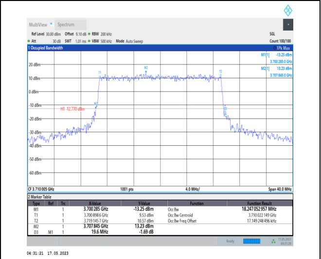
1-N78-3700-3800-PC1-30-20-L-6-CP-QPSK-Outer_Full-51@0-Ant0-18.247-19.600-≤20-PASS
