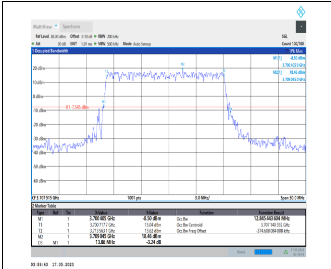
1-N78-3700-3800-PC1-30-15-L-2-DFT-PI2BPSK-Out er_Full-36@0-Ant0-12.845-13.860-≤15-PASS
