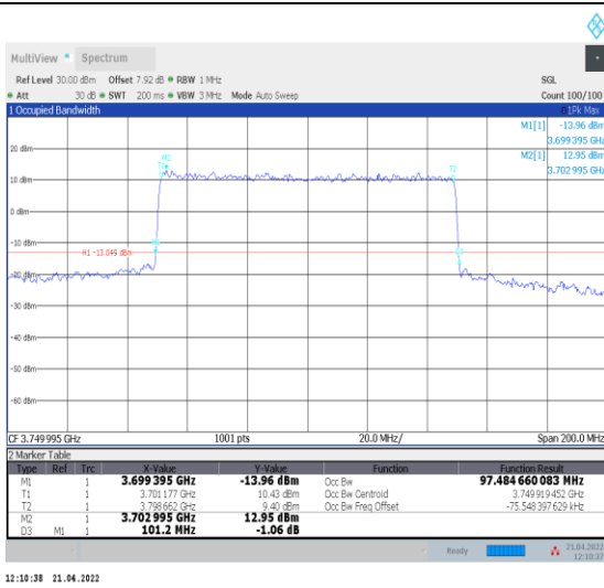
1-N78-3700-3800--30-100-M-6-CP-QPSK-Outer_Full -273@0-Ant0-97.485-101.200-≤100-PASS
