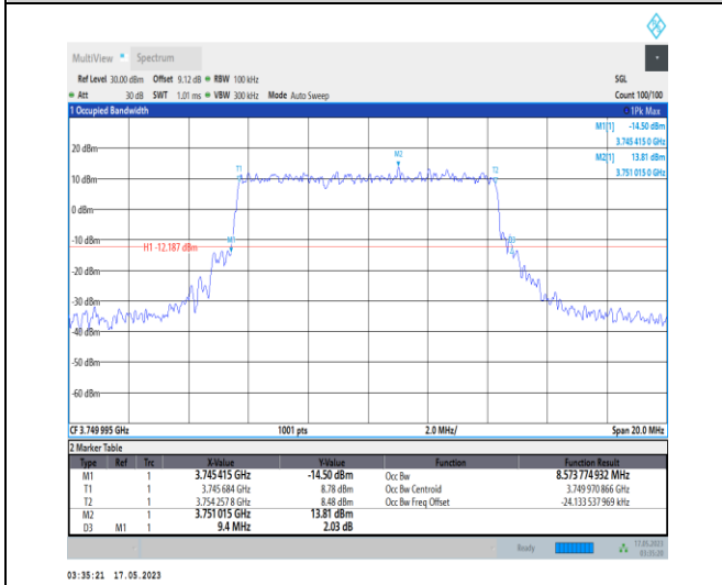
1-N78-3700-3800-PC1-30-10-M-6-CP-QPSK-Outer_Full-24@0-Ant0-8.574-9.400-≤10-PASS
