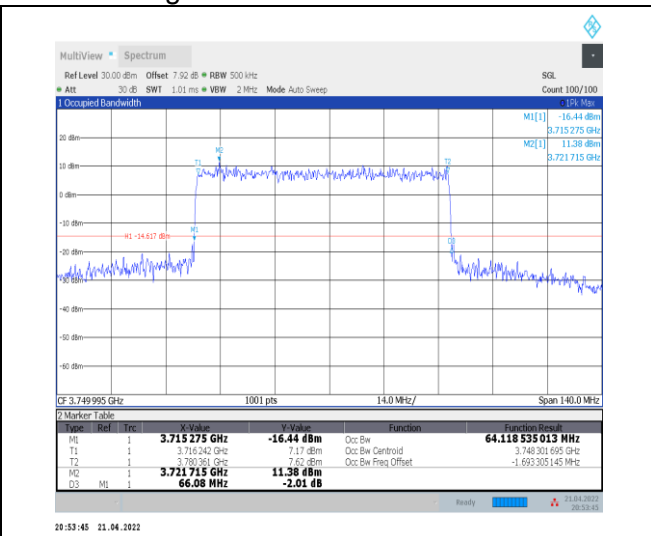
1-N78-3700-3800--30-70-M-4-DFT-64QAM-Outer_Full-180@0-Ant0-64.119-66.080-≤70-PASS
