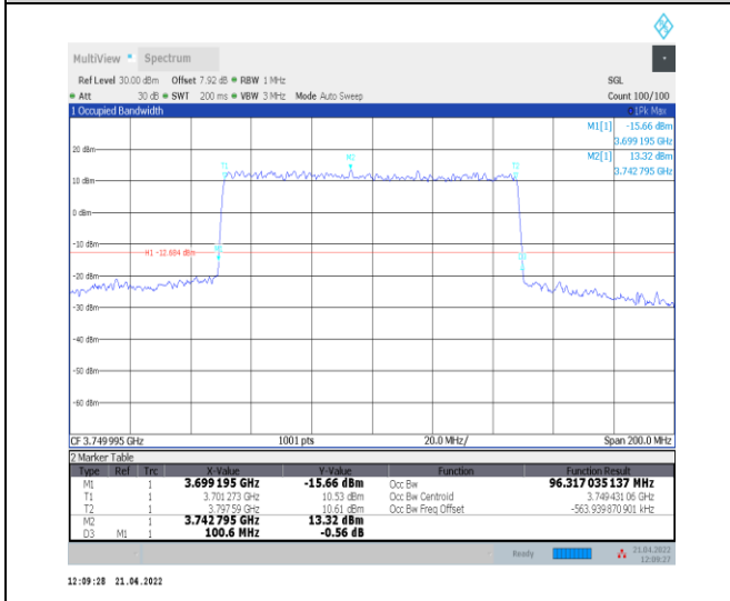
1-N78-3700-3800--30-100-M-4-DFT-64QAM-Outer_Full-270@0-Ant0-96.317-100.600-≤100-PASS
