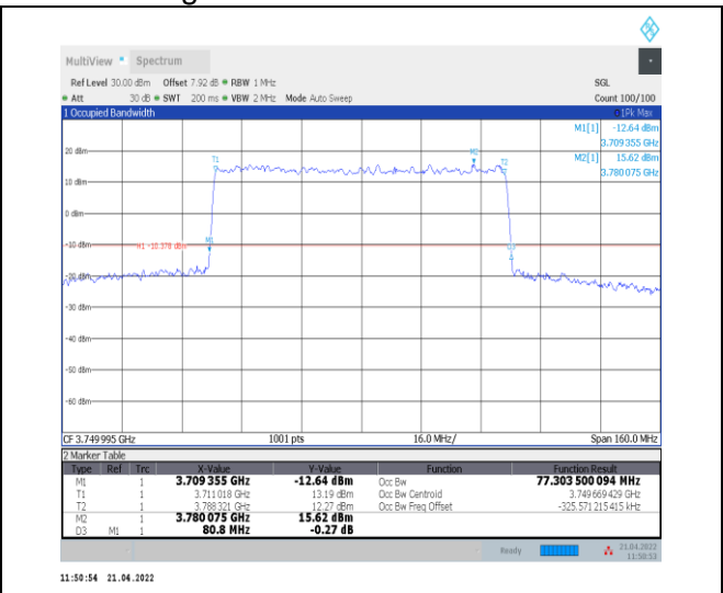
1-N78-3700-3800--30-80-M-1-DFT-QPSK-Outer_Full-216@0-Ant0-77.304-80.800≤80-PASS
