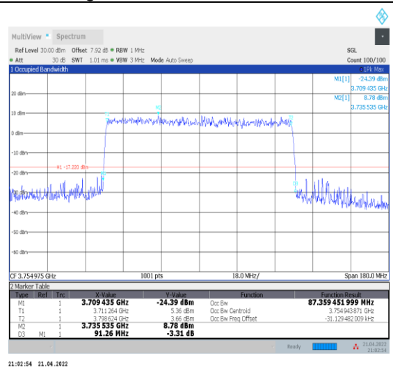
1-N78-3700-3800--30-90-H-9-CP-256QAM-Outer_Full -245@0-Ant0-87.359-91.260-≤90-PASS
