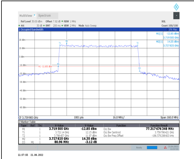
1-N78-3700-3800--30-80-H-3-DFT-16QAM-Outer_Fu II-216@0-Ant0-77.318-80.960-<math>\leq 80</math>-PASS
