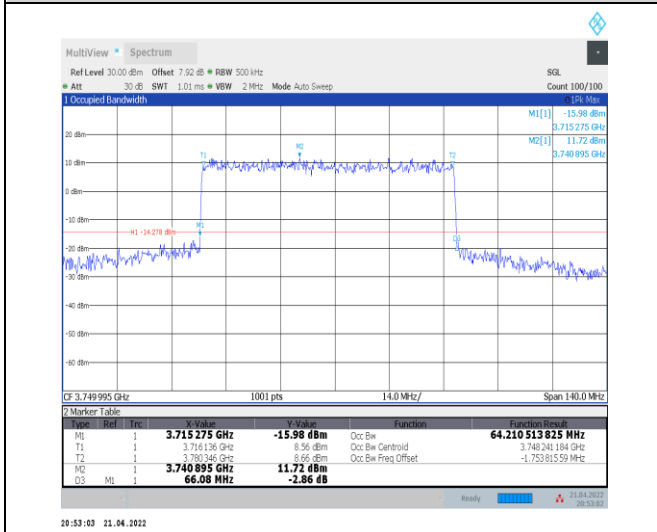
1-N78-3700-3800--30-70-M-1-DFT-QPSK-Outer_Full -180@0-Ant0-64.211-66.080-≤70-PASS
