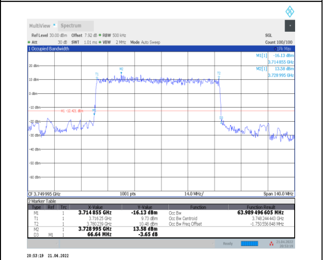
1-N78-3700-3800--30-70-M-2-DFT-PI2BPSK-Outer_Full Full-180@0-Ant0-63.989-66.640-≤70-PASS
