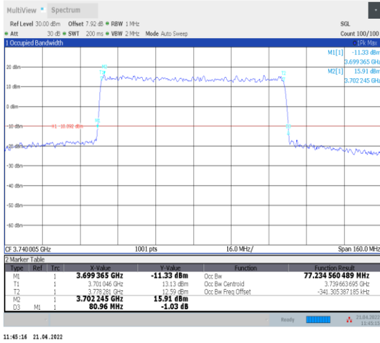
1-N78-3700-3800--30-80-L-1-DFT-QPSK-Outer_Full-216@0-Ant0-77.235-80.960-≤80-PASS
