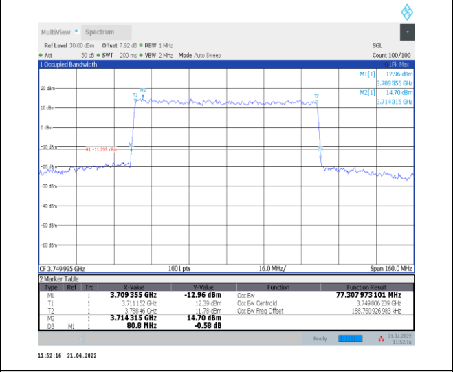
1-N78-3700-3800--30-80-M-3-DFT-16QAM-Outer_Full-216@0-Ant0-77.308-80.800≤80-PASS
