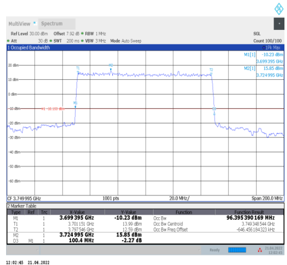
1-N78-3700-3800--30-100-L-2-DFT-PI2BPSK-Outer_Full Full-270@0-Ant0-96.395-100.400-≤100-PASS
