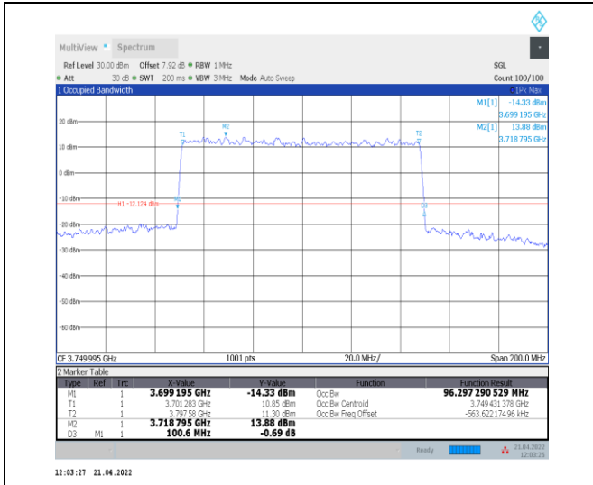
1-N78-3700-3800--30-100-L-3-DFT-16QAM-Outer_F ull-270@0-Ant0-96.297-100.600-≤100-PASS
