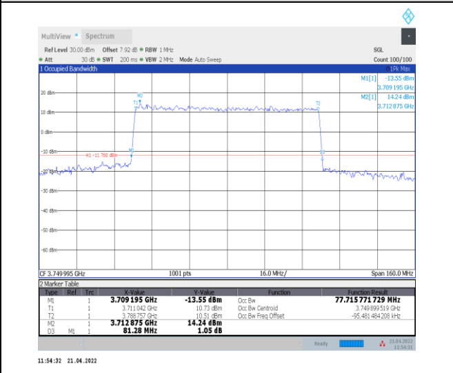
1-N78-3700-3800--30-80-M-7-CP-16QAM-Outer_Full-217@0-Ant0-77.716-81.280-<math>\leq</math>80-PASS
