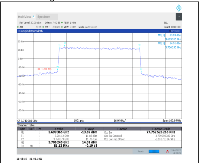
1-N78-3700-3800--30-80-L-6-CP-QPSK-Outer_Full-217@0-Ant0-77.753-81.120-≤80-PASS
