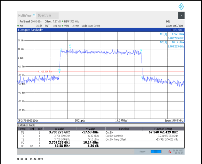
1-N78-3700-3800--30-70-L-7-CP-16QAM-Outer_Full-I-189@0-Ant0-67.341-69.580-≤70-PASS
