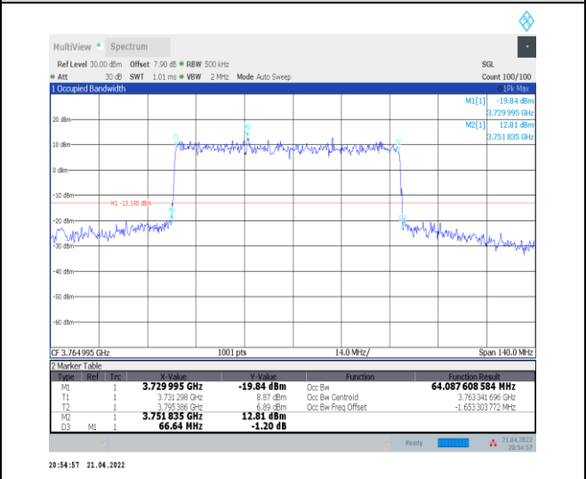
1-N78-3700-3800--30-70-H-1-DFT-QPSK-Outer_Full -180@0-Ant0-64.088-66.640-≤70-PASS
