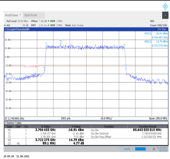
1-N78-3700-3800--30-90-M-2-DFT-PI2BPSK-Outer_Full -240@0-Ant0-85.644-89.100-≤90-PASS
