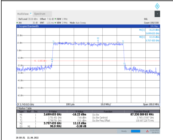
1-N78-3700-3800--30-90-L-8-CP-64QAM-Outer_Full-245@0-Ant0-87.331-90.900-<math>\leq 90</math>-PASS
