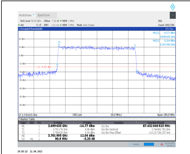
1-N78-3700-3800--30-90-L-6-CP-QPSK-Outer_Full-245@0-Ant0-87.452-90.900-<math>\leq 90</math>-PASS
