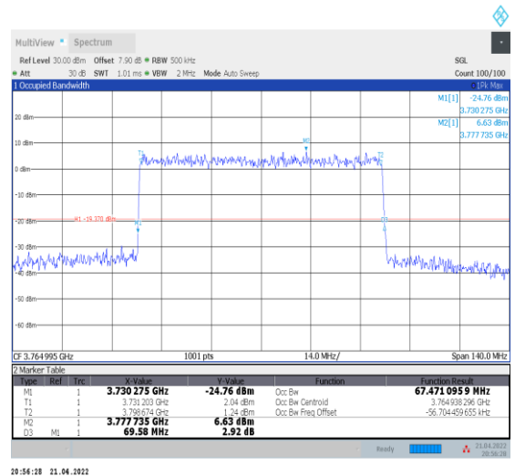
1-N78-3700-3800--30-70-H-9-CP-256QAM-Outer_Full-189@0-Ant0-67.471-69.580-≤70-PASS
