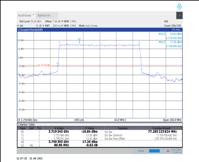
1-N78-3700-3800--30-80-H-2-DFT-PI2BPSK-Outer_Full-216@0-Ant0-77.285-80.960-<math>\leq 80</math>-PASS
