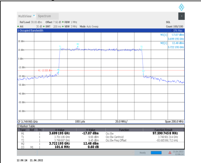
1-N78-3700-3800--30-100-L-8-CP-64QAM-Outer_Fu II-273@0-Ant0-97.591-101.600-≤100-PASS
