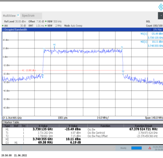
1-N78-3700-3800--30-70-H-6-CP-QPSK-Outer_Full-189@0-Ant0-67.379-69.580-≤70-PASS
