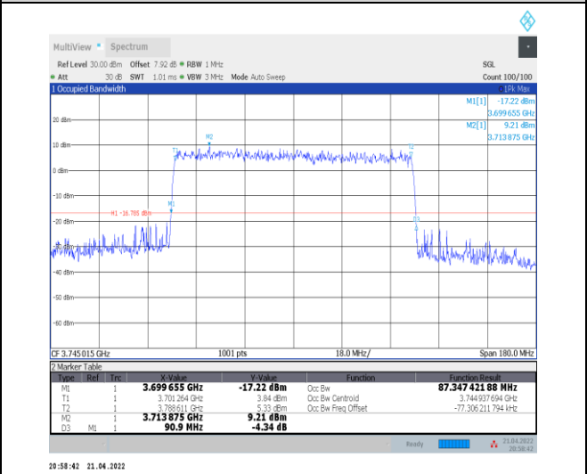
1-N78-3700-3800--30-90-L-9-CP-256QAM-Outer_Full-245@0-Ant0-87.347-90.900-<math>\leq 90</math>-PASS
