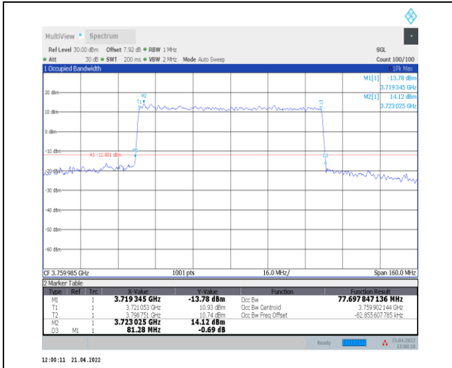
1-N78-3700-3800--30-80-H-7-CP-16QAM-Outer_Full -217@0-Ant0-77.698-81.280-<math>\leq 80</math>-PASS
