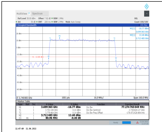
1-N78-3700-3800--30-80-L-5-DFT-256QAM-Outer_Full-216@0-Ant0-77.275-80.960-≤80-PASS
