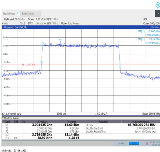
1-N78-3700-3800--30-90-M-3-DFT-16QAM-Outer_Full -240@0-Ant0-85.768-88.920-≤90-PASS
