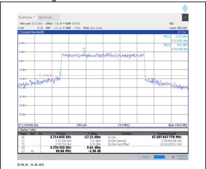
1-N78-3700-3800--30-70-M-8-CP-64QAM-Outer_Ful I-189@0-Ant0-67.508-69.860-≤70-PASS
