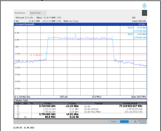
1-N78-3700-3800--30-80-H-4-DFT-64QAM-Outer_Fu II-216@0-Ant0-77.22-80.800-<math>\leq 80</math>-PASS
