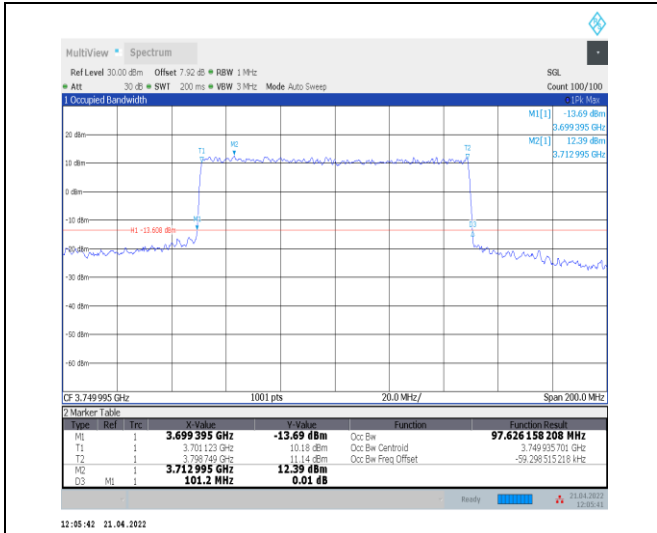
1-N78-3700-3800--30-100-L-7-CP-16QAM-Outer_Fu II-273@0-Ant0-97.626-101.200-≤100-PASS
