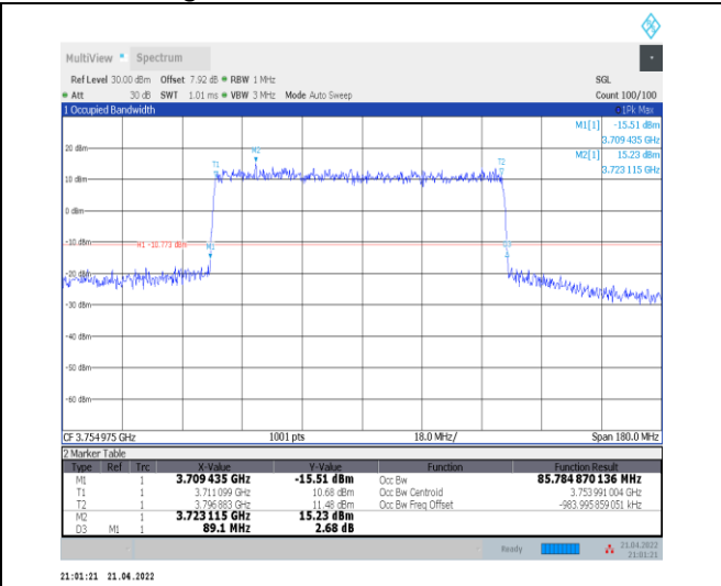
1-N78-3700-3800--30-90-H-1-DFT-QPSK-Outer_Full-240@0-Ant0-85.785-89.100-≤90-PASS
