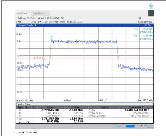
1-N78-3700-3800--30-90-H-4-DFT-64QAM-Outer_Fu II-240@0-Ant0-85.781-88.920-<=90-PASS
