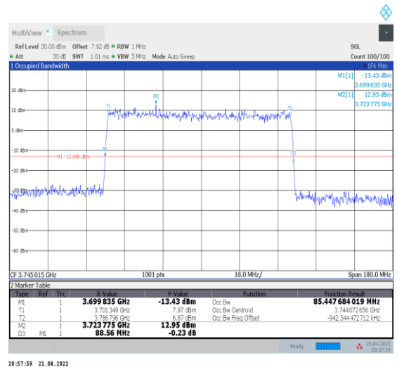
1-N78-3700-3800--30-90-L-5-DFT-256QAM-Outer_F ull-240@0-Ant0-85.448-88.560-<math>\leq 90</math>-PASS
