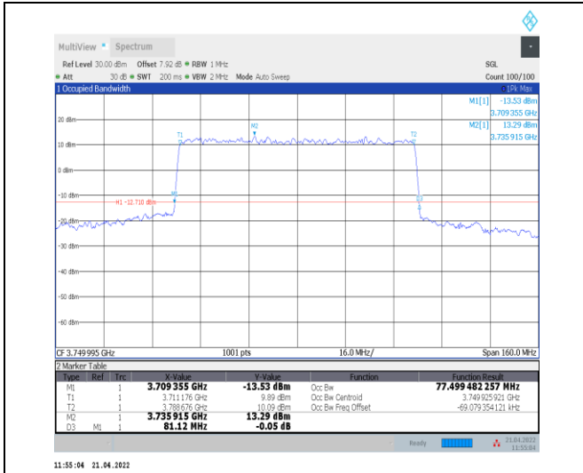
1-N78-3700-3800--30-80-M-8-CP-64QAM-Outer_Full -217@0-Ant0-77.499-81.120-<math>\leq 80</math>-PASS
