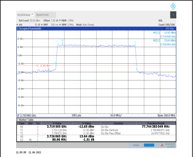
1-N78-3700-3800--30-80-H-6-CP-QPSK-Outer_Full-217@0-Ant0-77.744-80.960-<math>\leq 80</math>-PASS
