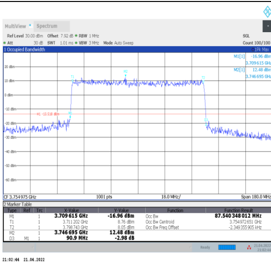
1-N78-3700-3800--30-90-H-8-CP-64QAM-Outer_Full -245@0-Ant0-87.54-90.900-≤90-PASS
