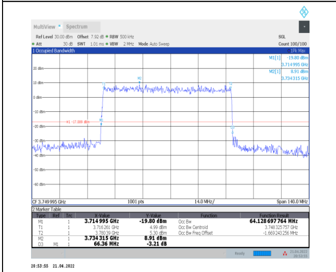
1-N78-3700-3800--30-70-M-5-DFT-256QAM-Outer_Full-180@0-Ant0-64.129-66.360-≤70-PASS
