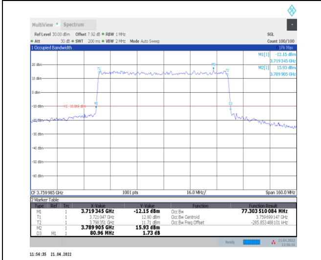
1-N78-3700-3800--30-80-H-1-DFT-QPSK-Outer_Full -216@0-Ant0-77.304-80.960-<math>\leq 80</math>-PASS
