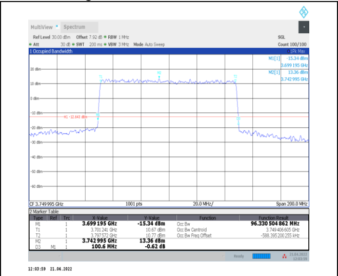
1-N78-3700-3800--30-100-L-4-DFT-64QAM-Outer_F ull-270@0-Ant0-96.331-100.600-≤100-PASS
