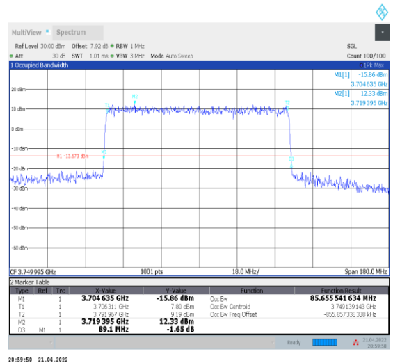
1-N78-3700-3800--30-90-M-4-DFT-64QAM-Outer_Full -240@0-Ant0-85.656-89.100-≤90-PASS
