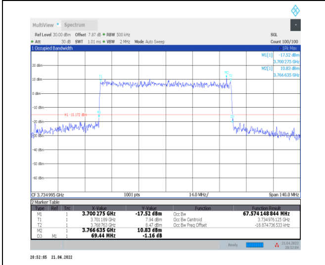
1-N78-3700-3800--30-70-L-6-CP-QPSK-Outer_Full-I-89@0-Ant0-67.574-69.440-≤70-PASS
