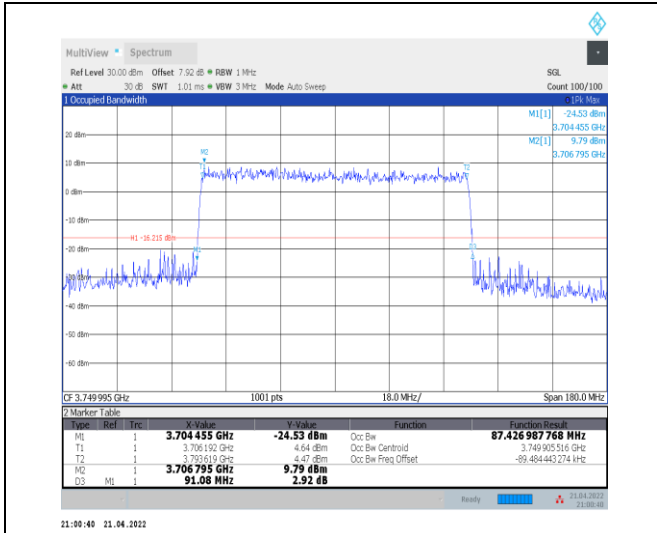
1-N78-3700-3800--30-90-M-9-CP-256QAM-Outer_Full-245@0-Ant0-87.427-91.080-≤90-PASS
