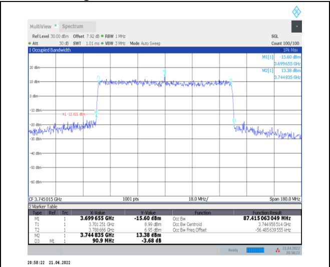
1-N78-3700-3800--30-90-L-7-CP-16QAM-Outer_Full-245@0-Ant0-87.415-90.900-<math>\leq 90</math>-PASS
