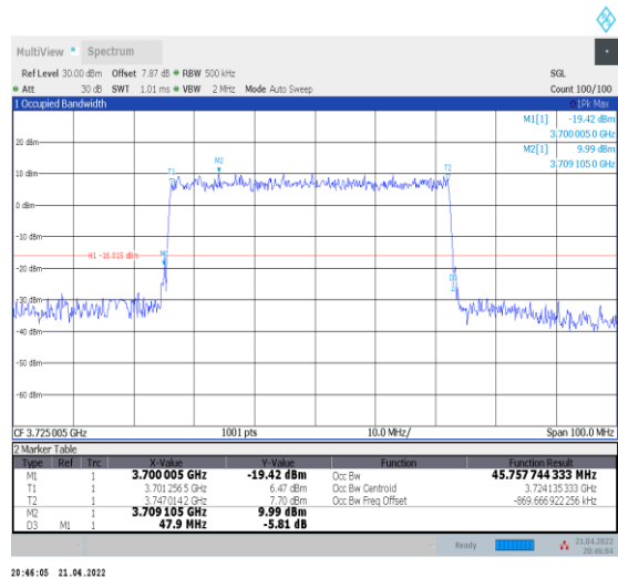
1-N78-3700-3800--30-50-L-5-DFT-256QAM-Outer_F ull-128@0-Ant0-45.758-47.900-≤50-PASS
