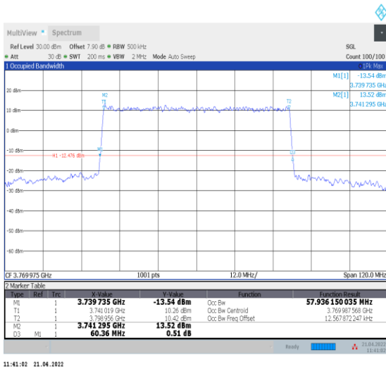
1-N78-3700-3800--30-60-H-3-DFT-16QAM-Outer_Fu ll-162@0-Ant0-57.936-60.360-≤60-PASS
