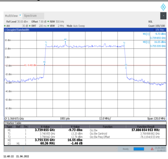
1-N78-3700-3800--30-60-H-2-DFT-PI2BPSK-Outer_Full Full-162@0-Ant0-57.887-60.360-≤60-PASS
