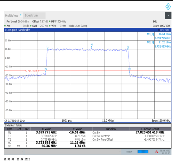
1-N78-3700-3800--30-60-L-8-CP-64QAM-Outer_Full -162@0-Ant0-57.82-60.360-≤60-PASS
