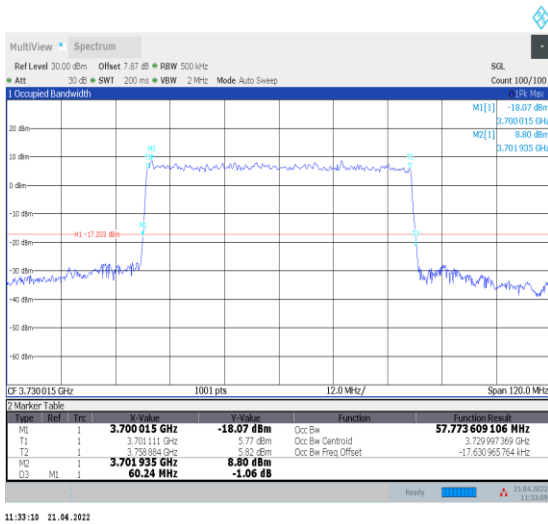
1-N78-3700-3800--30-60-L-9-CP-256QAM-Outer_Fu II-162@0-Ant0-57.774-60.240-≤60-PASS
