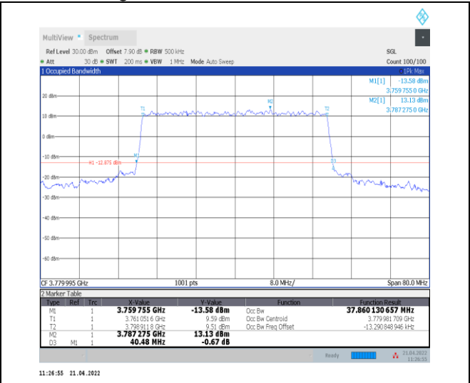
1-N78-3700-3800--30-40-H-8-CP-64QAM-Outer_Full -106@0-Ant0-37.86-40.480-≤40-PASS
