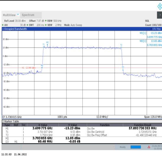
1-N78-3700-3800--30-60-L-7-CP-16QAM-Outer_Full -162@0-Ant0-57.894-60.480-≤60-PASS
