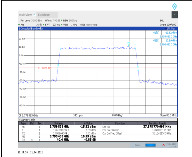
1-N78-3700-3800--30-40-H-9-CP-256QAM-Outer_Fu ll-106@0-Ant0-37.879-40.400-≤40-PASS
