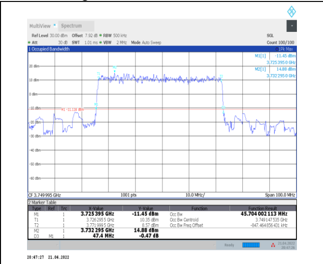
1-N78-3700-3800--30-50-M-2-DFT-PI2BPSK-Outer_Full Full-128@0-Ant0-45.704-47.400-≤50-PASS
