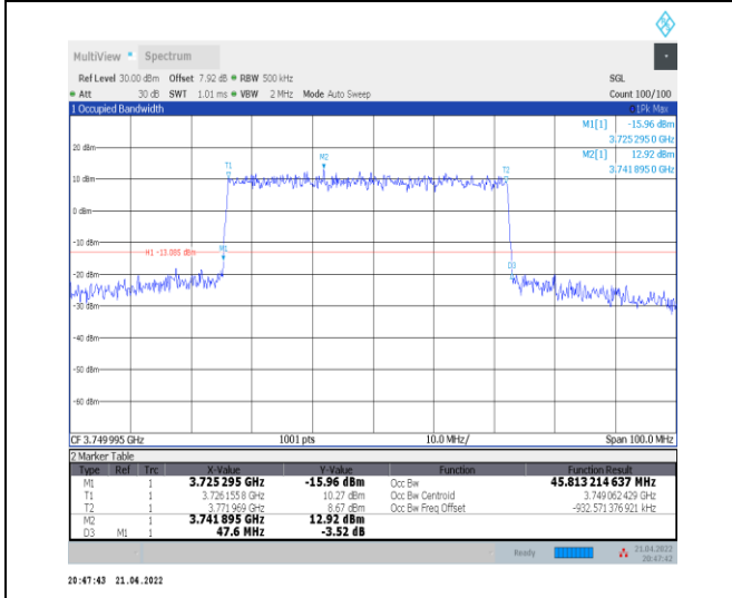
1-N78-3700-3800--30-50-M-3-DFT-16QAM-Outer_Full ull-128@0-Ant0-45.813-47.600-≤50-PASS
