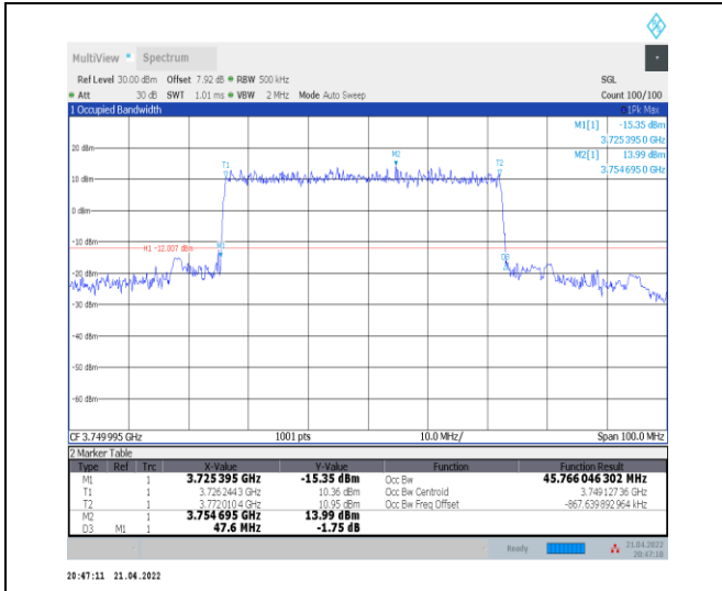
1-N78-3700-3800--30-50-M-1-DFT-QPSK-Outer_Full -128@0-Ant0-45.766-47.600-≤50-PASS
