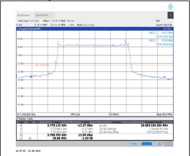
1-N78-3700-3800--30-30-H-3-DFT-16QAM-Outer_Fu II-75@0-Ant0-26.865-28.860-≤30-PASS
