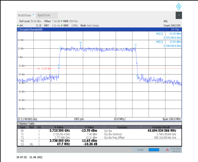
1-N78-3700-3800--30-50-M-4-DFT-64QAM-Outer_Full ull-128@0-Ant0-45.695-47.700-≤50-PASS
