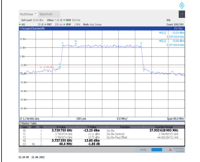
1-N78-3700-3800--30-40-M-6-CP-QPSK-Outer_Full-106@0-Ant0-37.954-40.400-≤40-PASS
