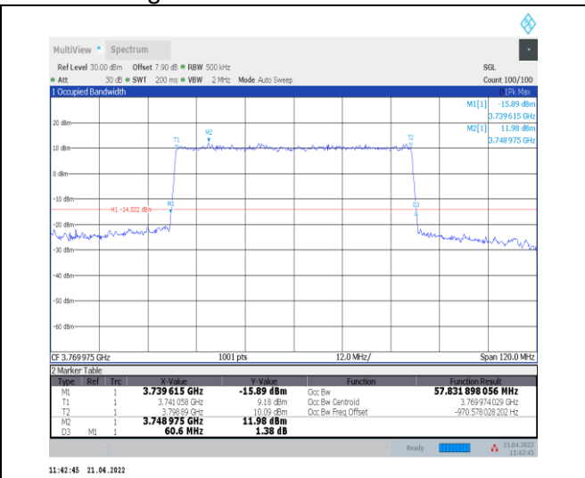
1-N78-3700-3800--30-60-H-6-CP-QPSK-Outer_Full-162@0-Ant0-57.832-60.600-≤60-PASS
