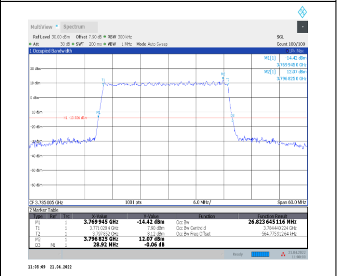
1-N78-3700-3800--30-30-H-5-DFT-256QAM-Outer_Full-75@0-Ant0-26.824-28.920-≤30-PASS
