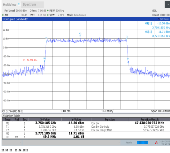
1-N78-3700-3800--30-50-H-8-CP-64QAM-Outer_Full -133@0-Ant0-47.438-49.400-≤50-PASS
