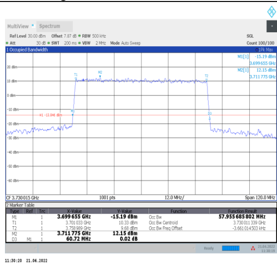
1-N78-3700-3800--30-60-L-4-DFT-64QAM-Outer_Fu II-162@0-Ant0-57.956-60.720-≤60-PASS
