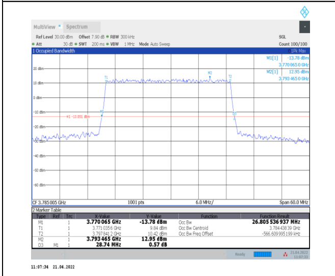
1-N78-3700-3800--30-30-H-4-DFT-64QAM-Outer_Fu II-75@0-Ant0-26.806-28.740-≤30-PASS
