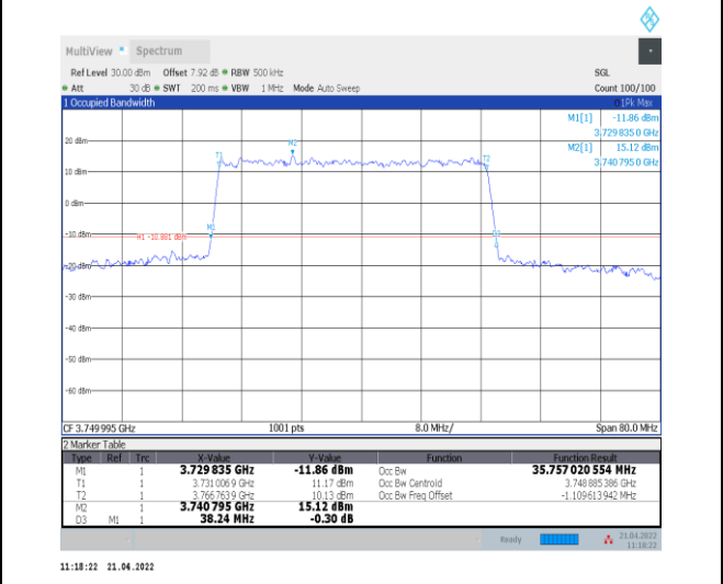
1-N78-3700-3800--30-40-M-3-DFT-16QAM-Outer_Full-100@0-Ant0-35.757-38.240-≤40-PASS
