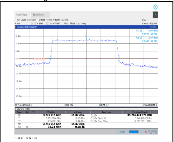
1-N78-3700-3800--30-40-M-1-DFT-QPSK-Outer_Full -100@0-Ant0-35.766-38.240-≤40-PASS
