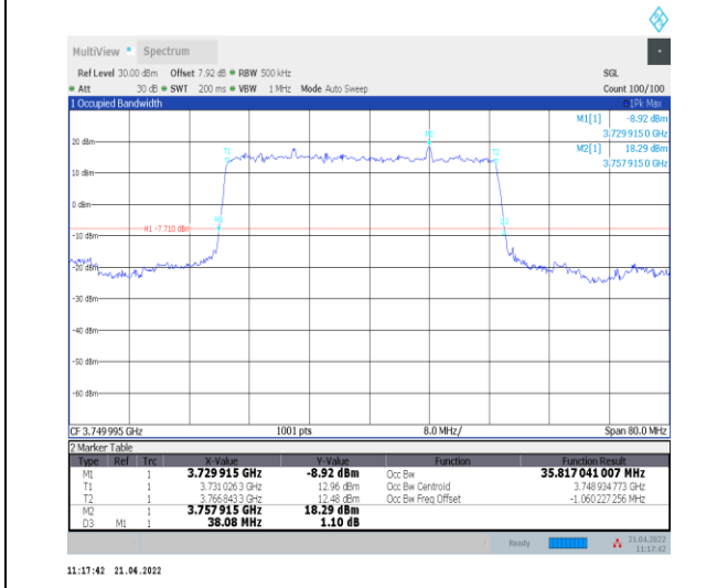
1-N78-3700-3800--30-40-M-2-DFT-PI2BPSK-Outer_Full-100@0-Ant0-35.817-38.080-≤40-PASS
