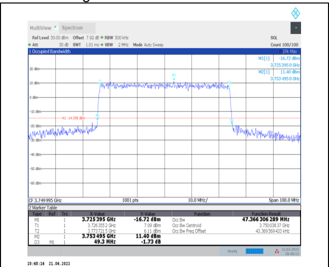
1-N78-3700-3800--30-50-M-6-CP-QPSK-Outer_Full-133@0-Ant0-47.366-49.300-<math>\leq 50</math>-PASS
