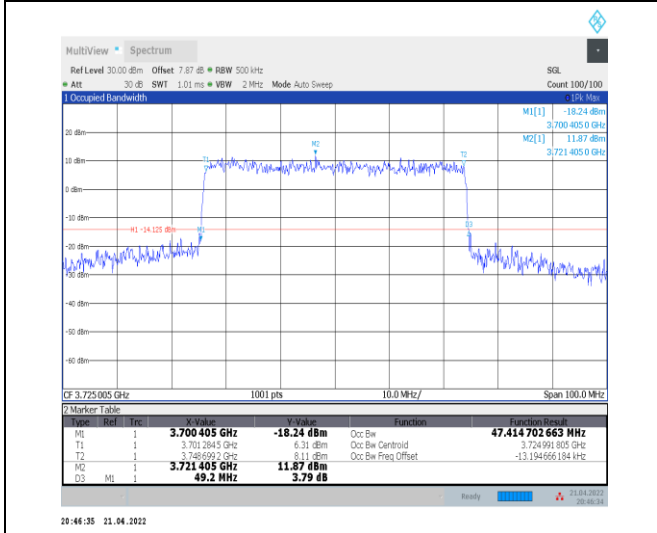
1-N78-3700-3800--30-50-L-8-CP-64QAM-Outer_Full -133@0-Ant0-47.415-49.200≤50-PASS
