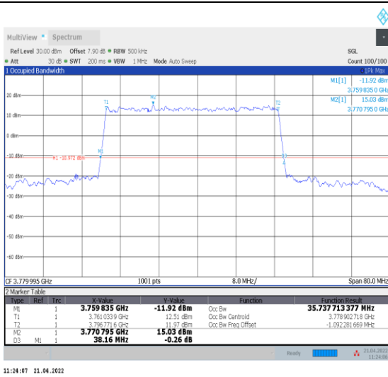
1-N78-3700-3800--30-40-H-3-DFT-16QAM-Outer_Fu II-100@0-Ant0-35.738-38.160-≤40-PASS
