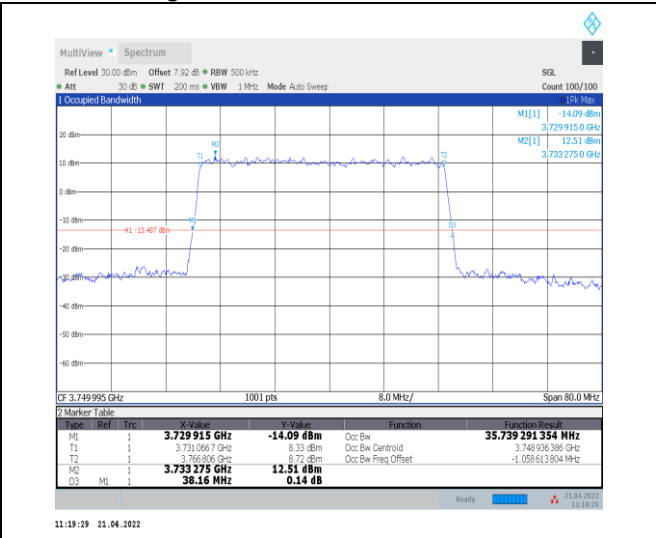
1-N78-3700-3800--30-40-M-5-DFT-256QAM-Outer_Full-100@0-Ant0-35.739-38.160-≤40-PASS
