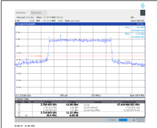
1-N78-3700-3800--30-50-L-6-CP-QPSK-Outer_Full-1 33@0-Ant0-47.445-49.400≤50-PASS
