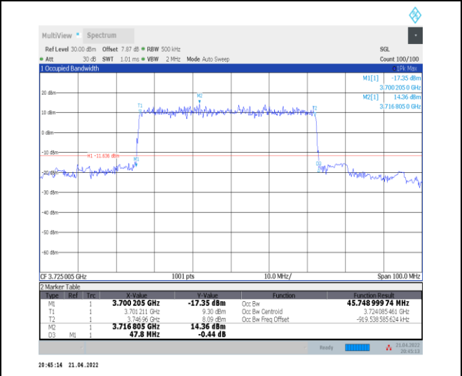
1-N78-3700-3800--30-50-L-1-DFT-QPSK-Outer_Full- 128@0-Ant0-45.749-47.800-≤50-PASS
