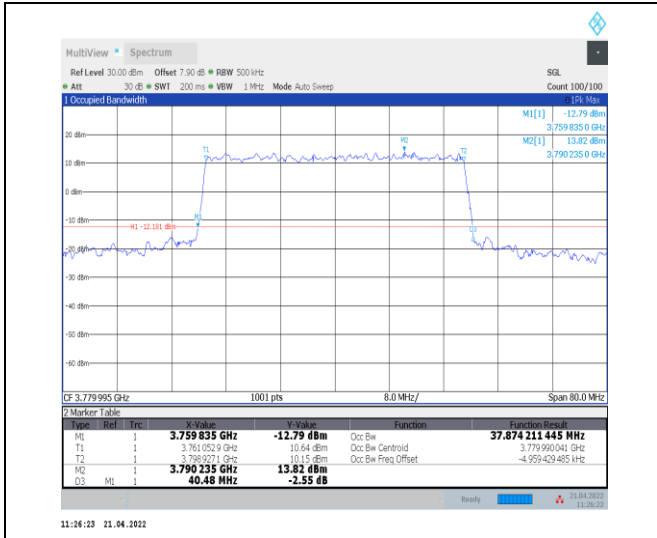
1-N78-3700-3800--30-40-H-7-CP-16QAM-Outer_Full -106@0-Ant0-37.874-40.480-≤40-PASS
