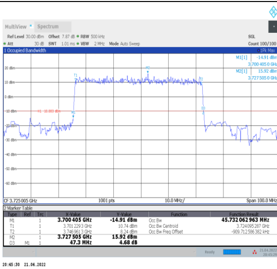
1-N78-3700-3800--30-50-L-2-DFT-PI2BPSK-Outer_F ull-128@0-Ant0-45.732-47.300-≤50-PASS
