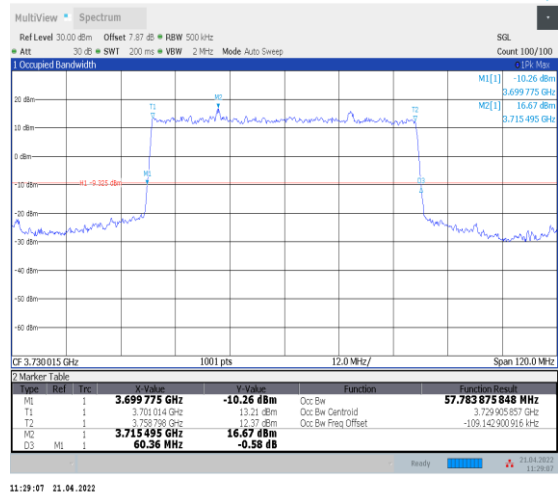
1-N78-3700-3800--30-60-L-2-DFT-PI2BPSK-Outer_Full-162@0-Ant0-57.784-60.360-≤60-PASS
