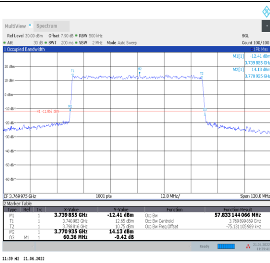
1-N78-3700-3800--30-60-H-1-DFT-QPSK-Outer_Full -162@0-Ant0-57.833-60.360-≤60-PASS
