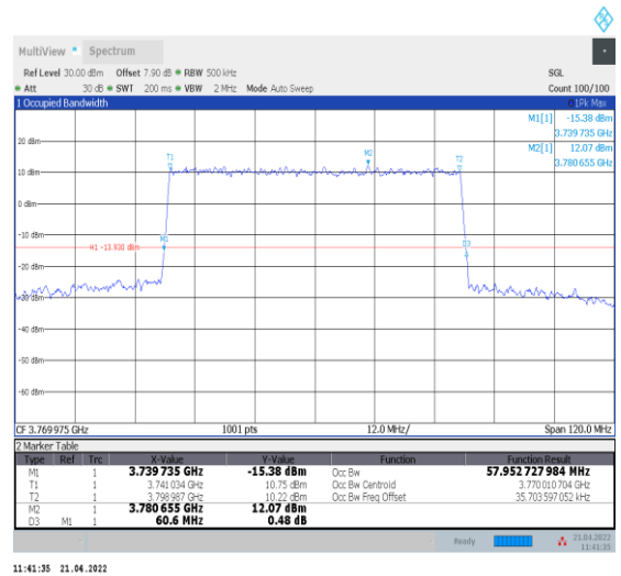
1-N78-3700-3800--30-60-H-4-DFT-64QAM-Outer_Fu ll-162@0-Ant0-57.953-60.600-≤60-PASS
