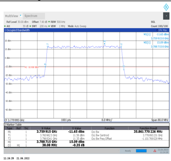
1-N78-3700-3800--30-40-H-4-DFT-64QAM-Outer_Fu II-100@0-Ant0-35.862-38.080-≤40-PASS
