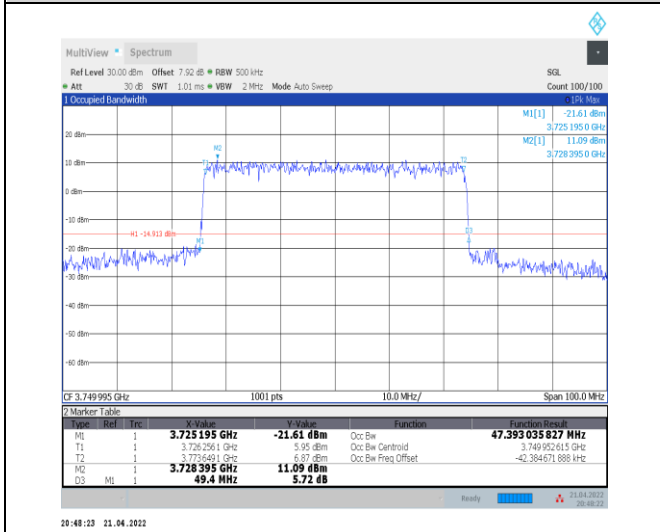
1-N78-3700-3800--30-50-M-7-CP-16QAM-Outer_Full-133@0-Ant0-47.393-49.400-<math>\leq 50</math>-PASS
