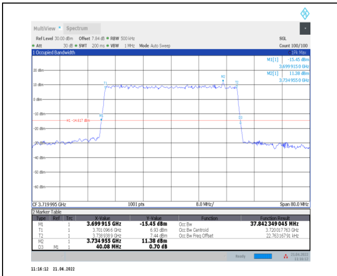
1-N78-3700-3800--30-40-L-9-CP-256QAM-Outer_Fu II-106@0-Ant0-37.842-40.080-≤40-PASS
