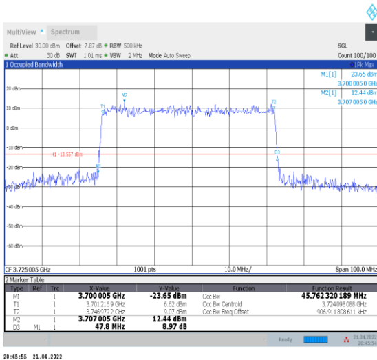
1-N78-3700-3800--30-50-L-4-DFT-64QAM-Outer_Ful l-128@0-Ant0-45.762-47.800-≤50-PASS
