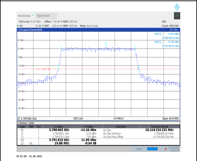
1-N78-3700-3800--30-20-H-8-CP-64QAM-Outer_Full-51@0-Ant0-18.218-19.880-≤20-PASS
