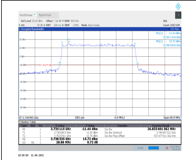
1-N78-3700-3800--30-30-M-1-DFT-QPSK-Outer_Full -75@0-Ant0-26.834-28.860-<30-PASS
