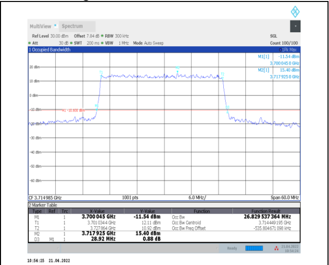
1-N78-3700-3800--30-30-L-1-DFT-QPSK-Outer_Full-75@0-Ant0-26.83-28.920-≤30-PASS
