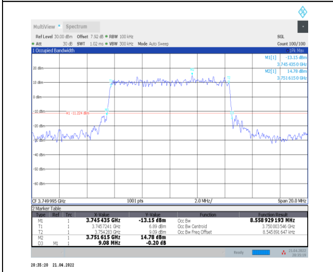
1-N78-3700-3800--30-10-M-2-DFT-PI2BPSK-Outer_Full-24@0-Ant0-8.559-9.080-≤10-PASS
