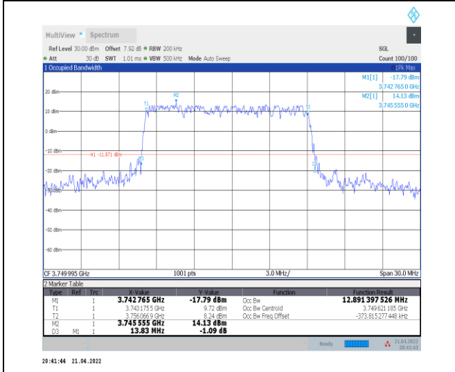
1-N78-3700-3800--30-15-M-3-DFT-16QAM-Outer_Full ull-36@0-Ant0-12.891-13.830-≤15-PASS
