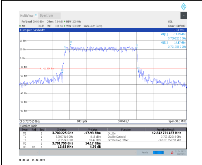
1-N78-3700-3800--30-15-L-4-DFT-64QAM-Outer_Full-36@0-Ant0-12.843-13.650-≤15-PASS
