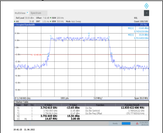
1-N78-3700-3800--30-15-M-2-DFT-PI2BPSK-Outer_Full Full-36@0-Ant0-12.935-14.070-≤15-PASS
