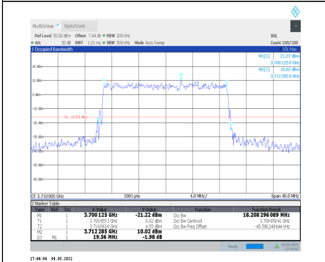
1-N78-3700-3800--30-20-L-9-CP-256QAM-Outer_Fu II-51@0-Ant0-18.208-19.560-<=20-PASS
