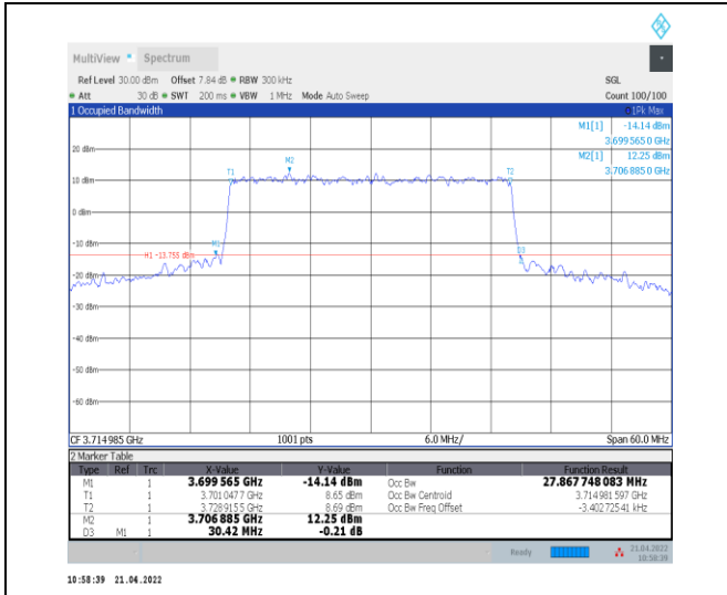
1-N78-3700-3800--30-30-L-8-CP-64QAM-Outer_Full -78@0-Ant0-27.868-30.420-<30-PASS
