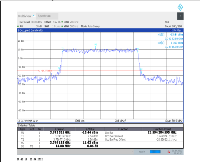
1-N78-3700-3800--30-15-M-6-CP-QPSK-Outer_Full-38@0-Ant0-13.594-14.880-≤15-PASS
