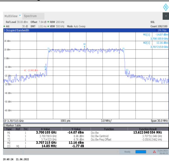
1-N78-3700-3800--30-15-L-7-CP-16QAM-Outer_Full -38@0-Ant0-13.622-14.850-≤15-PASS
