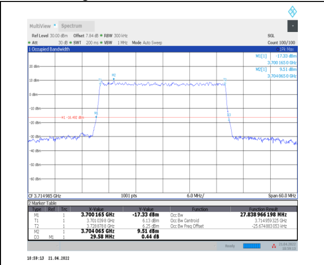
1-N78-3700-3800--30-30-L-9-CP-256QAM-Outer_Fu II-78@0-Ant0-27.839-29.580-<30-PASS
