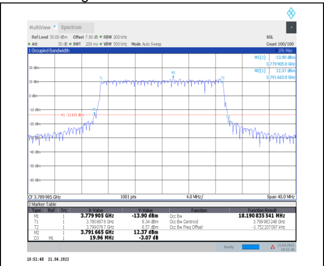
1-N78-3700-3800--30-20-H-6-CP-QPSK-Outer_Full-51@0-Ant0-18.191-19.960-≤20-PASS
