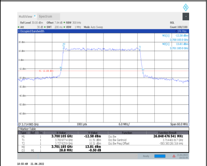
1-N78-3700-3800--30-30-L-3-DFT-16QAM-Outer_Full-75@0-Ant0-26.848-28.800-≤30-PASS
