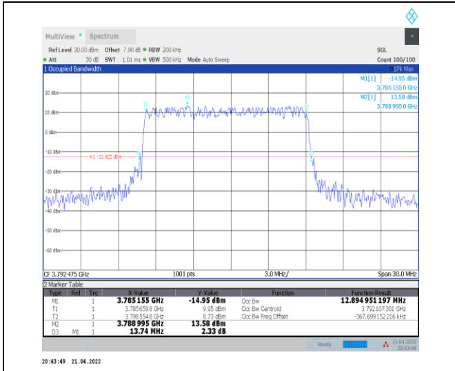
1-N78-3700-3800--30-15-H-4-DFT-64QAM-Outer_Fu II-36@0-Ant0-12.895-13.740-≤15-PASS
