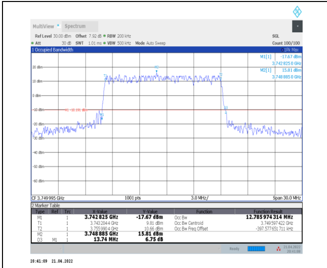
1-N78-3700-3800--30-15-M-1-DFT-QPSK-Outer_Full -36@0-Ant0-12.786-13.740-≤15-PASS
