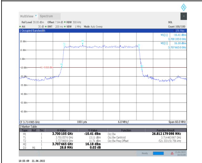
1-N78-3700-3800--30-30-L-2-DFT-PI2BPSK-Outer_Full-75@0-Ant0-26.812-28.800-≤30-PASS
