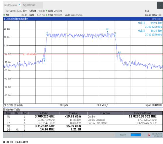
1-N78-3700-3800--30-15-L-1-DFT-QPSK-Outer_Full- 36@0-Ant0-12.828-14.160≤15-PASS
