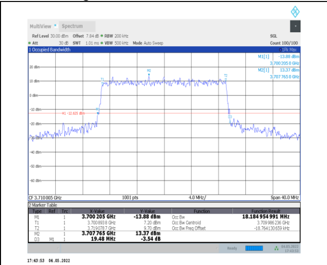
1-N78-3700-3800--30-20-L-8-CP-64QAM-Outer_Full -51@0-Ant0-18.185-19.480-<=20-PASS
