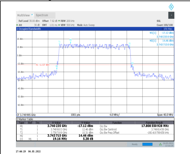
1-N78-3700-3800--30-20-M-3-DFT-16QAM-Outer_Full-50@0-Ant0-17.809-19.160-≤20-PASS
