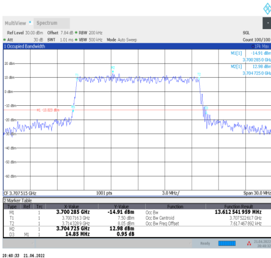
1-N78-3700-3800--30-15-L-8-CP-64QAM-Outer_Full -38@0-Ant0-13.613-14.850-≤15-PASS
