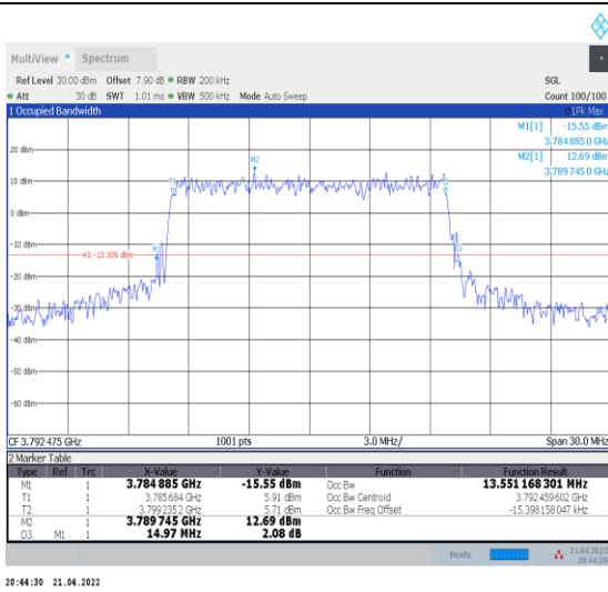
1-N78-3700-3800--30-15-H-8-CP-64QAM-Outer_Full -38@0-Ant0-13.551-14.970-≤15-PASS
