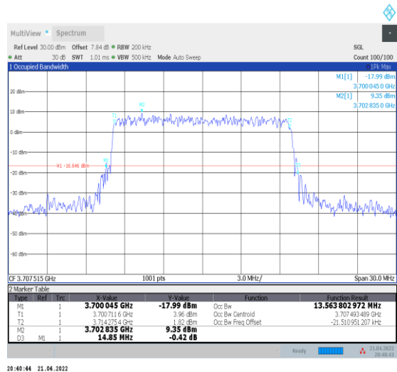
1-N78-3700-3800--30-15-L-9-CP-256QAM-Outer_Fu ll-38@0-Ant0-13.564-14.850-≤15-PASS
