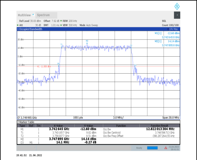
1-N78-3700-3800--30-15-M-4-DFT-64QAM-Outer_Full ull-36@0-Ant0-12.822-14.100-≤15-PASS
