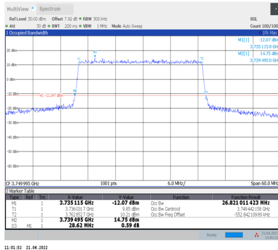
1-N78-3700-3800--30-30-M-4-DFT-64QAM-Outer_Full-75@0-Ant0-26.821-28.620-≤30-PASS
