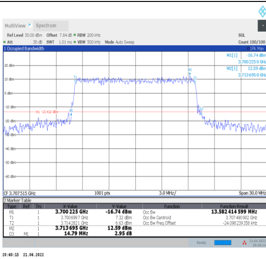
1-N78-3700-3800--30-15-L-6-CP-QPSK-Outer_Full-3 8@0-Ant0-13.582-14.790-≤15-PASS
