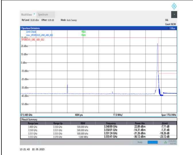
1-N78-3450-3550-PC1-30-100-H-5-CP-QPSK-Edge_1RB_Right-1@272-Ant0-1--PASS-see graph
