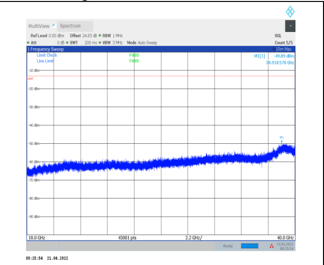
1-N78-3450-3550--30-100-H-1-DFT-PI2BPSK-Inner_1RB_Left-1 @ 1-18000-40000-Ant0--49.89--13-PASS
