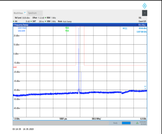
1-N78-3450-3550-PC1-30-100-H-1-DFT-PI2BPSK- Inner_1RB_Left-1@1-1000-6000-Ant0-5937.50--39.46- -13-PASS
