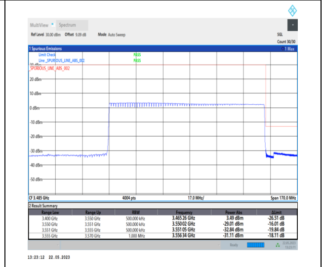
1-N78-3450-3550-PC1-30-100-H-6-CP-QPSK-Outer_Full-273@0-Ant0-1--PASS-see graph
