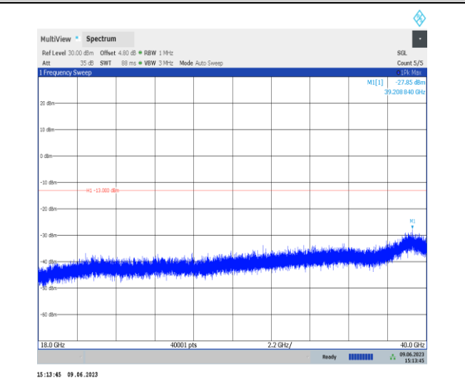
1-N78-3450-3550-PC1-30-100-M-1-DFT-PI2BPSK- Inner_1RB_Left-1@1-18000-40000-Ant0-18000.00--61 .78--13-PASS
