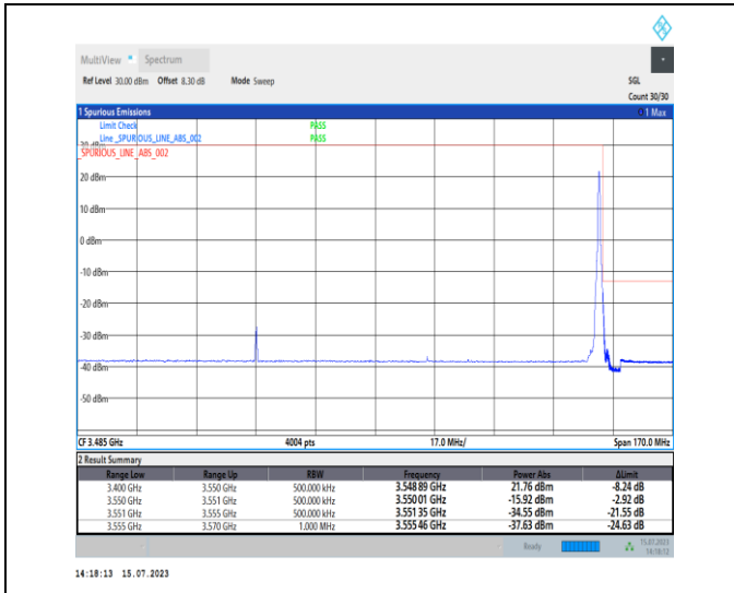
1-N78-3450-3550-PC1-30-100-H-2-DFT-PI2BPSK-Edge_1RB_Right-1@272-Ant0-1--PASS-see graph
