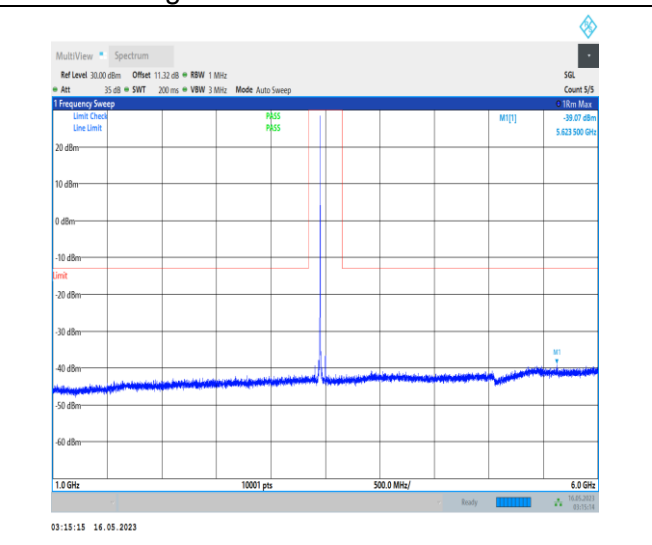
1-N78-3450-3550-PC1-30-100-M-1-DFT-PI2BPSK- Inner_1RB_Left-1@1-1000-6000-Ant0-5623.50--39.07-- 13-PASS
