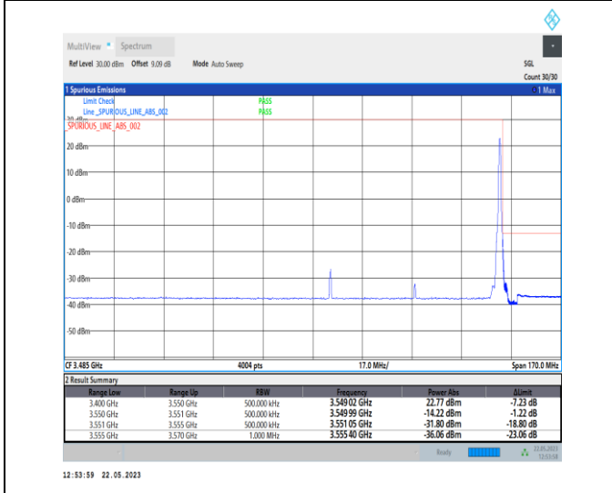
1-N78-3450-3550-PC1-30-60-H-5-CP-QPSK-Edge_1RB_Right-1@161-Ant0-1--PASS-see graph
