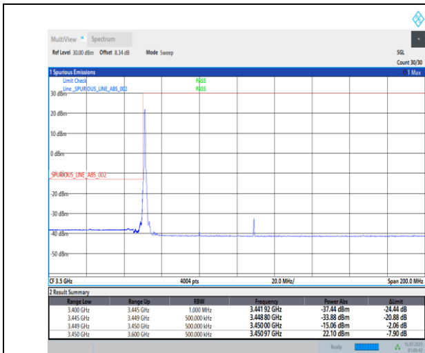
1-N78-3450-3550-PC1-30-60-L-1-DFT-PI2BPSK-Edge_1RB_Left-1@0-Ant0-1--PASS-see graph
