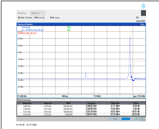
1-N78-3450-3550-PC1-30-60-H-2-DFT-PI2BPSK-Edge_1RB_Right-1@161-Ant0-1--PASS-see graph
