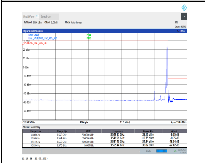
1-N78-3450-3550-PC1-30-15-H-5-CP-QPSK-Edge_1RB_Right-1@37-Ant0-1--PASS-see graph
