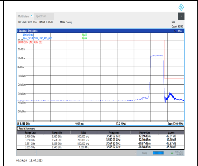
1-N78-3450-3550-PC1-30-15-H-3-DFT-PI2BPSK-Outer_Full-36@0-Ant0-1--PASS-see graph
