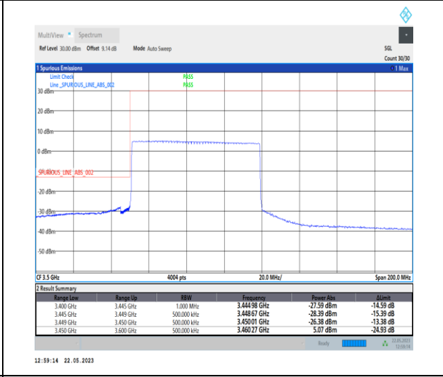
1-N78-3450-3550-PC1-30-70-L-6-CP-QPSK-Outer_Full-189@0-Ant0-1--PASS-see graph
