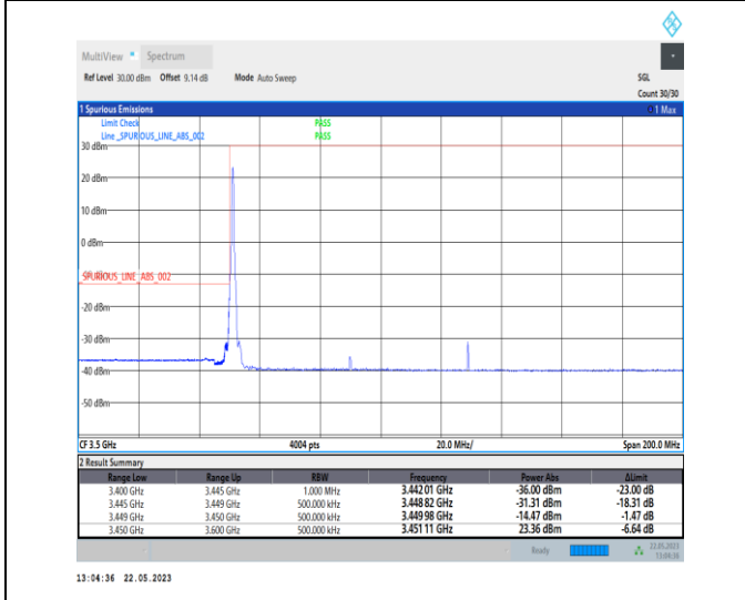
1-N78-3450-3550-PC1-30-80-L-4-CP-QPSK-Edge_1RB_Left-1@0-Ant0-1--PASS-see graph
