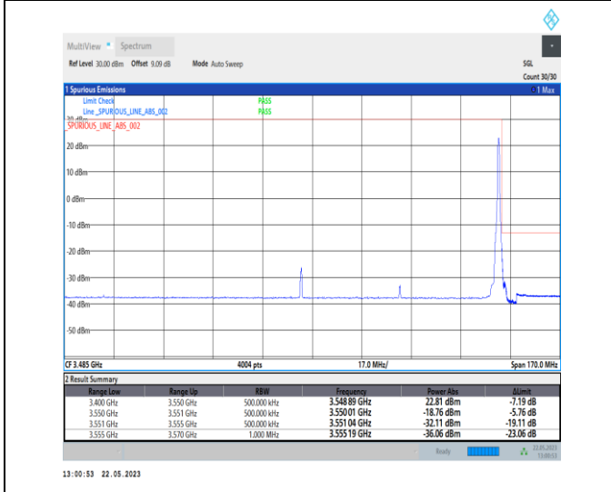
1-N78-3450-3550-PC1-30-70-H-5-CP-QPSK-Edge_1RB_Right-1@188-Ant0-1--PASS-see graph
