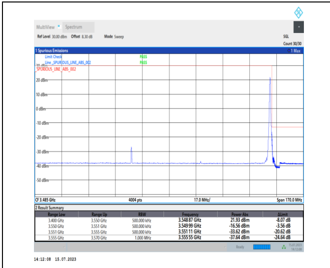
1-N78-3450-3550-PC1-30-90-H-2-DFT-PI2BPSK-Edge_1RB_Right-1@244-Ant0-1--PASS-see graph
