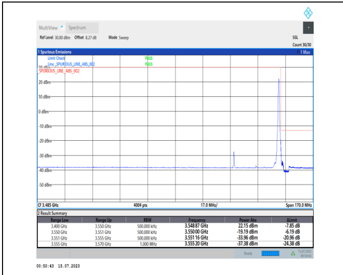
1-N78-3450-3550-PC1-30-30-H-2-DFT-PI2BPSK-Edge _1RB_Right-1@77-Ant0-1--PASS-see graph
