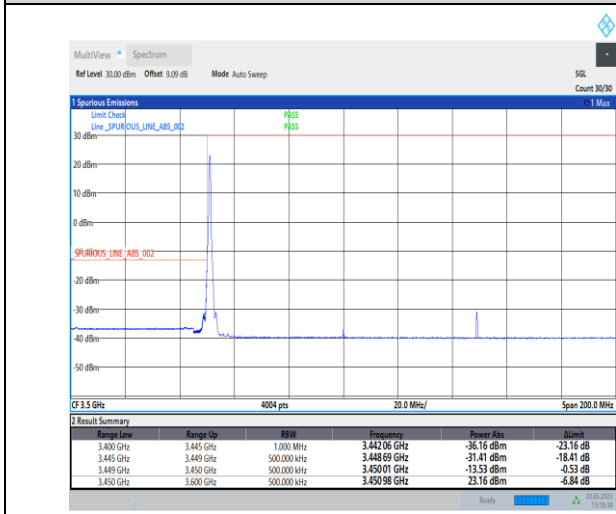
1-N78-3450-3550-PC1-30-100-L-1-DFT-PI2BPSK-Edge_1RB_Left-1@0-Ant0-1--PASS-see graph
