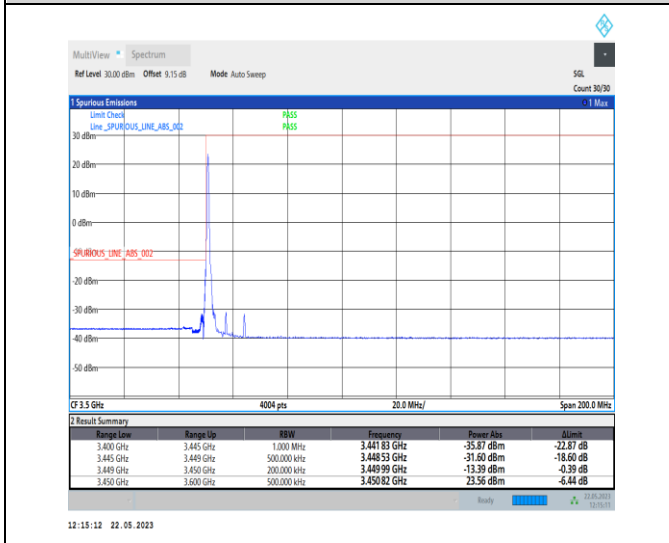
1-N78-3450-3550-PC1-30-15-L-4-CP-QPSK-Edge_1RB_Left-1@0-Ant0-1--PASS-see graph
