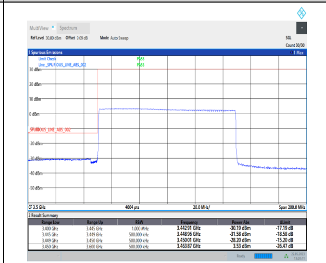
1-N78-3450-3550-PC1-30-100-L-3-DFT-PI2BPSK-Outer_Full-270@0-Ant0-1--PASS-see graph
