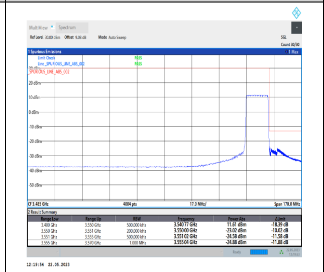
1-N78-3450-3550-PC1-30-15-H-6-CP-QPSK-Outer_Full-38@0-Ant0-1--PASS-see graph
