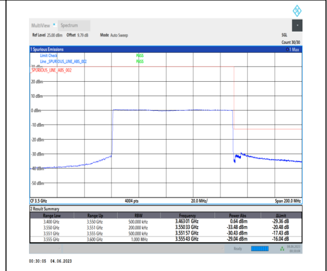
1-N78-3450-3550-PC1-30-90-H-6-CP-QPSK-Outer_Full-245@0-Ant0-1--PASS-see graph
