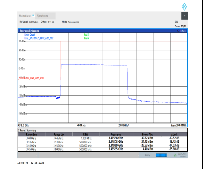
1-N78-3450-3550-PC1-30-80-L-6-CP-QPSK-Outer_Full-217@0-Ant0-1--PASS-see graph
