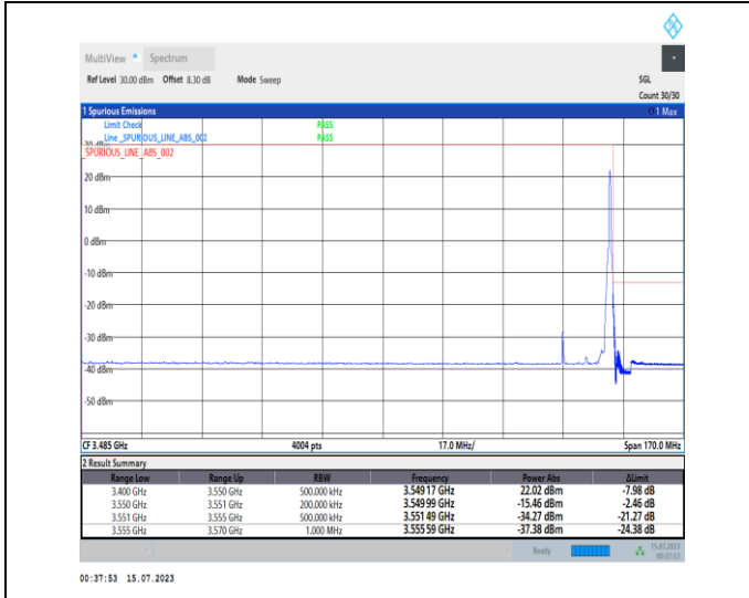
1-N78-3450-3550-PC1-30-15-H-2-DFT-PI2BPSK-Edge_1RB_Right-1@37-Ant0-1--PASS-see graph
