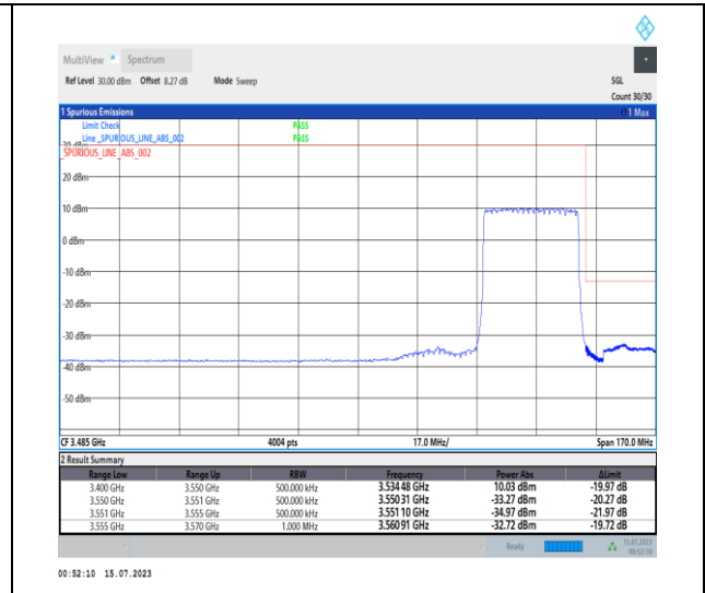
1-N78-3450-3550-PC1-30-30-H-3-DFT-PI2BPSK- Outer_Full-75@0-Ant0-1--PASS-see graph
