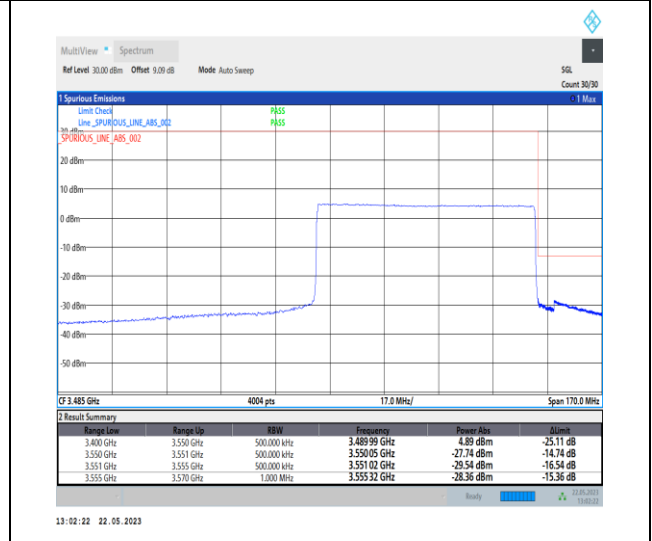
1-N78-3450-3550-PC1-30-70-H-6-CP-QPSK-Outer_Full-189@0-Ant0-1--PASS-see graph
