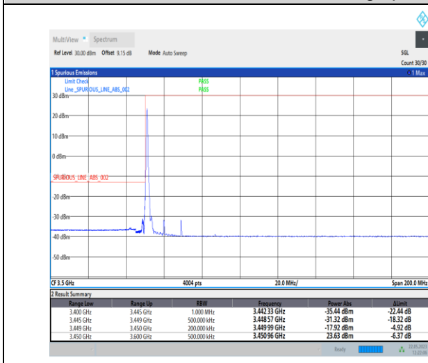
1-N78-3450-3550-PC1-30-20-L-4-CP-QPSK-Edge_1_RB_Left-1@0-Ant0-1--PASS-see graph
