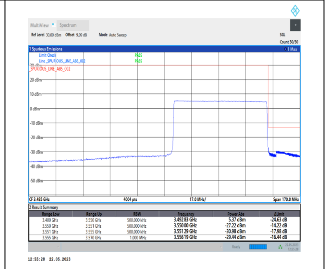
1-N78-3450-3550-PC1-30-60-H-6-CP-QPSK-Outer_Full-162@0-Ant0-1--PASS-see graph
