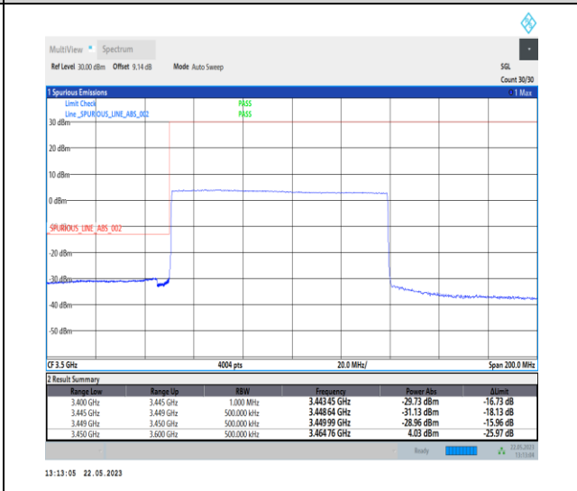
1-N78-3450-3550-PC1-30-90-L-6-CP-QPSK-Outer_Full-245@0-Ant0-1--PASS-see graph
