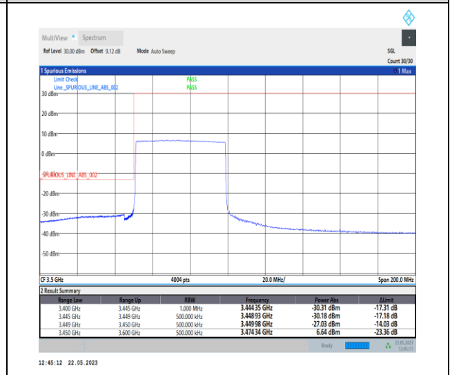
1-N78-3450-3550-PC1-30-50-L-6-CP-QPSK-Outer_Full-133@0-Ant0-1--PASS-see graph
