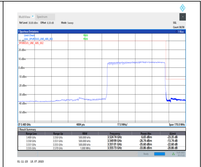
1-N78-3450-3550-PC1-30-60-H-3-DFT-PI2BPSK-Outer_Full-162@0-Ant0-1--PASS-see graph
