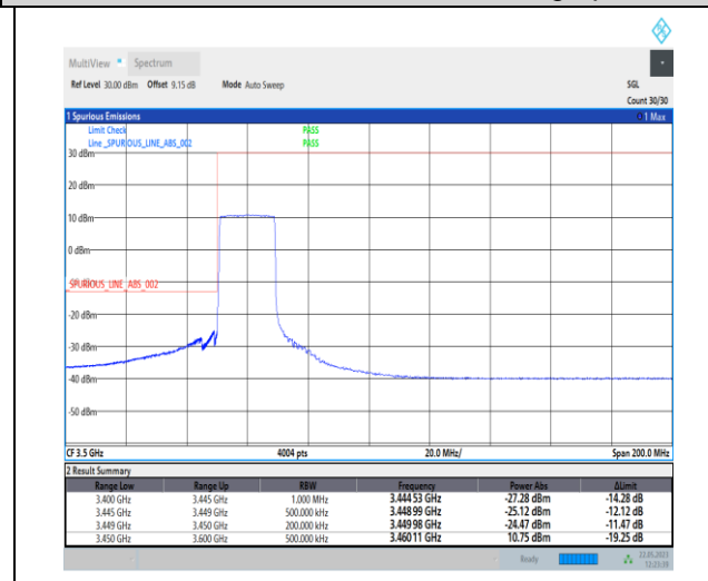
1-N78-3450-3550-PC1-30-20-L-6-CP-QPSK-Outer_Full-51@0-Ant0-1--PASS-see graph
