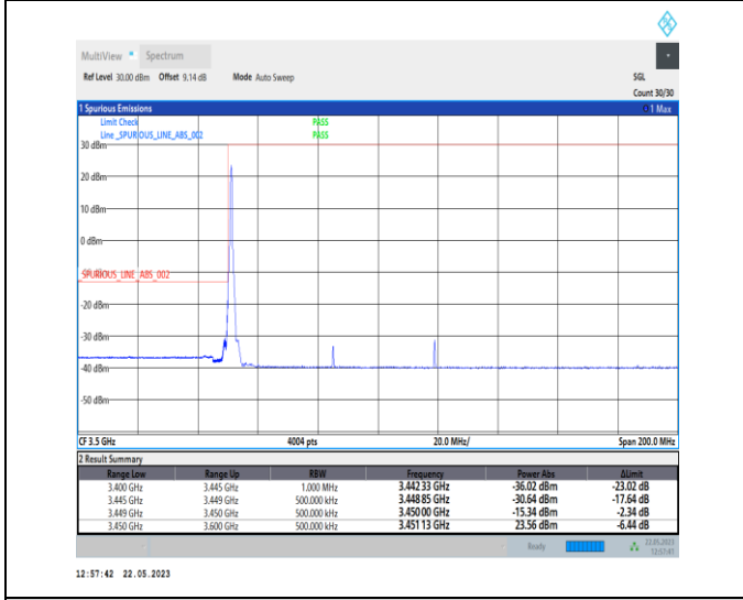
1-N78-3450-3550-PC1-30-70-L-4-CP-QPSK-Edge_1RB_Left-1@0-Ant0-1--PASS-see graph
