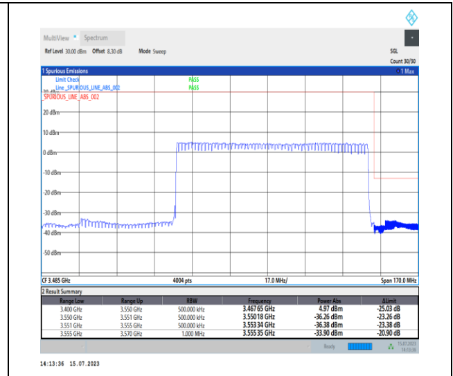
1-N78-3450-3550-PC1-30-90-H-3-DFT-PI2BPSK-Outer_Full-240@0-Ant0-1--PASS-see graph
