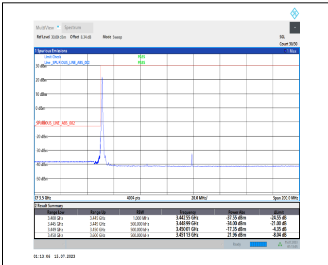
1-N78-3450-3550-PC1-30-70-L-1-DFT-PI2BPSK-Edge_1RB_Left-1@0-Ant0-1--PASS-see graph
