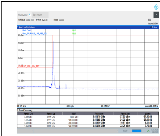
1-N78-3450-3550-PC1-30-20-L-1-DFT-PI2BPSK-Edge_1_RB_Left-1@0-Ant0-1--PASS-see graph
