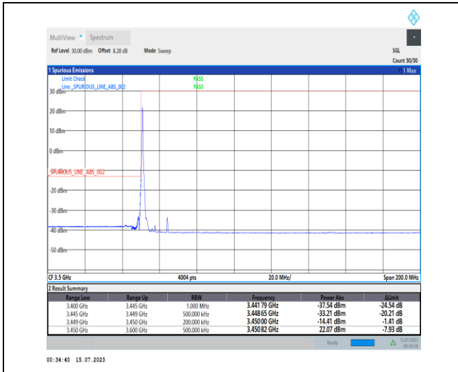
1-N78-3450-3550-PC1-30-15-L-1-DFT-PI2BPSK-Edge_e_1RB_Left-1@0-Ant0-1--PASS-see graph
