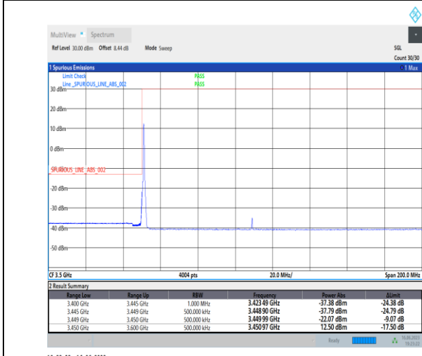
1-N78-3450-3550-PC1-30-60-L-4-CP-QPSK-Edge_1RB_Left-1@0-Ant0-1--PASS-see graph
