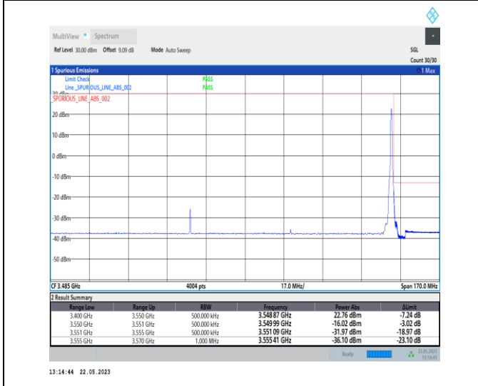
1-N78-3450-3550-PC1-30-90-H-5-CP-QPSK-Edge_1RB_Right-1@244-Ant0-1--PASS-see graph
