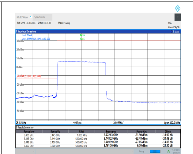
1-N78-3450-3550-PC1-30-60-L-3-DFT-PI2BPSK-Outer_Full-162@0-Ant0-1--PASS-see graph
