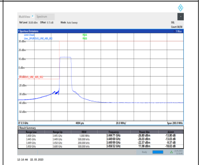
1-N78-3450-3550-PC1-30-15-L-6-CP-QPSK-Outer_Full-38@0-Ant0-1--PASS-see graph
