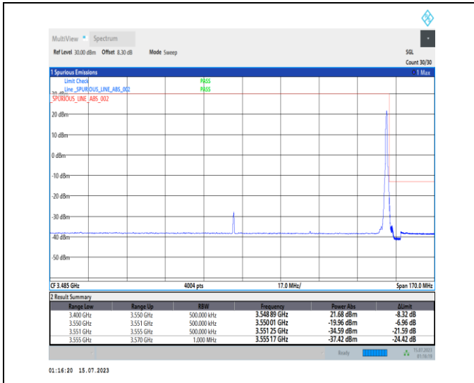
1-N78-3450-3550-PC1-30-70-H-2-DFT-PI2BPSK-Edge_1RB_Right-1@188-Ant0-1--PASS-see graph
