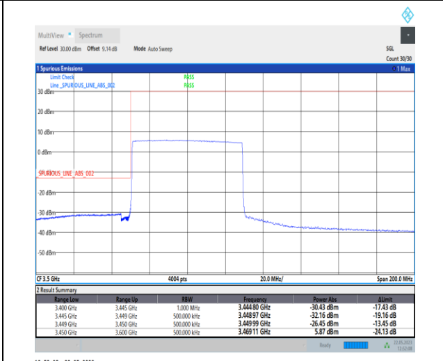
1-N78-3450-3550-PC1-30-60-L-6-CP-QPSK-Outer_Full-162@0-Ant0-1--PASS-see graph
