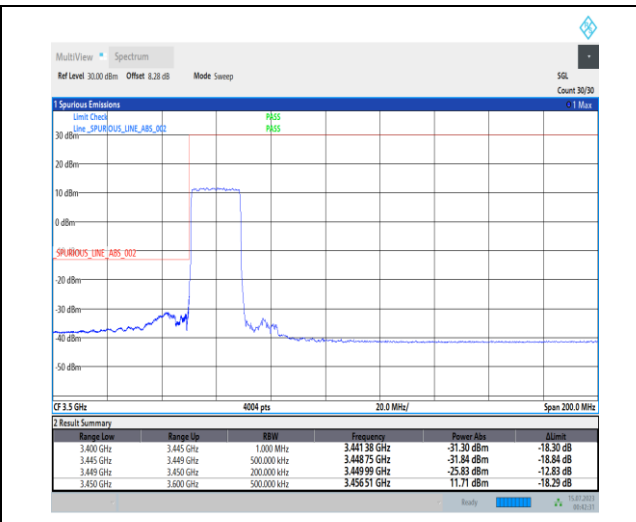
1-N78-3450-3550-PC1-30-20-L-3-DFT-PI2BPSK-Outer_Full-50@0-Ant0-1--PASS-see graph
