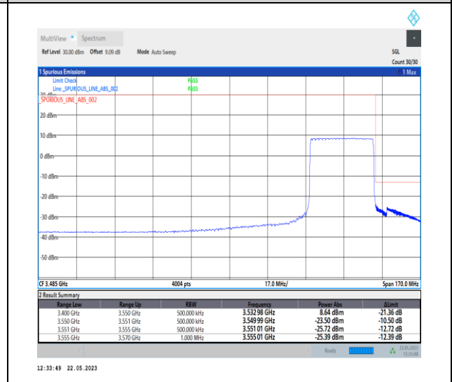
1-N78-3450-3550-PC1-30-30-H-6-CP-QPSK-Outer _Full-78@0-Ant0-1--PASS-see graph
