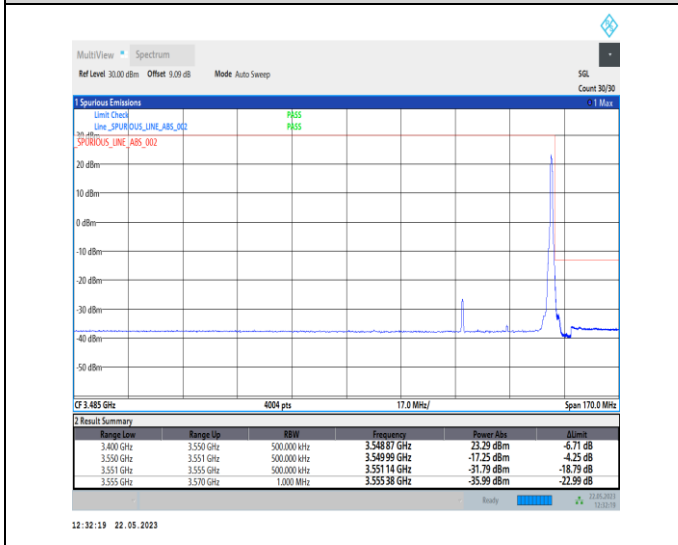
1-N78-3450-3550-PC1-30-30-H-5-CP-QPSK-Edge_1R B_Right-1@77-Ant0-1--PASS-see graph
