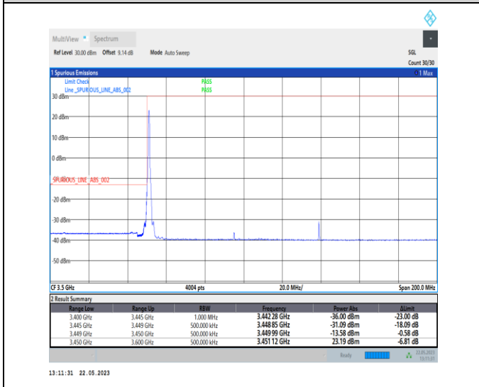
1-N78-3450-3550-PC1-30-90-L-4-CP-QPSK-Edge_1RB_Left-1@0-Ant0-1--PASS-see graph
