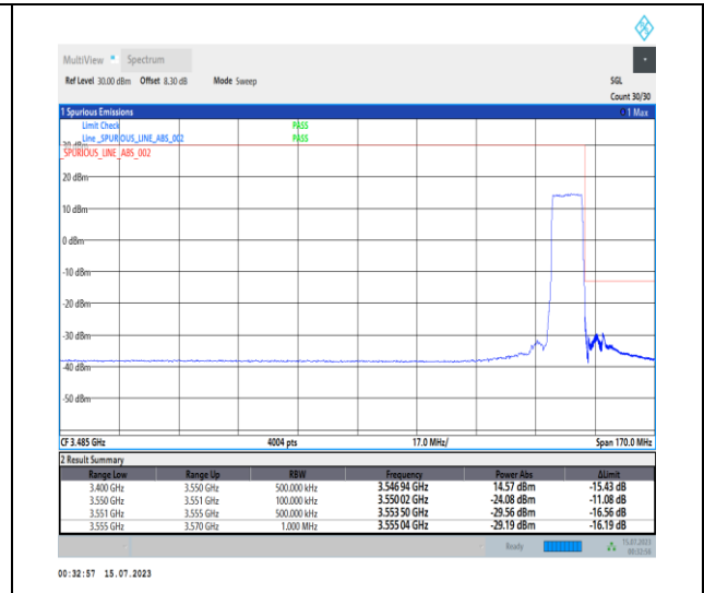
1-N78-3450-3550-PC1-30-10-H-3-DFT-PI2BPSK-Outer_Full-24@0-Ant0-1--PASS-see graph
