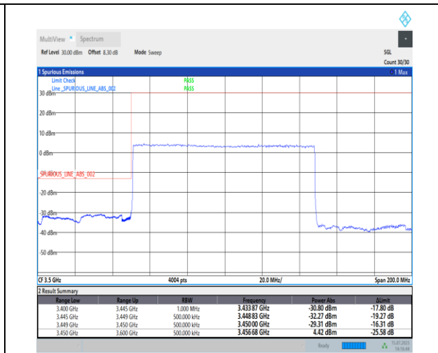
1-N78-3450-3550-PC1-30-100-L-3-DFT-PI2BPSK-Outer_Full-270@0-Ant0-1--PASS-see graph
