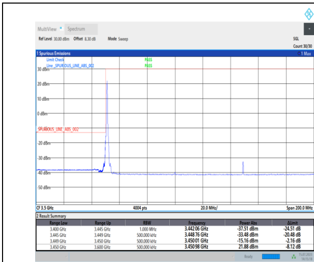
1-N78-3450-3550-PC1-30-100-L-1-DFT-PI2BPSK-Edge_1RB_Left-1@0-Ant0-1--PASS-see graph
