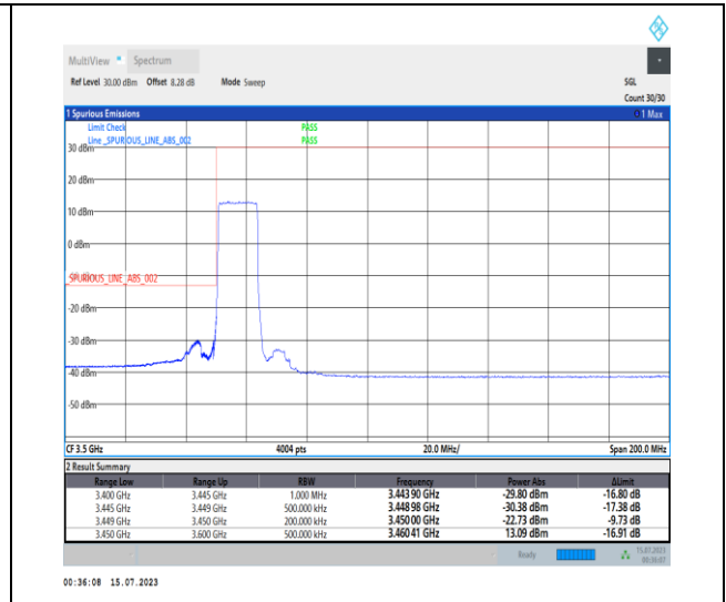
1-N78-3450-3550-PC1-30-15-L-3-DFT-PI2BPSK-Outer_Full-36@0-Ant0-1--PASS-see graph
