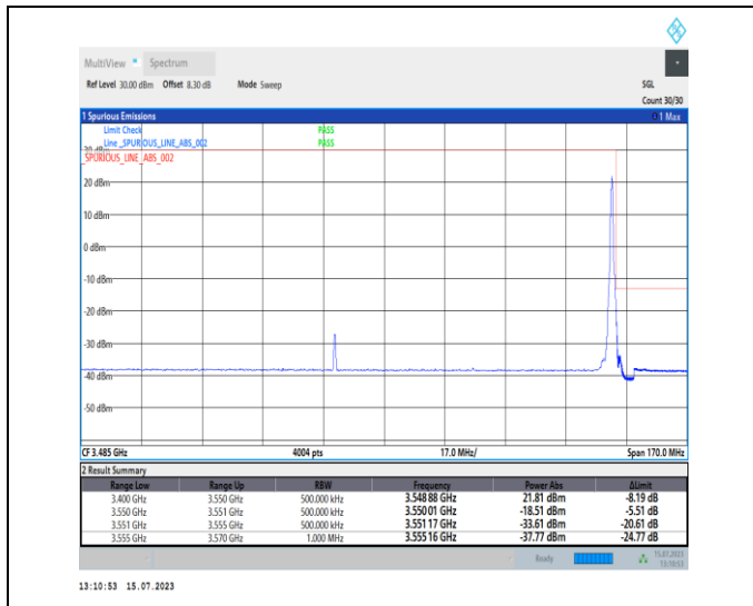
1-N78-3450-3550-PC1-30-80-H-2-DFT-PI2BPSK-Edge_e_1RB_Right-1@216-Ant0-1--PASS-see graph
