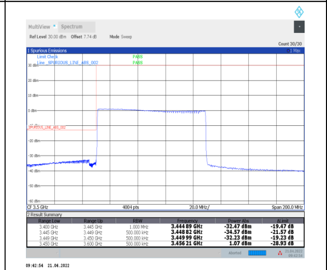
1-N78-3450-3550--30-80-L-6-CP-QPSK-Outer_Ful_I-217@0-Ant0-PASS-see graph
