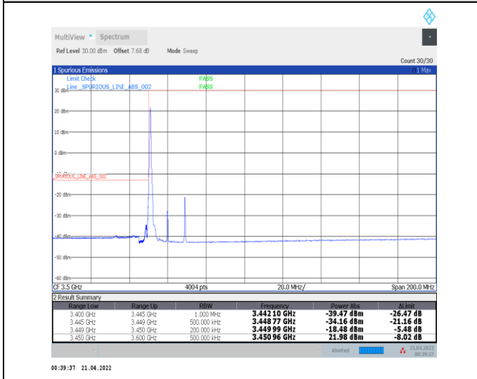
1-N78-3450-3550--30-20-L-4-CP-QPSK-Edge_1RB_L_eff-1@0-Ant0-PASS-see graph
