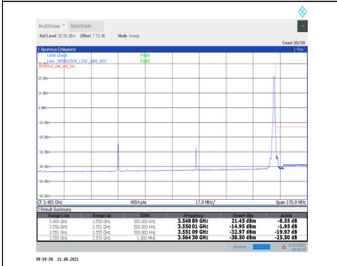
1-N78-3450-3550--30-100-H-5-CP-QPSK-Edge_1RB_Right-1@272-Ant0-PASS-see graph
