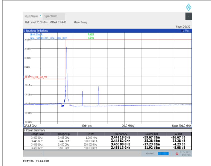
1-N78-3450-3550--30-40-L-4-CP-QPSK-Edge_1RB_L_eff-1@0-Ant0-PASS-see graph
