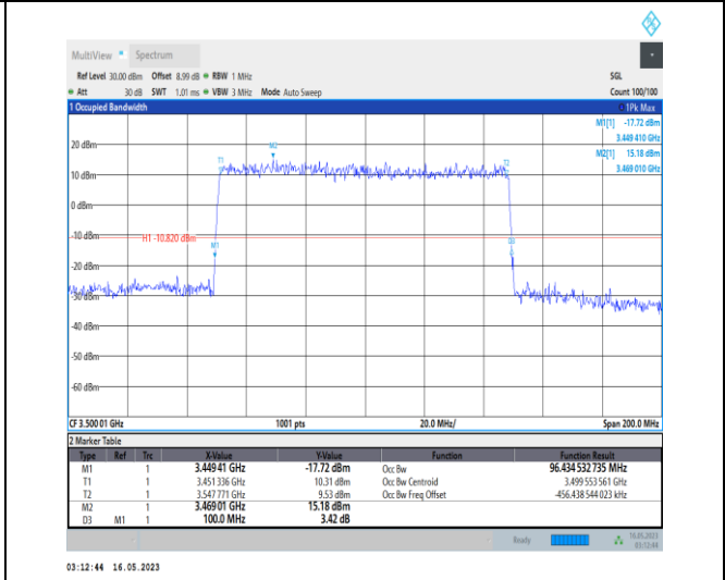
1-N78-3450-3550-PC1-30-100-H-4-DFT-64QAM-Outer_Full-270@0-Ant0-96.435-100.000-≤100-PASS
