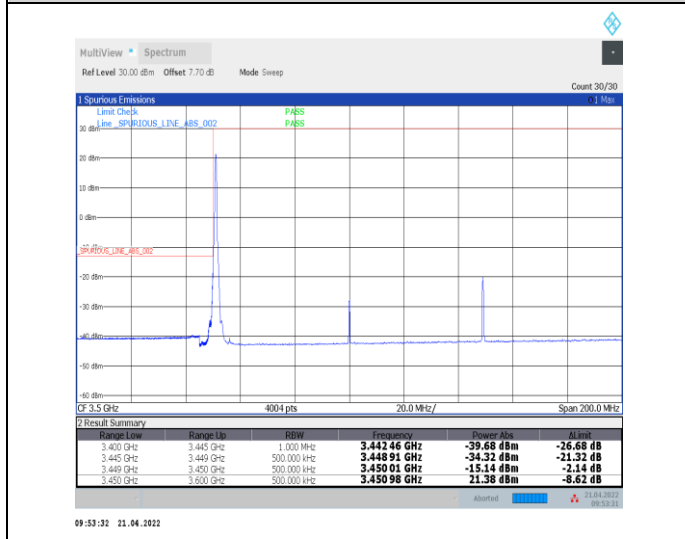
1-N78-3450-3550--30-100-L-4-CP-QPSK-Edge_1RB_Left-1@0-Ant0-PASS-see graph
