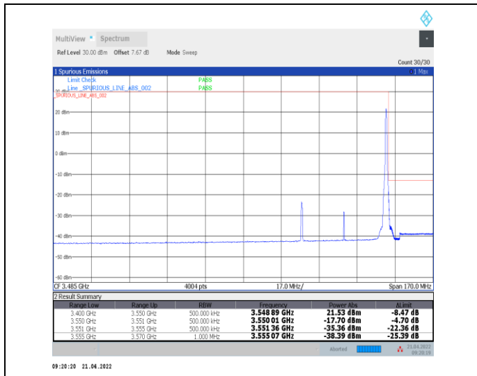
1-N78-3450-3550--30-40-H-2-DFT-PI2BPSK-Edge_1R_B_Right-1@105-Ant0-PASS-see graph
