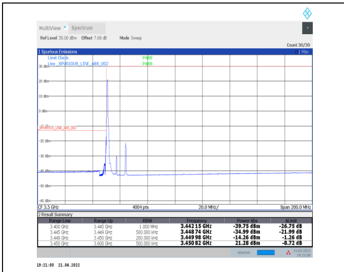
1-N78-3450-3550--30-15-L-1-DFT-PI2BPSK-Edge_1R_B_Left-1@0-Ant0-PASS-see graph
