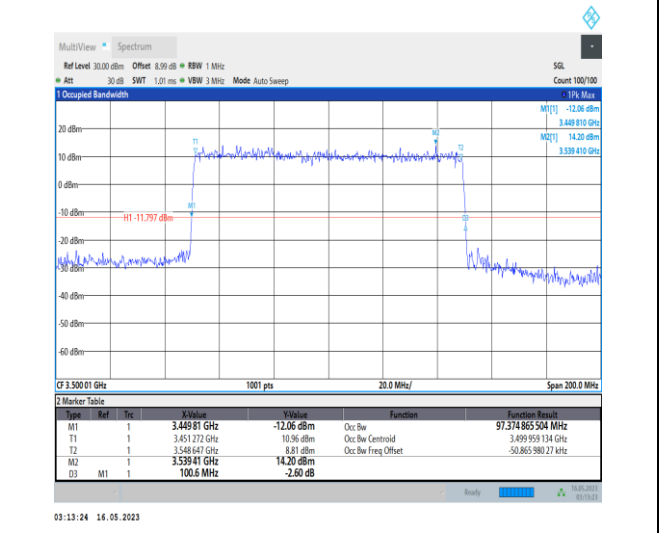
1-N78-3450-3550-PC1-30-100-H-8-CP-64QAM-Outer_Full-273@0-Ant0-97.375-100.600-≤100-PASS
