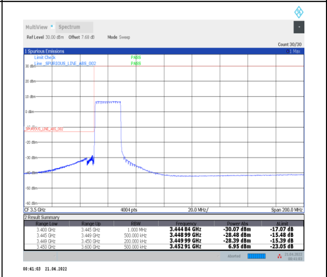
1-N78-3450-3550--30-20-L-6-CP-QPSK-Outer_Ful_I-51@0-Ant0-PASS-see graph
