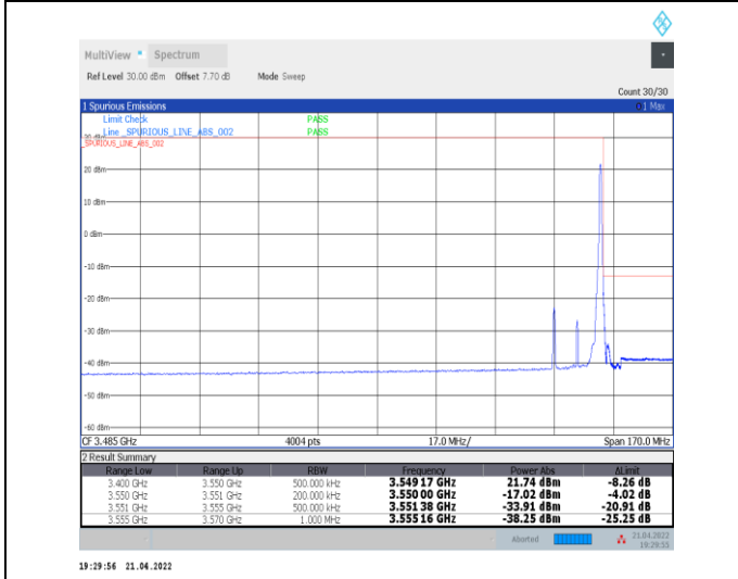
1-N78-3450-3550--30-15-H-5-CP-QPSK-Edge_1RB_Right-1@37-Ant0-PASS-see graph
