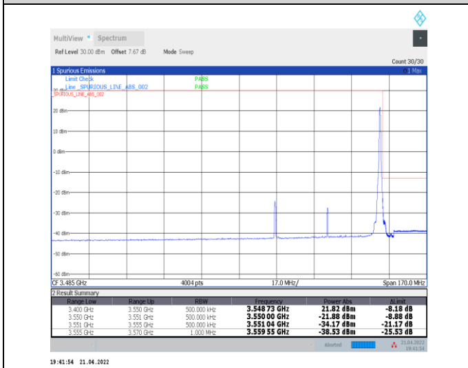
1-N78-3450-3550--30-50-H-5-CP-QPSK-Edge_1RB_Right-1@132-Ant0-PASS-see graph
