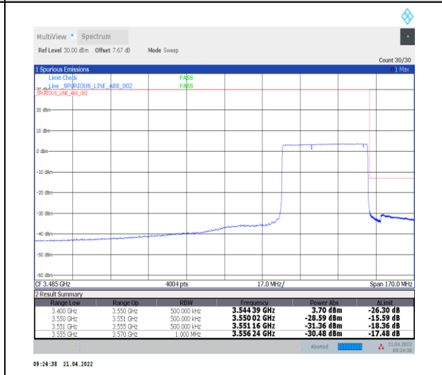
1-N78-3450-3550--30-40-H-6-CP-QPSK-Outer_Full-106@0-Ant0-PASS-see graph
