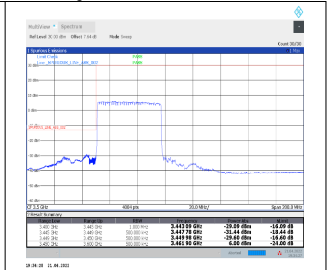
1-N78-3450-3550--30-50-L-3-DFT-PI2BPSK-Outer_Full-128@0-Ant0-PASS-see graph
