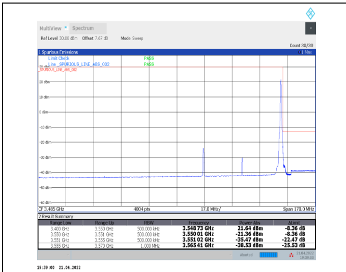
1-N78-3450-3550--30-50-H-2-DFT-PI2BPSK-Edge_1R_B_Right-1@132-Ant0-PASS-see graph
