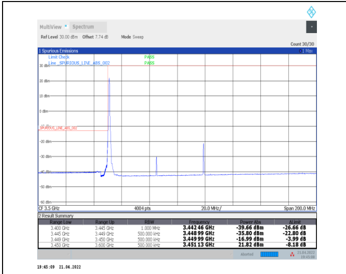
1-N78-3450-3550--30-70-L-1-DFT-PI2BPSK-Edge_1R_B_Left-1@0-Ant0-PASS-see graph
