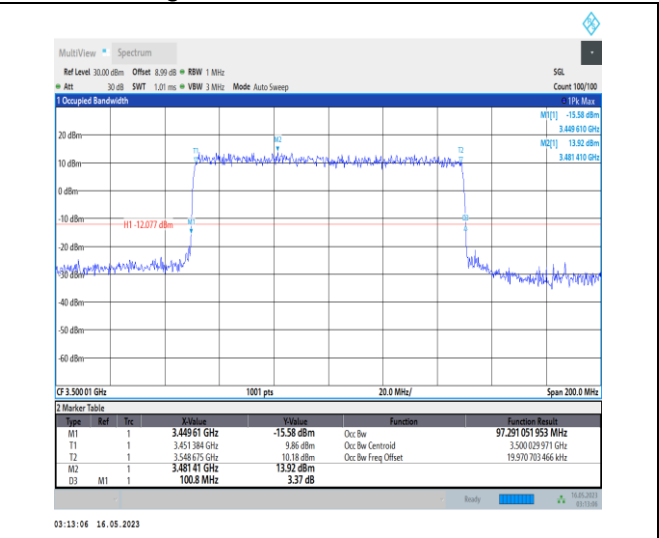
1-N78-3450-3550-PC1-30-100-H-6-CP-QPSK-Outer_Full-273@0-Ant0-97.291-100.800-≤100-PASS
