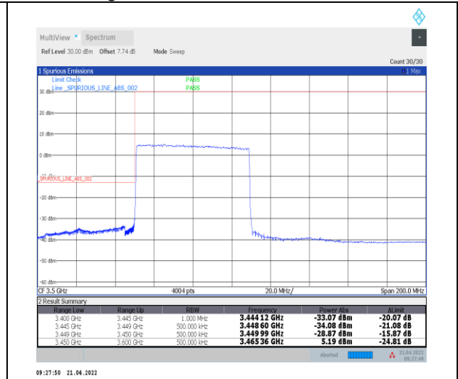
1-N78-3450-3550--30-60-L-3-DFT-PI2BPSK-Outer_Full-162@0-Ant0-PASS-see graph
