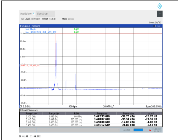
1-N78-3450-3550--30-30-L-1-DFT-PI2BPSK-Edge_1R_B_Left-1@0-Ant0-PASS-see graph
