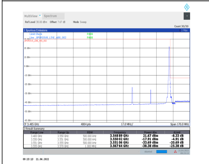
1-N78-3450-3550--30-40-H-5-CP-QPSK-Edge_1RB_Right-1@105-Ant0-PASS-see graph
