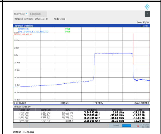
1-N78-3450-3550--30-50-H-6-CP-QPSK-Outer_Full-113@0-Ant0-PASS-see graph
