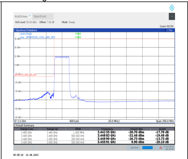
1-N78-3450-3550--30-20-L-3-DFT-PI2BPSK-Outer_Full-50@0-Ant0-PASS-see graph
