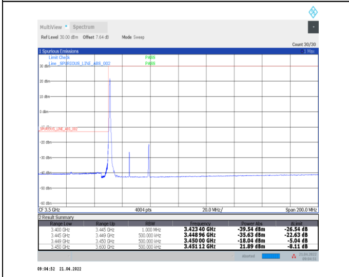
1-N78-3450-3550--30-30-L-4-CP-QPSK-Edge_1RB_L_eff-1@0-Ant0-PASS-see graph
