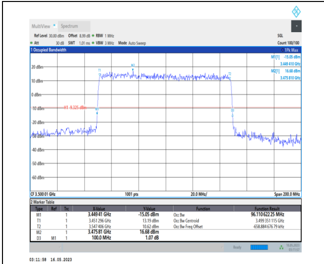
1-N78-3450-3550-PC1-30-100-H-1-DFT-QPSK-Outer_Full-270@0-Ant0-96.111-100.000-≤100-PASS
