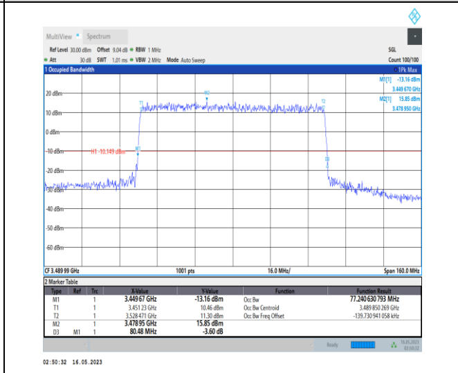
1-N78-3450-3550-PC1-30-80-L-4-DFT-64QAM-Outer_Full-216@0-Ant0-77.241-80.480-≤80-PASS
