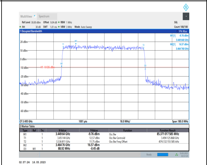
1-N78-3450-3550-PC1-30-90-L-1-DFT-QPSK-Outer_Full-240@0-Ant0-85.371-88.920-≤90-PASS
