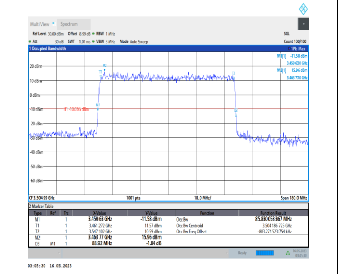
1-N78-3450-3550-PC1-30-90-H-3-DFT-16QAM-Outer_Full-240@0-Ant0-85.83-88.920-≤90-PASS
