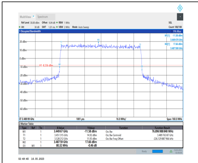
1-N78-3450-3550-PC1-30-80-L-1-DFT-QPSK-Outer_Full-216@0-Ant0-76.897-80.320-≤80-PASS
