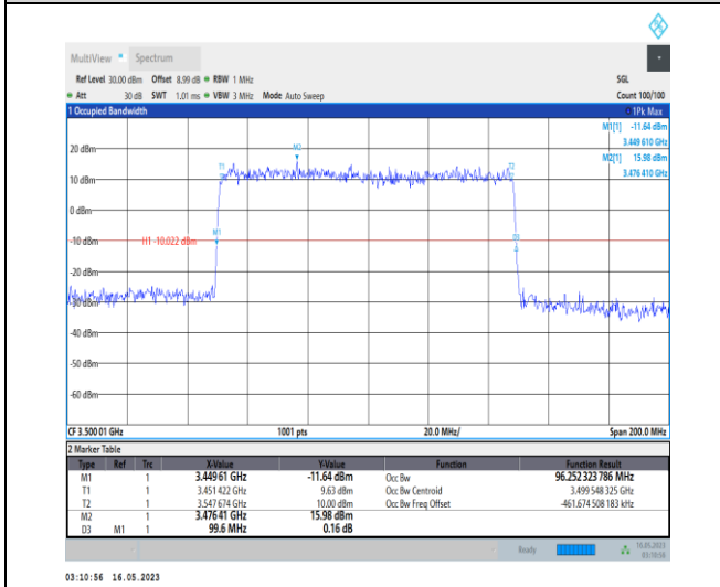
1-N78-3450-3550-PC1-30-100-M-4-DFT-64QAM-Out_Full-270@0-Ant0-96.252-99.600-≤100-PASS
