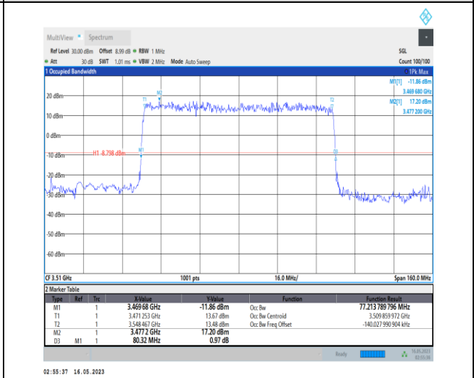
1-N78-3450-3550-PC1-30-80-H-2-DFT-PI2BPSK-Outer_Full-216@0-Ant0-77.214-80.320-≤80-PASS
