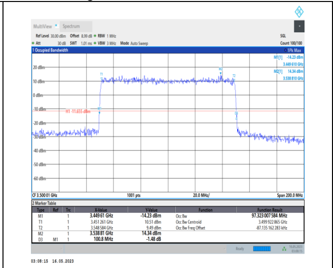
1-N78-3450-3550-PC1-30-100-L-8-CP-64QAM-Outer_Full-273@0-Ant0-97.323-100.800-≤100-PASS
