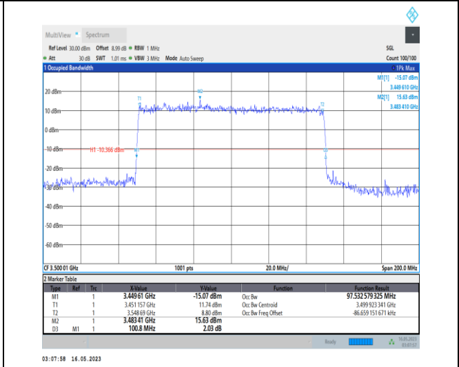
1-N78-3450-3550-PC1-30-100-L-6-CP-QPSK-Outer Full-273@0-Ant0-97.533-100.800-≤100-PASS
