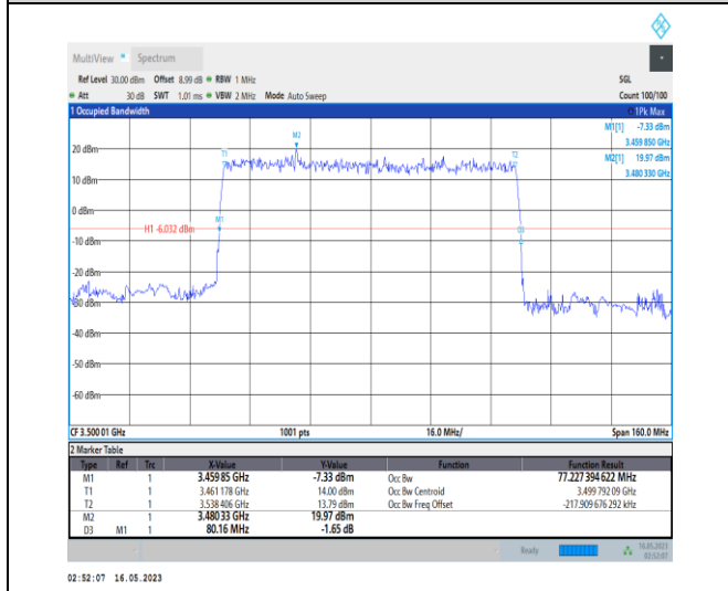
1-N78-3450-3550-PC1-30-80-M-2-DFT-PI2BPSK-Outer_Full-216@0-Ant0-77.227-80.160-≤80-PASS
