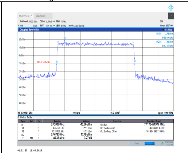
1-N78-3450-3550-PC1-30-80-M-1-DFT-QPSK-Outer_Full-216@0-Ant0-77.176-80.320-≤80-PASS
