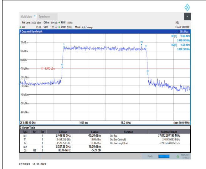
1-N78-3450-3550-PC1-30-80-L-3-DFT-16QAM-Outer_Full-216@0-Ant0-77.013-80.160-≤80-PASS
