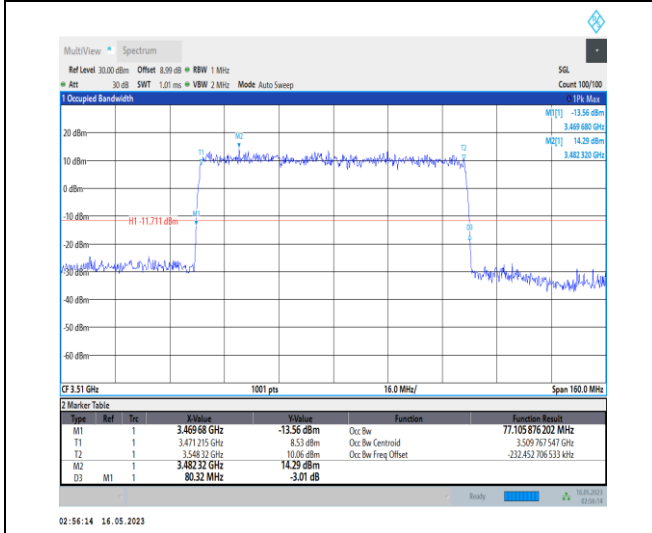
1-N78-3450-3550-PC1-30-80-H-5-DFT-256QAM-Outer_Full-216@0-Ant0-77.106-80.320-≤80-PASS
