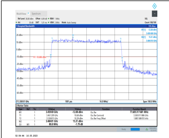
1-N78-3450-3550-PC1-30-80-M-8-CP-64QAM-Outer_Full-217@0-Ant0-77.605-80.800-≤80-PASS
