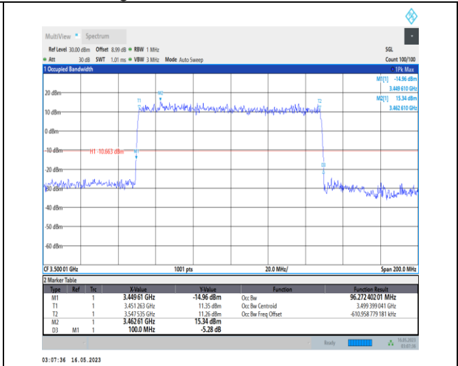
1-N78-3450-3550-PC1-30-100-L-4-DFT-64QAM-Out er_Full-270@0-Ant0-96.272-100.000-≤100-PASS
