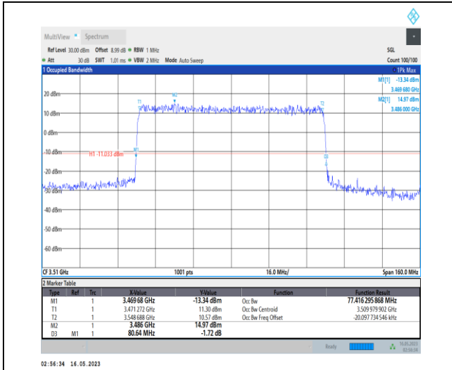
1-N78-3450-3550-PC1-30-80-H-7-CP-16QAM-Outer_Full-217@0-Ant0-77.416-80.640-≤80-PASS
