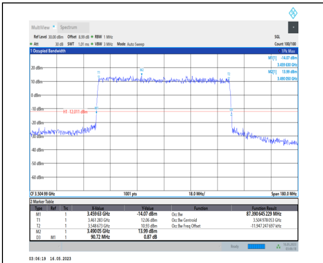
1-N78-3450-3550-PC1-30-90-H-8-CP-64QAM-Outer_Full-245@0-Ant0-87.391-90.720-≤90-PASS
