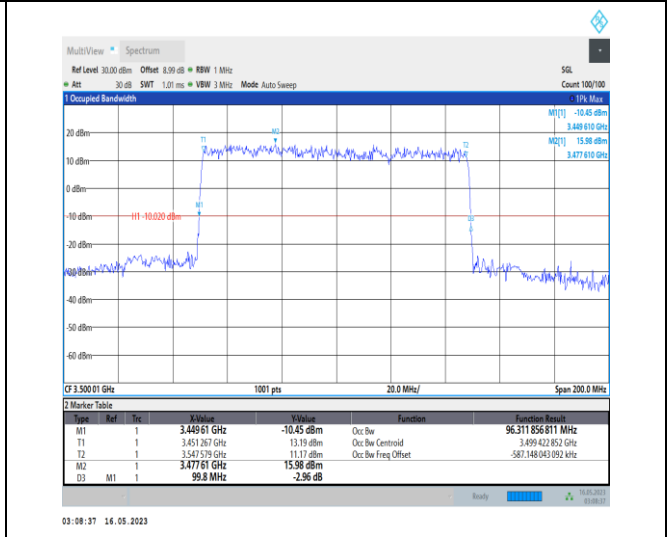
1-N78-3450-3550-PC1-30-100-M-1-DFT-QPSK-Outer_Full-270@0-Ant0-96.312-99.800-≤100-PASS
