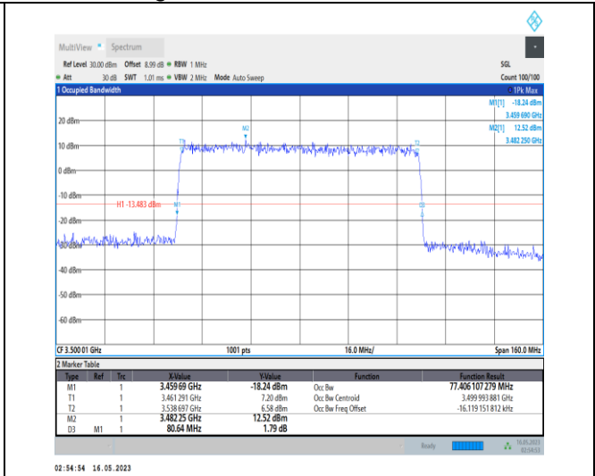
1-N78-3450-3550-PC1-30-80-M-9-CP-256QAM-Outer_Full-217@0-Ant0-77.406-80.640-≤80-PASS
