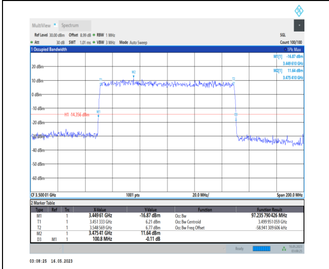
1-N78-3450-3550-PC1-30-100-L-9-CP-256QAM-Outer_Full-273@0-Ant0-97.236-100.800-≤100-PASS
