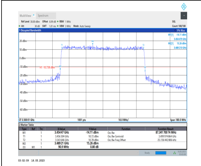
1-N78-3450-3550-PC1-30-90-M-7-CP-16QAM-Outer_Full-245@0-Ant0-87.342-90.900-≤90-PASS
