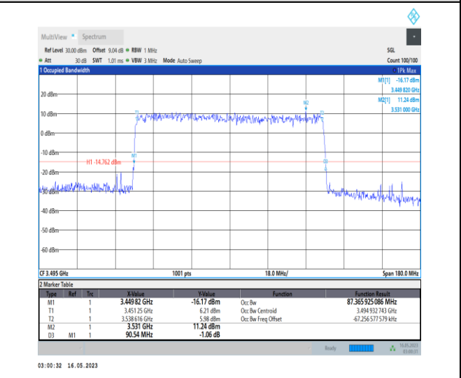
1-N78-3450-3550-PC1-30-90-L-9-CP-256QAM-Outer_Full-245@0-Ant0-87.366-90.540-<math>\leq 90</math>-PASS
