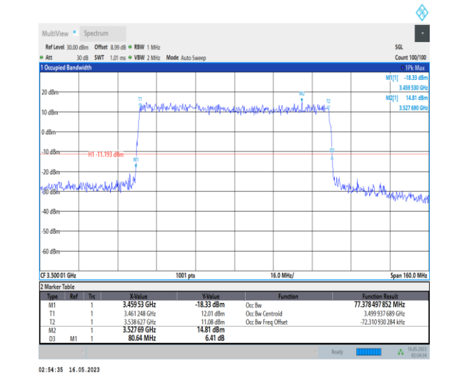
1-N78-3450-3550-PC1-30-80-M-7-CP-16QAM-Outer_Full-217@0-Ant0-77.378-80.640-≤80-PASS
