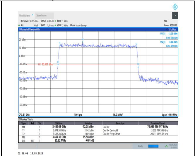
1-N78-3450-3550-PC1-30-80-H-4-DFT-64QAM-Outer_Full-216@0-Ant0-76.983-80.320-≤80-PASS
