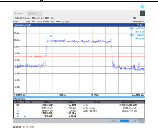
1-N78-3450-3550-PC1-30-90-H-9-CP-256QAM-Outer_Full-245@0-Ant0-87.41-90.900-≤90-PASS
