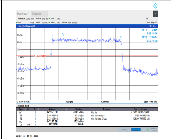
1-N78-3450-3550-PC1-30-80-M-3-DFT-16QAM-Outer_Full-216@0-Ant0-77.212-80.320-≤80-PASS
