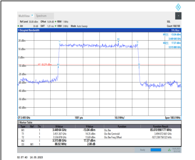
1-N78-3450-3550-PC1-30-90-L-2-DFT-PI2BPSK-Out er_Full-240@0-Ant0-85.611-88.920-≤90-PASS
