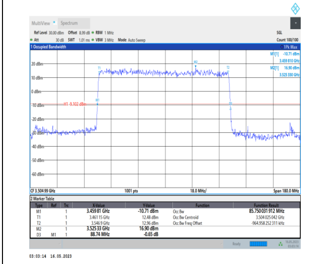
1-N78-3450-3550-PC1-30-90-H-2-DFT-PI2BPSK-Outer_Full-240@0-Ant0-85.75-88.740-≤90-PASS
