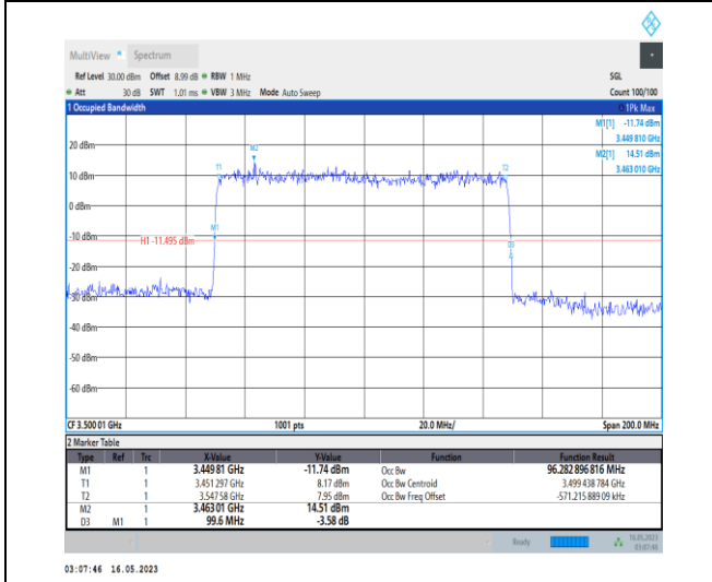
1-N78-3450-3550-PC1-30-100-L-5-DFT-256QAM-Out er_Full-270@0-Ant0-96.283-99.600-≤100-PASS
