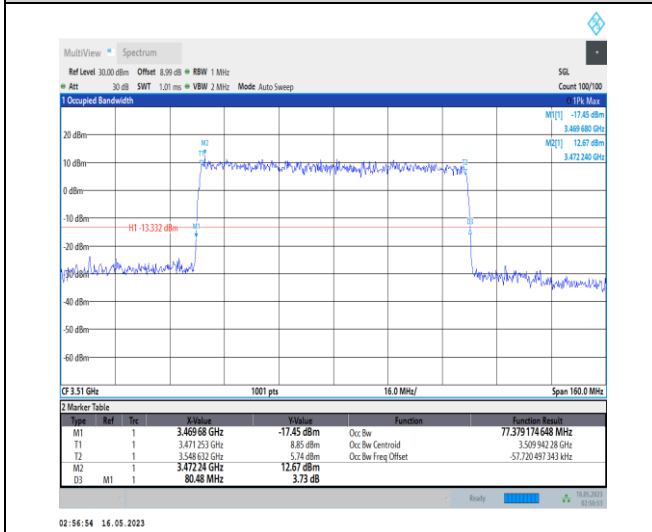
1-N78-3450-3550-PC1-30-80-H-9-CP-256QAM-Outer_Full-217@0-Ant0-77.379-80.480-≤80-PASS
