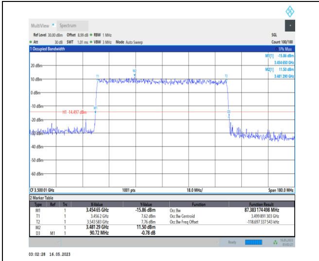
1-N78-3450-3550-PC1-30-90-M-9-CP-256QAM-Out er_Full-245@0-Ant0-87.383-90.720-≤90-PASS
