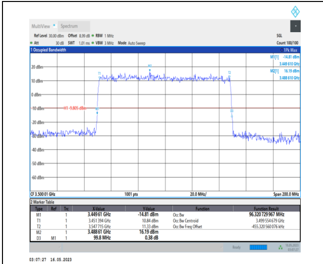
1-N78-3450-3550-PC1-30-100-L-3-DFT-16QAM-Out er_Full-270@0-Ant0-96.321-99.800-≤100-PASS
