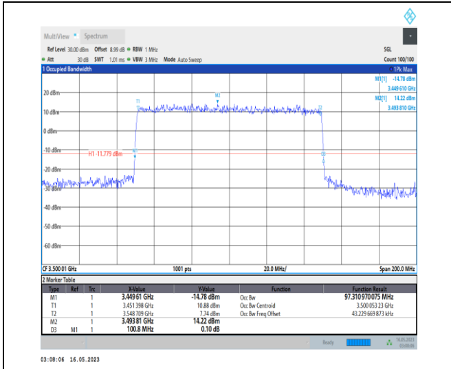
1-N78-3450-3550-PC1-30-100-L-7-CP-16QAM-Outer_Full-273@0-Ant0-97.311-100.800-≤100-PASS
