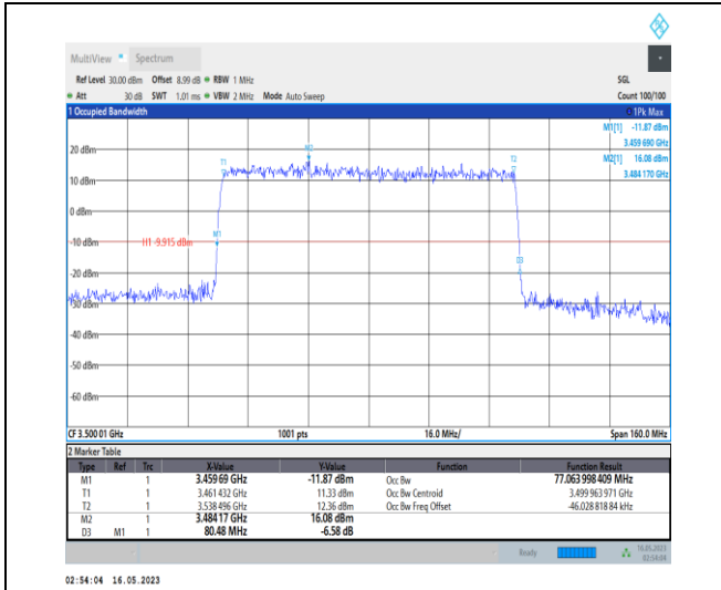
1-N78-3450-3550-PC1-30-80-M-4-DFT-64QAM-Out_er_Full-216@0-Ant0-77.064-80.480-≤80-PASS
