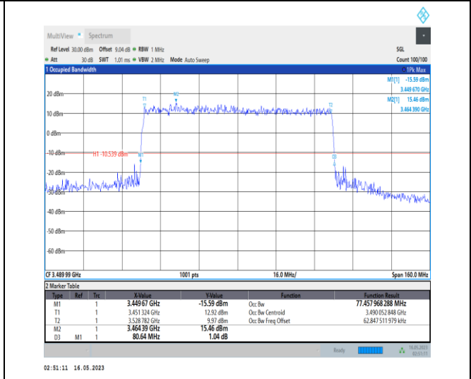
1-N78-3450-3550-PC1-30-80-L-8-CP-64QAM-Outer_Full-217@0-Ant0-77.458-80.640-<math>\leq 80</math>-PASS
