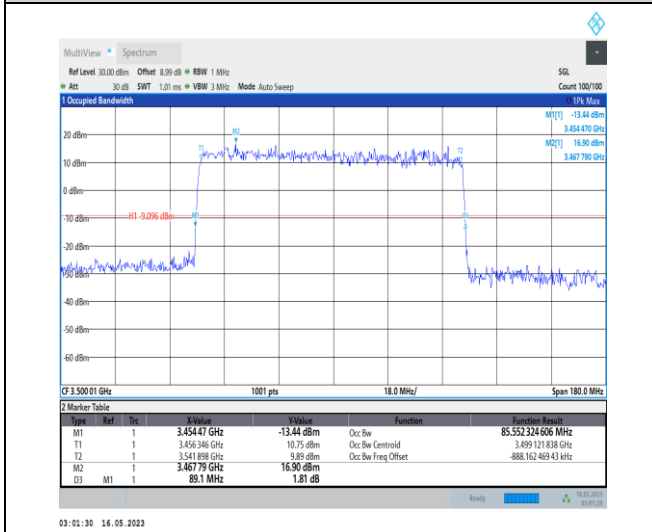
1-N78-3450-3550-PC1-30-90-M-3-DFT-16QAM-Outer_Full-240@0-Ant0-85.552-89.100-≤90-PASS
