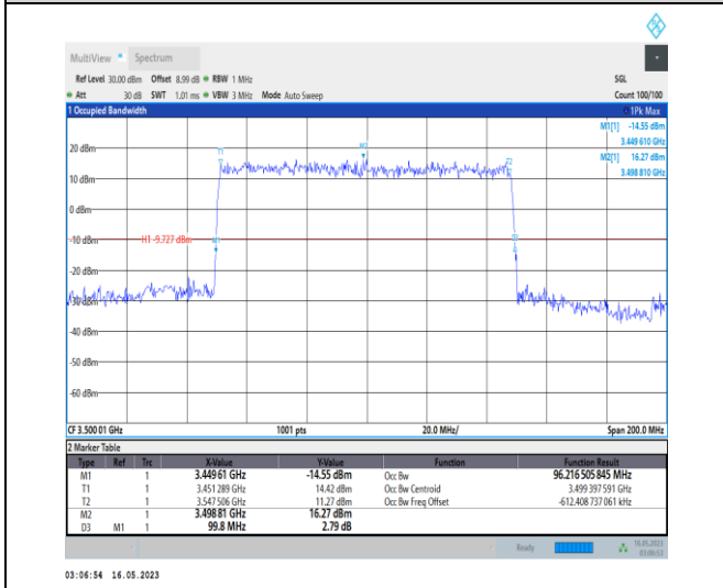
1-N78-3450-3550-PC1-30-100-L-1-DFT-QPSK-Outer_Full-270@0-Ant0-96.217-99.800-≤100-PASS
