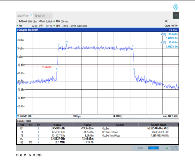
1-N78-3450-3550-PC1-30-70-L-3-DFT-16QAM-Outer_Full-180@0-Ant0-63.895-66.500-≤70-PASS
