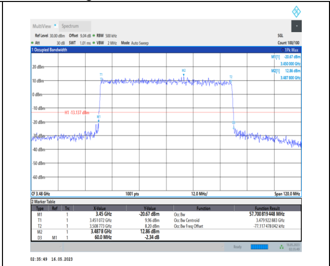
1-N78-3450-3550-PC1-30-60-L-8-CP-64QAM-Outer_Full-162@0-Ant0-57.701-60.000-≤60-PASS
