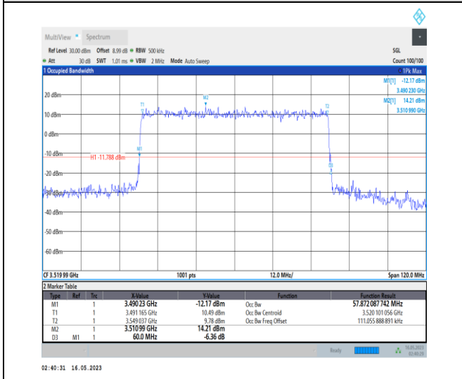
1-N78-3450-3550-PC1-30-60-H-3-DFT-16QAM-Outer_Full-162@0-Ant0-57.872-60.000-≤60-PASS
