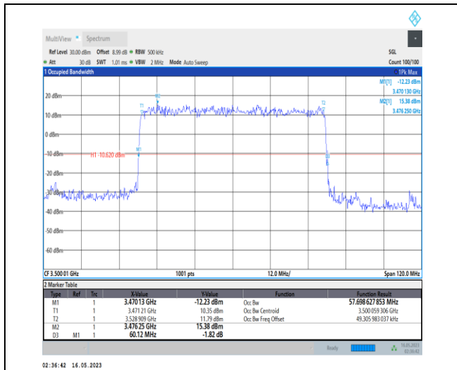
1-N78-3450-3550-PC1-30-60-M-2-DFT-PI2BPSK-Outer_Full-162@0-Ant0-57.699-60.120-≤60-PASS
