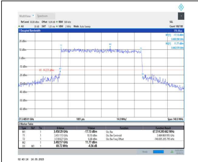
1-N78-3450-3550-PC1-30-70-L-8-CP-64QAM-Outer _Full-189@0-Ant0-67.514-69.720-≤70-PASS
