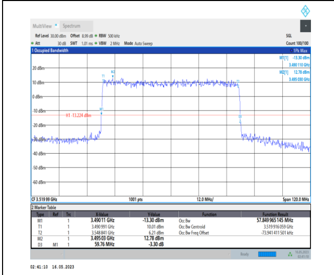
1-N78-3450-3550-PC1-30-60-H-7-CP-16QAM-Outer _Full-162@0-Ant0-57.85-59.760-≤60-PASS
