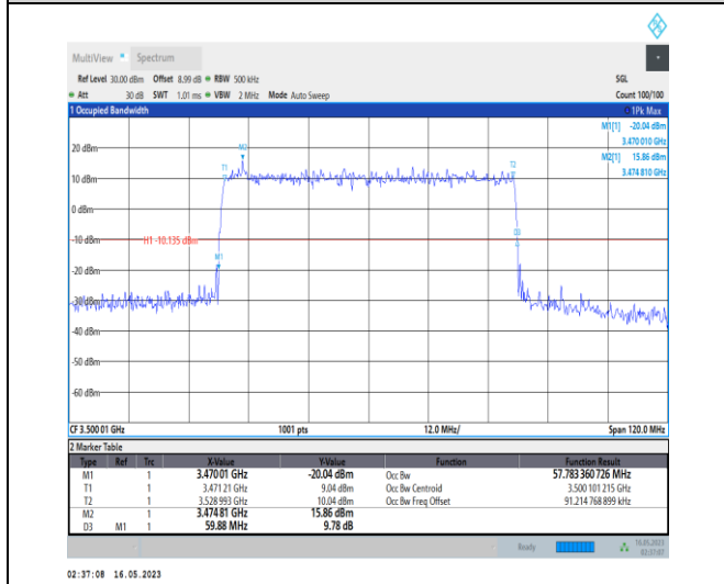
1-N78-3450-3550-PC1-30-60-M-4-DFT-64QAM-Outer_Full-162@0-Ant0-57.783-59.880-≤60-PASS
