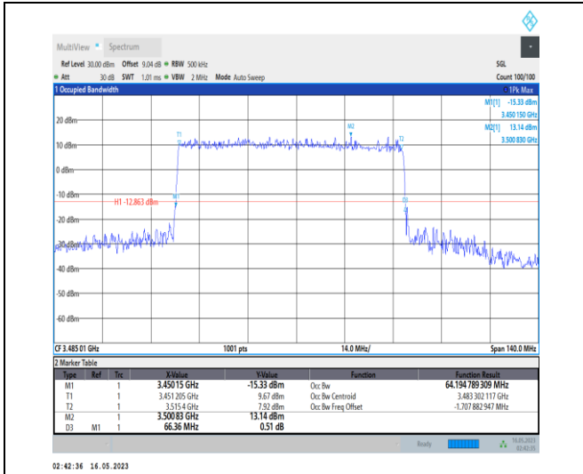
1-N78-3450-3550-PC1-30-70-L-4-DFT-64QAM-Outer_Full-180@0-Ant0-64.195-66.360-≤70-PASS
