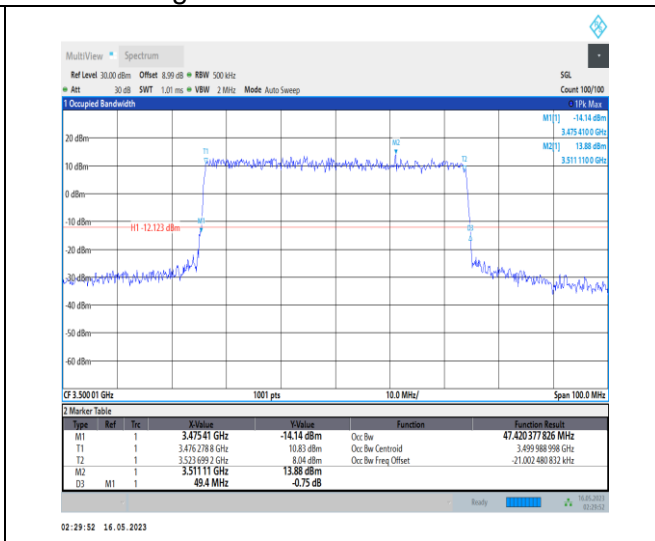
1-N78-3450-3550-PC1-30-50-M-6-CP-QPSK-Outer_Full-133@0-Ant0-47.42-49.400-≤50-PASS
