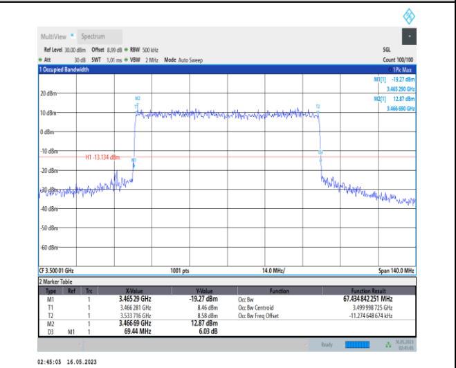
1-N78-3450-3550-PC1-30-70-M-6-CP-QPSK-Outer_Full-189@0-Ant0-67.435-69.440-≤70-PASS
