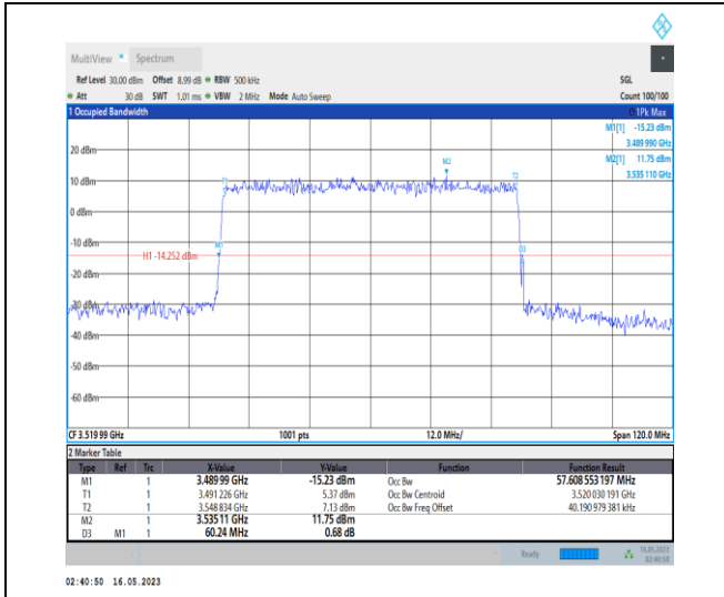
1-N78-3450-3550-PC1-30-60-H-5-DFT-256QAM-Out er_Full-162@0-Ant0-57.609-60.240-≤60-PASS
