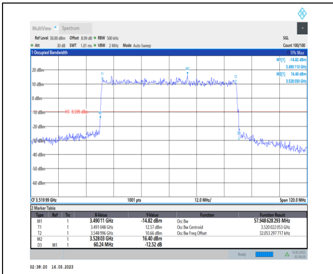
1-N78-3450-3550-PC1-30-60-H-1-DFT-QPSK-Outer_Full-162@0-Ant0-57.949-60.240-≤60-PASS
