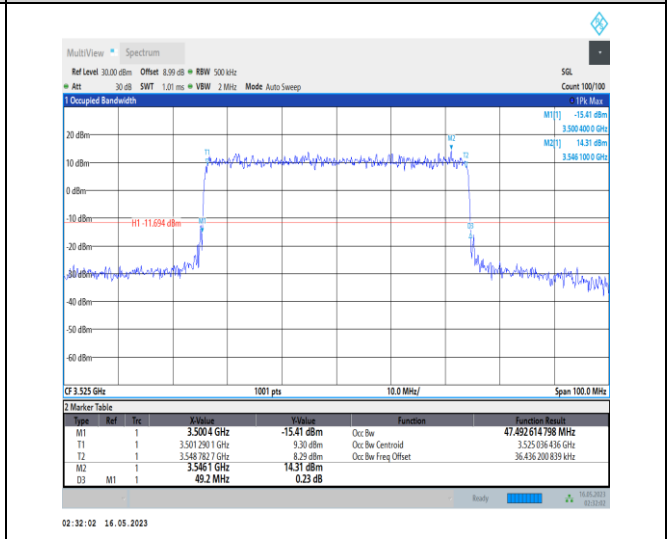
1-N78-3450-3550-PC1-30-50-H-7-CP-16QAM-Outer_Full-133@0-Ant0-47.493-49.200-≤50-PASS
