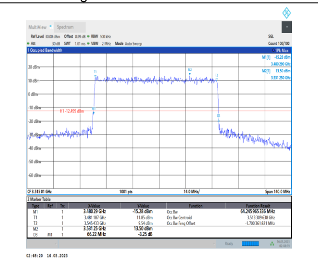
1-N78-3450-3550-PC1-30-70-H-3-DFT-16QAM-Outer_Full-180@0-Ant0-64.246-66.220-≤70-PASS
