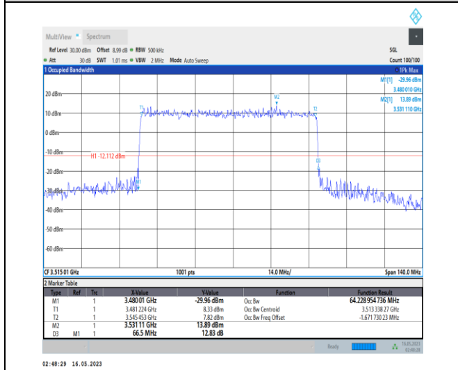
1-N78-3450-3550-PC1-30-70-H-4-DFT-64QAM-Outer_Full-180@0-Ant0-64.229-66.500-≤70-PASS
