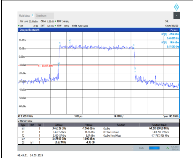
1-N78-3450-3550-PC1-30-70-M-1-DFT-QPSK-Outer _Full-180@0-Ant0-64.27-66.220-≤70-PASS
