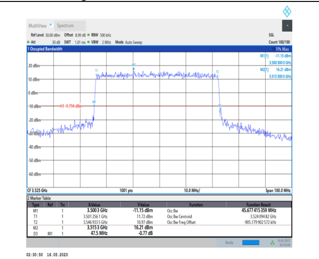
1-N78-3450-3550-PC1-30-50-H-1-DFT-QPSK-Outer _Full-128@0-Ant0-45.677-47.500-≤50-PASS
