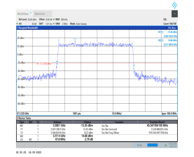
1-N78-3450-3550-PC1-30-50-H-3-DFT-16QAM-Outer _Full-128@0-Ant0-45.548-47.800-≤50-PASS
