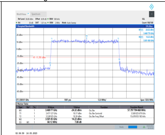
1-N78-3450-3550-PC1-30-60-M-3-DFT-16QAM-Outer_Full-162@0-Ant0-57.798-60.120-≤60-PASS
