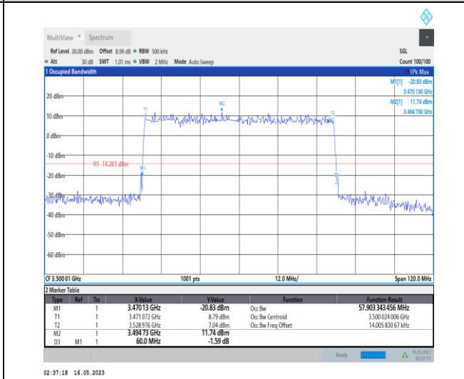
1-N78-3450-3550-PC1-30-60-M-5-DFT-256QAM-Outer_Full-162@0-Ant0-57.903-60.000-≤60-PASS
