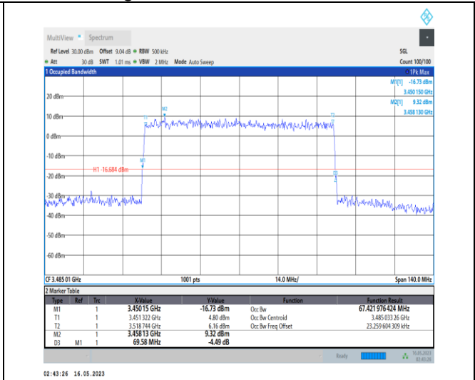
1-N78-3450-3550-PC1-30-70-L-9-CP-256QAM-Outer _Full-189@0-Ant0-67.422-69.580-≤70-PASS
