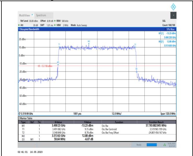
1-N78-3450-3550-PC1-30-60-H-6-CP-QPSK-Outer Full-162@0-Ant0-57.766-59.640-≤60-PASS
