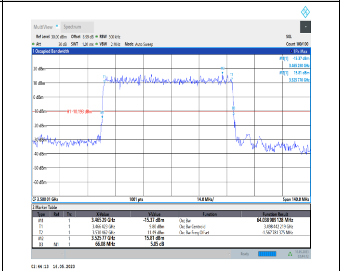
1-N78-3450-3550-PC1-30-70-M-2-DFT-PI2BPSK-Outer _Full-180@0-Ant0-64.039-66.080-≤70-PASS
