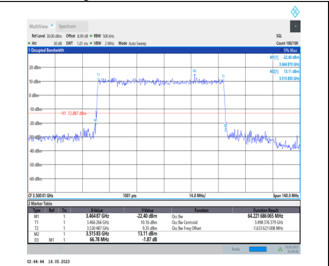
1-N78-3450-3550-PC1-30-70-M-4-DFT-64QAM-Out_r_Full-180@0-Ant0-64.222-66.780-≤70-PASS
