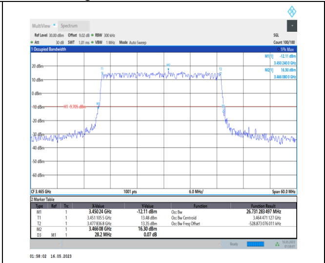
1-N78-3450-3550-PC1-30-30-L-1-DFT-QPSK-Outer_Full-75@0-Ant0-26.731-28.200-≤30-PASS
