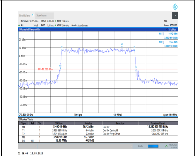
1-N78-3450-3550-PC1-30-20-M-9-CP-256QAM-Outer_Full-51 @ 0-Ant0-18.233-18.960-≤20-PASS
