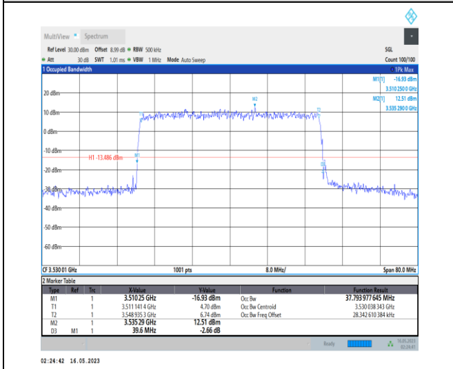
1-N78-3450-3550-PC1-30-40-H-9-CP-256QAM-Outer _Full-106@0-Ant0-37.794-39.600-≤40-PASS
