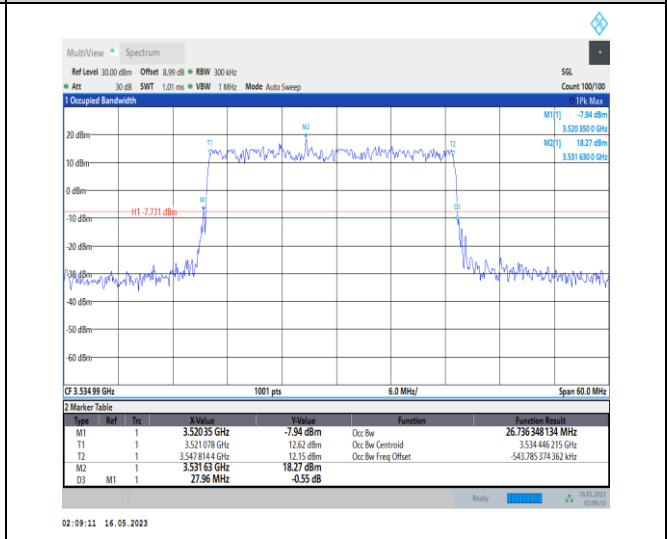
1-N78-3450-3550-PC1-30-30-H-1-DFT-QPSK-Outer_Full-75@0-Ant0-26.736-27.960-≤30-PASS
