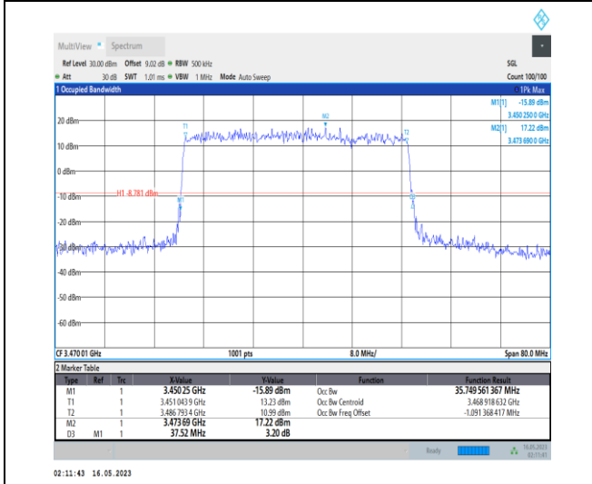
1-N78-3450-3550-PC1-30-40-L-3-DFT-16QAM-Outer_Full-100@0-Ant0-35.75-37.520-≤40-PASS
