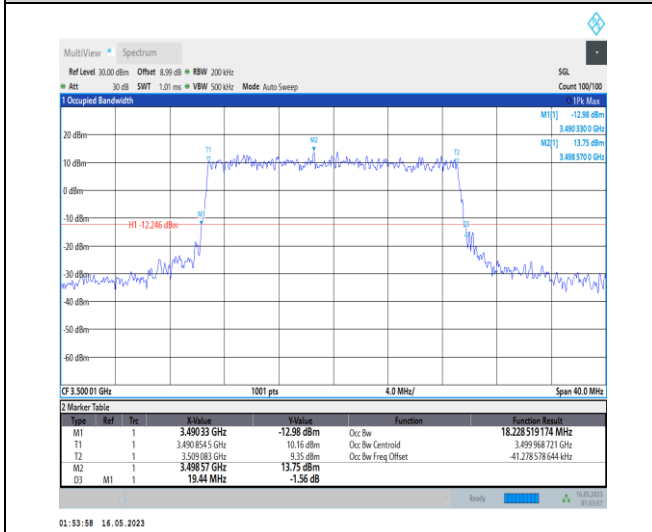
1-N78-3450-3550-PC1-30-20-M-8-CP-64QAM-Outer_Full-51 @ 0-Ant0-18.229-19.440-≤20-PASS
