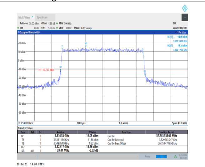
1-N78-3450-3550-PC1-30-40-H-8-CP-64QAM-Outer _Full-106@0-Ant0-37.743-39.440-≤40-PASS
