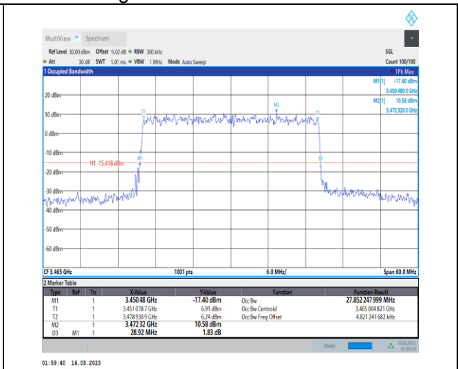
1-N78-3450-3550-PC1-30-30-L-9-CP-256QAM-Outer _Full-78@0-Ant0-27.852-28.920-≤30-PASS
