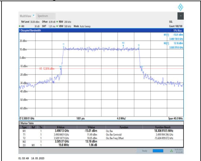
1-N78-3450-3550-PC1-30-20-M-7-CP-16QAM-Outer_Full-51 @ 0-Ant0-18.307-19.800-≤20-PASS
