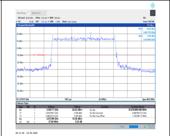
1-N78-3450-3550-PC1-30-40-L-4-DFT-64QAM-Outer_Full-100@0-Ant0-35.819-37.840-≤40-PASS
