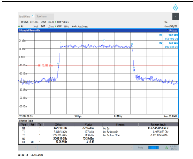
1-N78-3450-3550-PC1-30-40-M-4-DFT-64QAM-Out er_Full-100@0-Ant0-35.775-37.760-≤40-PASS
