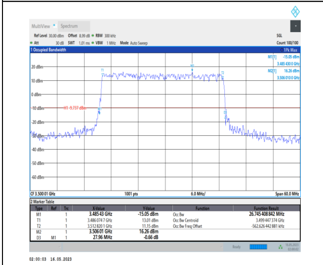
1-N78-3450-3550-PC1-30-30-M-1-DFT-QPSK-Outer _Full-75@0-Ant0-26.745-27.960-≤30-PASS
