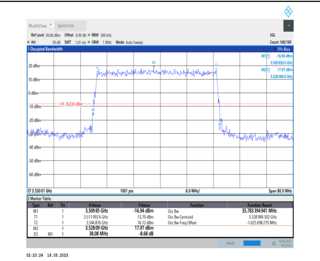
1-N78-3450-3550-PC1-30-40-H-2-DFT-PI2BPSK-Outer_Full-100@0-Ant0-35.783-38.080-≤40-PASS
