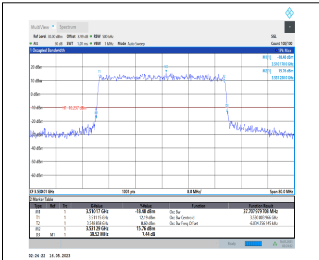
1-N78-3450-3550-PC1-30-40-H-7-CP-16QAM-Outer _Full-106@0-Ant0-37.708-39.520-≤40-PASS
