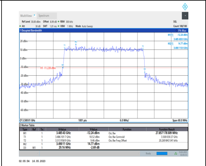
1-N78-3450-3550-PC1-30-30-M-6-CP-QPSK-Out er_Full-78@0-Ant0-27.857-29.160-≤30-PASS
