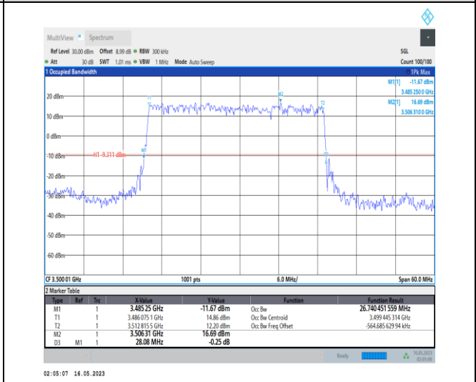
1-N78-3450-3550-PC1-30-30-M-2-DFT-PI2BPSK-Outer _Full-75@0-Ant0-26.74-28.080-≤30-PASS
