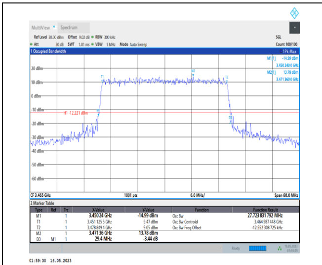
1-N78-3450-3550-PC1-30-30-L-8-CP-64QAM-Outer _Full-78@0-Ant0-27.724-29.400-≤30-PASS
