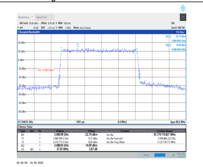
1-N78-3450-3550-PC1-30-40-M-5-DFT-256QAM-Out er_Full-100@0-Ant0-35.774-37.920-≤40-PASS
