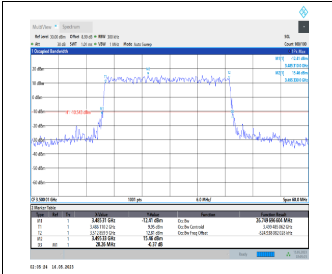
1-N78-3450-3550-PC1-30-30-M-3-DFT-16QAM-Out er_Full-75@0-Ant0-26.75-28.260-≤30-PASS
