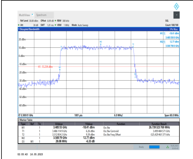
1-N78-3450-3550-PC1-30-30-M-5-DFT-256QAM-Out er_Full-75@0-Ant0-26.739-28.080-≤30-PASS
