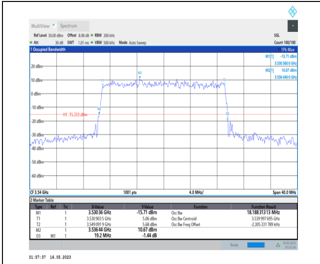
1-N78-3450-3550-PC1-30-20-H-9-CP-256QAM-Outer_Full-51@0-Ant0-18.188-19.200-≤20-PASS
