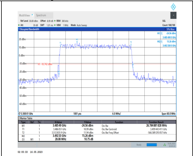
1-N78-3450-3550-PC1-30-30-M-4-DFT-64QAM-Out er_Full-75@0-Ant0-26.785-28.080-≤30-PASS
