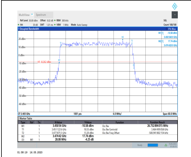
1-N78-3450-3550-PC1-30-30-L-2-DFT-PI2BPSK-Outer_Full-75@0-Ant0-26.753-28.080-≤30-PASS
