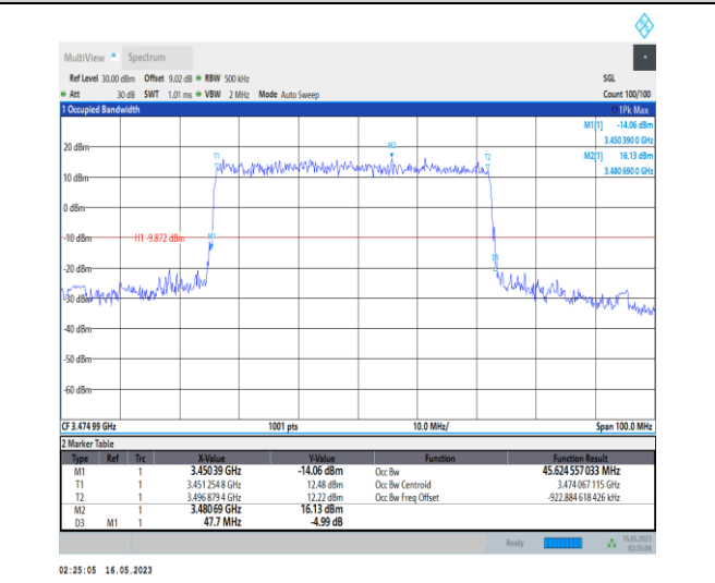
1-N78-3450-3550-PC1-30-50-L-1-DFT-QPSK-Outer Full-128@0-Ant0-45.625-47.700-≤50-PASS
