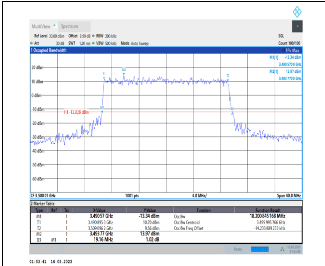
1-N78-3450-3550-PC1-30-20-M-6-CP-QPSK-Outer_Full-51 @ 0-Ant0-18.201-19.160-≤20-PASS
