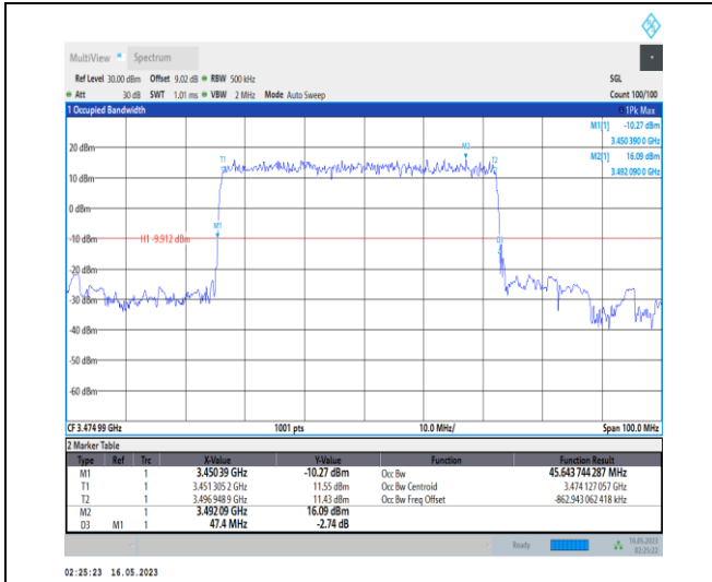
1-N78-3450-3550-PC1-30-50-L-2-DFT-PI2BPSK-Out er_Full-128@0-Ant0-45.644-47.400-≤50-PASS
