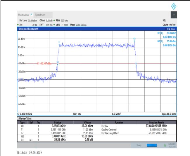
1-N78-3450-3550-PC1-30-40-L-7-CP-16QAM-Outer_Full-106@0-Ant0-37.685-39.360-≤40-PASS
