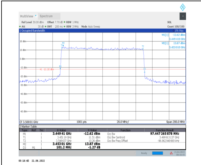
1-N78-3450-3550--30-100-M-6-CP-QPSK-Outer_Full -273@0-Ant0-97.447-101.200-≤100-PASS
