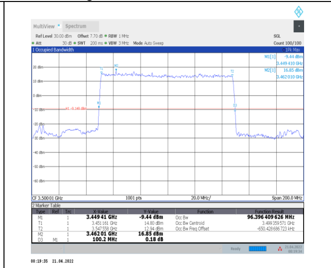
1-N78-3450-3550--30-100-H-2-DFT-PI2BPSK-Outer_Full-270@0-Ant0-96.396-100.200-≤100-PASS
