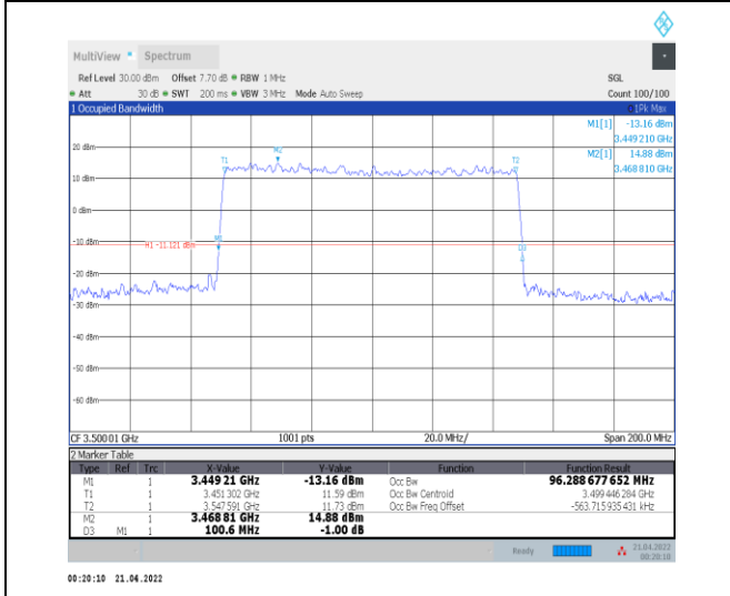
1-N78-3450-3550--30-100-H-3-DFT-16QAM-Outer_Full-270@0-Ant0-96.289-100.600-≤100-PASS
