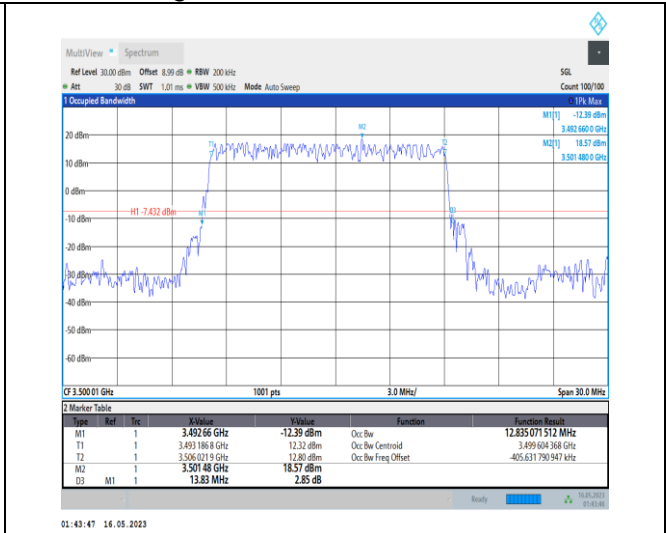
1-N78-3450-3550-PC1-30-15-M-2-DFT-PI2BPSK-Outer_Full-36@0-Ant0-12.835-13.830-≤15-PASS
