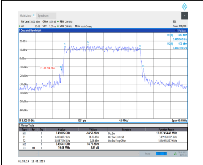
1-N78-3450-3550-PC1-30-20-M-4-DFT-64QAM-Outer_Full-50@0-Ant0-17.867-19.480-≤20-PASS
