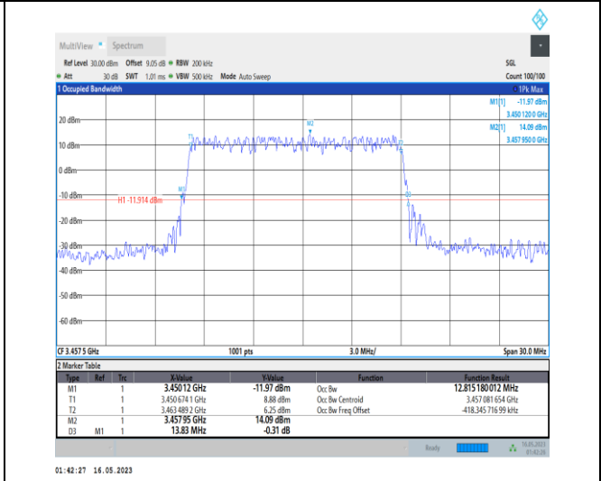
1-N78-3450-3550-PC1-30-15-L-5-DFT-256QAM-Outer_Full-36@0-Ant0-12.815-13.830-≤15-PASS
