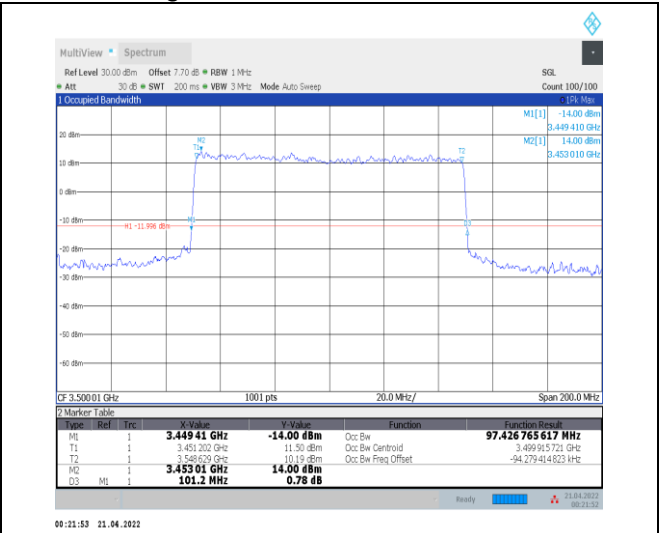
1-N78-3450-3550--30-100-H-6-CP-QPSK-Outer_Full-273@0-Ant0-97.427-101.200-≤100-PASS
