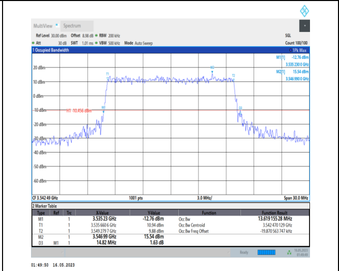
1-N78-3450-3550-PC1-30-15-H-7-CP-16QAM-Outer_Full-38@0-Ant0-13.619-14.820-≤15-PASS
