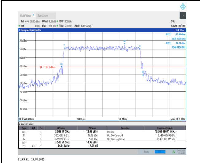
1-N78-3450-3550-PC1-30-15-H-6-CP-QPSK-Outer_Full-38@0-Ant0-13.566-14.640-≤15-PASS
