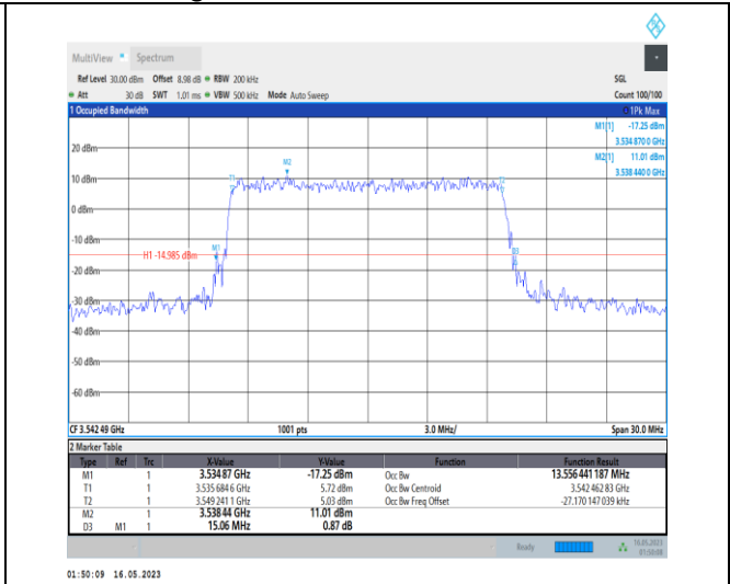
1-N78-3450-3550-PC1-30-15-H-9-CP-256QAM-Outer_Full-38@0-Ant0-13.556-15.060-≤15-PASS
