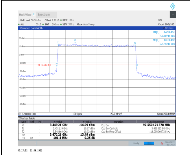
1-N78-3450-3550--30-100-M-8-CP-64QAM-Outer_Full -273@0-Ant0-97.55-101.400-≤100-PASS
