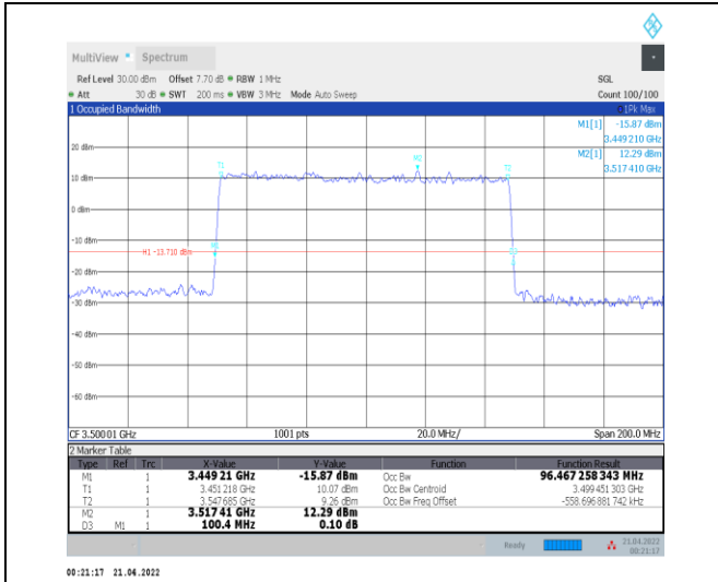
1-N78-3450-3550--30-100-H-5-DFT-256QAM-Outer_Full-270@0-Ant0-96.467-100.400-≤100-PASS
