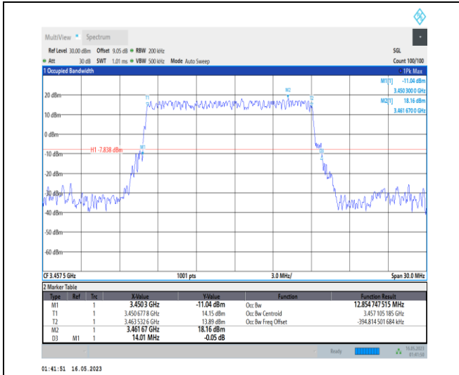
1-N78-3450-3550-PC1-30-15-L-2-DFT-PI2BPSK-Out er_Full-36@0-Ant0-12.855-14.010-≤15-PASS
