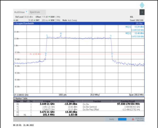
1-N78-3450-3550--30-100-H-8-CP-64QAM-Outer_Full-273@0-Ant0-97.55-101.400-≤100-PASS
