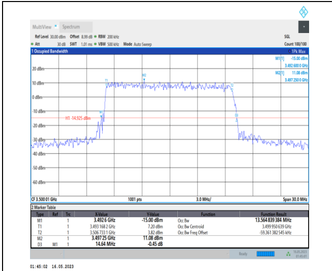
1-N78-3450-3550-PC1-30-15-M-9-CP-256QAM-Out er_Full-38@0-Ant0-13.565-14.640-≤15-PASS
