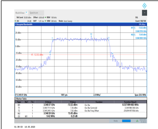
1-N78-3450-3550-PC1-30-10-H-7-CP-16QAM-Outer_Full-24@0-Ant0-8.538-9.420-≤10-PASS
