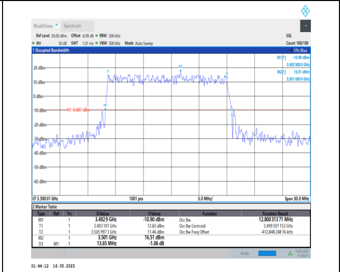
1-N78-3450-3550-PC1-30-15-M-4-DFT-64QAM-Outer_Full-36@0-Ant0-12.8-13.650-≤15-PASS
