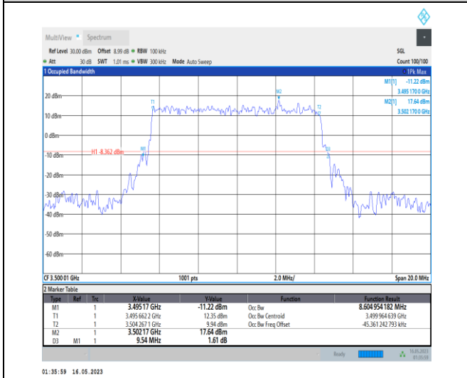
1-N78-3450-3550-PC1-30-10-M-2-DFT-PI2BPSK-Outer_Full-24@0-Ant0-8.605-9.540-≤10-PASS
