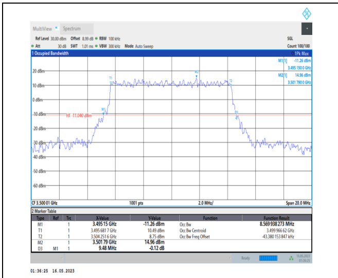
1-N78-3450-3550-PC1-30-10-M-4-DFT-64QAM-Out er_Full-24@0-Ant0-8.57-9.480-≤10-PASS
