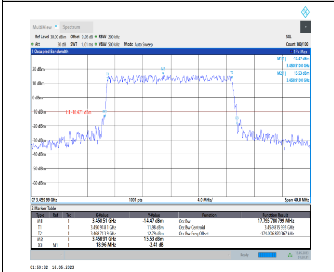
1-N78-3450-3550-PC1-30-20-L-1-DFT-QPSK-Outer_Full-50@0-Ant0-17.796-18.960-≤20-PASS
