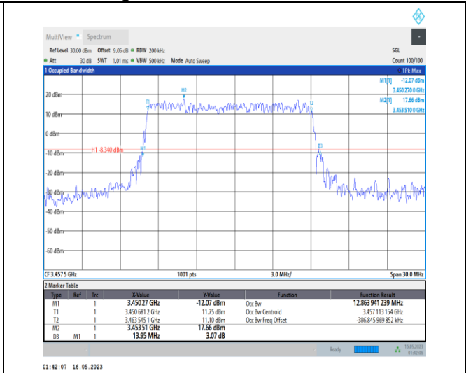
1-N78-3450-3550-PC1-30-15-L-3-DFT-16QAM-Outer_Full-36@0-Ant0-12.864-13.950-≤15-PASS
