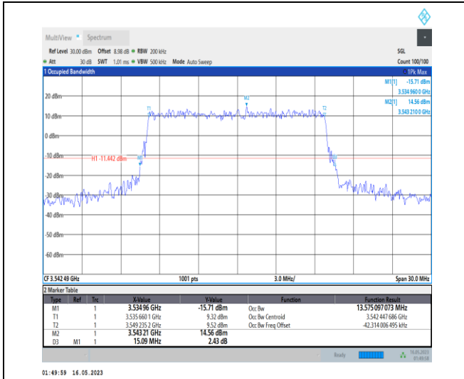
1-N78-3450-3550-PC1-30-15-H-8-CP-64QAM-Outer_Full-38@0-Ant0-13.575-15.090-≤15-PASS
