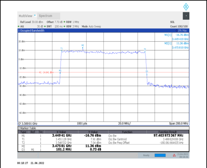
1-N78-3450-3550--30-100-M-9-CP-256QAM-Outer_Full -273@0-Ant0-97.404-101.200-≤100-PASS
