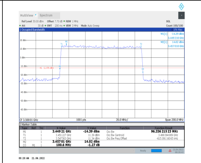
1-N78-3450-3550--30-100-H-4-DFT-64QAM-Outer_Full-270@0-Ant0-96.336-100.600-≤100-PASS
