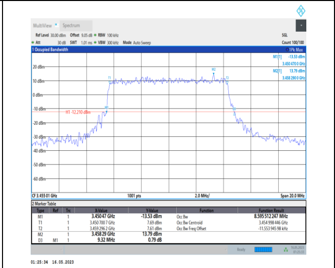
1-N78-3450-3550-PC1-30-10-L-8-CP-64QAM-Outer_Full-24@0-Ant0-8.596-9.320-≤10-PASS
