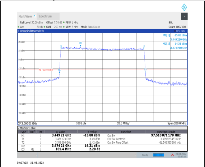
1-N78-3450-3550--30-100-M-7-CP-16QAM-Outer_Full -273@0-Ant0-97.511-101.400-≤100-PASS
