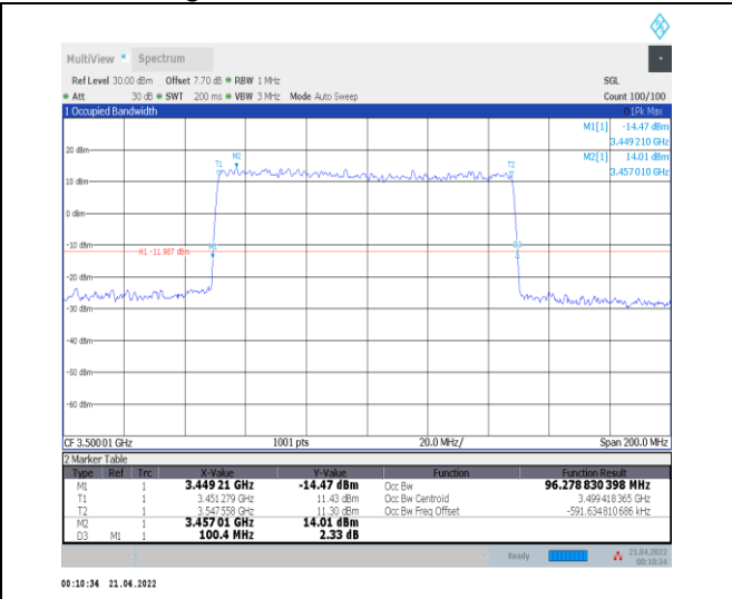
1-N78-3450-3550--30-100-L-4-DFT-64QAM-Outer_F ull-270@0-Ant0-96.279-100.400-≤100-PASS
