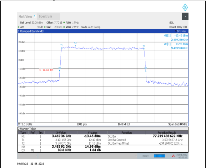
1-N78-3450-3550--30-80-H-4-DFT-64QAM-Outer_Fu II-216@0-Ant0-77.219-80.800-<math>\leq 80</math>-PASS
