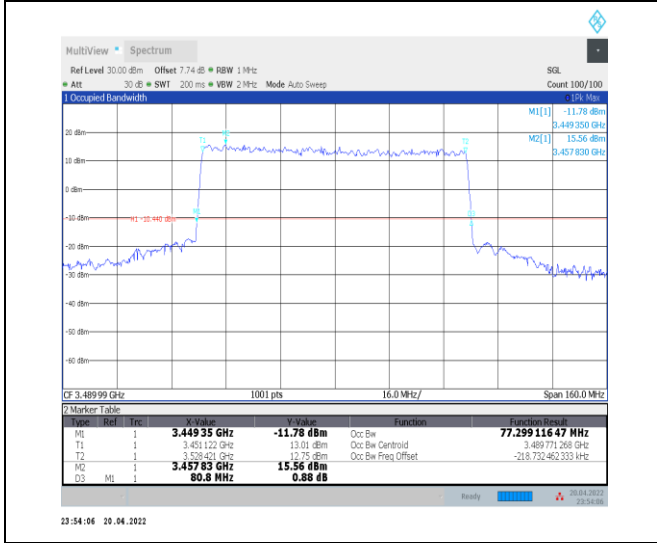
1-N78-3450-3550--30-80-L-3-DFT-16QAM-Outer_Full-216@0-Ant0-77.299-80.800-≤80-PASS
