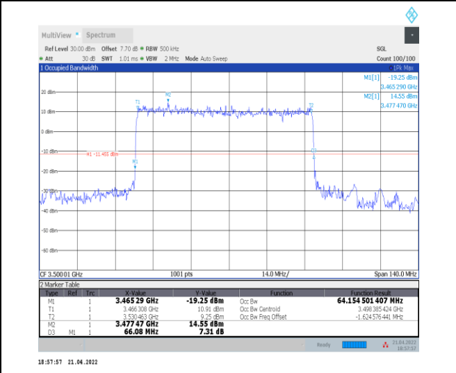
1-N78-3450-3550--30-70-M-2-DFT-PI2BPSK-Outer_Full Full-180@0-Ant0-64.155-66.080-≤70-PASS
