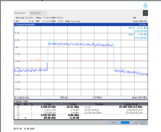
1-N78-3450-3550--30-70-L-9-CP-256QAM-Outer_Fu ll-189@0-Ant0-67.487-69.580-≤70-PASS
