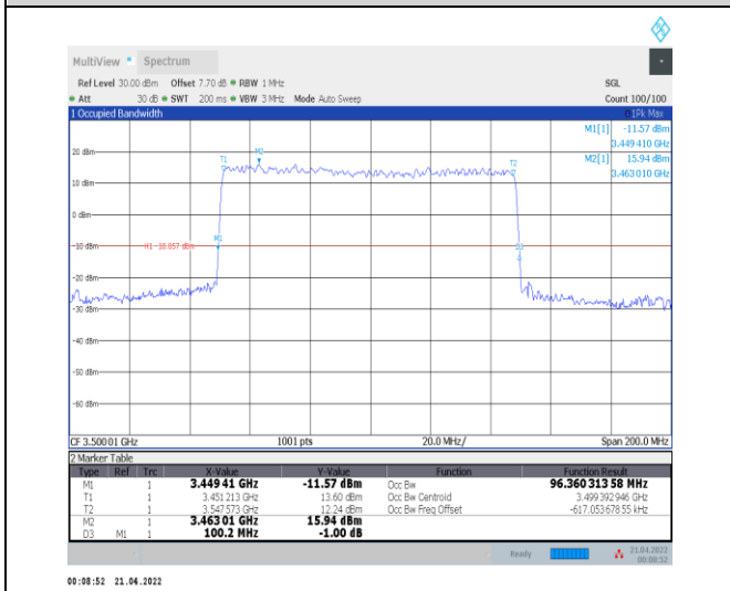
1-N78-3450-3550--30-100-L-1-DFT-QPSK-Outer_Full I-270@0-Ant0-96.36-100.200-≤100-PASS
