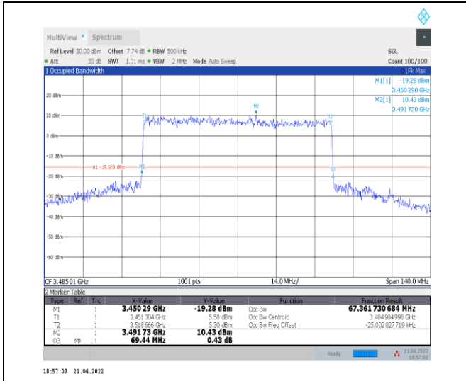
1-N78-3450-3550--30-70-L-8-CP-64QAM-Outer_Full -189@0-Ant0-67.362-69.440-≤70-PASS
