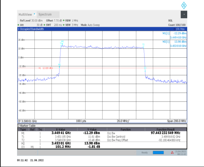
1-N78-3450-3550--30-100-L-6-CP-QPSK-Outer_F ull-273@0-Ant0-97.443-101.200-≤100-PASS
