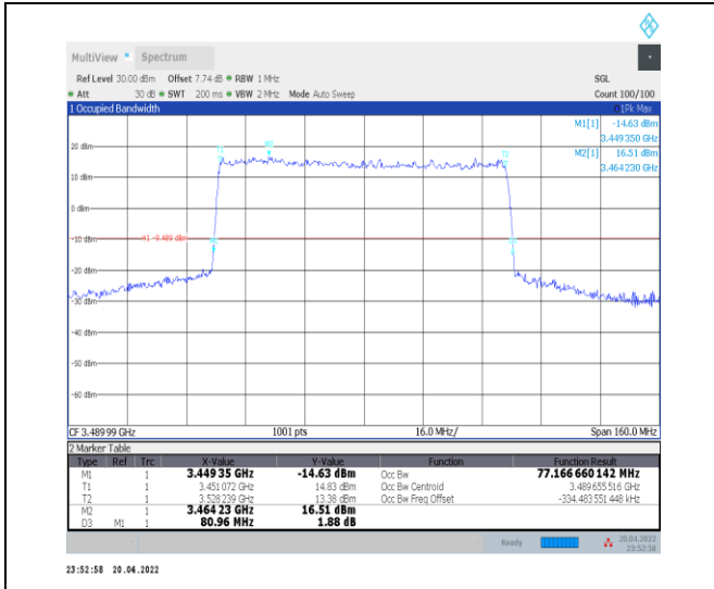
1-N78-3450-3550--30-80-L-1-DFT-QPSK-Outer_Full-216@0-Ant0-77.167-80.960-≤80-PASS
