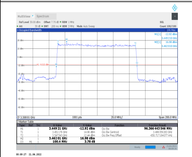
1-N78-3450-3550--30-100-L-2-DFT-P12BPSK-Outer_Full Full-270@0-Ant0-96.366-100.400-≤100-PASS
