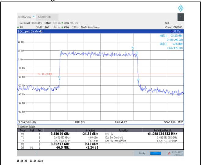
1-N78-3450-3550--30-70-L-5-DFT-256QAM-Outer_Full-180@0-Ant0-64.088-66.500-≤70-PASS
