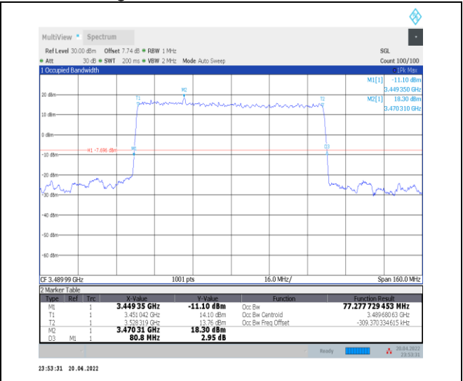
1-N78-3450-3550--30-80-L-2-DFT-PI2BPSK-Outer_Full-216@0-Ant0-77.278-80.800-≤80-PASS
