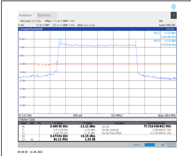
1-N78-3450-3550--30-80-H-7-CP-16QAM-Outer_Full -217@0-Ant0-77.716-81.120-≤80-PASS
