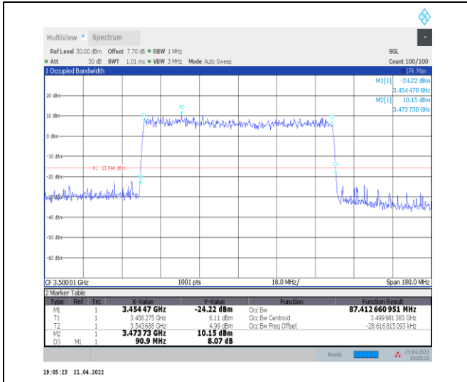
1-N78-3450-3550--30-90-M-9-CP-256QAM-Outer_Full-245@0-Ant0-87.413-90.900-<=90-PASS
