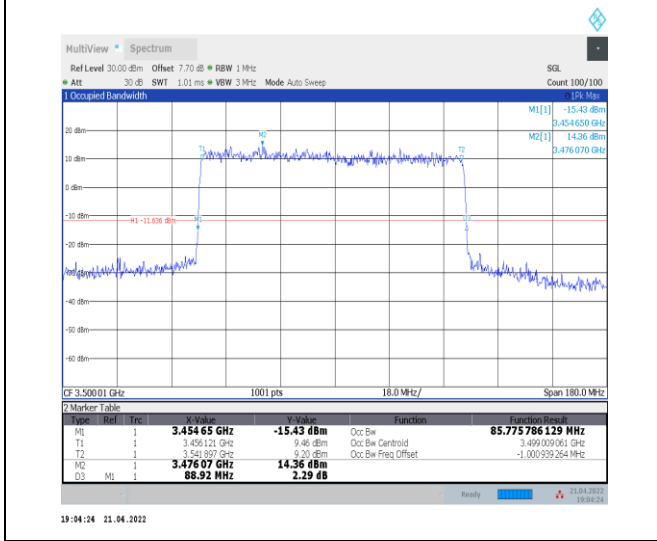
1-N78-3450-3550--30-90-M-3-DFT-16QAM-Outer_Full -240@0-Ant0-85.776-88.920-≤90-PASS
