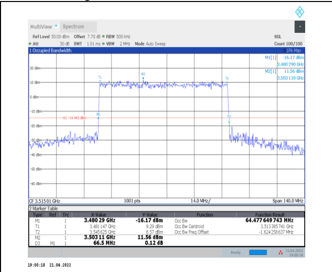
1-N78-3450-3550--30-70-H-3-DFT-16QAM-Outer_Full-180@0-Ant0-64.478-66.500-≤70-PASS
