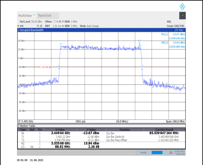
1-N78-3450-3550--30-90-L-1-DFT-QPSK-Outer_Full- 240@0-Ant0-85.54-88.920-≤90-PASS
