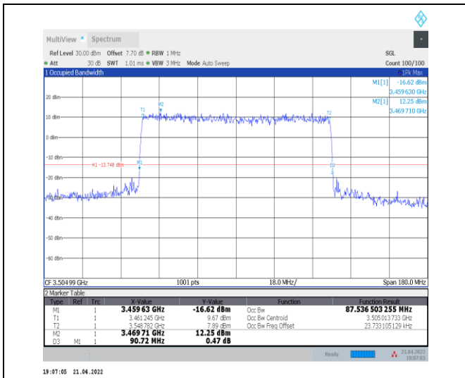
1-N78-3450-3550--30-90-H-8-CP-64QAM-Outer_Full -245@0-Ant0-87.537-90.720-≤90-PASS
