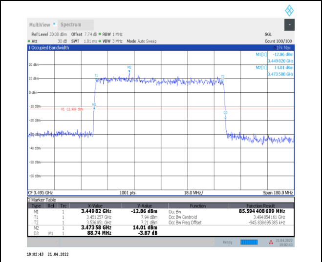
1-N78-3450-3550--30-90-L-5-DFT-256QAM-Outer_Full-240@0-Ant0-85.594-88.740-<=90-PASS
