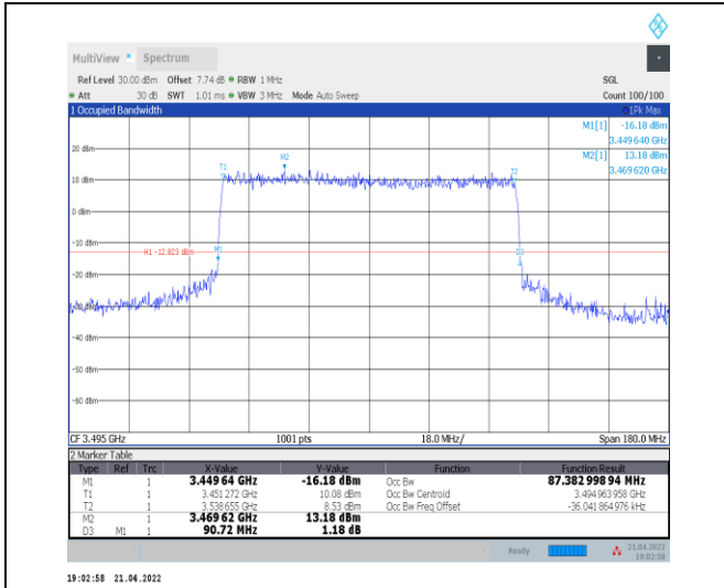
1-N78-3450-3550--30-90-L-6-CP-QPSK-Outer_Full-2 45@0-Ant0-87.383-90.720<=90-PASS
