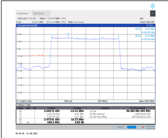
1-N78-3450-3550--30-100-M-2-DFT-PI2BPSK-Outer_Full-270@0-Ant0-96.385-100.400-≤100-PASS
