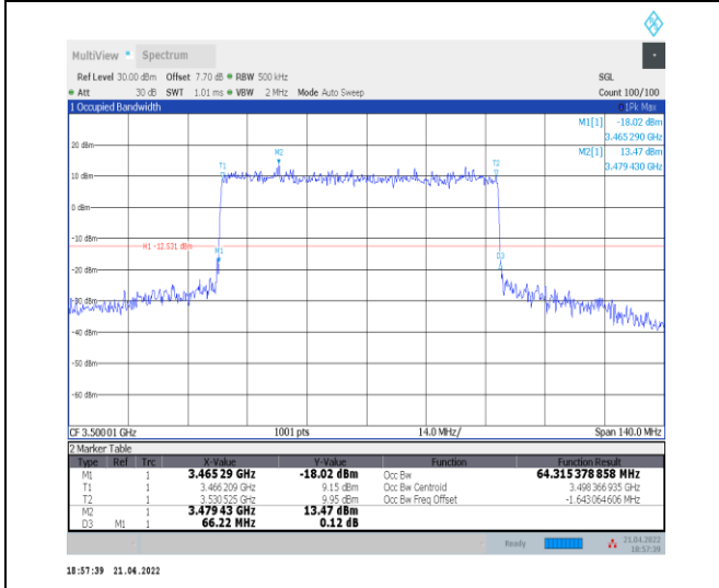
1-N78-3450-3550--30-70-M-1-DFT-QPSK-Outer_Full -180@0-Ant0-64.315-66.220-≤70-PASS
