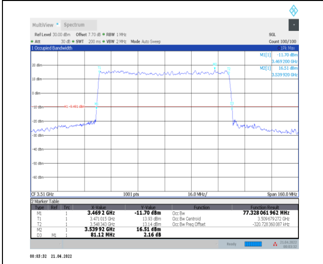
1-N78-3450-3550--30-80-H-1-DFT-QPSK-Outer_Full -216@0-Ant0-77.328-81.120-≤80-PASS
