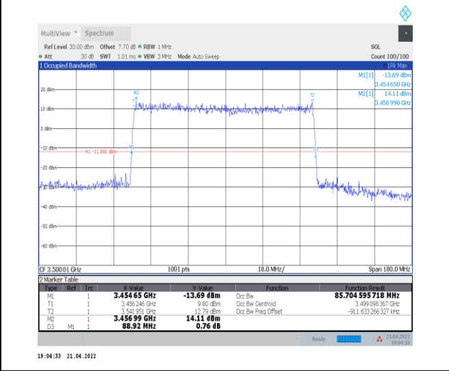
1-N78-3450-3550--30-90-M-4-DFT-64QAM-Outer_Full -240@0-Ant0-85.705-88.920-≤90-PASS
