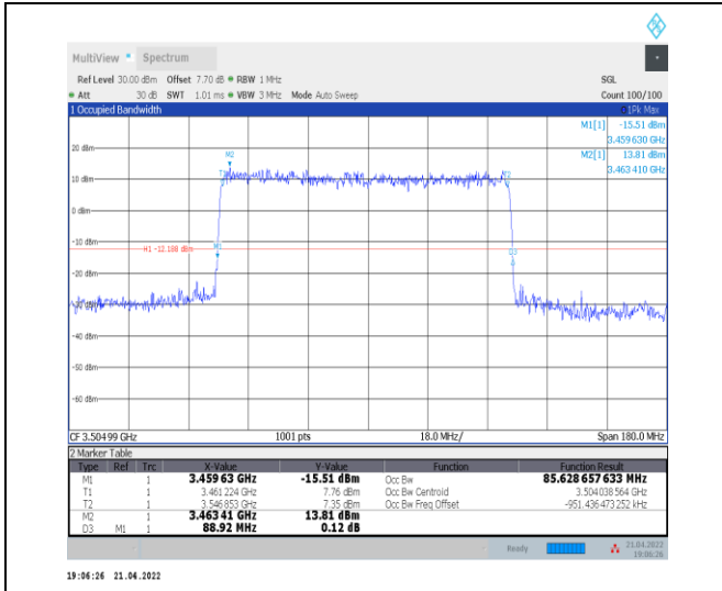
1-N78-3450-3550--30-90-H-4-DFT-64QAM-Outer_Fu II-240@0-Ant0-85.629-88.920-≤90-PASS
