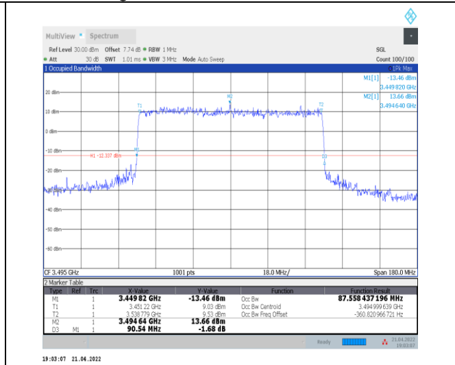
1-N78-3450-3550--30-90-L-7-CP-16QAM-Outer_Full -245@0-Ant0-87.558-90.540<=90-PASS
