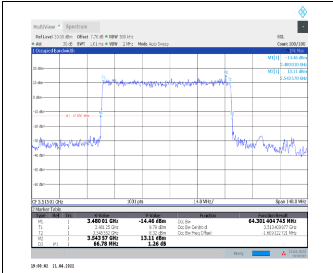
1-N78-3450-3550--30-70-H-2-DFT-PI2BPSK-Outer_Full-180@0-Ant0-64.301-66.780-≤70-PASS
