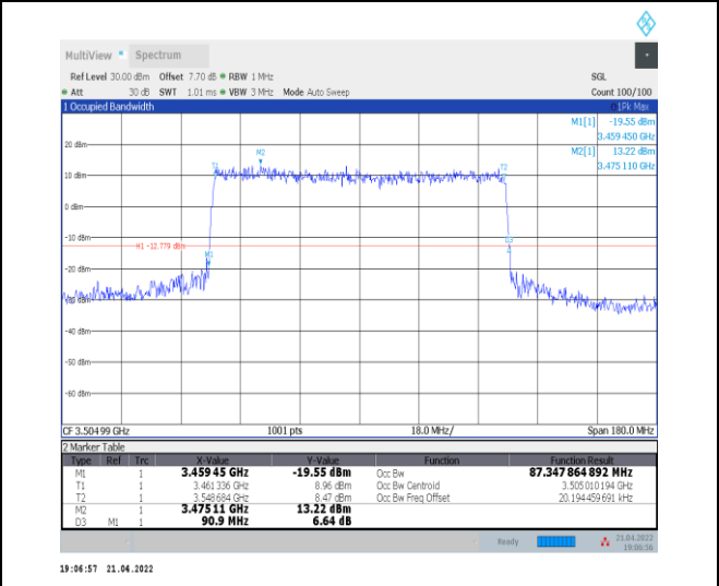
1-N78-3450-3550--30-90-H-7-CP-16QAM-Outer_Full-245@0-Ant0-87.348-90.900-≤90-PASS
