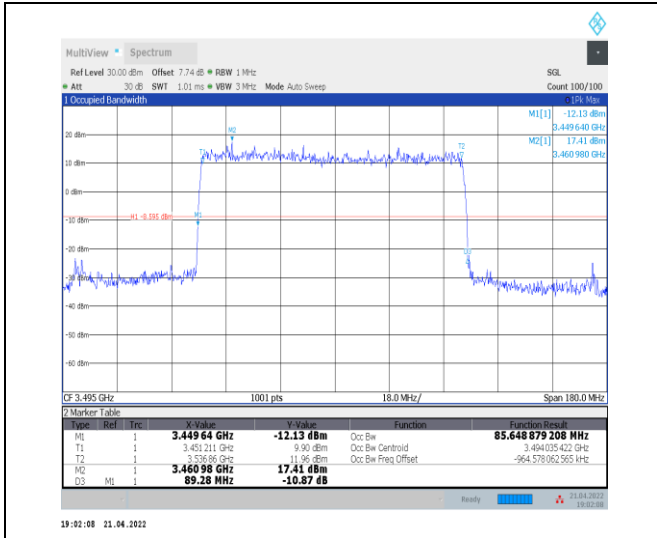
1-N78-3450-3550--30-90-L-2-DFT-PI2BPSK-Outer_Full-240@0-Ant0-85.649-89.280-<=90-PASS
