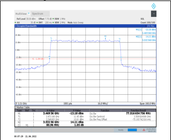
1-N78-3450-3550--30-80-H-8-CP-64QAM-Outer_Full -217@0-Ant0-77.517-80.960-≤80-PASS
