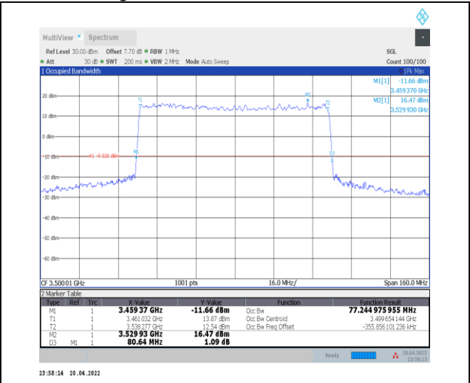
1-N78-3450-3550--30-80-M-1-DFT-QPSK-Outer_Full -216@0-Ant0-77.245-80.640≤80-PASS
