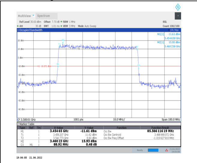
1-N78-3450-3550--30-90-M-2-DFT-PI2BPSK-Outer_Full -240@0-Ant0-85.566-88.920-≤90-PASS
