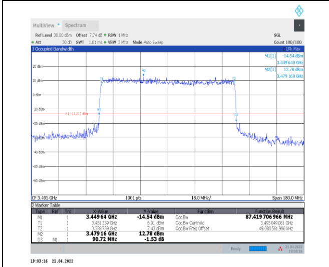
1-N78-3450-3550--30-90-L-8-CP-64QAM-Outer_Full -245@0-Ant0-87.42-90.720<=90-PASS
