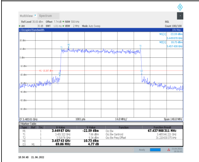
1-N78-3450-3550--30-70-L-6-CP-QPSK-Outer_Full-189@0-Ant0-67.438-69.860-≤70-PASS
