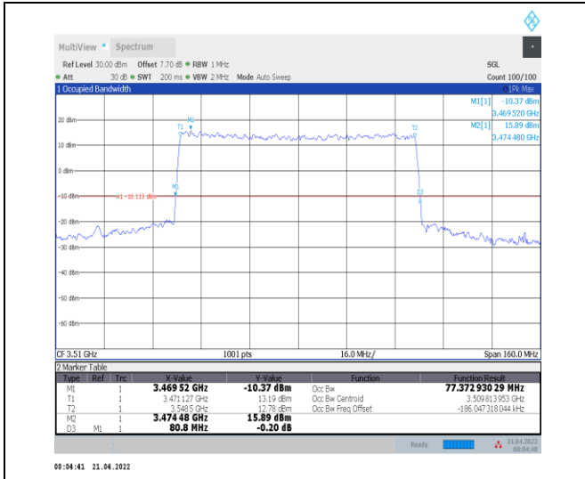
1-N78-3450-3550--30-80-H-3-DFT-16QAM-Outer_Fu II-216@0-Ant0-77.373-80.800-<math>\leq 80</math>-PASS
