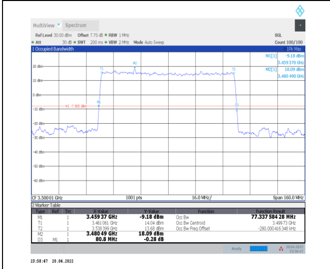
1-N78-3450-3550--30-80-M-2-DFT-PI2BPSK-Outer_Full Full-216@0-Ant0-77.338-80.800≤80-PASS
