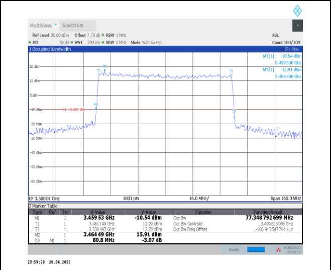
1-N78-3450-3550--30-80-M-3-DFT-16QAM-Outer_Full ull-216@0-Ant0-77.349-80.800≤80-PASS
