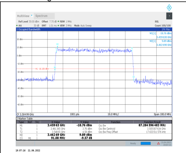
1-N78-3450-3550--30-90-H-9-CP-256QAM-Outer_Full -245@0-Ant0-87.285-91.080-≤90-PASS
