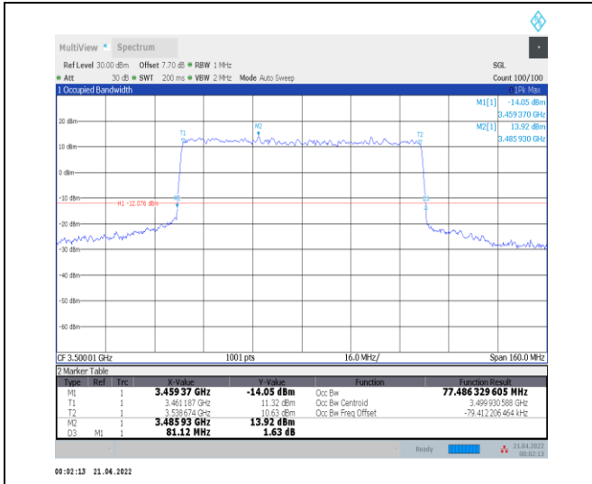
1-N78-3450-3550--30-80-M-8-CP-64QAM-Outer_Full -217@0-Ant0-77.486-81.120-≤80-PASS
