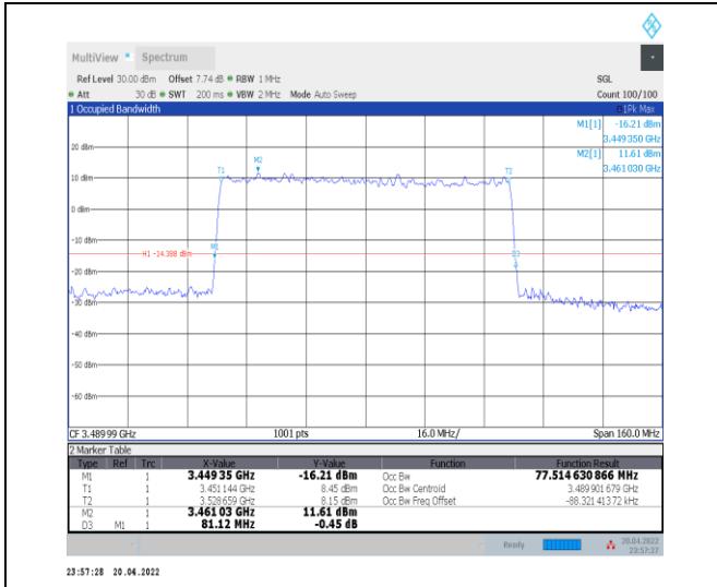
1-N78-3450-3550--30-80-L-9-CP-256QAM-Outer_Full ll-217@0-Ant0-77.515-81.120≤80-PASS
