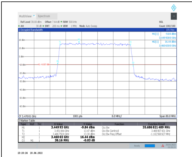
1-N78-3450-3550--30-40-L-1-DFT-QPSK-Outer_Full-100@0-Ant0-35.687-38.160-≤40-PASS
