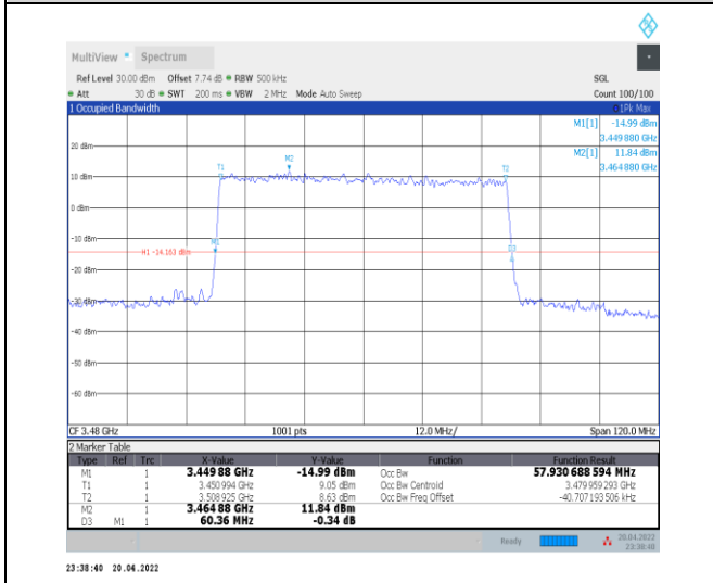
1-N78-3450-3550--30-60-L-5-DFT-256QAM-Outer_Full-162@0-Ant0-57.931-60.360-≤60-PASS
