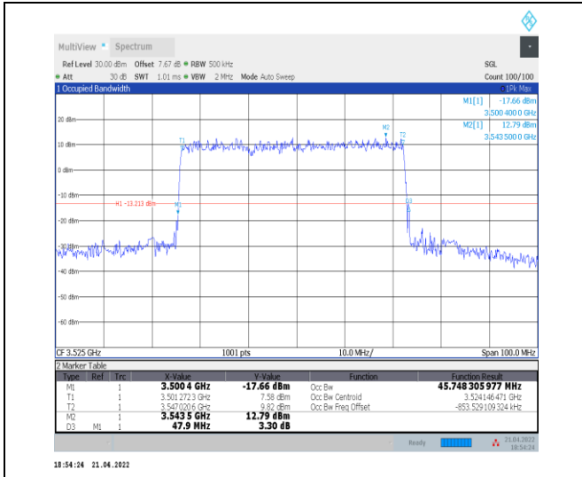
1-N78-3450-3550--30-50-H-4-DFT-64QAM-Outer_Fu II-128@0-Ant0-45.748-47.900-≤50-PASS
