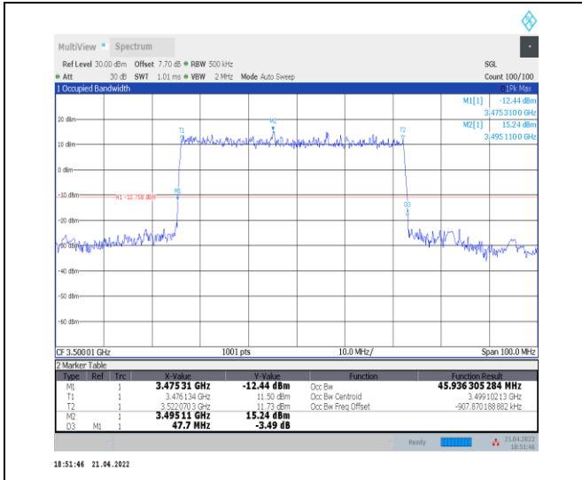
1-N78-3450-3550--30-50-M-1-DFT-QPSK-Outer_Full -128@0-Ant0-45.936-47.700-≤50-PASS
