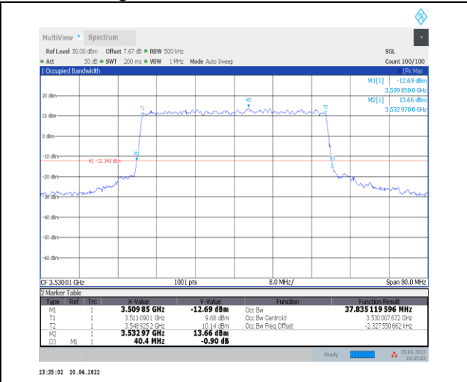
1-N78-3450-3550--30-40-H-8-CP-64QAM-Outer_Full -106@0-Ant0-37.835-40.400-≤40-PASS
