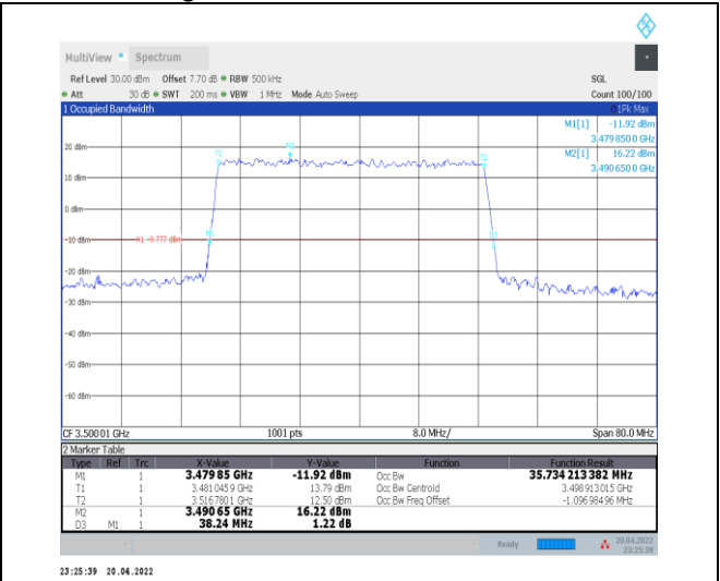
1-N78-3450-3550--30-40-M-1-DFT-QPSK-Outer_Full -100@0-Ant0-35.734-38.240-≤40-PASS
