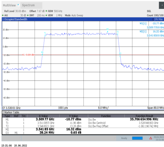
1-N78-3450-3550--30-40-H-1-DFT-QPSK-Outer_Full -100@0-Ant0-35.707-38.240-<math>\leq 40</math>-PASS
