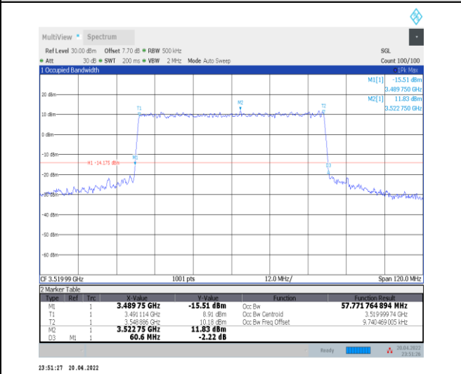
1-N78-3450-3550--30-60-H-8-CP-64QAM-Outer_Full-162@0-Ant0-57.772-60.600-≤60-PASS
