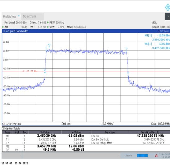
1-N78-3450-3550--30-50-L-6-CP-QPSK-Outer_Full-1 33@0-Ant0-47.358-49.200≤50-PASS
