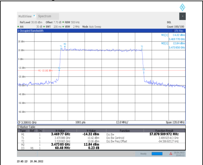
1-N78-3450-3550--30-60-M-7-CP-16QAM-Outer_Full-162@0-Ant0-57.879-60.480-<math>\leq 60</math>-PASS
