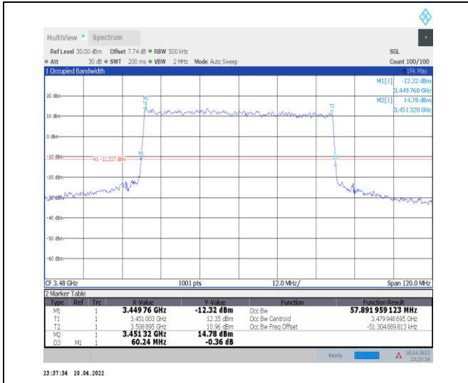
1-N78-3450-3550--30-60-L-3-DFT-16QAM-Outer_Full-162@0-Ant0-57.892-60.240-≤60-PASS
