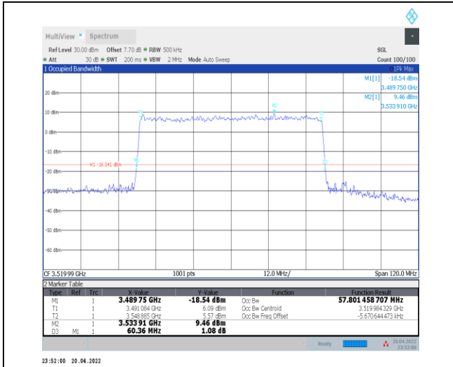
1-N78-3450-3550--30-60-H-9-CP-256QAM-Outer_Fu II-162@0-Ant0-57.801-60.360-≤60-PASS
