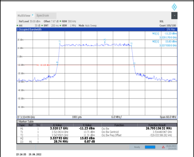
1-N78-3450-3550--30-30-H-1-DFT-QPSK-Outer_Full -75@0-Ant0-26.795-28.740-≤30-PASS
