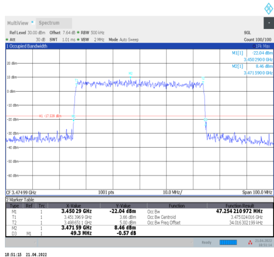
1-N78-3450-3550--30-50-L-9-CP-256QAM-Outer_Fu ll-133@0-Ant0-47.254-49.300≤50-PASS
