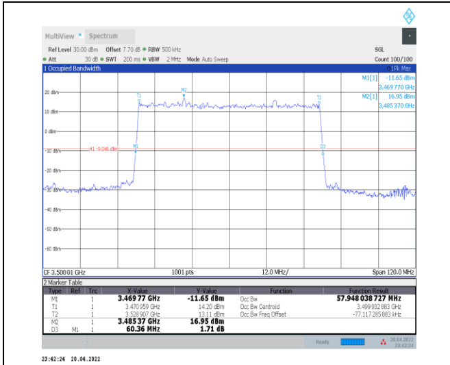
1-N78-3450-3550--30-60-M-2-DFT-PI2BPSK-Outer_Full-162@0-Ant0-57.948-60.360-≤60-PASS
