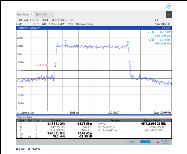
1-N78-3450-3550--30-50-M-4-DFT-64QAM-Outer_Full -128@0-Ant0-45.719-48.100-≤50-PASS
