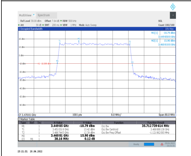
1-N78-3450-3550--30-40-L-3-DFT-16QAM-Outer_Ful-I-100@0-Ant0-35.713-38.160-≤40-PASS
