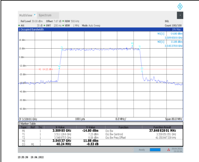
1-N78-3450-3550--30-40-H-9-CP-256QAM-Outer_Fu ll-106@0-Ant0-37.849-40.240-≤40-PASS
