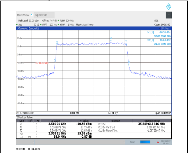
1-N78-3450-3550--30-40-H-4-DFT-64QAM-Outer_Fu II-100@0-Ant0-35.85-38.000-≤40-PASS
