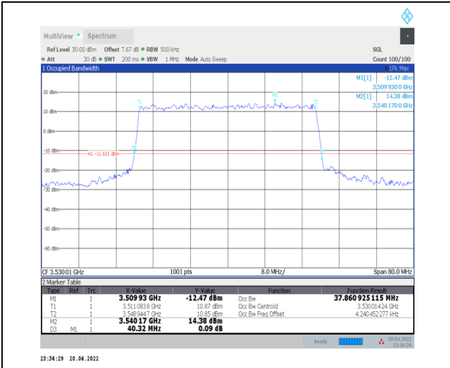
1-N78-3450-3550--30-40-H-7-CP-16QAM-Outer_Full -106@0-Ant0-37.861-40.320-≤40-PASS
