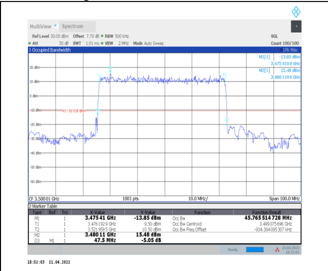
1-N78-3450-3550--30-50-M-2-DFT-PI2BPSK-Outer_Full -128@0-Ant0-45.766-47.500-≤50-PASS
