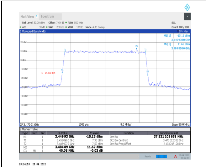
1-N78-3450-3550--30-40-L-9-CP-256QAM-Outer_Fu II-106@0-Ant0-37.831-40.080-≤40-PASS
