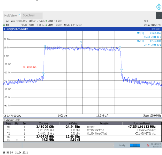
1-N78-3450-3550--30-50-L-7-CP-16QAM-Outer_Full -133@0-Ant0-47.354-49.300≤50-PASS
