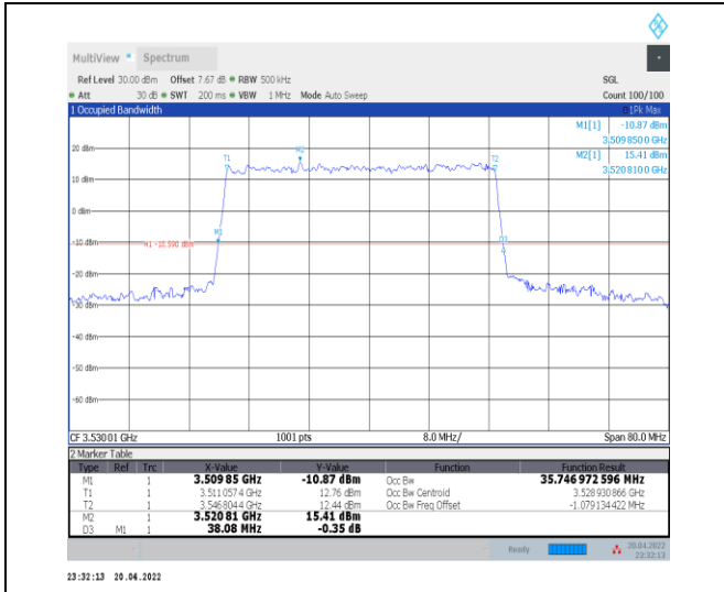
1-N78-3450-3550--30-40-H-3-DFT-16QAM-Outer_Fu II-100@0-Ant0-35.747-38.080-≤40-PASS
