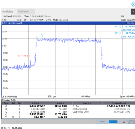
1-N78-3450-3550--30-50-L-8-CP-64QAM-Outer_Full -133@0-Ant0-47.418-49.800≤50-PASS
