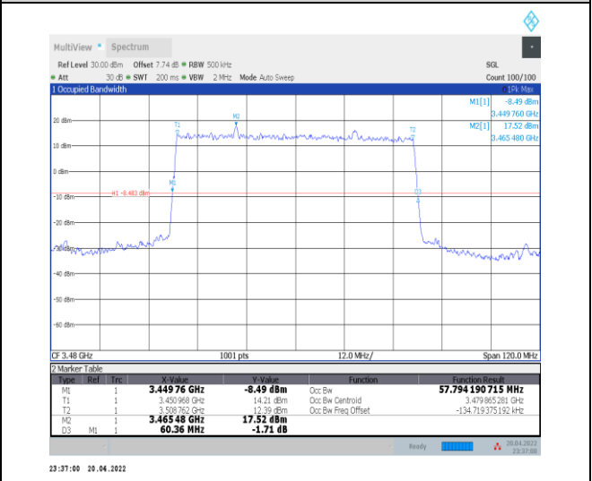
1-N78-3450-3550--30-60-L-2-DFT-PI2BPSK-Outer_Full -162@0-Ant0-57.794-60.360-≤60-PASS
