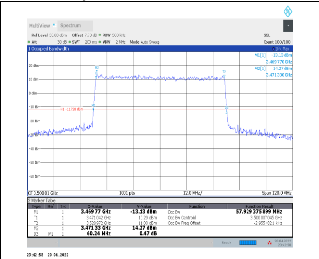
1-N78-3450-3550--30-60-M-3-DFT-16QAM-Outer_Full-162@0-Ant0-57.929-60.240-≤60-PASS
