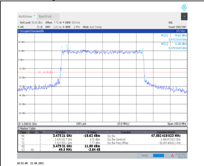
1-N78-3450-3550--30-50-M-6-CP-QPSK-Outer_Full-133@0-Ant0-47.582-49.500-≤50-PASS
