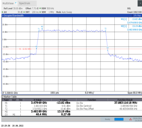
1-N78-3450-3550--30-40-M-8-CP-64QAM-Outer_Full -106@0-Ant0-37.883-40.400-<math>\leq 40</math>-PASS
