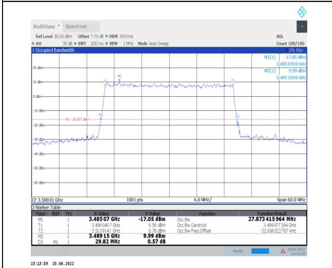
1-N78-3450-3550--30-30-M-9-CP-256QAM-Outer_F ull-78@0-Ant0-27.873-29.820-≤30-PASS
