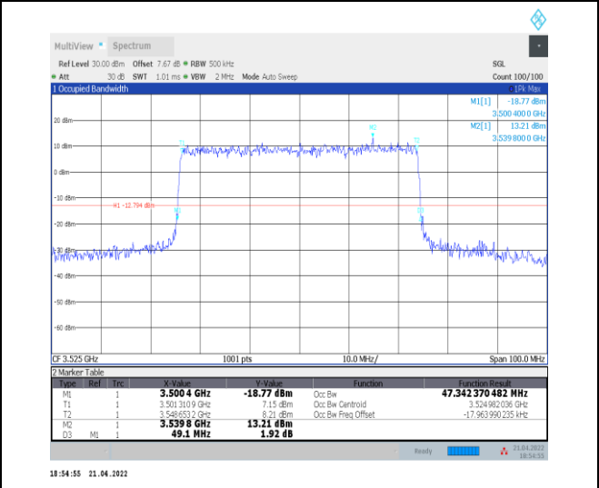
1-N78-3450-3550--30-50-H-7-CP-16QAM-Outer_Full-133@0-Ant0-47.342-49.100-≤50-PASS
