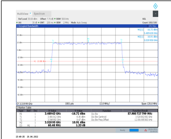
1-N78-3450-3550--30-60-H-5-DFT-256QAM-Outer_Full-162@0-Ant0-57.981-60.480-≤60-PASS
