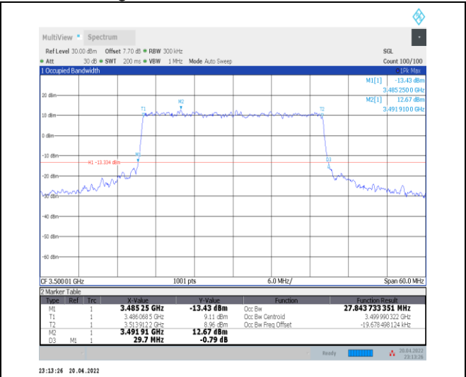
1-N78-3450-3550--30-30-M-8-CP-64QAM-Outer_Ful I-78@0-Ant0-27.844-29.700-≤30-PASS
