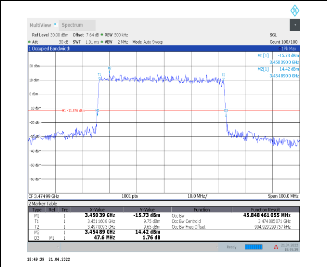
1-N78-3450-3550--30-50-L-1-DFT-QPSK-Outer_Full- 128@0-Ant0-45.848-47.600-≤50-PASS
