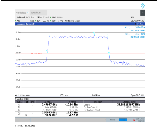
1-N78-3450-3550--30-40-M-4-DFT-64QAM-Outer_Full-100@0-Ant0-35.888-38.240-<math>\leq 40</math>-PASS
