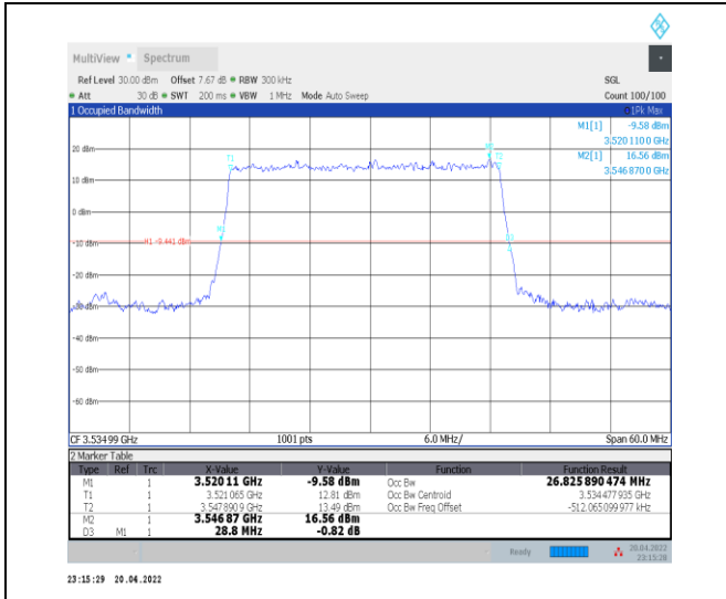
1-N78-3450-3550--30-30-H-2-DFT-PI2BPSK-Outer_Full-75@0-Ant0-26.826-28.800-≤30-PASS
