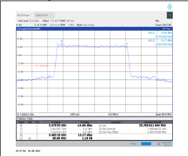
1-N78-3450-3550--30-40-M-5-DFT-256QAM-Outer_Full-100@0-Ant0-35.761-38.080-<math>\leq 40</math>-PASS
