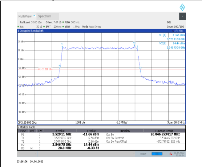
1-N78-3450-3550--30-30-H-3-DFT-16QAM-Outer_Fu II-75@0-Ant0-26.847-28.800-≤30-PASS
