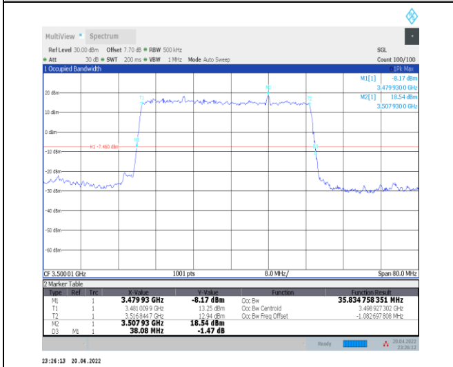
1-N78-3450-3550--30-40-M-2-DFT-PI2BPSK-Outer_Full-100@0-Ant0-35.835-38.080-≤40-PASS
