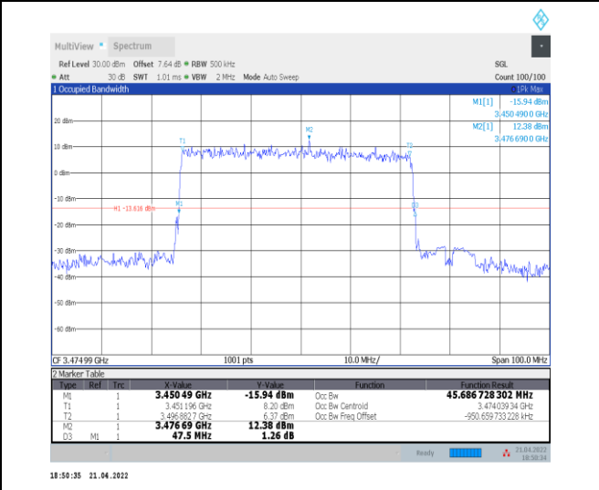
1-N78-3450-3550--30-50-L-5-DFT-256QAM-Outer_F ull-128@0-Ant0-45.687-47.500-≤50-PASS
