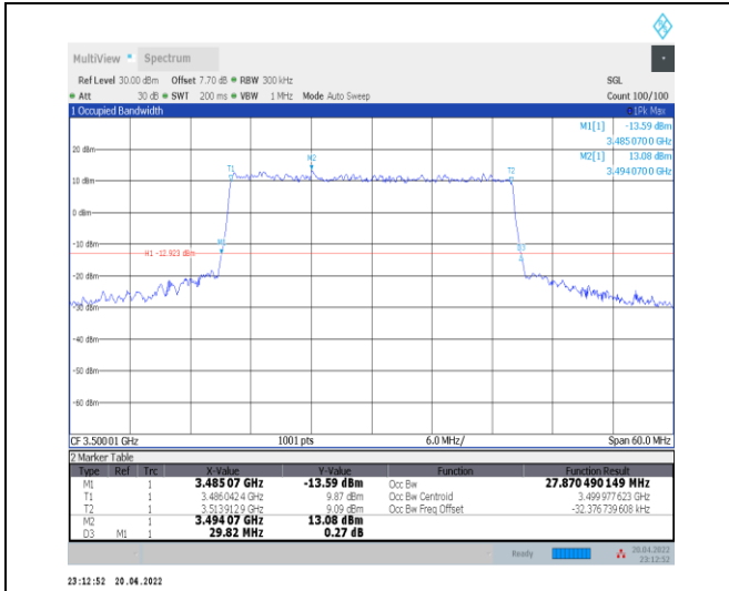
1-N78-3450-3550--30-30-M-7-CP-16QAM-Outer_Full -78@0-Ant0-27.87-29.820-≤30-PASS
