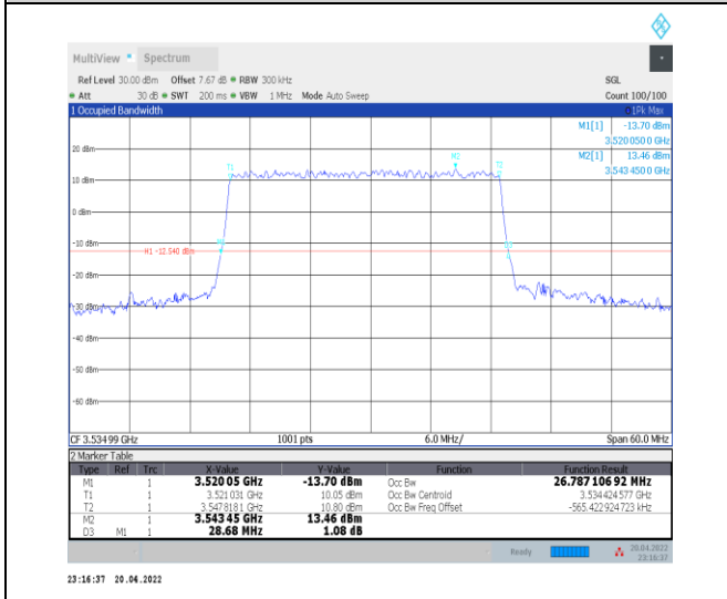
1-N78-3450-3550--30-30-H-4-DFT-64QAM-Outer_Fu II-75@0-Ant0-26.787-28.680-≤30-PASS
