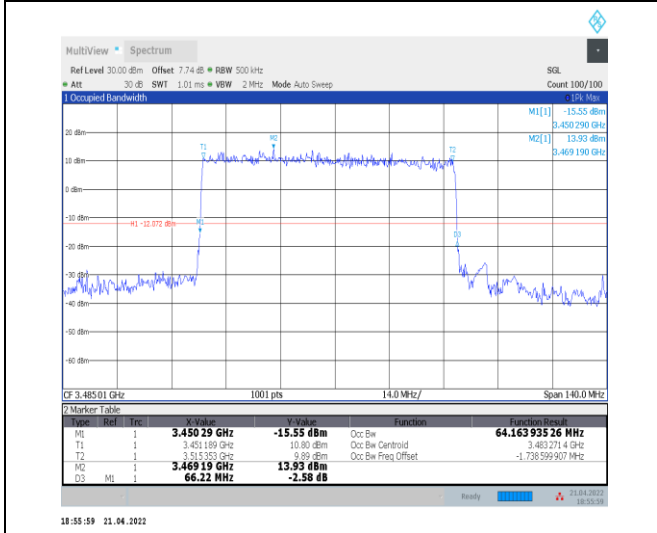
1-N78-3450-3550--30-70-L-2-DFT-PI2BPSK-Outer_Full-180@0-Ant0-64.164-66.220-≤70-PASS
