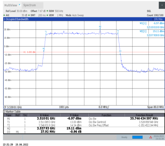
1-N78-3450-3550--30-40-H-2-DFT-PI2BPSK-Outer_Full-100@0-Ant0-35.746-37.920-<math>\leq 40</math>-PASS
