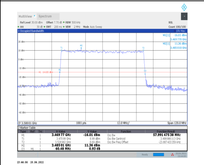
1-N78-3450-3550--30-60-M-5-DFT-256QAM-Outer_Full-162@0-Ant0-57.991-60.480-≤60-PASS
