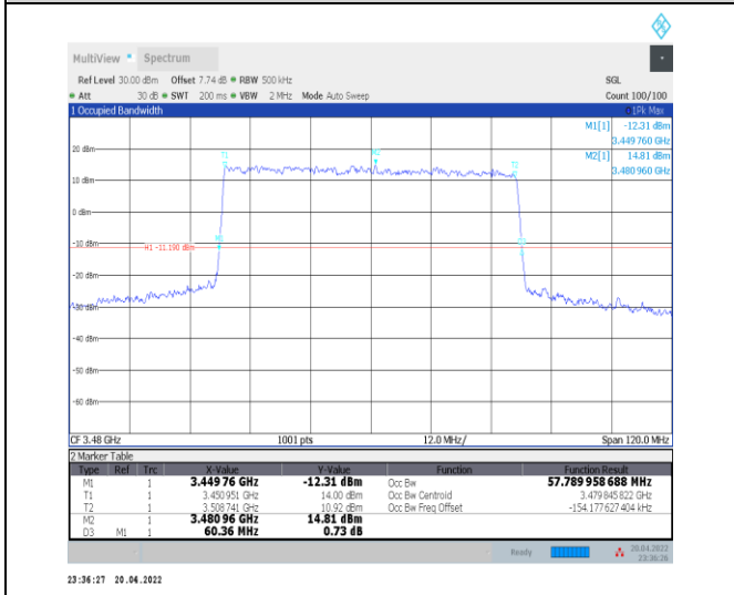
1-N78-3450-3550--30-60-L-1-DFT-QPSK-Outer_Full -162@0-Ant0-57.79-60.360-≤60-PASS
