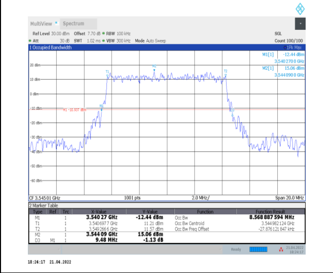
1-N78-3450-3550--30-10-H-2-DFT-PI2BPSK-Outer_ Full-24@0-Ant0-8.569-9.480-≤10-PASS
