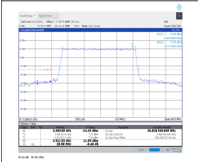
1-N78-3450-3550--30-30-M-5-DFT-256QAM-Outer_Full-75@0-Ant0-26.827-28.980-≤30-PASS
