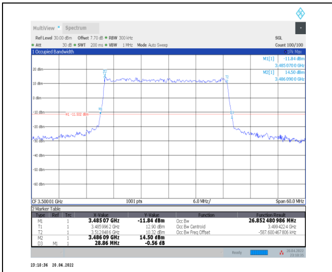
1-N78-3450-3550--30-30-M-3-DFT-16QAM-Outer_Full-75@0-Ant0-26.852-28.860-≤30-PASS
