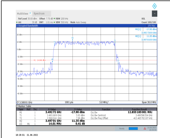
1-N78-3450-3550--30-15-M-5-DFT-256QAM-Outer_Full-36@0-Ant0-12.855-14.010-≤15-PASS
