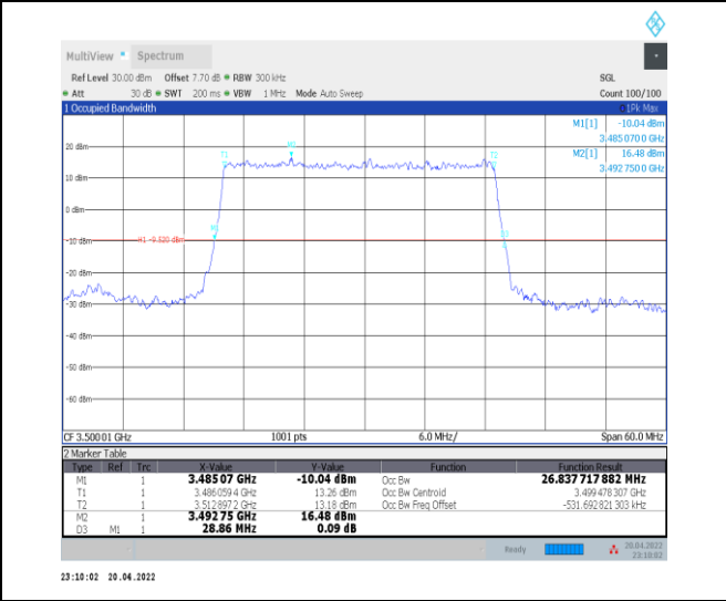
1-N78-3450-3550--30-30-M-2-DFT-PI2BPSK-Outer_Full-75@0-Ant0-26.838-28.860-<30-PASS
