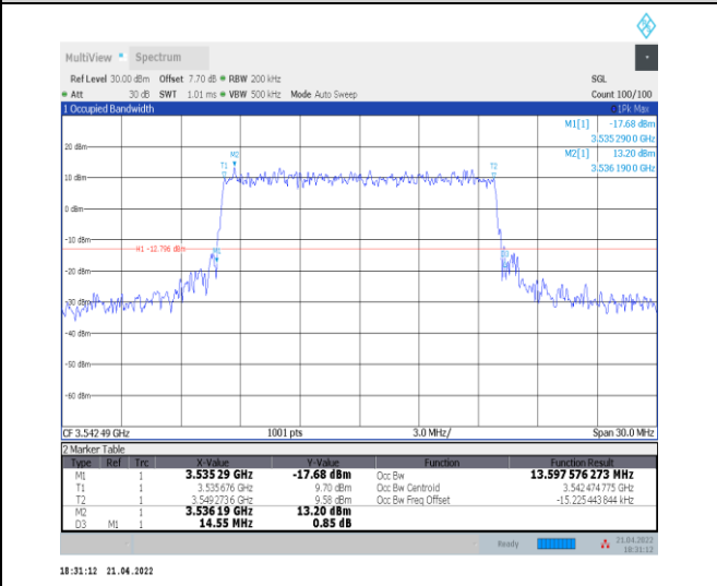
1-N78-3450-3550--30-15-H-7-CP-16QAM-Outer_Full-38@0-Ant0-13.598-14.550-≤15-PASS
