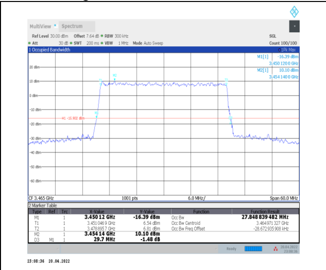
1-N78-3450-3550--30-30-L-9-CP-256QAM-Outer_Fu II-78@0-Ant0-27.849-29.700-<30-PASS
