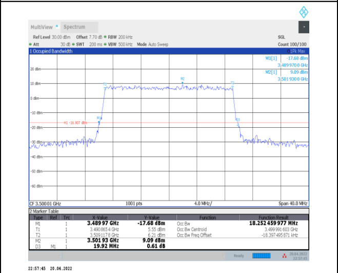
1-N78-3450-3550--30-20-M-9-CP-256QAM-Outer_Full-51@0-Ant0-18.252-19.920-≤20-PASS
