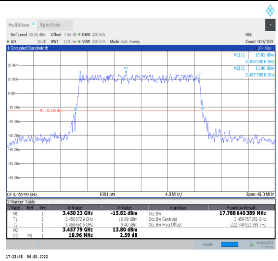
1-N78-3450-3550--30-20-L-4-DFT-64QAM-Outer_Fu II-50@0-Ant0-17.789-18.960-<=20-PASS
