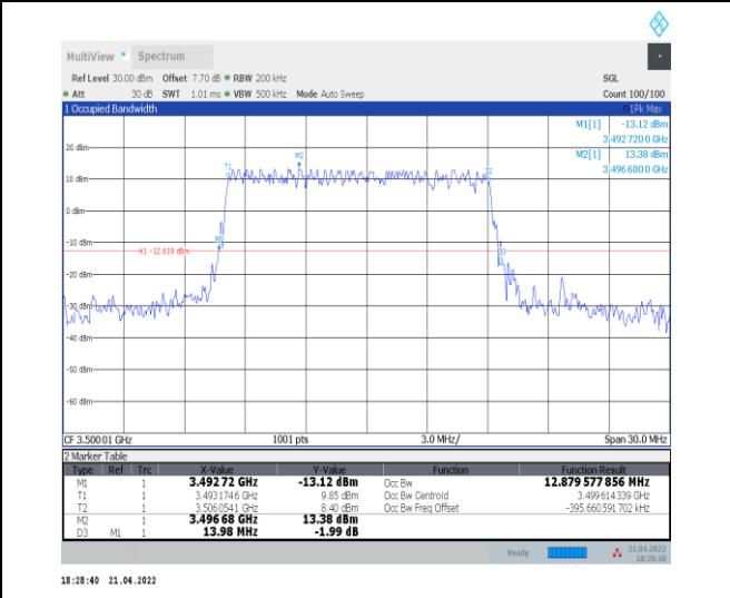
1-N78-3450-3550--30-15-M-4-DFT-64QAM-Outer_Full ull-36@0-Ant0-12.88-13.980-≤15-PASS
