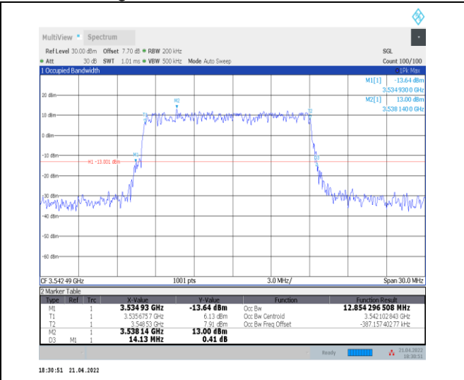
1-N78-3450-3550--30-15-H-5-DFT-256QAM-Outer_F ull-36@0-Ant0-12.854-14.130-≤15-PASS
