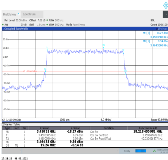
1-N78-3450-3550--30-20-L-9-CP-256QAM-Outer_Fu II-51@0-Ant0-18.218-19.240-<=20-PASS
