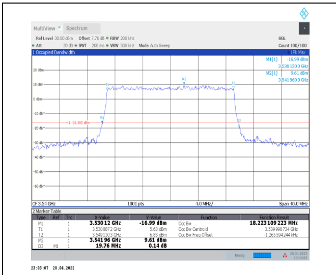
1-N78-3450-3550--30-20-H-9-CP-256QAM-Outer_Fu II-51 @0-Ant0-18.223-19.760-<math>\leq 20</math>-PASS
