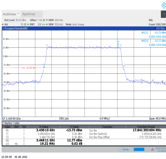
1-N78-3450-3550--30-20-L-5-DFT-256QAM-Outer_Full-50@0-Ant0-17.841-19.320-<=20-PASS
