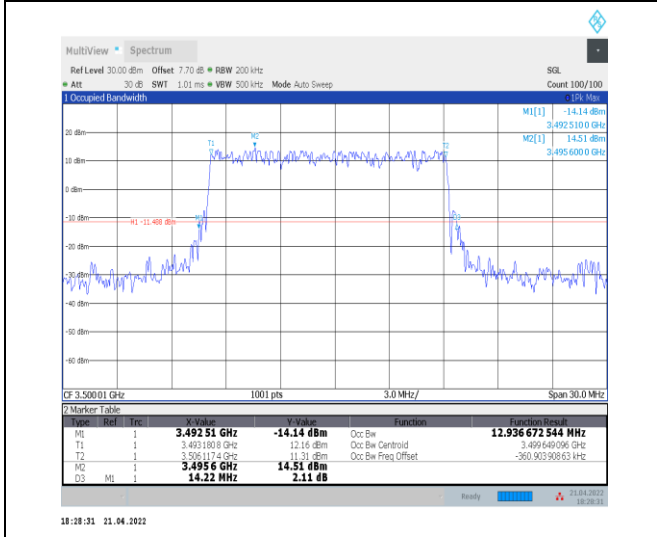
1-N78-3450-3550--30-15-M-3-DFT-16QAM-Outer_Full ull-36@0-Ant0-12.937-14.220-≤15-PASS
