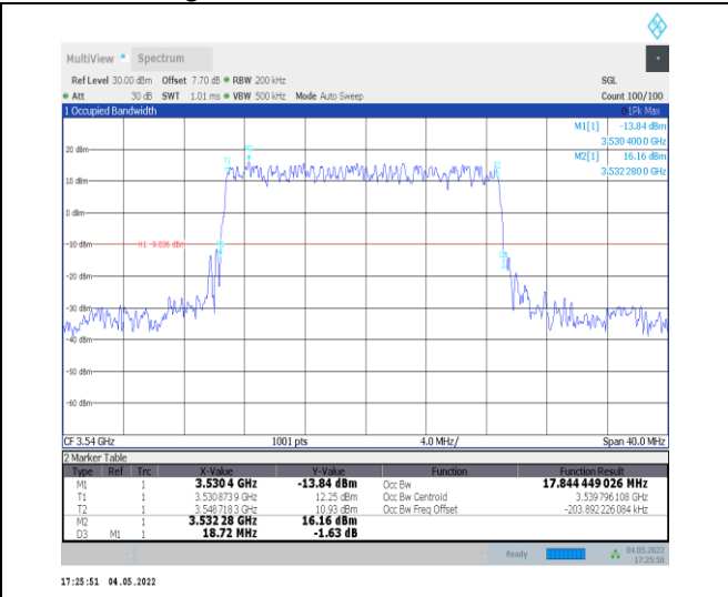
1-N78-3450-3550--30-20-H-2-DFT-PI2BPSK-Outer_Full Full-50@0-Ant0-17.844-18.720-≤20-PASS
