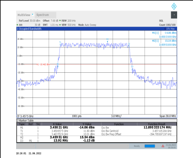
1-N78-3450-3550--30-15-L-1-DFT-QPSK-Outer_Full- 36@0-Ant0-12.895-13.920-≤15-PASS
