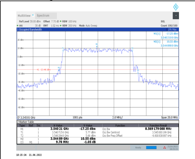
1-N78-3450-3550--30-10-H-8-CP-64QAM-Outer_Full -24@0-Ant0-8.569-9.780-≤10-PASS
