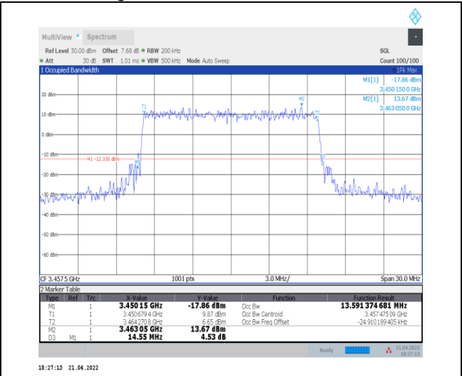
1-N78-3450-3550--30-15-L-7-CP-16QAM-Outer_Full -38@0-Ant0-13.591-14.550-≤15-PASS
