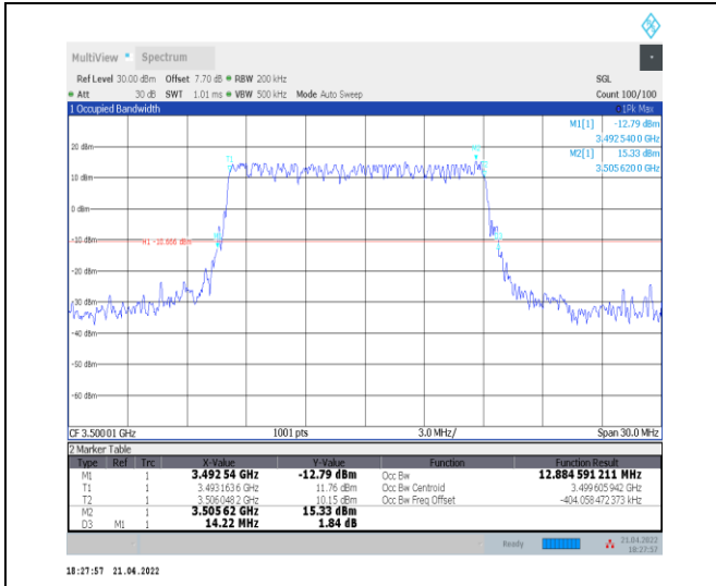
1-N78-3450-3550--30-15-M-1-DFT-QPSK-Outer_Full -36@0-Ant0-12.885-14.220-≤15-PASS
