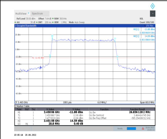
1-N78-3450-3550--30-30-L-3-DFT-16QAM-Outer_Full-75 @0-Ant0-26.836-28.800-<math>\leq 30</math>-PASS
