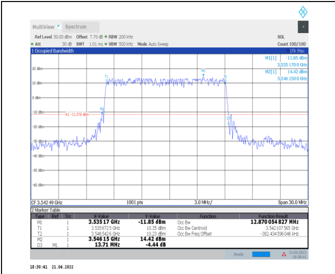
1-N78-3450-3550--30-15-H-4-DFT-64QAM-Outer_Fu ll-36@0-Ant0-12.87-13.710-≤15-PASS
