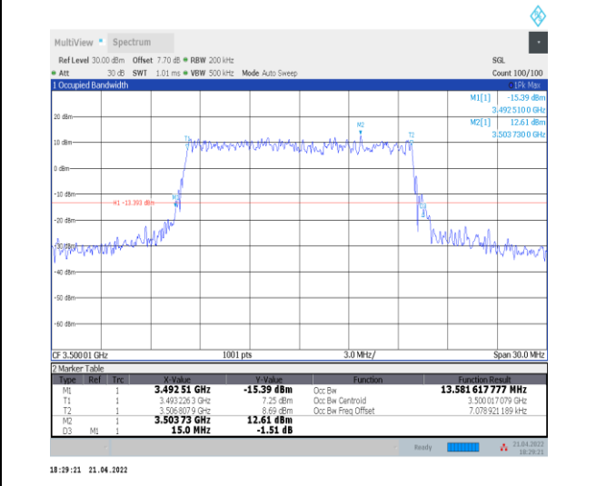
1-N78-3450-3550--30-15-M-8-CP-64QAM-Outer_Full-38@0-Ant0-13.582-15.000-≤15-PASS
