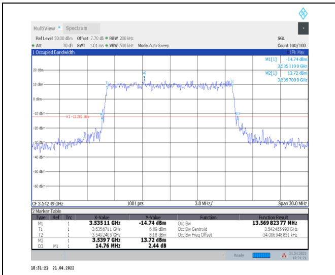
1-N78-3450-3550--30-15-H-8-CP-64QAM-Outer_Full -38@0-Ant0-13.57-14.760-≤15-PASS
