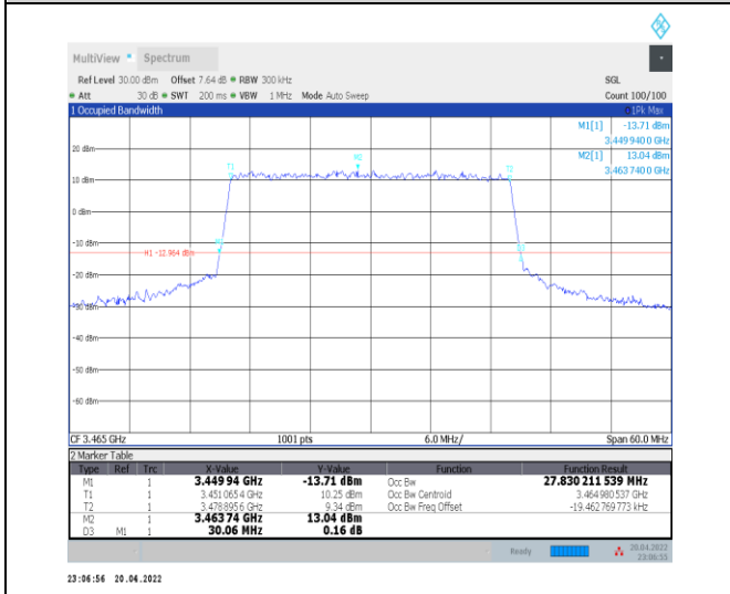
1-N78-3450-3550--30-30-L-6-CP-QPSK-Outer_Full-78@0-Ant0-27.83-30.060-≤30-PASS
