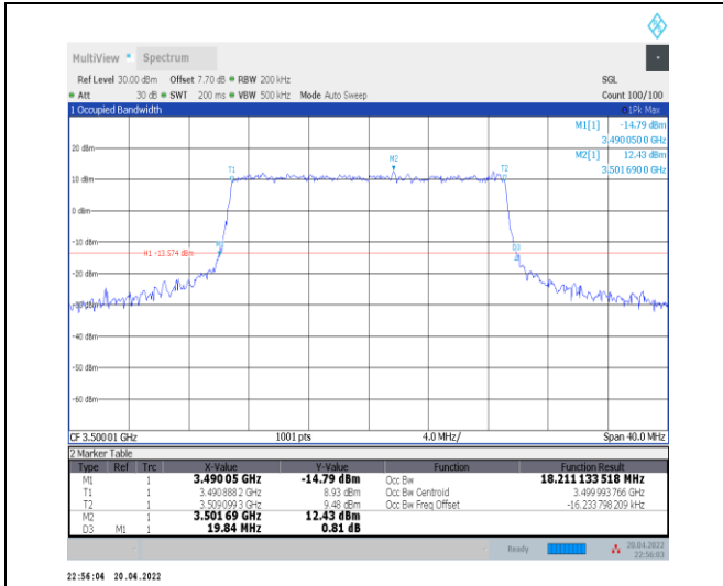
1-N78-3450-3550--30-20-M-6-CP-QPSK-Outer_Full-51@0-Ant0-18.211-19.840-≤20-PASS
