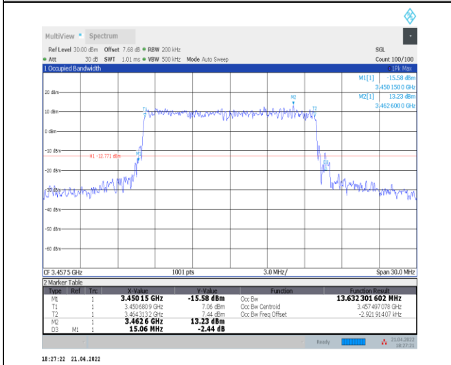
1-N78-3450-3550--30-15-L-8-CP-64QAM-Outer_Full -38@0-Ant0-13.632-15.060-≤15-PASS
