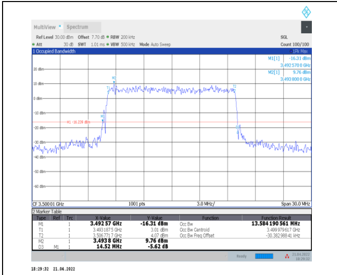
1-N78-3450-3550--30-15-M-9-CP-256QAM-Outer_Full-38@0-Ant0-13.584-14.520-≤15-PASS
