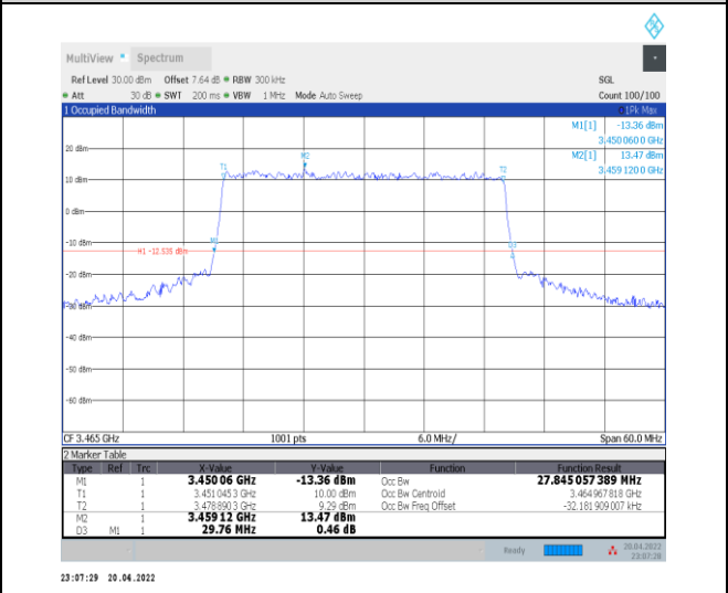
1-N78-3450-3550--30-30-L-7-CP-16QAM-Outer_Full-78@0-Ant0-27.845-29.760-≤30-PASS
