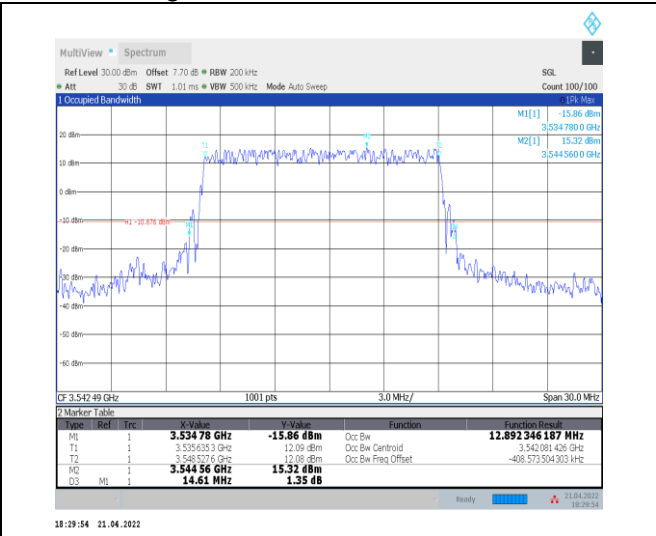
1-N78-3450-3550--30-15-H-1-DFT-QPSK-Outer_Full-36@0-Ant0-12.892-14.610-≤15-PASS
