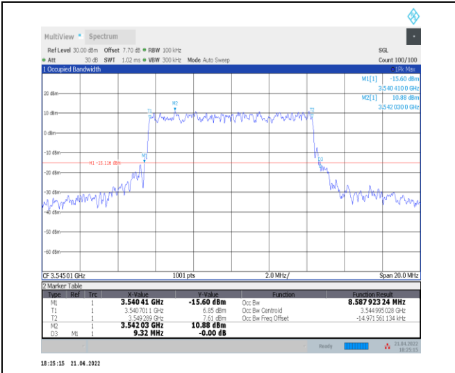
1-N78-3450-3550--30-10-H-7-CP-16QAM-Outer_Full -24@0-Ant0-8.588-9.320-≤10-PASS
