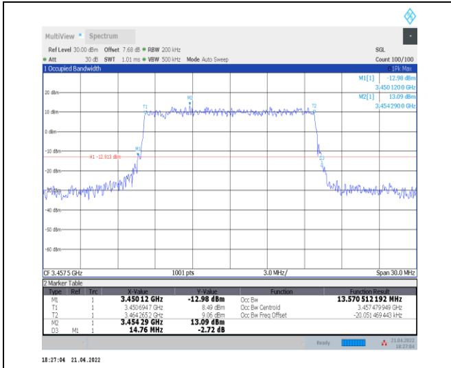
1-N78-3450-3550--30-15-L-6-CP-QPSK-Outer_Full-3 8@0-Ant0-13.571-14.760-≤15-PASS
