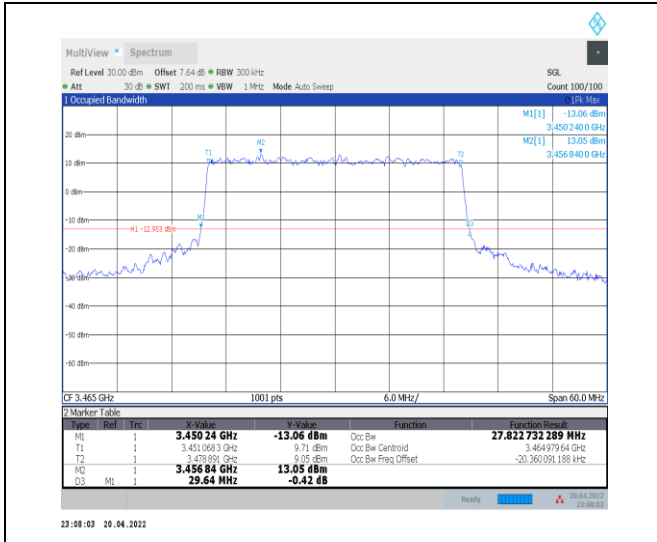
1-N78-3450-3550--30-30-L-8-CP-64QAM-Outer_Full -78@0-Ant0-27.823-29.640-<30-PASS
