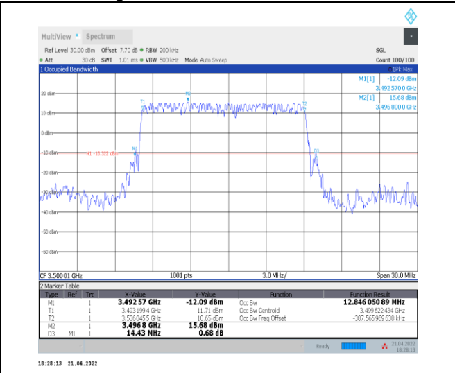
1-N78-3450-3550--30-15-M-2-DFT-PI2BPSK-Outer_Full Full-36@0-Ant0-12.846-14.430-≤15-PASS
