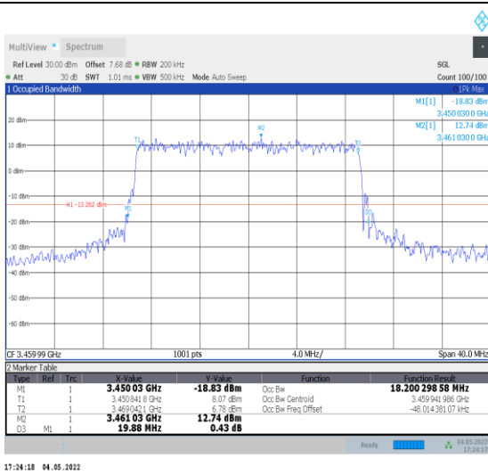
1-N78-3450-3550--30-20-L-7-CP-16QAM-Outer_Full -51@0-Ant0-18.2-19.880-<=20-PASS
