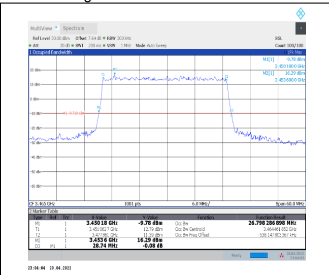
1-N78-3450-3550--30-30-L-1-DFT-QPSK-Outer_Full-75 @0-Ant0-26.798-28.740-<math>\leq 30</math>-PASS
