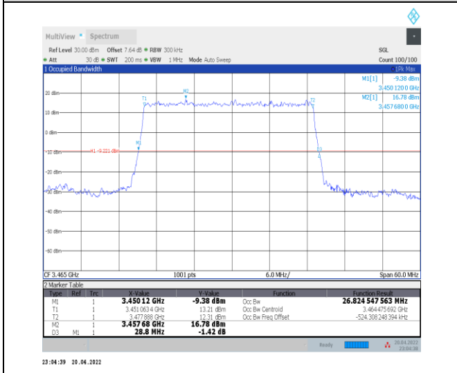
1-N78-3450-3550--30-30-L-2-DFT-PI2BPSK-Outer_Full-75 @0-Ant0-26.825-28.800-<math>\leq 30</math>-PASS
