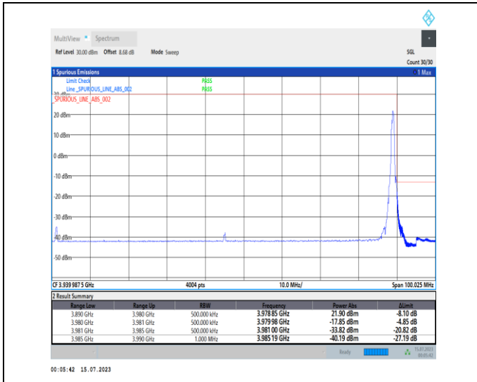
1-N77-3700-3980-PC1-30-90-H-2-DFT-PI2BPSK-Edge _1RB_Right-1@244-Ant0-1--PASS-see graph
