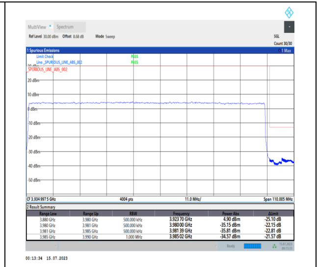
1-N77-3700-3980-PC1-30-100-H-3-DFT-PI2BPSK-Outer_Full-270@0-Ant0-1--PASS-see graph
