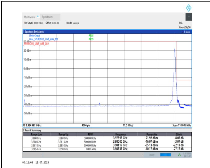
1-N77-3700-3980-PC1-30-100-H-2-DFT-PI2BPSK-Edge_e_1RB_Right-1@272-Ant0-1--PASS-see graph
