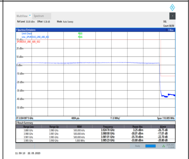
1-N77-3700-3980-PC1-30-100-H-6-CP-QPSK-Outer_Full-273@0-Ant0-1--PASS-see graph
