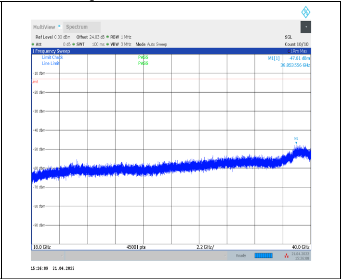
1-N77-3700-3980--30-100-L-1-DFT-PI2BPSK-Inner_1RB_Left-1 @ 1-18000-40000-Ant0--47.61--13-PASS
