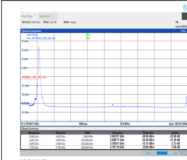
1-N77-3700-3980-PC1-30-90-L-4-CP-QPSK-Edge_1_RB_Left-1@0-Ant0-1--PASS-see graph
