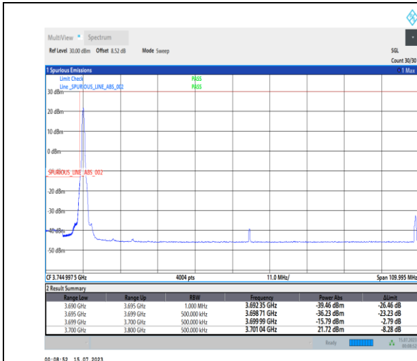
1-N77-3700-3980-PC1-30-100-L-1-DFT-PI2BPSK-Edge_1RB_Left-1@0-Ant0-1--PASS-see graph
