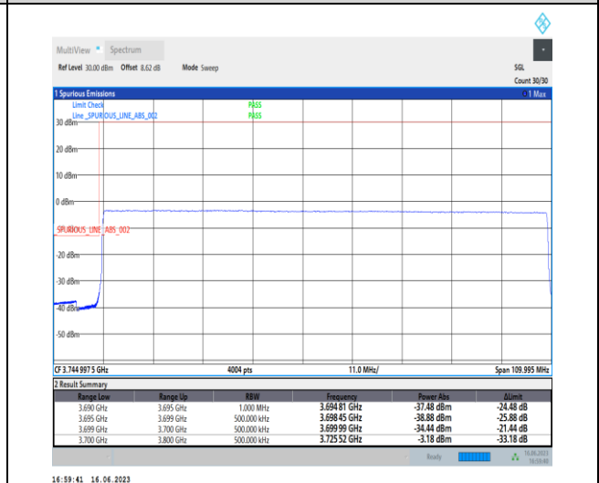
1-N77-3700-3980-PC1-30-100-L-6-CP-QPSK-Outer_Full-273@0-Ant0-1--PASS-see graph
