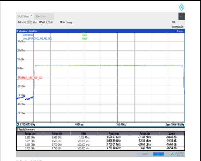
1-N77-3700-3980-PC1-30-90-L-6-CP-QPSK-Outer_Full-245@0-Ant0-1--PASS-see graph
