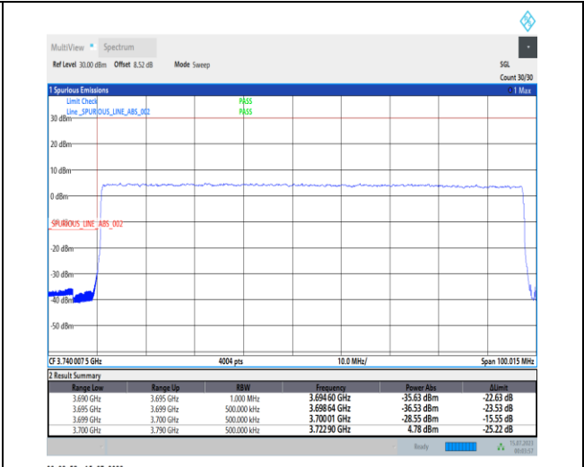
1-N77-3700-3980-PC1-30-90-L-3-DFT-PI2BPSK-Outer_Full-240@0-Ant0-1--PASS-see graph
