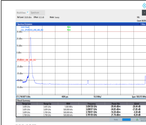
1-N77-3700-3980-PC1-30-90-L-1-DFT-PI2BPSK-Edge_1_RB_Left-1@0-Ant0-1--PASS-see graph
