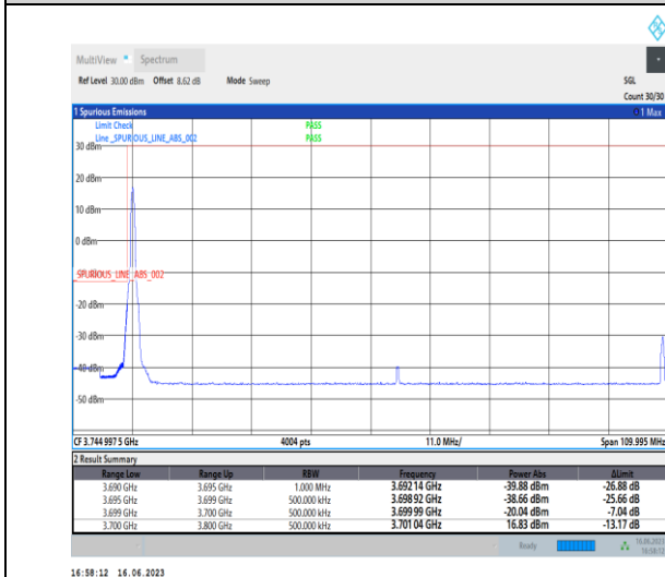
1-N77-3700-3980-PC1-30-100-L-4-CP-QPSK-Edge_1RB_Left-1@0-Ant0-1--PASS-see graph
