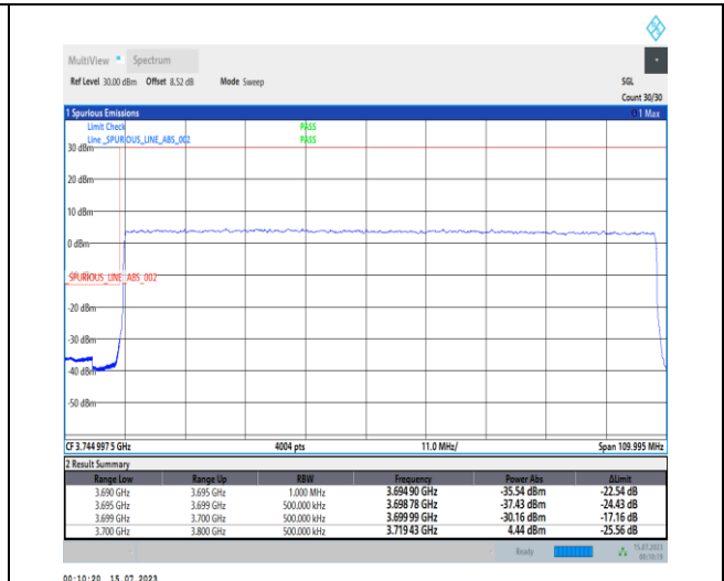
1-N77-3700-3980-PC1-30-100-L-3-DFT-PI2BPSK-Outer_Full-270@0-Ant0-1--PASS-see graph
