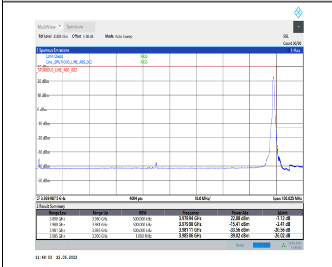
1-N77-3700-3980-PC1-30-90-H-5-CP-QPSK-Edge_1R B_Right-1@244-Ant0-1--PASS-see graph
