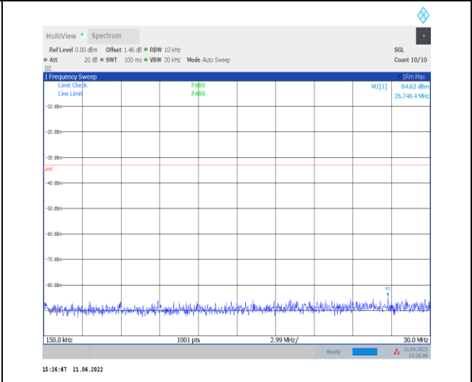
1-N77-3700-3980--30-100-M-1-DFT-PI2BPSK-Inner_1RB_Left-1 @ 1-0.15-30-Ant0--84.63--33-PASS
