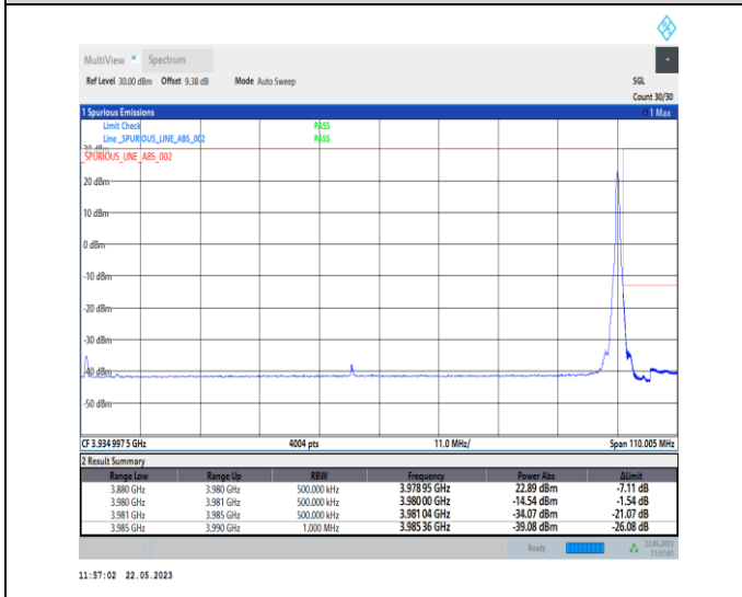
1-N77-3700-3980-PC1-30-100-H-5-CP-QPSK-Edge_1RB_Right-1@272-Ant0-1--PASS-see graph
