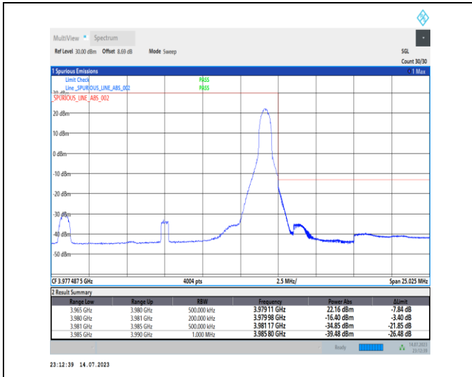
1-N77-3700-3980-PC1-30-15-H-2-DFT-PI2BPSK-Edge _1RB_Right-1@37-Ant0-1--PASS-see graph
