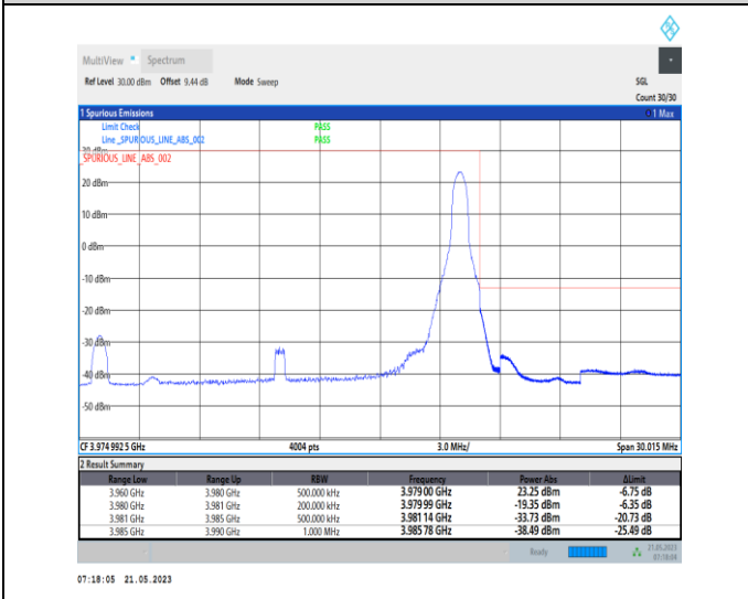
1-N77-3700-3980-PC1-30-20-H-5-CP-QPSK-Edge_1R B_Right-1@50-Ant0-1--PASS-see graph
