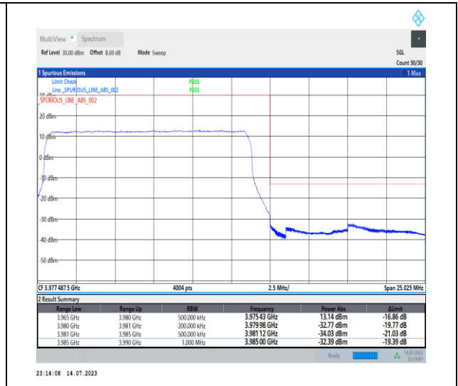
1-N77-3700-3980-PC1-30-15-H-3-DFT-PI2BPSK- Outer_Full-36@0-Ant0-1--PASS-see graph
