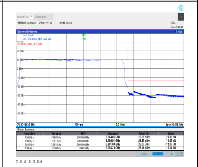
1-N77-3700-3980-PC1-30-20-H-6-CP-QPSK-Outer _Full-51@0-Ant0-1--PASS-see graph
