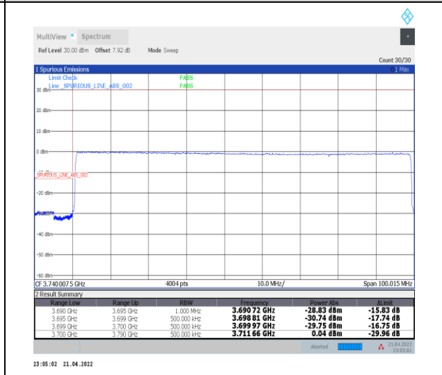
1-N77-3700-3980--30-90-L-6-CP-QPSK-Outer_Ful I-245@0-Ant0-PASS-see graph
