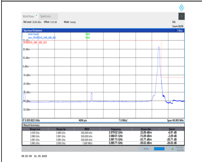
1-N77-3700-3980-PC1-30-60-H-5-CP-QPSK-Edge_1R B_Right-1@161-Ant0-1--PASS-see graph
