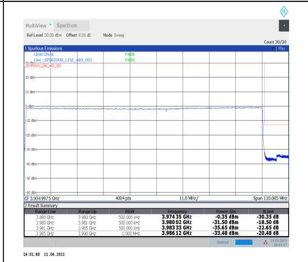
1-N77-3700-3980--30-100-H-6-CP-QPSK-Outer_F ull-273@0-Ant0-PASS-see graph
