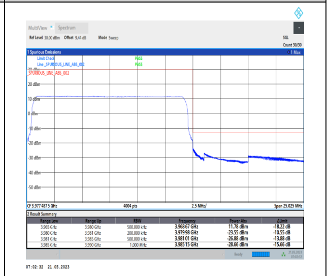
1-N77-3700-3980-PC1-30-15-H-6-CP-QPSK-Outer _Full-38@0-Ant0-1--PASS-see graph
