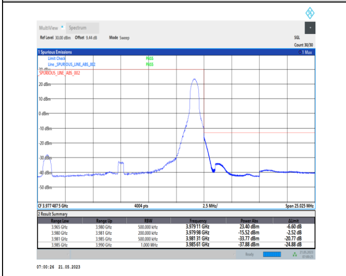
1-N77-3700-3980-PC1-30-15-H-5-CP-QPSK-Edge_1R B_Right-1@37-Ant0-1--PASS-see graph
