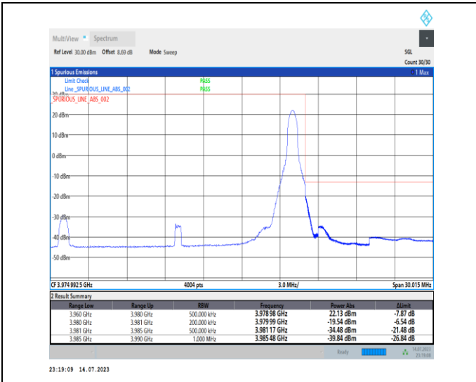
1-N77-3700-3980-PC1-30-20-H-2-DFT-PI2BPSK-Edge _1RB_Right-1@50-Ant0-1--PASS-see graph
