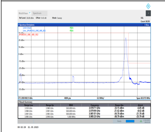
1-N77-3700-3980-PC1-30-50-H-5-CP-QPSK-Edge_1R B_Right-1@132-Ant0-1--PASS-see graph
