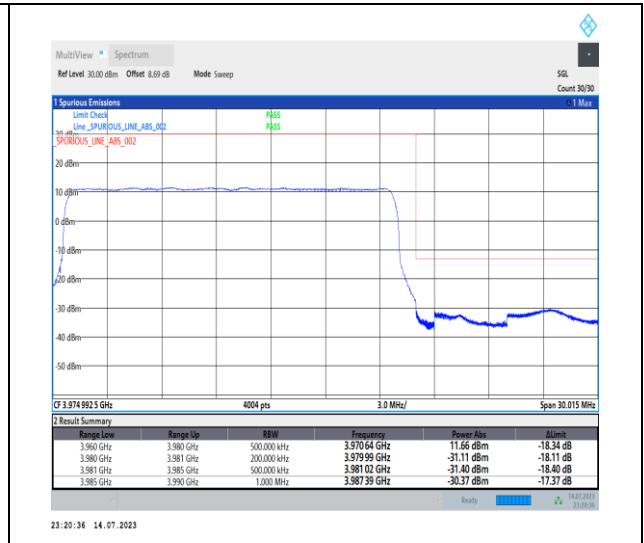
1-N77-3700-3980-PC1-30-20-H-3-DFT-PI2BPSK- Outer_Full-50@0-Ant0-1--PASS-see graph
