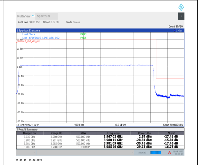
1-N77-3700-3980--30-50-H-6-CP-QPSK-Outer_Full-113@0-Ant0-PASS-see graph
