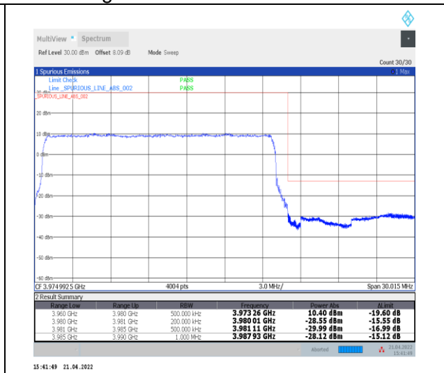
1-N77-3700-3980--30-20-H-3-DFT-PI2BPSK-Outer_Full-50@0-Ant0-PASS-see graph
