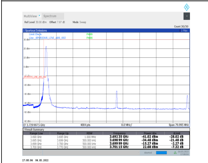
1-N77-3700-3980--30-70-L-4-CP-QPSK-Edge_1RB_L_eff-1@0-Ant0-PASS-see graph
