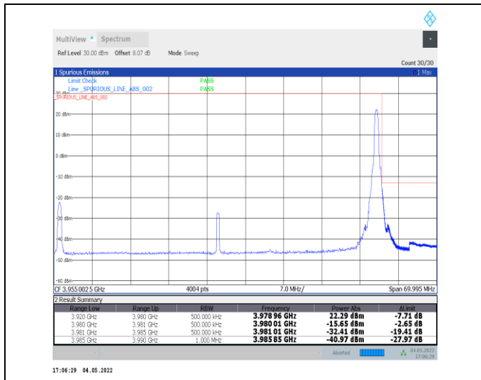
1-N77-3700-3980--30-60-H-2-DFT-PI2BPSK-Edge_1R_B_Right-1@161-Ant0-PASS-see graph
