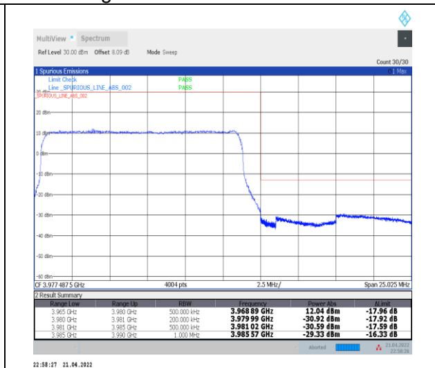
1-N77-3700-3980--30-15-H-3-DFT-PI2BPSK-Outer_Full-36@0-Ant0-PASS-see graph
