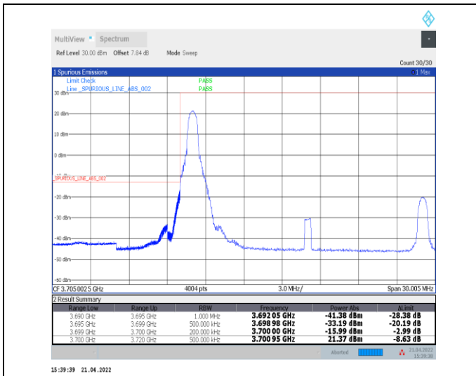
1-N77-3700-3980--30-20-L-1-DFT-PI2BPSK-Edge_1R_B_Left-1@0-Ant0-PASS-see graph
