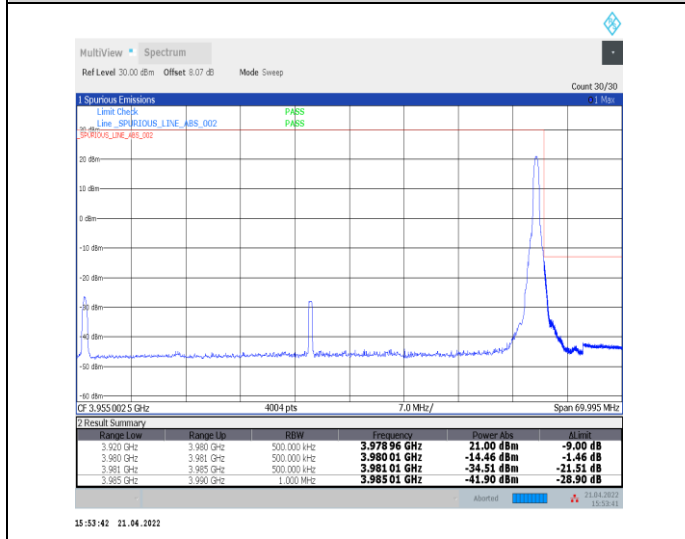
1-N77-3700-3980--30-60-H-5-CP-QPSK-Edge_1RB_Right-1@161-Ant0-PASS-see graph
