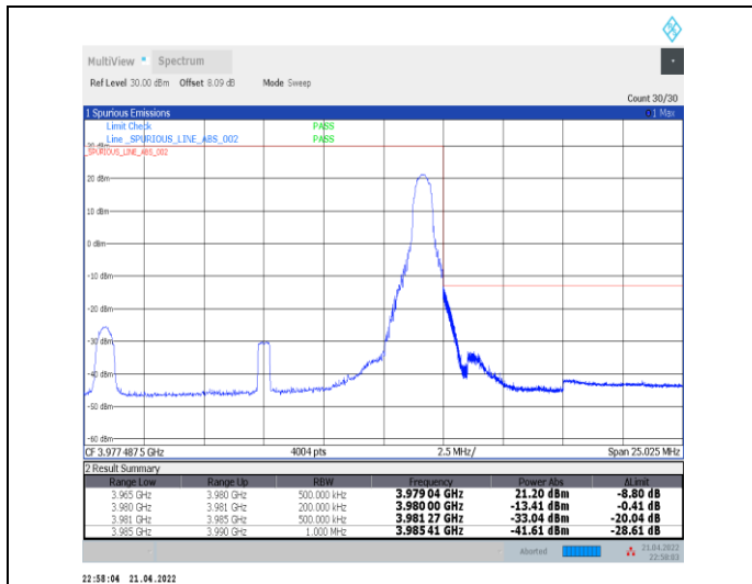
1-N77-3700-3980--30-15-H-2-DFT-PI2BPSK-Edge_1R_B_Right-1@37-Ant0-PASS-see graph
