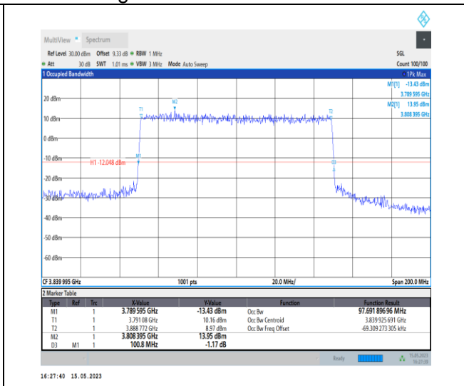
1-N77-3700-3980-PC1-30-100-M-7-CP-16QAM-Outer_Full-273@0-Ant0-97.692-100.800-≤100-PASS
