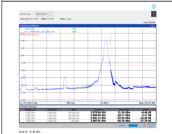
1-N77-3700-3980--30-20-H-5-CP-QPSK-Edge_1RB_Right-1@50-Ant0-PASS-see graph
