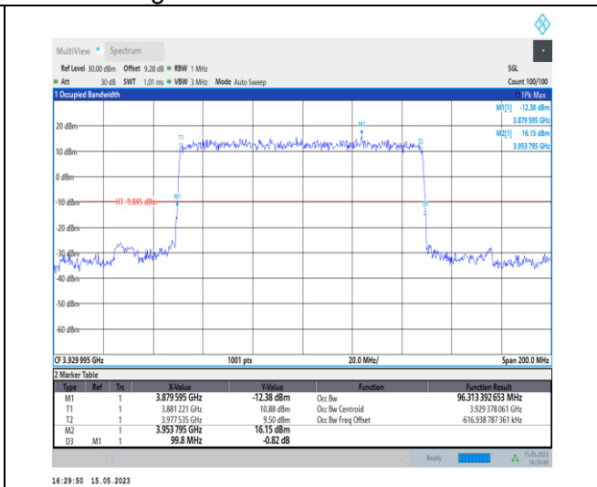
1-N77-3700-3980-PC1-30-100-H-2-DFT-PI2BPSK-Outer_Full-270@0-Ant0-96.313-99.800-≤100-PASS
