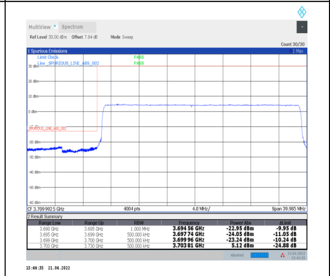
1-N77-3700-3980--30-30-L-6-CP-QPSK-Outer_Ful l-78@0-Ant0-PASS-see graph
