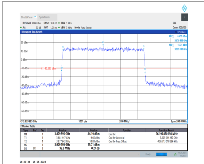
1-N77-3700-3980-PC1-30-100-H-1-DFT-QPSK-Outer_Full-270@0-Ant0-96.195-99.800-≤100-PASS
