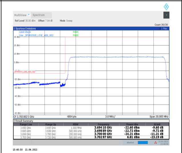
1-N77-3700-3980--30-20-L-6-CP-QPSK-Outer_Ful l-51@0-Ant0-PASS-see graph
