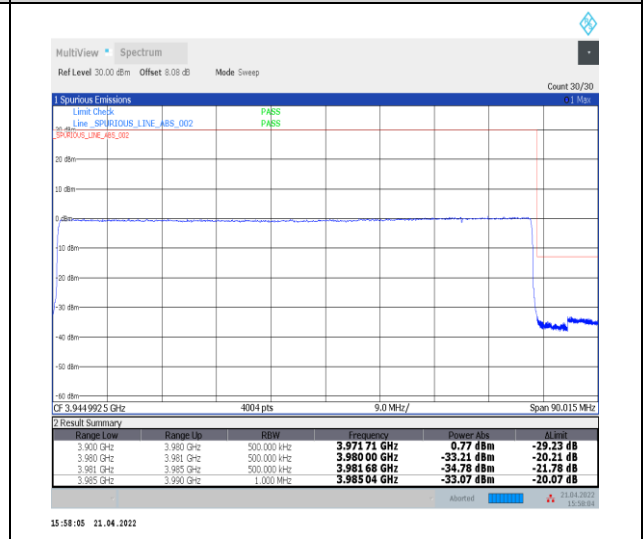
1-N77-3700-3980--30-80-H-6-CP-QPSK-Outer_Full-217@0-Ant0-PASS-see graph
