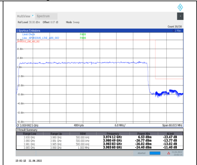
1-N77-3700-3980--30-50-H-3-DFT-PI2BPSK-Outer_Full-128@0-Ant0-PASS-see graph
