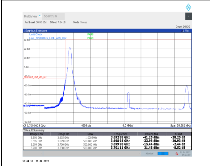
1-N77-3700-3980--30-30-L-4-CP-QPSK-Edge_1RB_L_eft-1@0-Ant0-PASS-see graph
