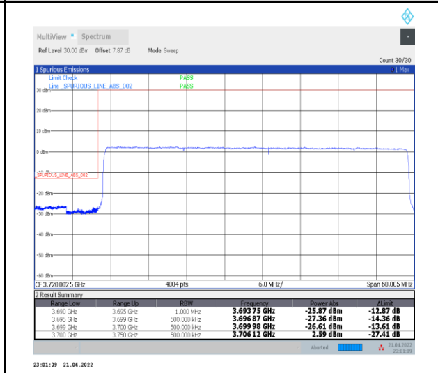
1-N77-3700-3980--30-50-L-6-CP-QPSK-Outer_Ful I-133@0-Ant0-PASS-see graph
