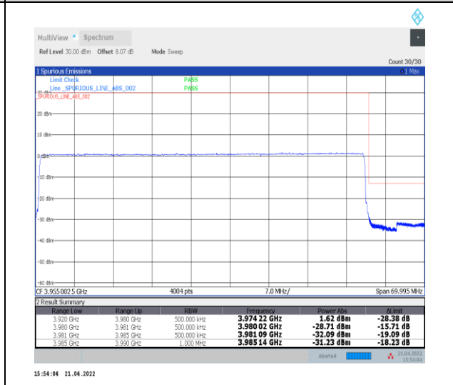
1-N77-3700-3980--30-60-H-6-CP-QPSK-Outer_Full-162@0-Ant0-PASS-see graph
