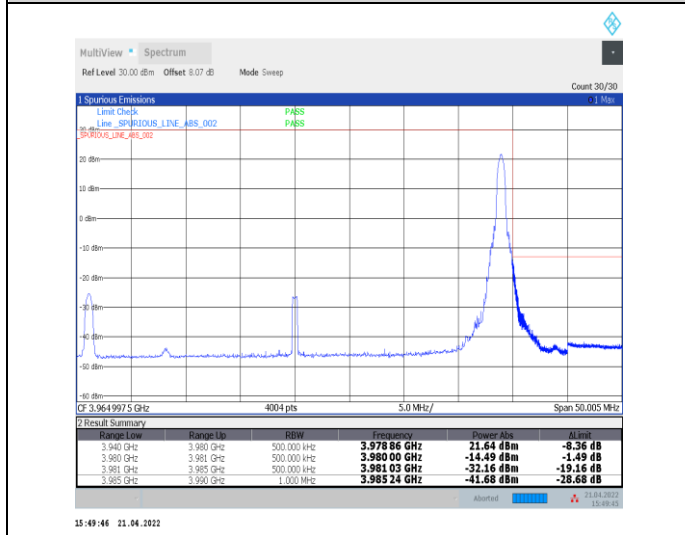
1-N77-3700-3980--30-40-H-5-CP-QPSK-Edge_1RB_Right-1@105-Ant0-PASS-see graph
