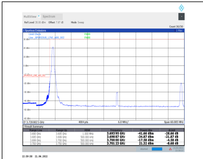
1-N77-3700-3980--30-50-L-1-DFT-PI2BPSK-Edge_1R_B_Left-1@0-Ant0-PASS-see graph
