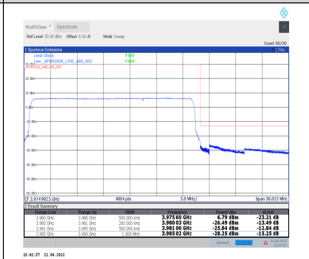
1-N77-3700-3980--30-20-H-6-CP-QPSK-Outer_Full-51@0-Ant0-PASS-see graph
