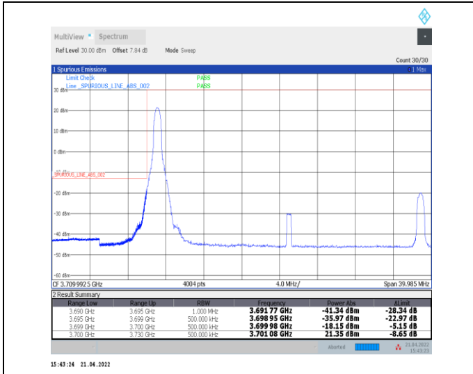
1-N77-3700-3980--30-30-L-1-DFT-PI2BPSK-Edge_1R_B_Left-1@0-Ant0-PASS-see graph
