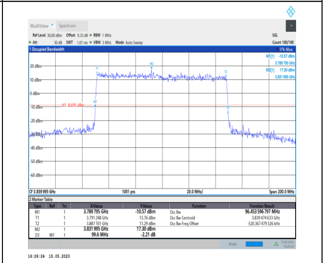
1-N77-3700-3980-PC1-30-100-M-1-DFT-QPSK-Outer_Full-270@0-Ant0-96.454-99.600-≤100-PASS
