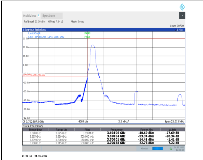
1-N77-3700-3980--30-15-L-1-DFT-PI2BPSK-Edge_1R_B_Left-1@0-Ant0-PASS-see graph
