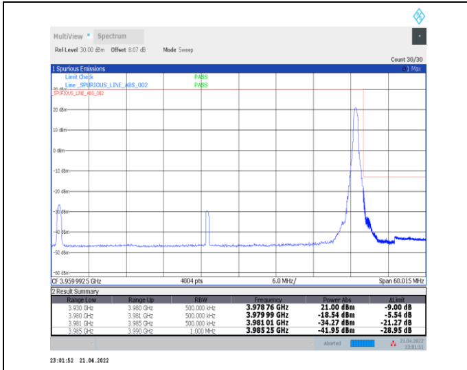
1-N77-3700-3980--30-50-H-2-DFT-PI2BPSK-Edge_1R_B_Right-1@132-Ant0-PASS-see graph
