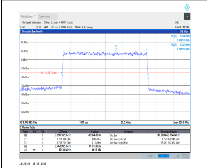
1-N77-3700-3980-PC1-30-100-L-9-CP-256QAM-Outer_Full-273@0-Ant0-97.369-101.000-≤100-PASS
