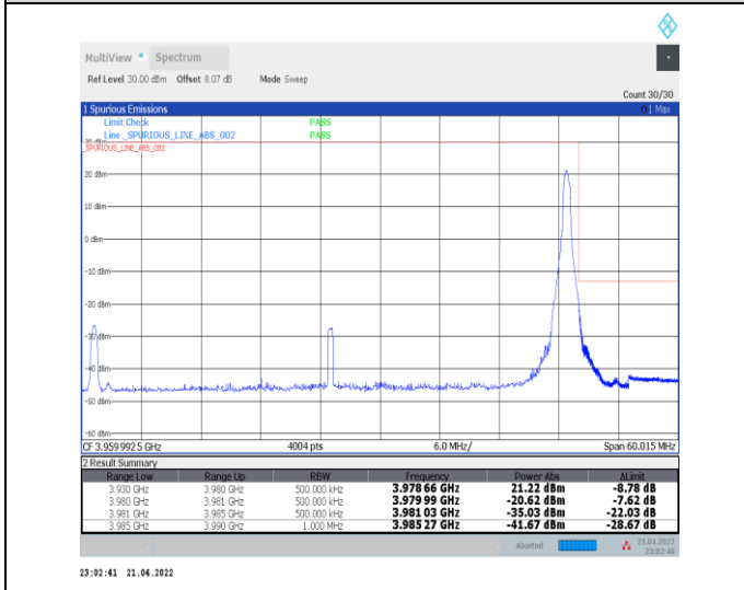
1-N77-3700-3980--30-50-H-5-CP-QPSK-Edge_1RB_Right-1@132-Ant0-PASS-see graph
