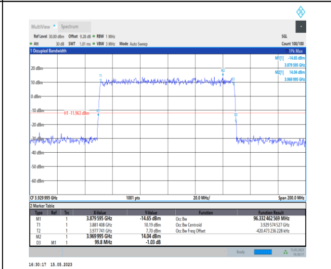
1-N77-3700-3980-PC1-30-100-H-4-DFT-64QAM-Outer_Full-270@0-Ant0-96.332-99.800-≤100-PASS
