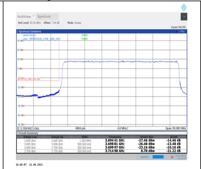
1-N77-3700-3980--30-30-L-3-DFT-PI2BPSK-Outer_Full-75@0-Ant0-PASS-see graph
