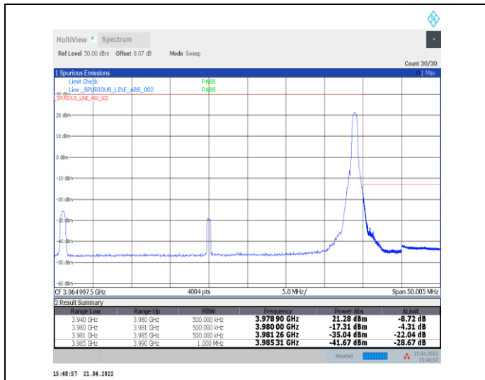
1-N77-3700-3980--30-40-H-2-DFT-PI2BPSK-Edge_1R_B_Right-1@105-Ant0-PASS-see graph
