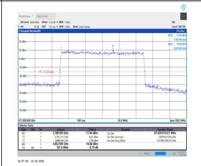
1-N77-3700-3980-PC1-30-100-M-9-CP-256QAM-Outer_Full-273@0-Ant0-97.429-101.000-≤100-PASS
