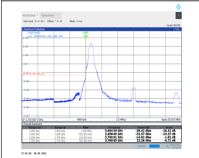
1-N77-3700-3980--30-15-L-4-CP-QPSK-Edge_1RB_L_eff-1@0-Ant0-PASS-see graph
