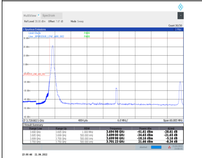
1-N77-3700-3980--30-50-L-4-CP-QPSK-Edge_1RB_L_eff-1@0-Ant0-PASS-see graph
