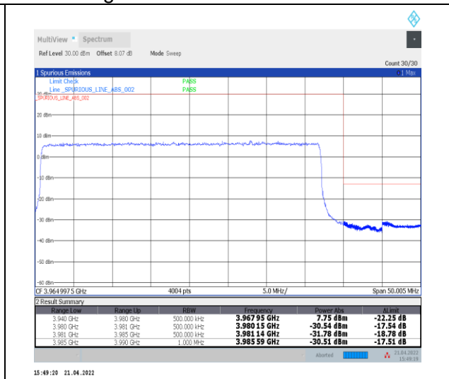
1-N77-3700-3980--30-40-H-3-DFT-PI2BPSK-Outer_Full-100@0-Ant0-PASS-see graph
