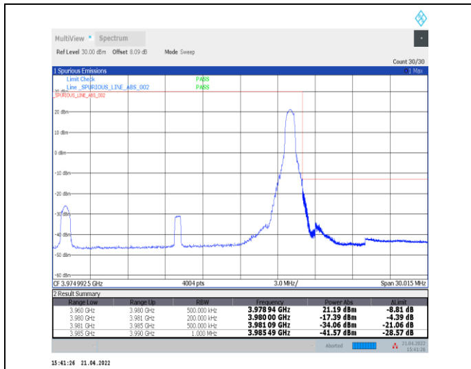
1-N77-3700-3980--30-20-H-2-DFT-PI2BPSK-Edge_1R_B_Right-1@50-Ant0-PASS-see graph
