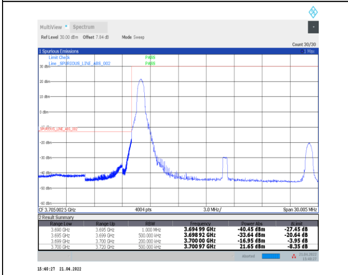
1-N77-3700-3980--30-20-L-4-CP-QPSK-Edge_1RB_L eft-1@0-Ant0-PASS-see graph
