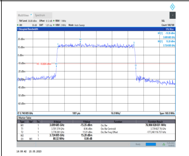
1-N77-3700-3980-PC1-30-80-L-4-DFT-64QAM-Outer_Full-216@0-Ant0-76.907-80.320-≤80-PASS
