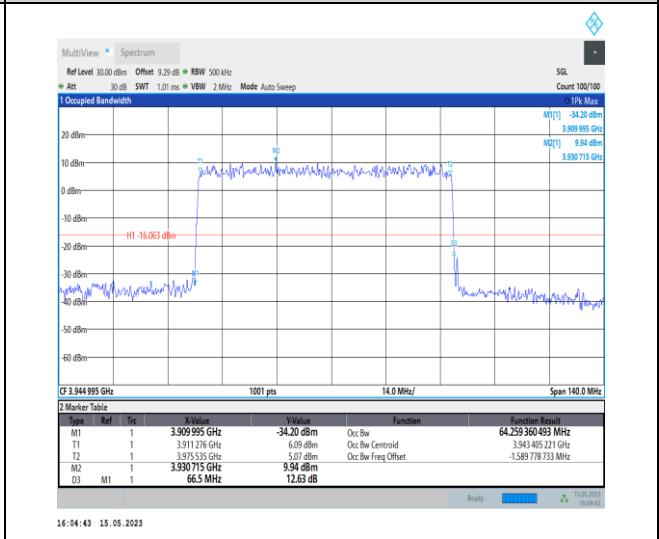
1-N77-3700-3980-PC1-30-70-H-5-DFT-256QAM-Out er_Full-180@0-Ant0-64.259-66.500-≤70-PASS
