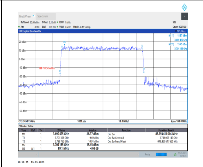
1-N77-3700-3980-PC1-30-90-L-1-DFT-QPSK-Outer_Full-240@0-Ant0-85.393-89.100-≤90-PASS
