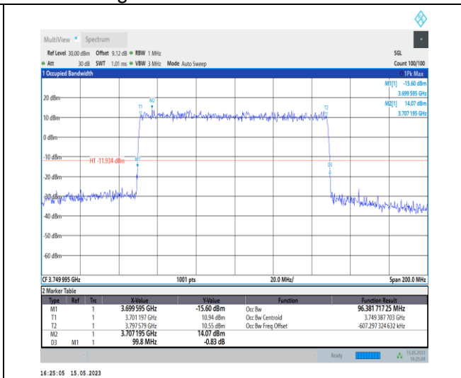
1-N77-3700-3980-PC1-30-100-L-4-DFT-64QAM-Out er_Full-270@0-Ant0-96.382-99.800-≤100-PASS
