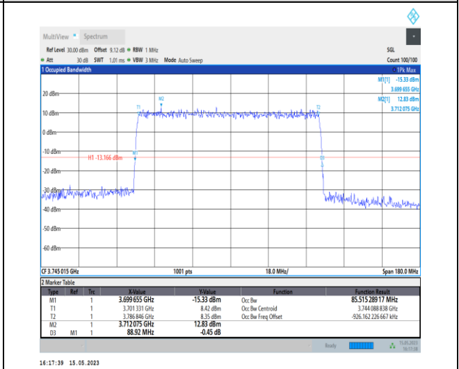
1-N77-3700-3980-PC1-30-90-L-5-DFT-256QAM-Outer_Full-240@0-Ant0-85.515-88.920-<math>\leq 90</math>-PASS
