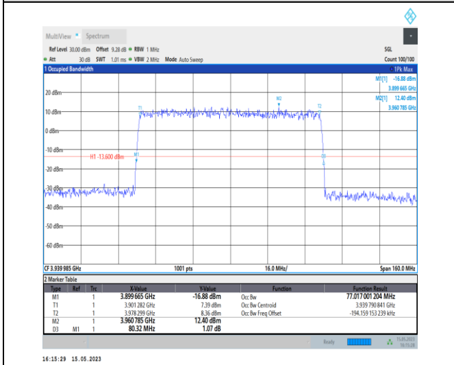
1-N77-3700-3980-PC1-30-80-H-5-DFT-256QAM-Outer_Full-216@0-Ant0-77.017-80.320-≤80-PASS
