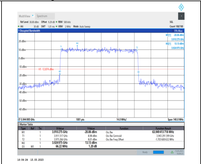
1-N77-3700-3980-PC1-30-70-H-3-DFT-16QAM-Out er_Full-180@0-Ant0-63.949-66.220-≤70-PASS
