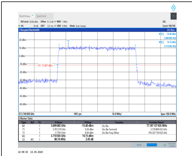
1-N77-3700-3980-PC1-30-80-L-5-DFT-256QAM-Out er_Full-216@0-Ant0-77.181-80.160-≤80-PASS
