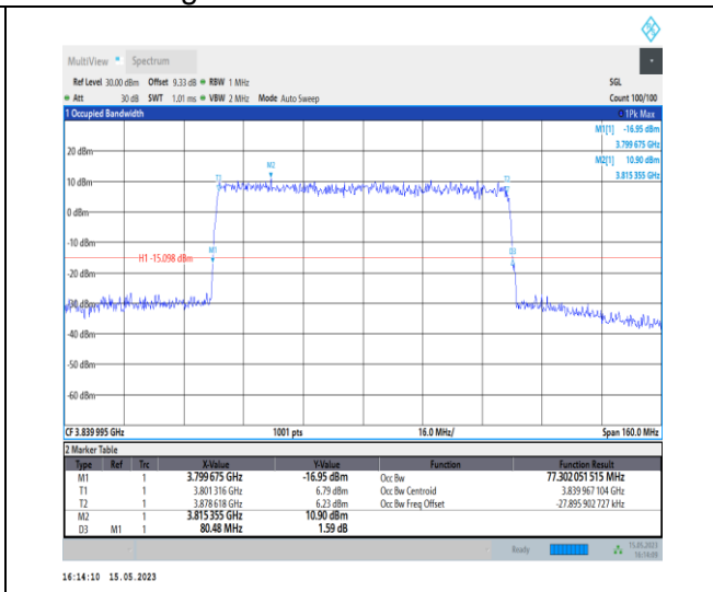
1-N77-3700-3980-PC1-30-80-M-9-CP-256QAM-Outer_Full-217@0-Ant0-77.302-80.480-≤80-PASS
