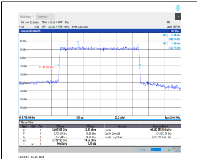
1-N77-3700-3980-PC1-30-100-L-3-DFT-16QAM-Out er_Full-270@0-Ant0-96.343-99.600-≤100-PASS
