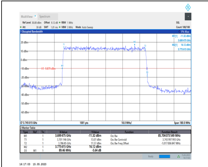
1-N77-3700-3980-PC1-30-90-L-2-DFT-PI2BPSK-Out er_Full-240@0-Ant0-85.704-89.460-<math>\leq 90</math>-PASS
