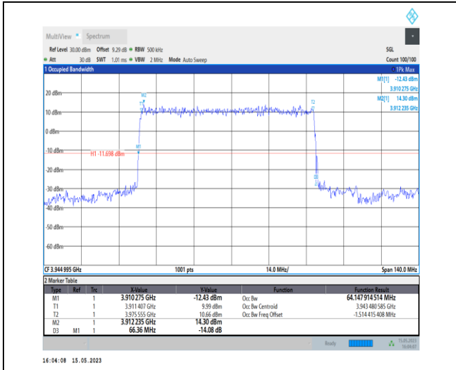
1-N77-3700-3980-PC1-30-70-H-2-DFT-PI2BPSK-Out er_Full-180@0-Ant0-64.148-66.360-≤70-PASS
