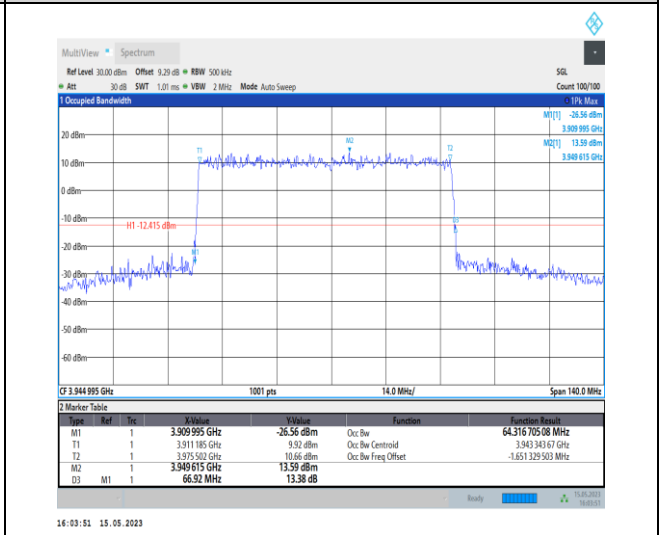
1-N77-3700-3980-PC1-30-70-H-1-DFT-QPSK-Outer_Full-180@0-Ant0-64.317-66.920-≤70-PASS
