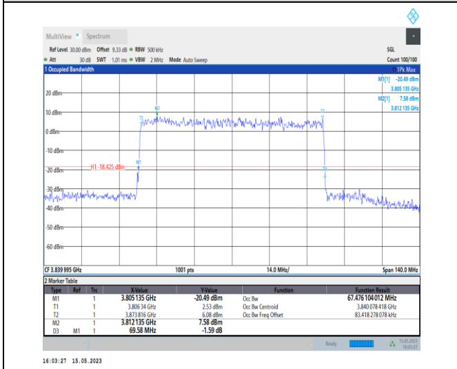
1-N77-3700-3980-PC1-30-70-M-9-CP-256QAM-Outer_Full-189@0-Ant0-67.476-69.580-≤70-PASS
