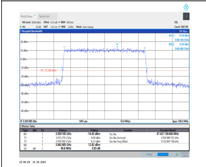
1-N77-3700-3980-PC1-30-50-H-6-CP-QPSK-Outer_Full-133@0-Ant0-47.421-49.800-≤50-PASS
