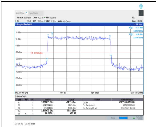
1-N77-3700-3980-PC1-30-60-M-2-DFT-PI2BPSK-Out_Full-162@0-Ant0-57.856-60.000-≤60-PASS
