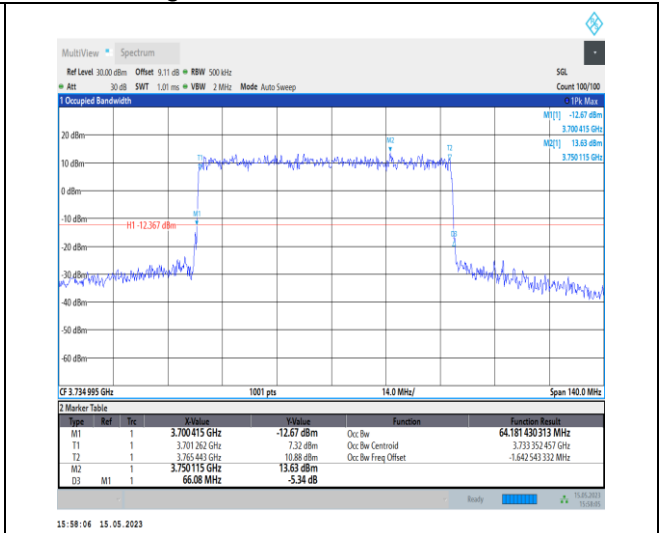
1-N77-3700-3980-PC1-30-70-L-1-DFT-QPSK-Outer_Full-180@0-Ant0-64.181-66.080-≤70-PASS
