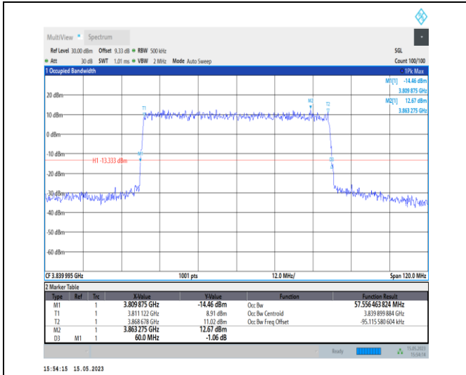
1-N77-3700-3980-PC1-30-60-M-6-CP-QPSK-Outer_Full-162@0-Ant0-57.556-60.000-≤60-PASS
