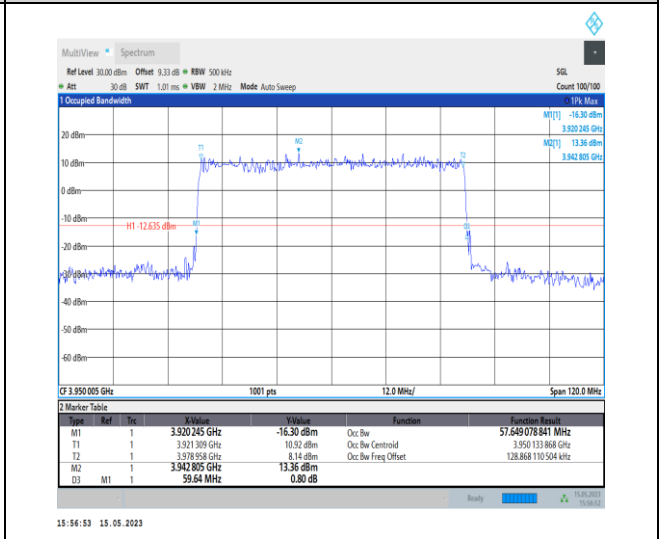
1-N77-3700-3980-PC1-30-60-H-4-DFT-64QAM-Outer_Full-162@0-Ant0-57.649-59.640-≤60-PASS
