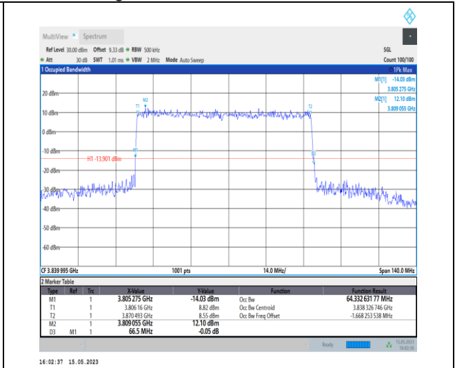
1-N77-3700-3980-PC1-30-70-M-4-DFT-64QAM-Outer_Full-180@0-Ant0-64.333-66.500-≤70-PASS
