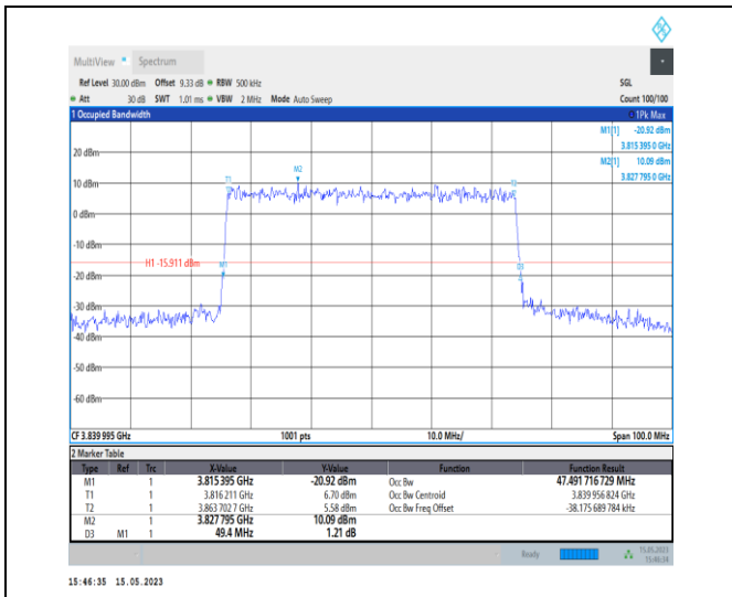
1-N77-3700-3980-PC1-30-50-M-9-CP-256QAM-Outer_Full-133@0-Ant0-47.492-49.400-≤50-PASS
