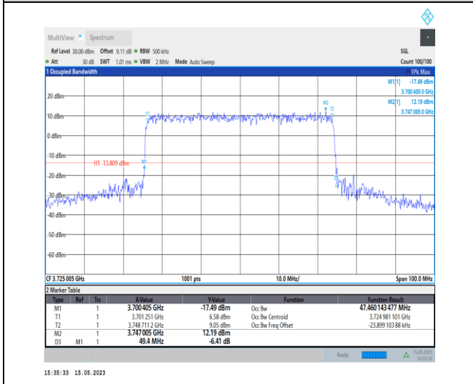
1-N77-3700-3980-PC1-30-50-L-8-CP-64QAM-Outer_Full-133@0-Ant0-47.46-49.400-≤50-PASS
