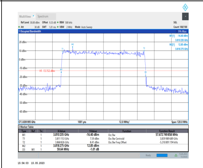
1-N77-3700-3980-PC1-30-60-M-5-DFT-256QAM-Out_Full-162@0-Ant0-57.673-59.640-≤60-PASS
