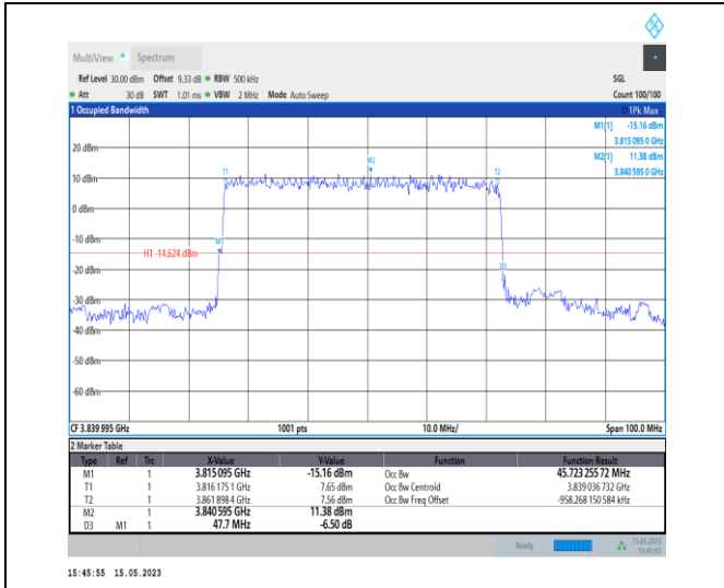
1-N77-3700-3980-PC1-30-50-M-5-DFT-256QAM-Out er_Full-128@0-Ant0-45.723-47.700-≤50-PASS
