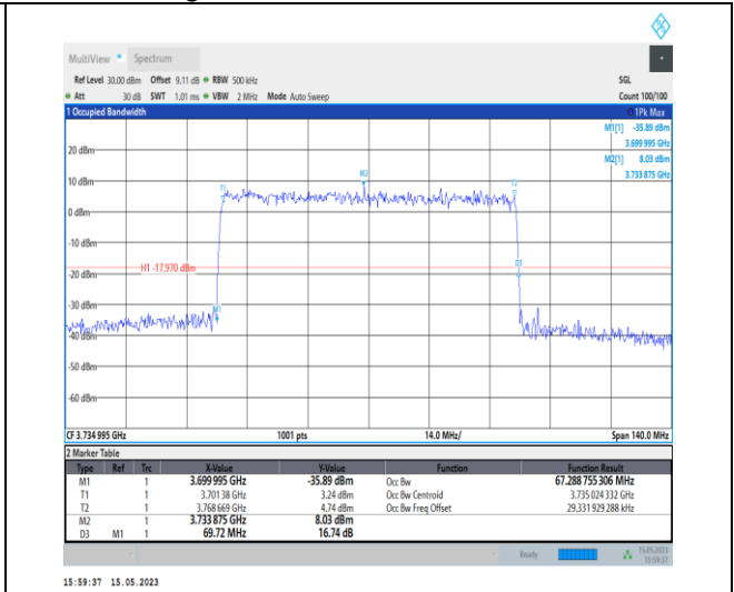
1-N77-3700-3980-PC1-30-70-L-9-CP-256QAM-Outer_Full-189@0-Ant0-67.289-69.720-≤70-PASS
