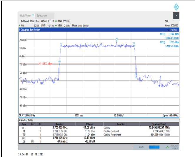
1-N77-3700-3980-PC1-30-50-L-2-DFT-PI2BPSK-Out er_Full-128@0-Ant0-45.645-47.600-≤50-PASS
