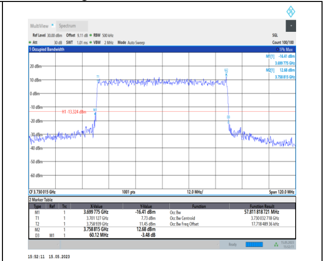
1-N77-3700-3980-PC1-30-60-L-8-CP-64QAM-Outer_Full-162@0-Ant0-57.812-60.120-≤60-PASS
