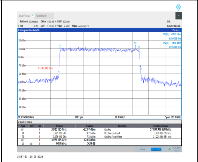
1-N77-3700-3980-PC1-30-60-H-8-CP-64QAM-Outer_Full-162@0-Ant0-57.834-60.000-≤60-PASS
