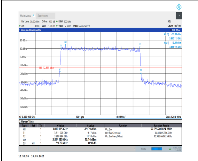
1-N77-3700-3980-PC1-30-60-M-4-DFT-64QAM-Out_Full-162@0-Ant0-57.955-59.760-≤60-PASS
