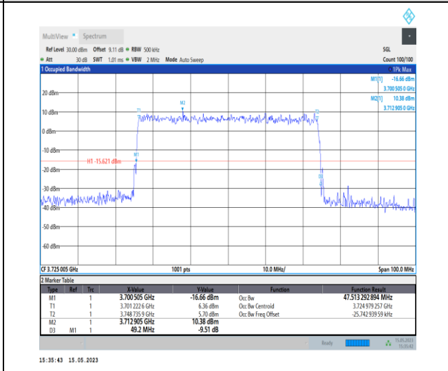
1-N77-3700-3980-PC1-30-50-L-9-CP-256QAM-Outer_Full-133@0-Ant0-47.513-49.200-≤50-PASS
