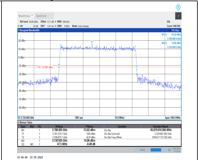
1-N77-3700-3980-PC1-30-50-L-3-DFT-16QAM-Out er_Full-128@0-Ant0-45.619-47.500-≤50-PASS
