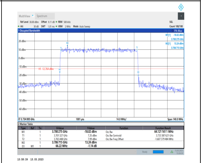
1-N77-3700-3980-PC1-30-70-L-3-DFT-16QAM-Outer_Full-180@0-Ant0-64.121-66.220-≤70-PASS
