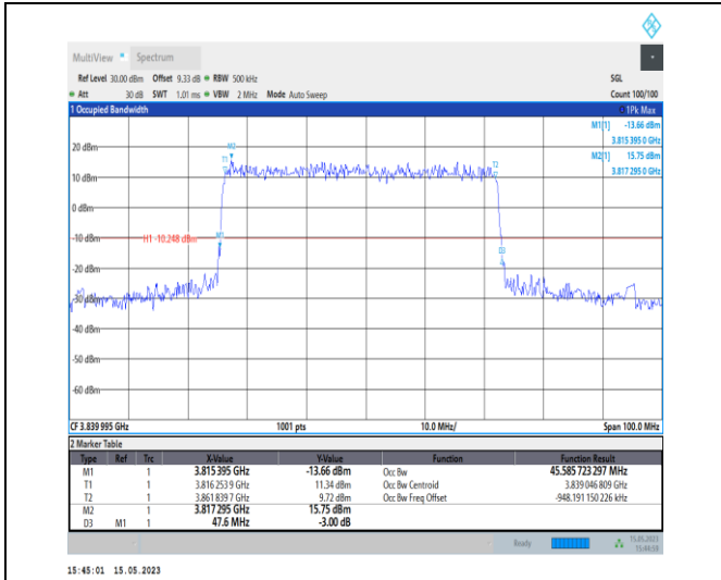
1-N77-3700-3980-PC1-30-50-M-1-DFT-QPSK-Outer_Full-128@0-Ant0-45.586-47.600-≤50-PASS
