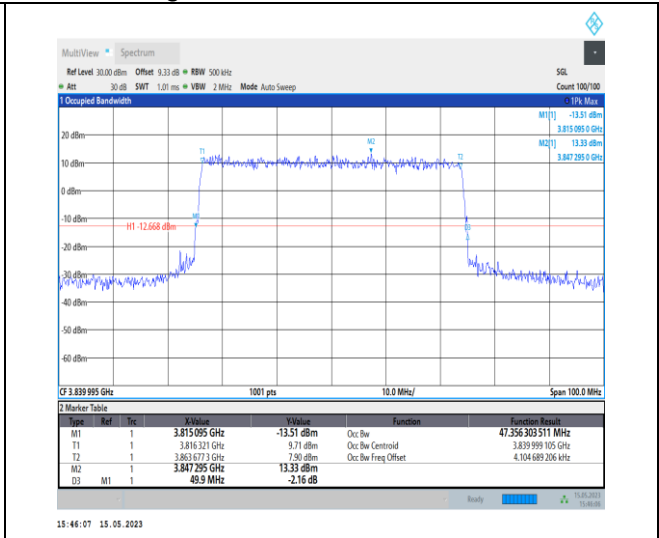
1-N77-3700-3980-PC1-30-50-M-6-CP-QPSK-Outer Full-133@0-Ant0-47.356-49.900-≤50-PASS
