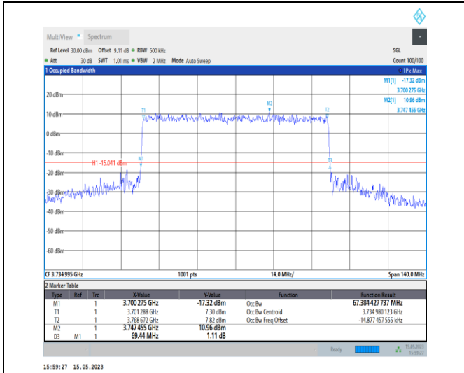
1-N77-3700-3980-PC1-30-70-L-8-CP-64QAM-Outer_Full-189@0-Ant0-67.384-69.440-≤70-PASS
