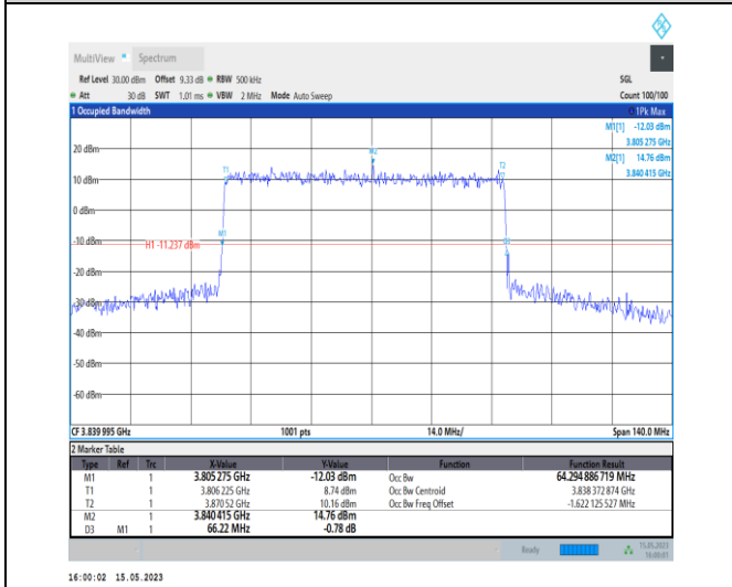
1-N77-3700-3980-PC1-30-70-M-1-DFT-QPSK-Outer_Full-180@0-Ant0-64.295-66.220-≤70-PASS
