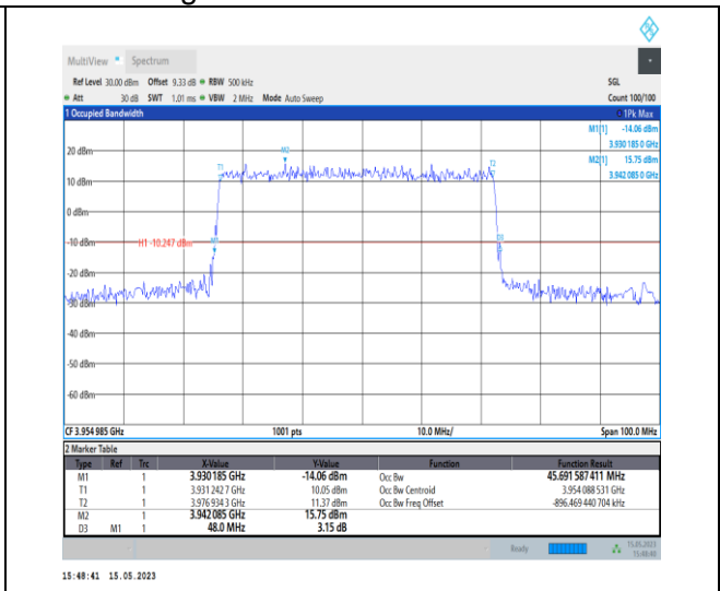
1-N77-3700-3980-PC1-30-50-H-1-DFT-QPSK-Outer_Full-128@0-Ant0-45.692-48.000-≤50-PASS
