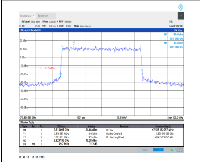
1-N77-3700-3980-PC1-30-50-M-7-CP-16QAM-Outer Full-133@0-Ant0-47.515-49.700-≤50-PASS
