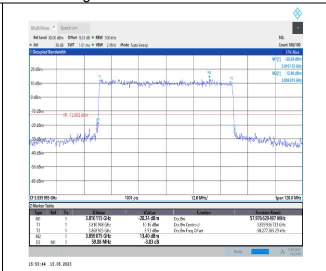
1-N77-3700-3980-PC1-30-60-M-3-DFT-16QAM-Out_Full-162@0-Ant0-57.977-59.880-≤60-PASS
