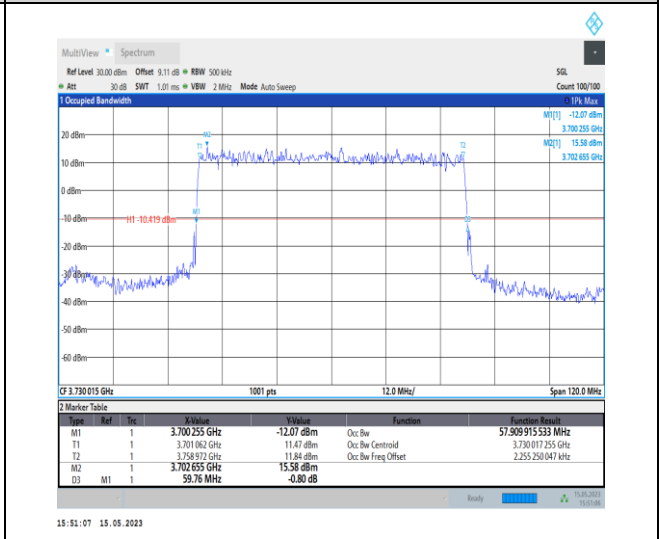
1-N77-3700-3980-PC1-30-60-L-2-DFT-PI2BPSK-Outer_Full-162@0-Ant0-57.91-59.760-≤60-PASS
