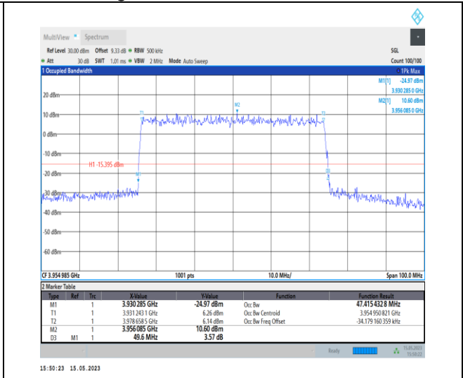
1-N77-3700-3980-PC1-30-50-H-9-CP-256QAM-Outer_Full-133@0-Ant0-47.415-49.600-≤50-PASS
