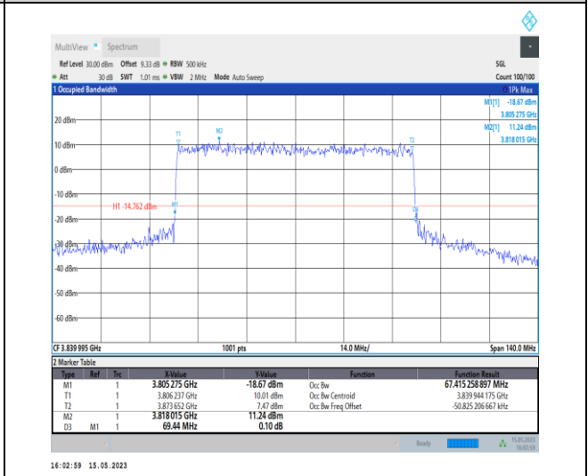
1-N77-3700-3980-PC1-30-70-M-6-CP-QPSK-Outer_Full-189@0-Ant0-67.415-69.440-≤70-PASS
