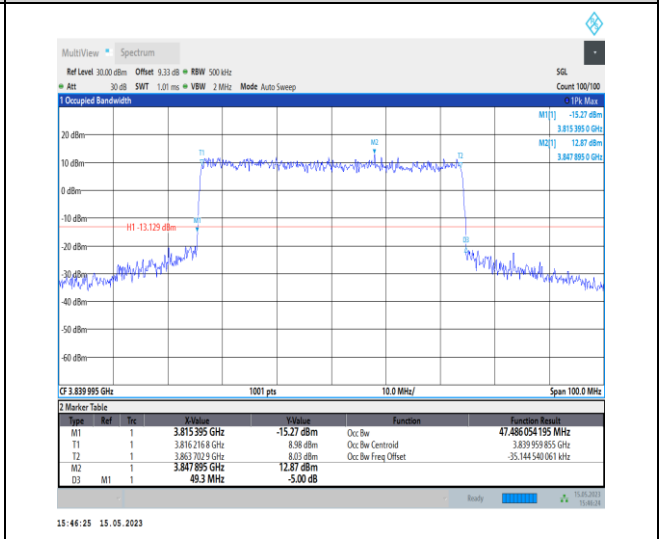
1-N77-3700-3980-PC1-30-50-M-8-CP-64QAM-Outer Full-133@0-Ant0-47.486-49.300-≤50-PASS
