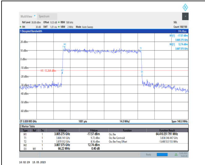
1-N77-3700-3980-PC1-30-70-M-3-DFT-16QAM-Outer_Full-180@0-Ant0-64.41-66.220-≤70-PASS
