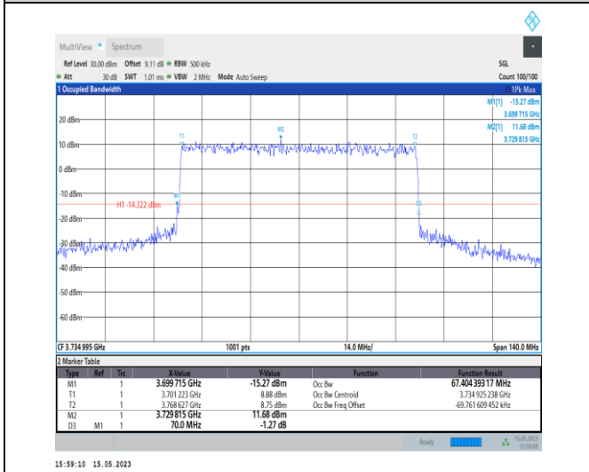
1-N77-3700-3980-PC1-30-70-L-6-CP-QPSK-Outer_Full-189@0-Ant0-67.404-70.000-≤70-PASS
