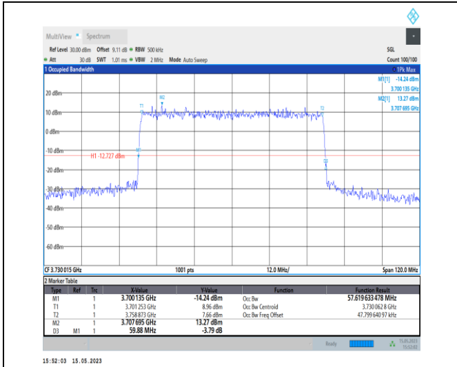
1-N77-3700-3980-PC1-30-60-L-7-CP-16QAM-Outer_Full-162@0-Ant0-57.62-59.880-≤60-PASS
