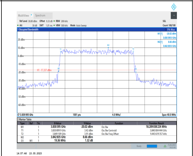
1-N77-3700-3980-PC1-30-20-M-9-CP-256QAM-Outer_Full-51@0-Ant0-18.209-19.360-≤20-PASS
