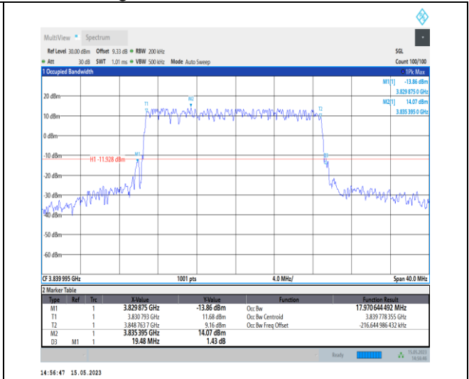
1-N77-3700-3980-PC1-30-20-M-3-DFT-16QAM-Outer_Full-50@0-Ant0-17.971-19.480-≤20-PASS
