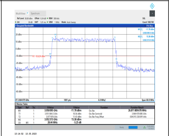
1-N77-3700-3980-PC1-30-30-H-1-DFT-QPSK-Outer_Full-75@0-Ant0-26.812-28.440-≤30-PASS
