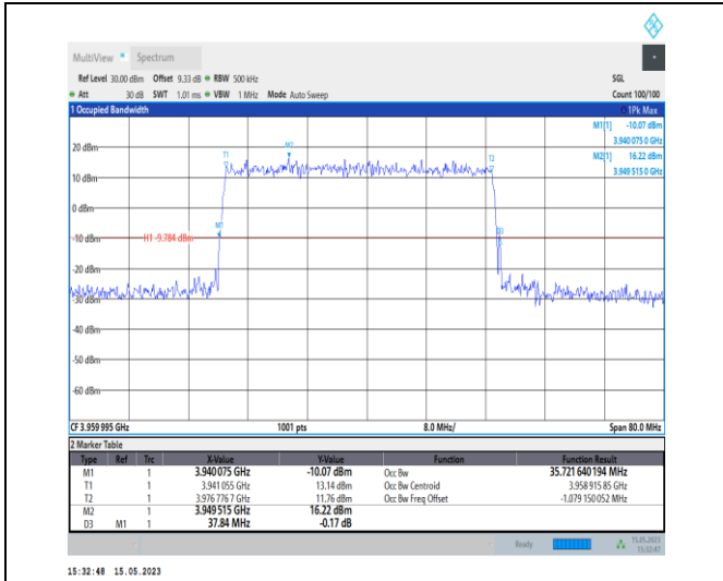
1-N77-3700-3980-PC1-30-40-H-3-DFT-16QAM-Outer_Full-100@0-Ant0-35.722-37.840-≤40-PASS
