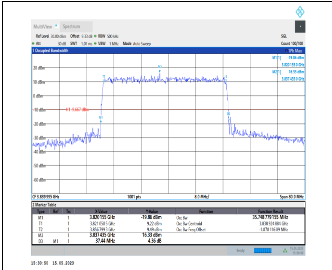
1-N77-3700-3980-PC1-30-40-M-4-DFT-64QAM-Outer_Full-100@0-Ant0-35.749-37.440-≤40-PASS
