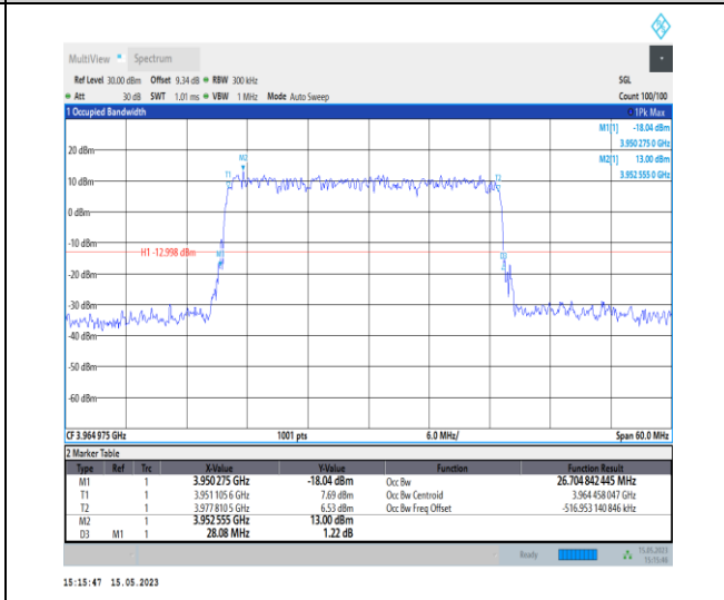
1-N77-3700-3980-PC1-30-30-H-5-DFT-256QAM-Out er_Full-75@0-Ant0-26.705-28.080-≤30-PASS
