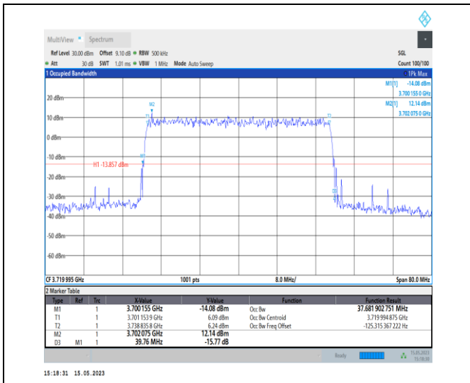
1-N77-3700-3980-PC1-30-40-L-9-CP-256QAM-Outer_Full-106@0-Ant0-37.682-39.760-≤40-PASS
