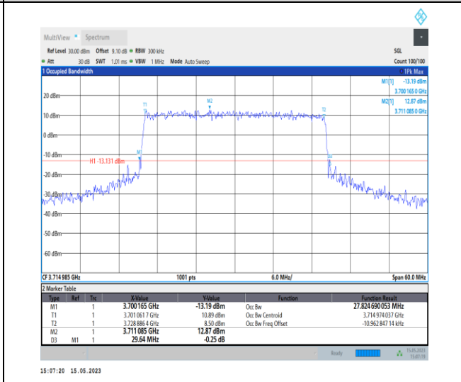
1-N77-3700-3980-PC1-30-30-L-7-CP-16QAM-Outer_Full-78@0-Ant0-27.825-29.640-≤30-PASS
