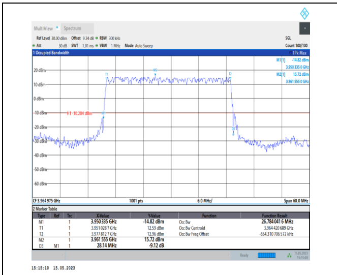
1-N77-3700-3980-PC1-30-30-H-2-DFT-PI2BPSK-Out er_Full-75@0-Ant0-26.784-28.140-≤30-PASS
