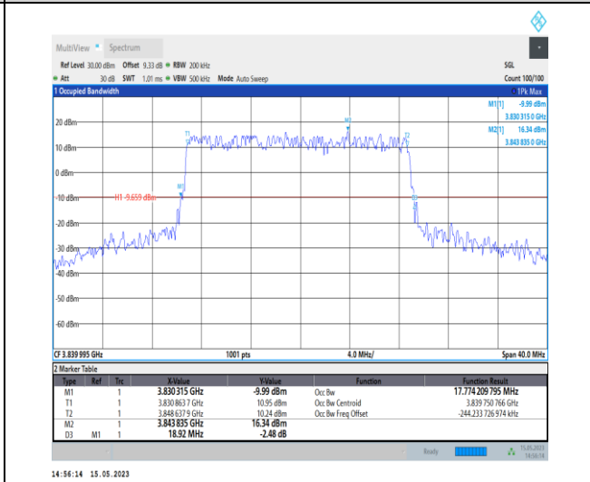
1-N77-3700-3980-PC1-30-20-M-1-DFT-QPSK-Outer_Full-50@0-Ant0-17.774-18.920-≤20-PASS
