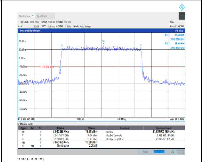
1-N77-3700-3980-PC1-30-40-H-6-CP-QPSK-Outer_Full-106@0-Ant0-37.835-39.440-≤40-PASS
