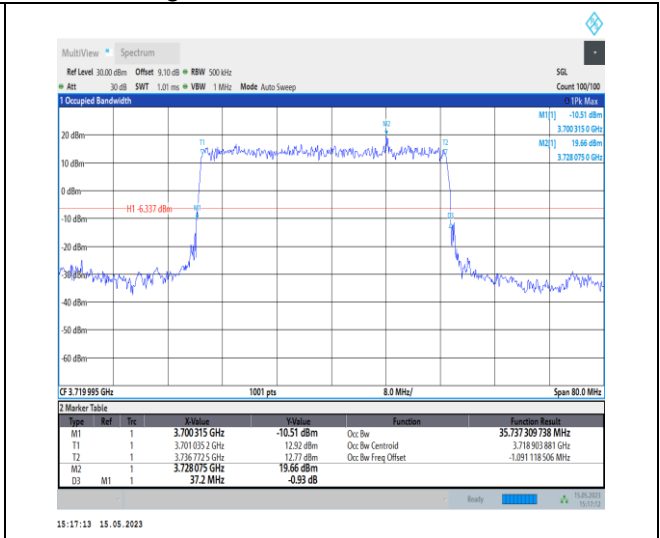
1-N77-3700-3980-PC1-30-40-L-2-DFT-PI2BPSK-Outer_Full-100@0-Ant0-35.737-37.200-≤40-PASS
