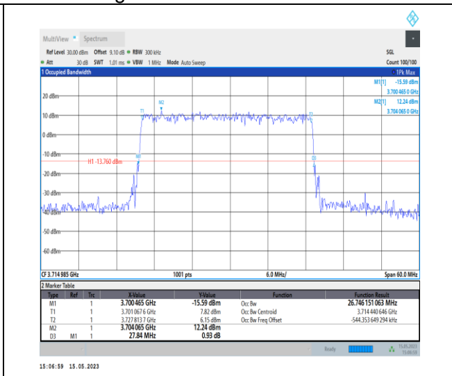
1-N77-3700-3980-PC1-30-30-L-5-DFT-256QAM-Outer_Full-75@0-Ant0-26.746-27.840-≤30-PASS
