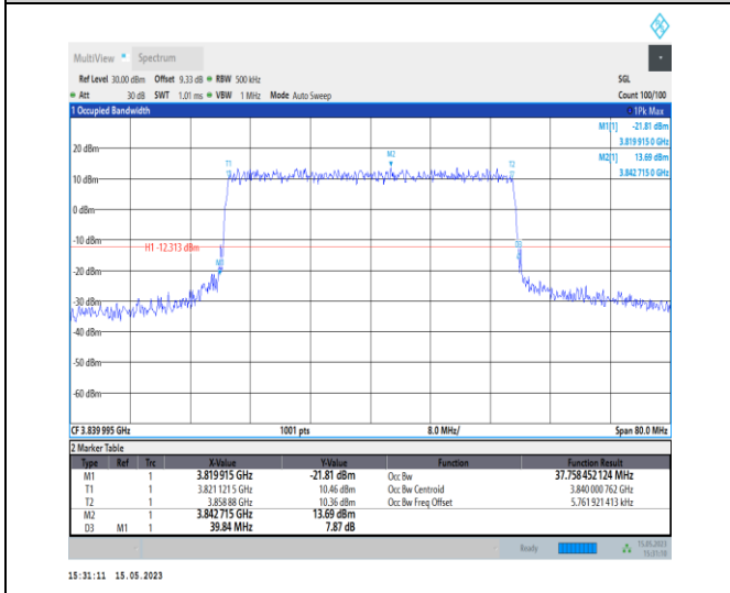
1-N77-3700-3980-PC1-30-40-M-6-CP-QPSK-Outer_Full-106@0-Ant0-37.758-39.840-≤40-PASS
