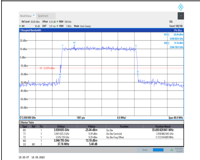
1-N77-3700-3980-PC1-30-40-H-5-DFT-256QAM-Outer_Full-100@0-Ant0-35.694-37.760-≤40-PASS
