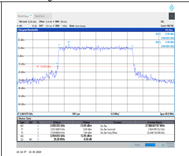
1-N77-3700-3980-PC1-30-30-H-7-CP-16QAM-Outer_Full-78@0-Ant0-27.881-29.280-≤30-PASS
