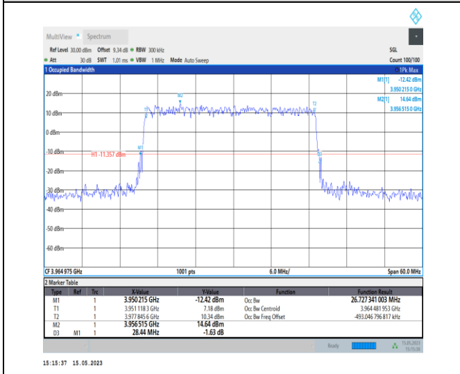
1-N77-3700-3980-PC1-30-30-H-4-DFT-64QAM-Out er_Full-75@0-Ant0-26.727-28.440-≤30-PASS
