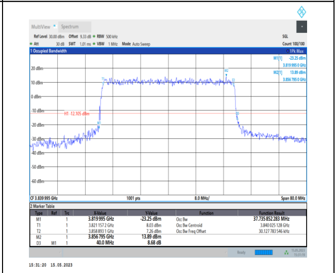
1-N77-3700-3980-PC1-30-40-M-7-CP-16QAM-Outer_Full-106@0-Ant0-37.736-40.000-≤40-PASS
