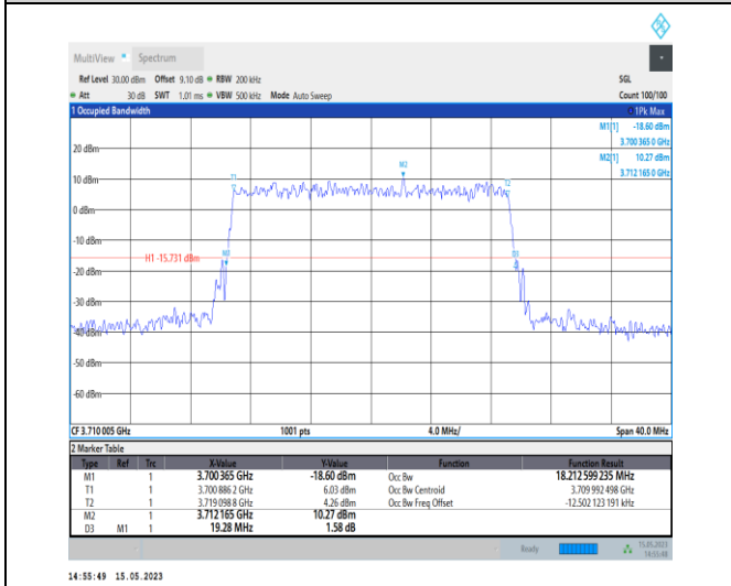
1-N77-3700-3980-PC1-30-20-L-9-CP-256QAM-Outer_Full-51@0-Ant0-18.213-19.280-≤20-PASS
