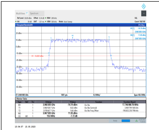
1-N77-3700-3980-PC1-30-20-H-5-DFT-256QAM-Outer_Full-50@0-Ant0-17.747-19.000-≤20-PASS
