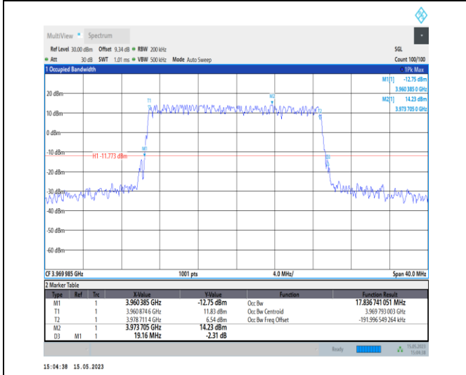
1-N77-3700-3980-PC1-30-20-H-3-DFT-16QAM-Outer_Full-50@0-Ant0-17.837-19.160-≤20-PASS
