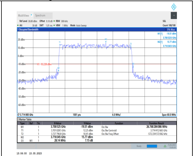
1-N77-3700-3980-PC1-30-30-L-1-DFT-QPSK-Outer_Full-75@0-Ant0-26.768-28.140-≤30-PASS
