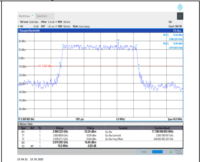
1-N77-3700-3980-PC1-30-20-H-2-DFT-PI2BPSK-Outer_Full-50@0-Ant0-17.78-19.000-≤20-PASS
