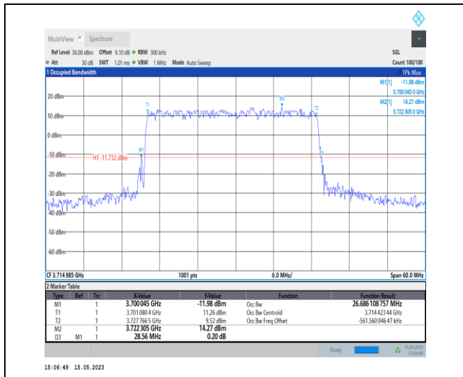
1-N77-3700-3980-PC1-30-30-L-4-DFT-64QAM-Outer_Full-75@0-Ant0-26.686-28.560-≤30-PASS
