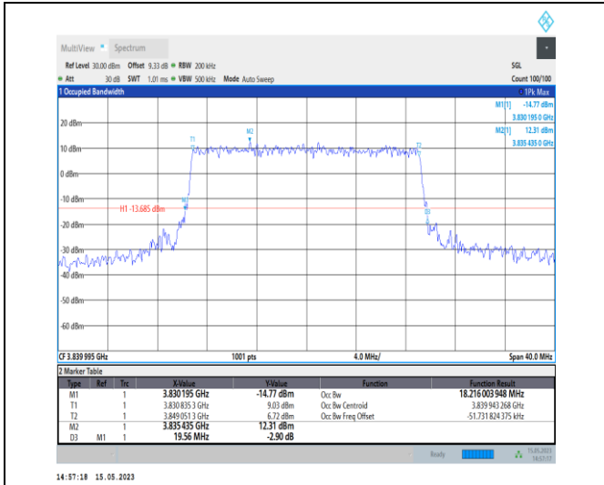
1-N77-3700-3980-PC1-30-20-M-6-CP-QPSK-Outer_Full-51@0-Ant0-18.216-19.560-≤20-PASS
