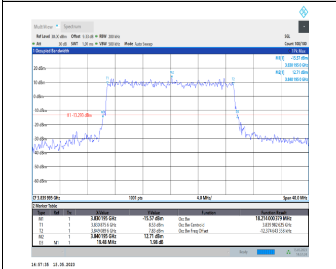
1-N77-3700-3980-PC1-30-20-M-8-CP-64QAM-Outer_Full-51@0-Ant0-18.214-19.480-≤20-PASS
