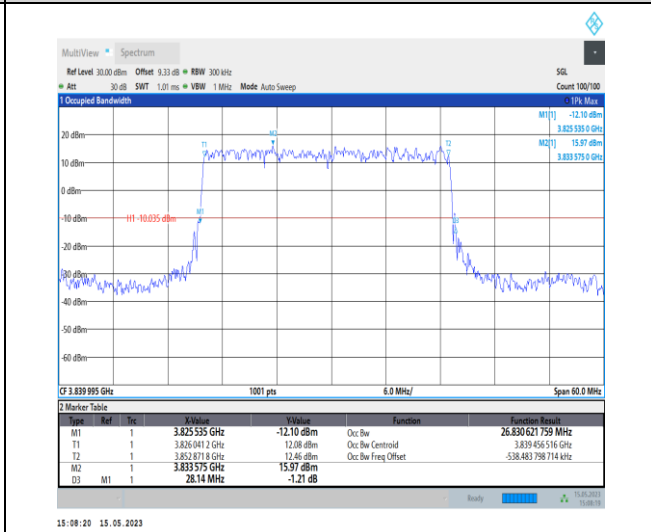
1-N77-3700-3980-PC1-30-30-M-2-DFT-PI2BPSK-Outer_Full-75@0-Ant0-26.831-28.140-≤30-PASS
