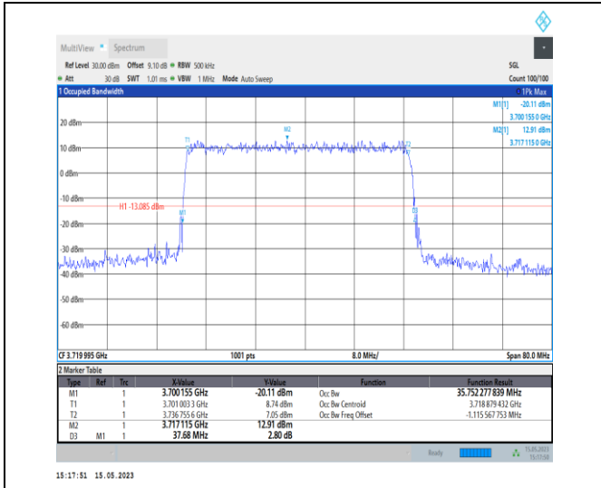
1-N77-3700-3980-PC1-30-40-L-5-DFT-256QAM-Out er_Full-100@0-Ant0-35.752-37.680-≤40-PASS
