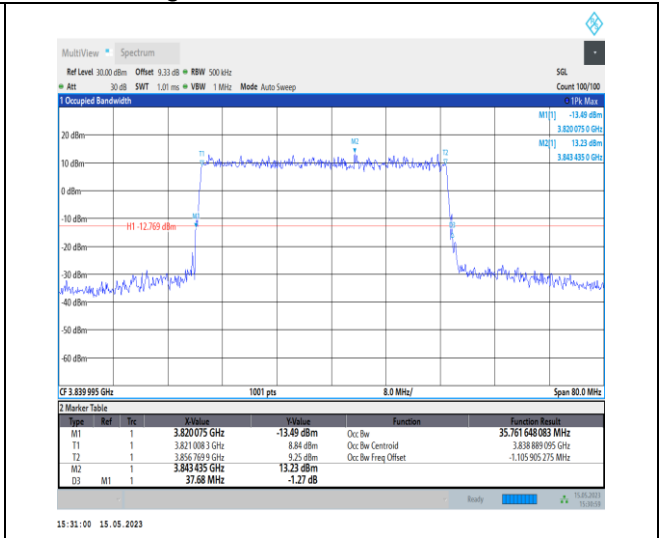
1-N77-3700-3980-PC1-30-40-M-5-DFT-256QAM-Outer_Full-100@0-Ant0-35.762-37.680-≤40-PASS
