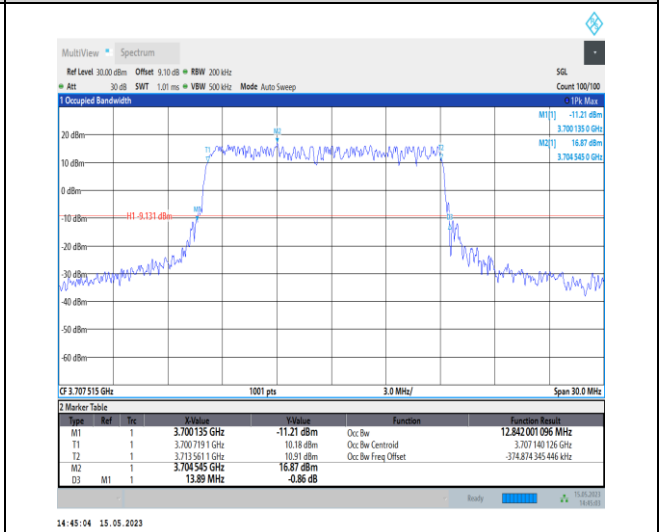
1-N77-3700-3980-PC1-30-15-L-1-DFT-QPSK-Outer _Full-36@0-Ant0-12.842-13.890-≤15-PASS
