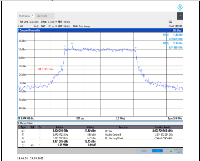
1-N77-3700-3980-PC1-30-10-H-8-CP-64QAM-Outer _Full-24@0-Ant0-8.601-9.380-≤10-PASS
