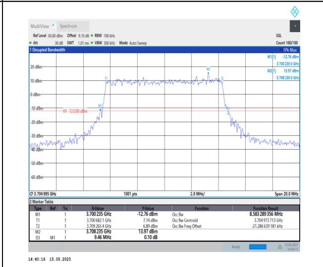
1-N77-3700-3980-PC1-30-10-L-8-CP-64QAM-Outer_Full-24@0-Ant0-8.583-9.460-≤10-PASS
