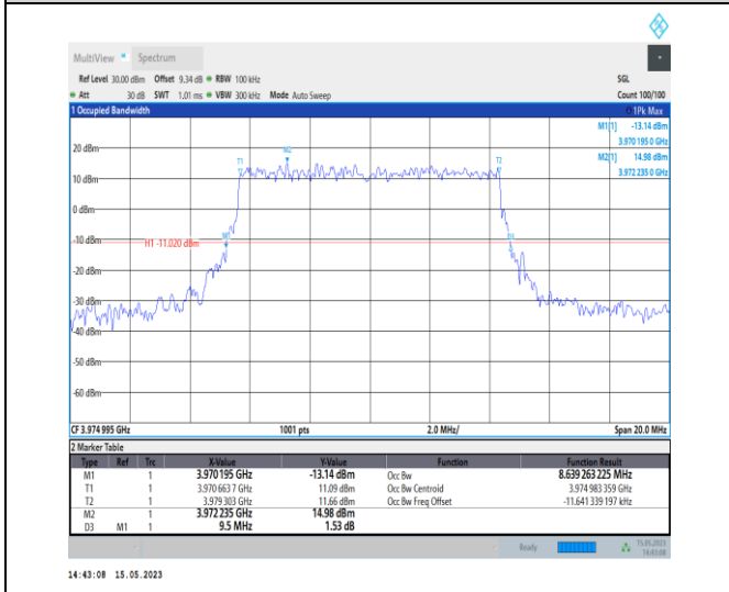
1-N77-3700-3980-PC1-30-10-H-1-DFT-QPSK-Outer_Full-24@0-Ant0-8.639-9.500-≤10-PASS
