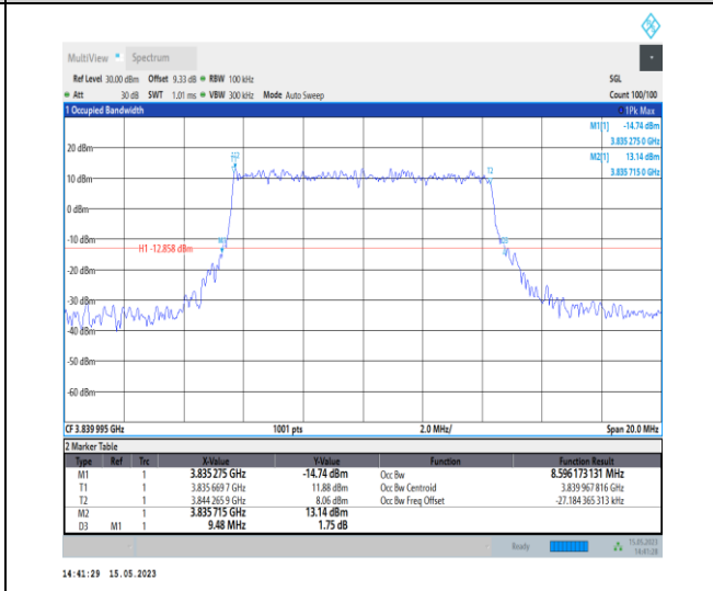
1-N77-3700-3980-PC1-30-10-M-3-DFT-16QAM-Outer_Full-24@0-Ant0-8.596-9.480-≤10-PASS
