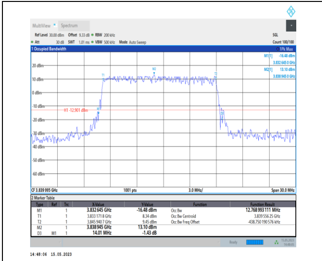
1-N77-3700-3980-PC1-30-15-M-5-DFT-256QAM-Out _Full-36@0-Ant0-12.769-14.010-≤15-PASS
