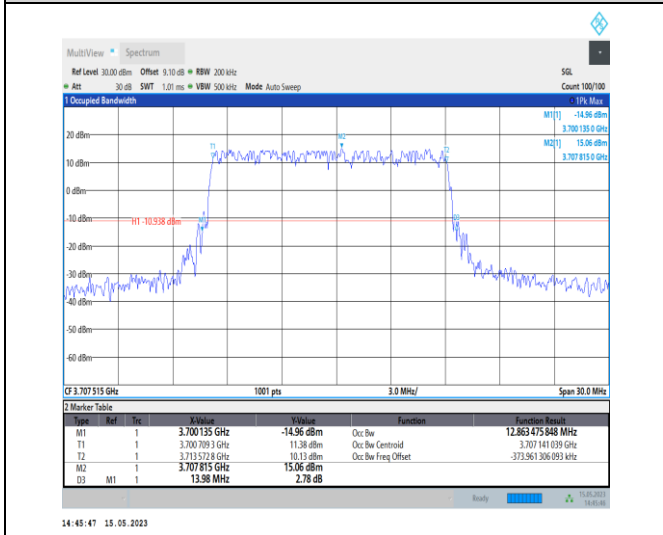
1-N77-3700-3980-PC1-30-15-L-4-DFT-64QAM-Outer_Full-36@0-Ant0-12.863-13.980-≤15-PASS
