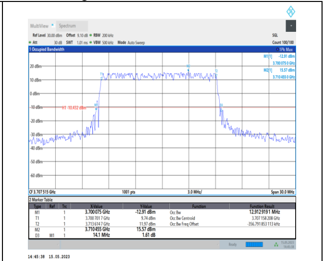
1-N77-3700-3980-PC1-30-15-L-3-DFT-16QAM-Out er_Full-36@0-Ant0-12.913-14.100-≤15-PASS
