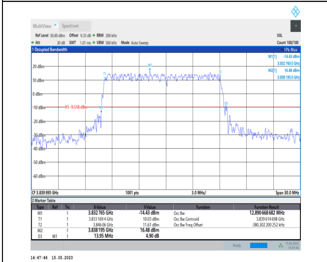
1-N77-3700-3980-PC1-30-15-M-3-DFT-16QAM-Outer_Full-36@0-Ant0-12.891-13.950-≤15-PASS
