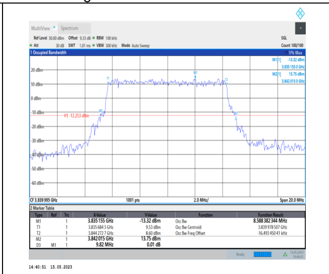
1-N77-3700-3980-PC1-30-10-M-1-DFT-QPSK-Outer_Full-24@0-Ant0-8.588-9.820-≤10-PASS
