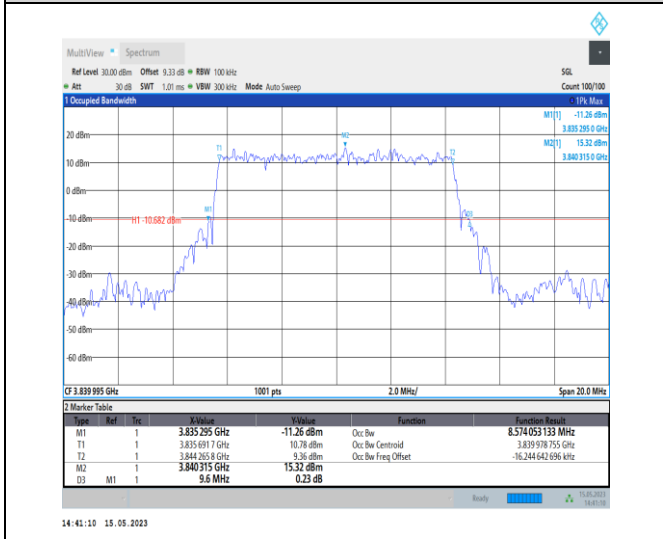
1-N77-3700-3980-PC1-30-10-M-2-DFT-PI2BPSK-Outer_Full-24@0-Ant0-8.574-9.600-≤10-PASS
