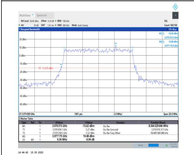
1-N77-3700-3980-PC1-30-10-H-9-CP-256QAM-Outer _Full-24@0-Ant0-8.564-9.340-≤10-PASS
