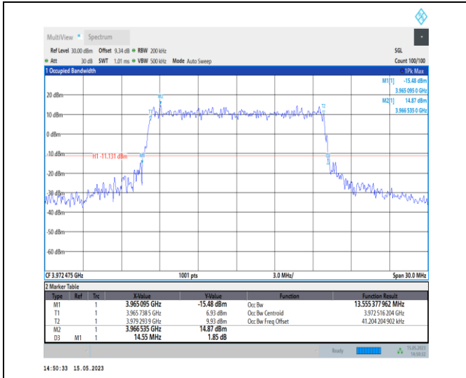
1-N77-3700-3980-PC1-30-15-H-8-CP-64QAM-Outer_Full-38@0-Ant0-13.555-14.550-≤15-PASS
