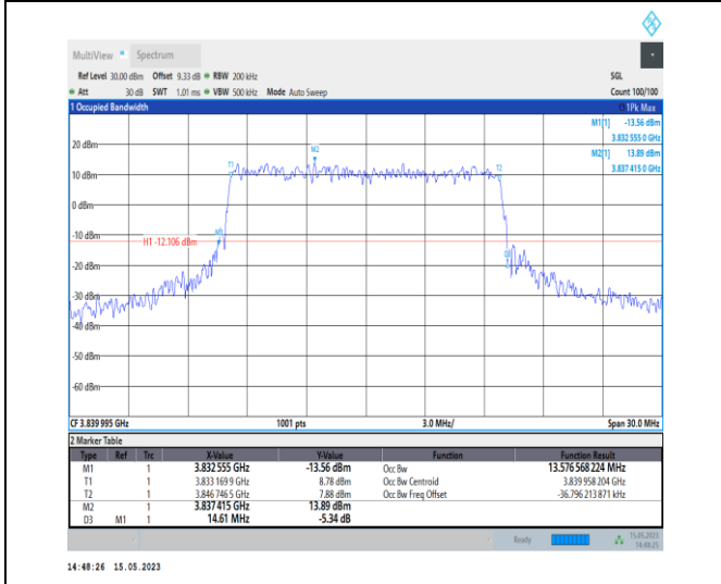
1-N77-3700-3980-PC1-30-15-M-7-CP-16QAM-Outer _Full-38@0-Ant0-13.577-14.610-≤15-PASS
