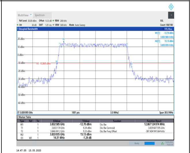
1-N77-3700-3980-PC1-30-15-M-4-DFT-64QAM-Outer_Full-36@0-Ant0-12.867-14.310-≤15-PASS
