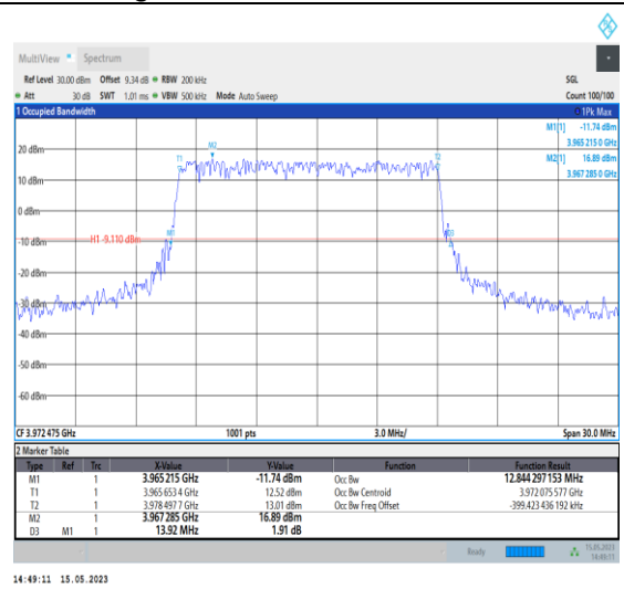
1-N77-3700-3980-PC1-30-15-H-1-DFT-QPSK-Outer_Full-36@0-Ant0-12.844-13.920-≤15-PASS
