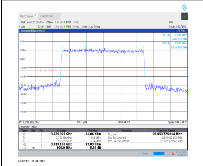
1-N77-3700-3980--30-100-M-4-DFT-64QAM-Outer_Full-270@0-Ant0-96.054-100.000-≤100-PASS
