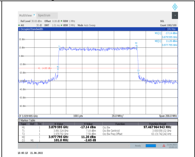
1-N77-3700-3980--30-100-H-6-CP-QPSK-Outer_Full-273@0-Ant0-97.468-101.000-≤100-PASS
