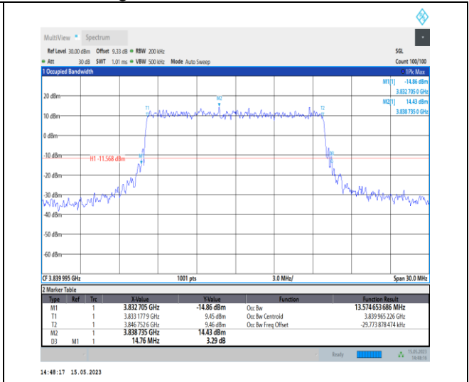
1-N77-3700-3980-PC1-30-15-M-6-CP-QPSK-Outer _Full-38@0-Ant0-13.575-14.760-≤15-PASS
