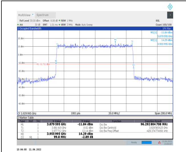
1-N77-3700-3980--30-100-H-1-DFT-QPSK-Outer_Fu II-270@0-Ant0-96.293-99.800-≤100-PASS
