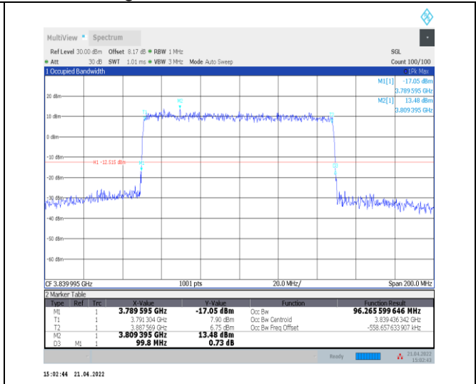
1-N77-3700-3980--30-100-M-3-DFT-16QAM-Outer_Full-270@0-Ant0-96.266-99.800-≤100-PASS
