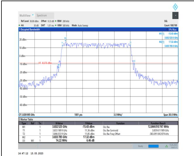
1-N77-3700-3980-PC1-30-15-M-1-DFT-QPSK-Outer_Full-36@0-Ant0-12.844-14.220-≤15-PASS
