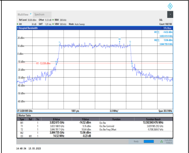
1-N77-3700-3980-PC1-30-15-M-8-CP-64QAM-Outer _Full-38@0-Ant0-13.593-14.520-≤15-PASS
