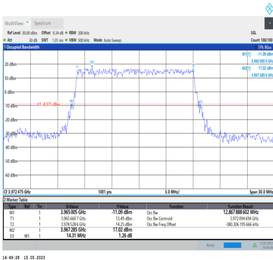
1-N77-3700-3980-PC1-30-15-H-2-DFT-PI2BPSK-Outer_Full-36@0-Ant0-12.868-14.310-≤15-PASS
