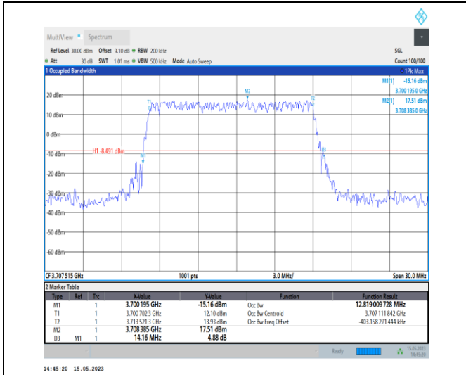
1-N77-3700-3980-PC1-30-15-L-2-DFT-PI2BPSK-Out er_Full-36@0-Ant0-12.819-14.160-≤15-PASS
