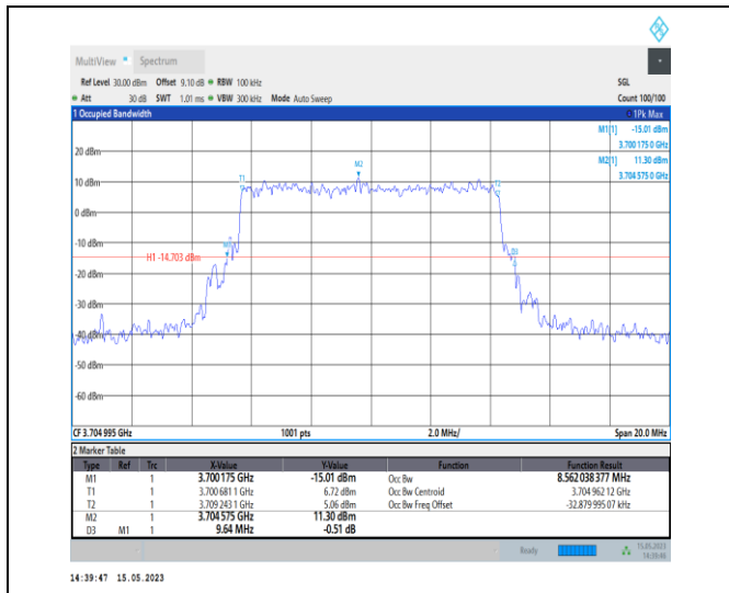
1-N77-3700-3980-PC1-30-10-L-5-DFT-256QAM-Out er_Full-24@0-Ant0-8.562-9.640-≤10-PASS
