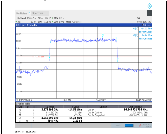
1-N77-3700-3980--30-100-H-2-DFT-PI2BPSK-Outer_Full-270@0-Ant0-96.35-99.800-≤100-PASS
