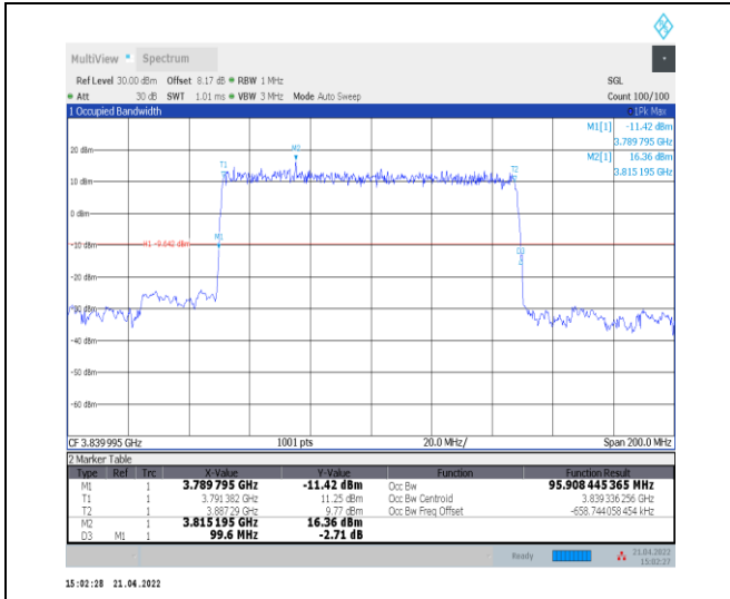
1-N77-3700-3980--30-100-M-2-DFT-PI2BPSK-Outer_Full-270@0-Ant0-95.908-99.600-≤100-PASS
