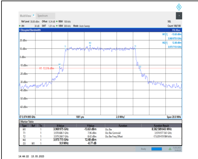
1-N77-3700-3980-PC1-30-10-H-7-CP-16QAM-Outer _Full-24@0-Ant0-8.583-9.900-≤10-PASS
