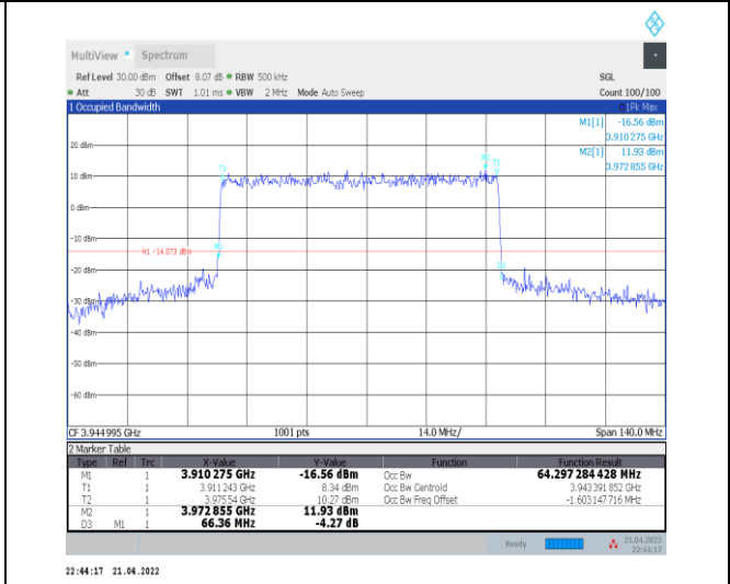
1-N77-3700-3980--30-70-H-1-DFT-QPSK-Outer_Full -180@0-Ant0-64.297-66.360-≤70-PASS
