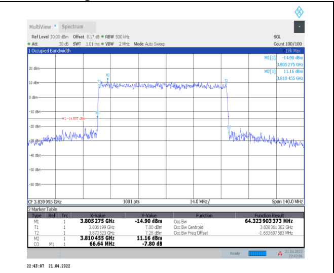
1-N77-3700-3980--30-70-M-4-DFT-64QAM-Outer_Full-180@0-Ant0-64.324-66.640-≤70-PASS
