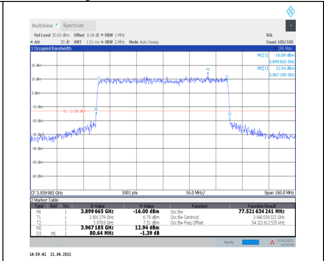
1-N77-3700-3980--30-80-H-8-CP-64QAM-Outer_Full -217@0-Ant0-77.522-80.640-<80-PASS
