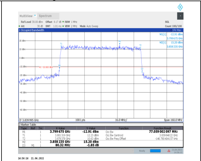
1-N77-3700-3980--30-80-M-1-DFT-QPSK-Outer_Full -216@0-Ant0-77.059-80.320-<math>\leq 80</math>-PASS
