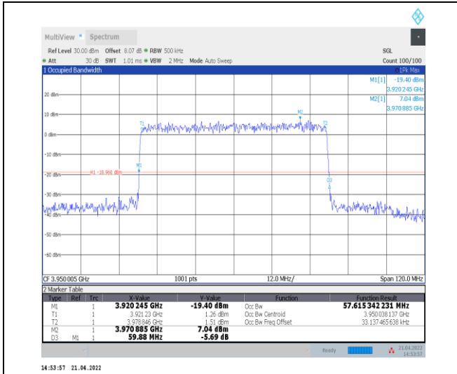
1-N77-3700-3980--30-60-H-9-CP-256QAM-Outer_Full-162@0-Ant0-57.615-59.880-≤60-PASS
