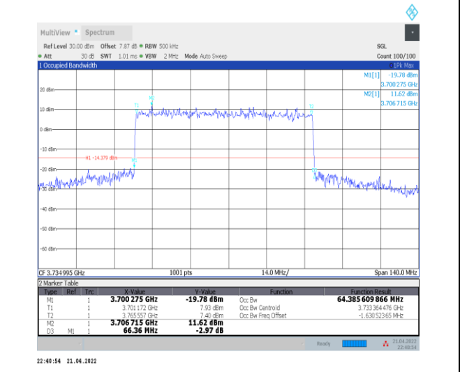
1-N77-3700-3980--30-70-L-3-DFT-16QAM-Outer_Full-180@0-Ant0-64.386-66.360-≤70-PASS
