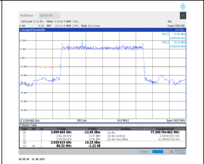
1-N77-3700-3980--30-80-H-2-DFT-PI2BPSK-Outer_Full-I-216@0-Ant0-77.301-80.320-<math>\leq 80</math>-PASS
