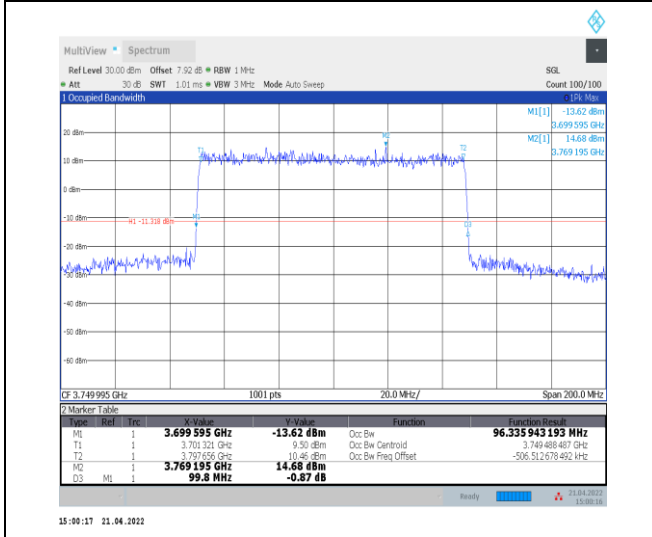
1-N77-3700-3980--30-100-L-1-DFT-QPSK-Outer_Fu ll-270@0-Ant0-96.336-99.800-<=100-PASS
