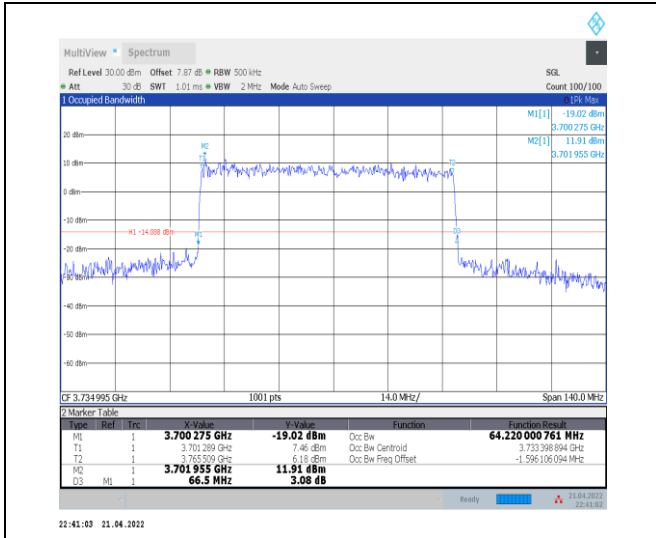
1-N77-3700-3980--30-70-L-4-DFT-64QAM-Outer_Fu II-180@0-Ant0-64.22-66.500-<=70-PASS
