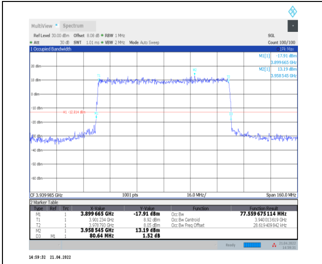
1-N77-3700-3980--30-80-H-7-CP-16QAM-Outer_Full -217@0-Ant0-77.56-80.640-<80-PASS
