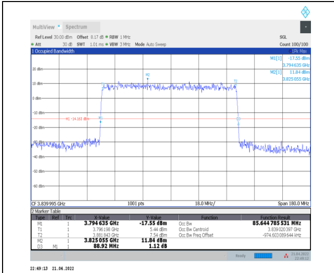
1-N77-3700-3980--30-90-M-5-DFT-256QAM-Outer_Full-240@0-Ant0-85.645-88.920<=90-PASS
