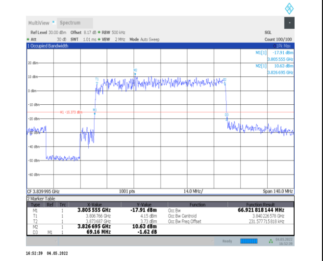
1-N77-3700-3980--30-70-M-6-CP-QPSK-Outer_Full-189@0-Ant0-66.922-69.160-≤70-PASS
