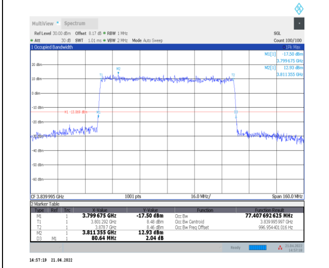
1-N77-3700-3980--30-80-M-6-CP-QPSK-Outer_Full-217@0-Ant0-77.408-80.640-≤80-PASS
