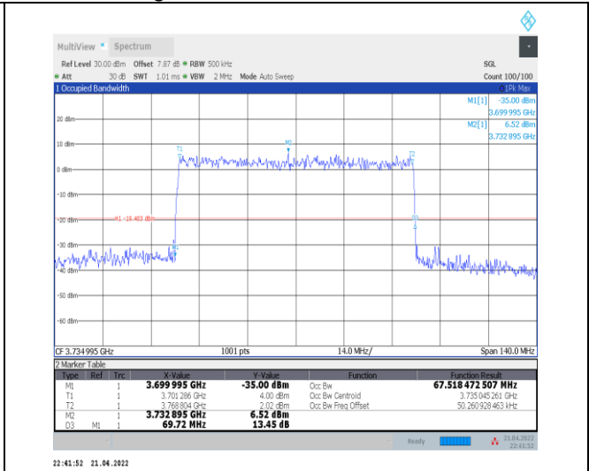
1-N77-3700-3980--30-70-L-9-CP-256QAM-Outer_Ful I-189@0-Ant0-67.518-69.720-≤70-PASS
