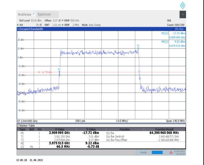
1-N77-3700-3980--30-70-H-5-DFT-256QAM-Outer_Full-180@0-Ant0-64.391-66.500-≤70-PASS
