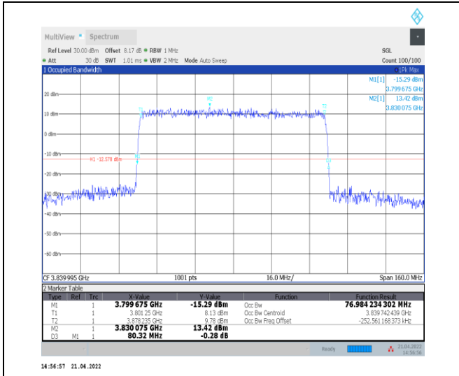
1-N77-3700-3980--30-80-M-4-DFT-64QAM-Outer_Full-216@0-Ant0-76.984-80.320-≤80-PASS
