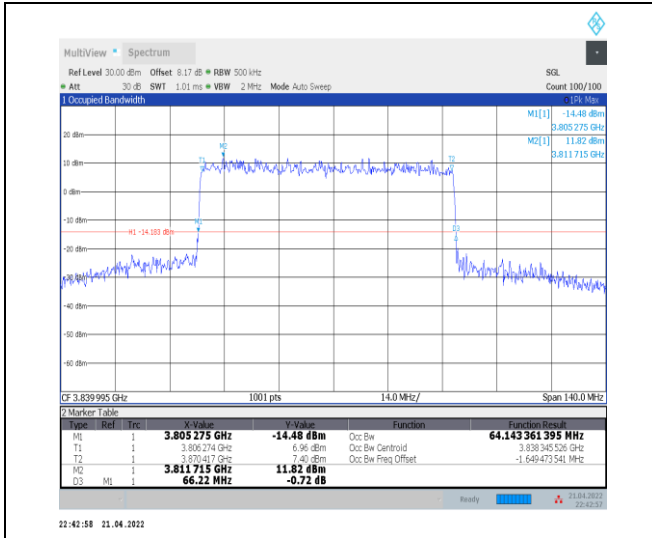
1-N77-3700-3980--30-70-M-3-DFT-16QAM-Outer_Full-180@0-Ant0-64.143-66.220-≤70-PASS
