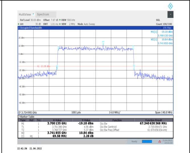
1-N77-3700-3980--30-70-L-7-CP-16QAM-Outer_Full-189@0-Ant0-67.341-69.580-<=70-PASS
