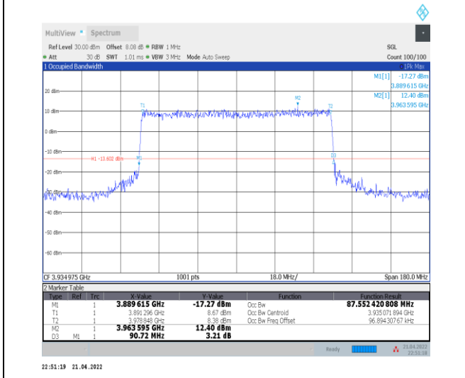
1-N77-3700-3980--30-90-H-6-CP-QPSK-Outer_Full-245@0-Ant0-87.552-90.720-≤90-PASS
