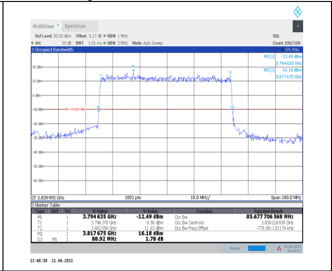
1-N77-3700-3980--30-90-M-2-DFT-PI2BPSK-Outer_Full Full-240@0-Ant0-85.678-88.920-≤90-PASS
