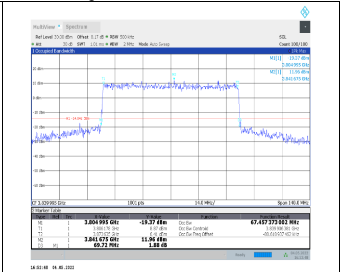
1-N77-3700-3980--30-70-M-8-CP-64QAM-Outer_Full -189@0-Ant0-67.457-69.720-≤70-PASS
