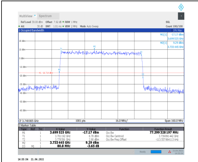
1-N77-3700-3980--30-80-L-9-CP-256QAM-Outer_Fu II-217@0-Ant0-77.399-80.800-<math>\leq 80</math>-PASS
