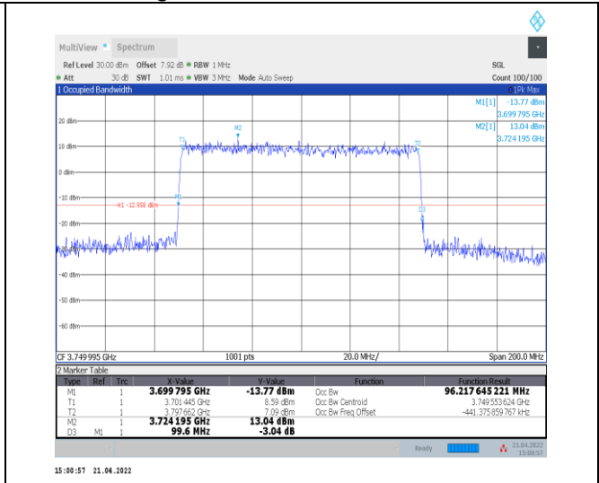
1-N77-3700-3980--30-100-L-4-DFT-64QAM-Outer_Full-270@0-Ant0-96.218-99.600-≤100-PASS
