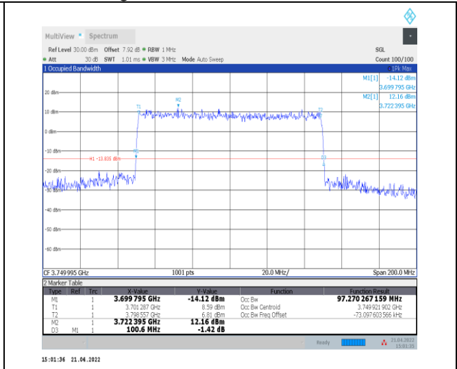
1-N77-3700-3980--30-100-L-8-CP-64QAM-Outer_Ful l-273@0-Ant0-97.27-100.600-≤100-PASS
