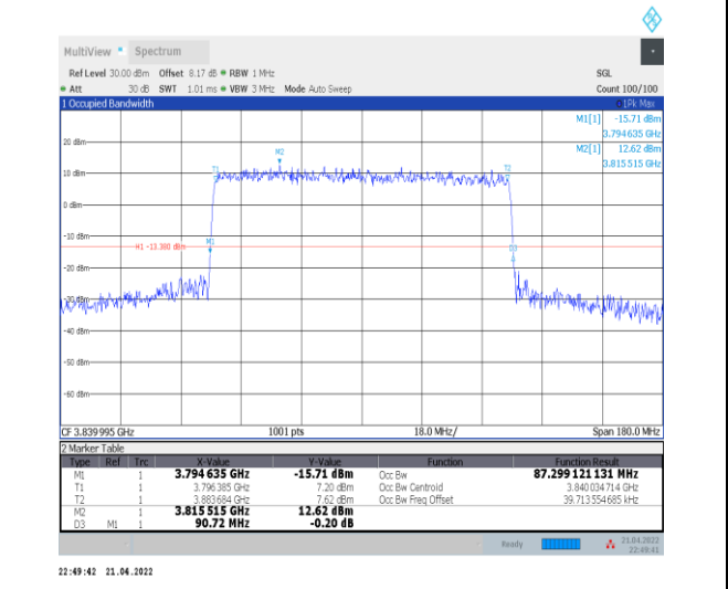
1-N77-3700-3980--30-90-M-8-CP-64QAM-Outer_Full-245@0-Ant0-87.299-90.720<=90-PASS
