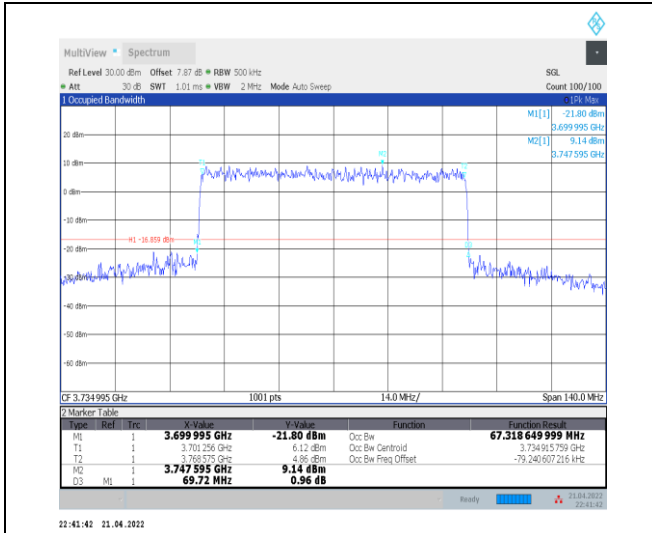
1-N77-3700-3980--30-70-L-8-CP-64QAM-Outer_Full -189@0-Ant0-67.319-69.720-≤70-PASS
