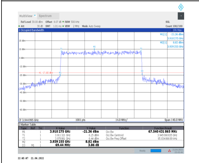
1-N77-3700-3980--30-70-H-8-CP-64QAM-Outer_Full-189@0-Ant0-67.54-69.440-<=70-PASS
