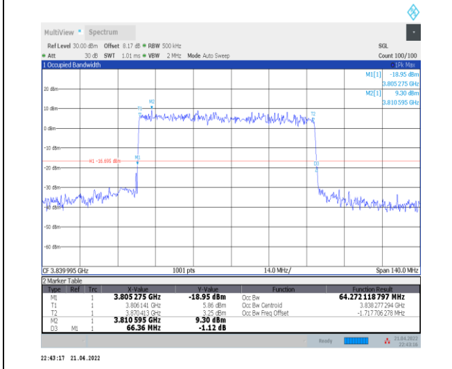
1-N77-3700-3980--30-70-M-5-DFT-256QAM-Outer_Full-180@0-Ant0-64.272-66.360-≤70-PASS
