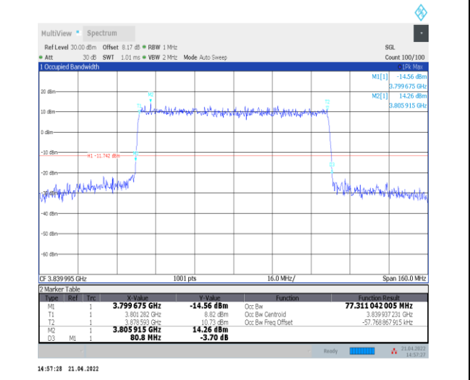
1-N77-3700-3980--30-80-M-7-CP-16QAM-Outer_Full-217@0-Ant0-77.311-80.800-≤80-PASS
