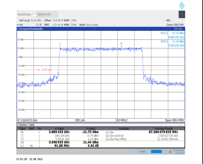
1-N77-3700-3980--30-90-H-7-CP-16QAM-Outer_Full-245@0-Ant0-87.566-91.080-≤90-PASS
