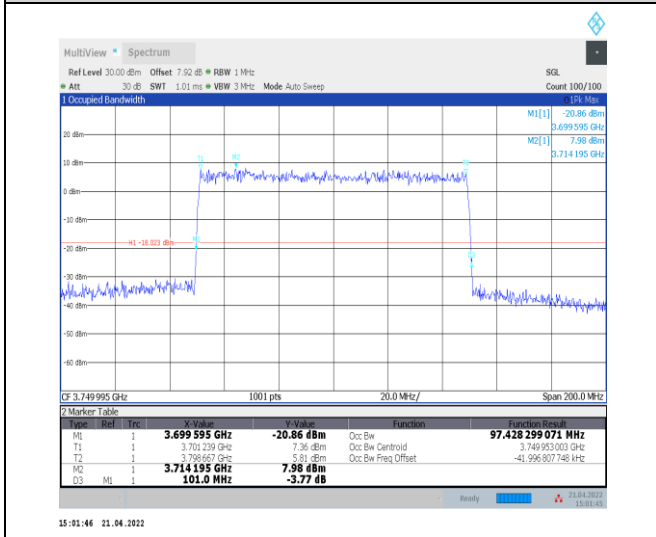
1-N77-3700-3980--30-100-L-9-CP-256QAM-Outer_F ull-273@0-Ant0-97.428-101.000-≤100-PASS
