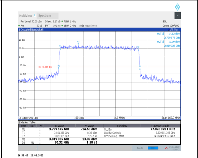
1-N77-3700-3980--30-80-M-3-DFT-16QAM-Outer_Fu II-216@0-Ant0-77.027-80.320-<math>\leq 80</math>-PASS
