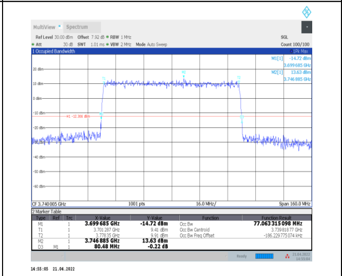
1-N77-3700-3980--30-80-L-4-DFT-64QAM-Outer_Full-216@0-Ant0-77.063-80.480-≤80-PASS
