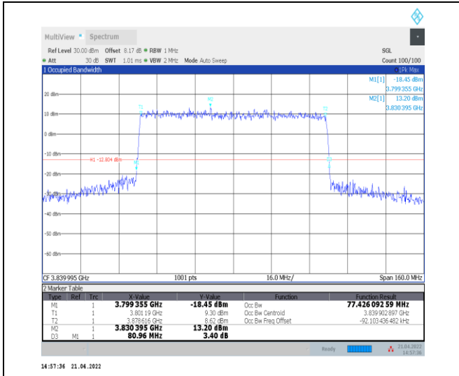
1-N77-3700-3980--30-80-M-8-CP-64QAM-Outer_Full-I-217@0-Ant0-77.426-80.960-<math>\leq 80</math>-PASS
