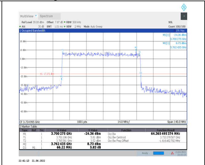
1-N77-3700-3980--30-70-L-5-DFT-256QAM-Outer_Full-180@0-Ant0-64.365-66.220-<=70-PASS
