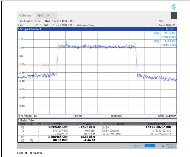
1-N77-3700-3980--30-80-L-1-DFT-QPSK-Outer_Full -216@0-Ant0-77.195-80.320-≤80-PASS
