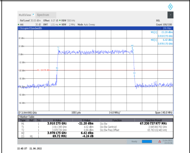
1-N77-3700-3980--30-70-H-9-CP-256QAM-Outer_Fu ll-189@0-Ant0-67.331-69.720-<=70-PASS
