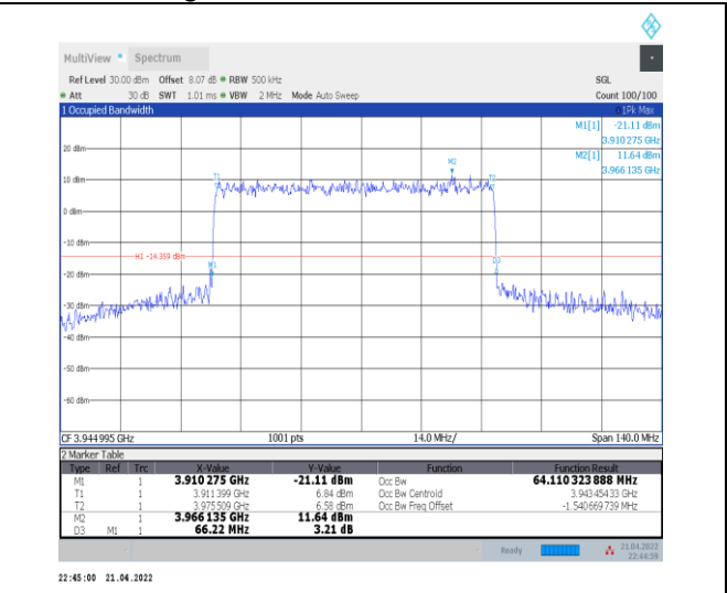
1-N77-3700-3980--30-70-H-3-DFT-16QAM-Outer_Fu II-180@0-Ant0-64.11-66.220-≤70-PASS
