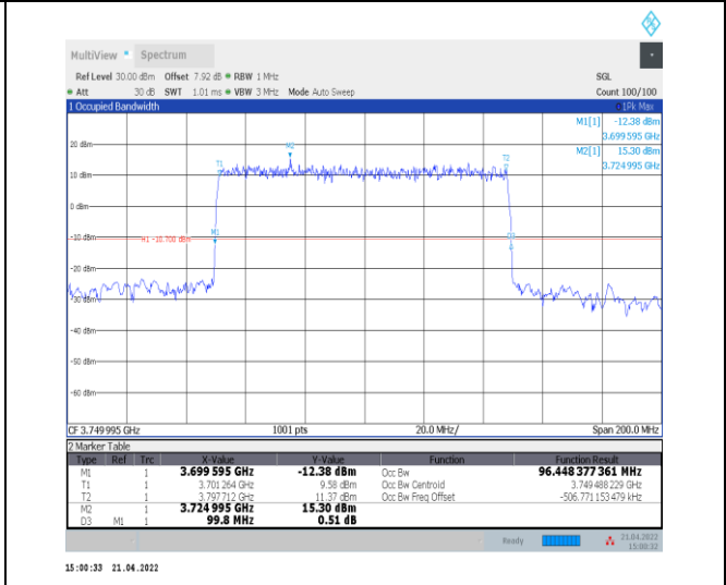
1-N77-3700-3980--30-100-L-2-DFT-Pl2BPSK-Outer_Full-270@0-Ant0-96.448-99.800-<=100-PASS
