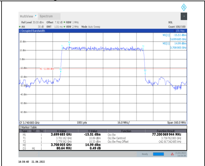
1-N77-3700-3980--30-80-L-2-DFT-PI2BPSK-Outer_Full-216@0-Ant0-77.2-80.640-≤80-PASS
