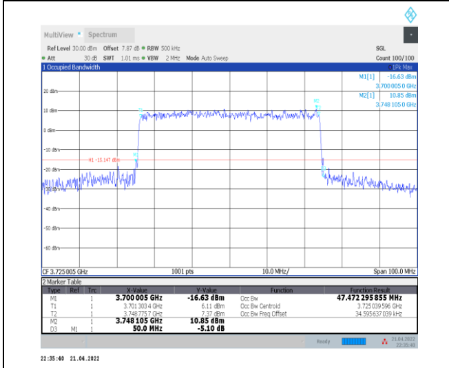
1-N77-3700-3980--30-50-L-8-CP-64QAM-Outer_Full-133@0-Ant0-47.472-50.000-<math>\leq 50</math>-PASS
