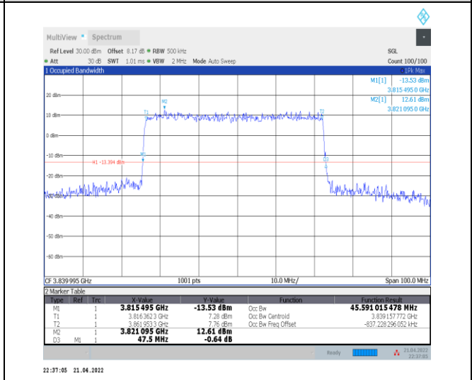
1-N77-3700-3980--30-50-M-4-DFT-64QAM-Outer_Full Full-128@0-Ant0-45.591-47.500-≤50-PASS
