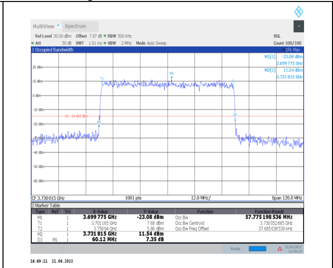
1-N77-3700-3980--30-60-L-4-DFT-64QAM-Outer_Ful I-162@0-Ant0-57.775-60.120-≤60-PASS
