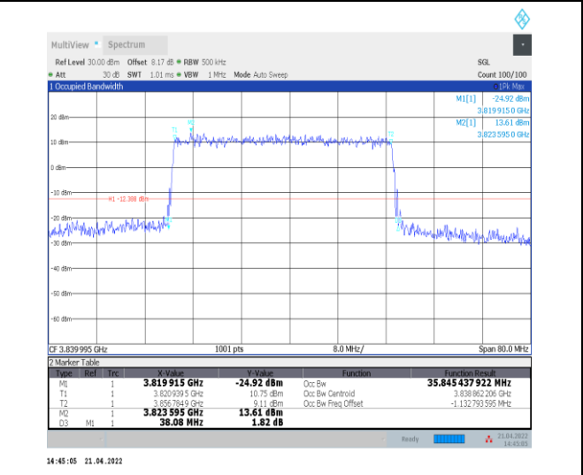
1-N77-3700-3980--30-40-M-3-DFT-16QAM-Outer_Full-100@0-Ant0-35.847-38.080-≤40-PASS
