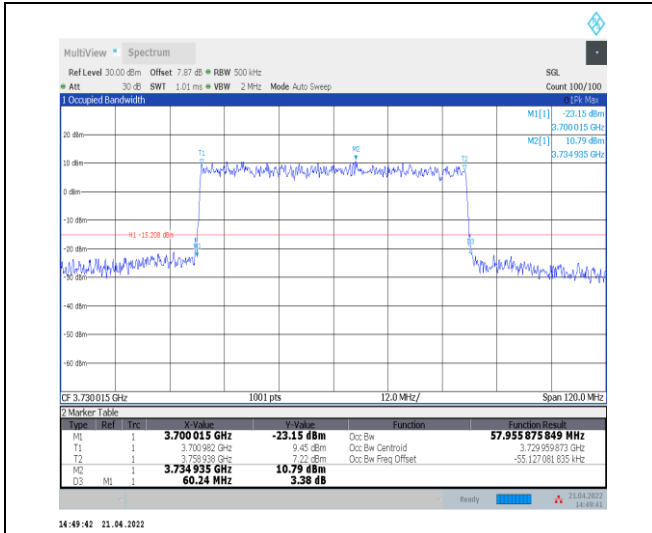
1-N77-3700-3980--30-60-L-7-CP-16QAM-Outer_Full -162@0-Ant0-57.956-60.240-≤60-PASS
