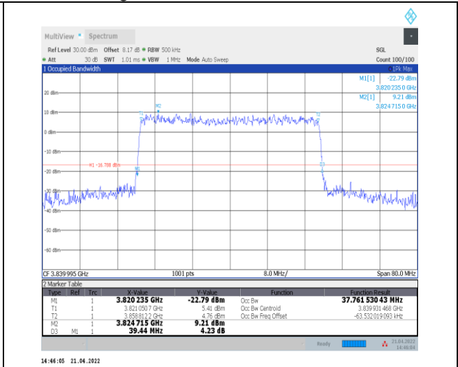
1-N77-3700-3980--30-40-M-9-CP-256QAM-Outer_Full-106@0-Ant0-37.71-39.440-≤40-PASS
