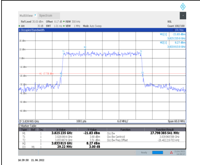
1-N77-3700-3980--30-30-M-9-CP-256QAM-Outer_Full I-78@0-Ant0-27.798-29.220-≤30-PASS
