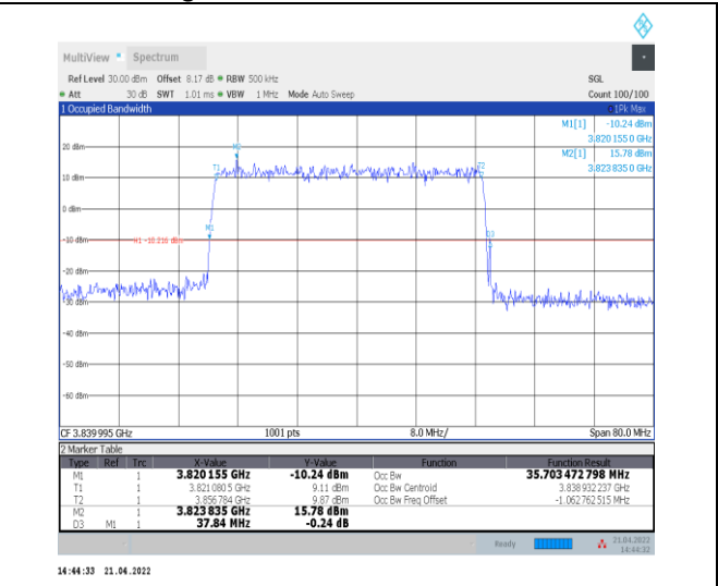
1-N77-3700-3980--30-40-M-1-DFT-QPSK-Outer_Full -100@0-Ant0-35.718-37.840-≤40-PASS
