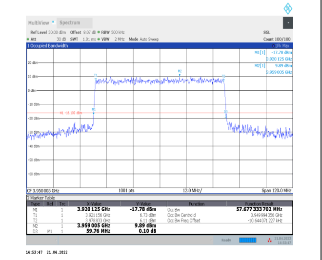
1-N77-3700-3980--30-60-H-8-CP-64QAM-Outer_Full-162@0-Ant0-57.677-59.760-≤60-PASS
