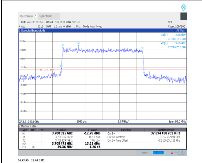
1-N77-3700-3980--30-40-L-7-CP-16QAM-Outer_Full-106@0-Ant0-37.895-39.360-<=40-PASS
