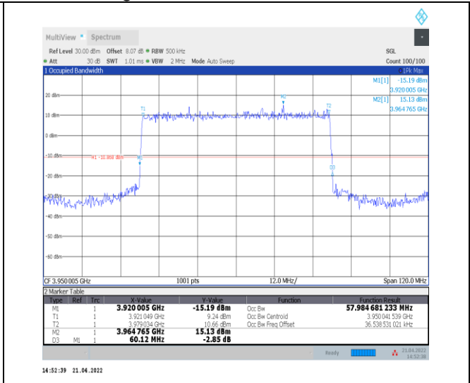
1-N77-3700-3980--30-60-H-2-DFT-PI2BPSK-Outer_Full Full-162@0-Ant0-57.985-60.120≤60-PASS
