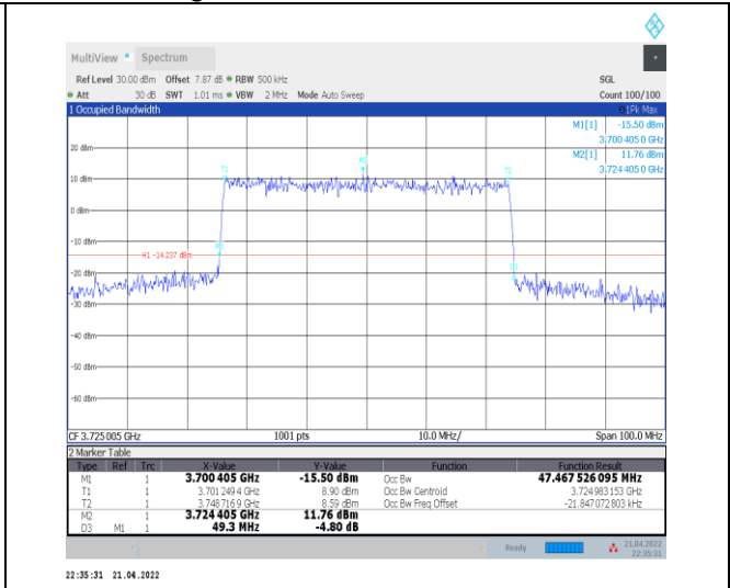
1-N77-3700-3980--30-50-L-7-CP-16QAM-Outer_Full-133@0-Ant0-47.468-49.300-<math>\leq 50</math>-PASS
