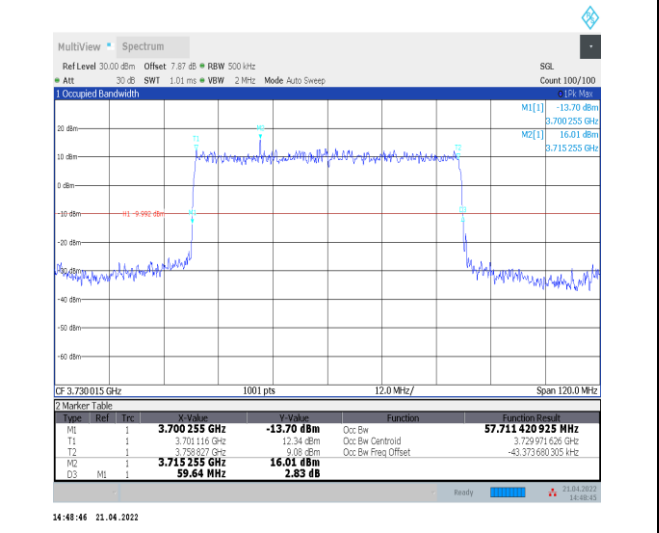
1-N77-3700-3980--30-60-L-2-DFT-PI2BPSK-Outer_F ull-162@0-Ant0-57.711-59.640-≤60-PASS
