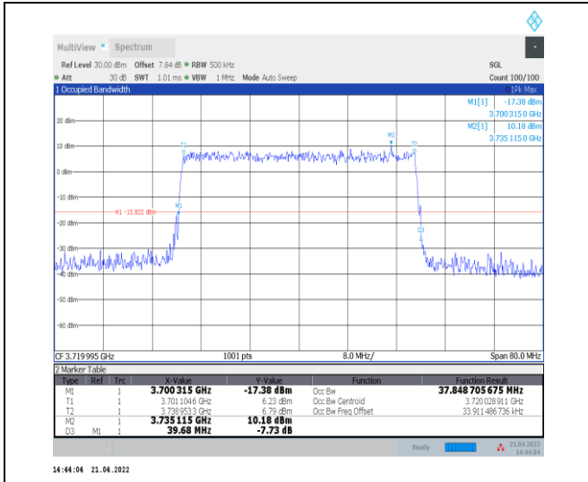
1-N77-3700-3980--30-40-L-9-CP-256QAM-Outer_Fu II-106@0-Ant0-37.853-39.680-≤40-PASS
