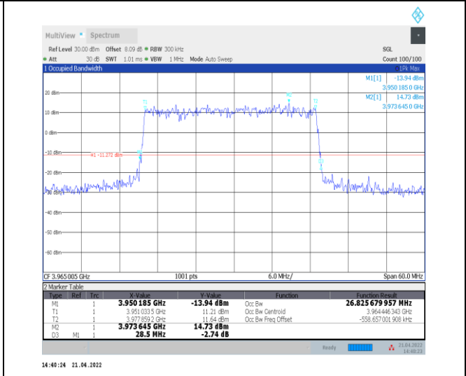
1-N77-3700-3980--30-30-H-1-DFT-QPSK-Outer_Full -75@0-Ant0-26.826-28.500-≤30-PASS
