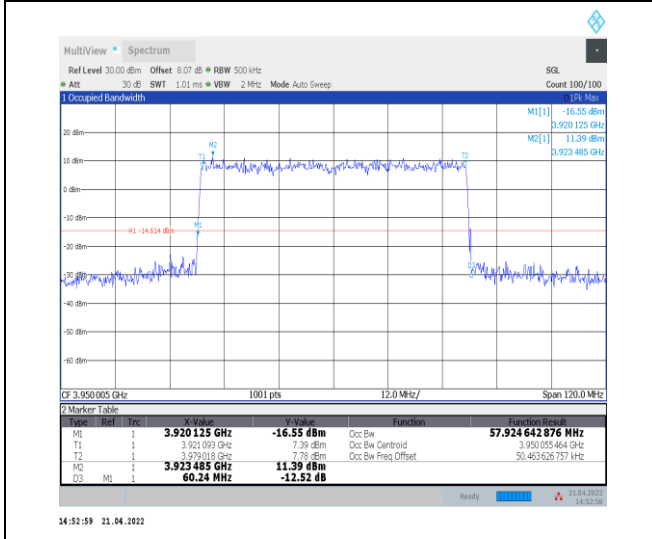
1-N77-3700-3980--30-60-H-3-DFT-16QAM-Outer_Full ull-162@0-Ant0-57.925-60.240≤60-PASS
