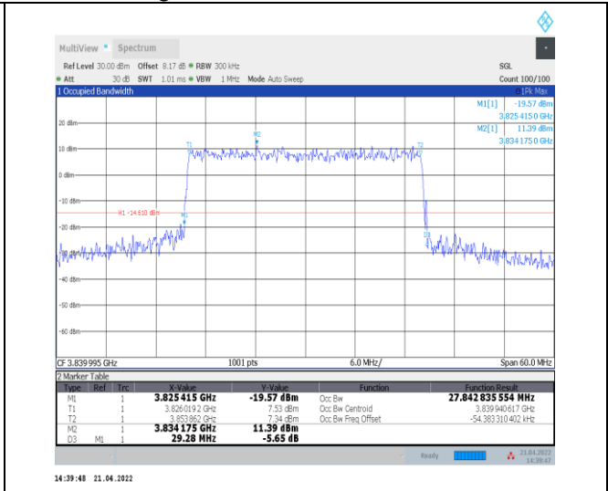
1-N77-3700-3980--30-30-M-8-CP-64QAM-Outer_Full -78@0-Ant0-27.843-29.280-≤30-PASS
