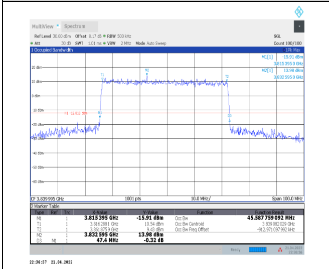
1-N77-3700-3980--30-50-M-3-DFT-16QAM-Outer_Full Full-128@0-Ant0-45.588-47.400-≤50-PASS
