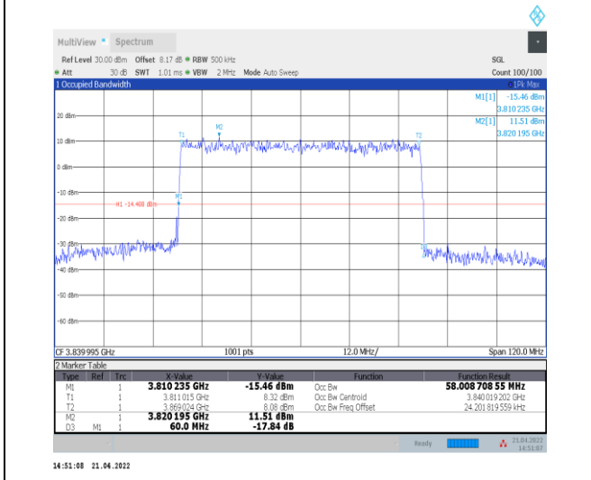
1-N77-3700-3980--30-60-M-4-DFT-64QAM-Outer_Full-162@0-Ant0-58.009-60.000-≤60-PASS
