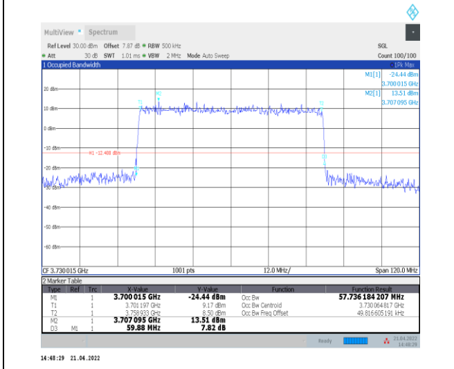
1-N77-3700-3980--30-60-L-1-DFT-QPSK-Outer_Full -162@0-Ant0-57.736-59.880-≤60-PASS
