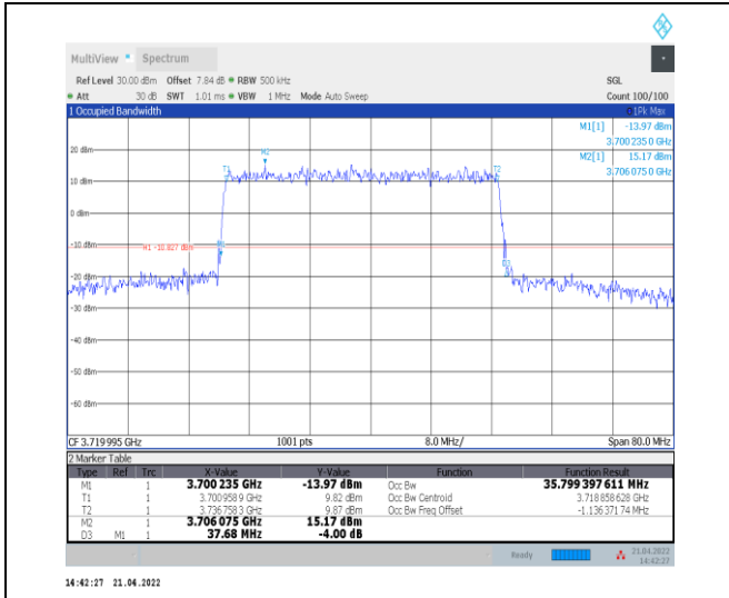
1-N77-3700-3980--30-40-L-1-DFT-QPSK-Outer_Full -100@0-Ant0-35.818-37.680-≤40-PASS
