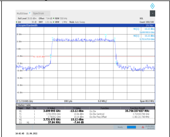
1-N77-3700-3980--30-40-L-2-DFT-PI2BPSK-Outer_Full -100@0-Ant0-35.776-37.840-≤40-PASS
