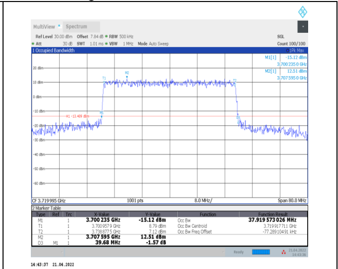
1-N77-3700-3980--30-40-L-6-CP-QPSK-Outer_Full-106@0-Ant0-37.912-39.680-<=40-PASS
