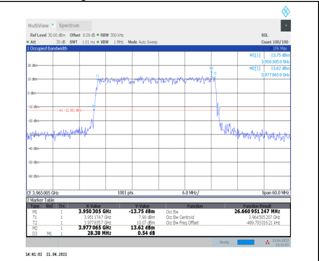
1-N77-3700-3980--30-30-H-3-DFT-16QAM-Outer_Fu II-75@0-Ant0-26.665-28.380-≤30-PASS
