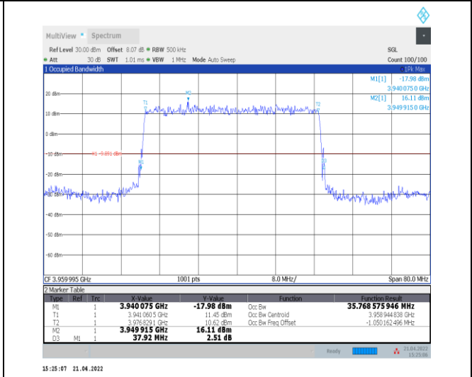
1-N77-3700-3980--30-40-H-2-DFT-PI2BPSK-Outer_Full-100@0-Ant0-35.784-37.920-≤40-PASS
