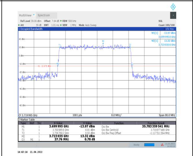
1-N77-3700-3980--30-40-L-4-DFT-64QAM-Outer_Full -100@0-Ant0-35.791-37.760-≤40-PASS
