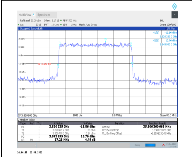
1-N77-3700-3980--30-40-M-2-DFT-PI2BPSK-Outer_Full-100@0-Ant0-35.824-37.280-≤40-PASS
