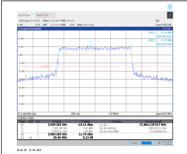
1-N77-3700-3980--30-30-H-6-CP-QPSK-Outer_Full-78@0-Ant0-27.806-29.460-≤30-PASS
