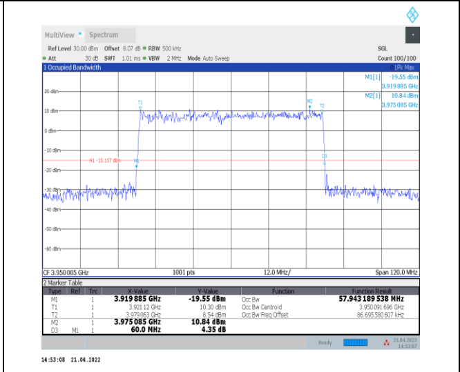
1-N77-3700-3980--30-60-H-4-DFT-64QAM-Outer_Full ll-162@0-Ant0-57.943-60.000≤60-PASS
