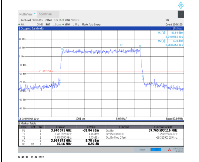
1-N77-3700-3980--30-40-H-9-CP-256QAM-Outer_Full -106@0-Ant0-37.692-40.160≤40-PASS
