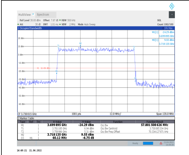
1-N77-3700-3980--30-60-L-5-DFT-256QAM-Outer_Full-162@0-Ant0-57.802-60.120-≤60-PASS
