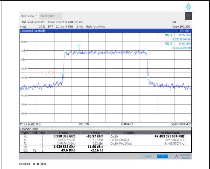
1-N77-3700-3980--30-50-H-7-CP-16QAM-Outer_Full-133@0-Ant0-47.484-49.600-≤50-PASS
