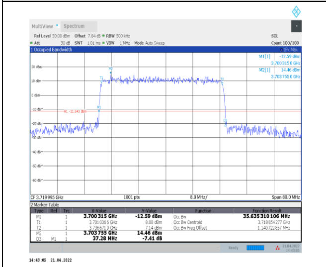
1-N77-3700-3980--30-40-L-3-DFT-16QAM-Outer_Full -100@0-Ant0-35.643-37.280-≤40-PASS
