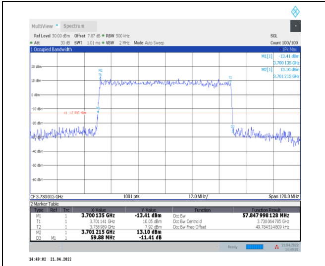
1-N77-3700-3980--30-60-L-3-DFT-16QAM-Outer_Fu II-162@0-Ant0-57.848-59.880-≤60-PASS
