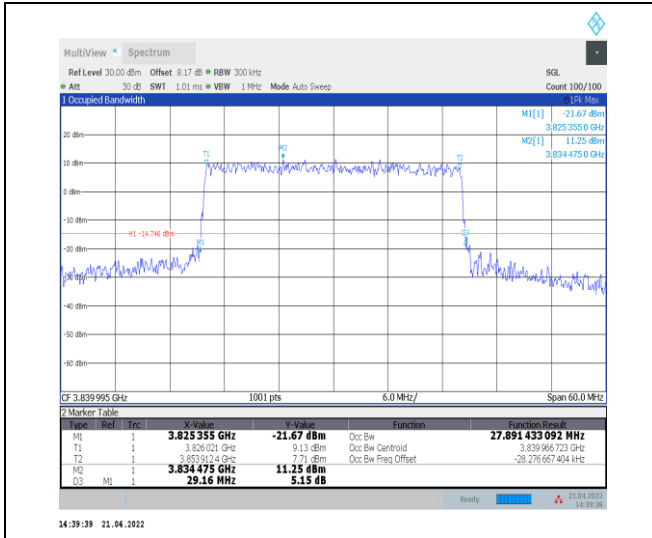
1-N77-3700-3980--30-30-M-7-CP-16QAM-Outer_Full I-78@0-Ant0-27.893-29.160-≤30-PASS
