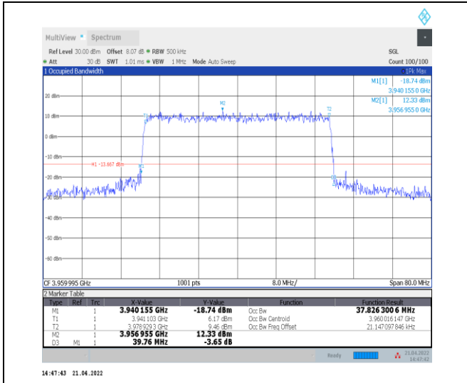
1-N77-3700-3980--30-40-H-7-CP-16QAM-Outer_Full -106@0-Ant0-37.823-39.760≤40-PASS
