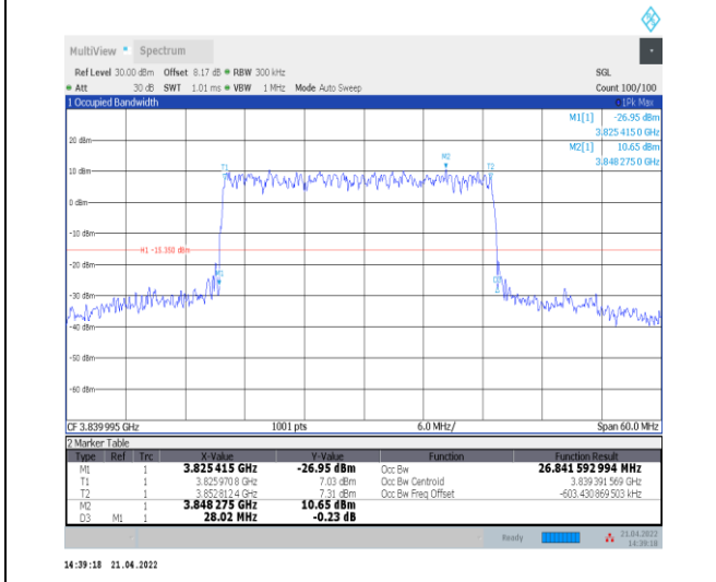
1-N77-3700-3980--30-30-M-5-DFT-256QAM-Outer_Full-75@0-Ant0-26.842-28.020-≤30-PASS
