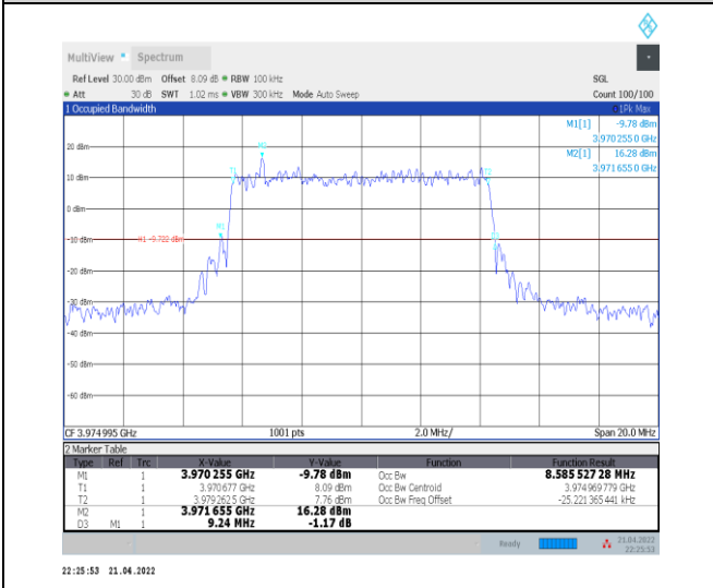
1-N77-3700-3980--30-10-H-1-DFT-QPSK-Outer_Full -24@0-Ant0-8.586-9.240-≤10-PASS
