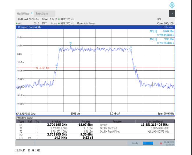
1-N77-3700-3980--30-15-L-9-CP-256QAM-Outer_Full-38@0-Ant0-13.551-14.700-≤15-PASS
