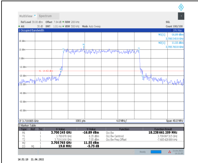
1-N77-3700-3980--30-20-L-7-CP-16QAM-Outer_Full -51@0-Ant0-18.239-19.800-<=20-PASS
