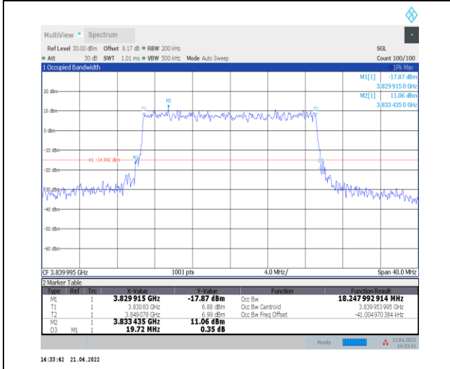
1-N77-3700-3980--30-20-M-8-CP-64QAM-Outer_Full-51@0-Ant0-18.248-19.720-≤20-PASS
