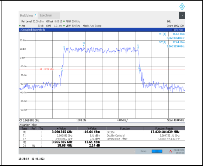
1-N77-3700-3980--30-20-H-4-DFT-64QAM-Outer_Full Full-50@0-Ant0-17.82-18.680-≤20-PASS
