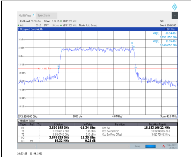
1-N77-3700-3980--30-20-M-6-CP-QPSK-Outer_Full-51@0-Ant0-18.153-19.320-≤20-PASS
