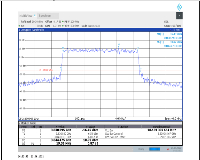
1-N77-3700-3980--30-20-M-7-CP-16QAM-Outer_Full-51@0-Ant0-18.191-19.360-≤20-PASS
