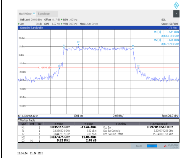
1-N77-3700-3980--30-10-M-6-CP-QPSK-Outer_Full-24@0-Ant0-8.598-9.820-≤10-PASS
