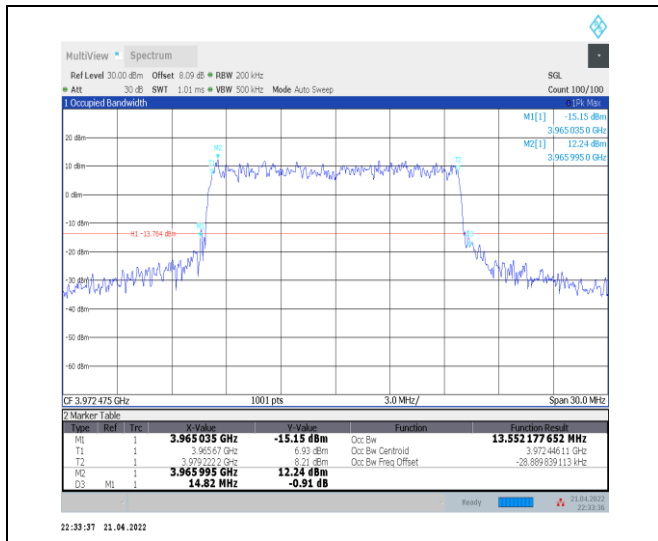
1-N77-3700-3980--30-15-H-8-CP-64QAM-Outer_Full -38@0-Ant0-13.552-14.820≤15-PASS
