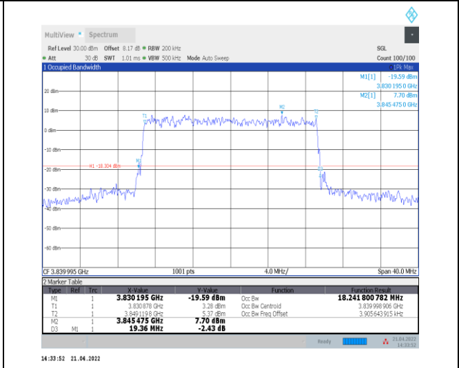
1-N77-3700-3980--30-20-M-9-CP-256QAM-Outer_Full-51@0-Ant0-18.242-19.360-≤20-PASS
