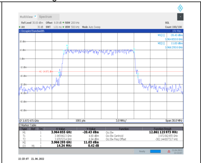
1-N77-3700-3980--30-15-H-5-DFT-256QAM-Outer_Full-36@0-Ant0-12.861-14.340-≤15-PASS
