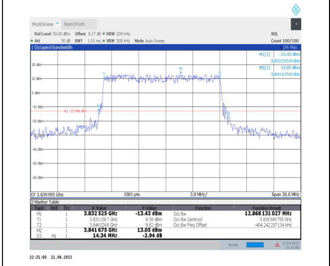
1-N77-3700-3980--30-15-M-4-DFT-64QAM-Outer_Full ll-36@0-Ant0-12.868-14.340≤15-PASS
