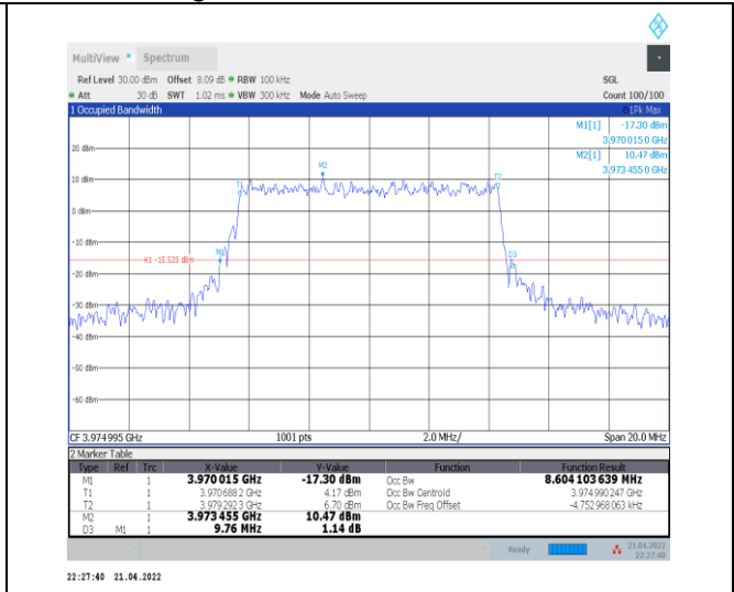
1-N77-3700-3980--30-10-H-8-CP-64QAM-Outer_Full -24@0-Ant0-8.604-9.760-≤10-PASS
