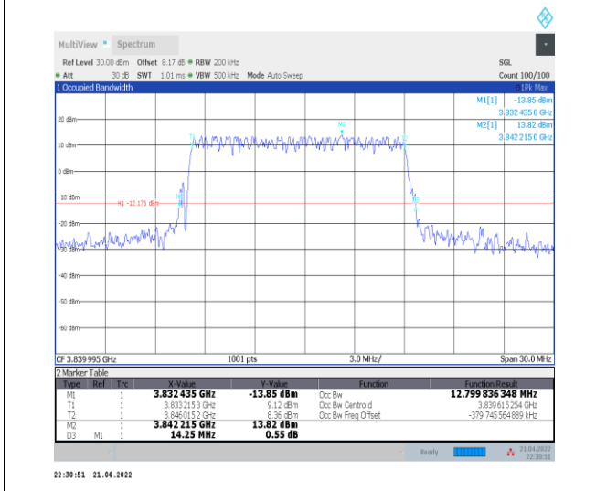
1-N77-3700-3980--30-15-M-3-DFT-16QAM-Outer_Full ull-36@0-Ant0-12.8-14.250≤15-PASS
