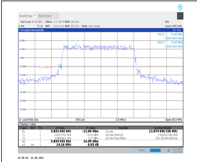
1-N77-3700-3980--30-15-M-1-DFT-QPSK-Outer_Full -36@0-Ant0-12.875-14.160≤15-PASS
