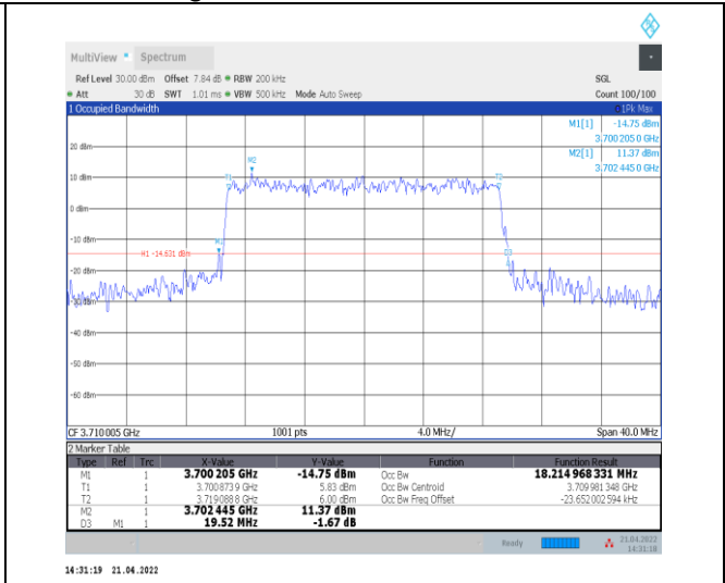
1-N77-3700-3980--30-20-L-8-CP-64QAM-Outer_Full -51@0-Ant0-18.215-19.520-<=20-PASS
