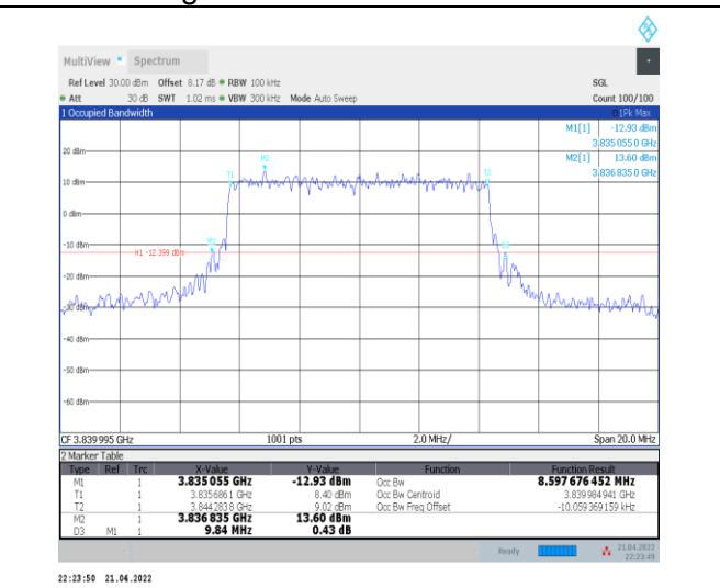
1-N77-3700-3980--30-10-M-1-DFT-QPSK-Outer_Full -24@0-Ant0-8.598-9.840-<=10-PASS
