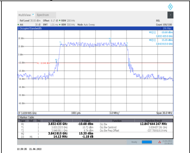
1-N77-3700-3980--30-15-M-2-DFT-PI2BPSK-Outer_Full Full-36@0-Ant0-12.848-14.130≤15-PASS
