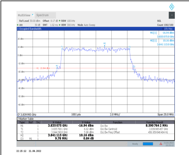
1-N77-3700-3980--30-10-M-8-CP-64QAM-Outer_Ful I-24@0-Ant0-8.591-9.780-≤10-PASS
