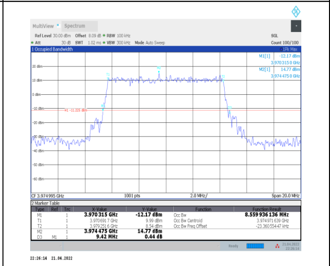
1-N77-3700-3980--30-10-H-2-DFT-PI2BPSK-Outer_ Full-24@0-Ant0-8.56-9.420-≤10-PASS
