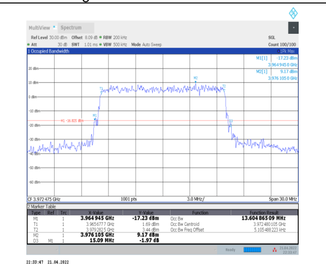
1-N77-3700-3980--30-15-H-9-CP-256QAM-Outer_Fu II-38@0-Ant0-13.605-15.090≤15-PASS
