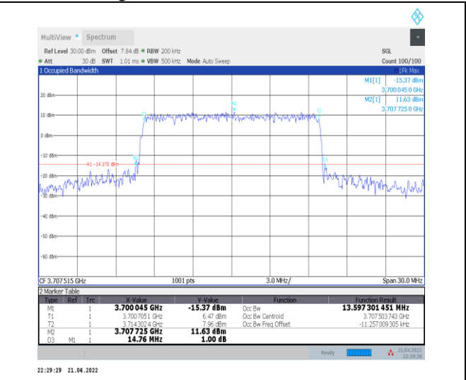
1-N77-3700-3980--30-15-L-7-CP-16QAM-Outer_Full-38@0-Ant0-13.597-14.760-≤15-PASS
