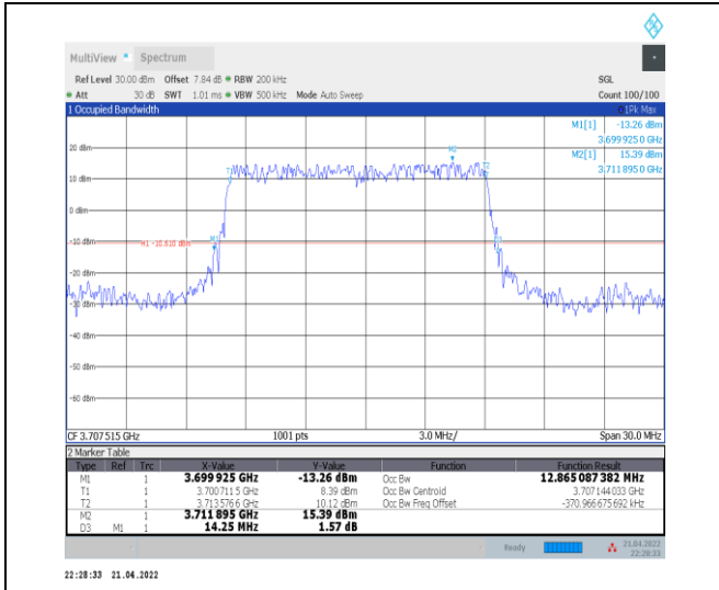
1-N77-3700-3980--30-15-L-2-DFT-PI2BPSK-Outer_Full-36@0-Ant0-12.865-14.250-≤15-PASS
