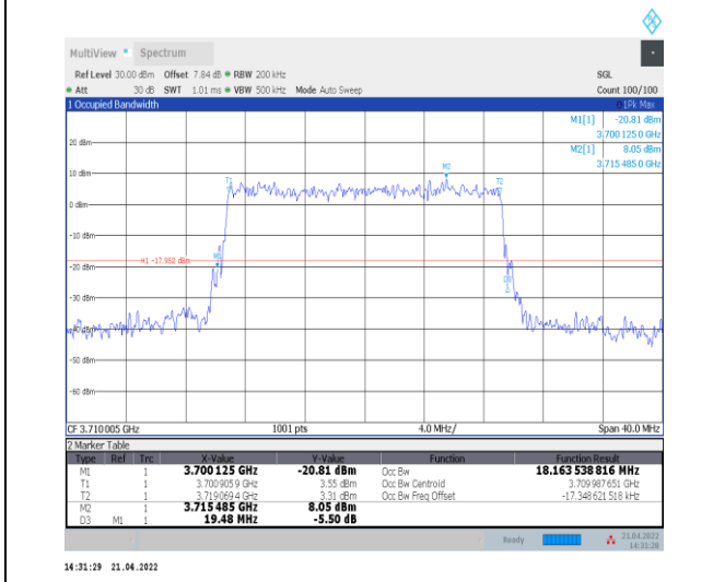
1-N77-3700-3980--30-20-L-9-CP-256QAM-Outer_Fu ll-51@0-Ant0-18.164-19.480-<=20-PASS
