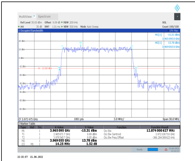
1-N77-3700-3980--30-15-H-4-DFT-64QAM-Outer_Full-36@0-Ant0-12.874-14.250-≤15-PASS
