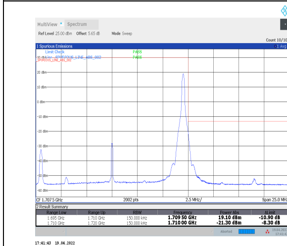
1-N70--15-15-H-5-CP-QPSK-Edge_1RB_Right-1@78-Ant2-seegraph-PASS-see graph
