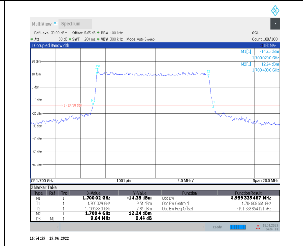
1-N70--15-10-H-3-DFT-16QAM-Outer_Full-50@0-Ant t2-8.959-9.640-<=10-PASS
