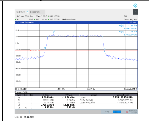
1-N70--15-10-H-1-DFT-QPSK-Outer_Full-50@0-Ant 2-8.958-9.720-<=10-PASS
