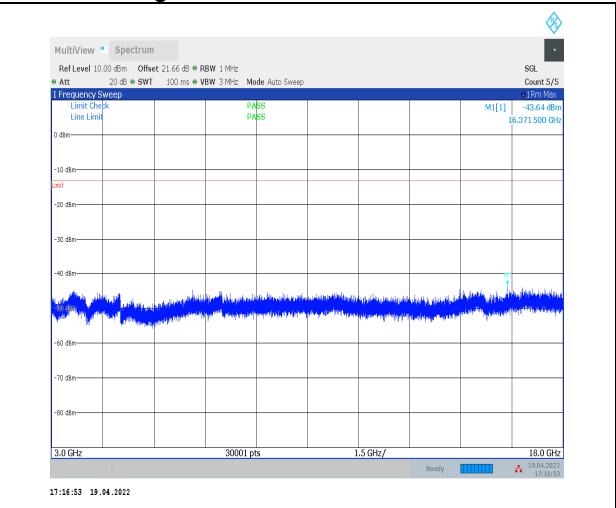
1-N70--15-15-M-1-DFT-PI2BPSK-Inner_1RB_Left-1 @1-3000-18000-Ant2--43.64--13-PASS
