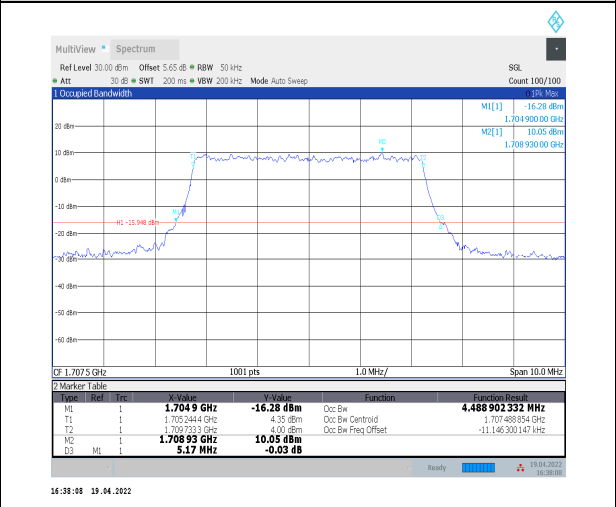
1-N70--15-5-H-6-CP-QPSK-Outer_Full-25@0-Ant2-4 .489-5.170-<math>\leq</math>5-PASS
