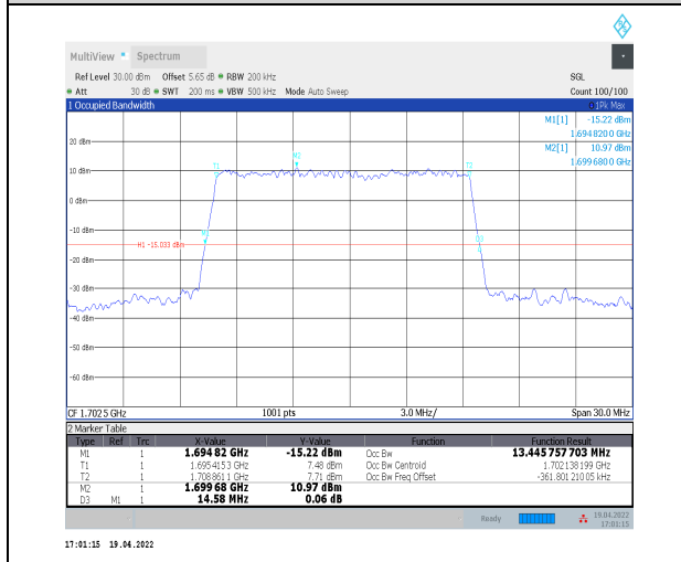
1-N70--15-15-L-5-DFT-256QAM-Outer_Full-75@0-A nt2-13.446-14.580-≤15-PASS
