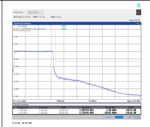
1-N70--15-5-H-6-CP-QPSK-Outer_Full-25@0-Ant2-seegraph-PASS-see graph
