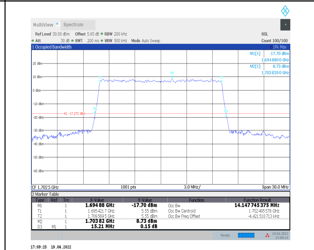
1-N70--15-15-M-9-CP-256QAM-Outer_Full-79@0-Ant 2-14.148-15.210-≤15-PASS
