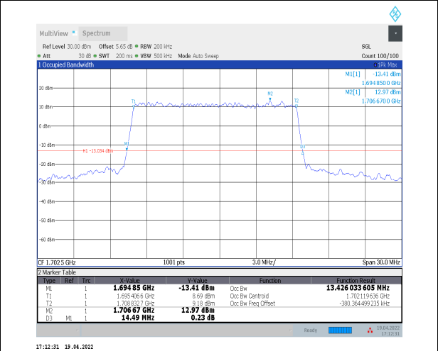
1-N70--15-15-H-4-DFT-64QAM-Outer_Full-75@0-An t2-13.426-14.490≤15-PASS
