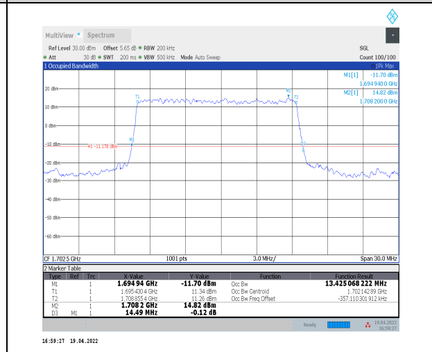
1-N70--15-15-L-2-DFT-PI2BPSK-Outer_Full-75@0-A nt2-13.425-14.490-≤15-PASS
