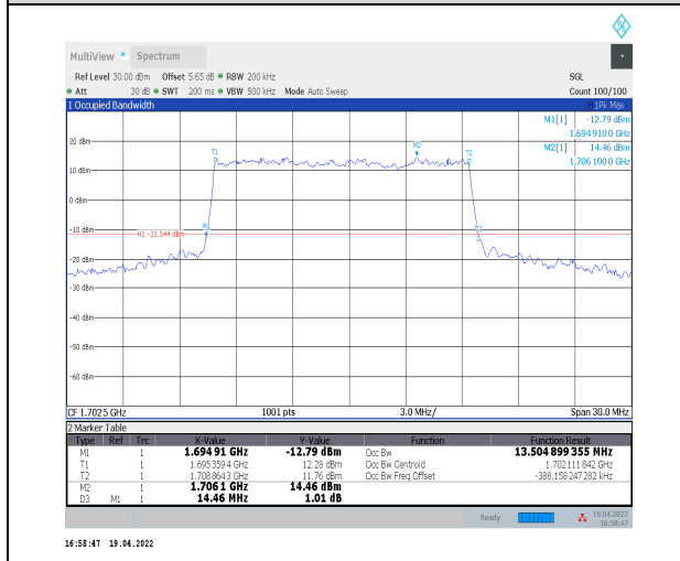
1-N70--15-15-L-1-DFT-QPSK-Outer_Full-75@0-Ant2 -13.505-14.460-≤15-PASS
