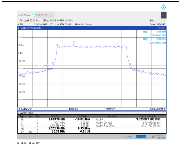
1-N70--15-10-H-8-CP-64QAM-Outer_Full-52@0-Ant 2-9.326-10.320-≤10-PASS
