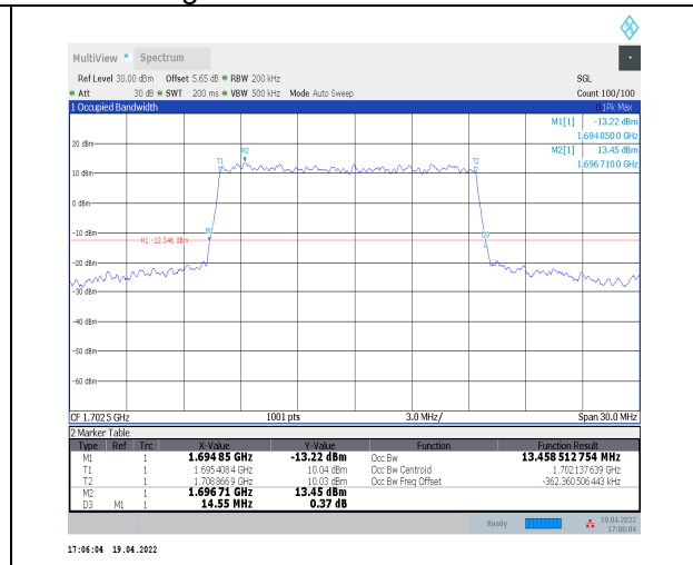
1-N70--15-15-M-3-DFT-16QAM-Outer_Full-75@0-Ant2-13.459-14.550-≤15-PASS
