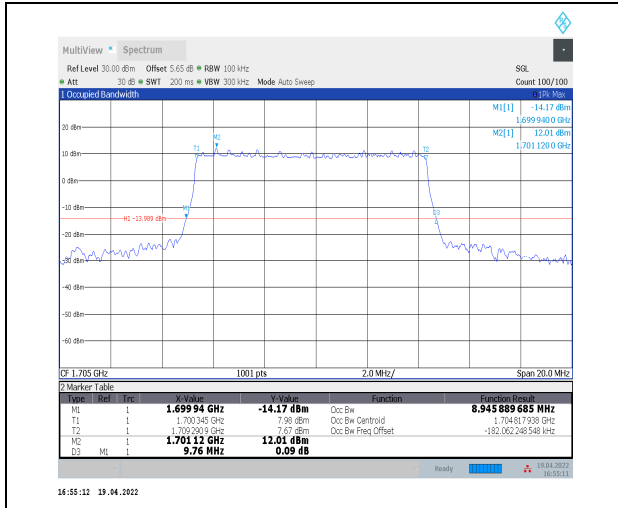
1-N70--15-10-H-4-DFT-64QAM-Outer_Full-50@0-Ant t2-8.946-9.760-≤10-PASS
