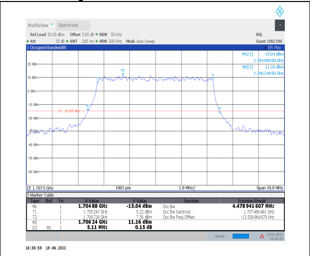
1-N70--15-5-H-4-DFT-64QAM-Outer_Full-25@0-Ant 2-4.479-5.110-<math>\leq</math>5-PASS
