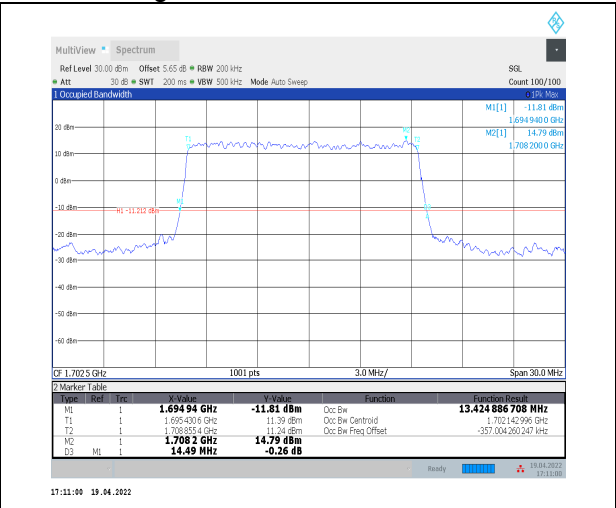
1-N70--15-15-H-2-DFT-PI2BPSK-Outer_Full-75@0-Ant 2-13.425-14.490≤15-PASS
