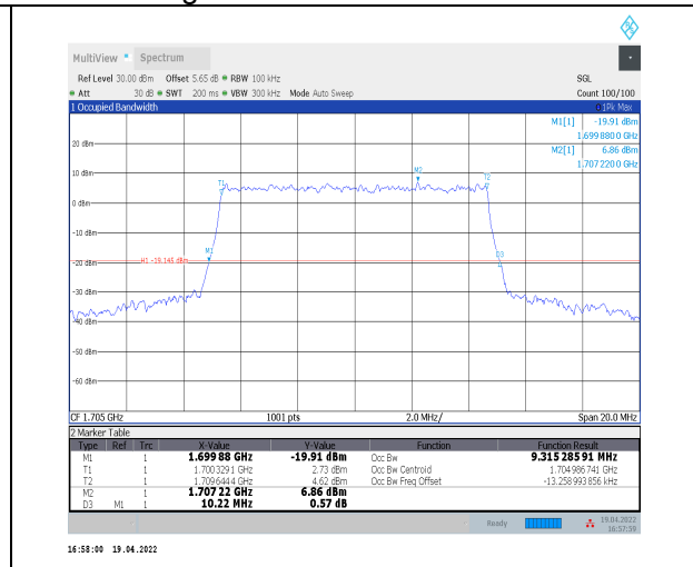
1-N70--15-10-H-9-CP-256QAM-Outer_Full-52@0-An t2-9.315-10.220-≤10-PASS
