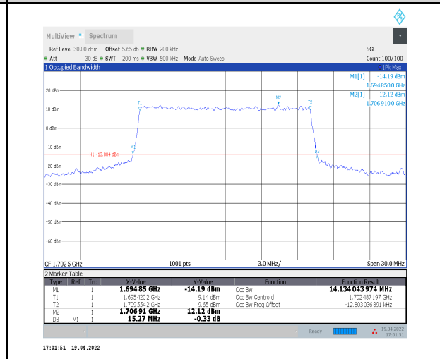
1-N70--15-15-L-6-CP-QPSK-Outer_Full-79@0-Ant2- 14.134-15.270-≤15-PASS
