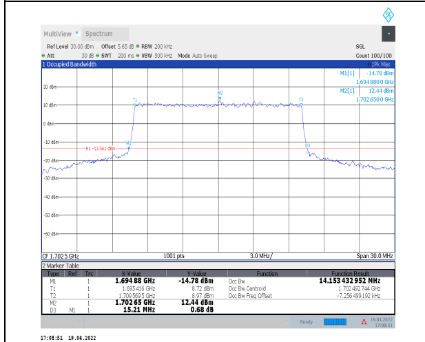
1-N70--15-15-M-8-CP-64QAM-Outer_Full-79@0-Ant 2-14.153-15.210-≤15-PASS
