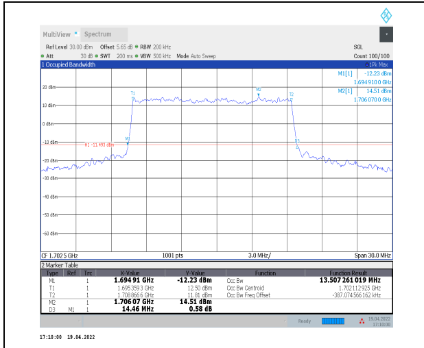
1-N70--15-15-H-1-DFT-QPSK-Outer_Full-75@0-Ant 2-13.507-14.460≤15-PASS
