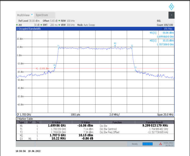
1-N70--15-10-H-7-CP-16QAM-Outer_Full-52@0-Ant 2-9.299-10.220-≤10-PASS
