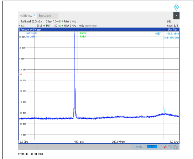
1-N70--15-15-M-1-DFT-PI2BPSK-Inner_1RB_Left-1 @1-1000-3000-Ant2--49.31--13-PASS
