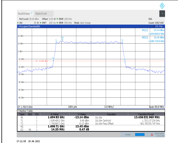
1-N70--15-15-H-3-DFT-16QAM-Outer_Full-75@0-An t2-13.456-14.550≤15-PASS
