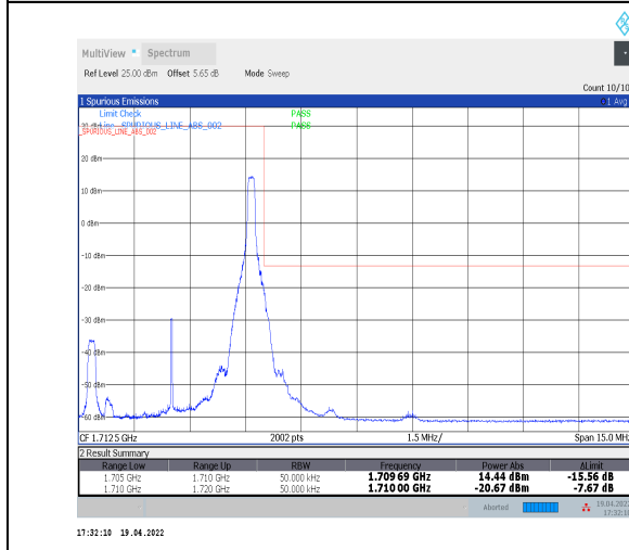
1-N70--15-5-H-5-CP-QPSK-Edge_1RB_Right-1@24-Ant2-seegraph-PASS-see graph
