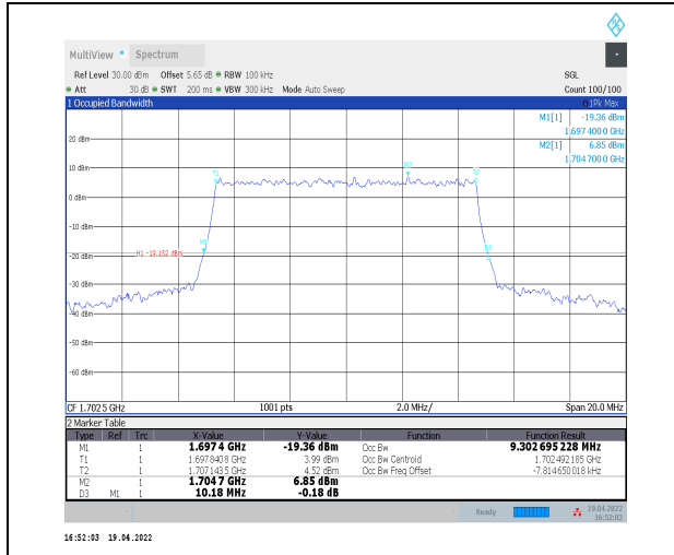
1-N70--15-10-M-9-CP-256QAM-Outer_Full-52@0-An t2-9.303-10.180-<=10-PASS
