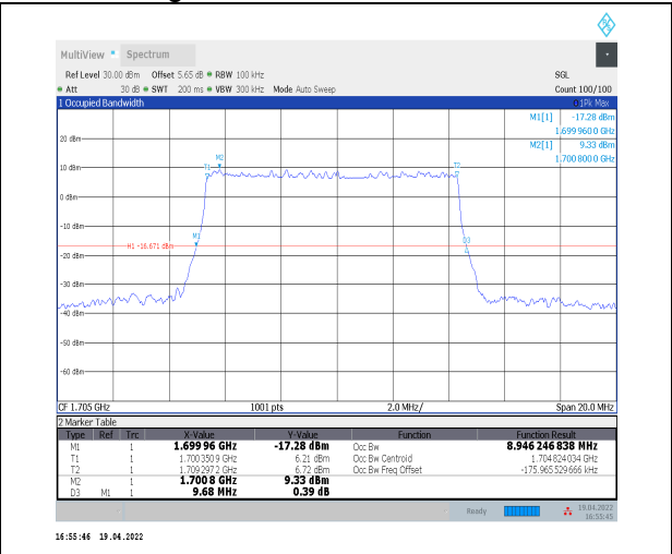
1-N70--15-10-H-5-DFT-256QAM-Outer_Full-50@0-Ant t2-8.946-9.680-≤10-PASS
