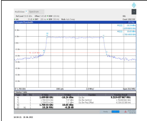
1-N70--15-10-H-6-CP-QPSK-Outer_Full-52@0-Ant2- 9.319-10.260-≤10-PASS
