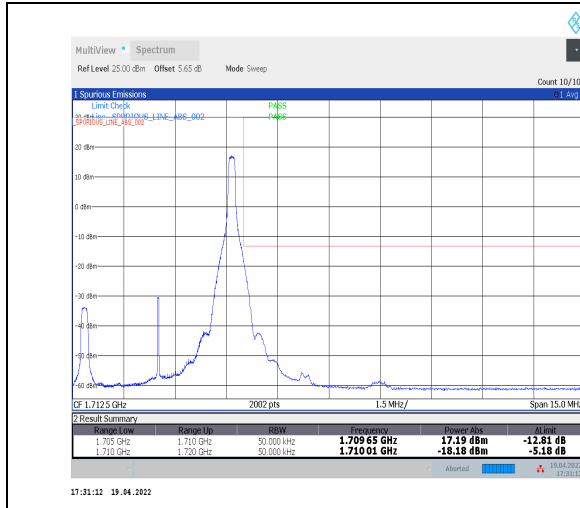
1-N70--15-5-H-2-DFT-PI2BPSK-Edge_1RB_Right-1@24-Ant2-seegraph-PASS-see graph
